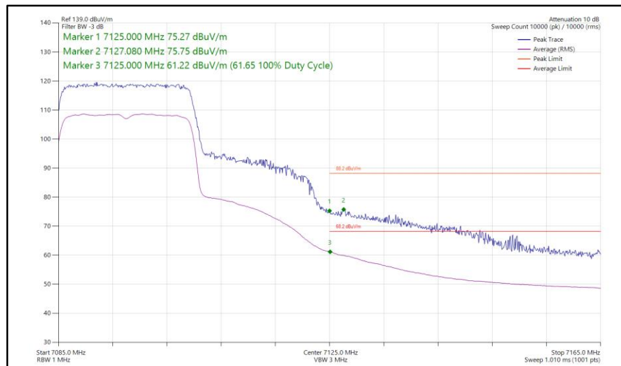
Figure 114 - 802.11ax HE20, SU, SDM, Core 0 - Core 1 - 7095 MHz Band Edge Frequency 7125 MHz
