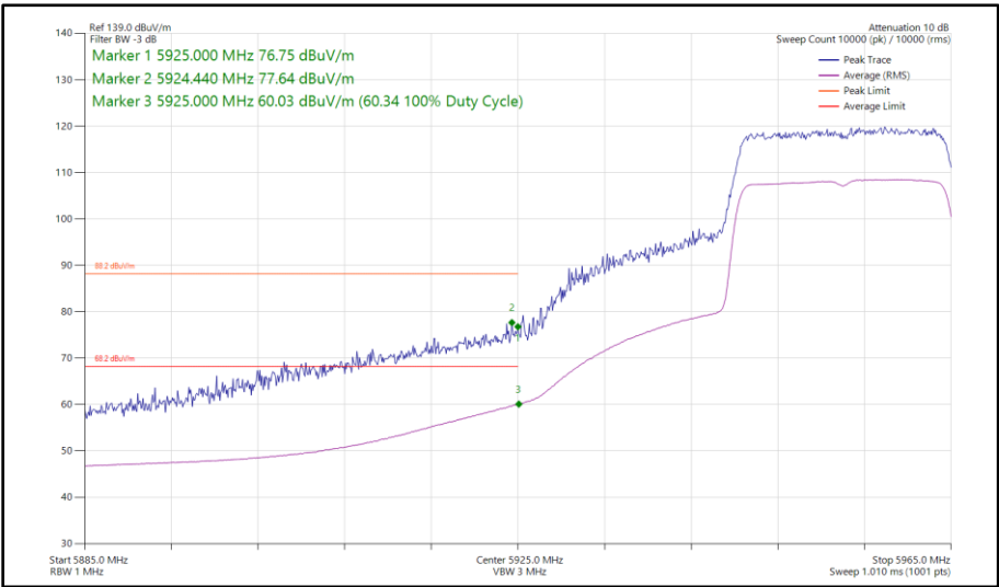
Figure 117 - 802.11ax HE20, SU, TxBF, Core 0 - Core 1 - 5955 MHz Band Edge Frequency 5925 MHz
