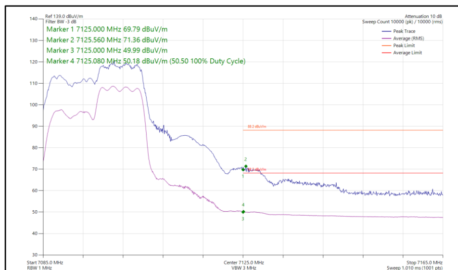
Figure 115 - 802.11ax HE20, RU 106-54, SDM, Core 0 - Core 1 - 7095 MHz Band Edge Frequency 7125 MHz
