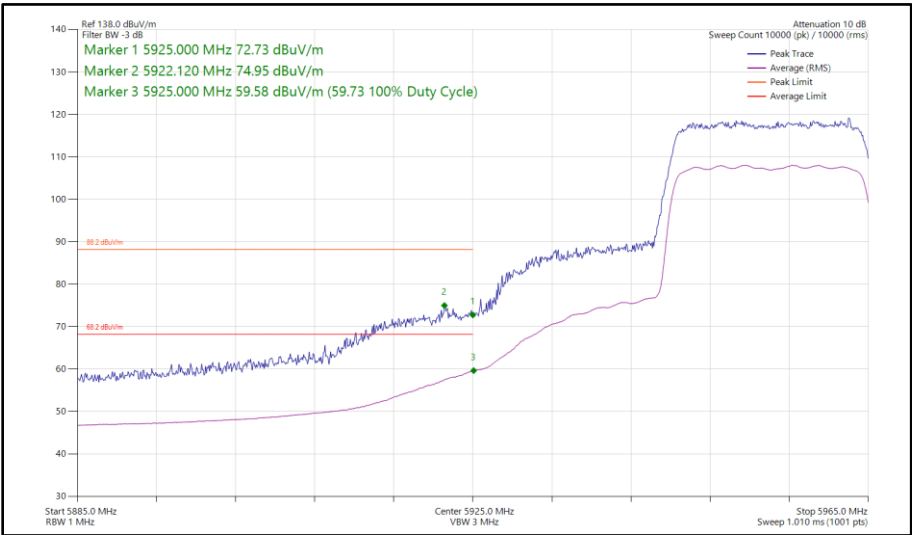
Figure 106 - 802.11ax HE20, SU, CDD, Core 0 - Core 1 - 5955 MHz Band Edge Frequency 5925 MHz
