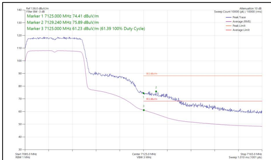
Figure 103 - 802.11ax HE20, SU, SISO, Core 1 - 7095 MHz Band Edge Frequency 7125 MHz
