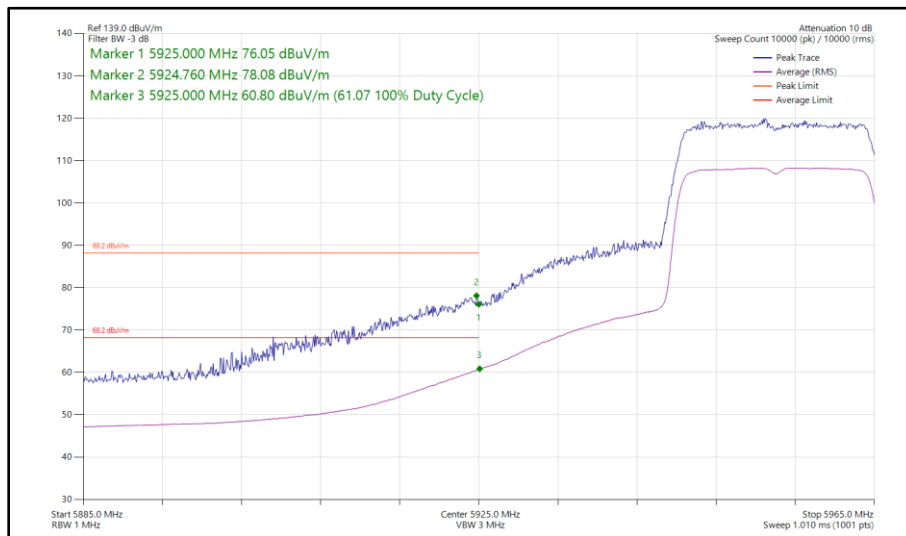
Figure 99 - 802.11ax HE20, SU, SISO, Core 1 - 5955 MHz Band Edge Frequency 5925 MHz
