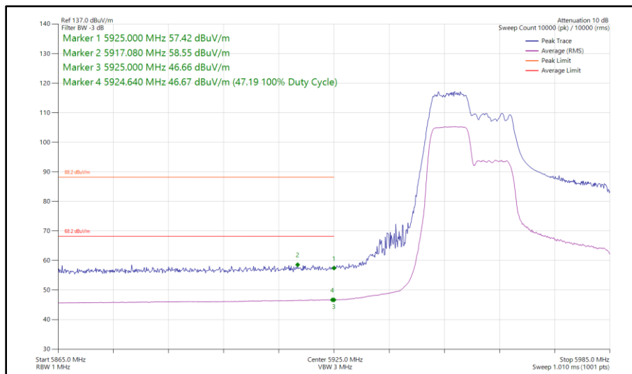
Figure 125 - 802.11ax HE40, RU 106-53, SISO, Core 1 - 5965 MHz Band Edge Frequency 5925 MHz
