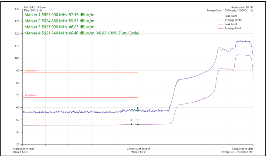
Figure 121 - 802.11ax HE40, RU 106-56, SISO, Core 0 - 5965 MHz Band Edge Frequency 5925 MHz
