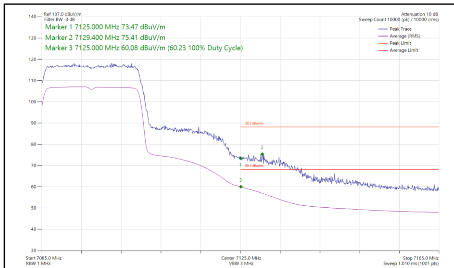
Figure 95 - 802.11ax HE20, SU, SISO, Core 0 - 7095 MHz Band Edge Frequency 7125 MHz
