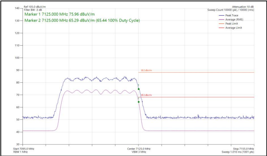
Figure 110 - 802.11ax HE20, SU, CDD, Core 0 - Core 1 - 7115 MHz Band Edge Frequency 7125 MHz
