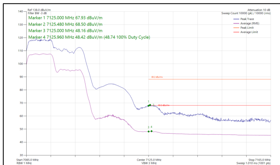
Figure 109 - 802.11ax HE20, RU 106-53, CDD, Core 0 - Core 1 - 7095 MHz Band Edge Frequency 7125 MHz
