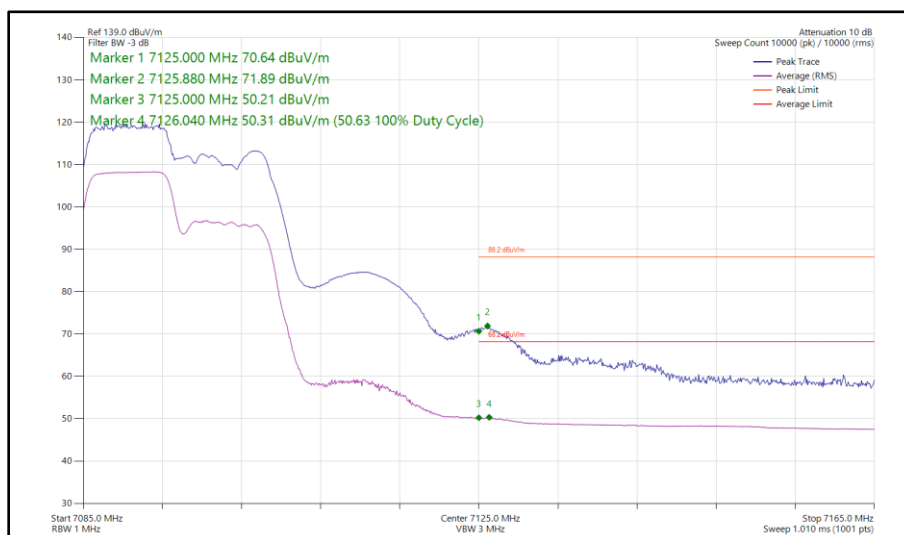
Figure 104 - 802.11ax HE20, RU 106-53, SISO, Core 1 - 7095 MHz Band Edge Frequency 7125 MHz
