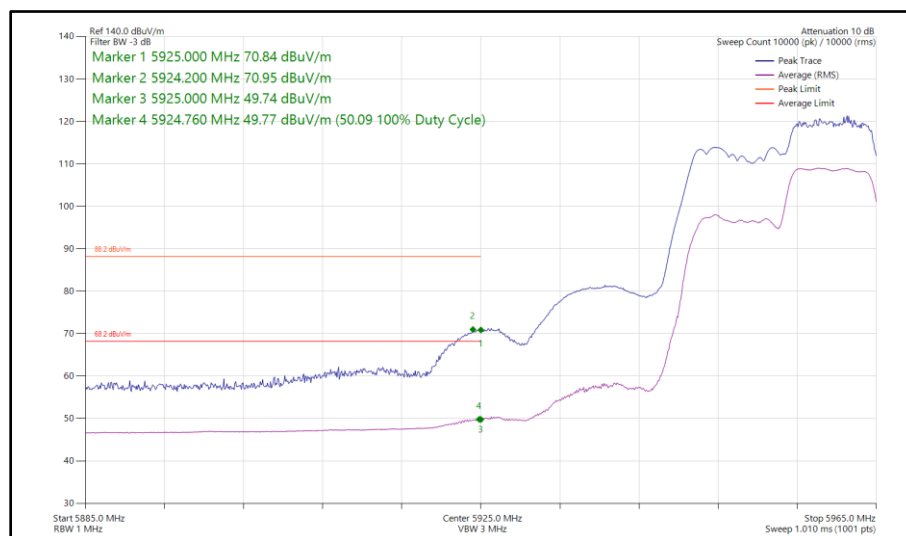
Figure 113 - 802.11ax HE20, RU 106-54, SDM, Core 0 - Core 1 - 5955 MHz Band Edge Frequency 5925 MHz
