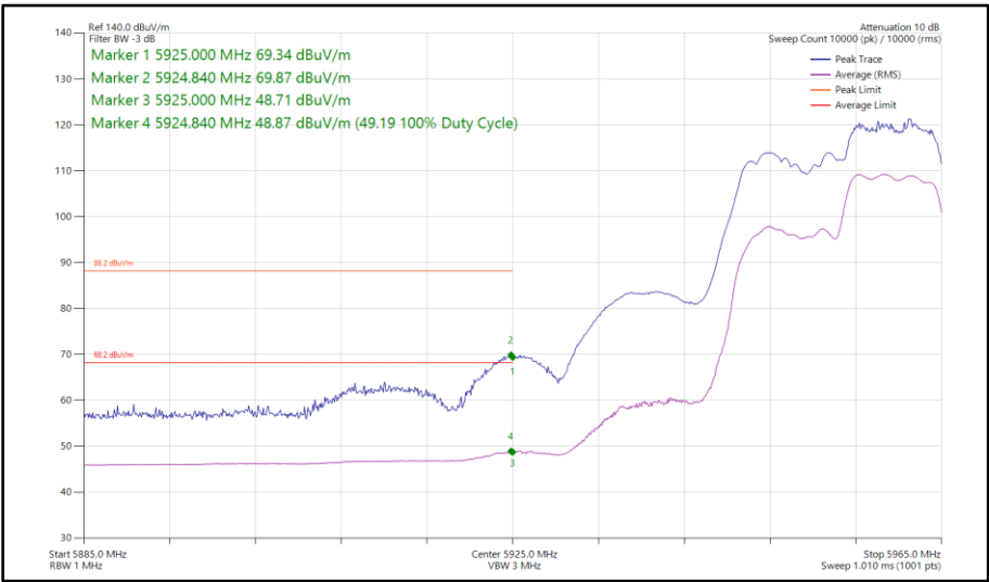
Figure 107 - 802.11ax HE20, RU 106-54, CDD, Core 0 - Core 1 - 5955 MHz Band Edge Frequency 5925 MHz
