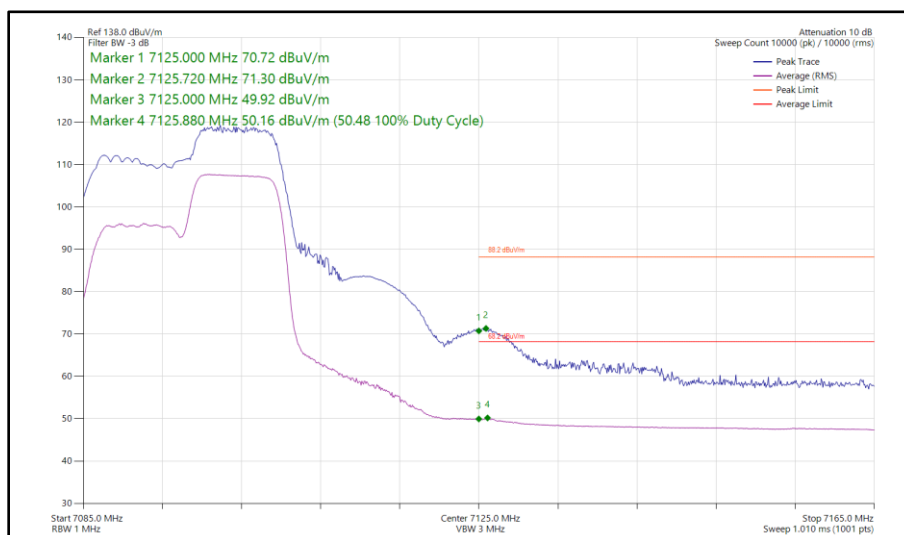
Figure 96 - 802.11ax HE20, RU 106-54, SISO, Core 0 - 7095 MHz Band Edge Frequency 7125 MHz
