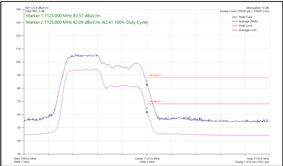
Figure 111 - 802.11ax HE20, RU 106-53, CDD, Core 0 - Core 1 - 7115 MHz Band Edge Frequency 7125 MHz
