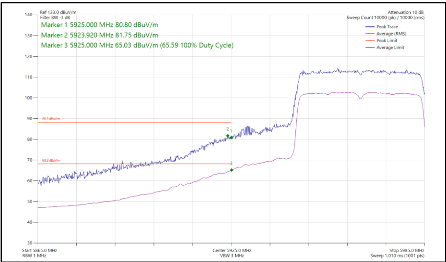
Figure 120 - 802.11ax HE40, SU, SISO, Core 0 - 5965 MHz Band Edge Frequency 5925 MHz
