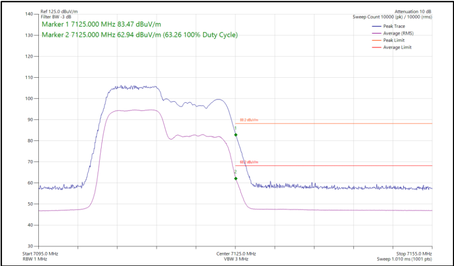
Figure 116 - 802.11ax HE20, RU 106-53, SDM, Core 0 - Core 1 - 7115 MHz Band Edge Frequency 7125 MHz
