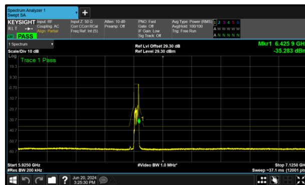
Figure 309 - B (Core 1) 802.11ax HE20 RU26 SP 6415 MHz (CH93)
