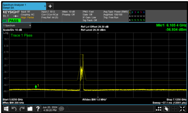
Figure 328 - B (Core 1) 802.11ax HE20 RU26 SP 6415 MHz (CH93)
