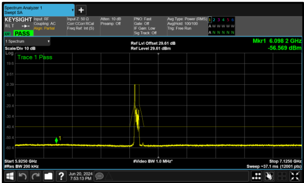
Figure 345 - B (Core 1) 802.11ax HE20 RU26 SP 6435 MHz (CH97)
