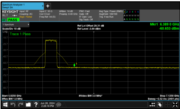
Figure 331 - B (Core 1) 802.11ax HE80 SU VLP 6225 MHz (CH55)
