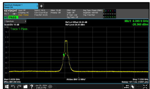
Figure 304 - B (Core 1) 802.11ax HE20 SU SP 6415 MHz (CH93)
