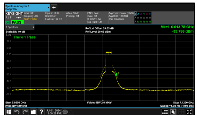
Figure 341 - B (Core 1) 802.11ax HE40 SU SP 6565 MHz (CH123)
