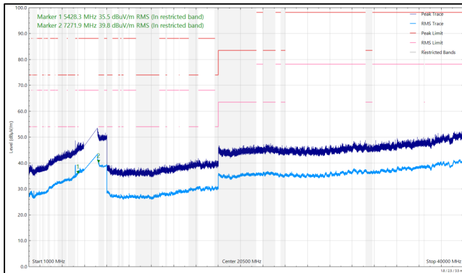
Figure 287 - U-NII-8 - 6895 MHz (CH189), HE20, SU, CDD, Core 0 + Core 1, 1 GHz to 40 GHz, Horizontal
