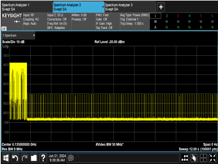
Figure 349 - U-NII-5, Minimum Bandwidth (AWGN Mid)
