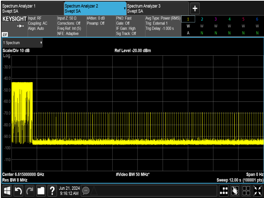
Figure 356 - U-NII-7, Minimum Bandwidth (AWGN Low)
