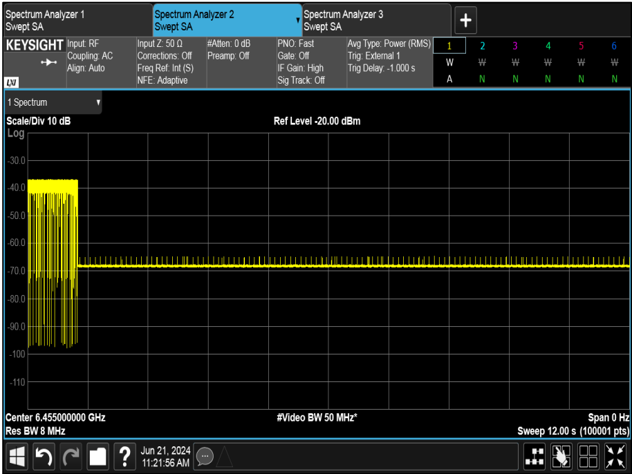
Figure 351 - U-NII-6, Minimum Bandwidth
