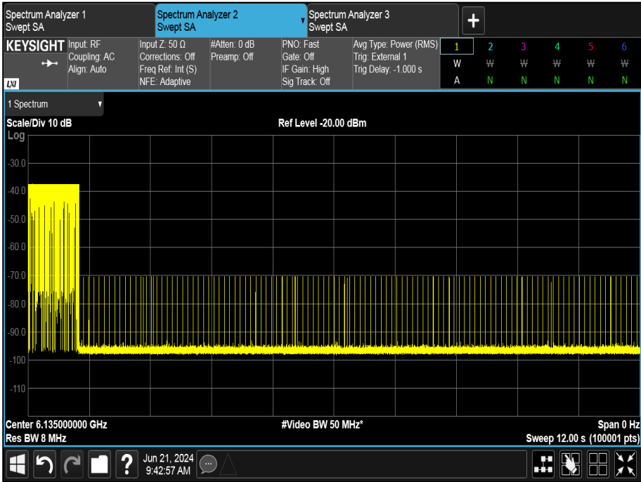
Figure 348 - U-NII-5, Minimum Bandwidth (AWGN Low)
