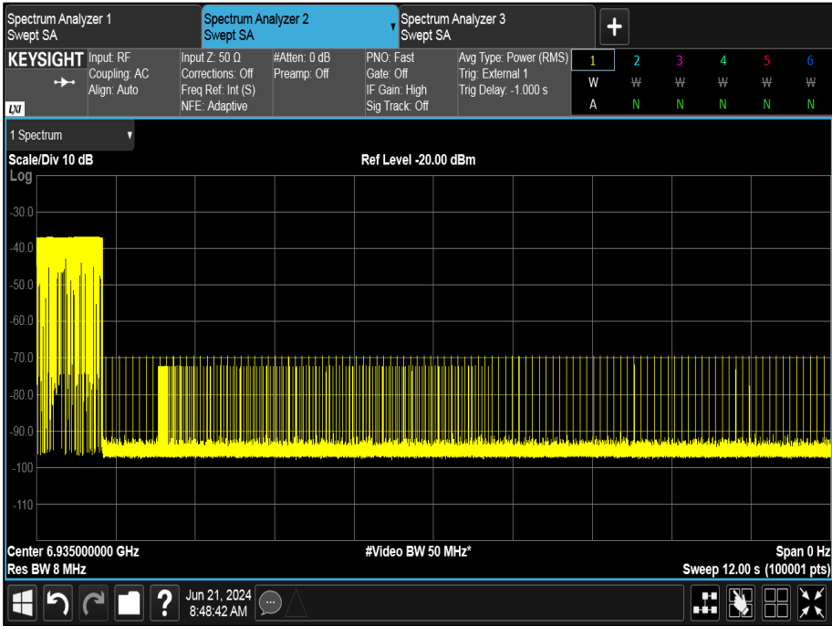
Figure 360 - U-NII-8, Minimum Bandwidth (AWGN Low)
