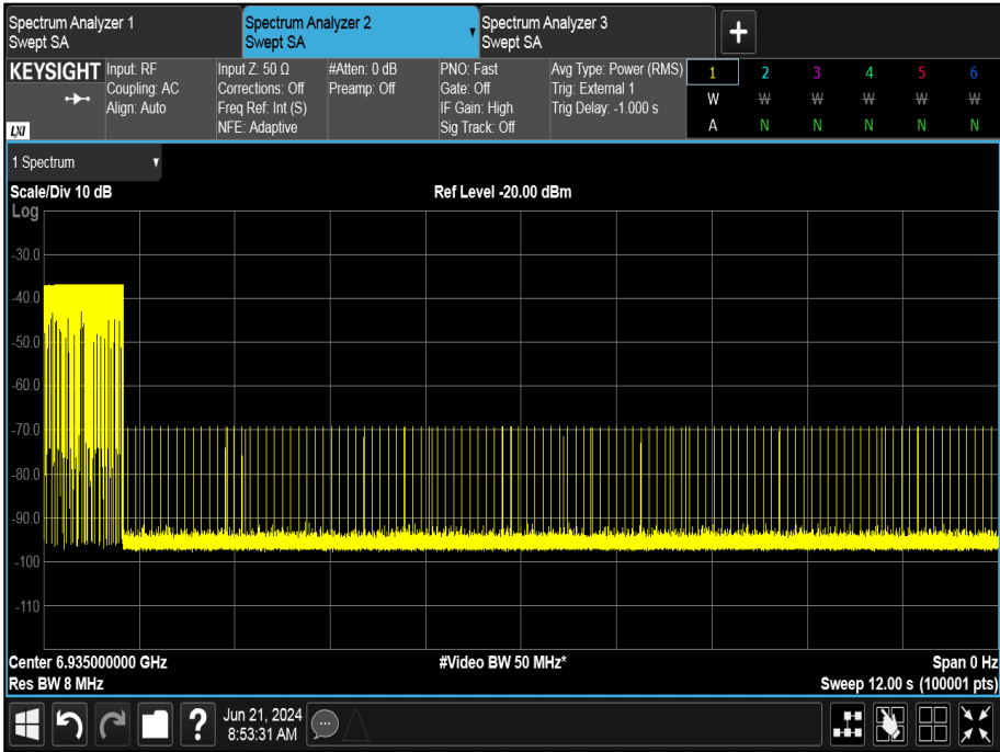
Figure 361 - U-NII-8, Minimum Bandwidth (AWGN Mid)
