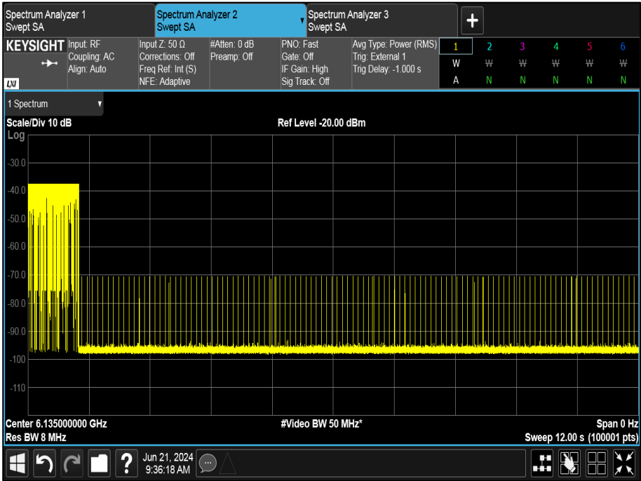
Figure 350 - U-NII-5, Minimum Bandwidth (AWGN High)
