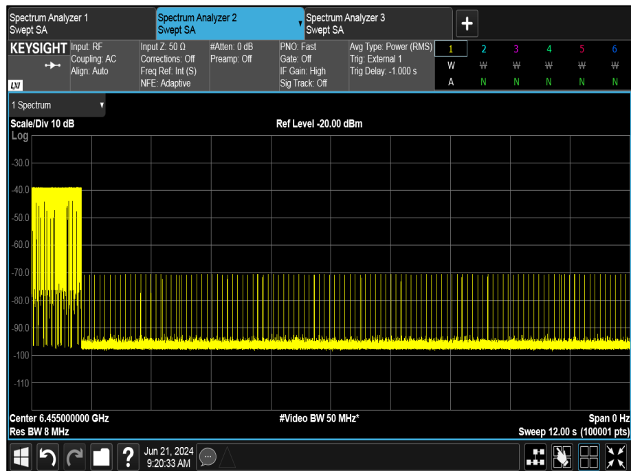
Figure 354 - U-NII-6, Minimum Bandwidth (AWGN High)
