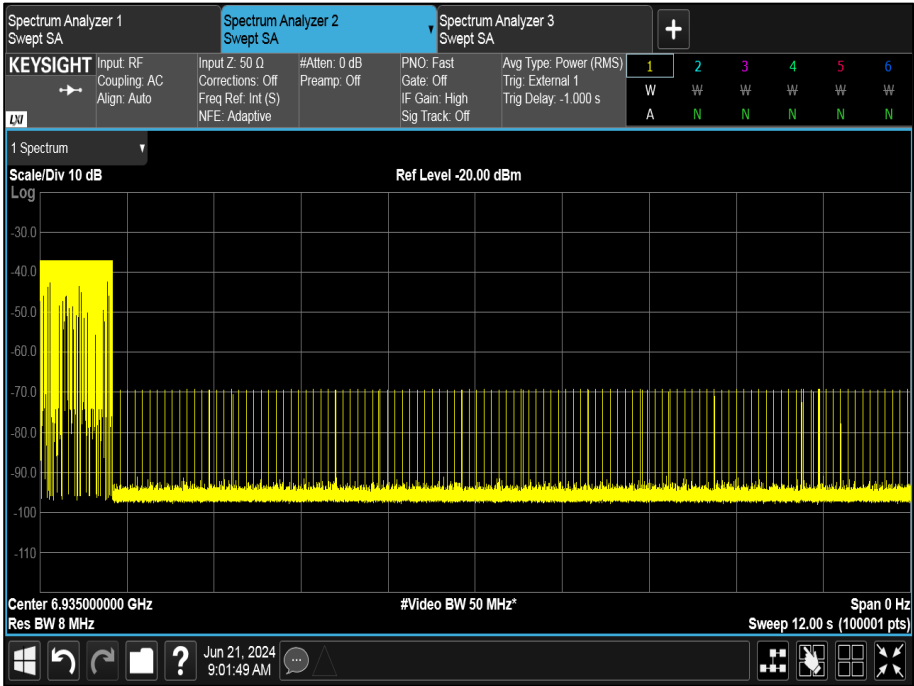
Figure 362 - U-NII-8, Minimum Bandwidth (AWGN High)
