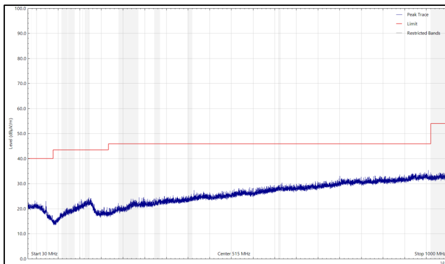
Figure 62 - U-NII-1 - 5240 MHz (CH48), HT20, CDD, Core 0 + Core 1 and 2440 MHz (CH18), Core 1, ePA, 30 MHz to 1 GHz, Horizontal (Peak)
