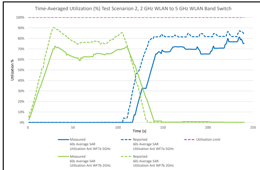
Figure I-7 60s Average Utilization vs. Time during Band Switch
