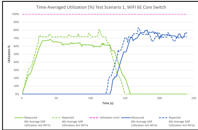
Figure I-5 60s Average SAR Utilization vs. Time, 6 GHz
