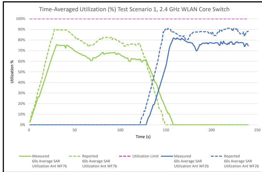
Figure I-1 60s Average SAR Utilization vs. Time, 2.4 GHz
