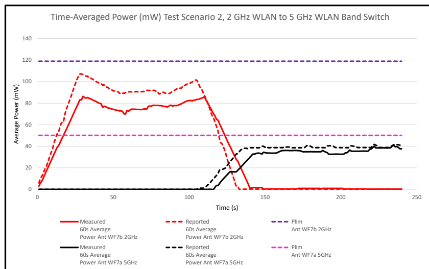
Figure I-8 60s Average Power vs. Time during Band Switch
