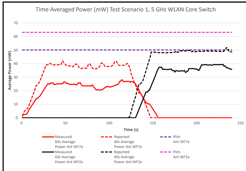
Figure I-4 60s Average Power vs. Time, 5 GHz
