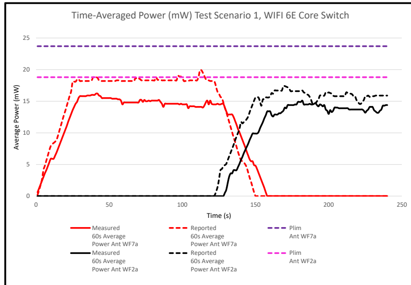
Figure I-6 60s Average Power vs. Time, 6 GHz
