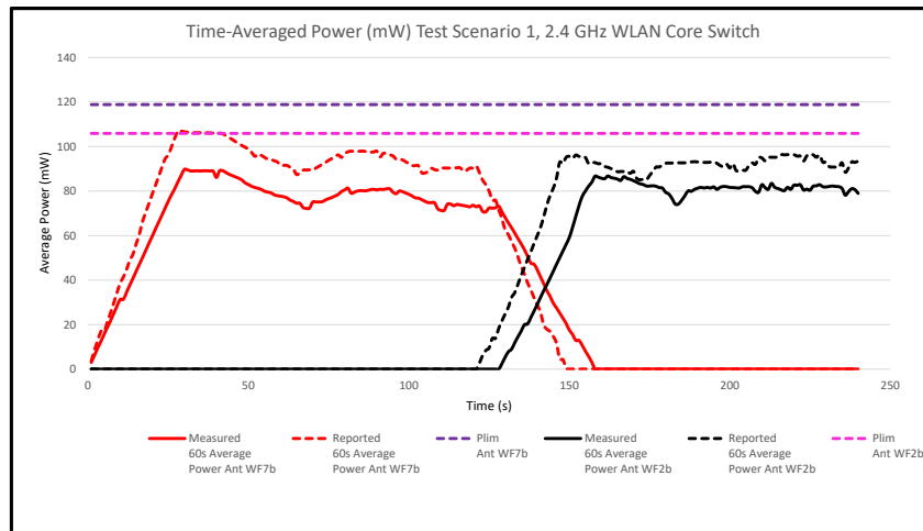
Figure I-2 60s Average Power vs. Time, 2.4 GHz
