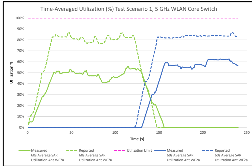
Figure I-3 60s Average SAR Utilization vs. Time, 5 GHz
