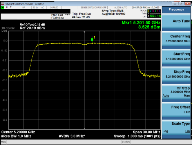
Plot 7-14. PSD Antenna 5T (20MHz BW 11ax– RU242 – Ch.40)
