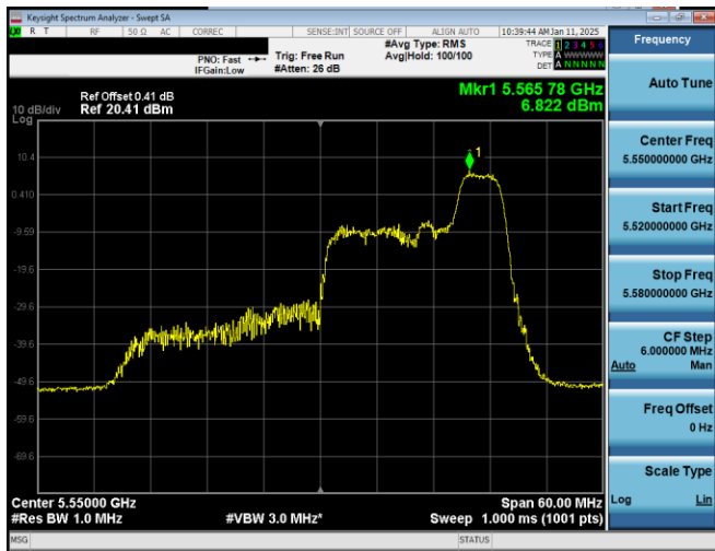
Plot 7-25. PSD Antenna 1b (40MHz BW 11ax Index 44 – RU52 – Ch.110)
