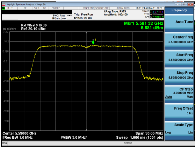
Plot 7-26. PSD Antenna 1b (20MHz BW 11ax– RU242 – Ch.116)
