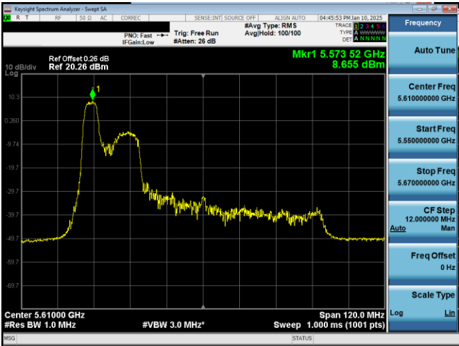
Plot 7-13. (FCC Only) PSD Antenna 5T (80MHz BW 11ax Index 37 – RU52 – Ch.122)
