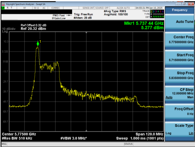
Plot 7-15. PSD Antenna 5T (80MHz BW 11ax Index 0 – RU26 – Ch.155)
