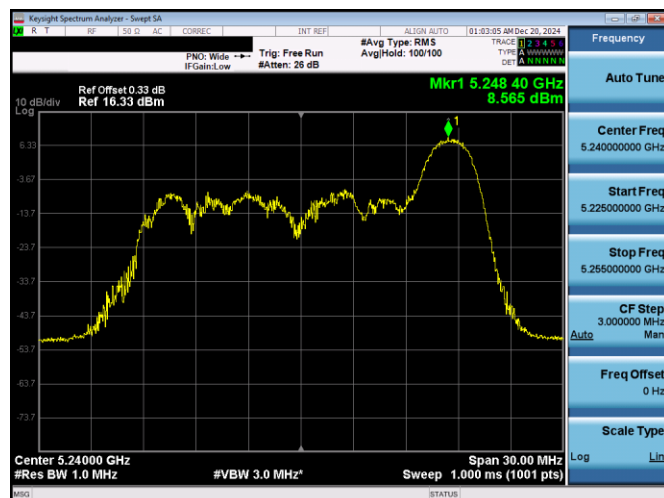
Plot 7-17. PSD Antenna 5T (20MHz BW 11ax Index 8 – RU26 – Ch.48)
