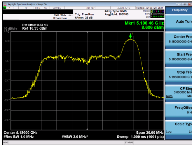
Plot 7-23. PSD Antenna 3b (20MHz BW 11ax Index 8 – RU26 – Ch.36)
