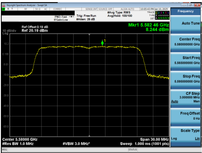
Plot 7-20. PSD Antenna 3b (20MHz BW 11ax– RU242 – Ch.116)
