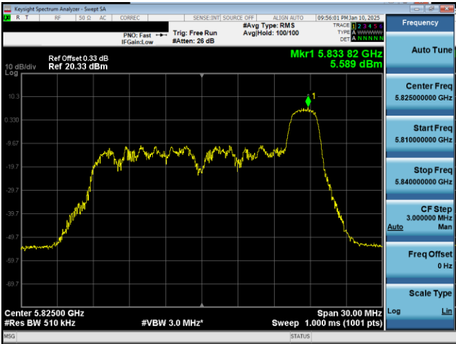
Plot 7-21. PSD Antenna 3b (20MHz BW 11ax Index 8 – RU26 – Ch.165)
