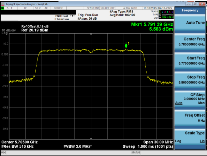
Plot 7-22. PSD Antenna 3b (20MHz BW 11ax– RU242 – Ch.157)
