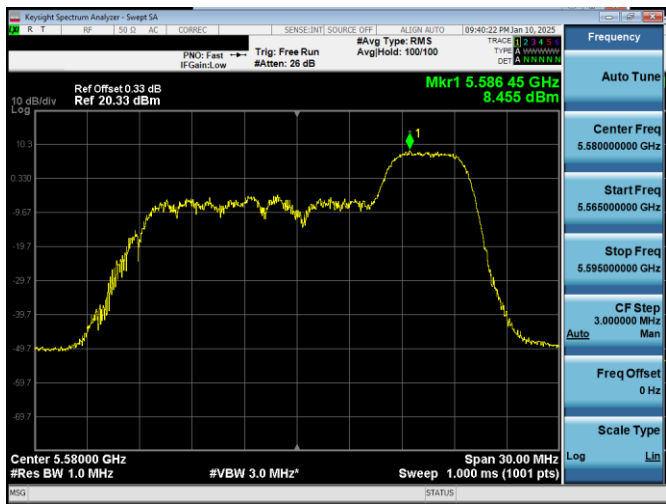
Plot 7-19. PSD Antenna 3b (20MHz BW 11ax Index40 – RU52 – Ch.116)
