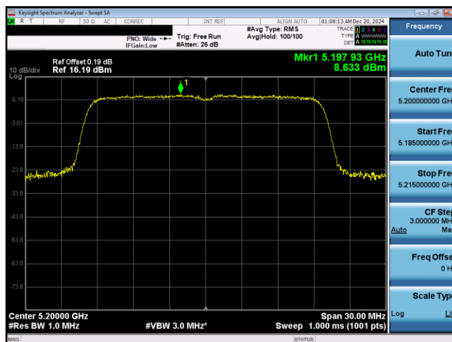
Plot 7-18. PSD Antenna 5T (20MHz BW 11ax– RU242 – Ch.40)
