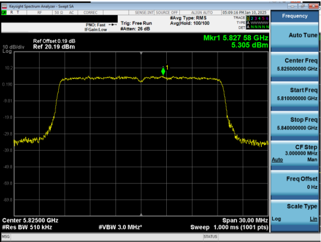
Plot 7-16. PSD Antenna 5T (20MHz BW 11ax– RU242 – Ch.165)
