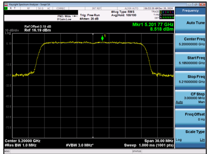
Plot 7-24. PSD Antenna 3b (20MHz BW 11ax– RU242 – Ch.40)
