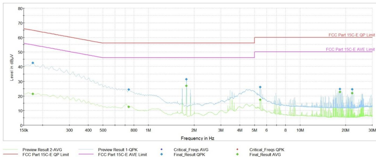
Plot 6-12. AC Line Conducted Plot (N - Mode 1, with host Laptop via USB-C cable)
