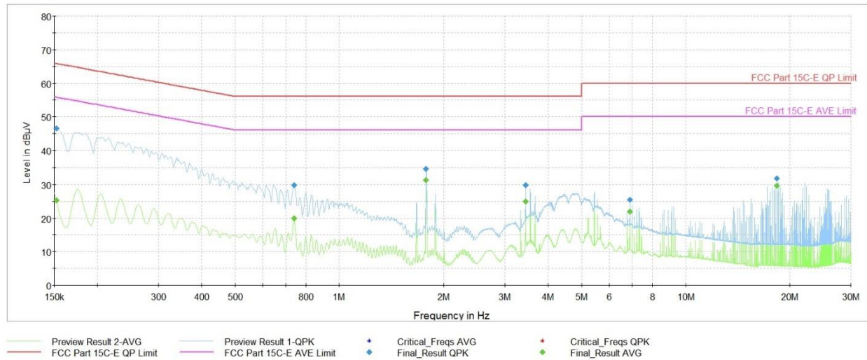
Plot 6-11. AC Line Conducted Plot (L1 - Mode 1, with host Laptop via USB-C cable)
