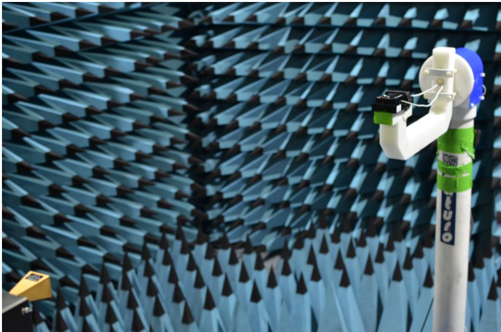
Figure 5: 60-90GHz Test Setup
