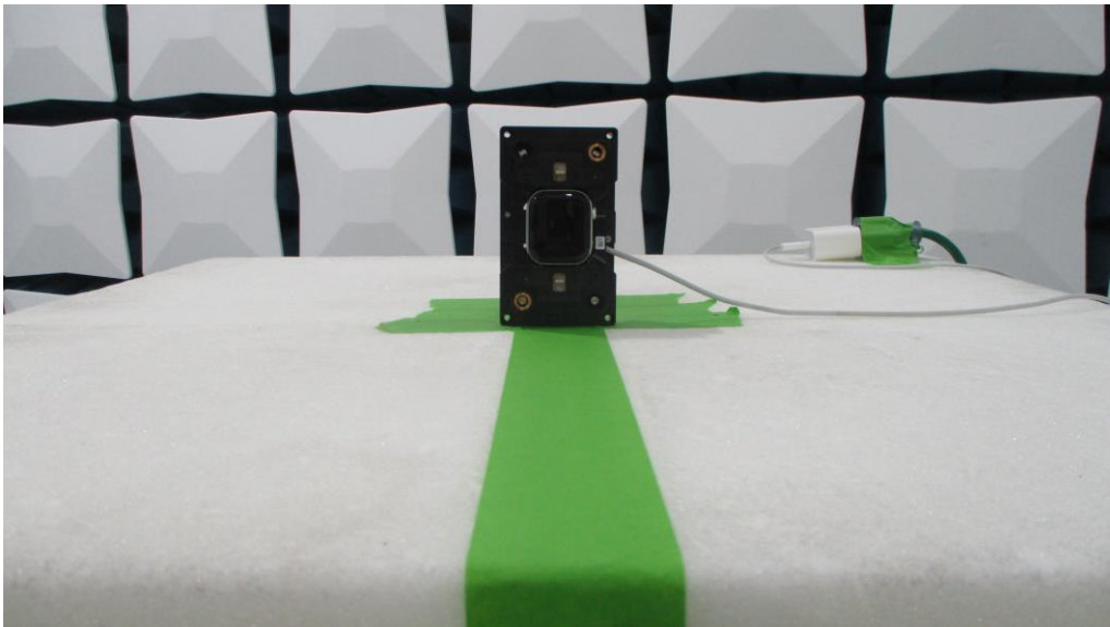
Figure 12: 1-18GHz Test Setup (Front View)
