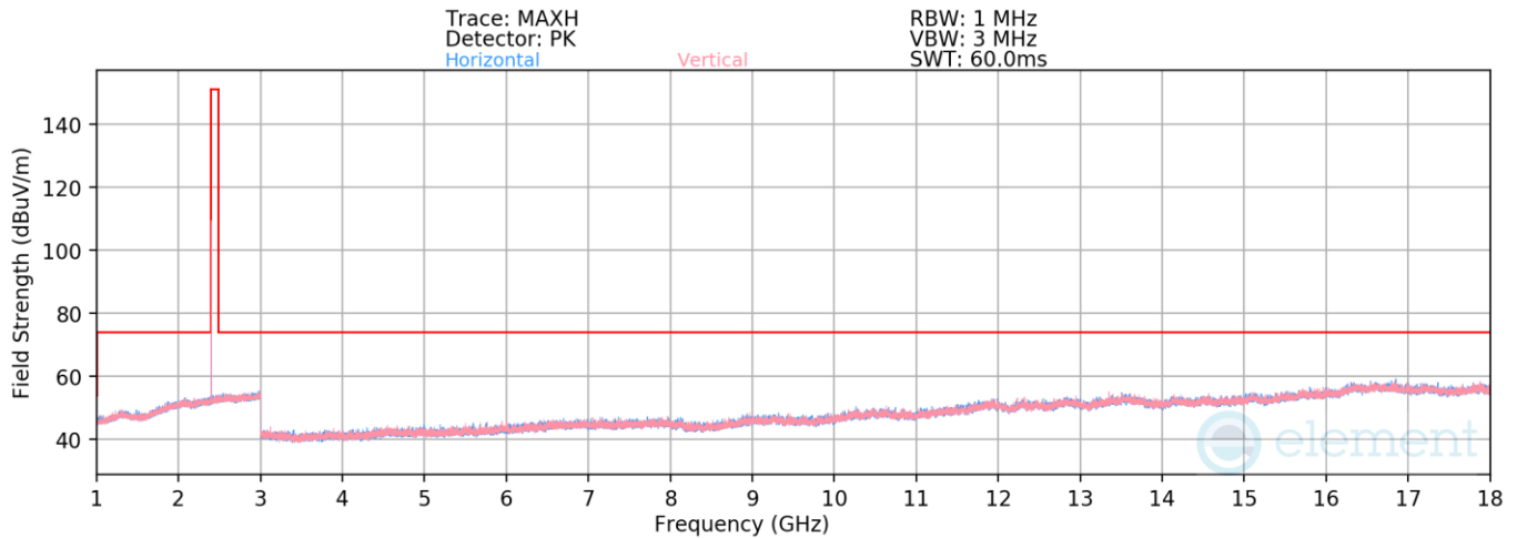
Plot 7-57. Radiated Spurious Emissions 1-18GHz Antenna 0 (Dedicated) (1Mbps, iPA – Ch. 37)
