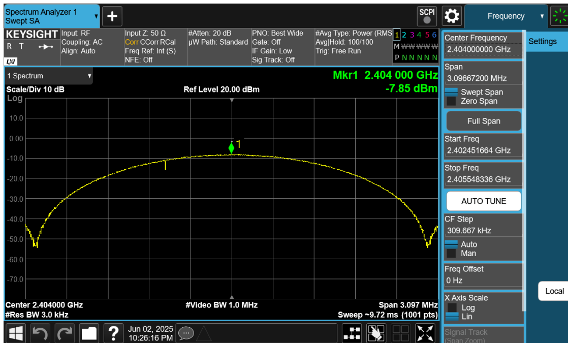
Plot 7-34. Power Spectral Density Plot Antenna 0 (Dedicated) (Bluetooth (LE), 2Mbps, iPA – Ch. 0)
