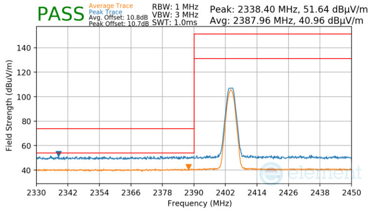
Plot 7-63. Radiated Restricted Lower Band Edge Measurement Antenna 0 (Common) (Average & Peak)
