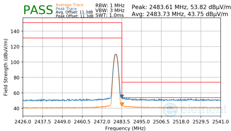
Plot 7-66. Radiated Restricted Upper Band Edge Measurement Antenna 0 (Dedicated) (Average & Peak)
