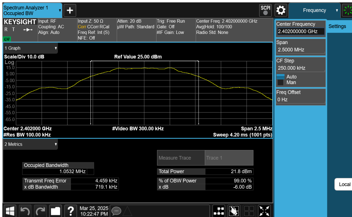
Plot 7-13. 6dB BW Plot Antenna 0 (Common) (Bluetooth (LE), 1Mbps, iPA – Ch. 37)
