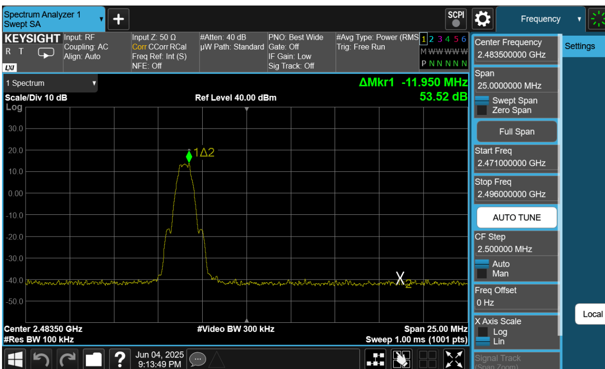
Plot 7-38. Band Edge Plot Antenna 0 (Common) (Bluetooth (LE), 1Mbps, iPA – Ch. 39)
