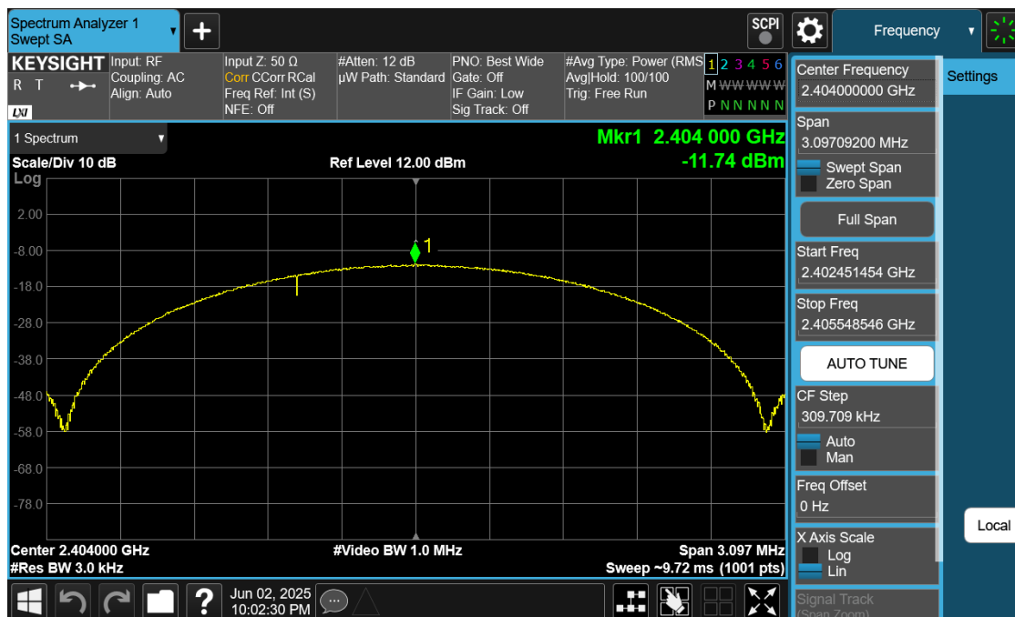
Plot 7-28. Power Spectral Density Plot Antenna 0 (Common) (Bluetooth (LE), 2Mbps, iPA – Ch. 0)
