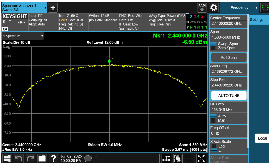
Plot 7-26. Power Spectral Density Plot Antenna 0 (Common) (Bluetooth (LE), 1Mbps, iPA – Ch. 17)
