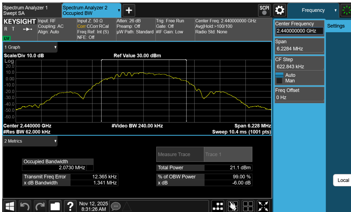
Plot 7-5. 99% OBW Plot Antenna 0 (Common) (Bluetooth (LE), 2Mbps, iPA – Ch. 17)
