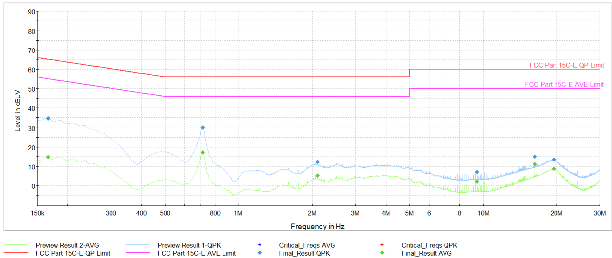
Plot 7-70. AC Line Conducted Plot with Bluetooth LE Antenna 0 (Dedicated) (L1, 1Mbps iPA – Ch.17 with AC/DC Adapter via USB-C cable)
