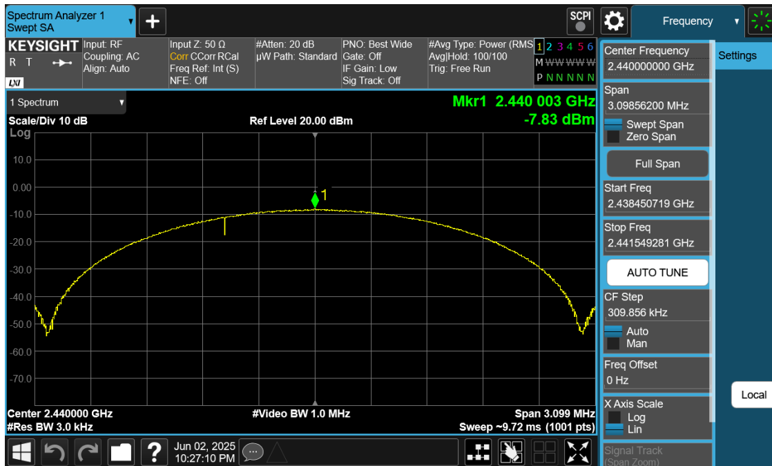
Plot 7-35. Power Spectral Density Plot Antenna 0 (Dedicated) (Bluetooth (LE), 2Mbps, iPA – Ch. 17)
