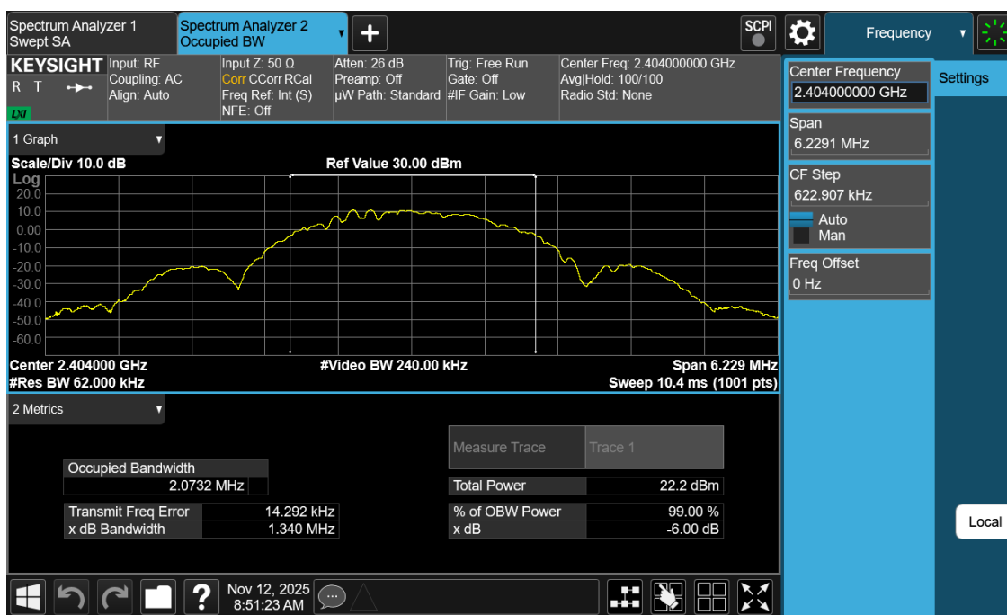
Plot 7-10. 99% OBW Plot Antenna 0 (Dedicated) (Bluetooth (LE), 2Mbps, iPA – Ch. 0)
