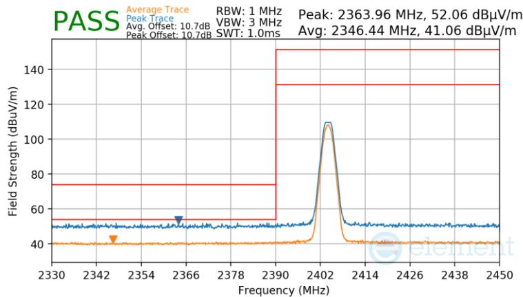
Plot 7-67. Radiated Restricted Lower Band Edge Measurement Antenna 0 (Dedicated) (Average & Peak)
