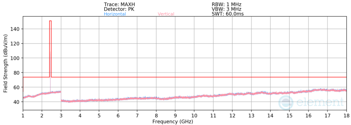
Plot 7-58. Radiated Spurious Emissions 1-18GHz Antenna 0 (Dedicated) (1Mbps, iPA – Ch. 17)
