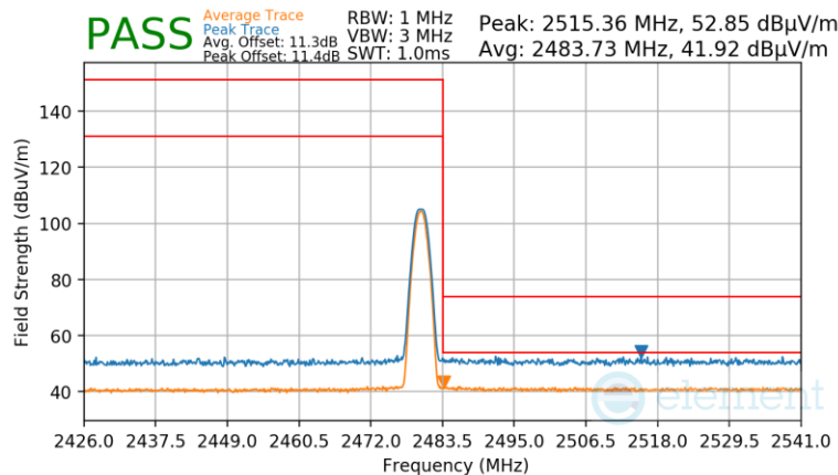
Plot 7-62. Radiated Restricted Upper Band Edge Measurement Antenna 0 (Common) (Average & Peak)
