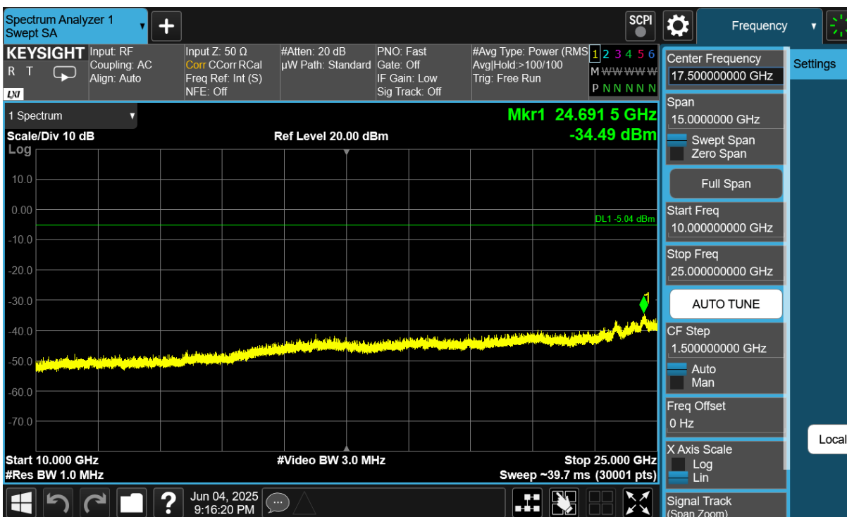
Plot 7-52. Conducted Spurious Plot Antenna 0 (Dedicated) (Bluetooth (LE), 1Mbps, iPA – Ch. 37)
