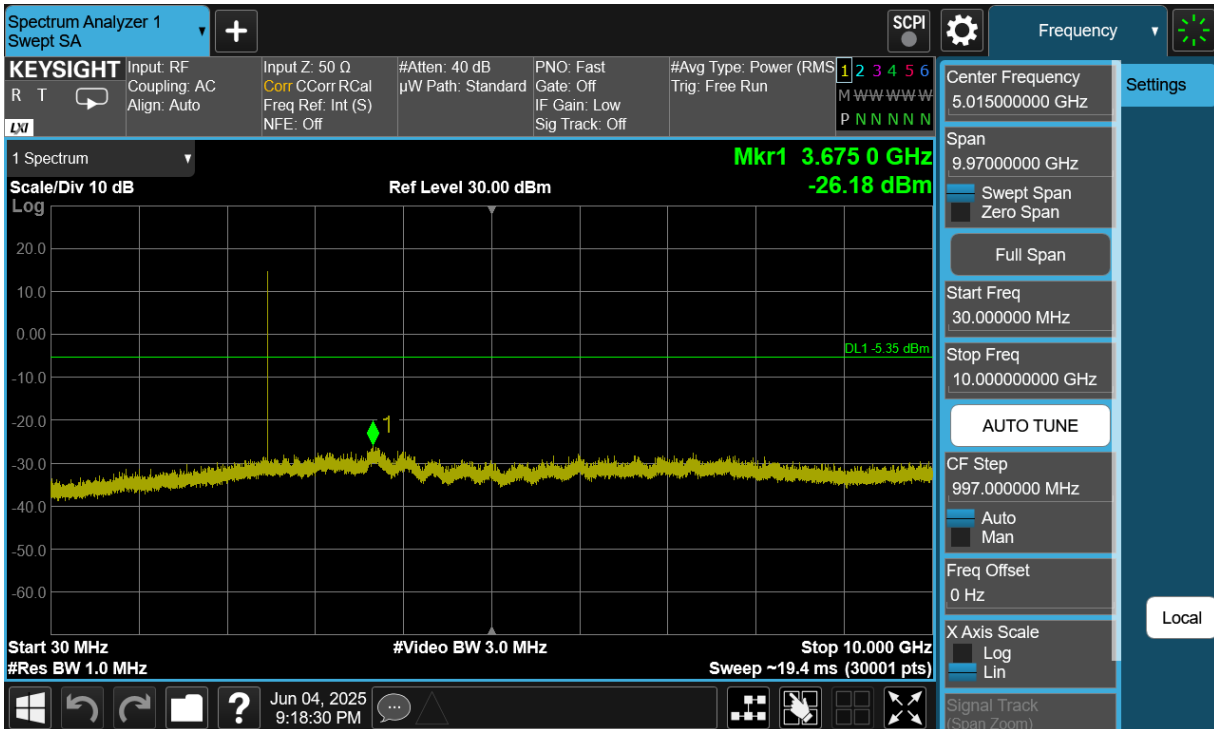
Plot 7-49. Conducted Spurious Plot Antenna 0 (Common) (Bluetooth (LE), 1Mbps, iPA – Ch. 39)
