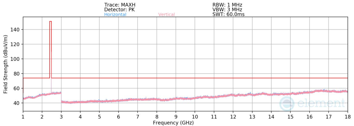
Plot 7-60. Radiated Spurious Emissions 1-18GHz Antenna 0 (Dedicated) (1Mbps iPA – Ch. 39)
