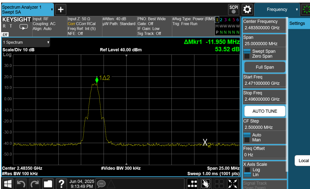
Plot 7-42. Band Edge Plot Antenna 0 (Dedicated) (Bluetooth (LE), 1Mbps, iPA – Ch. 39)
