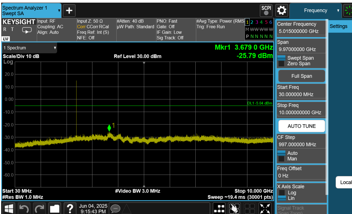
Plot 7-45. Conducted Spurious Plot Antenna 0 (Common) (Bluetooth (LE), 1Mbps, iPA – Ch. 37)
