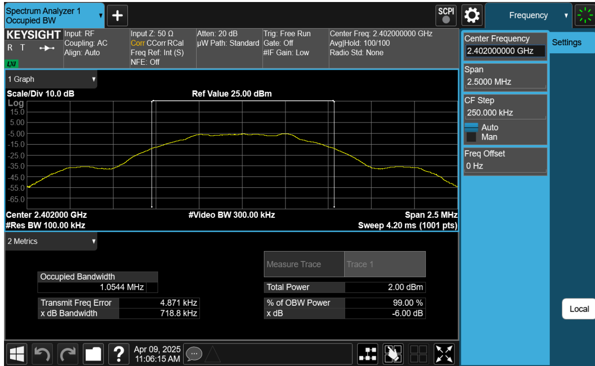
Plot 7-19. 6dB BW Plot Antenna 0 (Dedicated) (Bluetooth (LE), 1Mbps, iPA – Ch. 37)
