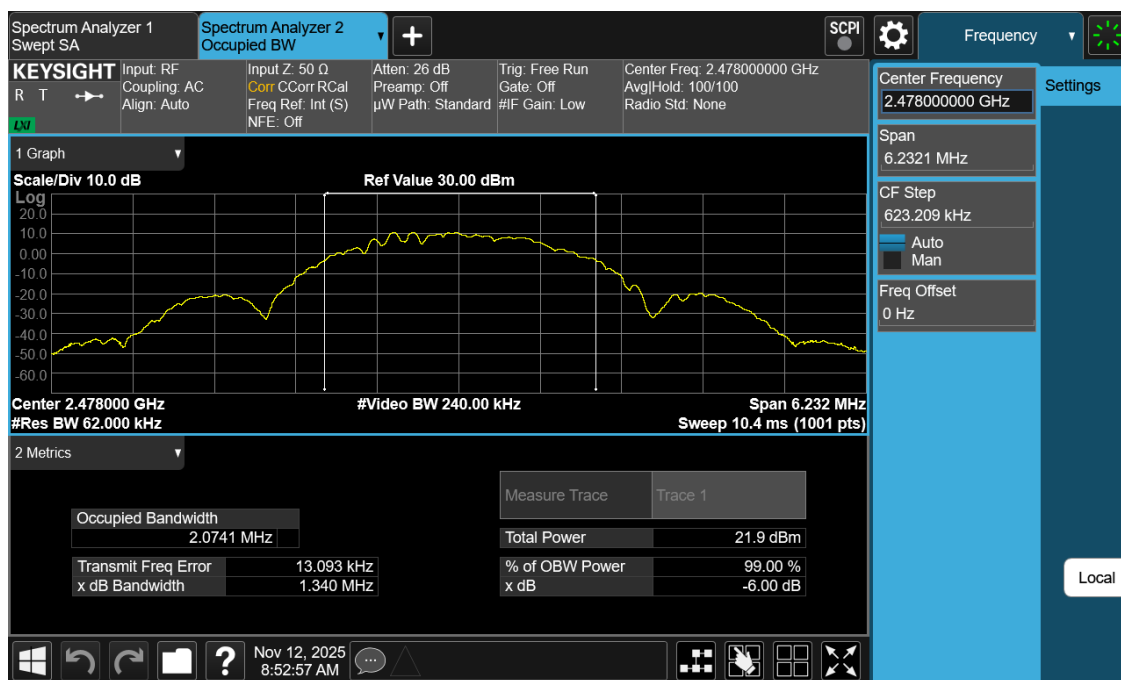
Plot 7-12. 99% OBW Plot Antenna 0 (Dedicated) (Bluetooth (LE), 2Mbps, iPA – Ch. 36)
