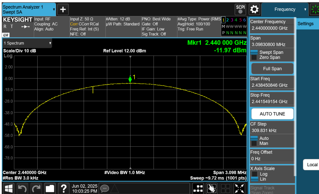
Plot 7-29. Power Spectral Density Plot Antenna 0 (Common) (Bluetooth (LE), 2Mbps, iPA – Ch. 17)
