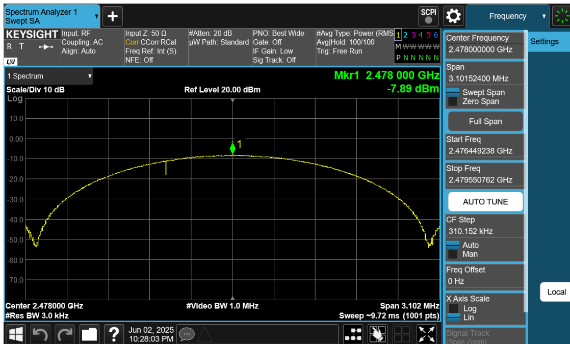
Plot 7-36. Power Spectral Density Plot Antenna 0 (Dedicated) (Bluetooth (LE), 2Mbps, iPA – Ch. 36)
