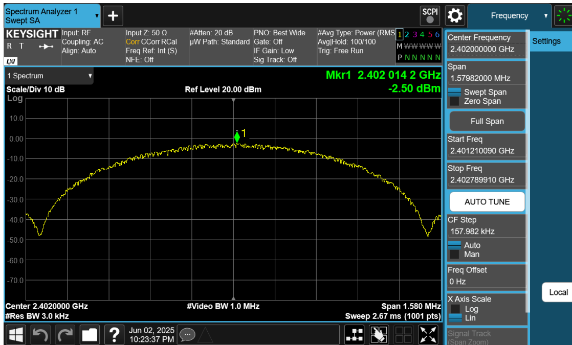
Plot 7-31. Power Spectral Density Plot Antenna 0 (Dedicated) (Bluetooth (LE), 1Mbps, iPA – Ch. 37)
