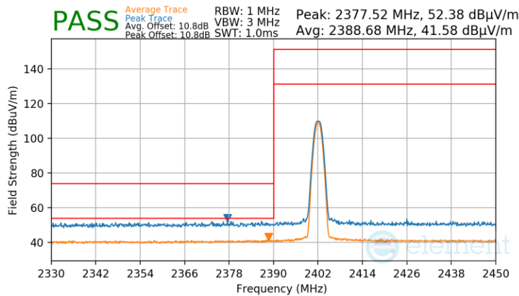
Plot 7-65. Radiated Restricted Lower Band Edge Measurement Antenna 0 (Dedicated) (Average & Peak)
