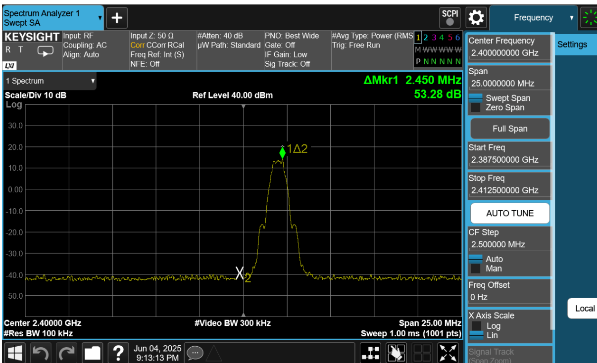
Plot 7-37. Band Edge Plot Antenna 0 (Common) (Bluetooth (LE), 1Mbps, iPA – Ch.37)
