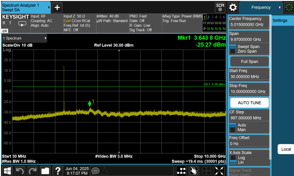
Plot 7-47. Conducted Spurious Plot Antenna 0 (Common) (Bluetooth (LE), 1Mbps, iPA – Ch. 17)
