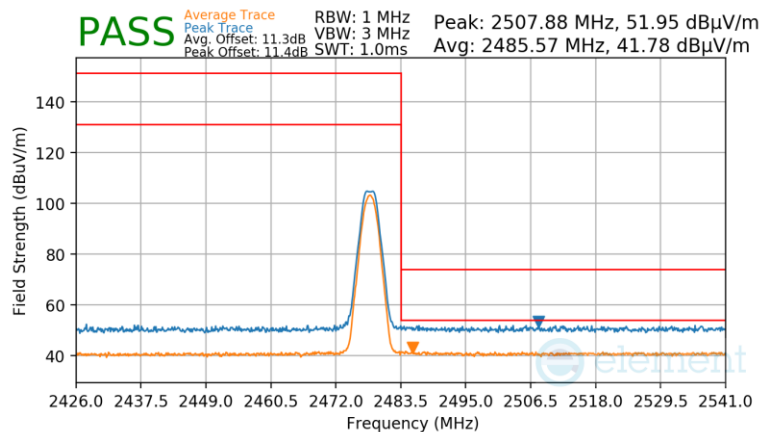
Plot 7-64. Radiated Restricted Upper Band Edge Measurement Antenna 0 (Common) (Average & Peak)
