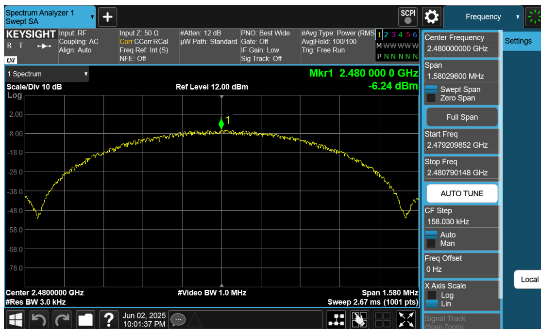
Plot 7-27. Power Spectral Density Plot Antenna 0 (Common) (Bluetooth (LE), 1Mbps, iPA – Ch. 39)
