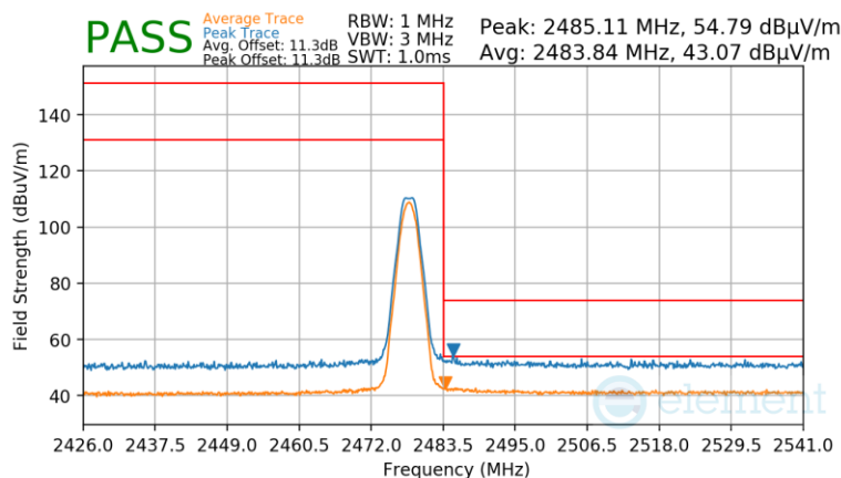
Plot 7-68. Radiated Restricted Upper Band Edge Measurement Antenna 0 (Dedicated) (Average & Peak)
