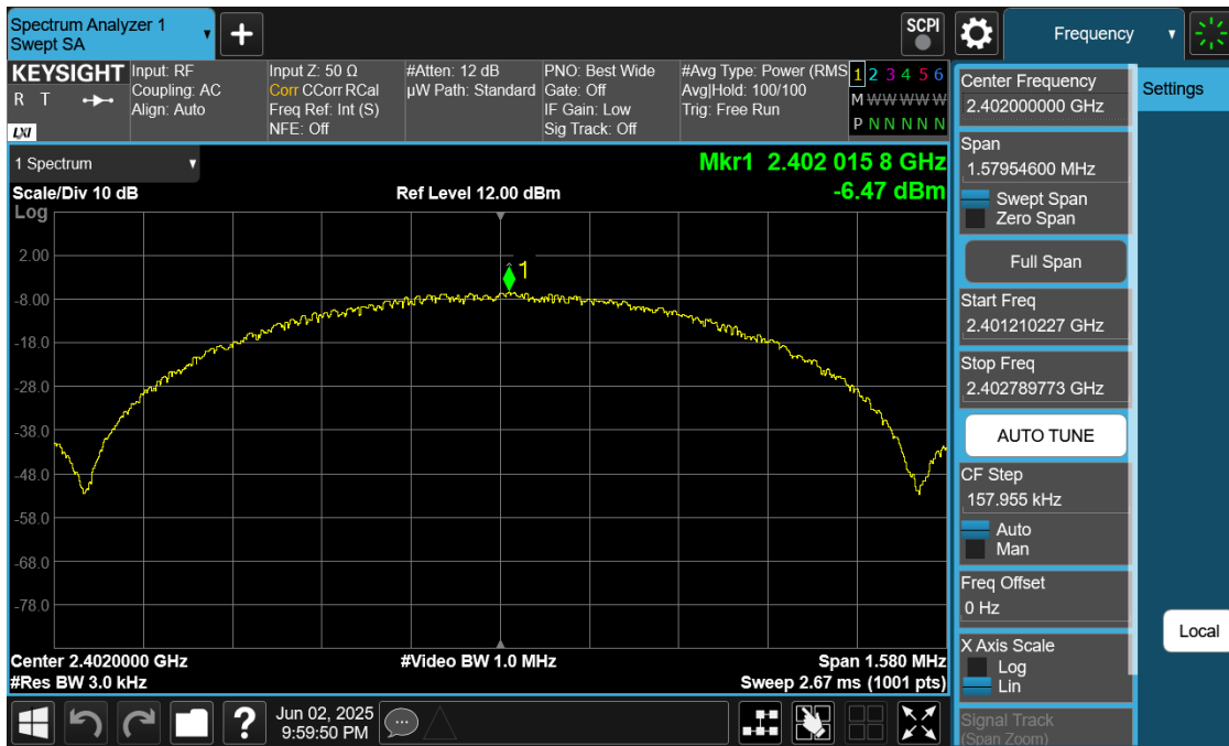
Plot 7-25. Power Spectral Density Plot Antenna 0 (Common) (Bluetooth (LE), 1Mbps, iPA – Ch. 37)
