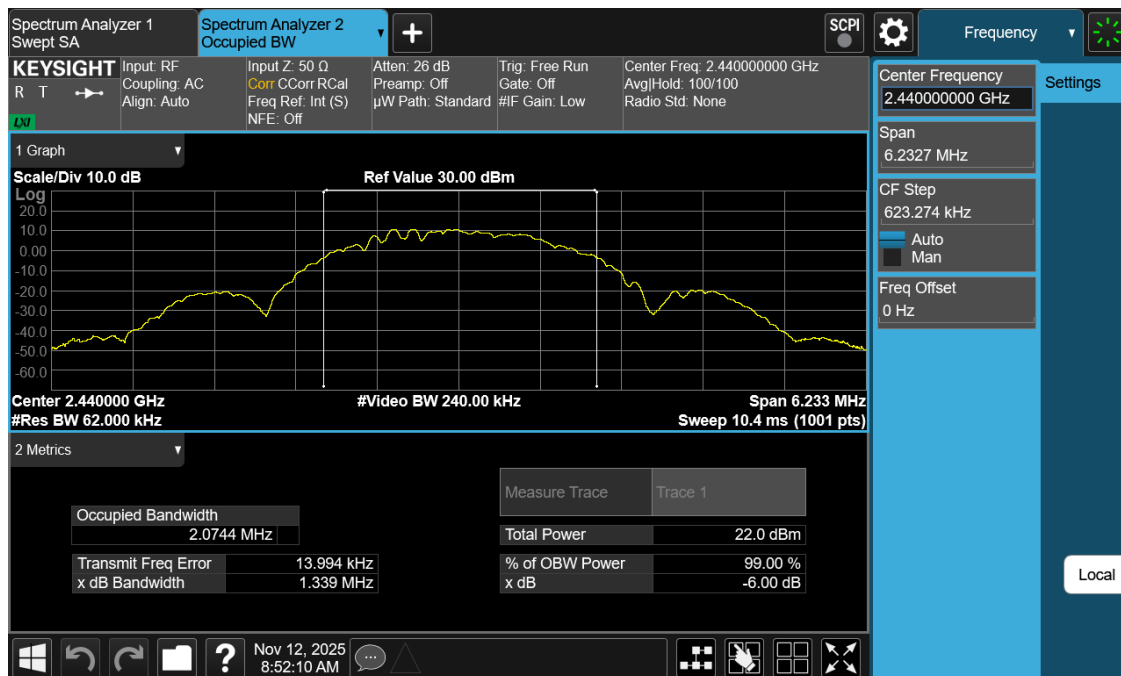
Plot 7-11. 99% OBW Plot Antenna 0 (Dedicated) (Bluetooth (LE), 2Mbps, iPA – Ch. 17)
