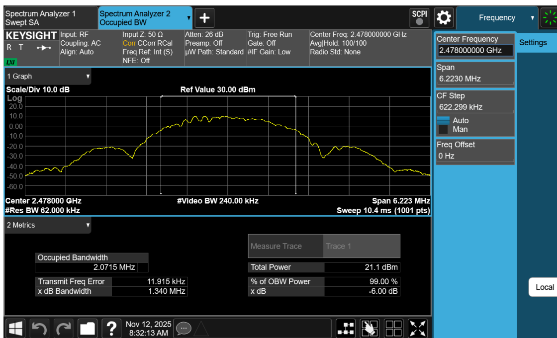
Plot 7-6. 99% OBW Plot Antenna 0 (Common) (Bluetooth (LE), 2Mbps, iPA – Ch. 36)
