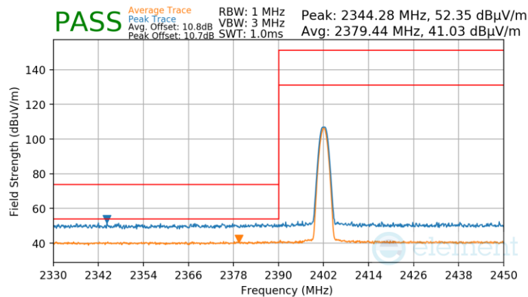
Plot 7-61. Radiated Restricted Lower Band Edge Measurement Antenna 0 (Common) (Average & Peak)
