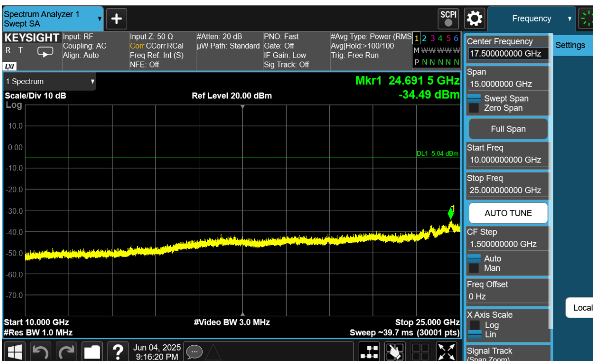
Plot 7-46. Conducted Spurious Plot Antenna 0 (Common) (Bluetooth (LE), 1Mbps, iPA – Ch. 37)
