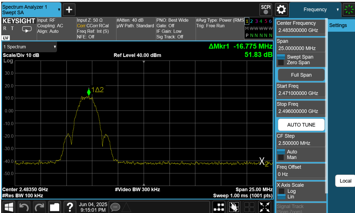
Plot 7-44. Band Edge Plot Antenna 0 (Dedicated) (Bluetooth (LE), 2Mbps, iPA – Ch. 36)
