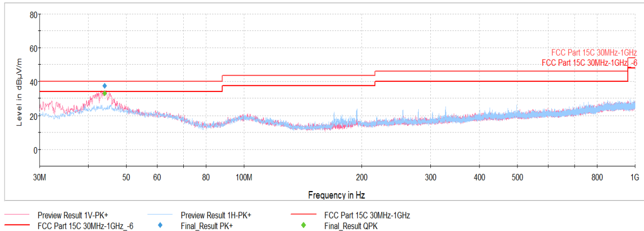
Plot 7-69. Radiated Spurious Emissions Below 1GHz Antenna 0 (Dedicated) (1Mbps, iPA – Ch.17, Pol. H & V, with AC/DC Adapter via USB-C cable)
