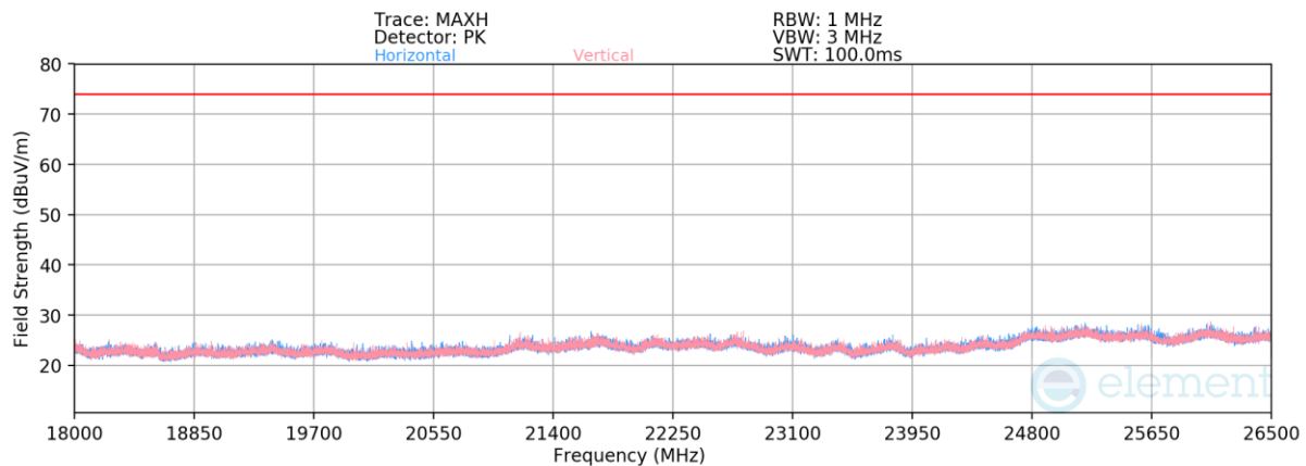
Plot 7-59. Radiated Spurious Emissions Above 18GHz Antenna 0 (Dedicated) (1Mbps, iPA – Ch. 17)
