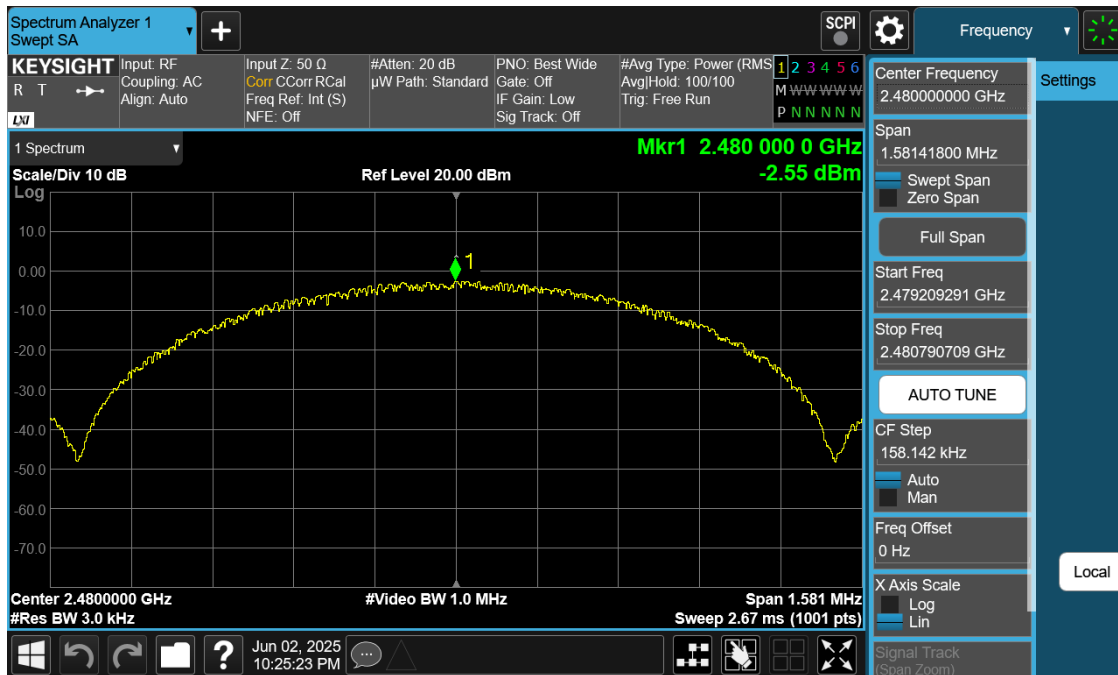
Plot 7-33. Power Spectral Density Plot Antenna 0 (Dedicated) (Bluetooth (LE), 1Mbps, iPA – Ch. 39)
