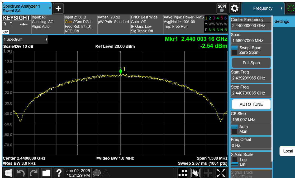
Plot 7-32. Power Spectral Density Plot Antenna 0 (Dedicated) (Bluetooth (LE), 1Mbps, iPA – Ch. 17)
