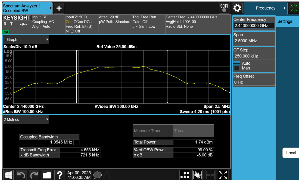
Plot 7-20. 6dB BW Plot Antenna 0 (Dedicated) (Bluetooth (LE), 1Mbps, iPA – Ch. 17)
