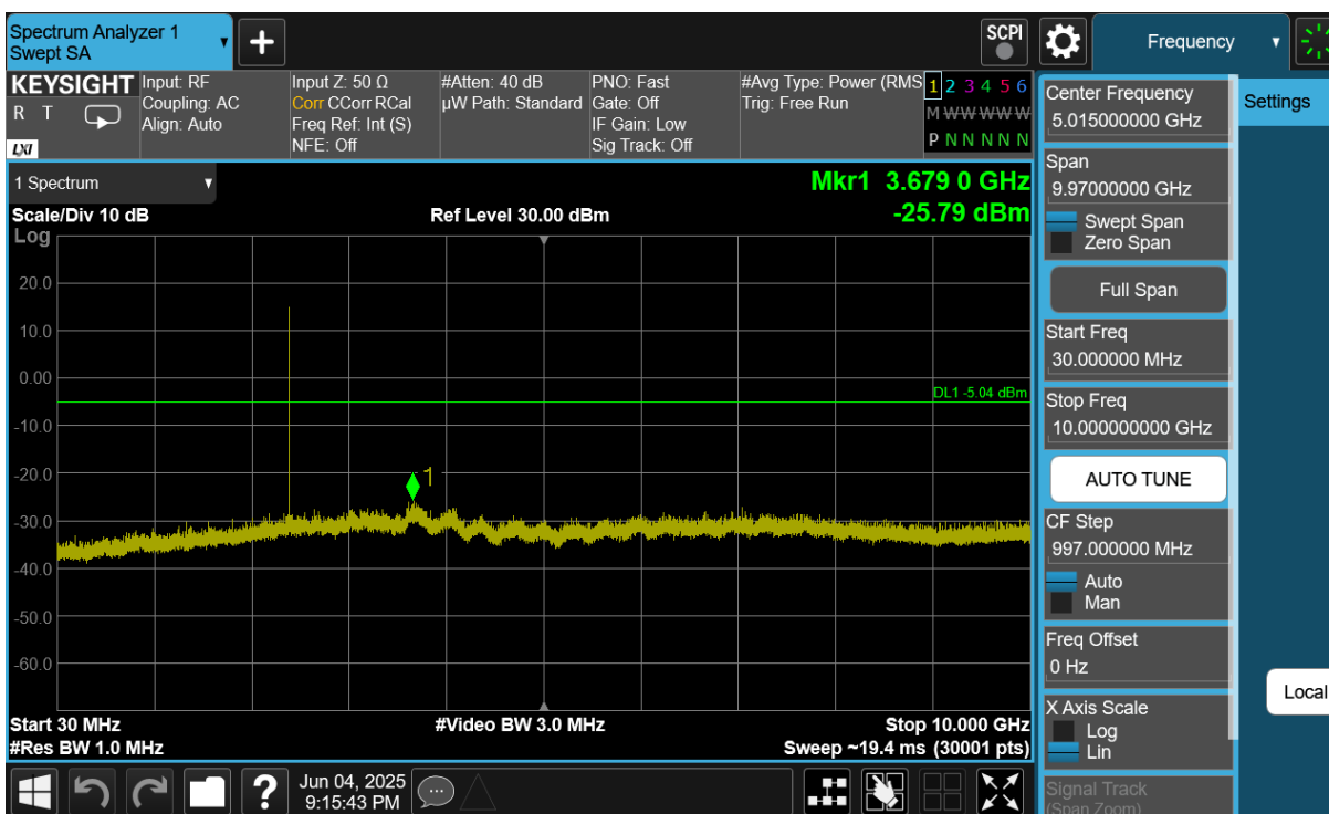
Plot 7-51. Conducted Spurious Plot Antenna 0 (Dedicated) (Bluetooth (LE), 1Mbps, iPA – Ch. 37)
