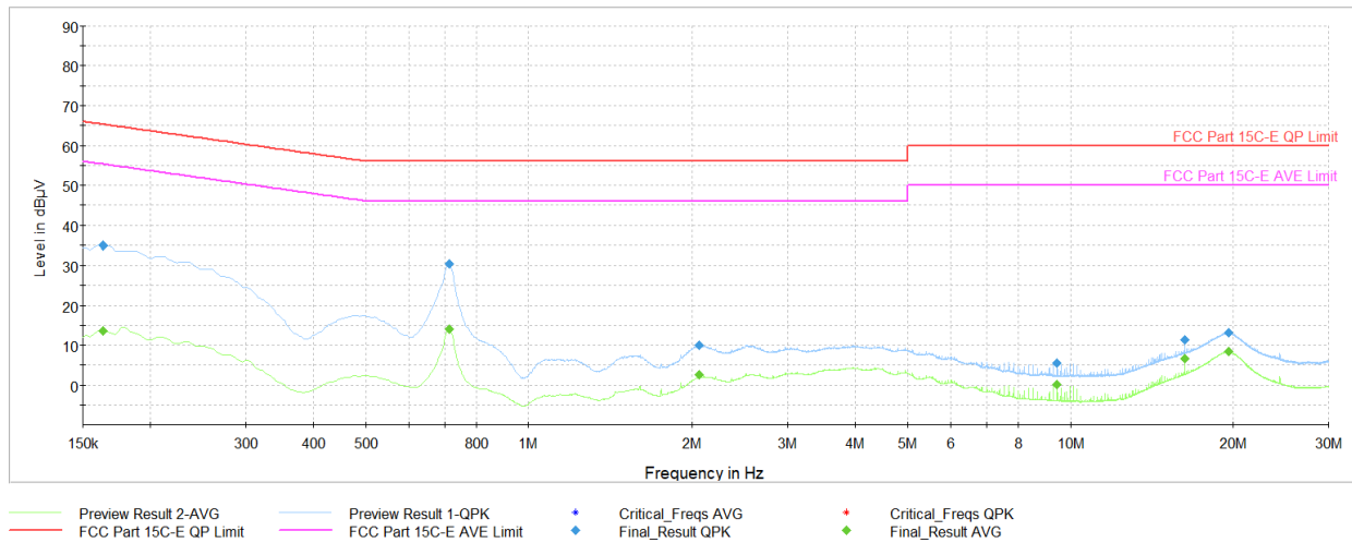
Plot 7-71. AC Line Conducted Plot with Bluetooth LE Antenna 0 (Dedicated) (N, 1Mbps iPA – Ch.17, with AC/DC Adapter via USB-C cable)
