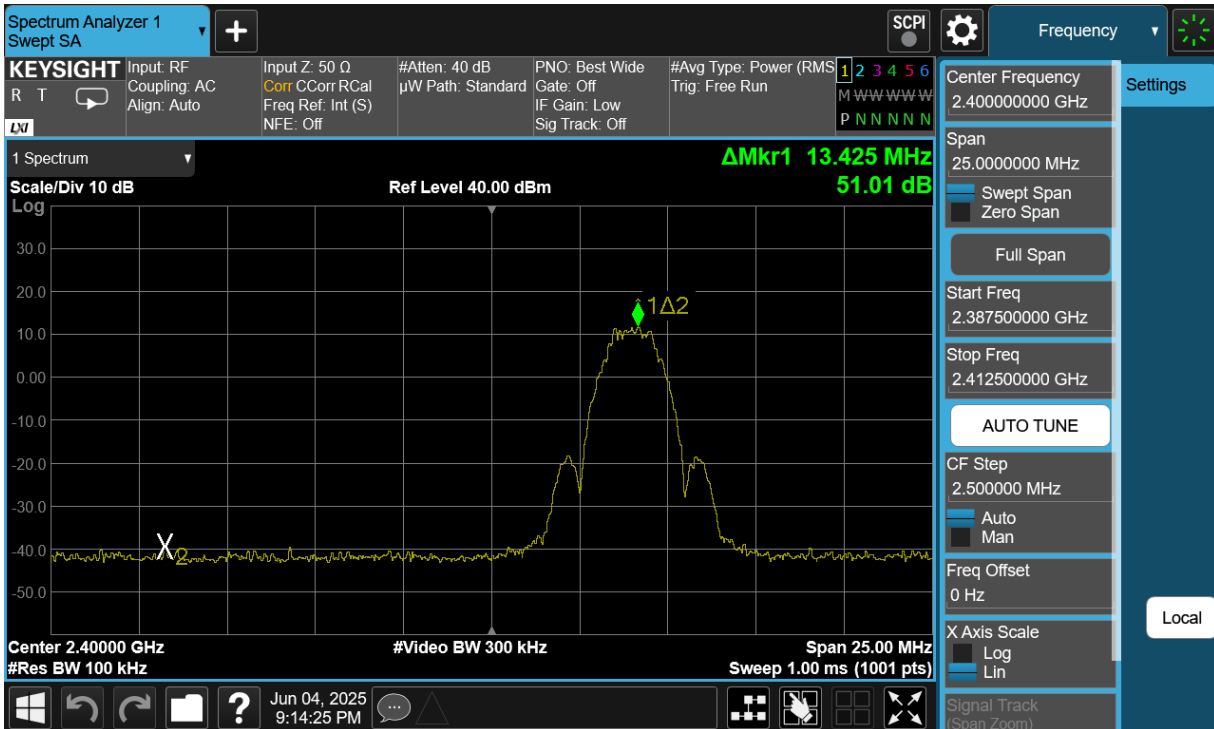
Plot 7-43. Band Edge Plot Antenna 0 (Dedicated) (Bluetooth (LE), 2Mbps, iPA – Ch. 0)
