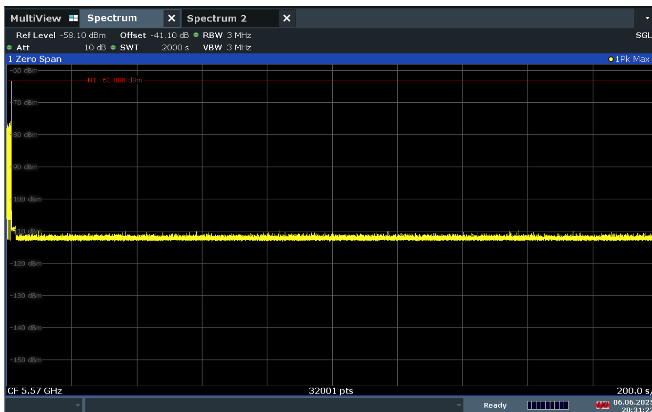
Figure 9-4. 5570MHz - Non-Occupancy Period (30 Minutes) - Mode 1 (160MHz)
