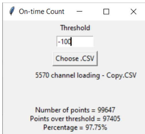
Figure 9-2. 5570MHz - Channel Loading Calculation - Mode 1 (160MHz)
