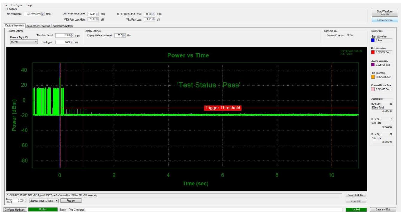
Figure 9-3. 5570MHz - Channel Move/ Closing Transmission Time - Mode 1 (160 MHz)
