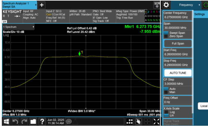
Plot 7-41. Power Spectral Density Plot Antenna 0 (20MHz 802.11a (UNII Band 5) – Ch. 65, 24Mbps)
