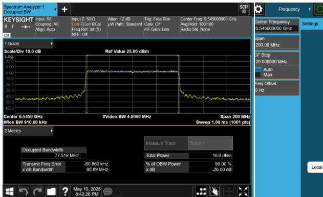
Plot 7-14. 26dB & 99% Bandwidth Plot Antenna 0 (80MHz 802.11ax (UNII Band 7) – Ch. 119, MCS11)
