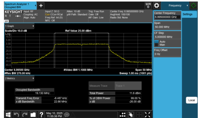
Plot 7-37. 26dB & 99% Bandwidth Plot Antenna 1 (20MHz 802.11ax (UNII Band 8) – Ch. 209, MCS11)
