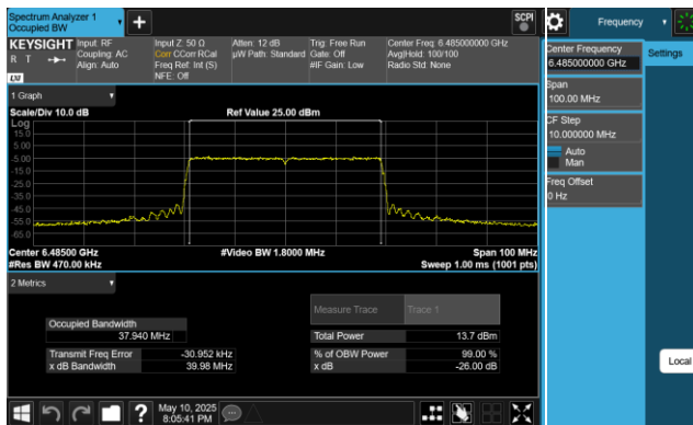
Plot 7-8. 26dB & 99% Bandwidth Plot Antenna 0 (40MHz 802.11ax (UNII Band 6) – Ch. 107, MCS11)
