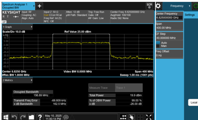
Plot 7-35. 26dB & 99% Bandwidth Plot Antenna 1 (160MHz 802.11ax (UNII Band 7) – Ch. 175, MCS2)
