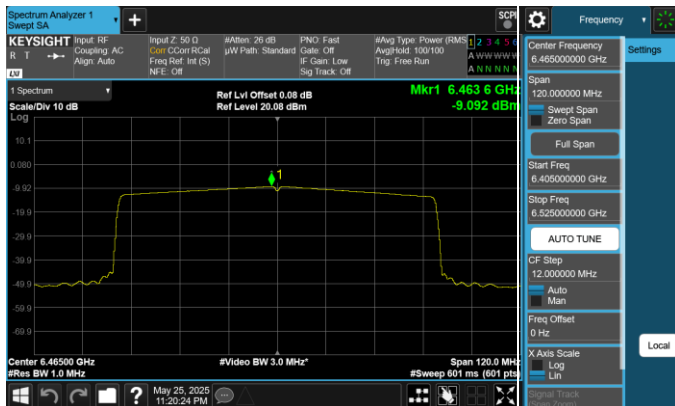
Plot 7-49. Power Spectral Density Plot Antenna 0 (80MHz 802.11ax (UNII Band 6) – Ch. 103, MCS2)
