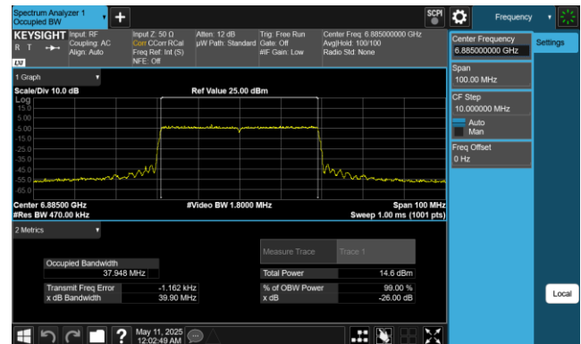
Plot 7-38. 26dB & 99% Bandwidth Plot Antenna 1 (40MHz 802.11ax (UNII Band 8) – Ch. 187, MCS2)
