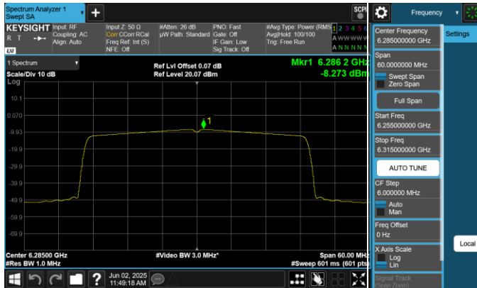
Plot 7-43. Power Spectral Density Plot Antenna 0 (40MHz 802.11ax (UNII Band 5) – Ch. 67, MCS2)
