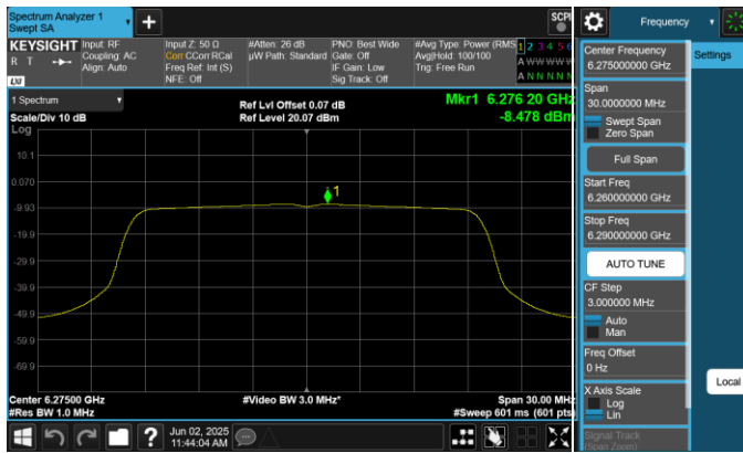
Plot 7-42. Power Spectral Density Plot Antenna 0 (20MHz 802.11ax (UNII Band 5) – Ch. 65, MCS4)
