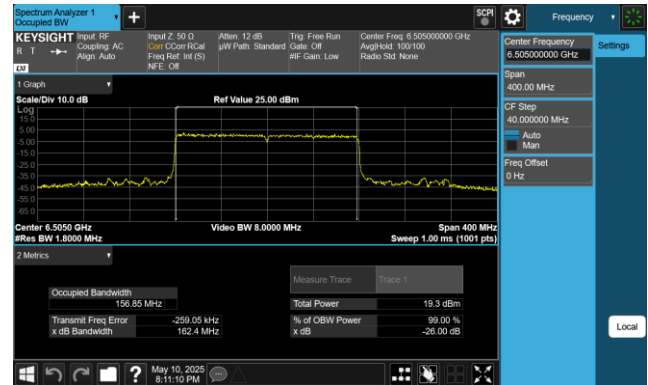
Plot 7-10. 26dB & 99% Bandwidth Plot Antenna 0 (160MHz 802.11ax (UNII Band 6) – Ch. 111, MCS11)
