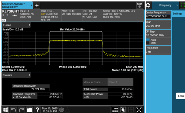
Plot 7-34. 26dB & 99% Bandwidth Plot Antenna 1 (80MHz 802.11ax (UNII Band 7) – Ch. 151, MCS11)
