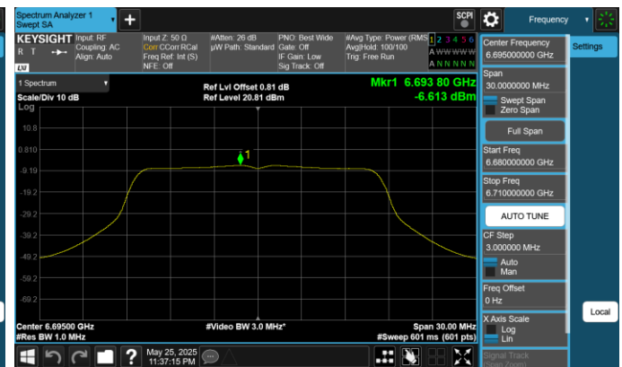
Plot 7-51. Power Spectral Density Plot Antenna 0 (20MHz 802.11ax (UNII Band 7) – Ch. 149, 54Mbps)
