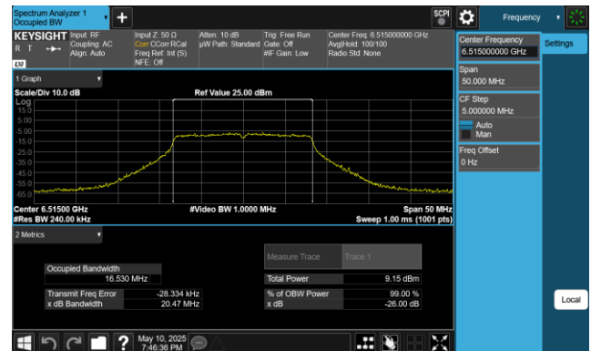
Plot 7-6. 26dB & 99% Bandwidth Plot Antenna 0 (20MHz 802.11a (UNII Band 6) – Ch. 113, 12Mbps)
