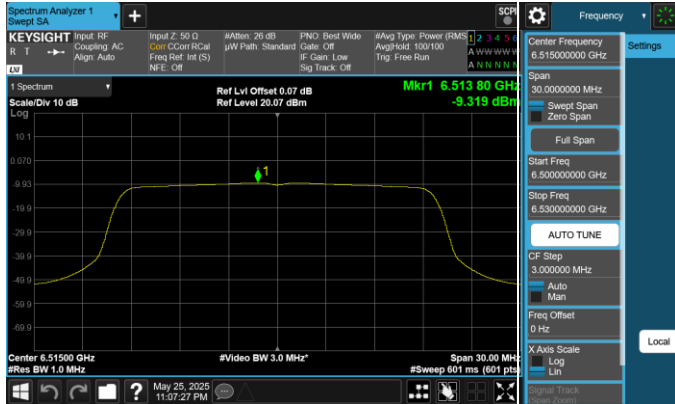
Plot 7-47. Power Spectral Density Plot Antenna 0 (20MHz 802.11ax (UNII Band 6) – Ch. 113, MCS4)
