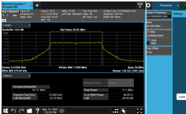
Plot 7-2. 26dB & 99% Bandwidth Plot Antenna 0 (20MHz 802.11ax (UNII Band 5) – Ch. 93, MCS11)
