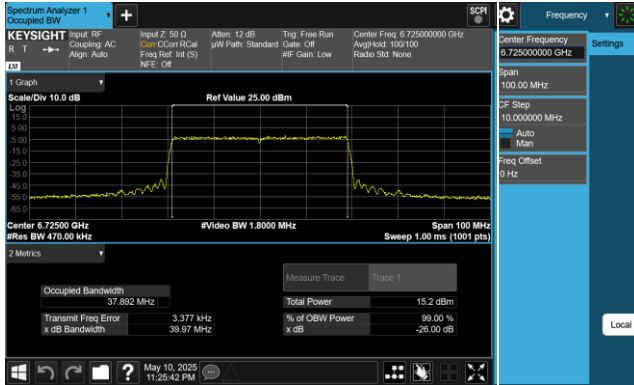
Plot 7-33. 26dB & 99% Bandwidth Plot Antenna 1 (40MHz 802.11ax (UNII Band 7) – Ch. 155, MCS11)
