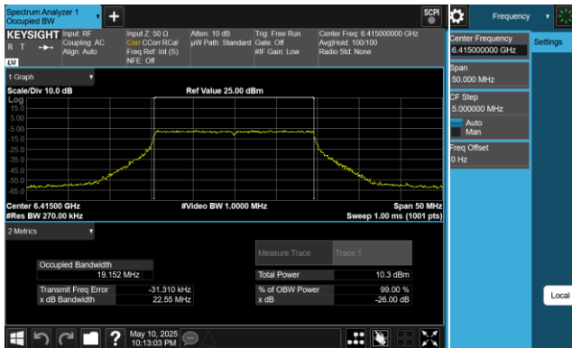
Plot 7-22. 26dB & 99% Bandwidth Plot Antenna 1 (20MHz 802.11ax (UNII Band 5) – Ch. 93, MCS11)
