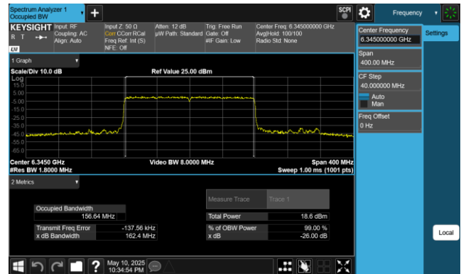
Plot 7-25. 26dB & 99% Bandwidth Plot Antenna 1 (160MHz 802.11ax (UNII Band 5) – Ch. 79, MCS11)
