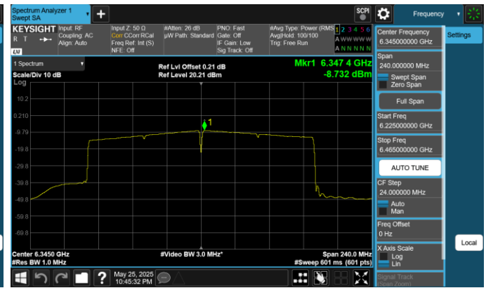
Plot 7-45. Power Spectral Density Plot Antenna 0 (160MHz 802.11ax (UNII Band 5) – Ch. 79, MCS4)
