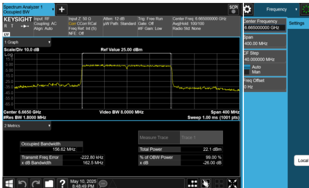
Plot 7-15. 26dB & 99% Bandwidth Plot Antenna 0 (160MHz 802.11ax (UNII Band 7) – Ch. 143, MCS11)
