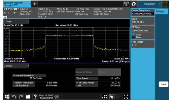
Plot 7-24. 26dB & 99% Bandwidth Plot Antenna 1 (80MHz 802.11ax (UNII Band 5) – Ch. 71, MCS11)
