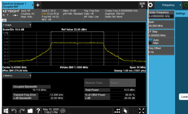
Plot 7-7. 26dB & 99% Bandwidth Plot Antenna 0 (20MHz 802.11ax (UNII Band 6) – Ch. 97, MCS11)
