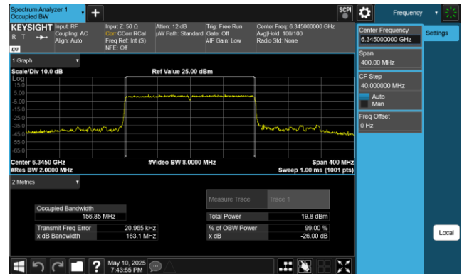
Plot 7-5. 26dB & 99% Bandwidth Plot Antenna 0 (160MHz 802.11ax (UNII Band 5) – Ch. 79, MCS11)
