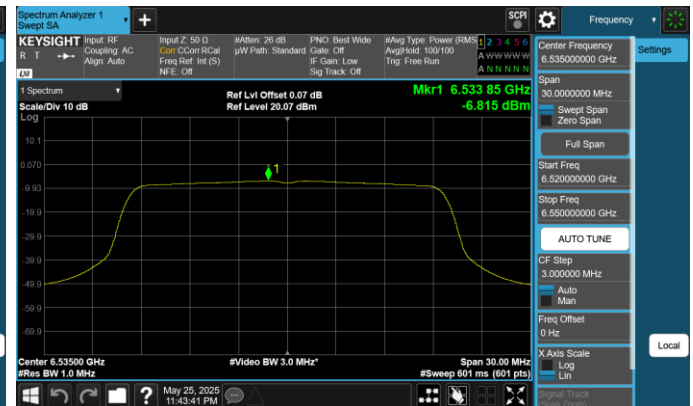
Plot 7-52. Power Spectral Density Plot Antenna 0 (20MHz 802.11ax (UNII Band 7) – Ch. 117, MCS4)
