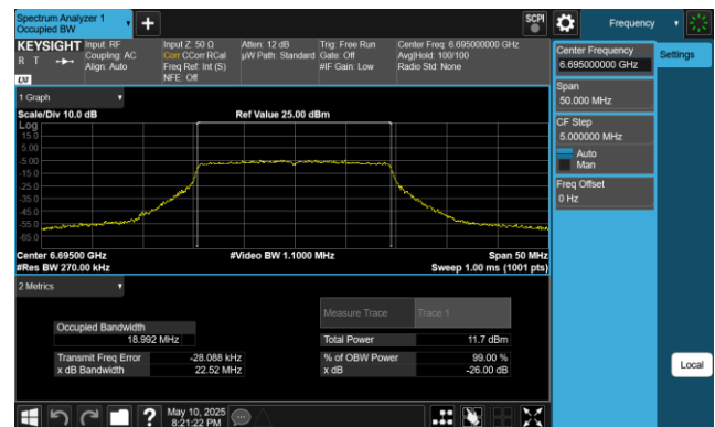
Plot 7-12. 26dB & 99% Bandwidth Plot Antenna 0 (20MHz 802.11ax (UNII Band 7) – Ch. 149, MCS2)
