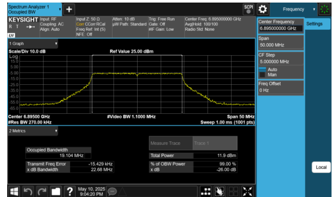
Plot 7-17. 26dB & 99% Bandwidth Plot Antenna 0 (20MHz 802.11ax (UNII Band 8) – Ch. 189, MCS11)
