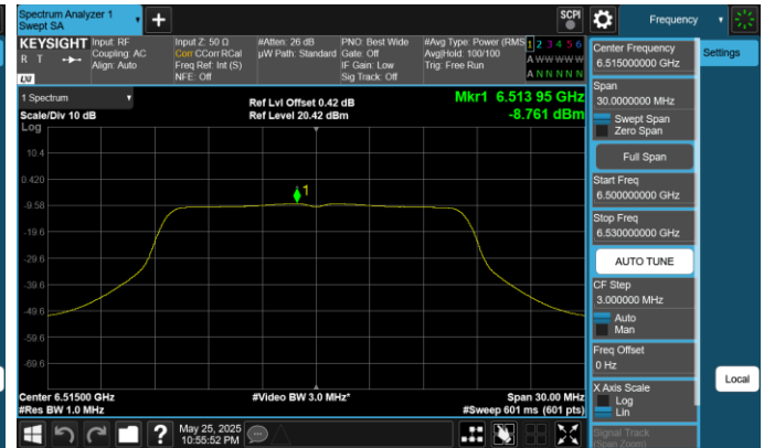
Plot 7-46. Power Spectral Density Plot Antenna 0 (20MHz 802.11a (UNII Band 6) – Ch. 113, 24Mbps)
