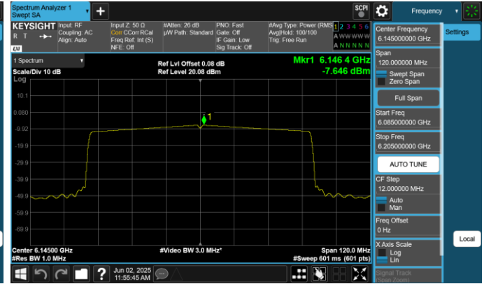
Plot 7-44. Power Spectral Density Plot Antenna 0 (80MHz 802.11ax (UNII Band 5) – Ch. 39, MCS2)
