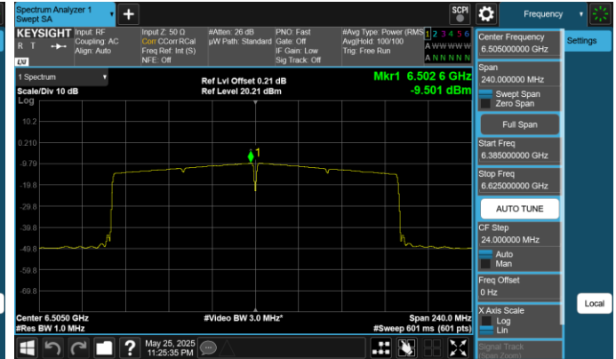
Plot 7-50. Power Spectral Density Plot Antenna 0 (160MHz 802.11ax (UNII Band 6) – Ch. 111, MCS4)
