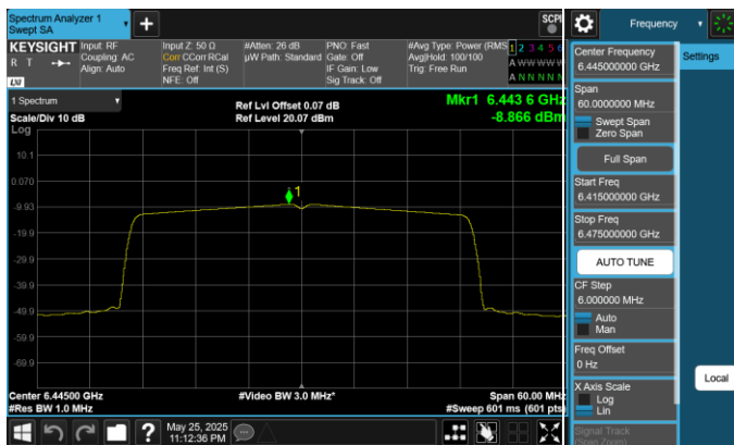
Plot 7-48. Power Spectral Density Plot Antenna 0 (40MHz 802.11ax (UNII Band 6) – Ch. 99, MCS2)
