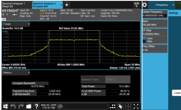
Plot 7-21. 26dB & 99% Bandwidth Plot Antenna 0 (20MHz 802.11ax (UNII Band 7) – Ch. 149)
