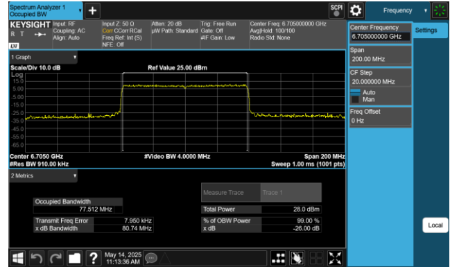
Plot 7-39. 26dB & 99% Bandwidth Plot Antenna 1 (80MHz 802.11ax (UNII Band 7) – Ch. 151)
