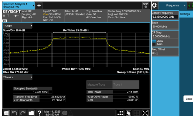
Plot 7-9. 26dB & 99% Bandwidth Plot Antenna 0 (20MHz 802.11ax (UNII Band 7) – Ch. 117)
