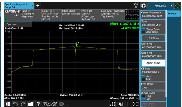
Plot 7-60. Power Spectral Density Plot Antenna 0 (160MHz 802.11ax (UNII Band 5) – Ch. 79)
