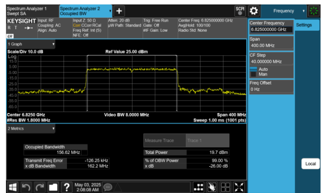
Plot 7-52. 26dB & 99% Bandwidth Plot Antenna 1 (160MHz 802.11ax (UNII Band 7) – Ch. 175)
