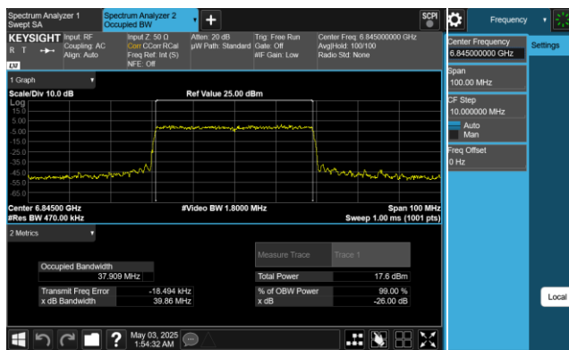
Plot 7-50. 26dB & 99% Bandwidth Plot Antenna 1 (40MHz 802.11ax (UNII Band 7) – Ch. 179)
