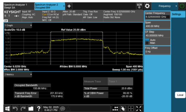
Plot 7-16. 26dB & 99% Bandwidth Plot Antenna 0 (160MHz 802.11ax (UNII Band 5) – Ch. 15)
