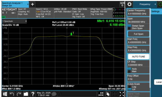
Plot 7-57. Power Spectral Density Plot Antenna 0 (20MHz 802.11a (UNII Band 5) – Ch. 93)
