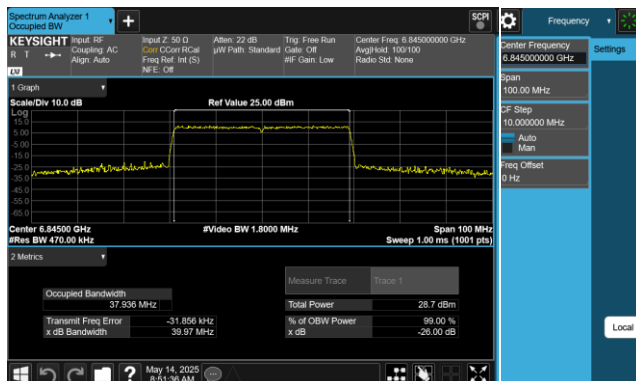
Plot 7-10. 26dB & 99% Bandwidth Plot Antenna 0 (40MHz 802.11ax (UNII Band 7) – Ch. 179)
