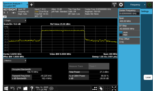
Plot 7-40. 26dB & 99% Bandwidth Plot Antenna 1 (160MHz 802.11ax (UNII Band 7) – Ch. 175)
