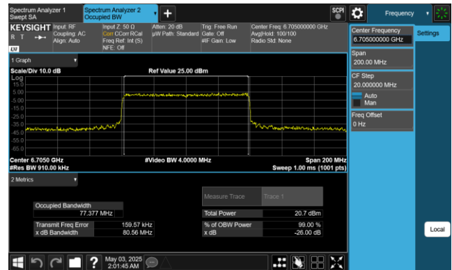
Plot 7-51. 26dB & 99% Bandwidth Plot Antenna 1 (80MHz 802.11ax (UNII Band 7) – Ch. 151)
