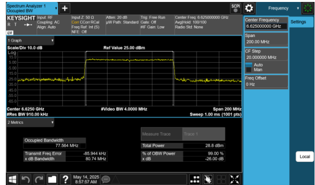
Plot 7-11. 26dB & 99% Bandwidth Plot Antenna 0 (80MHz 802.11ax (UNII Band 7) – Ch. 135)
