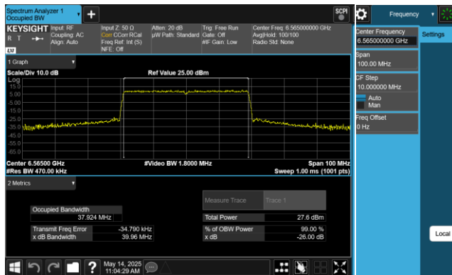
Plot 7-38. 26dB & 99% Bandwidth Plot Antenna 1 (40MHz 802.11ax (UNII Band 7) – Ch. 123)
