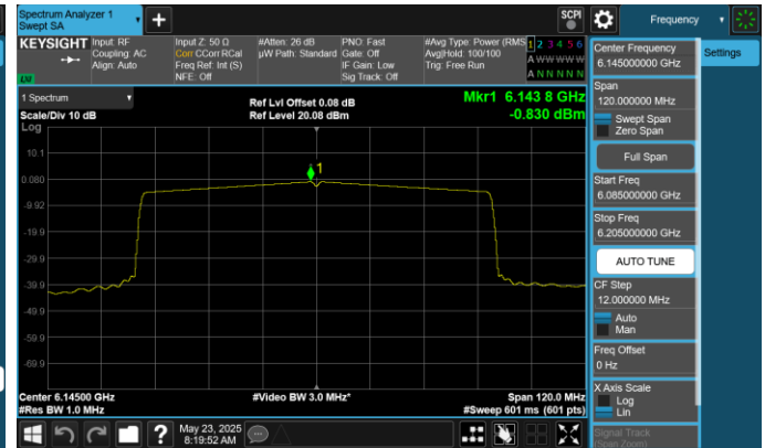
Plot 7-59. Power Spectral Density Plot Antenna 0 (80MHz 802.11ax (UNII Band 5) – Ch. 39)
