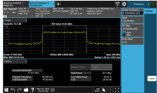
Plot 7-23. 26dB & 99% Bandwidth Plot Antenna 0 (80MHz 802.11ax (UNII Band 7) – Ch. 151)
