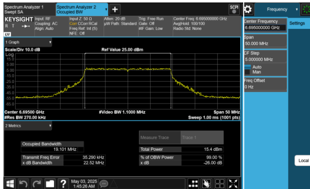
Plot 7-49. 26dB & 99% Bandwidth Plot Antenna 1 (20MHz 802.11ax (UNII Band 7) – Ch. 149)
