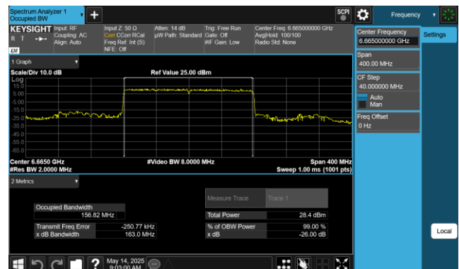
Plot 7-12. 26dB & 99% Bandwidth Plot Antenna 0 (160MHz 802.11ax (UNII Band 7) – Ch. 143)
