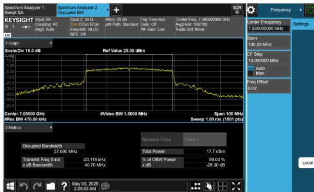
Plot 7-54. 26dB & 99% Bandwidth Plot Antenna 1 (40MHz 802.11ax (UNII Band 8) – Ch. 227)
