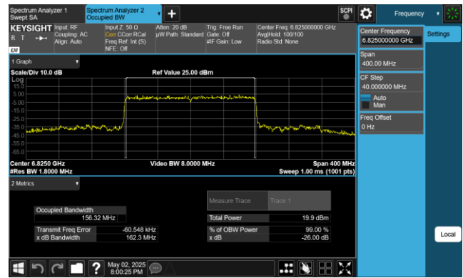
Plot 7-24. 26dB & 99% Bandwidth Plot Antenna 0 (160MHz 802.11ax (UNII Band 7) – Ch. 175)
