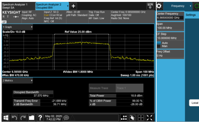
Plot 7-22. 26dB & 99% Bandwidth Plot Antenna 0 (40MHz 802.11ax (UNII Band 7) – Ch. 123)
