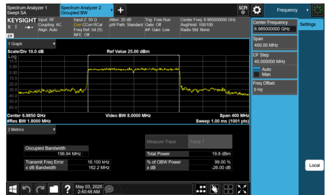
Plot 7-56. 26dB & 99% Bandwidth Plot Antenna 1 (160MHz 802.11ax (UNII Band 8) – Ch. 207)
