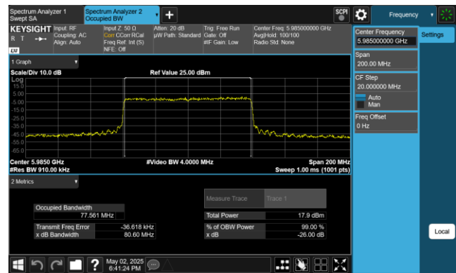
Plot 7-15. 26dB & 99% Bandwidth Plot Antenna 0 (80MHz 802.11ax (UNII Band 5) – Ch. 7)
