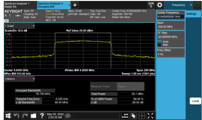
Plot 7-55. 26dB & 99% Bandwidth Plot Antenna 1 (80MHz 802.11ax (UNII Band 8) – Ch. 199)
