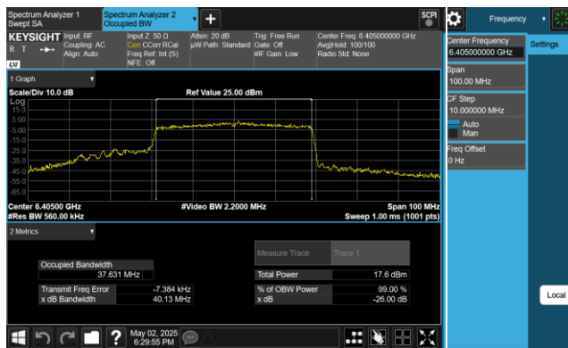
Plot 7-14. 26dB & 99% Bandwidth Plot Antenna 0 (40MHz 802.11ax (UNII Band 5) – Ch. 91)
