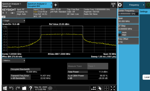
Plot 7-13. 26dB & 99% Bandwidth Plot Antenna 0 (20MHz 802.11ax (UNII Band 5) – Ch. 1)
