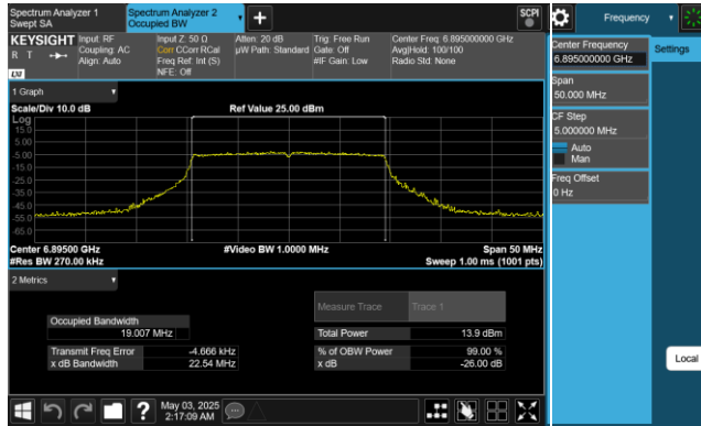
Plot 7-53. 26dB & 99% Bandwidth Plot Antenna 1 (20MHz 802.11ax (UNII Band 8) – Ch. 189)
