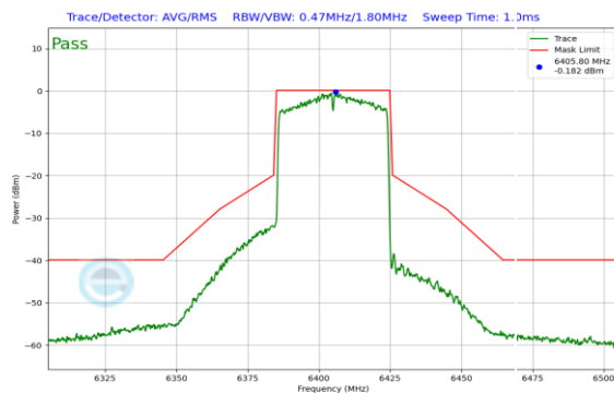
Plot 7-227. In Band Emission Plot CDD Antenna 0 (40MHz 802.11ax (UNII Band 5) – Ch. 91)
