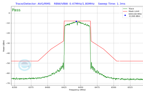
Plot 7-214. In-Band Emission Plot Antenna 1 (40MHz 802.11ax (UNII Band 6) – Ch. 99)
