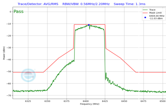
Plot 7-251. In-Band Emission Plot SDM Antenna 0 (40MHz 802.11ax (UNII Band 5) – Ch. 91)
