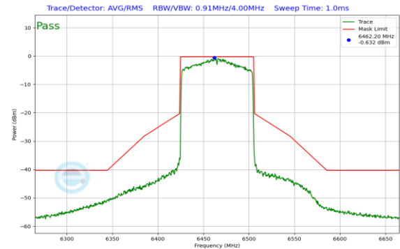
Plot 7-238. In Band Emission Plot CDD Antenna 1 (80MHz 802.11ax (UNII Band 6) – Ch. 103)
