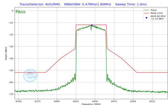
Plot 7-259. In-Band Emission Plot SDM Antenna 0 (40MHz 802.11ax (UNII Band 6) – Ch. 99)
