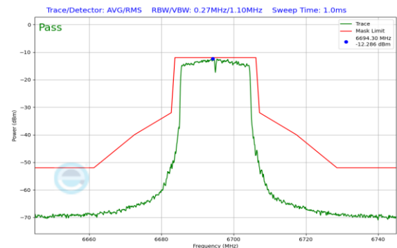
Plot 7-265. In-Band Emission Plot SDM Antenna 0 (20MHz 802.11ax (UNII Band 7) – Ch. 149)
