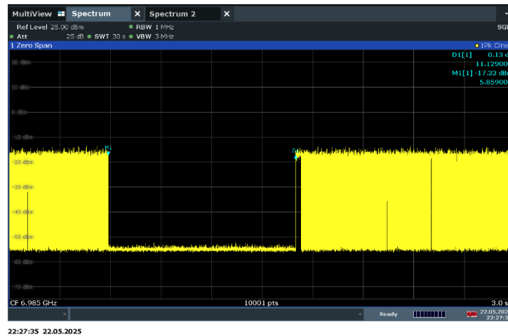
Plot 7-295. Contention Based Protocol Timing Plot – UNII 8 – 160MHz Channel 207 – Low
