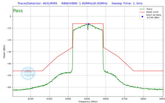
Plot 7-263. In-Band Emission Plot SDM Antenna 0 (160MHz 802.11ax (UNII Band 6) – Ch. 111)
