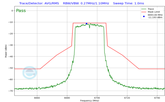
Plot 7-266. In-Band Emission Plot SDM Antenna 1 (20MHz 802.11ax (UNII Band 7) – Ch. 149)
