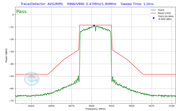
Plot 7-276. In-Band Emission Plot SDM Antenna 1 (40MHz 802.11ax (UNII Band 8) – Ch. 211)
