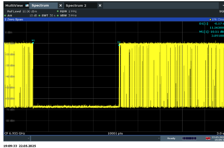
Plot 7-294. Contention Based Protocol Timing Plot – UNII 8 – 20MHz Channel 197
