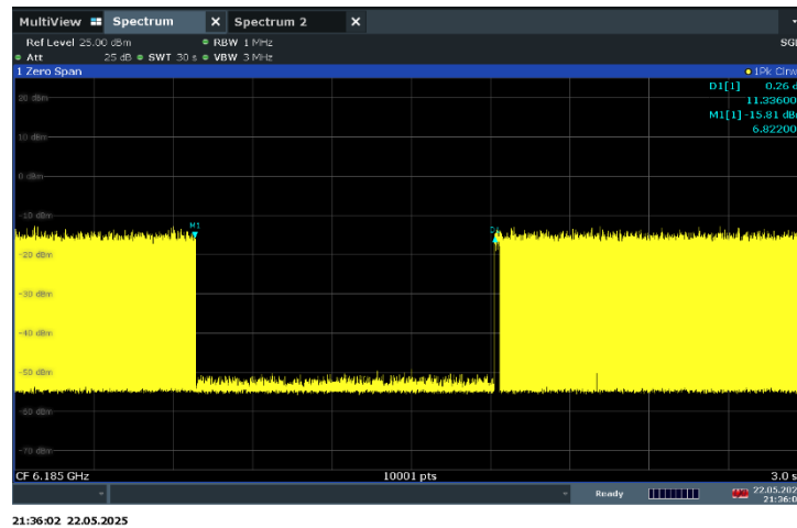
Plot 7-283. Contention Based Protocol Timing Plot – UNII 5 – 160MHz Channel 47 – Low
