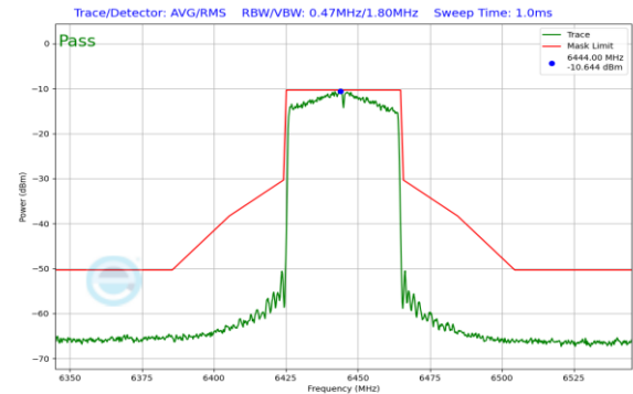
Plot 7-260. In-Band Emission Plot SDM Antenna 1 (40MHz 802.11ax (UNII Band 6) – Ch. 99)
