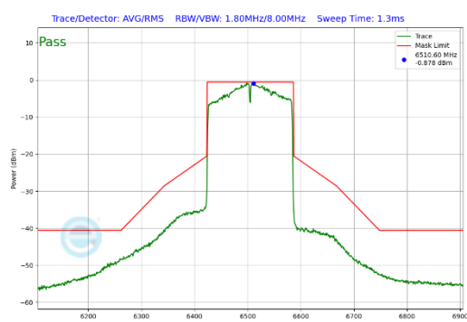
Plot 7-240. In Band Emission Plot CDD Antenna 1 (160MHz 802.11ax (UNII Band 6) – Ch. 111)
