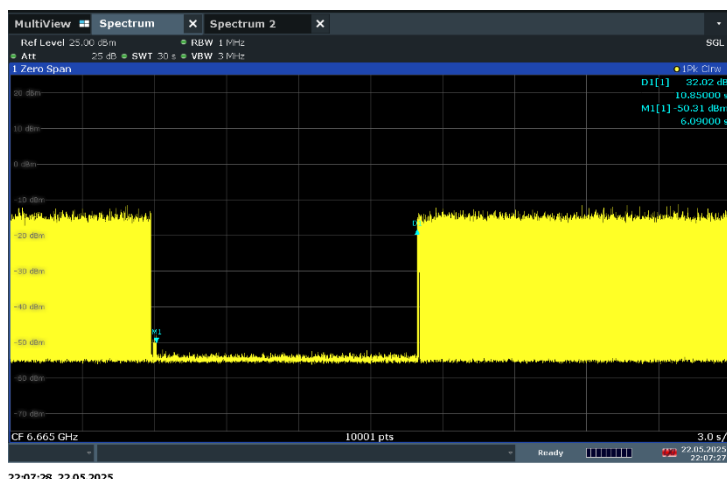
Plot 7-292. Contention Based Protocol Timing Plot – UNII 7 – 160MHz Channel 143 – Mid
