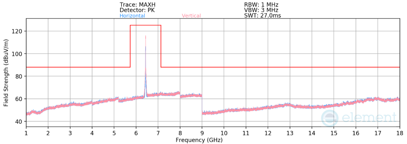
Plot 7-305. Radiated Spurious Emissions 1-18GHz SDM (802.11ax – Ch. 97)
