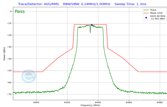
Plot 7-213. In-Band Emission Plot Antenna 1 (20MHz 802.11a (UNII Band 6) – Ch. 97)
