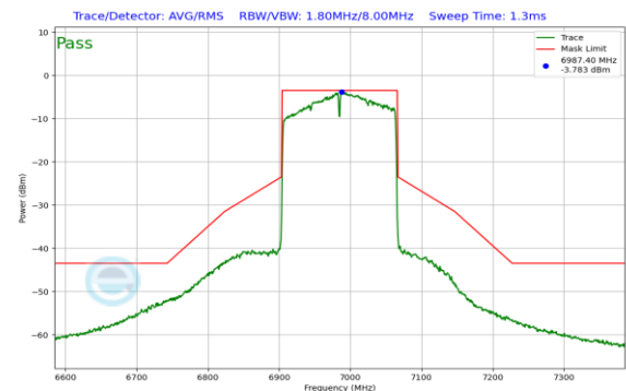
Plot 7-280. In-Band Emission Plot SDM Antenna 1 (160MHz 802.11ax (UNII Band 8) – Ch. 207)
