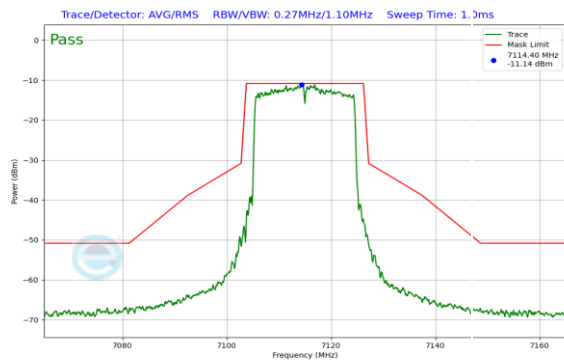
Plot 7-274. In-Band Emission Plot SDM Antenna 1 (20MHz 802.11ax (UNII Band 8) – Ch. 233)
