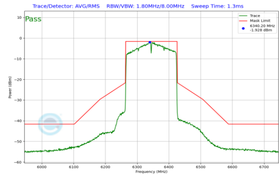
Plot 7-212. In-Band Emission Plot Antenna 1 (160MHz 802.11ax (UNII Band 5) – Ch. 79)
