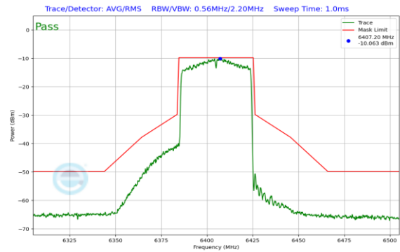
Plot 7-252. In-Band Emission Plot SDM Antenna 1 (40MHz 802.11ax (UNII Band 5) – Ch. 91)
