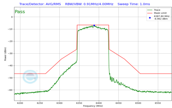
Plot 7-254. In-Band Emission Plot SDM Antenna 1 (80MHz 802.11ax (UNII Band 5) – Ch. 87)
