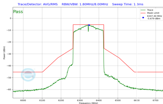
Plot 7-256. In-Band Emission Plot SDM Antenna 1 (160MHz 802.11ax (UNII Band 5) – Ch. 79)
