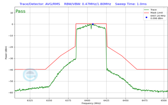
Plot 7-228. In Band Emission Plot CDD Antenna 1 (40MHz 802.11ax (UNII Band 5) – Ch. 91)
