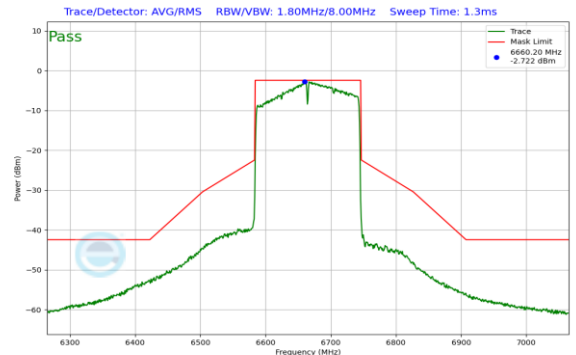
Plot 7-272. In-Band Emission Plot SDM Antenna 1 (160MHz 802.11ax (UNII Band 7) – Ch. 143)
