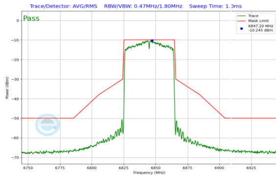
Plot 7-267. In-Band Emission Plot SDM Antenna 0 (40MHz 802.11ax (UNII Band 7) – Ch. 179)
