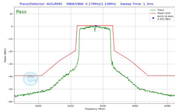
Plot 7-233. In Band Emission Plot CDD Antenna 0 (20MHz 802.11ax (UNII Band 6) – Ch. 97)
