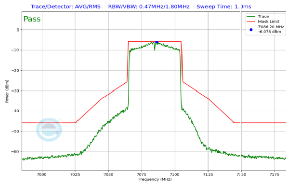
Plot 7-222. In-Band Emission Plot Antenna 1 (40MHz 802.11ax (UNII Band 8) – Ch. 227)
