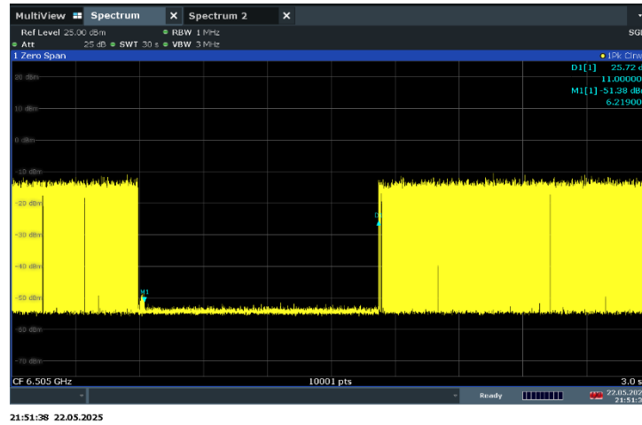
Plot 7-288. Contention Based Protocol Timing Plot – UNII 6 – 160MHz Channel 111 – Mid
