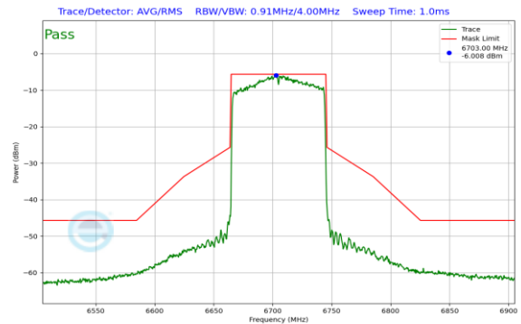
Plot 7-270. In-Band Emission Plot SDM Antenna 1 (80MHz 802.11ax (UNII Band 7) – Ch. 151)
