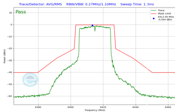
Plot 7-225. In Band Emission Plot CDD Antenna 0 (20MHz 802.11ax (UNII Band 5) – Ch. 93)
