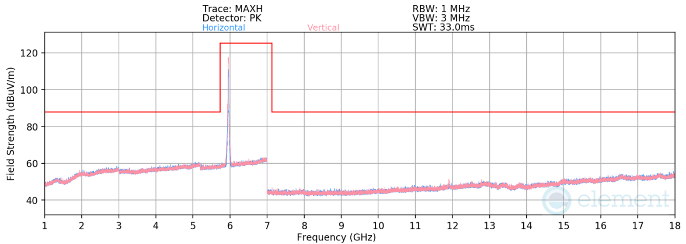
Plot 7-301. Radiated Spurious Emissions 1-18GHz SDM (802.11ax – Ch. 1)
