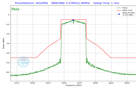
Plot 7-218. In-Band Emission Plot Antenna 1 (40MHz 802.11ax (UNII Band 7) – Ch. 123)
