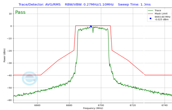
Plot 7-242. In Band Emission Plot CDD Antenna 1 (20MHz 802.11ax (UNII Band 7) – Ch. 149)
