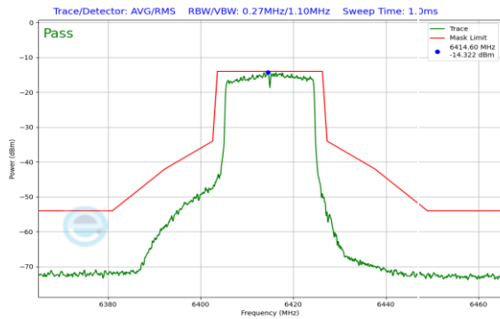
Plot 7-249. In-Band Emission Plot SDM Antenna 0 (20MHz 802.11ax (UNII Band 5) – Ch. 93)
