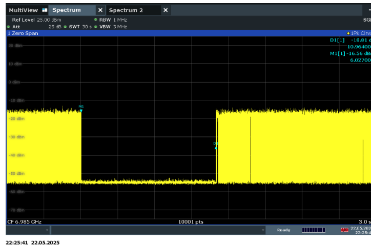
Plot 7-296. Contention Based Protocol Timing Plot – UNII 8 – 160MHz Channel 207 – Mid
