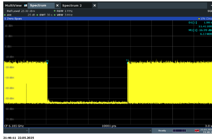
Plot 7-285. Contention Based Protocol Timing Plot – UNII 5 – 160MHz Channel 47 – High
