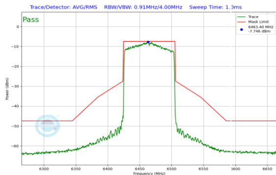
Plot 7-262. In-Band Emission Plot SDM Antenna 1 (80MHz 802.11ax (UNII Band 6) – Ch. 103)
