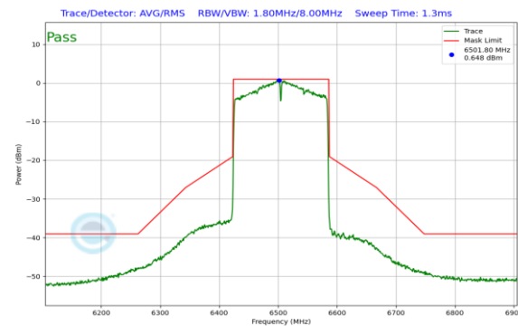
Plot 7-216. In-Band Emission Plot Antenna 1 (160MHz 802.11ax (UNII Band 6) – Ch. 111)
