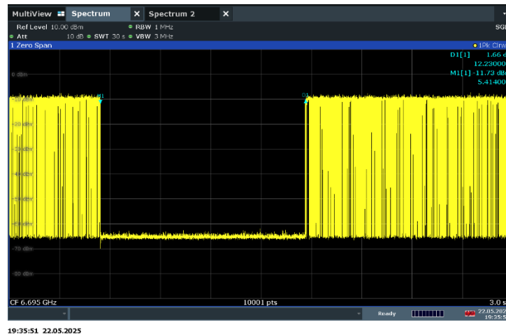
Plot 7-290. Contention Based Protocol Timing Plot – UNII 7 – 20MHz Channel 149
