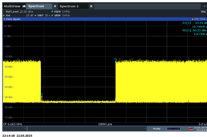
Plot 7-293. Contention Based Protocol Timing Plot – UNII 7 – 160MHz Channel 143 – High
