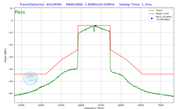
Plot 7-271. In-Band Emission Plot SDM Antenna 0 (160MHz 802.11ax (UNII Band 7) – Ch. 143)
