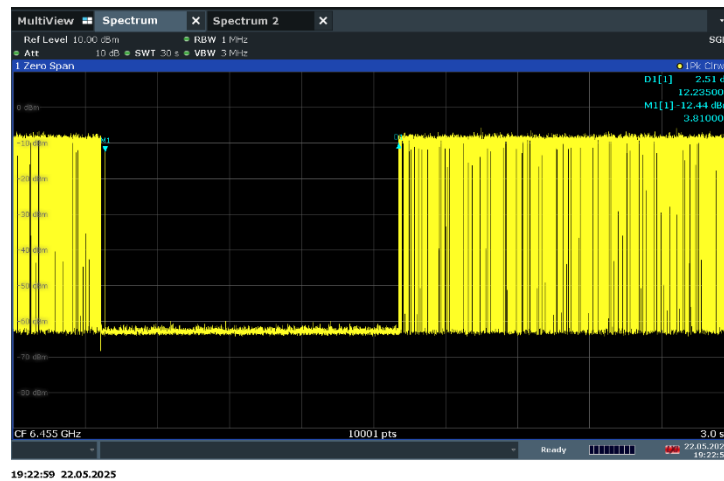
Plot 7-286. Contention Based Protocol Timing Plot – UNII 6 – 20MHz Channel 101
