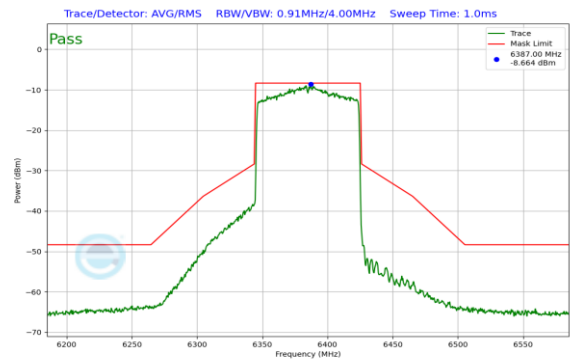
Plot 7-253. In-Band Emission Plot SDM Antenna 0 (80MHz 802.11ax (UNII Band 5) – Ch. 87)
