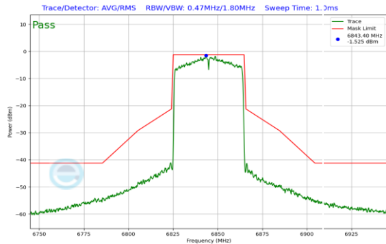
Plot 7-243. In Band Emission Plot CDD Antenna 0 (40MHz 802.11ax (UNII Band 7) – Ch. 179)
