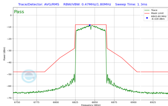
Plot 7-268. In-Band Emission Plot SDM Antenna 1 (40MHz 802.11ax (UNII Band 7) – Ch. 179)
