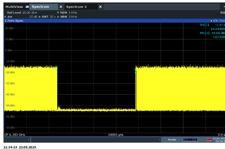
Plot 7-284. Contention Based Protocol Timing Plot –UNII 5 – 160MHz Channel 47 – Mid
