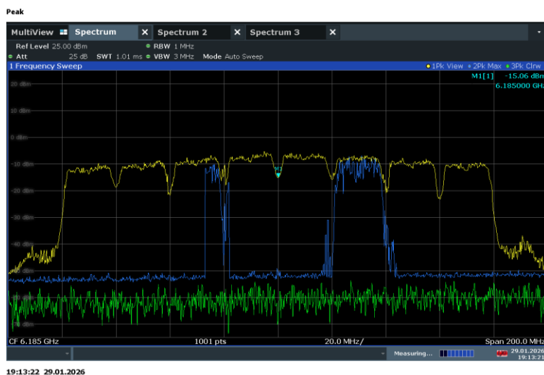
Plot 7-299. 160MHz Bandwidth, AWGN Signal Injected – 6185Mhz
