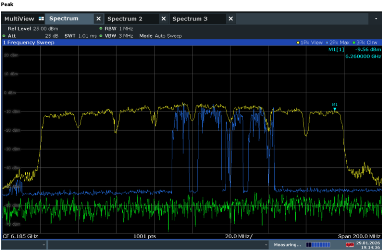
Plot 7-300. 160MHz Bandwidth, AWGN Signal Injected – 6260Mhz
