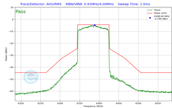
Plot 7-211. In-Band Emission Plot Antenna 1 (80MHz 802.11ax (UNII Band 5) – Ch. 87)
