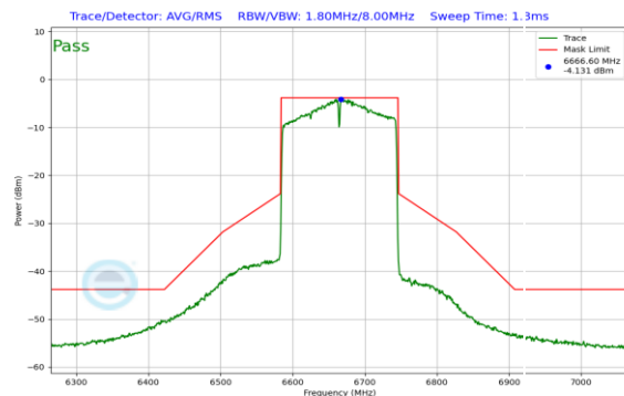
Plot 7-247. In Band Emission Plot CDD Antenna 0 (160MHz 802.11ax (UNII Band 7) – Ch. 143)
