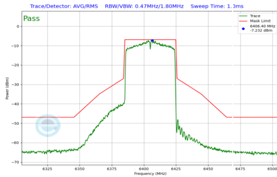
Plot 7-210. In-Band Emission Plot Antenna 1 (40MHz 802.11ax (UNII Band 5) – Ch. 91)
