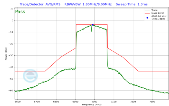
Plot 7-224. In-Band Emission Plot Antenna 1 (160MHz 802.11ax (UNII Band 8) – Ch. 207)
