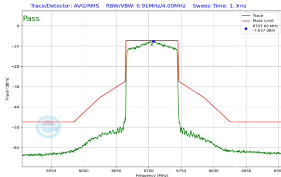
Plot 7-269. In-Band Emission Plot SDM Antenna 0 (80MHz 802.11ax (UNII Band 7) – Ch. 151)
