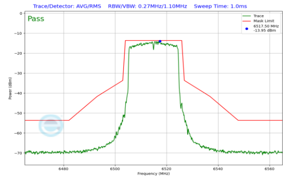
Plot 7-258. In-Band Emission Plot SDM Antenna 1 (20MHz 802.11ax (UNII Band 6) – Ch. 113)
