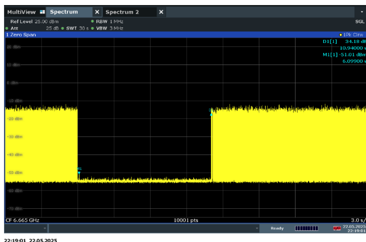
Plot 7-291. Contention Based Protocol Timing Plot – UNII 7 – 160MHz Channel 143 – Low
