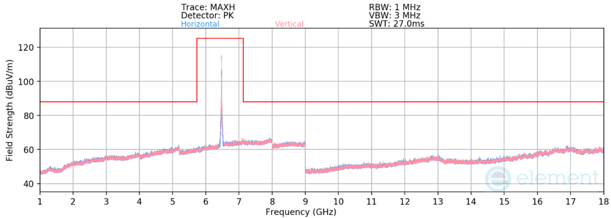
Plot 7-306. Radiated Spurious Emissions 1-18GHz SDM (802.11ax – Ch. 105)
