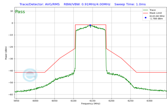
Plot 7-229. In Band Emission Plot CDD Antenna 0 (80MHz 802.11ax (UNII Band 5) – Ch. 39)
