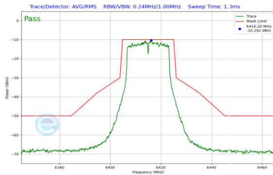
Plot 7-209. In-Band Emission Plot Antenna 1 (20MHz 802.11a (UNII Band 5) – Ch. 93)
