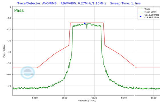
Plot 7-257. In-Band Emission Plot SDM Antenna 0 (20MHz 802.11ax (UNII Band 6) – Ch. 113)
