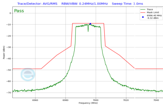
Plot 7-221. In-Band Emission Plot Antenna 1 (20MHz 802.11a (UNII Band 8) – Ch. 209)
