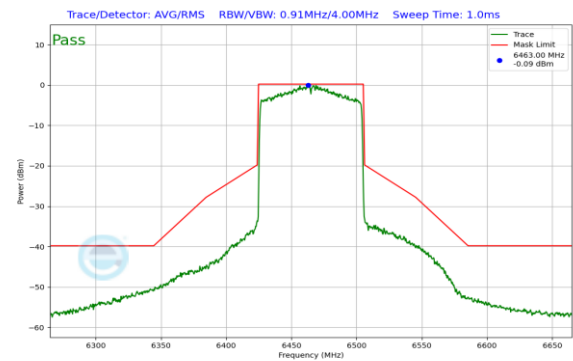
Plot 7-237. In Band Emission Plot CDD Antenna 0 (80MHz 802.11ax (UNII Band 6) – Ch. 103)
