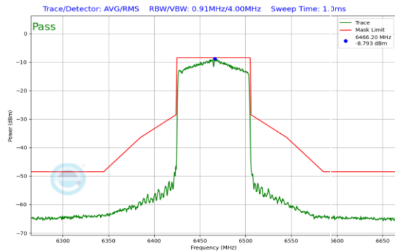
Plot 7-261. In-Band Emission Plot SDM Antenna 0 (80MHz 802.11ax (UNII Band 6) – Ch. 103)
