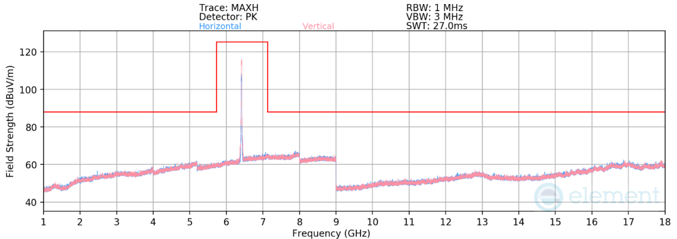
Plot 7-304. Radiated Spurious Emissions 1-18GHz SDM (802.11ax – Ch. 93)
