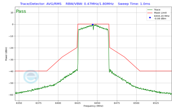
Plot 7-236. In Band Emission Plot CDD Antenna 1 (40MHz 802.11ax (UNII Band 6) – Ch. 99)
