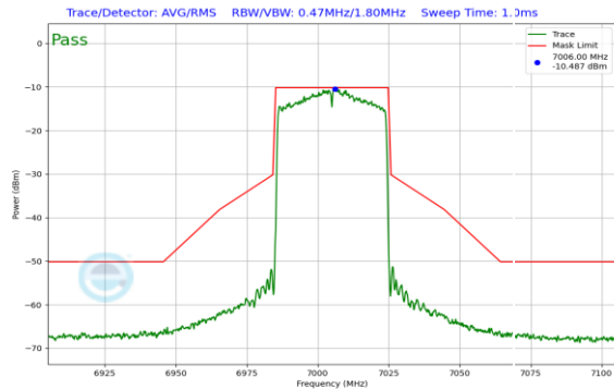
Plot 7-275. In-Band Emission Plot SDM Antenna 0 (40MHz 802.11ax (UNII Band 8) – Ch. 211)
