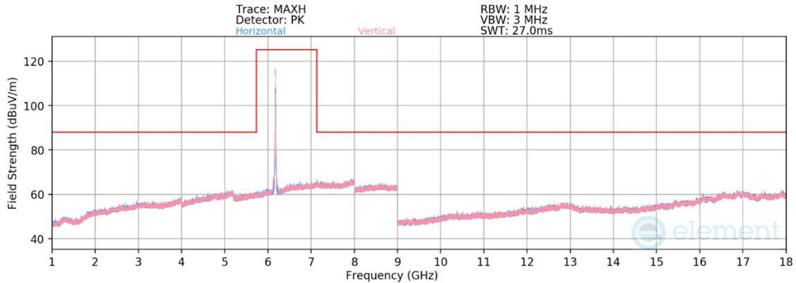
Plot 7-302. Radiated Spurious Emissions 1-18GHz SDM (802.11ax – Ch. 45)
