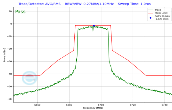
Plot 7-241. In Band Emission Plot CDD Antenna 0 (20MHz 802.11ax (UNII Band 7) – Ch. 149)
