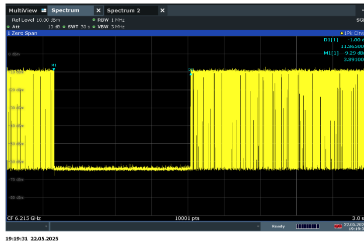
Plot 7-282. Contention Based Protocol Timing Plot – UNII 5 – 20MHz Channel 53
