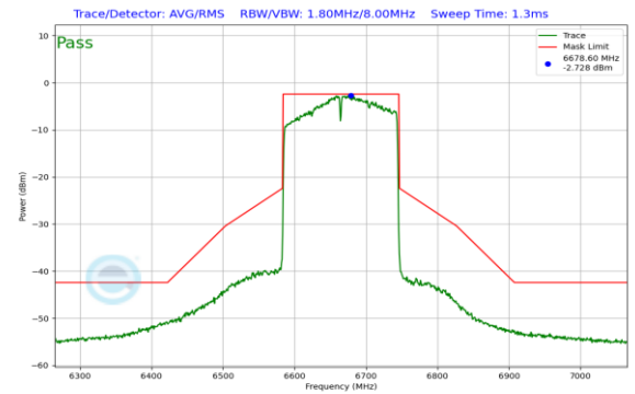
Plot 7-220. In-Band Emission Plot Antenna 1 (160MHz 802.11ax (UNII Band 7) – Ch. 143)
