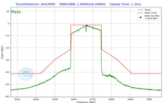
Plot 7-248. In Band Emission Plot CDD Antenna 1 (160MHz 802.11ax (UNII Band 7) – Ch. 143)
