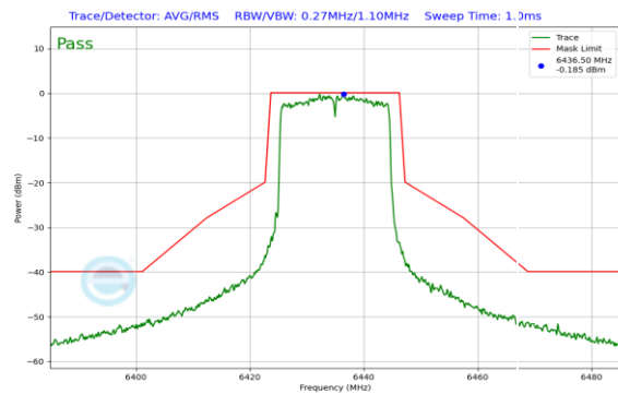
Plot 7-234. In Band Emission Plot CDD Antenna 1 (20MHz 802.11ax (UNII Band 6) – Ch. 97)
