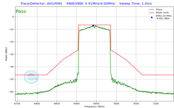
Plot 7-278. In-Band Emission Plot SDM Antenna 1 (80MHz 802.11ax (UNII Band 8) – Ch. 199)
