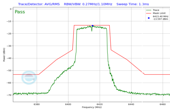
Plot 7-250. In-Band Emission Plot SDM Antenna 1 (20MHz 802.11ax (UNII Band 5) – Ch. 93)
