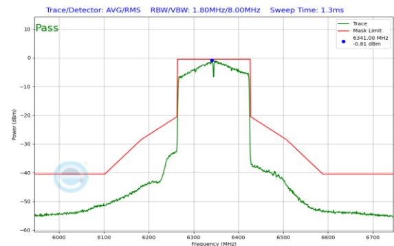
Plot 7-232. In Band Emission Plot CDD Antenna 1 (160MHz 802.11ax (UNII Band 5) – Ch. 79)
