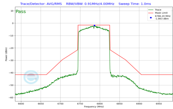
Plot 7-245. In Band Emission Plot CDD Antenna 0 (80MHz 802.11ax (UNII Band 7) – Ch. 167)
