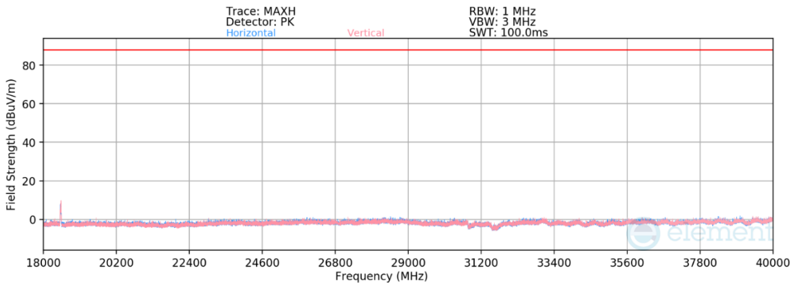
Plot 7-303. Radiated Spurious Emissions 18-40GHz SDM (802.11ax – Ch. 45)
