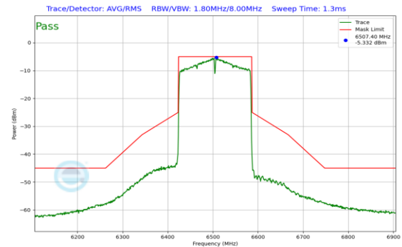
Plot 7-264. In-Band Emission Plot SDM Antenna 1 (160MHz 802.11ax (UNII Band 6) – Ch. 111)
