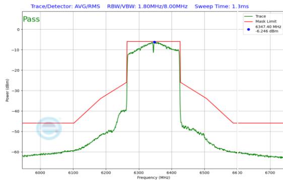
Plot 7-255. In-Band Emission Plot SDM Antenna 0 (160MHz 802.11ax (UNII Band 5) – Ch. 79)
