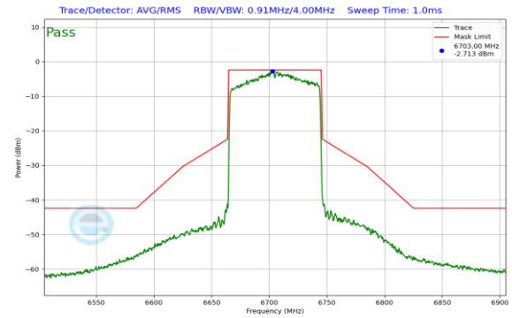
Plot 7-219. In-Band Emission Plot Antenna 1 (80MHz 802.11ax (UNII Band 7) – Ch. 151)
