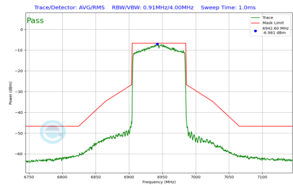
Plot 7-277. In-Band Emission Plot SDM Antenna 0 (80MHz 802.11ax (UNII Band 8) – Ch. 199)
