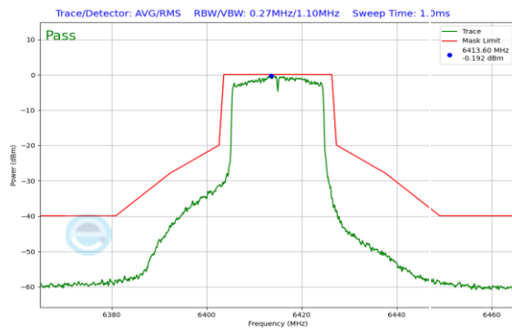
Plot 7-226. In Band Emission Plot CDD Antenna 1 (20MHz 802.11ax (UNII Band 5) – Ch. 93)
