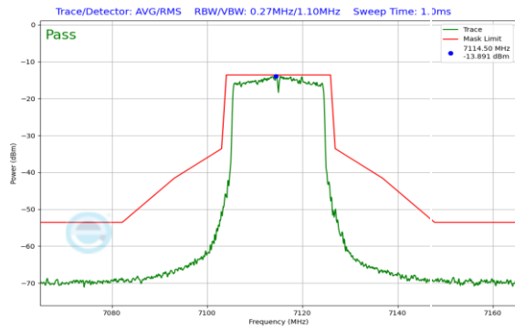
Plot 7-273. In-Band Emission Plot SDM Antenna 0 (20MHz 802.11ax (UNII Band 8) – Ch. 233)
