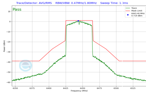
Plot 7-235. In Band Emission Plot CDD Antenna 0 (40MHz 802.11ax (UNII Band 6) – Ch. 99)
