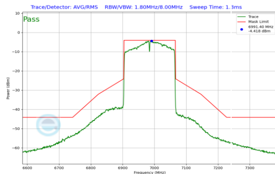
Plot 7-279. In-Band Emission Plot SDM Antenna 0 (160MHz 802.11ax (UNII Band 8) – Ch. 207)
