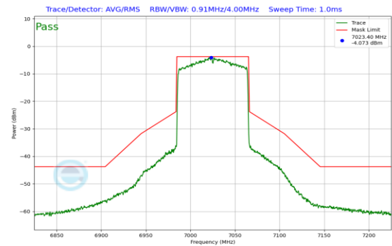
Plot 7-223. In-Band Emission Plot Antenna 1 (80MHz 802.11ax (UNII Band 8) – Ch. 215)
