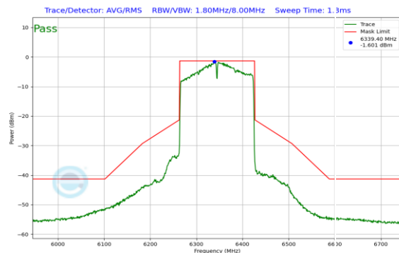
Plot 7-231. In Band Emission Plot CDD Antenna 0 (160MHz 802.11ax (UNII Band 5) – Ch. 79)
