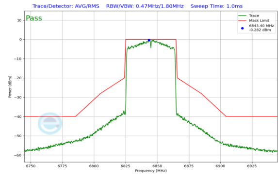
Plot 7-244. In Band Emission Plot CDD Antenna 1 (40MHz 802.11ax (UNII Band 7) – Ch. 179)
