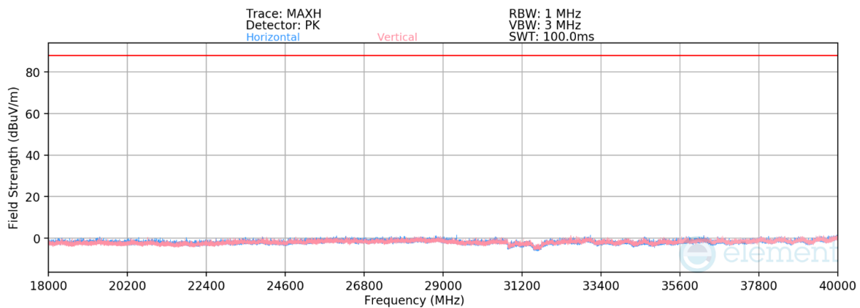
Plot 7-307. Radiated Spurious Emissions 18-40GHz SDM (802.11ax – Ch. 105)
