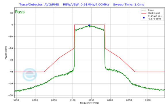
Plot 7-230. In Band Emission Plot CDD Antenna 1 (80MHz 802.11ax (UNII Band 5) – Ch. 39)
