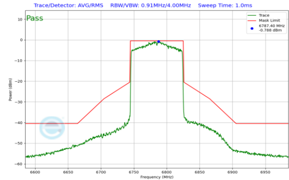
Plot 7-246. In Band Emission Plot CDD Antenna 1 (80MHz 802.11ax (UNII Band 7) – Ch. 167)
