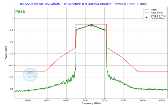
Plot 7-215. In-Band Emission Plot Antenna 1 (80MHz 802.11ax (UNII Band 6) – Ch. 103)
