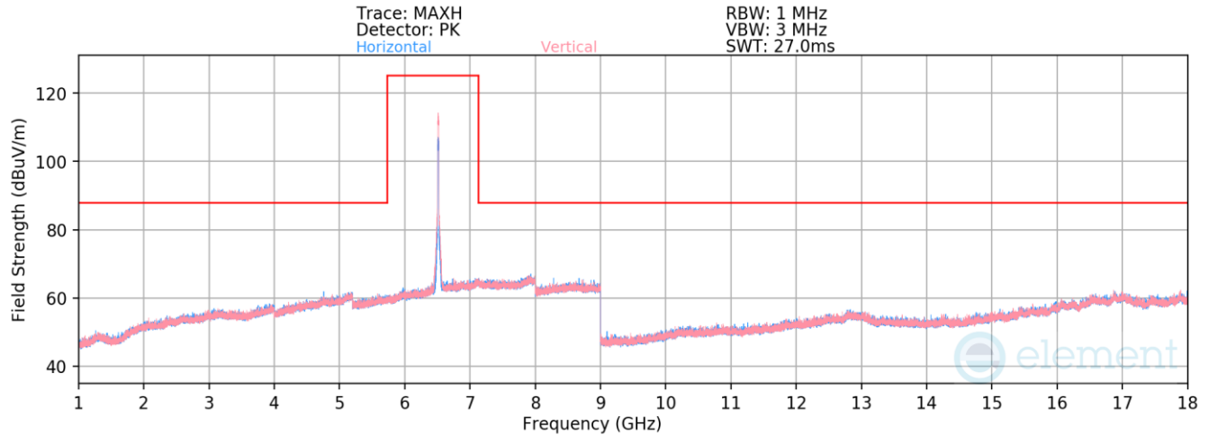
Plot 7-620. Radiated Spurious Emissions above 1GHz SDM (802.11ax – Ch. 113 – RU242)
