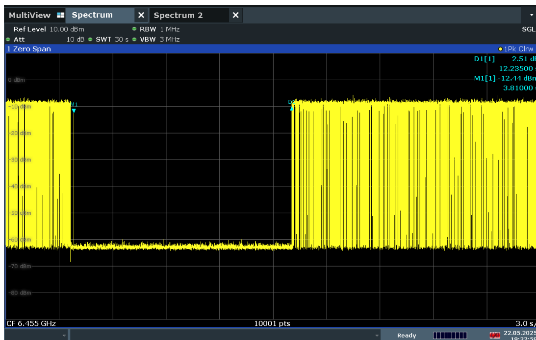
Plot 7-566. Contention Based Protocol Timing Plot – UNII 6 – 20MHz Channel 101
