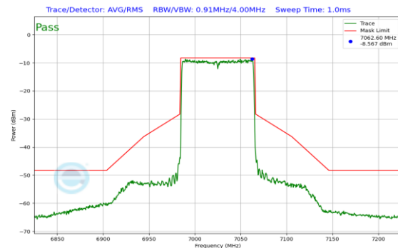
Plot 7-558. In Band Emission Plot SDM Antenna 0 (80MHz 802.11ax RU996 (UNII Band 8) – Ch. 215)
