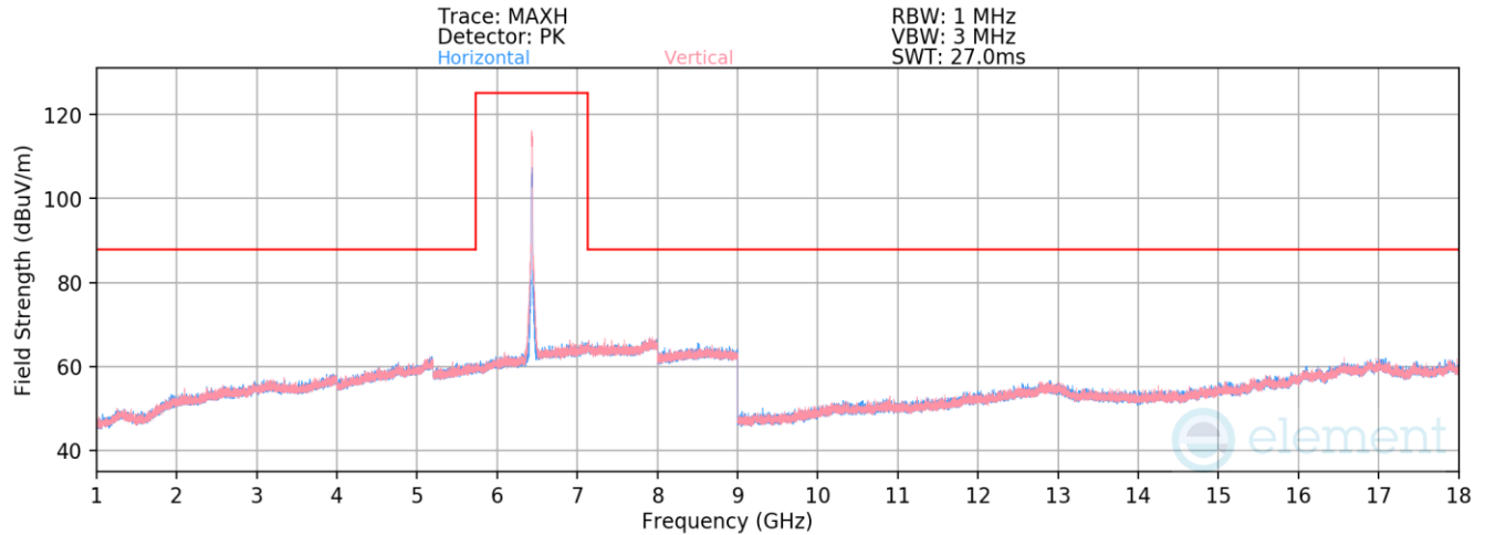
Plot 7-617. Radiated Spurious Emissions above 1GHz SDM (802.11ax – Ch. 97 – RU242)
