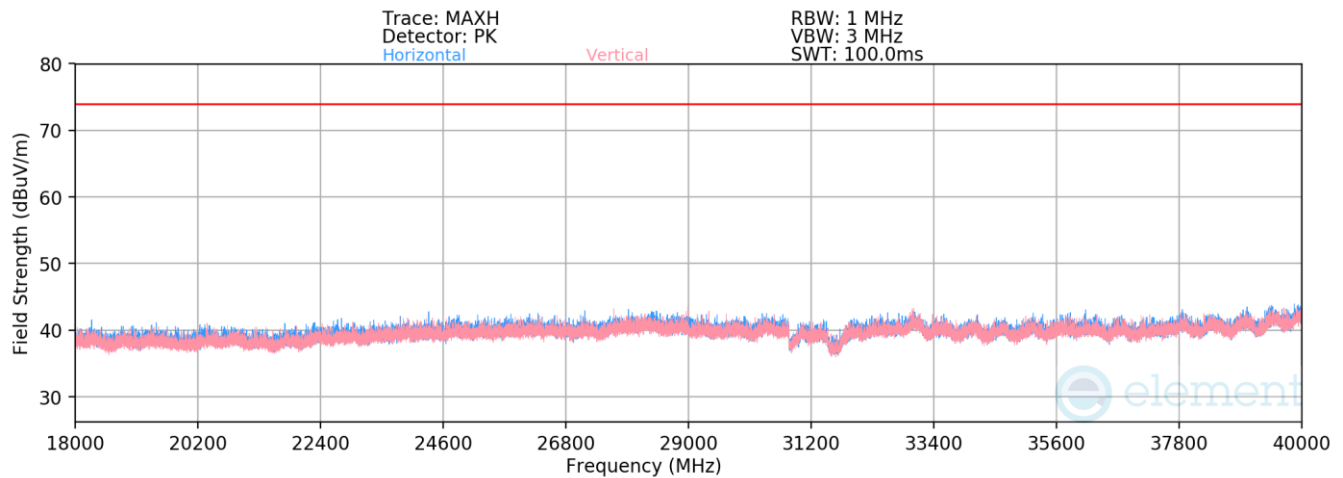
Plot 7-623. Radiated Spurious Emissions 18-40GHz SDM (802.11ax – Ch. 149 – RU242)
