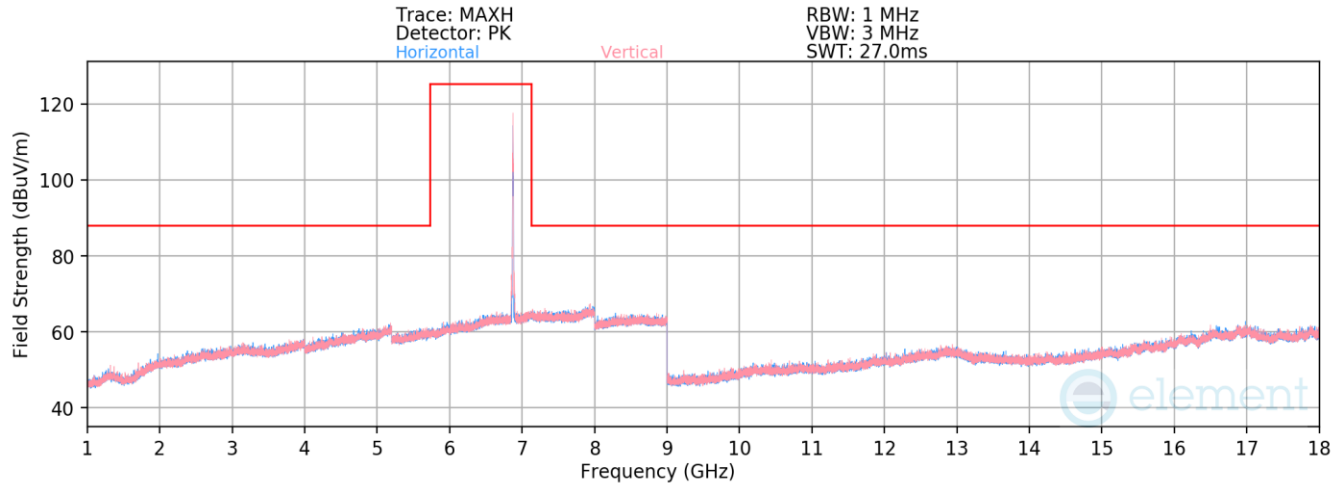
Plot 7-608. Radiated Spurious Emissions above 1GHz SDM (802.11ax – Ch. 185 – RU26)
