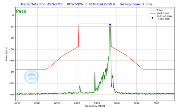
Plot 7-549. In Band Emission Plot SDM Antenna 0 (80MHz 802.11ax RU26 (UNII Band 8) – Ch. 199)
