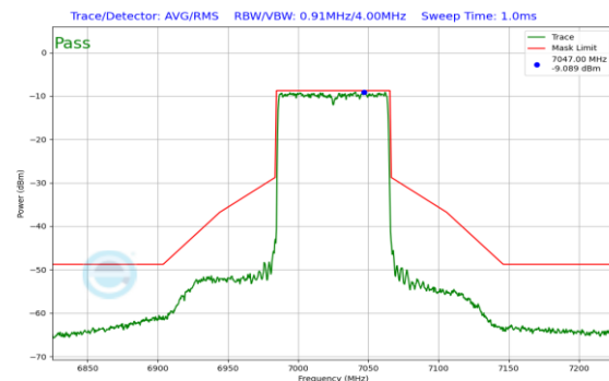
Plot 7-557. In Band Emission Plot SDM Antenna 0 (80MHz 802.11ax RU996 (UNII Band 8) – Ch. 215)
