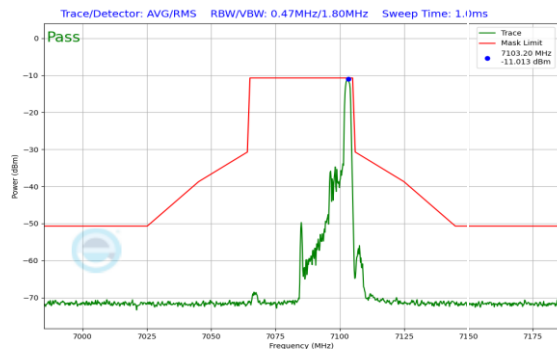
Plot 7-547. In Band Emission Plot SDM Antenna 0 (40MHz 802.11ax RU26 (UNII Band 8) – Ch. 227)
