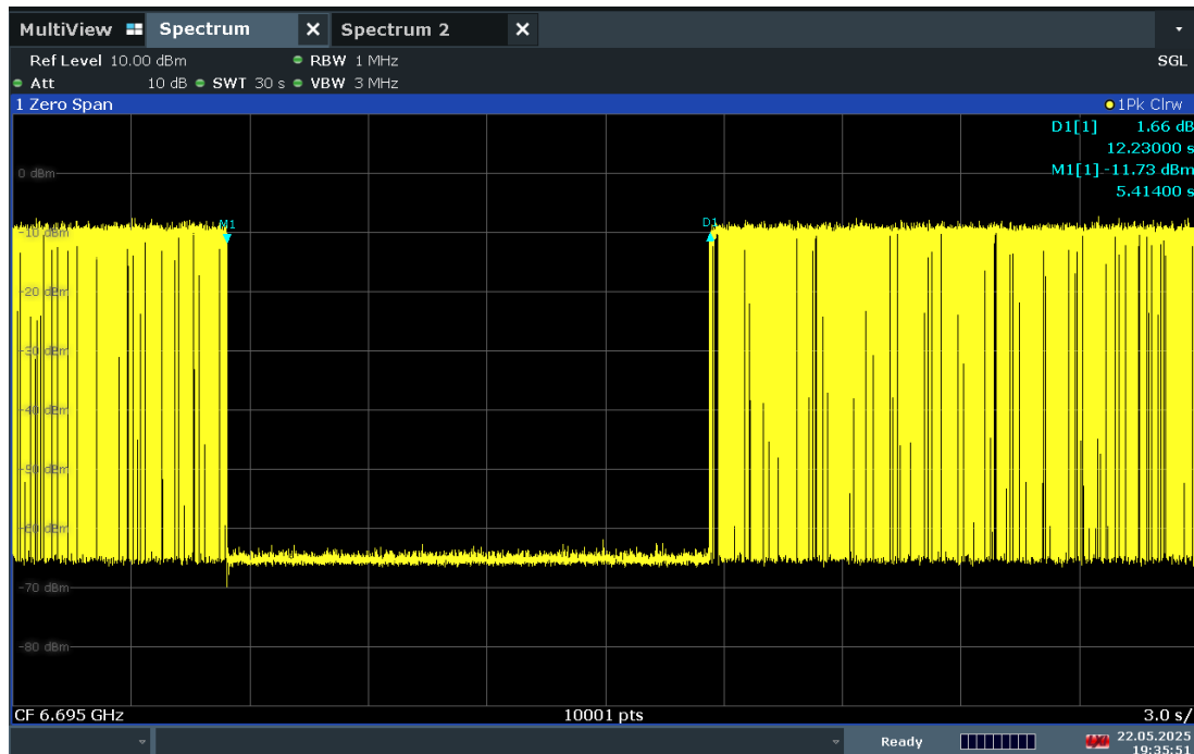
Plot 7-570. Contention Based Protocol Timing Plot – UNII 7 – 2.0MHz Channel 149
