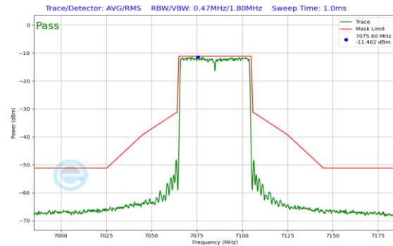
Plot 7-556. In Band Emission Plot SDM Antenna 0 (40MHz 802.11ax RU484 (UNII Band 8) – Ch. 227)
