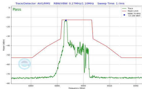
Plot 7-546. In Band Emission Plot SDM Antenna 0 (20MHz 802.11ax RU26 (UNII Band 8) – Ch. 189)
