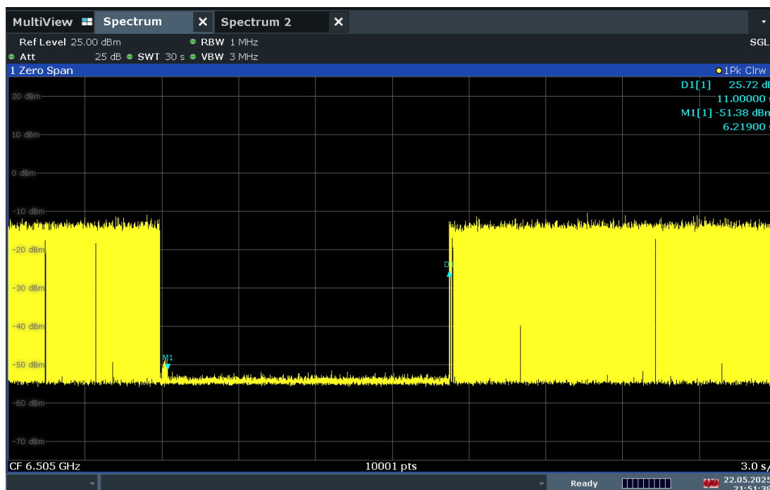
Plot 7-568. Contention Based Protocol Timing Plot – UNII 6 – 160MHz Channel 111 – Mid
