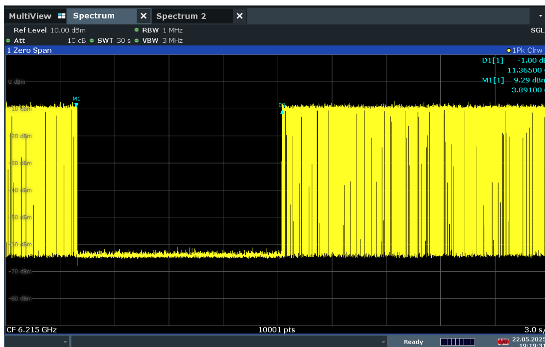
Plot 7-562. Contention Based Protocol Timing Plot – UNII 5 – 20MHz Channel 53
