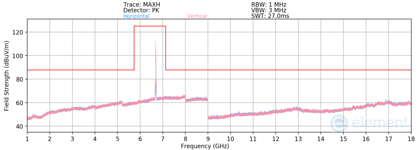
Plot 7-606. Radiated Spurious Emissions above 1GHz SDM (802.11ax – Ch. 149 – RU26)
