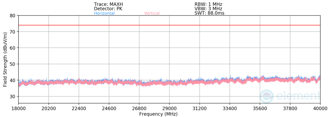
Plot 7-603. Radiated Spurious Emissions 18-40GHz SDM (802.11ax – Ch.105 – RU26)
