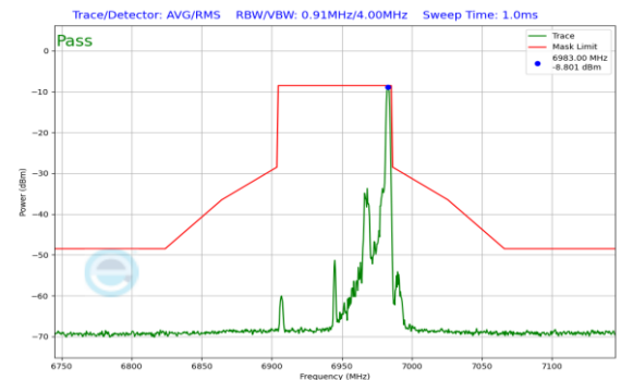
Plot 7-550. In Band Emission Plot SDM Antenna 0 (80MHz 802.11ax RU26 (UNII Band 8) – Ch. 199)
