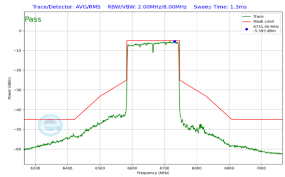
Plot 7-544. In Band Emission Plot SDM Antenna 0 (160MHz 802.11ax RU996x2 (UNII Band 7) – Ch. 143)
