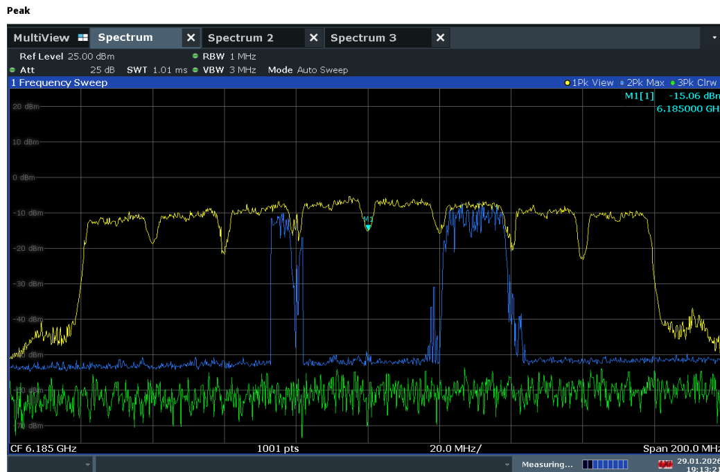
Plot 7-595. 160MHz Bandwidth, AWGN Signal Injected – 6185Mhz
