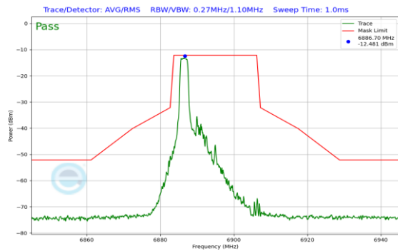
Plot 7-545. In Band Emission Plot SDM Antenna 0 (20MHz 802.11ax RU26 (UNII Band 8) – Ch. 189)
