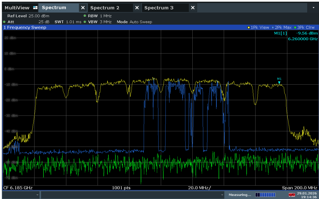
Plot 7-596. 160MHz Bandwidth, AWGN Signal Injected – 6260Mhz
