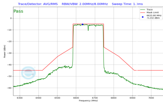
Plot 7-543. In Band Emission Plot SDM Antenna 0 (160MHz 802.11ax RU996x2 (UNII Band 7) – Ch. 143)
