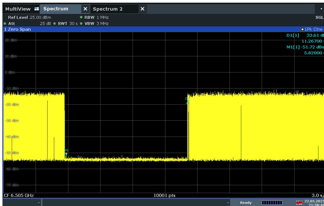
Plot 7-567. Contention Based Protocol Timing Plot – UNII 6 – 160MHz Channel 111 – Low
