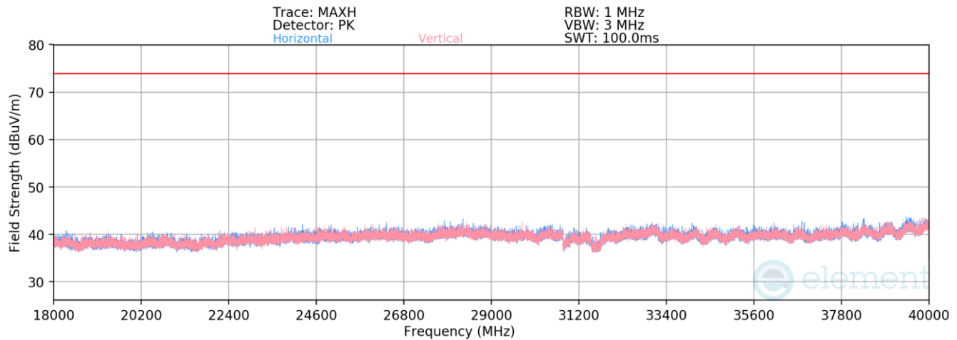
Plot 7-599. Radiated Spurious Emissions 18-40GHz SDM (802.11ax – Ch.45 – RU26)
