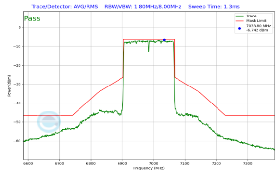
Plot 7-560. In Band Emission Plot SDM Antenna 0 (160MHz 802.11ax RU996x2 (UNII Band 8) – Ch. 207)
