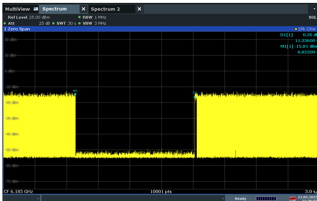
Plot 7-563. Contention Based Protocol Timing Plot – UNII 5 – 160MHz Channel 47 – Low
