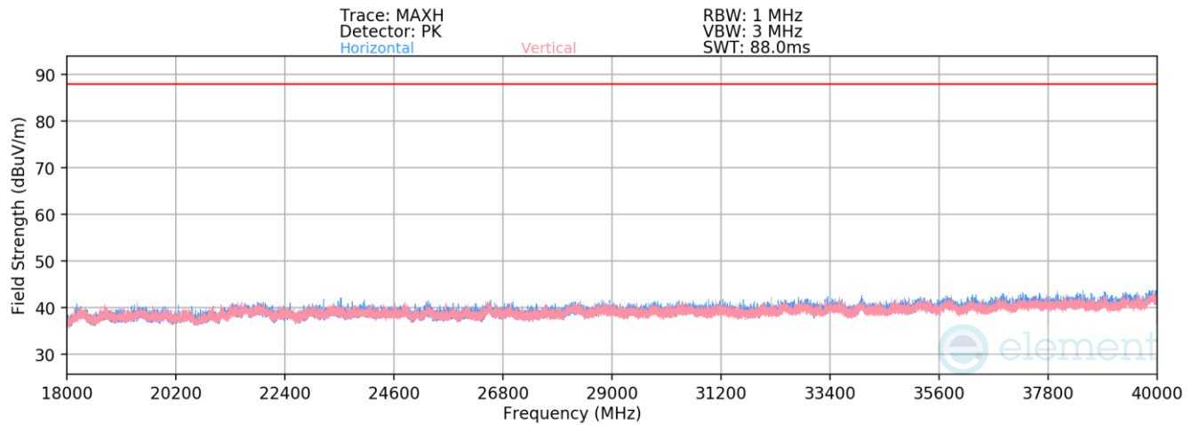
Plot 7-607. Radiated Spurious Emissions 18-40GHz SDM (802.11ax – Ch.149 – RU26)
