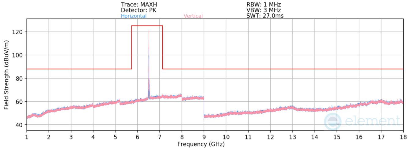
Plot 7-604. Radiated Spurious Emissions above 1GHz SDM (802.11ax – Ch. 113 – RU26)
