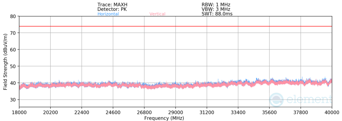
Plot 7-615. Radiated Spurious Emissions 18-40GHz SDM (802.11ax – Ch. 45 – RU242)
