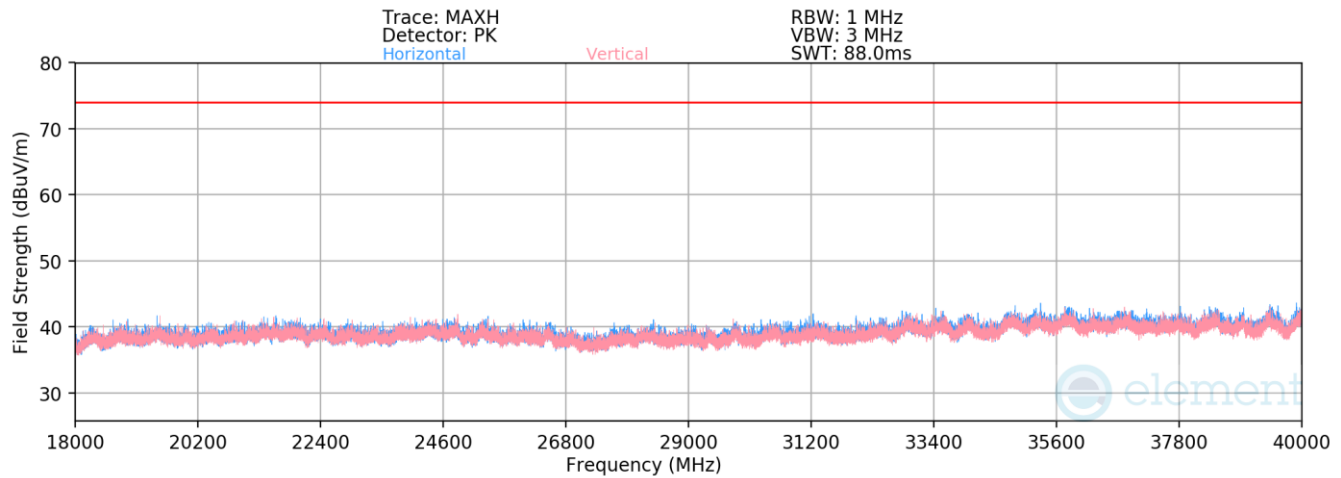
Plot 7-611. Radiated Spurious Emissions 18-40GHz SDM (802.11ax – Ch. 209 – RU26)
