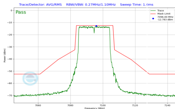
Plot 7-554. In Band Emission Plot SDM Antenna 0 (20MHz 802.11ax RU242 (UNII Band 8) – Ch. 229)
