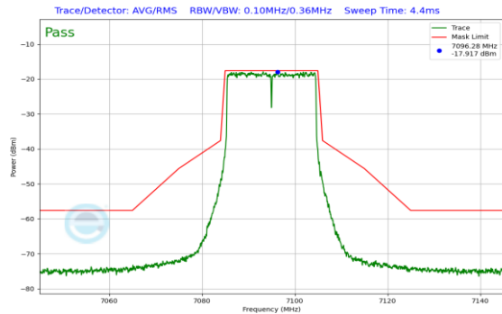
Plot 7-553. In Band Emission Plot SDM Antenna 0 (20MHz 802.11ax RU242 (UNII Band 8) – Ch. 229)
