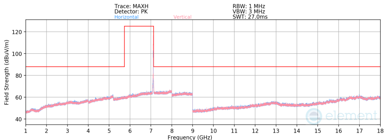
Plot 7-612. Radiated Spurious Emissions above 1GHz SDM (802.11ax – Ch. 229 – RU26)
