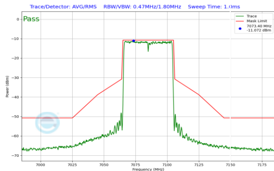
Plot 7-555. In Band Emission Plot SDM Antenna 0 (40MHz 802.11ax RU484 (UNII Band 8) – Ch. 227)
