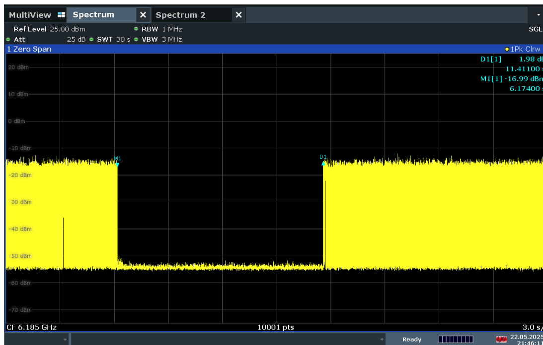
Plot 7-565. Contention Based Protocol Timing Plot – UNII 5 – 160MHz Channel 47 – High
