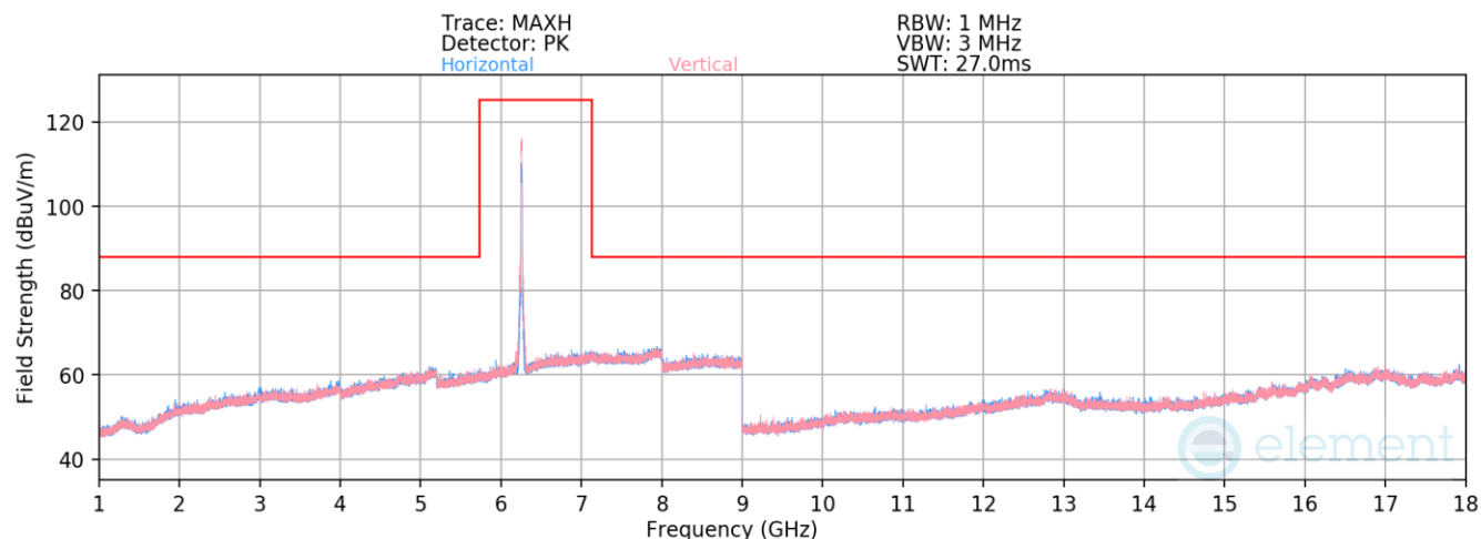
Plot 7-616. Radiated Spurious Emissions above 1GHz SDM (802.11ax – Ch. 93 – RU242)
