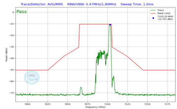
Plot 7-548. In Band Emission Plot SDM Antenna 0 (40MHz 802.11ax RU26 (UNII Band 8) – Ch. 227)
