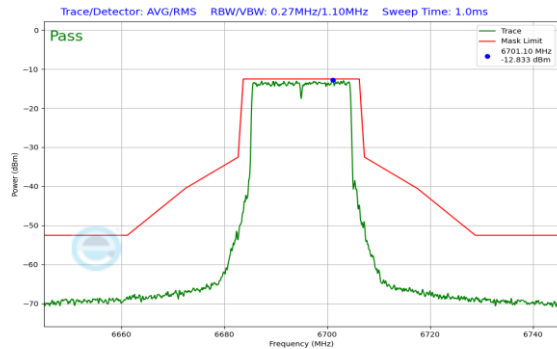
Plot 7-537. In Band Emission Plot SDM Antenna 0 (20MHz 802.11ax RU242 (UNII Band 7) – Ch. 149)
