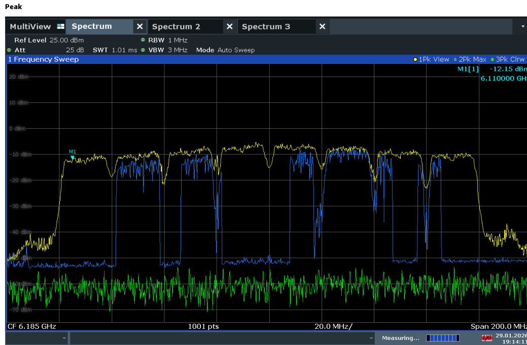
Plot 7-594. 160MHz Bandwidth, AWGN Signal Injected – 6110Mhz
