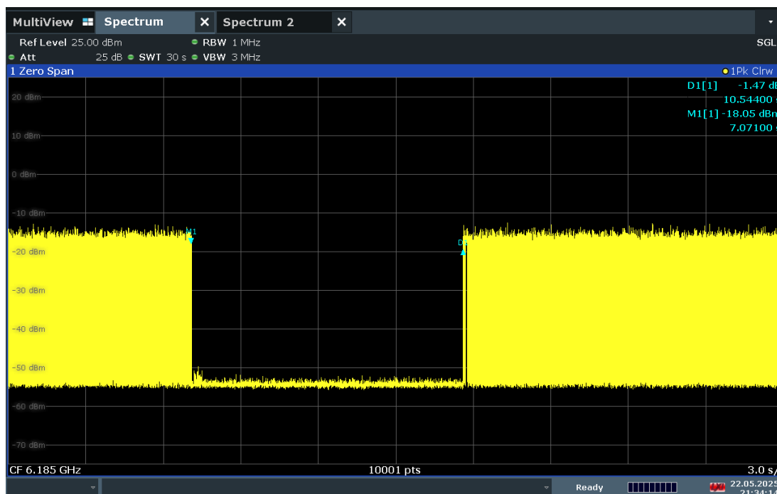
Plot 7-564. Contention Based Protocol Timing Plot –UNII 5 – 160MHz Channel 47 – Mid
