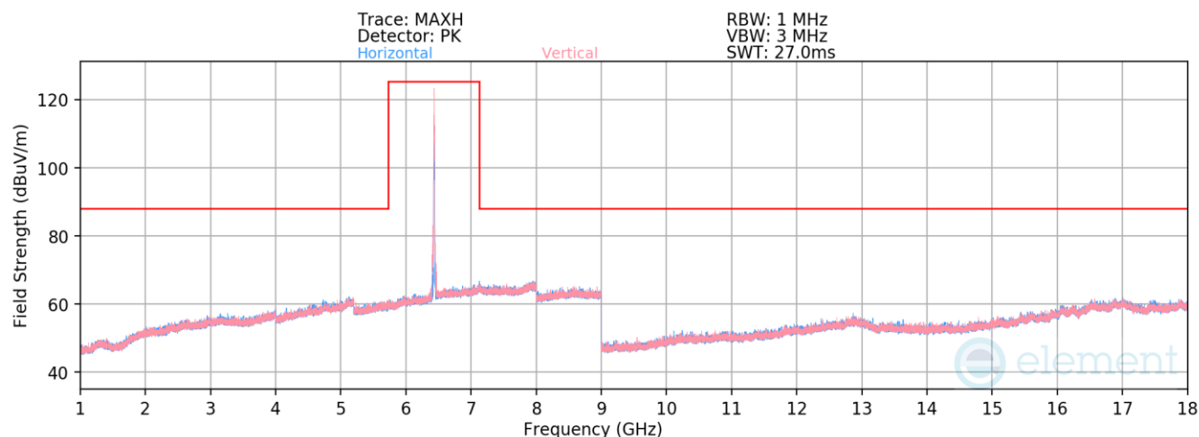
Plot 7-601. Radiated Spurious Emissions above 1GHz SDM (802.11ax – Ch. 97 – RU26)
