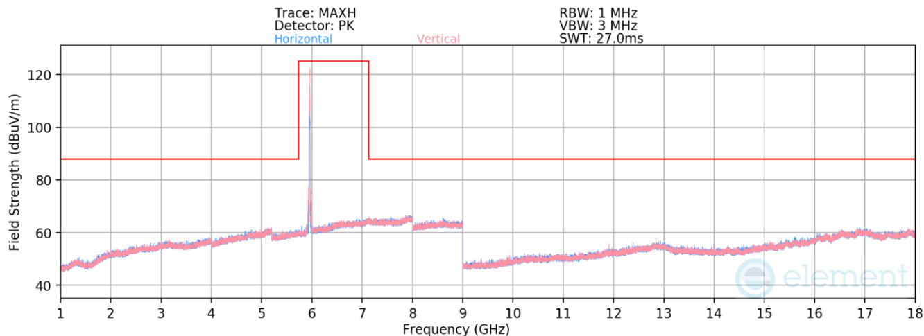
Plot 7-597. Radiated Spurious Emissions above 1GHz SDM (802.11ax – Ch. 1 – RU26)
