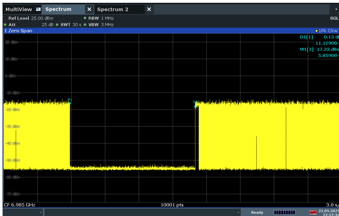
Plot 7-575. Contention Based Protocol Timing Plot – UNII 8 – 160MHz Channel 207 – Low
