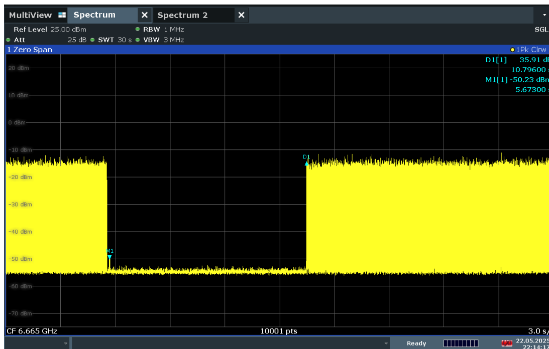
Plot 7-573. Contention Based Protocol Timing Plot – UNII 7 – 160MHz Channel 143 – High
