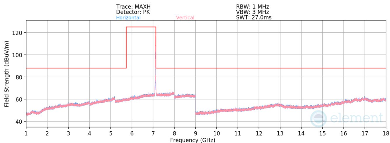
Plot 7-613. Radiated Spurious Emissions above 1GHz SDM (802.11ax – Ch. 1 – RU242)
