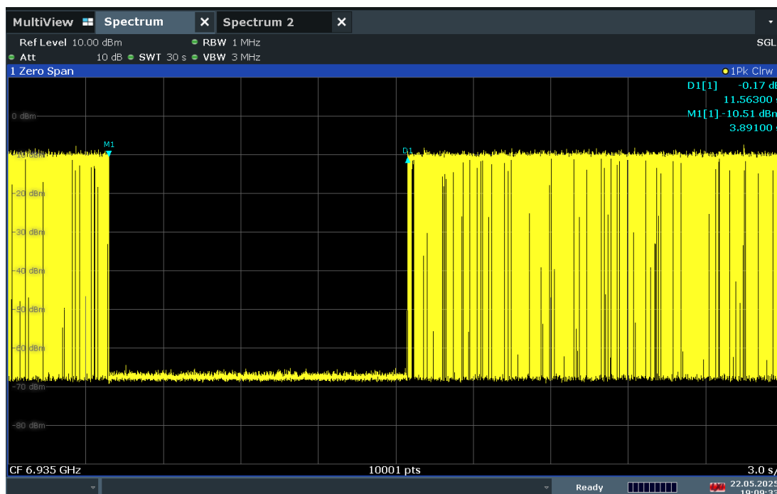
Plot 7-574. Contention Based Protocol Timing Plot – UNII 8 – 20MHz Channel 197
