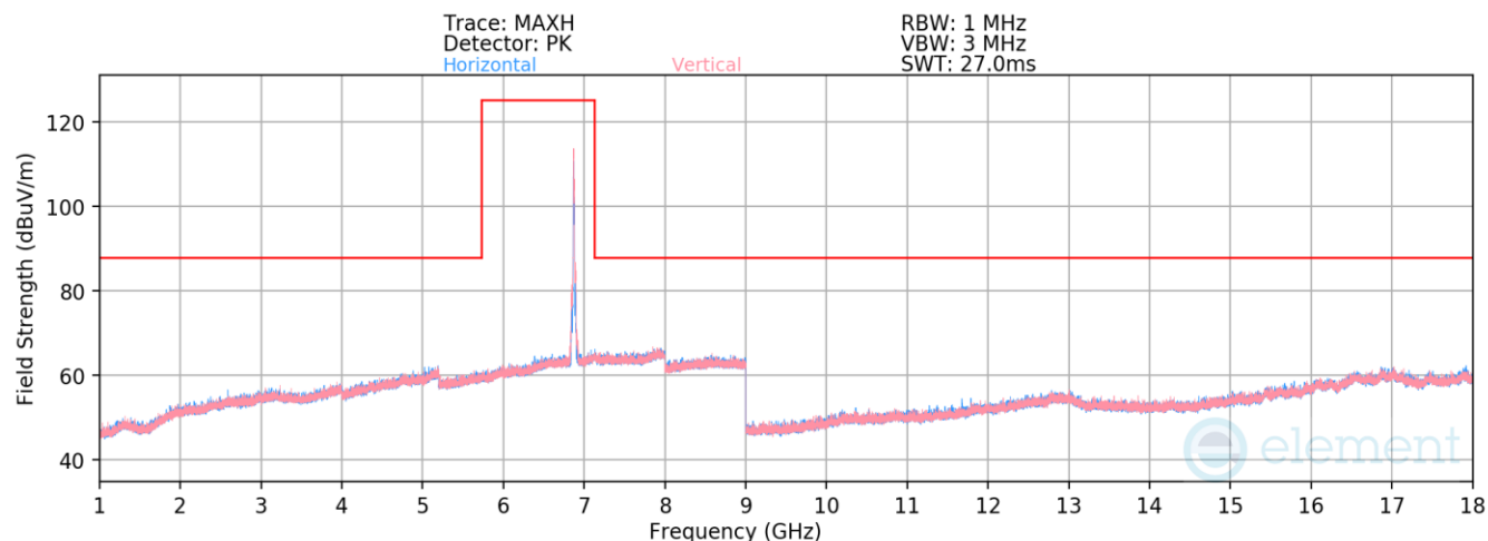
Plot 7-609. Radiated Spurious Emissions above 1GHz SDM (802.11ax – Ch. 189 – RU26)
