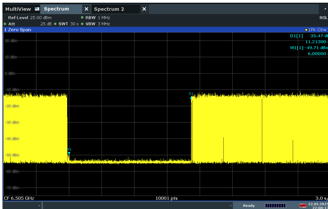
Plot 7-569. Contention Based Protocol Timing Plot – UNII 6 – 160MHz Channel 111 – High
