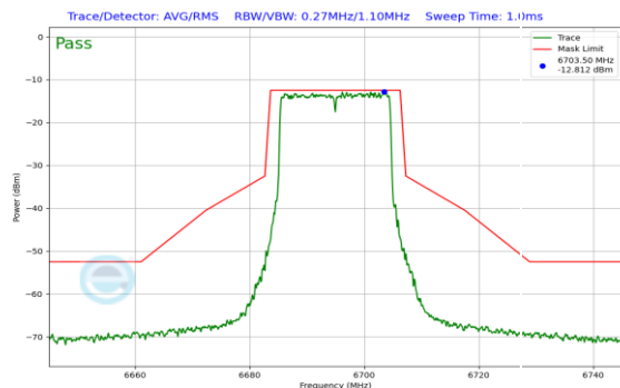
Plot 7-538. In Band Emission Plot SDM Antenna 0 (20MHz 802.11ax RU242 (UNII Band 7) – Ch. 149)
