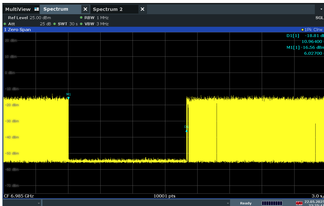
Plot 7-576. Contention Based Protocol Timing Plot – UNII 8 – 160MHz Channel 207 – Mid
