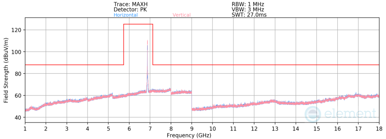
Plot 7-624. Radiated Spurious Emissions above 1GHz SDM (802.11ax – Ch. 185 – RU242)
