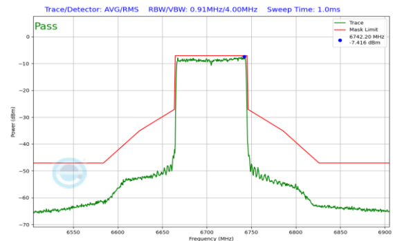
Plot 7-542. In Band Emission Plot SDM Antenna 0 (80MHz 802.11ax RU996 (UNII Band 7) – Ch. 151)
