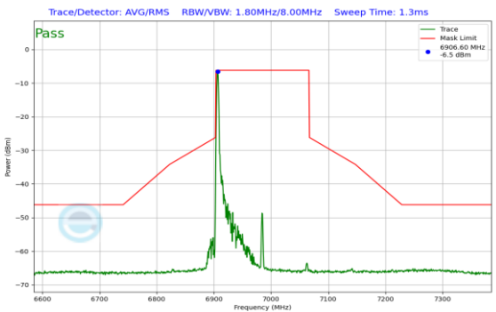
Plot 7-552. In Band Emission Plot SDM Antenna 0 (160MHz 802.11ax RU26 (UNII Band 8) – Ch. 207)
