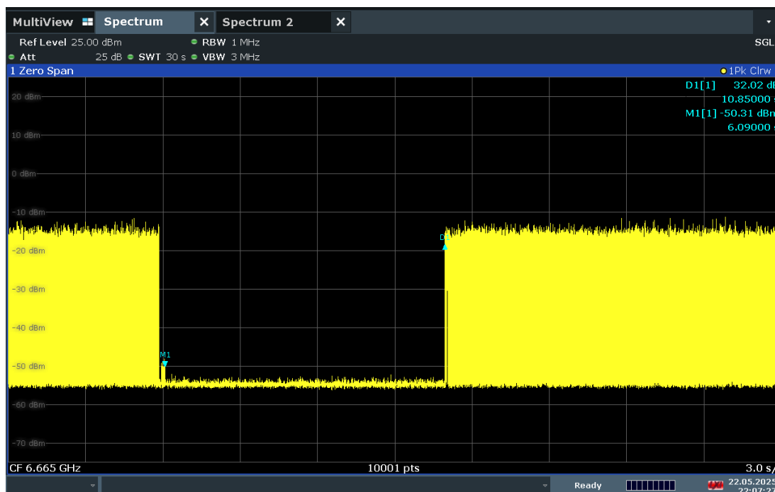
Plot 7-572. Contention Based Protocol Timing Plot – UNII 7 – 160MHz Channel 143 – Mid
