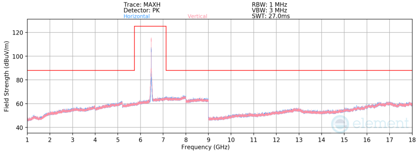
Plot 7-618. Radiated Spurious Emissions above 1GHz SDM (802.11ax – Ch. 105 – RU242)
