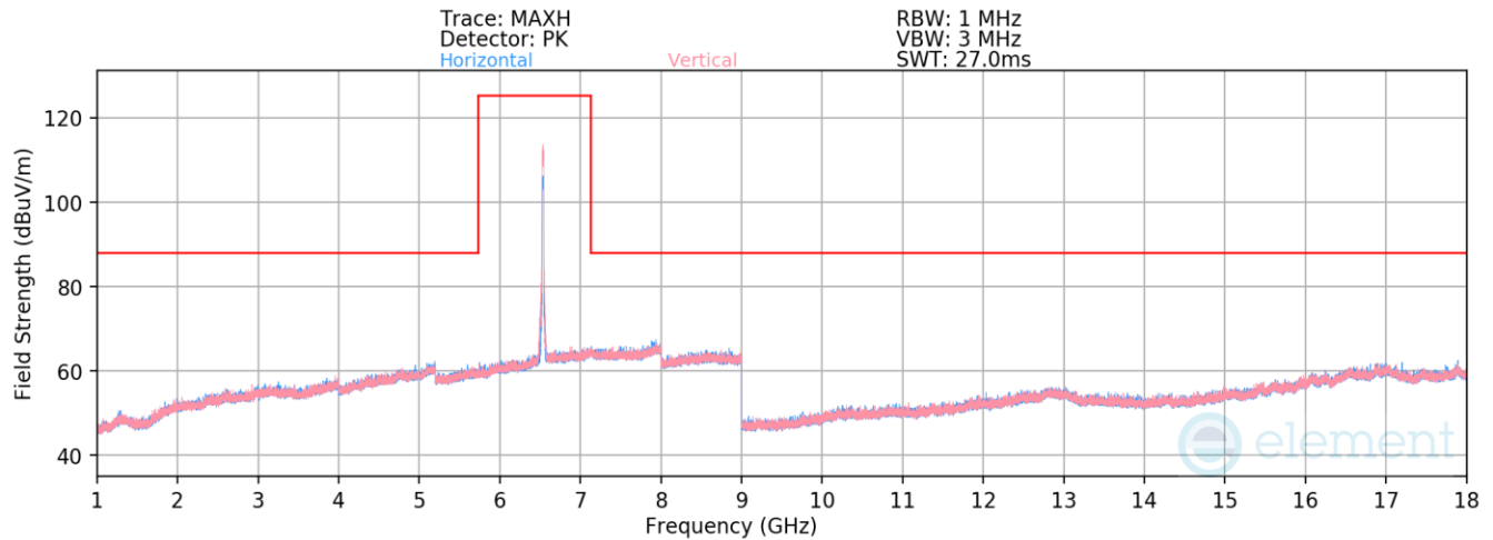
Plot 7-621. Radiated Spurious Emissions above 1GHz SDM (802.11ax – Ch. 117 – RU242)
