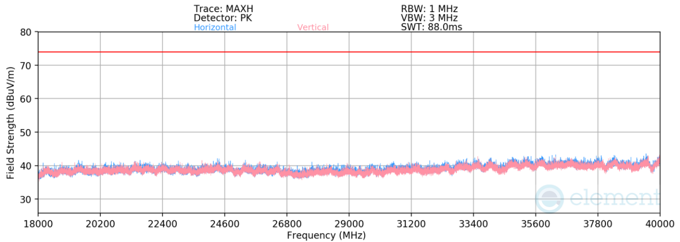
Plot 7-619. Radiated Spurious Emissions 18-40GHz SDM (802.11ax – Ch. 105 – RU242)
