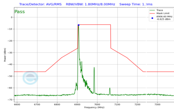
Plot 7-551. In Band Emission Plot SDM Antenna 0 (160MHz 802.11ax RU26 (UNII Band 8) – Ch. 207)
