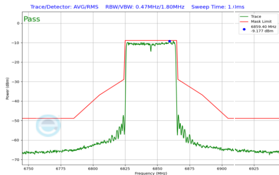
Plot 7-539. In Band Emission Plot SDM Antenna 0 (40MHz 802.11ax RU484 (UNII Band 7) – Ch. 179)
