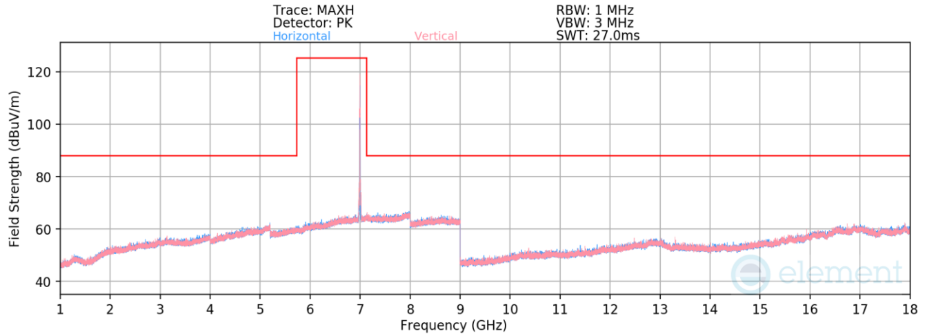
Plot 7-610. Radiated Spurious Emissions above 1GHz SDM (802.11ax – Ch. 209 – RU26)
