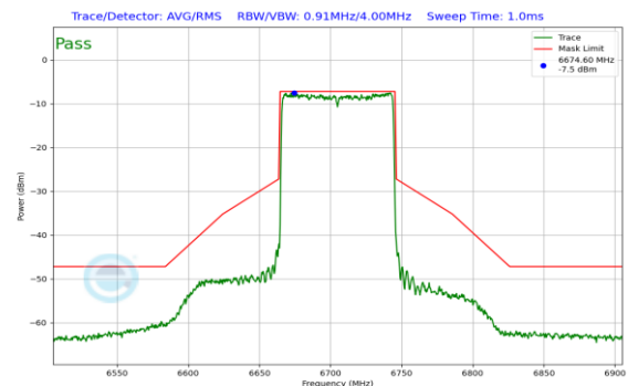
Plot 7-541. In Band Emission Plot SDM Antenna 0 (80MHz 802.11ax RU996 (UNII Band 7) – Ch. 151)
