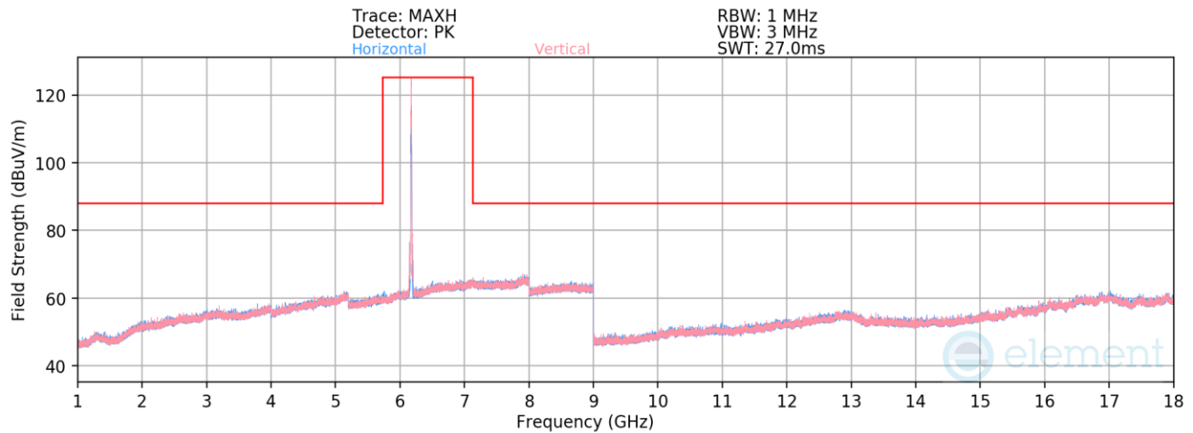
Plot 7-598. Radiated Spurious Emissions above 1GHz SDM (802.11ax – Ch. 45 – RU26)
