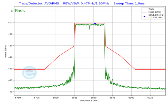
Plot 7-540. In Band Emission Plot SDM Antenna 0 (40MHz 802.11ax RU484 (UNII Band 7) – Ch. 179)
