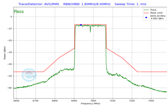
Plot 7-559. In Band Emission Plot SDM Antenna 0 (160MHz 802.11ax RU996x2 (UNII Band 8) – Ch. 207)
