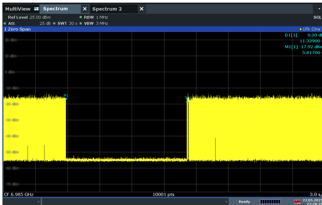
Plot 7-577. Contention Based Protocol Timing Plot – UNII 8 – 160MHz Channel 207 – High
