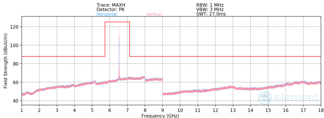
Plot 7-605. Radiated Spurious Emissions above 1GHz SDM (802.11ax – Ch. 117 – RU26)
