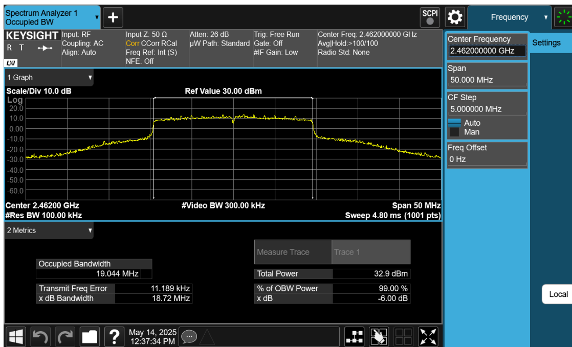
Plot 7-28. 6 dB BW Plot Antenna 0 Dedicated (802.11ax(SU) – Ch. 11)
