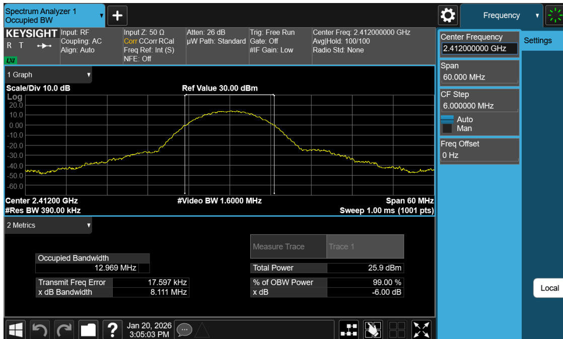
Plot 7-1. 99% OBW Plot Antenna 0 Common (802.11b – Ch. 1)
