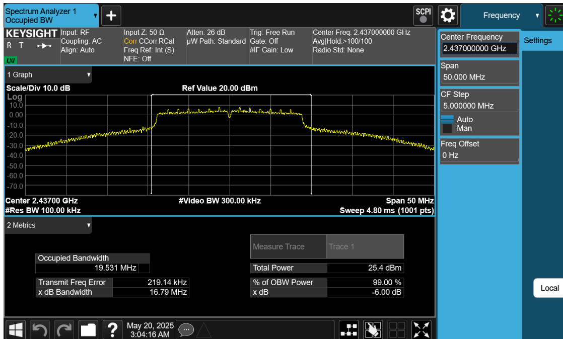
Plot 7-19. 6 dB BW Plot Antenna 0 Common (802.11n – Ch. 6)
