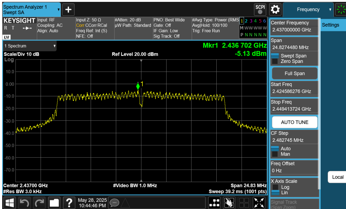
Plot 7-46. Power Spectral Density Plot Antenna 1 Dedicated (802.11g – Ch. 6)
