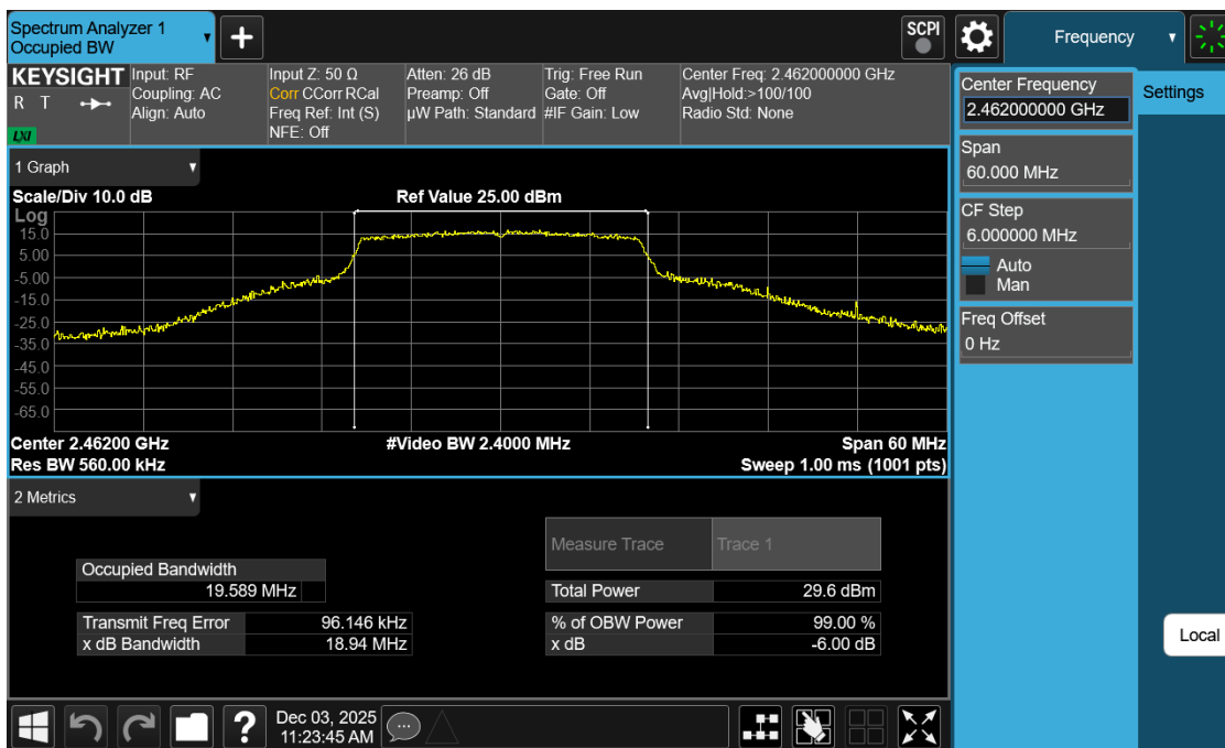
Plot 7-16. 99% OBW Plot Antenna 1 Dedicated (802.11ax(SU) – Ch. 11)
