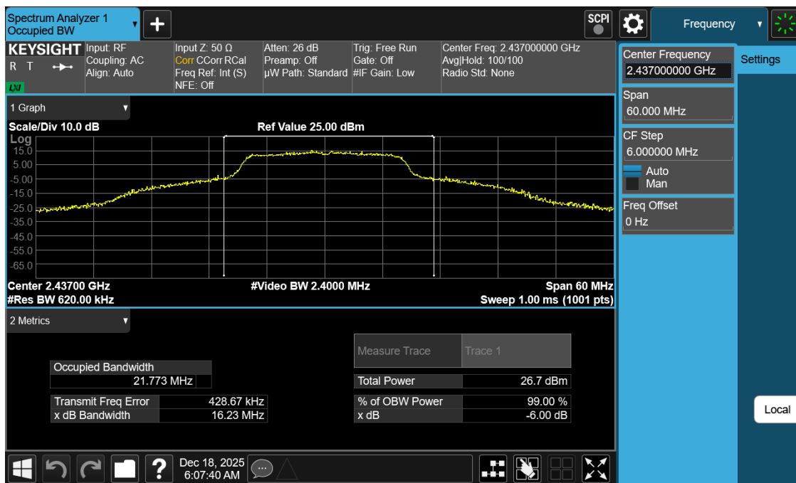
Plot 7-2. 99% OBW Plot Antenna 0 Common (802.11g – Ch. 6)
