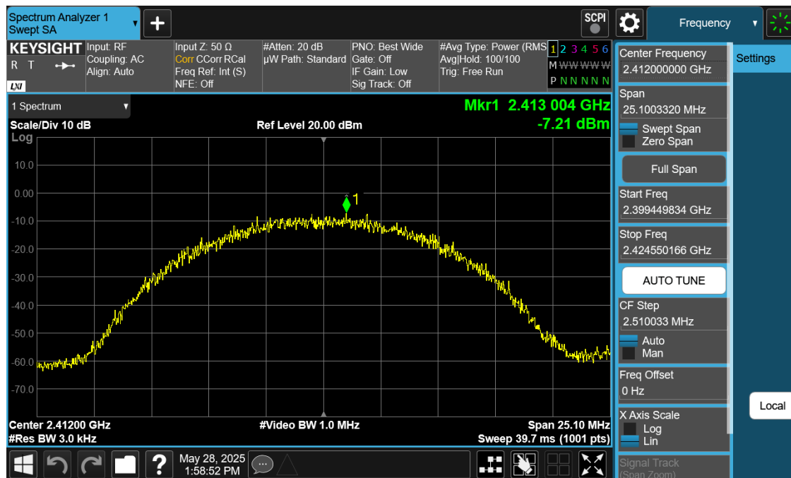
Plot 7-33. Power Spectral Density Plot Antenna 0 Common (802.11b – Ch. 1)
