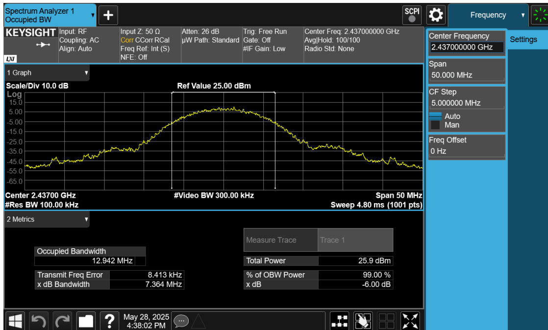
Plot 7-21. 6 dB BW Plot Antenna 1 Common (802.11b – Ch. 6)
