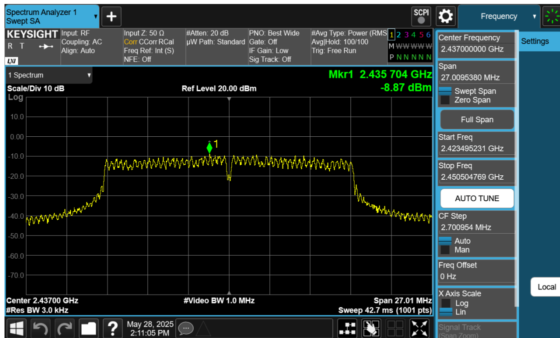
Plot 7-34. Power Spectral Density Plot Antenna 0 Common (802.11g – Ch. 6)
