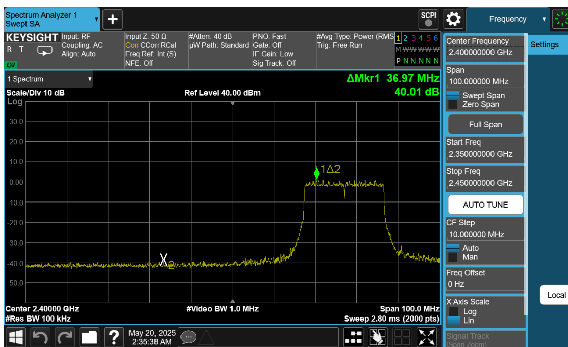
Plot 7-38. Band Edge Antenna 0 (Common) (802.11ax OFDMA – RU242 – Ch. 4)
