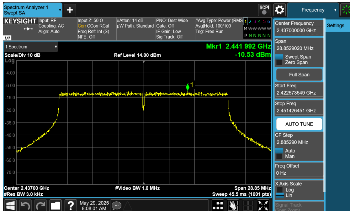
Plot 7-31. Power Spectral Density Plot Antenna 0 Dedicated (802.11ax OFDMA – RU242 – Ch. 6)
