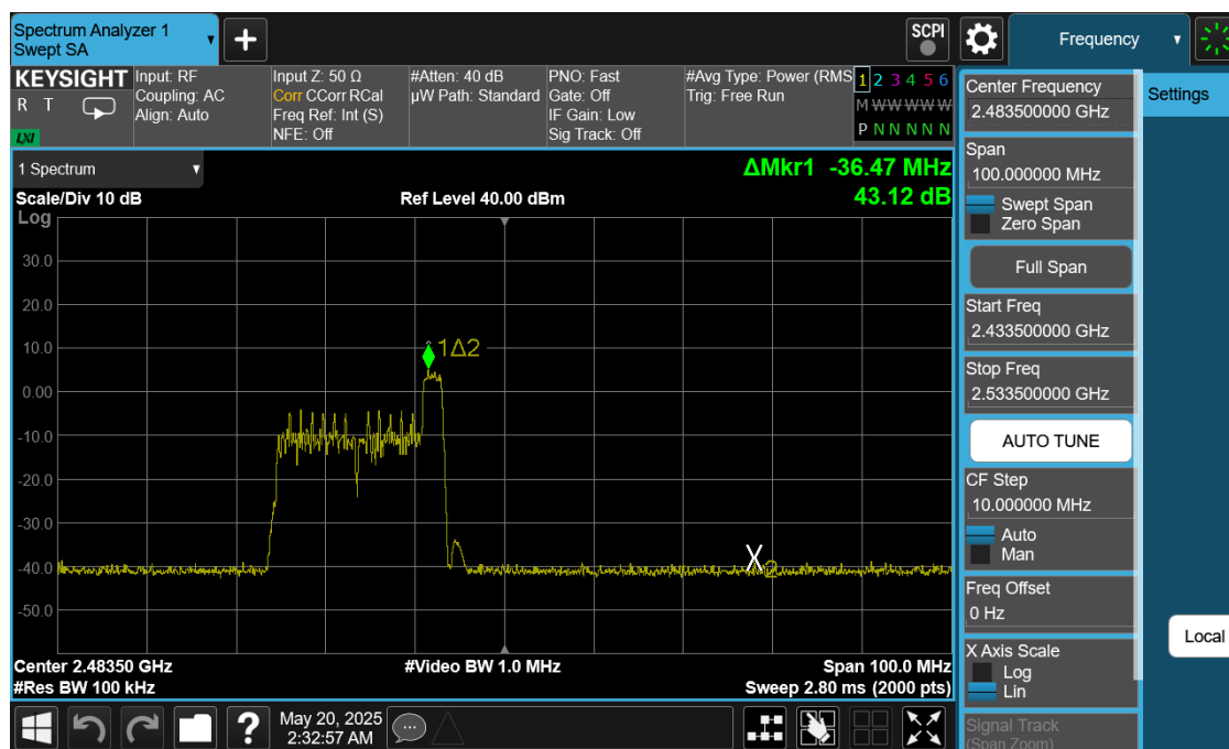
Plot 7-34. Band Edge Antenna 0 (Common) (802.11ax OFDMA – RU26 Index 8 – Ch. 12)
