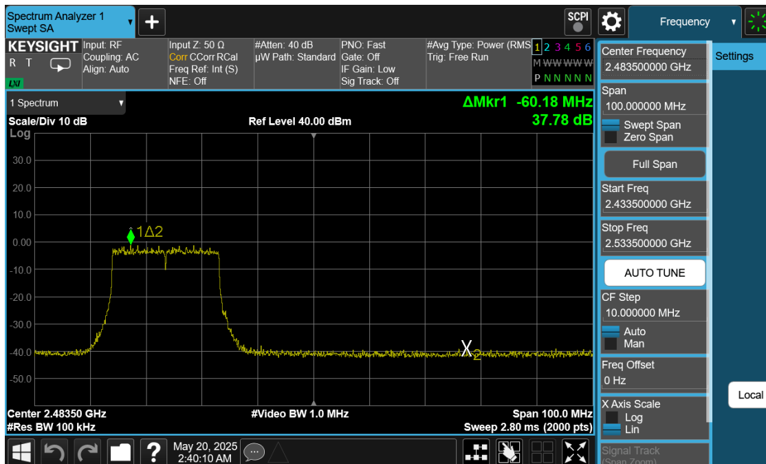
Plot 7-45. Band Edge Antenna 0 (Common) (802.11ax OFDMA – RU242 – Ch. 10)
