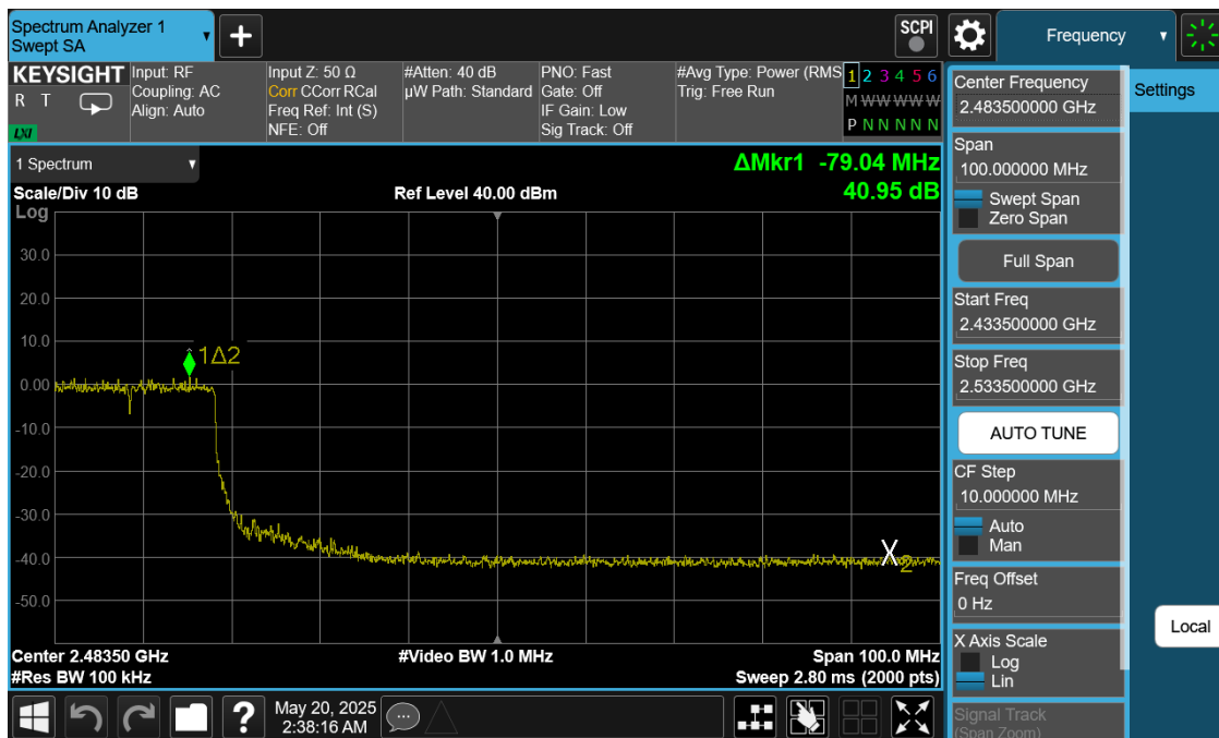
Plot 7-42. Band Edge Antenna 0 (Common) (802.11ax OFDMA – RU242 – Ch. 7)
