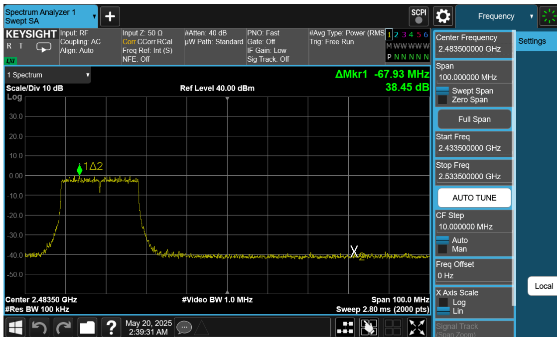
Plot 7-44. Band Edge Antenna 0 (Common) (802.11ax OFDMA – RU242 – Ch. 9)
