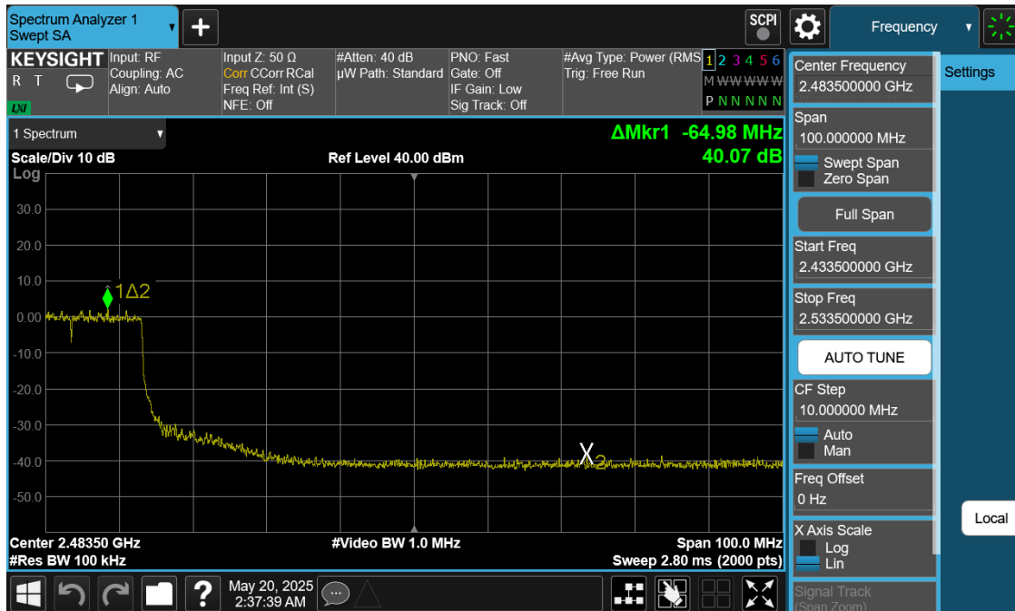
Plot 7-41. Band Edge Antenna 0 (Common) (802.11ax OFDMA – RU242 – Ch. 6(High Channel))
