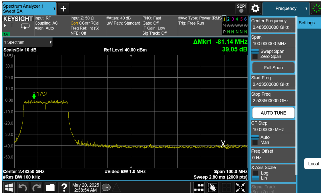
Plot 7-43. Band Edge Antenna 0 (Common) (802.11ax OFDMA – RU242 – Ch. 8)
