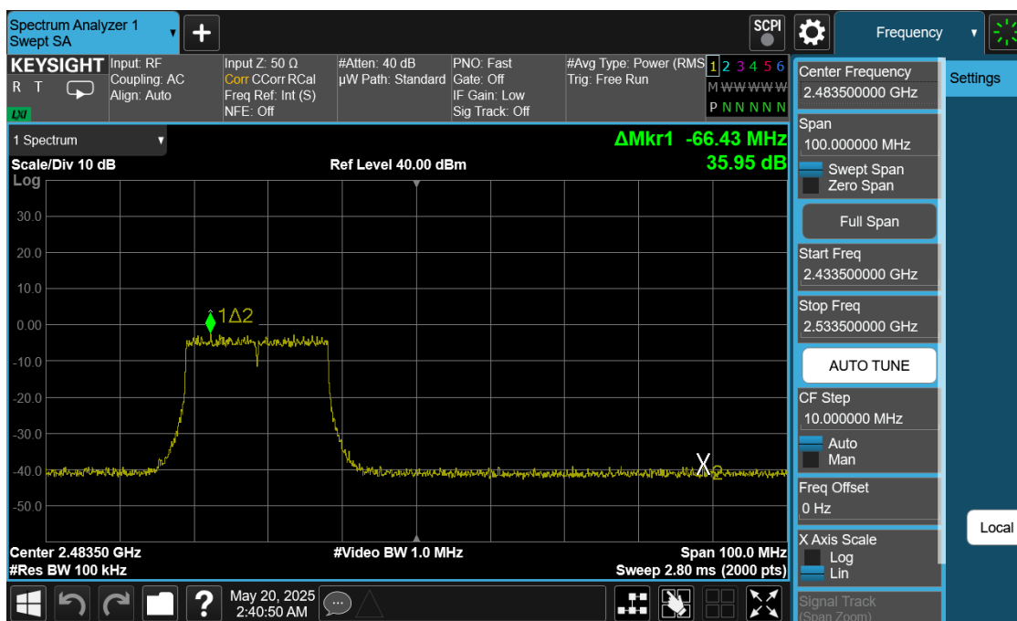
Plot 7-46. Band Edge Antenna 0 (Common) (802.11ax OFDMA – RU242 – Ch. 11)
