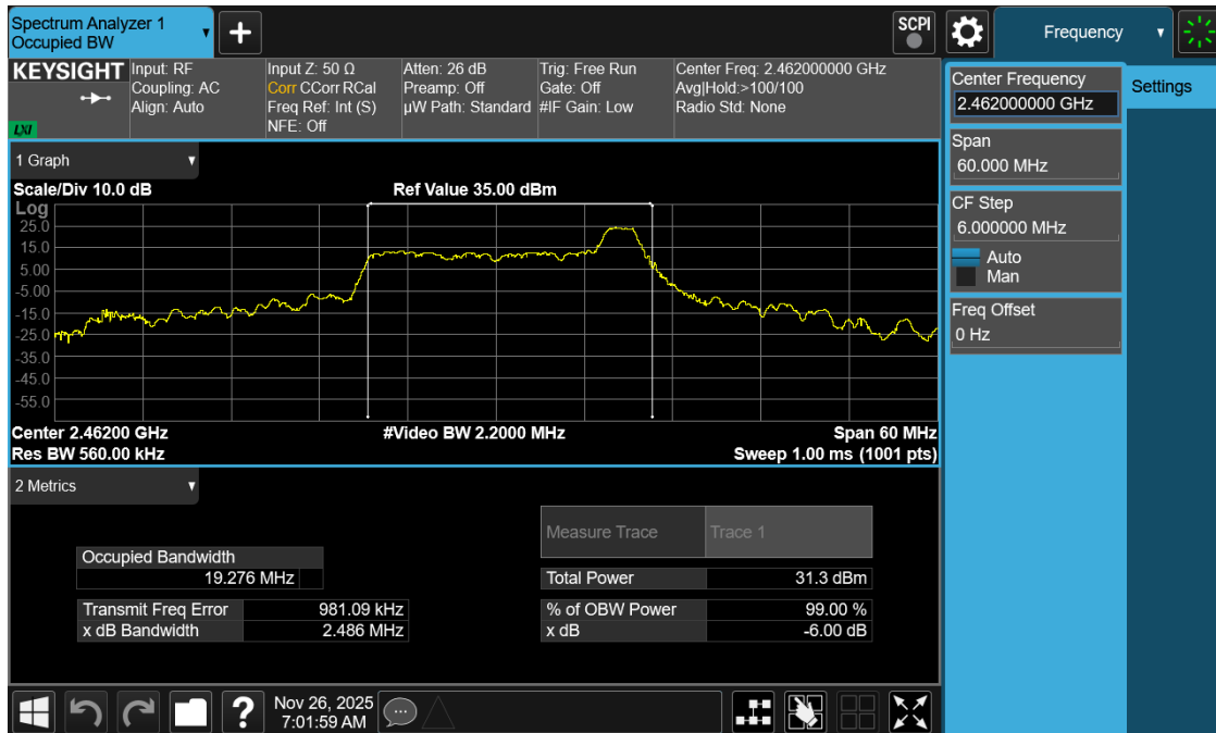
Plot 7-7. 99% OBW Plot Antenna 1 (Dedicated) (802.11ax OFDMA – RU26 Index 8 – Ch. 11)
