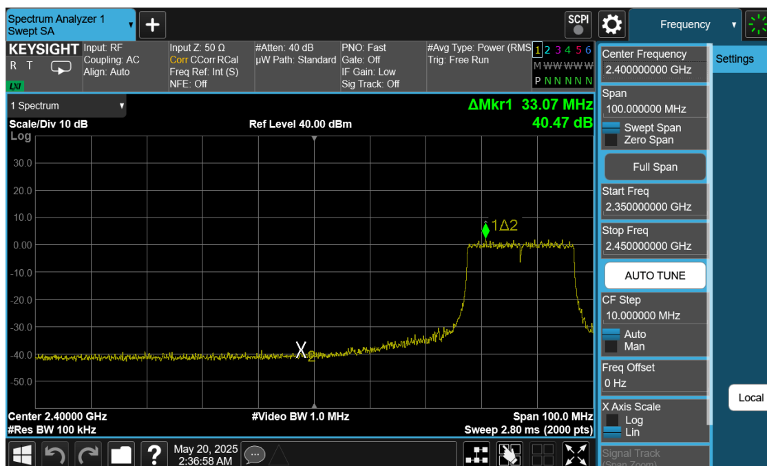
Plot 7-40. Band Edge Antenna 0 (Common) (802.11ax OFDMA – RU242 – Ch. 6(Low Channel))
