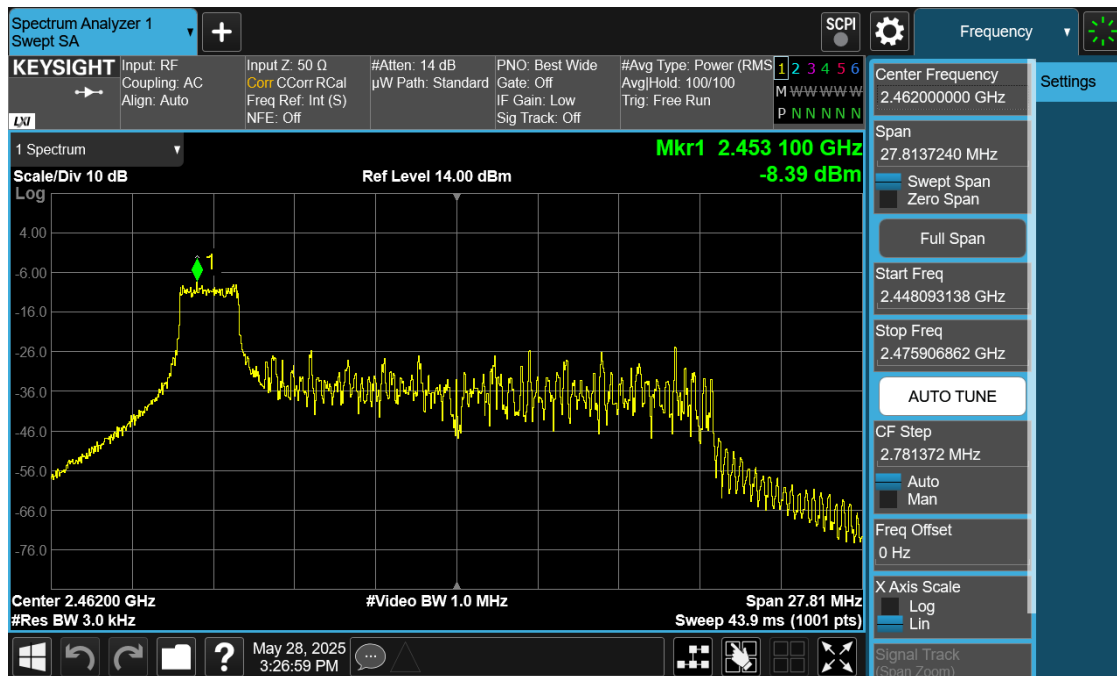
Plot 7-19. Power Spectral Density Plot Antenna 1 (Common) (802.11ax OFDMA – RU26 Index 8 – Ch. 11)
