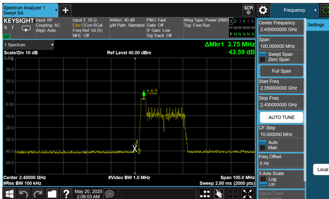
Plot 7-33. Band Edge Antenna 0 (Common) (802.11ax OFDMA – RU26 Index 0 – Ch. 1)
