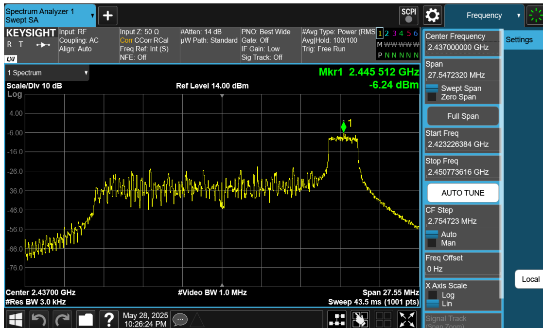
Plot 7-27. Power Spectral Density Plot Antenna 1 (Dedicated) (802.11ax OFDMA – RU26 Index 8 – Ch. 6)
