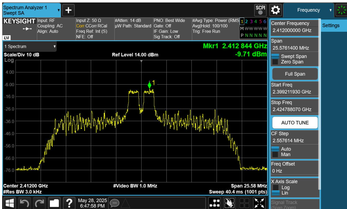
Plot 7-22. Power Spectral Density Plot Antenna 1 (802.11ax OFDMA – RU26 Index 4 – Ch. 1)
