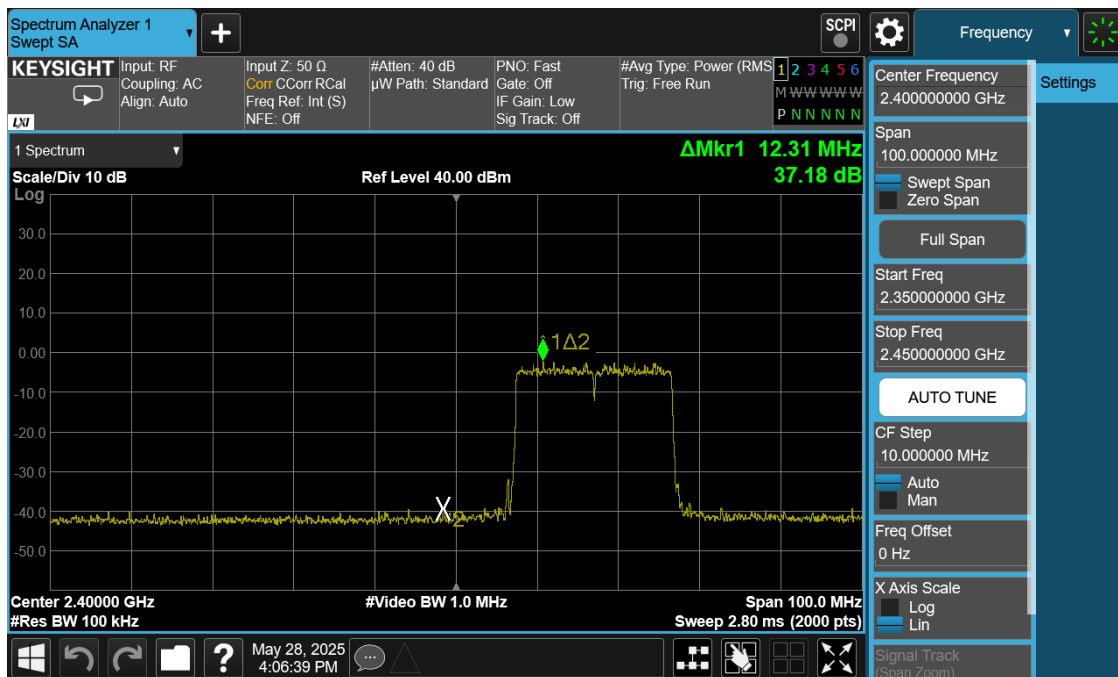
Plot 7-51. Band Edge Antenna 1 (Common) (802.11ax OFDMA – RU242 – Ch. 2)
