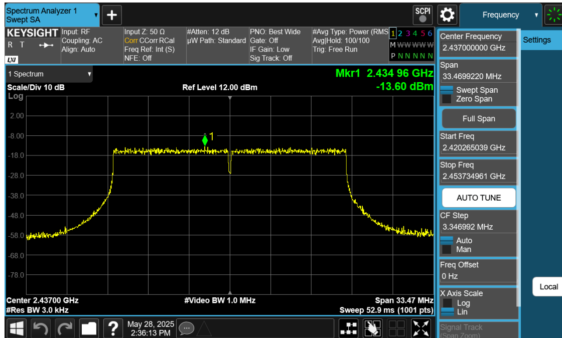
Plot 7-23. Power Spectral Density Plot Antenna 0 (802.11ax OFDMA – RU242 – Ch. 6)
