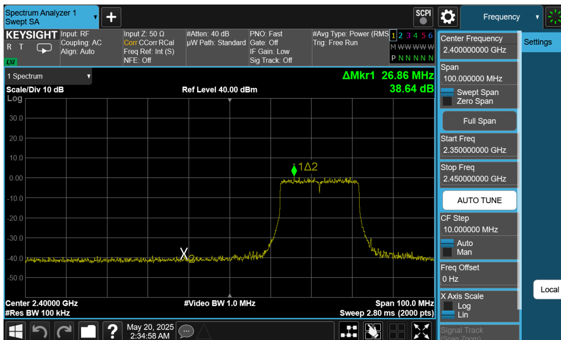
Plot 7-37. Band Edge Antenna 0 (Common) (802.11ax OFDMA – RU242 – Ch. 3)
