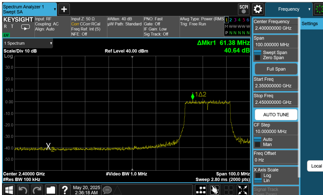
Plot 7-39. Band Edge Antenna 0 (Common) (802.11ax OFDMA – RU242 – Ch. 5)
