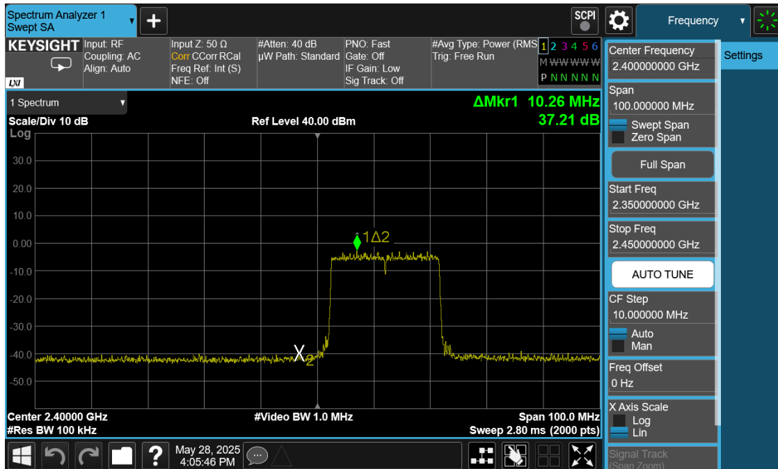
Plot 7-50. Band Edge Antenna 1 (Common) (802.11ax OFDMA – RU242 – Ch. 1)
