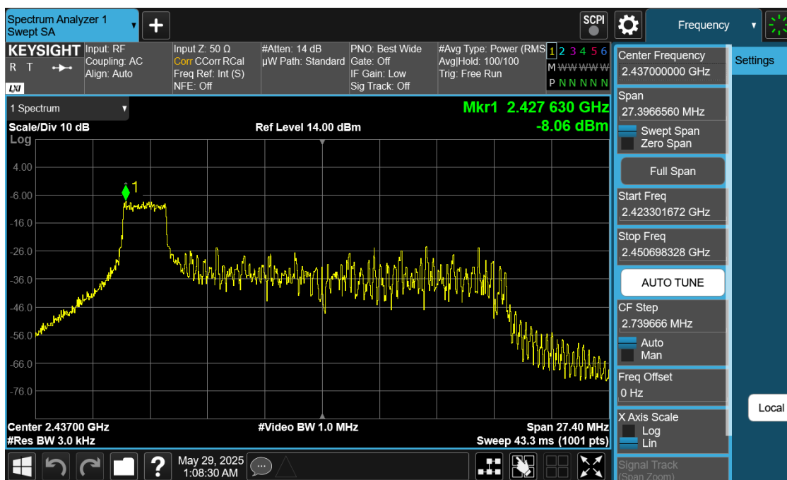
Plot 7-30. Power Spectral Density Plot Antenna 1 Dedicated (802.11ax OFDMA – RU26 Index 0 – Ch. 6)
