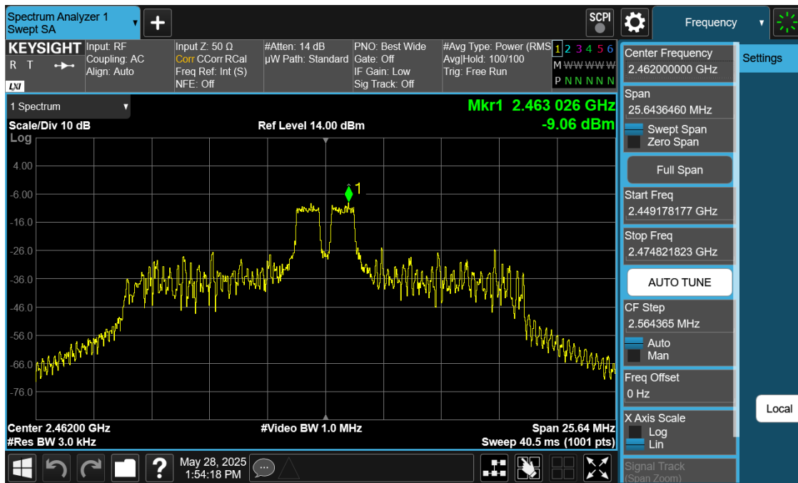
Plot 7-17. Power Spectral Density Plot Antenna 0 (Common) (802.11ax OFDMA – RU26 Index 4 – Ch. 11)
