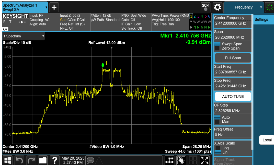
Plot 7-21. Power Spectral Density Plot Antenna 0 (802.11ax OFDMA – RU26 Index 4 – Ch. 1)
