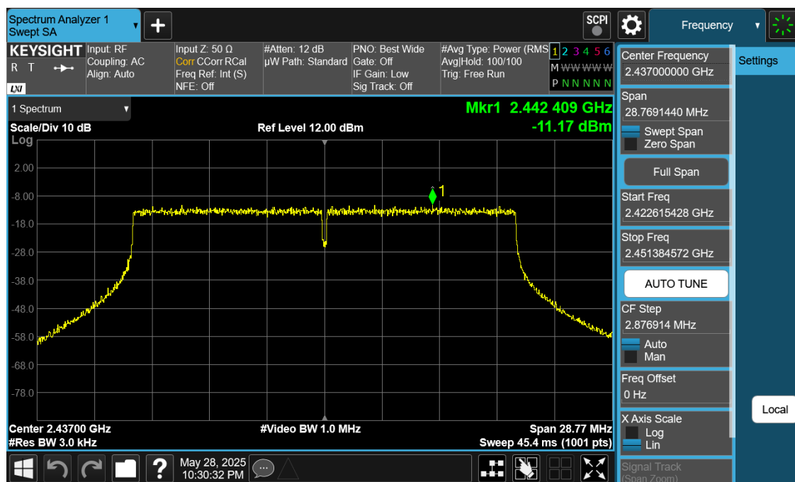
Plot 7-28. Power Spectral Density Plot Antenna 1 (Dedicated) (802.11ax OFDMA – RU242 – Ch. 6)
