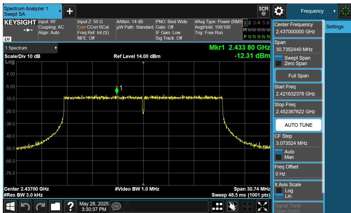
Plot 7-20. Power Spectral Density Plot Antenna 1 (Common) (802.11ax OFDMA – RU242 – Ch. 6)
