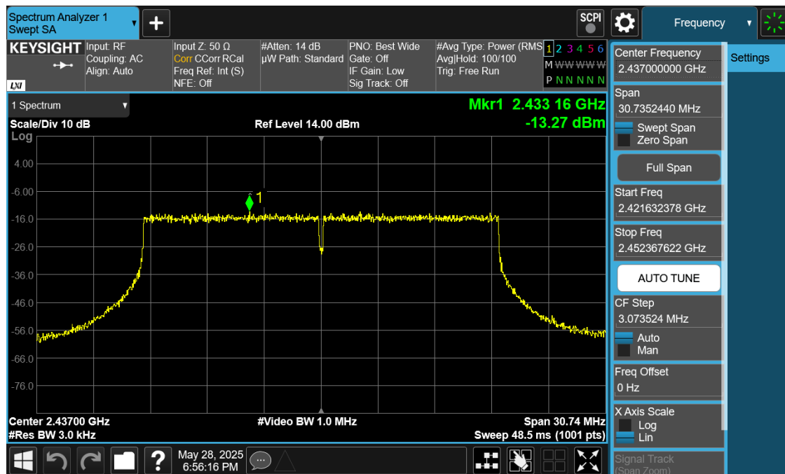
Plot 7-24. Power Spectral Density Plot Antenna 1 (802.11ax OFDMA – RU242 – Ch. 6)
