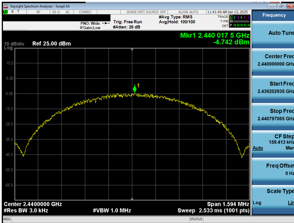
Plot 7-46. Power Spectral Density Plot Antenna 1a (Bluetooth (LE), 1Mbps, iPA – Ch. 19)
