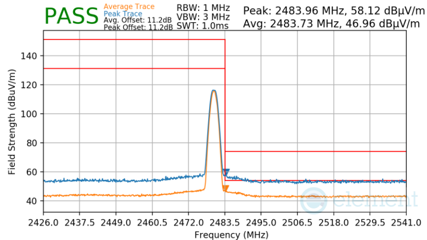
Plot 7-90. Radiated Restricted Upper Band Edge Measurement Antenna 1a (Average & Peak)
