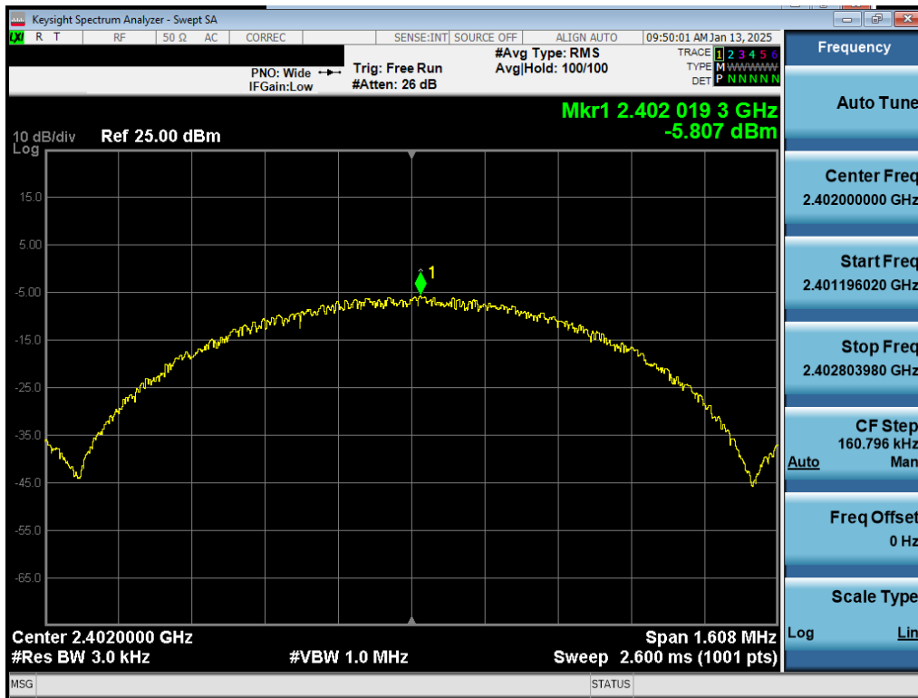
Plot 7-43. Power Spectral Density Plot Antenna 3a (Bluetooth (LE), 1Mbps, iPA – Ch. 0)
