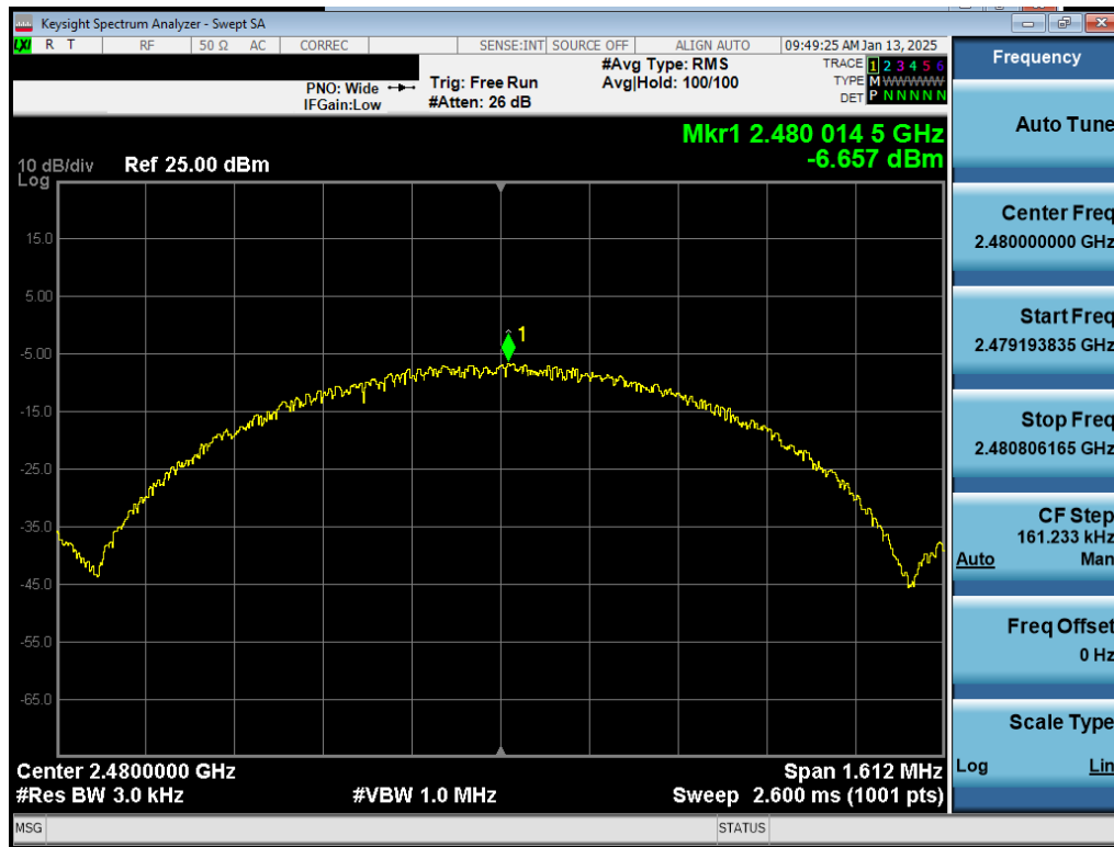
Plot 7-41. Power Spectral Density Plot Antenna 3a (Bluetooth (LE), 1Mbps, ePA – Ch. 39)
