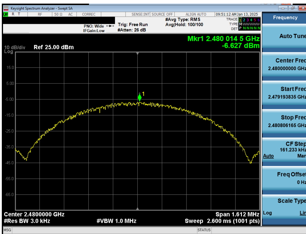
Plot 7-47. Power Spectral Density Plot Antenna 3a (Bluetooth (LE), 1Mbps, iPA – Ch. 39)
