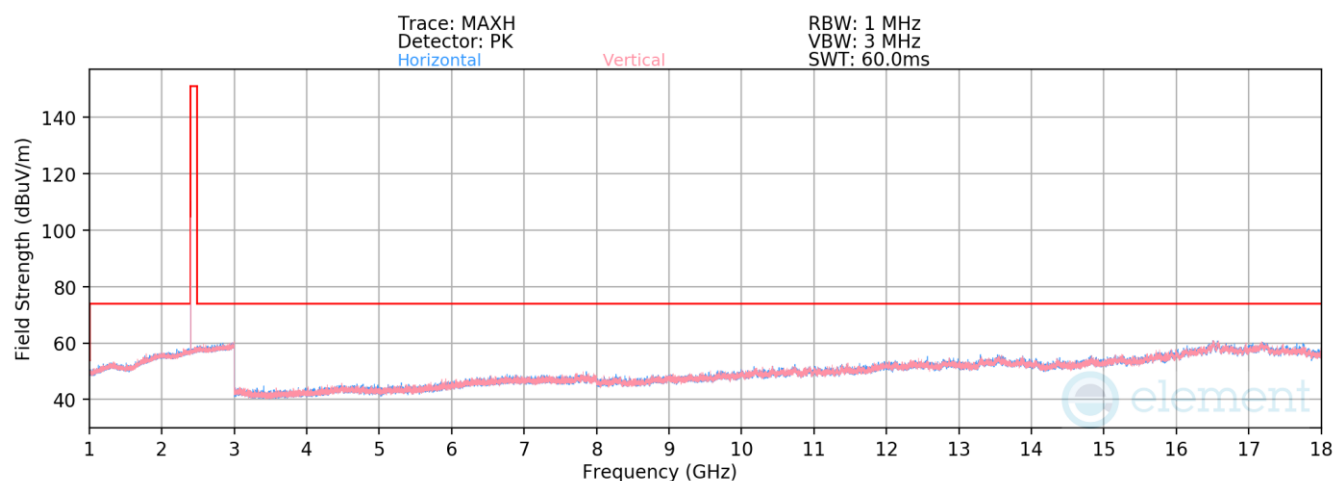
Plot 7-81. Radiated Spurious Emissions 1-18GHz TxBF (1Mbps, ePA – Ch. 0)
