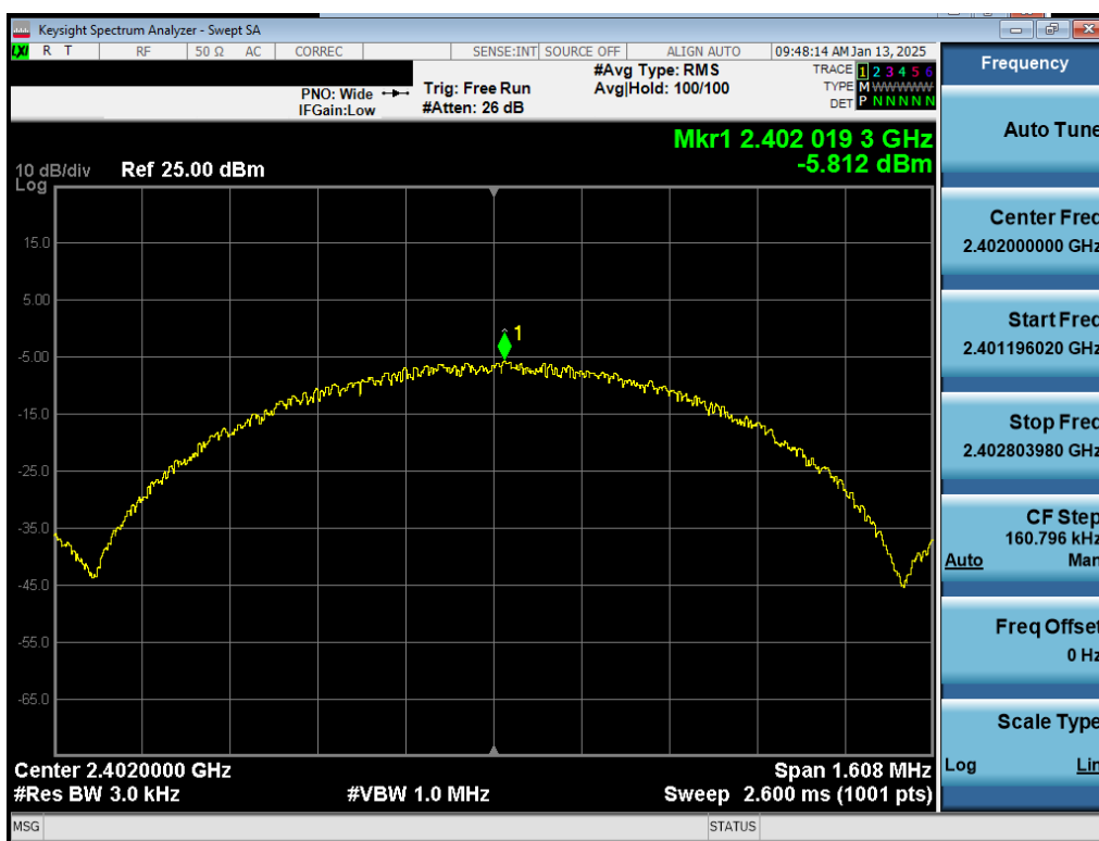
Plot 7-37. Power Spectral Density Plot Antenna 3a (Bluetooth (LE), 1Mbps, ePA – Ch. 0)
