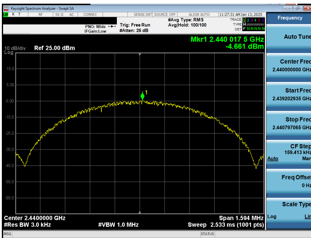
Plot 7-29. Power Spectral Density Plot Antenna 1a (Bluetooth (LE), 1Mbps, iPA – Ch. 19)
