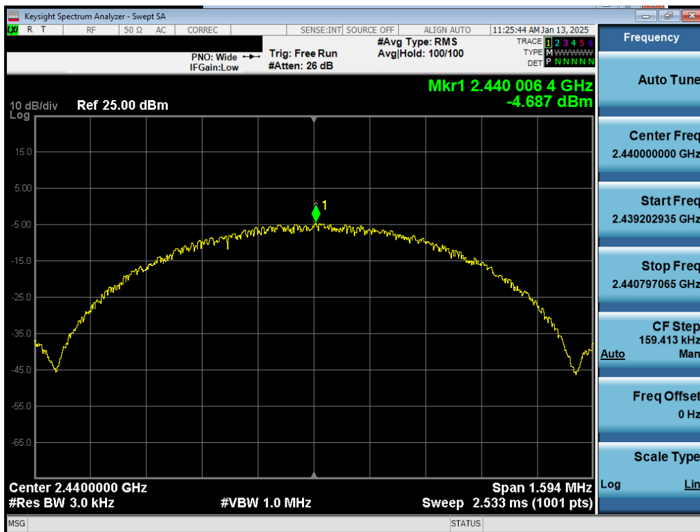
Plot 7-26. Power Spectral Density Plot Antenna 1a (Bluetooth (LE), 1Mbps, ePA – Ch. 19)
