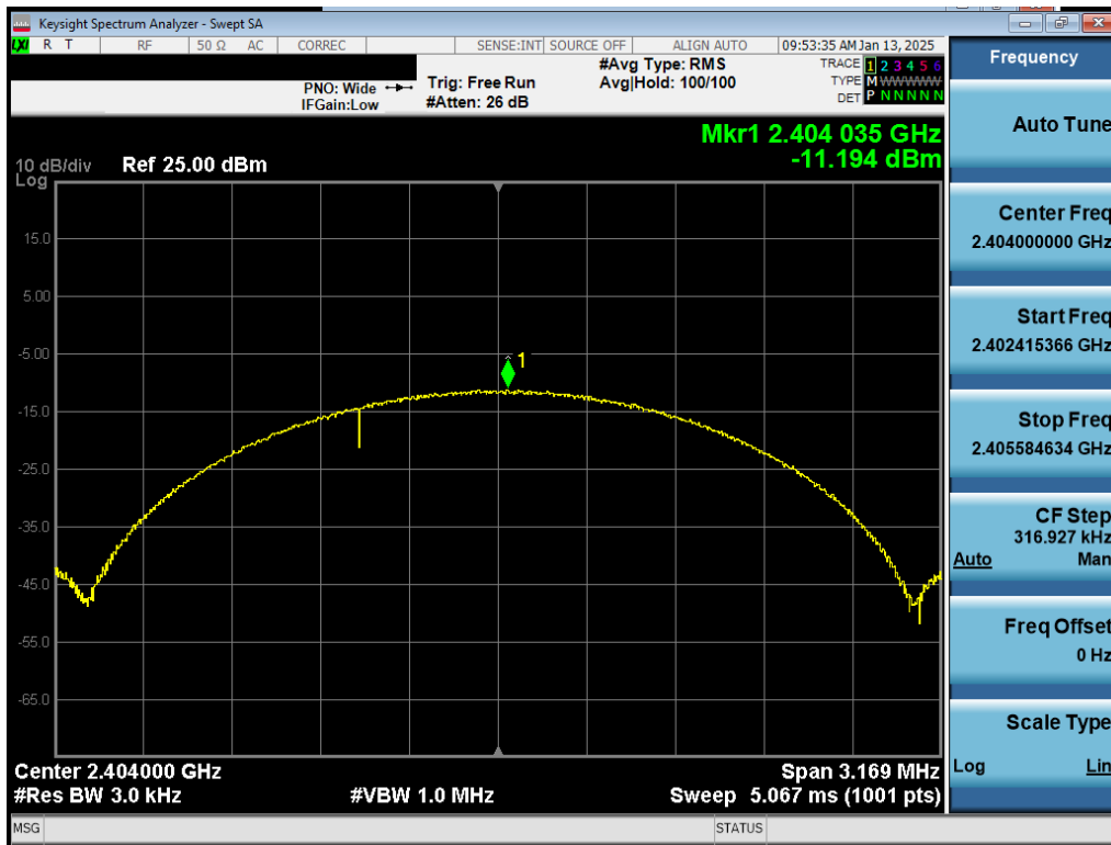
Plot 7-55. Power Spectral Density Plot Antenna 3a (Bluetooth (LE), 2Mbps, iPA – Ch. 1)
