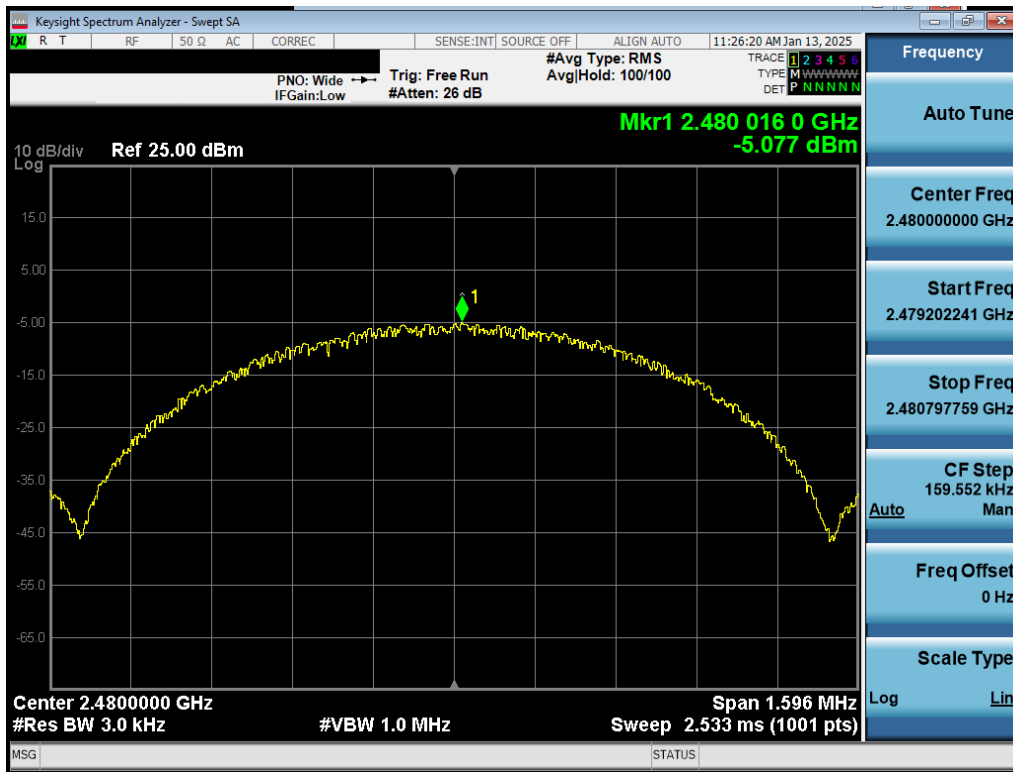
Plot 7-27. Power Spectral Density Plot Antenna 1a (Bluetooth (LE), 1Mbps, ePA – Ch. 39)
