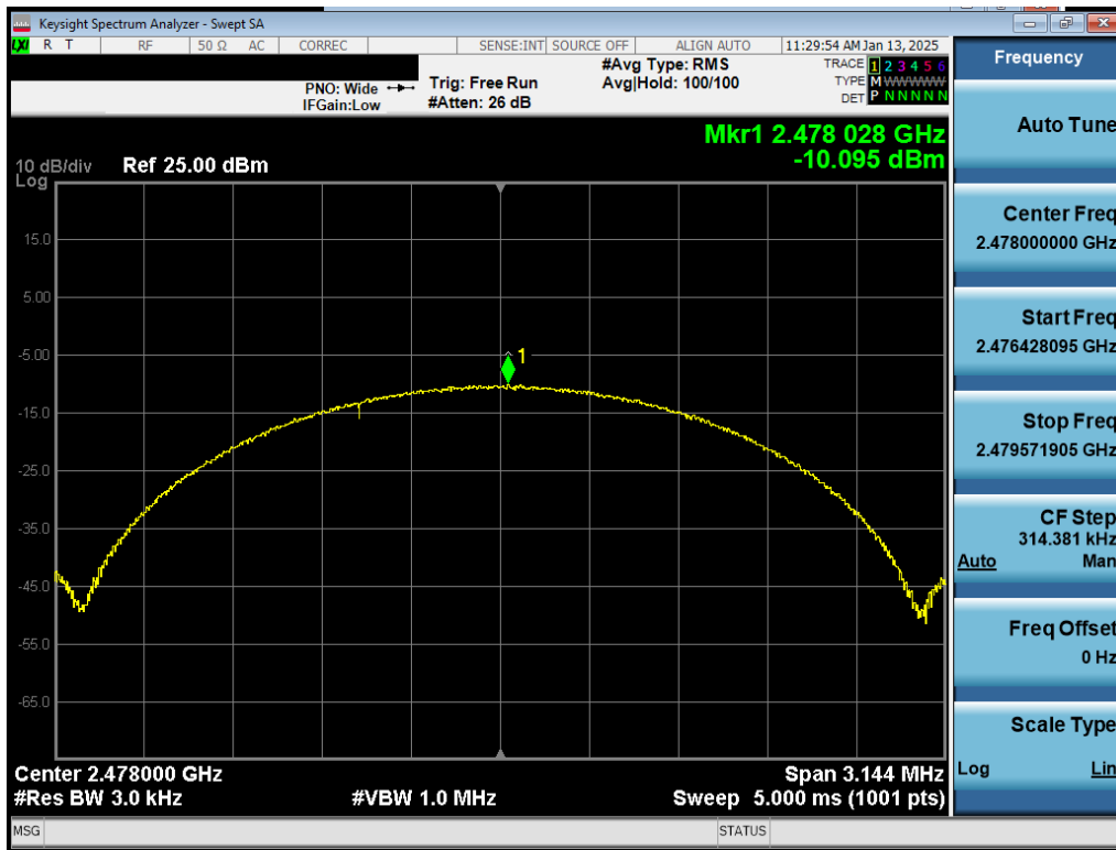
Plot 7-33. Power Spectral Density Plot Antenna 1a (Bluetooth (LE), 2Mbps, ePA – Ch. 38)
