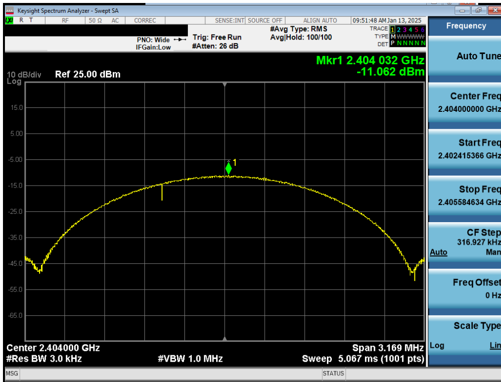
Plot 7-49. Power Spectral Density Plot Antenna 3a (Bluetooth (LE), 2Mbps, ePA – Ch. 1)
