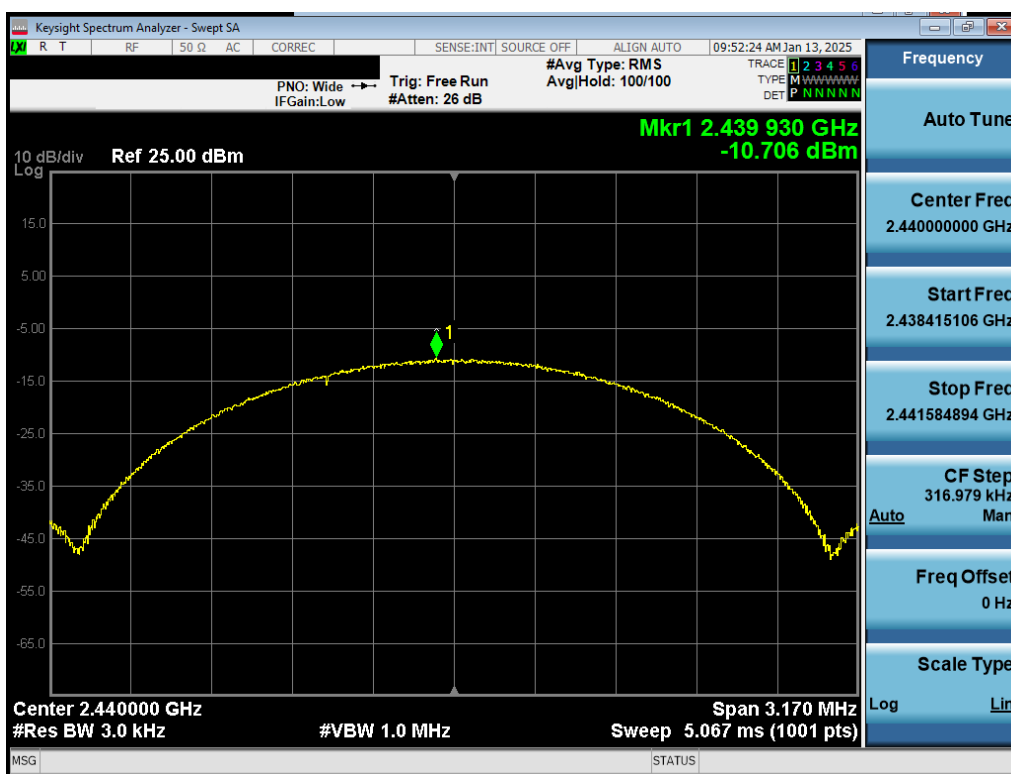
Plot 7-51. Power Spectral Density Plot Antenna 3a (Bluetooth (LE), 2Mbps, ePA – Ch. 19)
