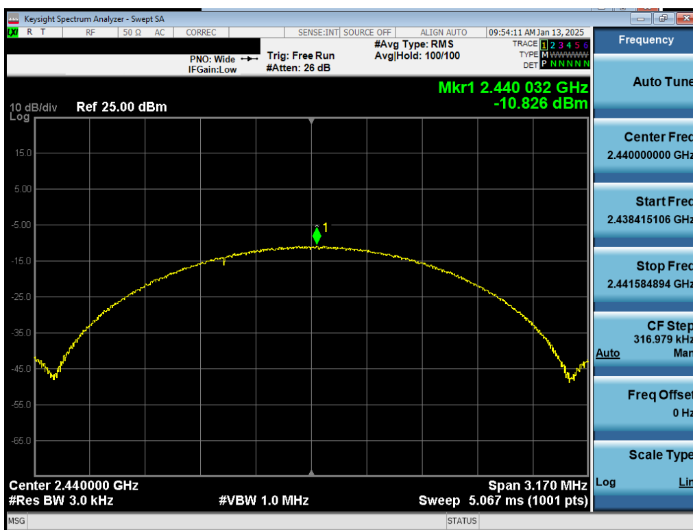
Plot 7-57. Power Spectral Density Plot Antenna 3a (Bluetooth (LE), 2Mbps, iPA – Ch. 19)
