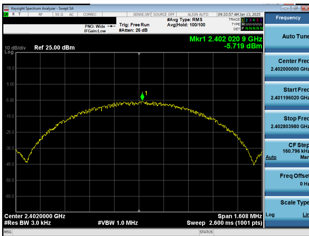
Plot 7-13. Power Spectral Density Plot Antenna 3a (Bluetooth (LE), 1Mbps, ePA – Ch. 0)
