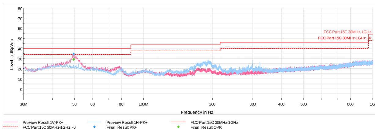
Plot 7-97. Radiated Spurious Emissions Below 1GHz TxBF (1Mbps, ePA – Ch.19, Pol. H & V, with AC/DC Adapter)
