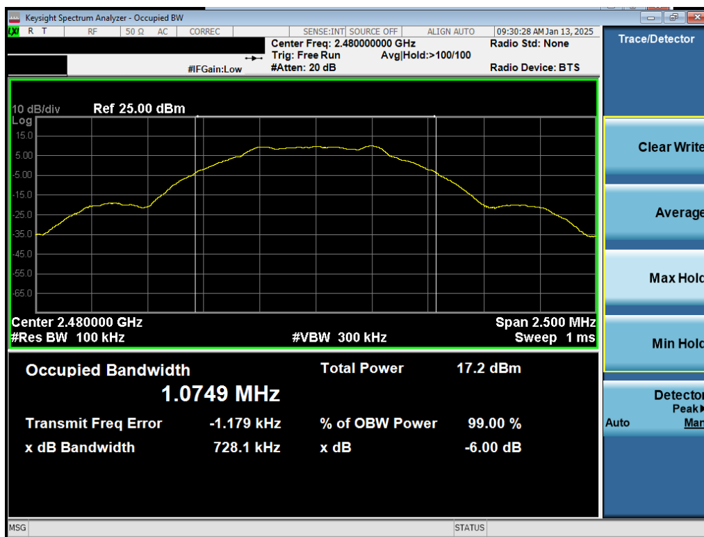
Plot 7-3. 6dB BW & 99% OBW Plot Antenna 3a (Bluetooth (LE), 1Mbps, ePA – Ch. 39)
