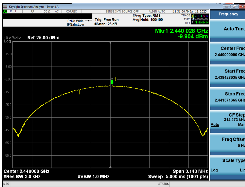
Plot 7-35. Power Spectral Density Plot Antenna 1a (Bluetooth (LE), 2Mbps, iPA – Ch. 19)
