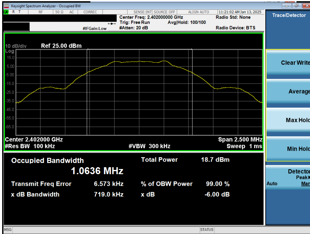
Plot 7-7. 6dB BW & 99% OBW Plot Antenna 1a (Bluetooth (LE), 1Mbps, ePA – Ch. 0)
