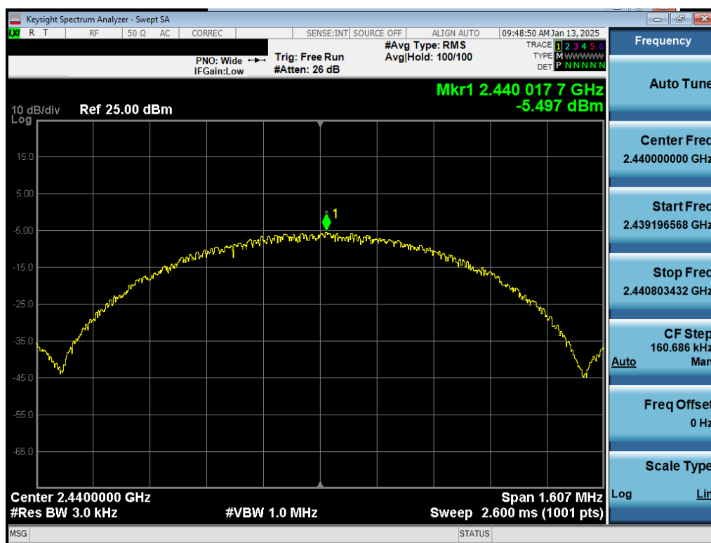
Plot 7-39. Power Spectral Density Plot Antenna 3a (Bluetooth (LE), 1Mbps, ePA – Ch. 19)
