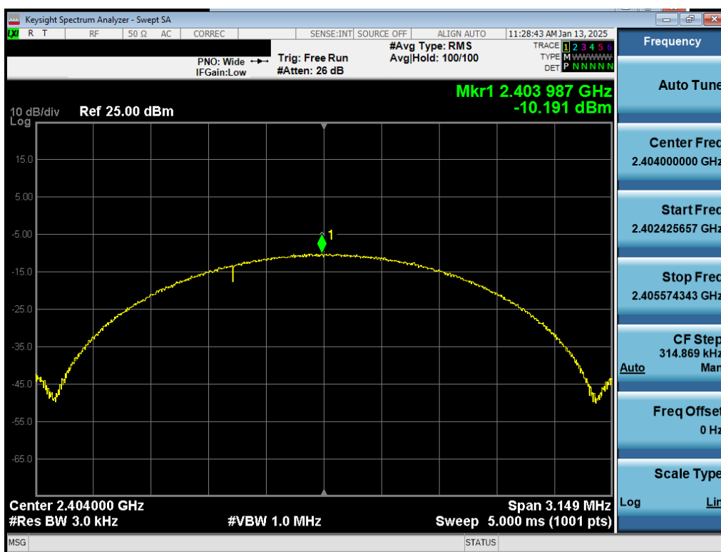
Plot 7-31. Power Spectral Density Plot Antenna 1a (Bluetooth (LE), 2Mbps, ePA – Ch. 1)
