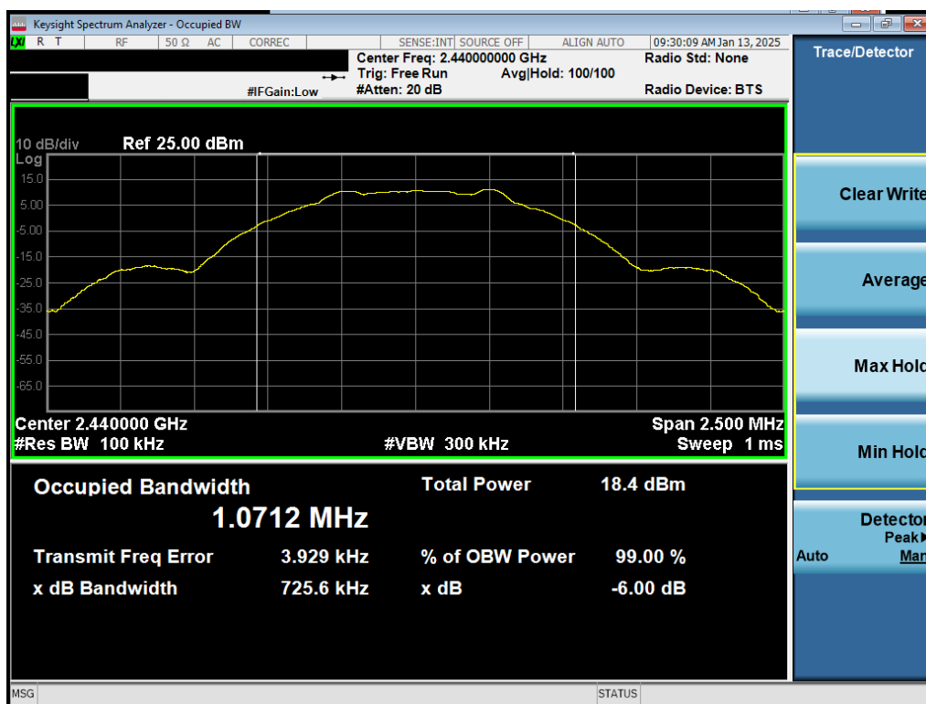
Plot 7-2. 6dB BW & 99% OBW Plot Antenna 3a (Bluetooth (LE), 1Mbps, ePA – Ch. 19)
