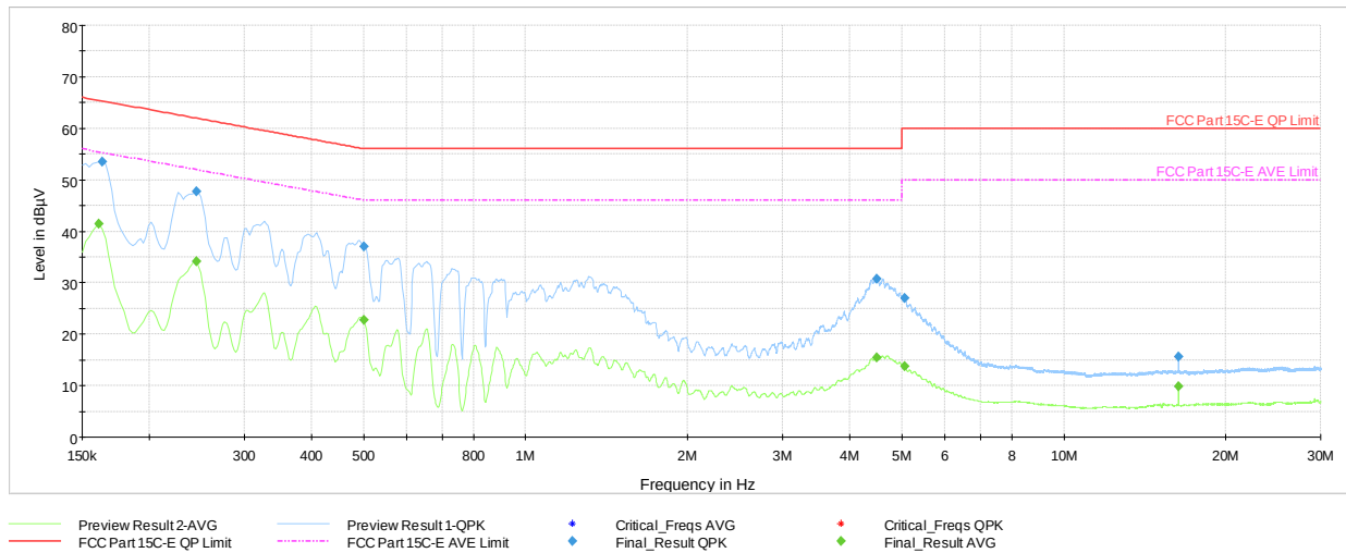
Plot 7-98. AC Line Conducted Plot with Bluetooth LE Tx BF (L1, 1Mbps ePA – Ch.19 with AC/DC Adapter)
