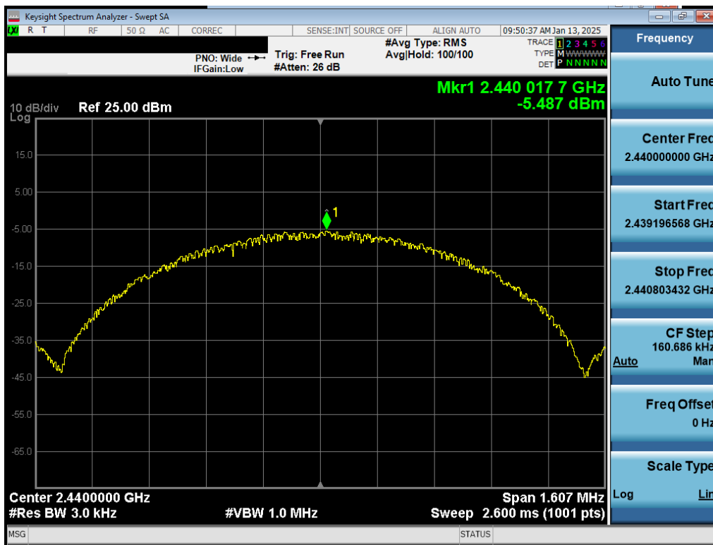
Plot 7-45. Power Spectral Density Plot Antenna 3a (Bluetooth (LE), 1Mbps, iPA – Ch. 19)
