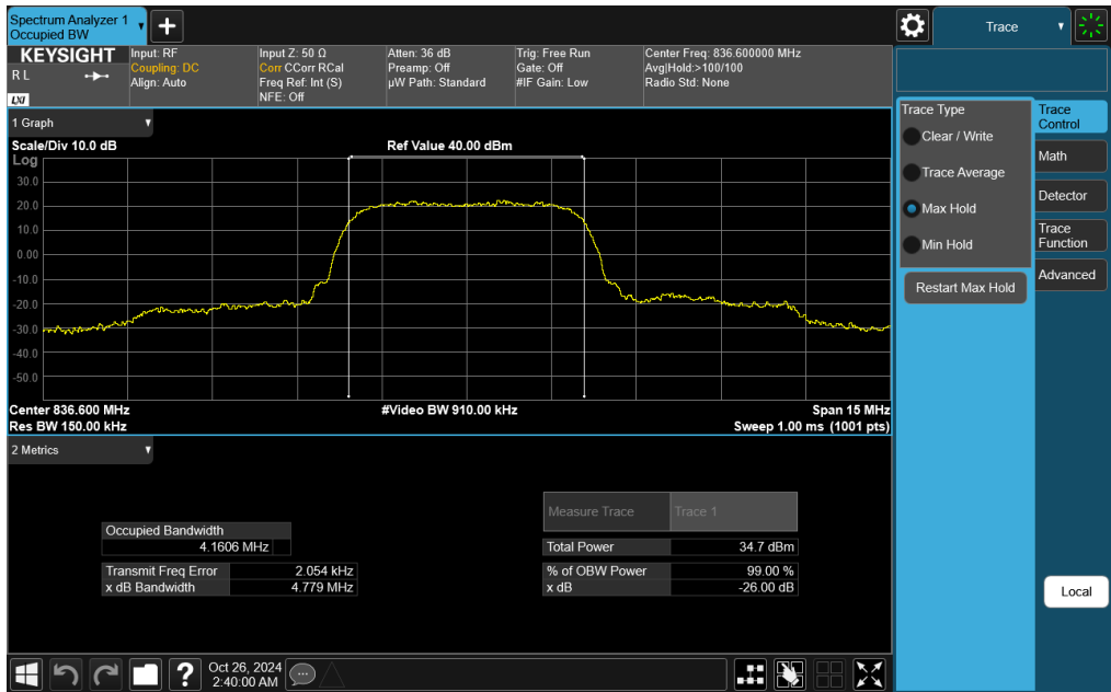
Plot 7-41. Occupied Bandwidth Plot (WCDMA, Ch. 4183)
