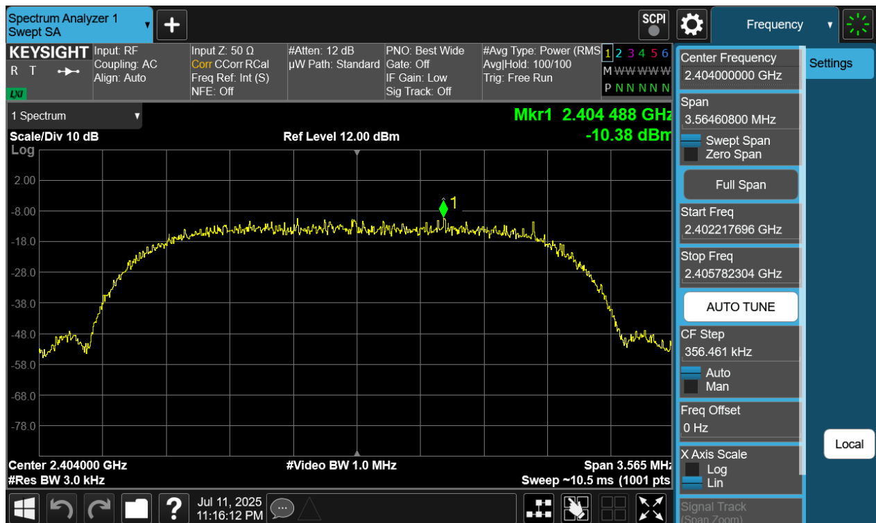
Plot 7-70. Power Spectral Density Plot Antenna WF8 (Bluetooth (HDRPS2), 2Mbps, iPA – Ch. 1)
