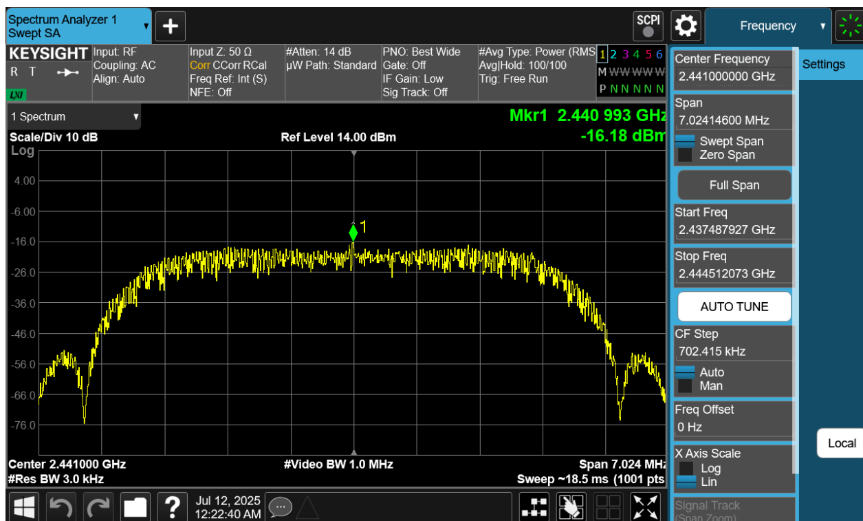
Plot 7-119. Power Spectral Density Plot Antenna WF7 (Bluetooth (HDRPM16), 16Mbps, iPA – Ch. 38)
