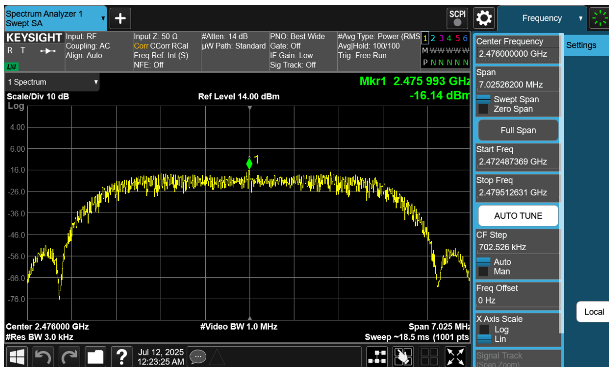
Plot 7-120. Power Spectral Density Plot Antenna WF7 (Bluetooth (HDRPM16), 16Mbps, iPA – Ch. 73)
