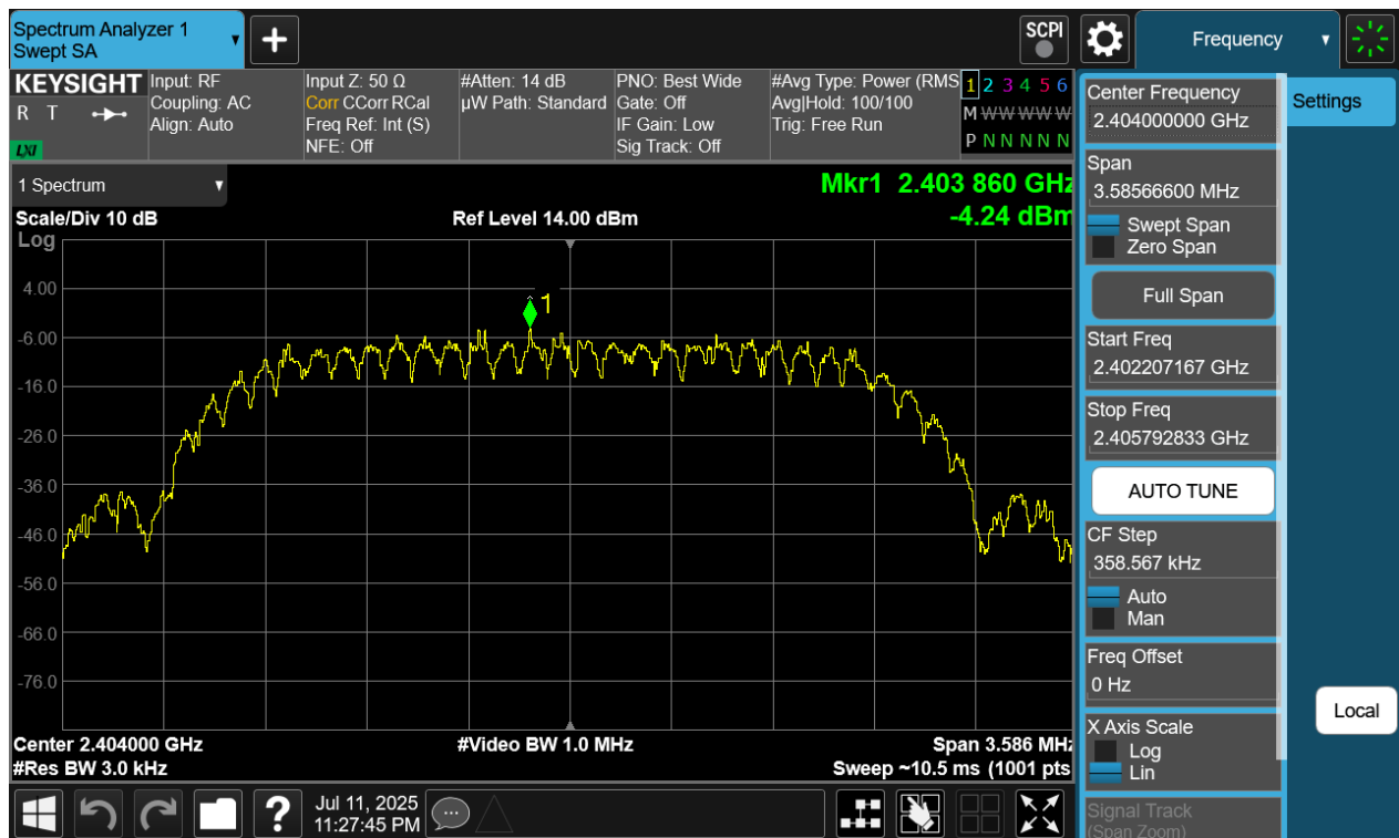
Plot 7-85. Power Spectral Density Plot Antenna WF8 (Bluetooth (HDT2), 2Mbps, ePA – Ch. 1)
