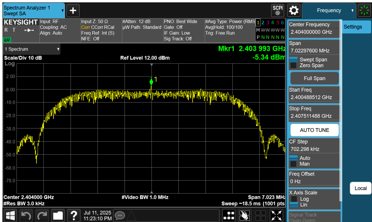
Plot 7-79. Power Spectral Density Plot Antenna WF8 (Bluetooth (HDRPM16), 16Mbps, ePA – Ch. 1)
