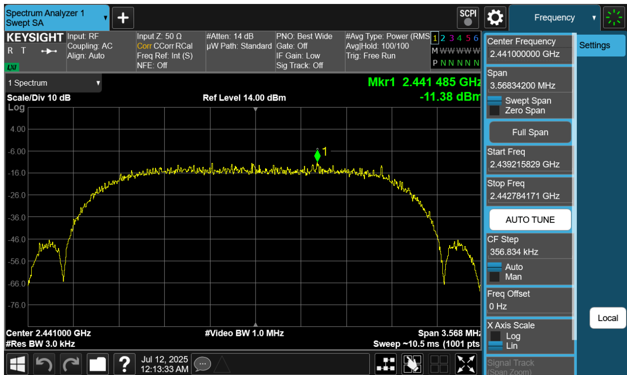
Plot 7-107. Power Spectral Density Plot Antenna WF7 (Bluetooth (HDRPS2), 2Mbps, iPA – Ch. 38)
