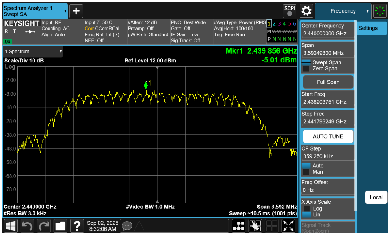
Plot 7-86. Power Spectral Density Plot Antenna WF8 (Bluetooth (HDT2), 2Mbps, ePA – Ch. 37)
