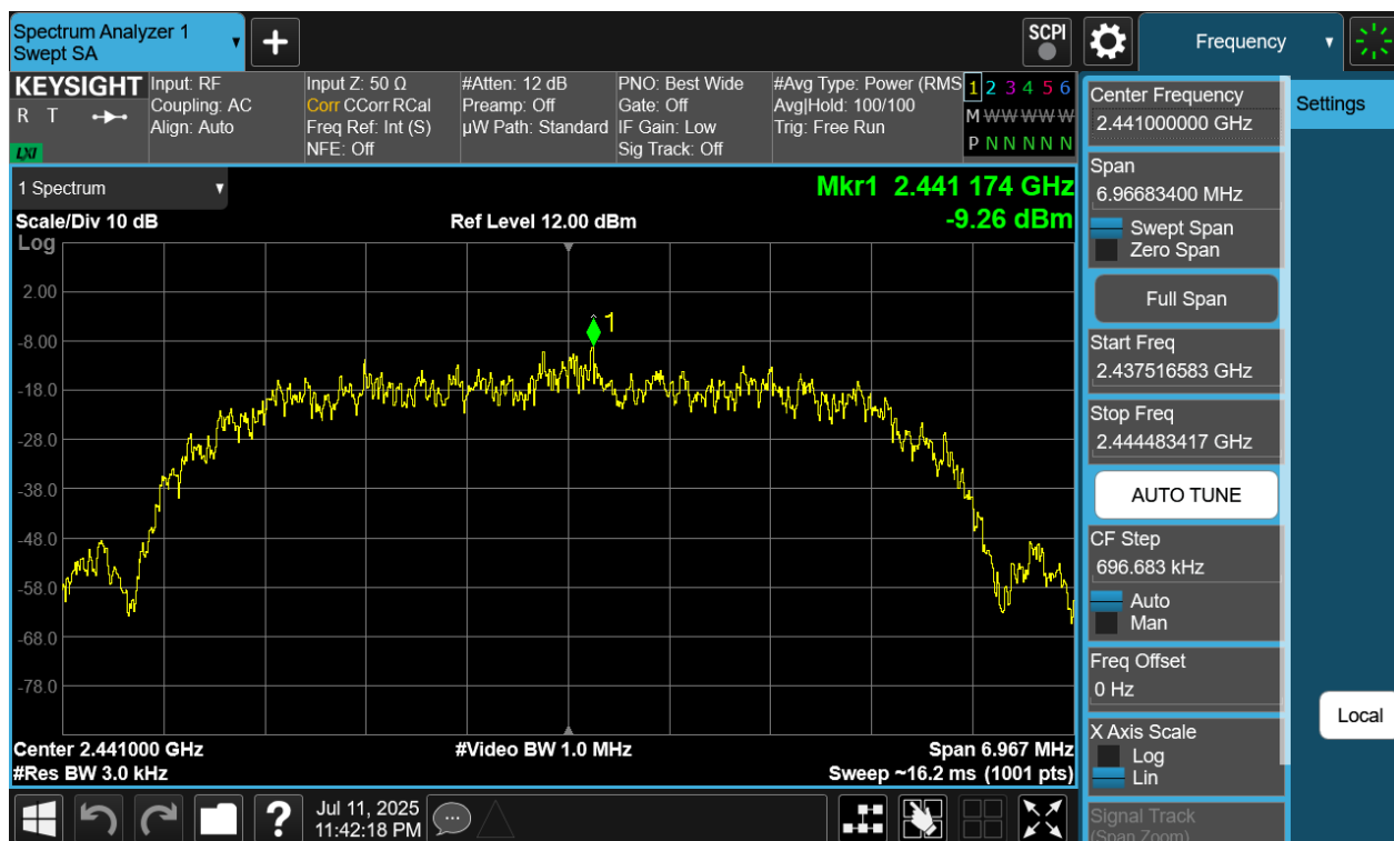
Plot 7-65. Power Spectral Density Plot Antenna WF8 (Bluetooth (HDR8), 8Mbps, iPA – Ch. 38)
