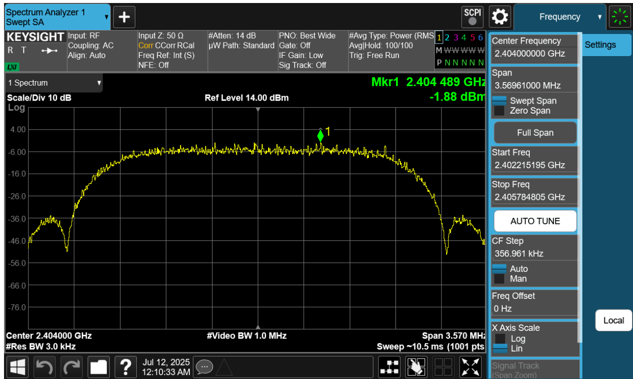
Plot 7-103. Power Spectral Density Plot Antenna WF7 (Bluetooth (HDRPS2), 2Mbps, ePA – Ch. 1)
