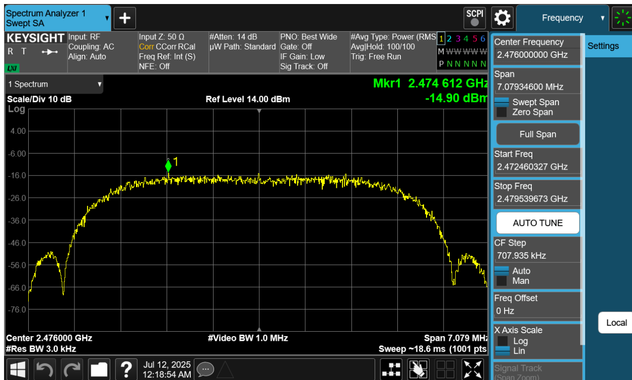
Plot 7-114. Power Spectral Density Plot Antenna WF7 (Bluetooth (XHDRPM6), 6Mbps, iPA - Ch. 73)
