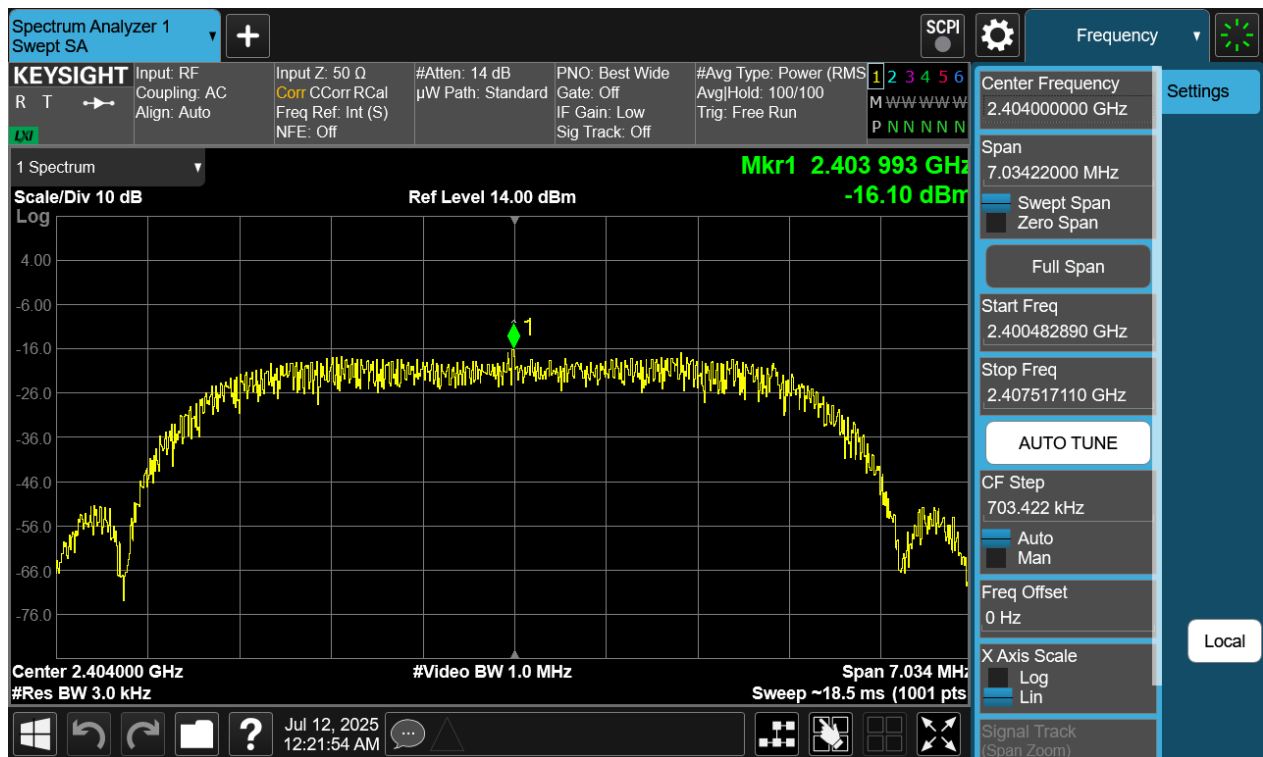
Plot 7-118. Power Spectral Density Plot Antenna WF7 (Bluetooth (HDRPM16), 16Mbps, iPA – Ch. 1)
