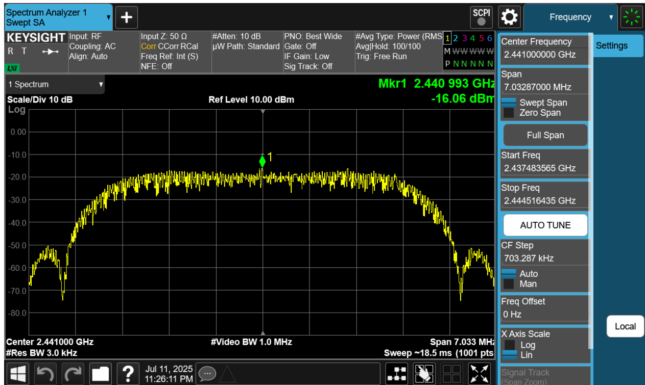
Plot 7-83. Power Spectral Density Plot Antenna WF8 (Bluetooth (HDRPM16), 16Mbps, iPA – Ch. 38)
