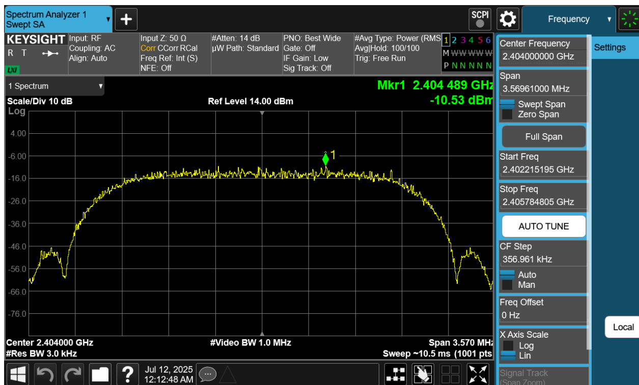
Plot 7-106. Power Spectral Density Plot Antenna WF7 (Bluetooth (HDRPS2), 2Mbps, iPA – Ch. 1)
