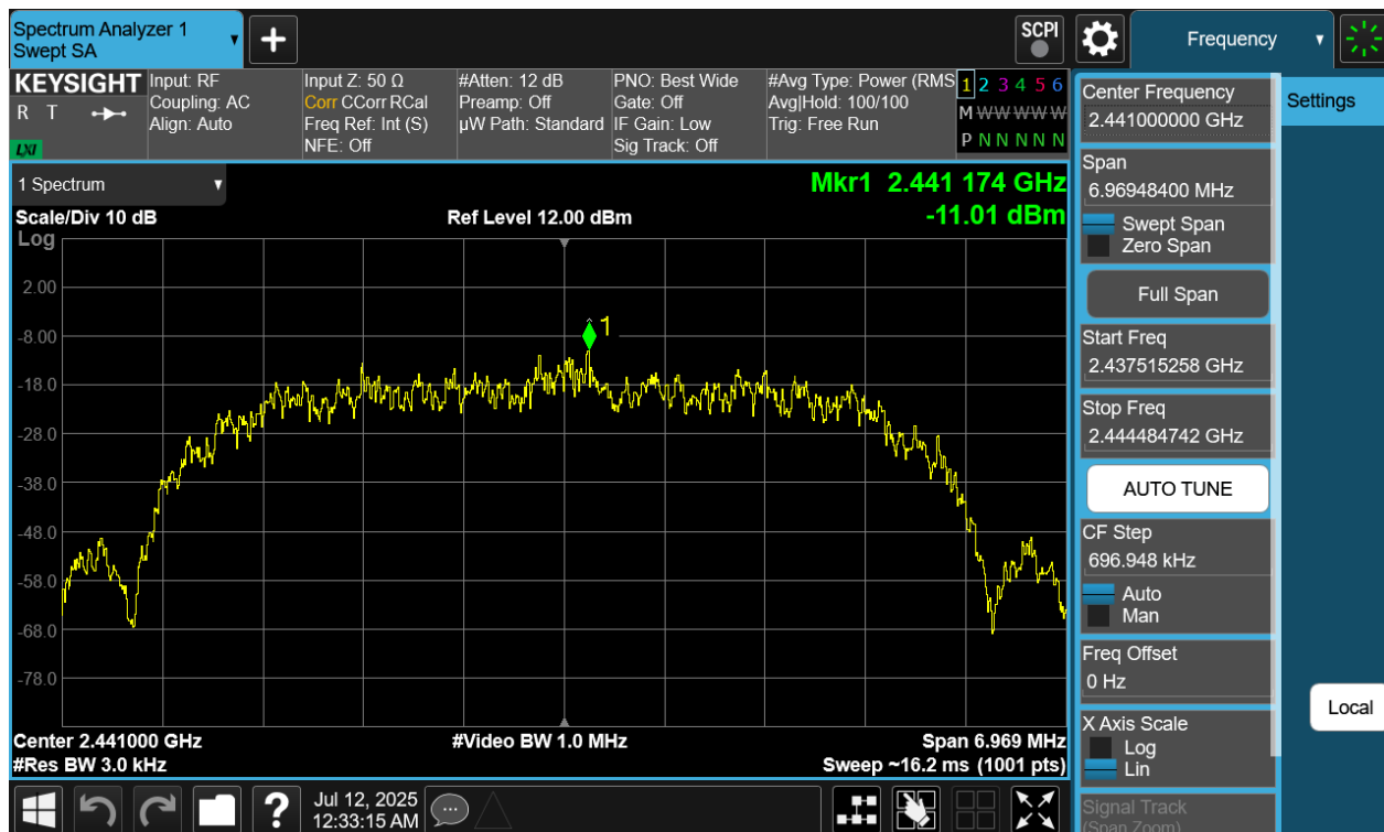
Plot 7-101. Power Spectral Density Plot Antenna WF7 (Bluetooth (HDR8), 8Mbps, iPA – Ch. 38)
