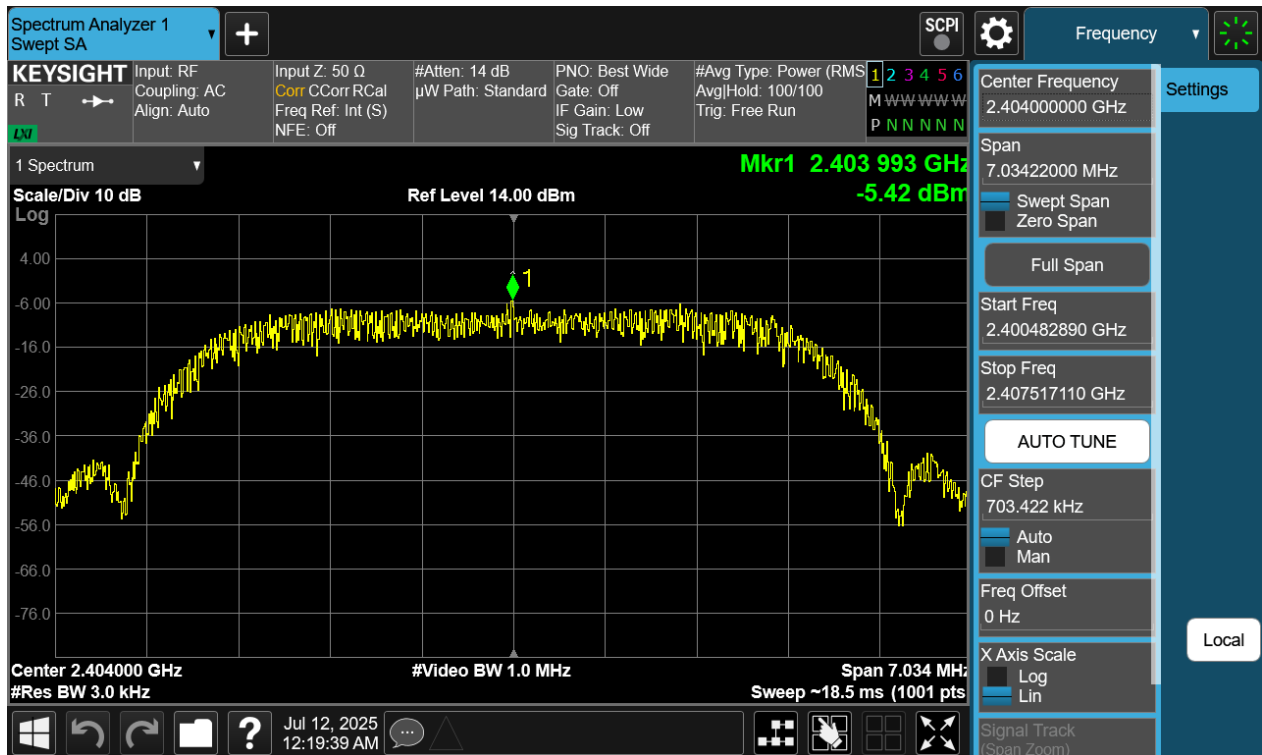
Plot 7-115. Power Spectral Density Plot Antenna WF7 (Bluetooth (HDRPM16), 16Mbps, ePA – Ch. 1)
