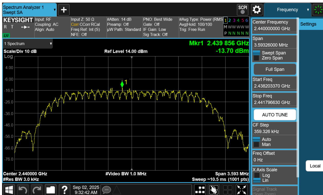
Plot 7-232. Power Spectral Density Plot TxBF Primary Antenna WF7 (Bluetooth (HDT2), 2Mbps, iPA – Ch. 37)
