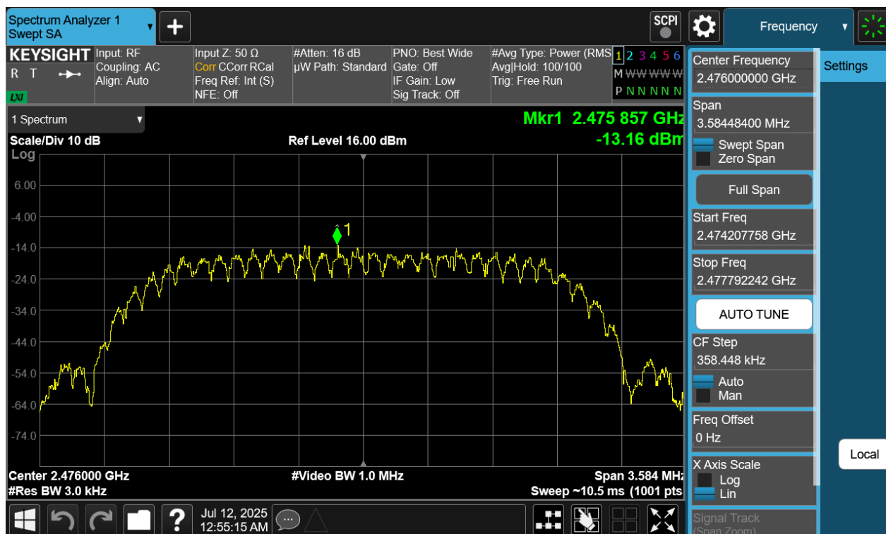
Plot 7-234. Power Spectral Density Plot TxBF Primary Antenna WF7 (Bluetooth (HDT2), 2Mbps, iPA – Ch. 73)
