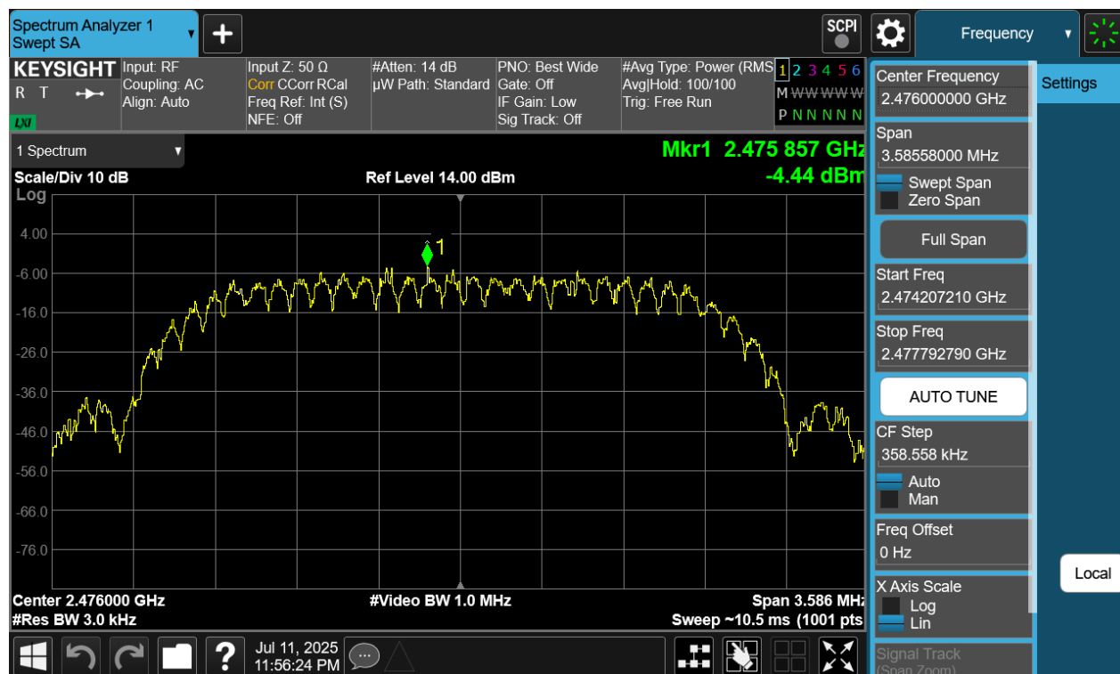
Plot 7-227. Power Spectral Density Plot TxBF Primary Antenna WF8 (Bluetooth (HDT2), 2Mbps, ePA – Ch. 73)
