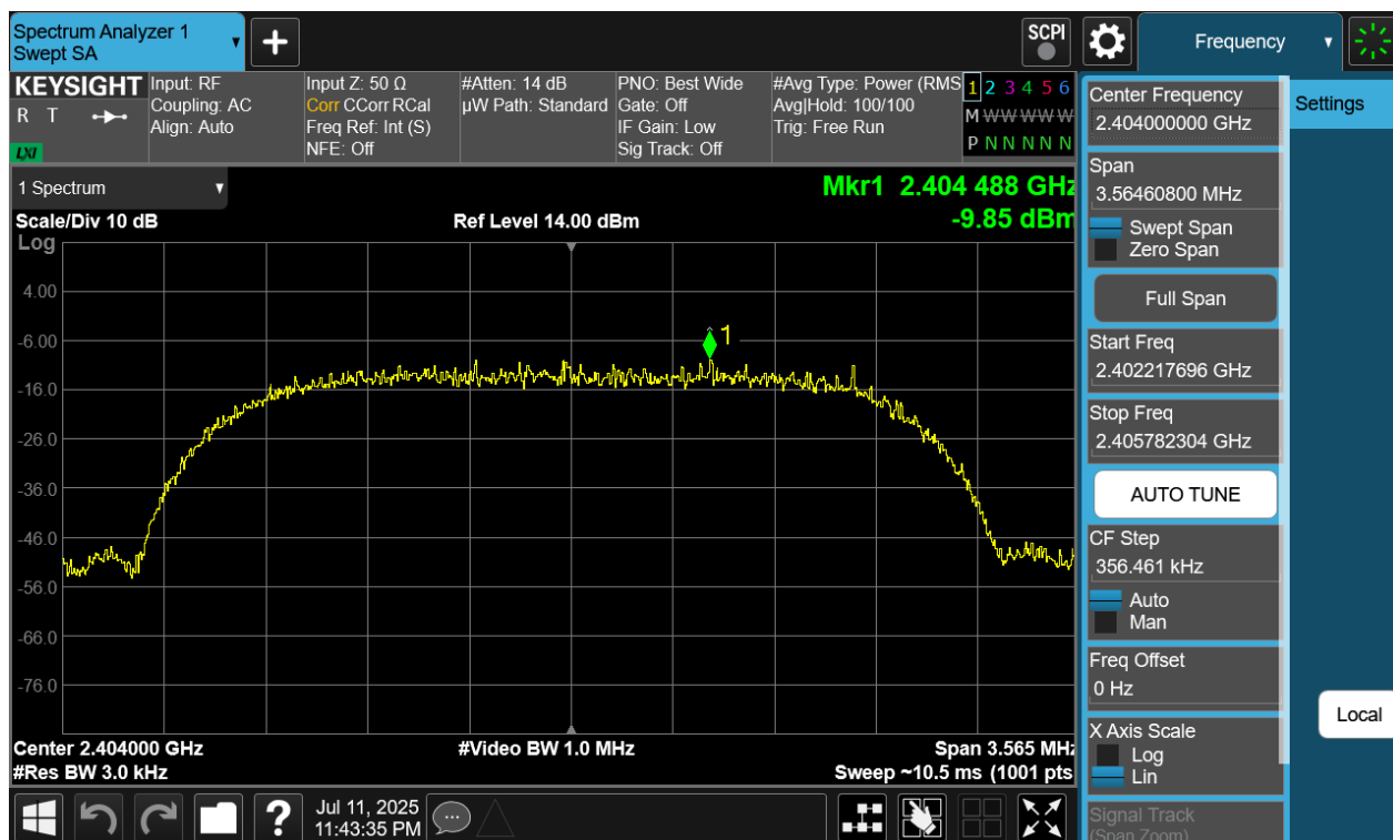
Plot 7-193. Power Spectral Density Plot Tx BF Primary Antenna WF8 (Bluetooth (HDRPS2), 8Mbps, iPA – Ch. 1)
