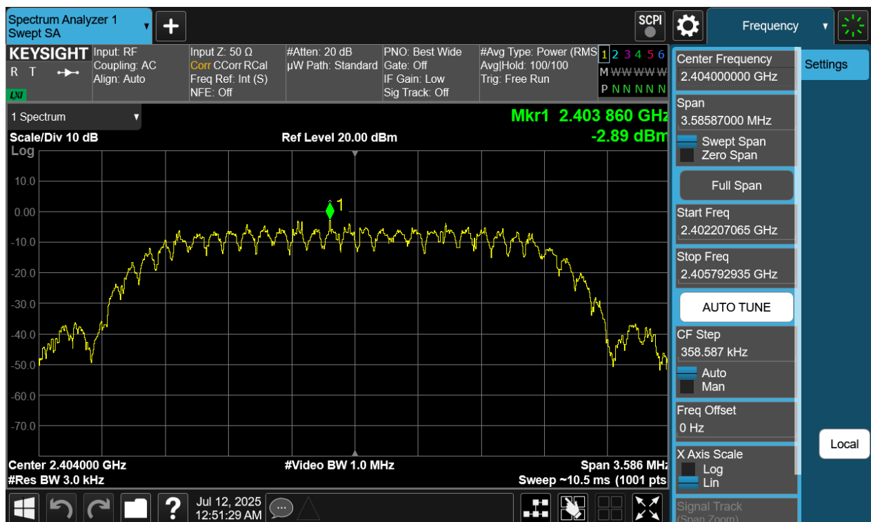
Plot 7-224. Power Spectral Density Plot Tx BF Primary Antenna WF7 (Bluetooth (HDT2), 2Mbps, ePA – Ch. 1)
