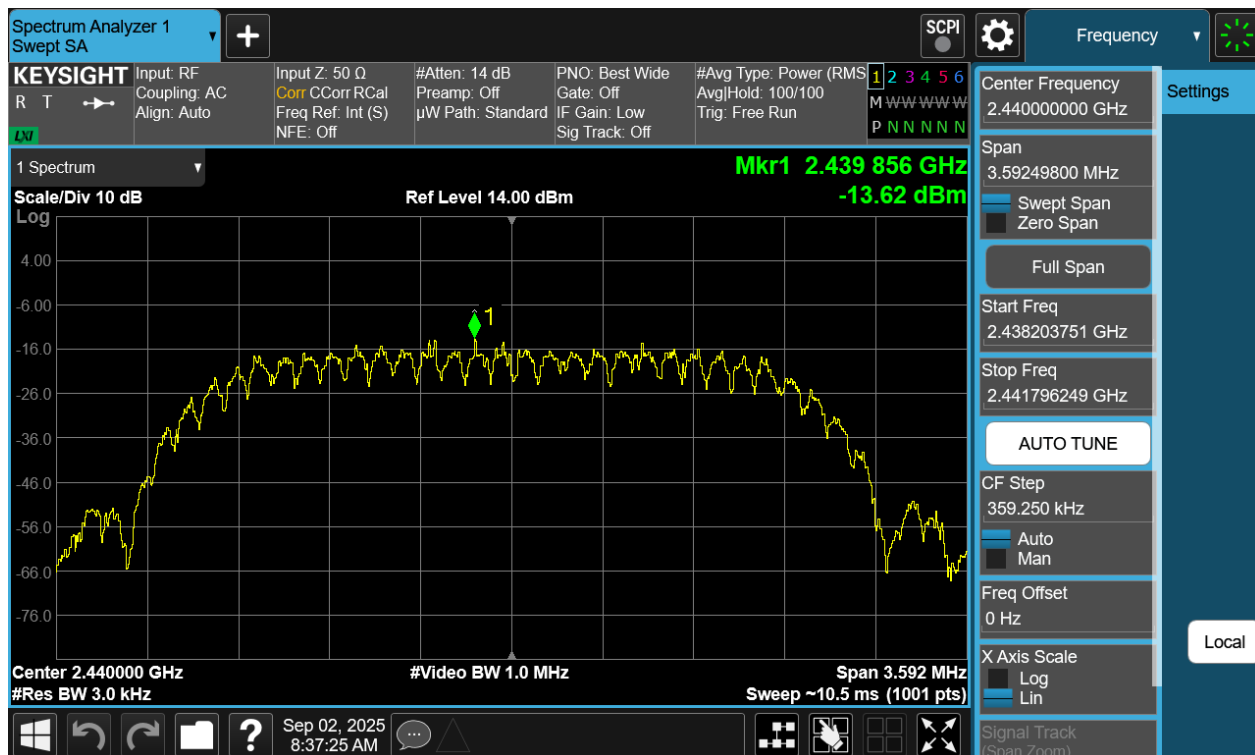
Plot 7-231. Power Spectral Density Plot TxBF Primary Antenna WF8 (Bluetooth (HDT2), 2Mbps, iPA – Ch. 37)
