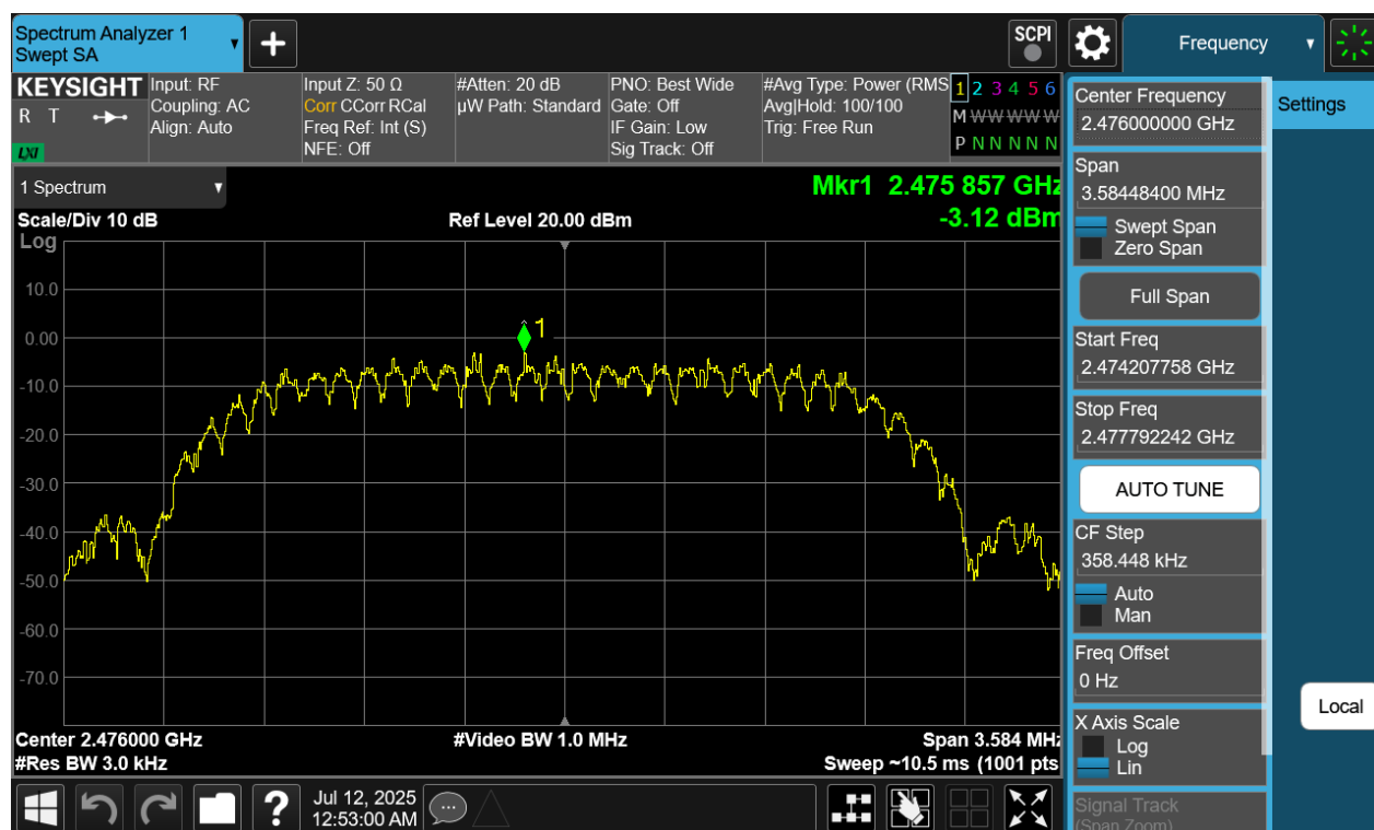
Plot 7-228. Power Spectral Density Plot TxBF Primary Antenna WF7 (Bluetooth (HDT2), 2Mbps, ePA – Ch. 73)
