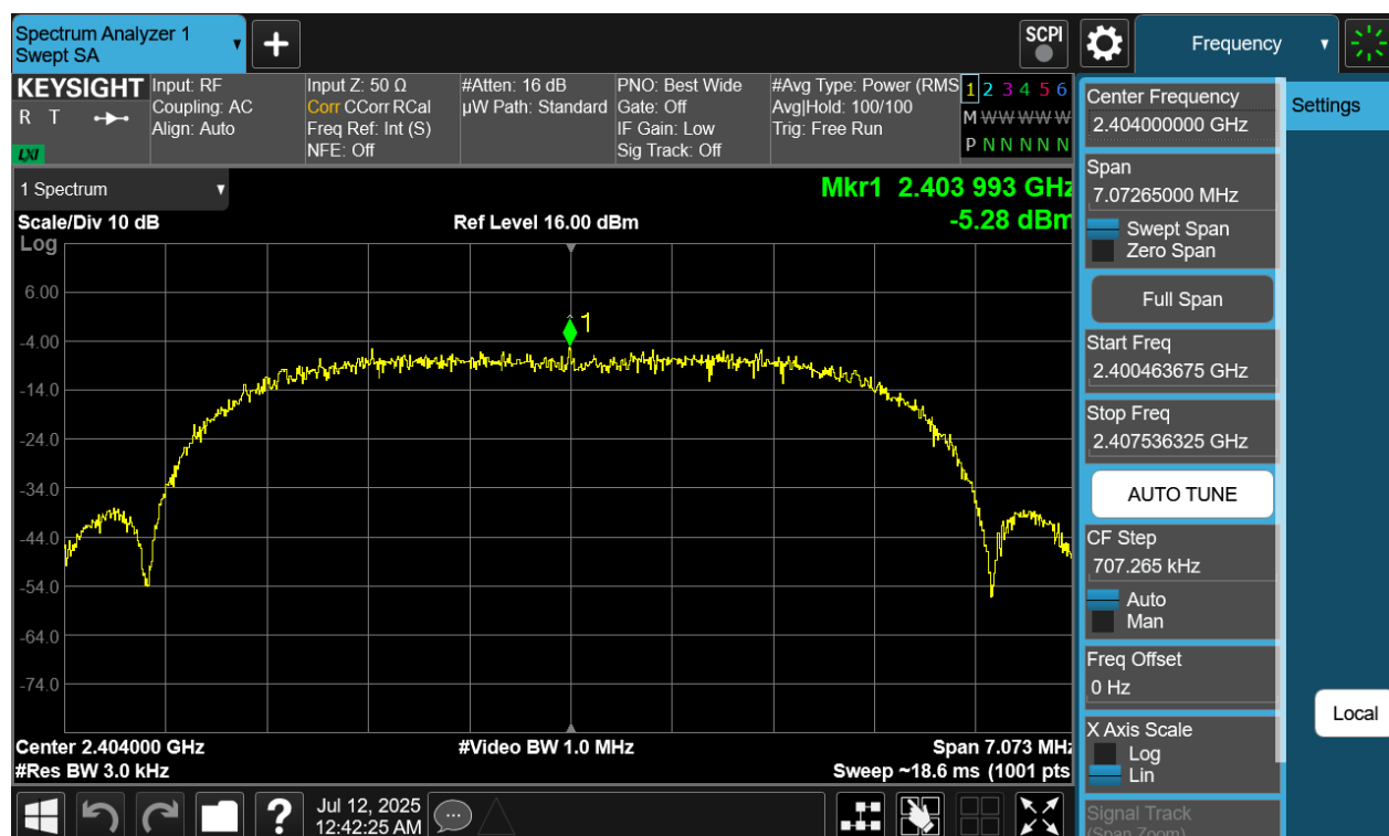
Plot 7-200. Power Spectral Density Plot Tx BF Primary Antenna WF7 (Bluetooth (XHDRPM6), 6Mbps, ePA – Ch. 1)
