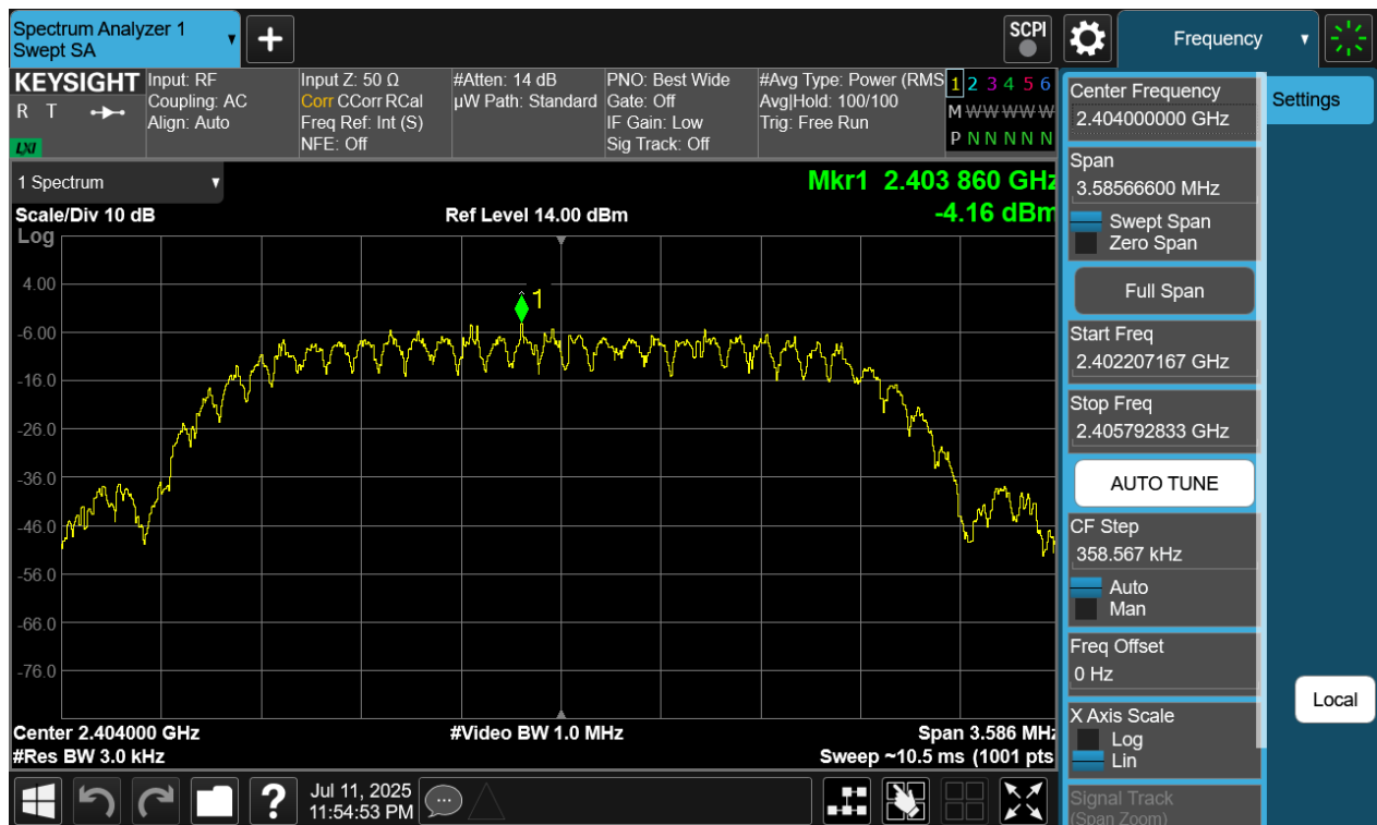
Plot 7-223. Power Spectral Density Plot Tx BF Primary Antenna WF8 (Bluetooth (HDT2), 2Mbps, ePA – Ch. 1)
