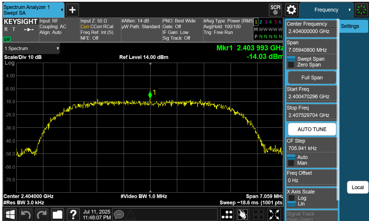
Plot 7-205. Power Spectral Density Plot Tx BF Primary Antenna WF8 (Bluetooth (XHDRPM6), 6Mbps, iPA – Ch. 1)
