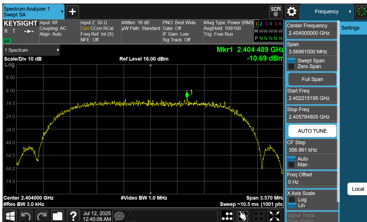
Plot 7-194. Power Spectral Density Plot Tx BF Primary Antenna WF7 (Bluetooth (HDRPS2), 8Mbps, iPA – Ch. 1)
