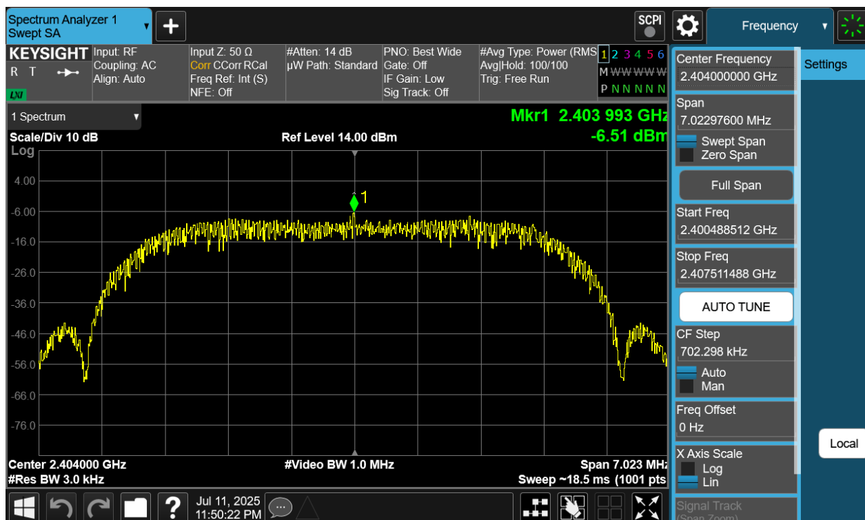
Plot 7-211. Power Spectral Density Plot Tx BF Primary Antenna WF8 (Bluetooth (HDRPM16), 16Mbps, ePA – Ch. 1)
