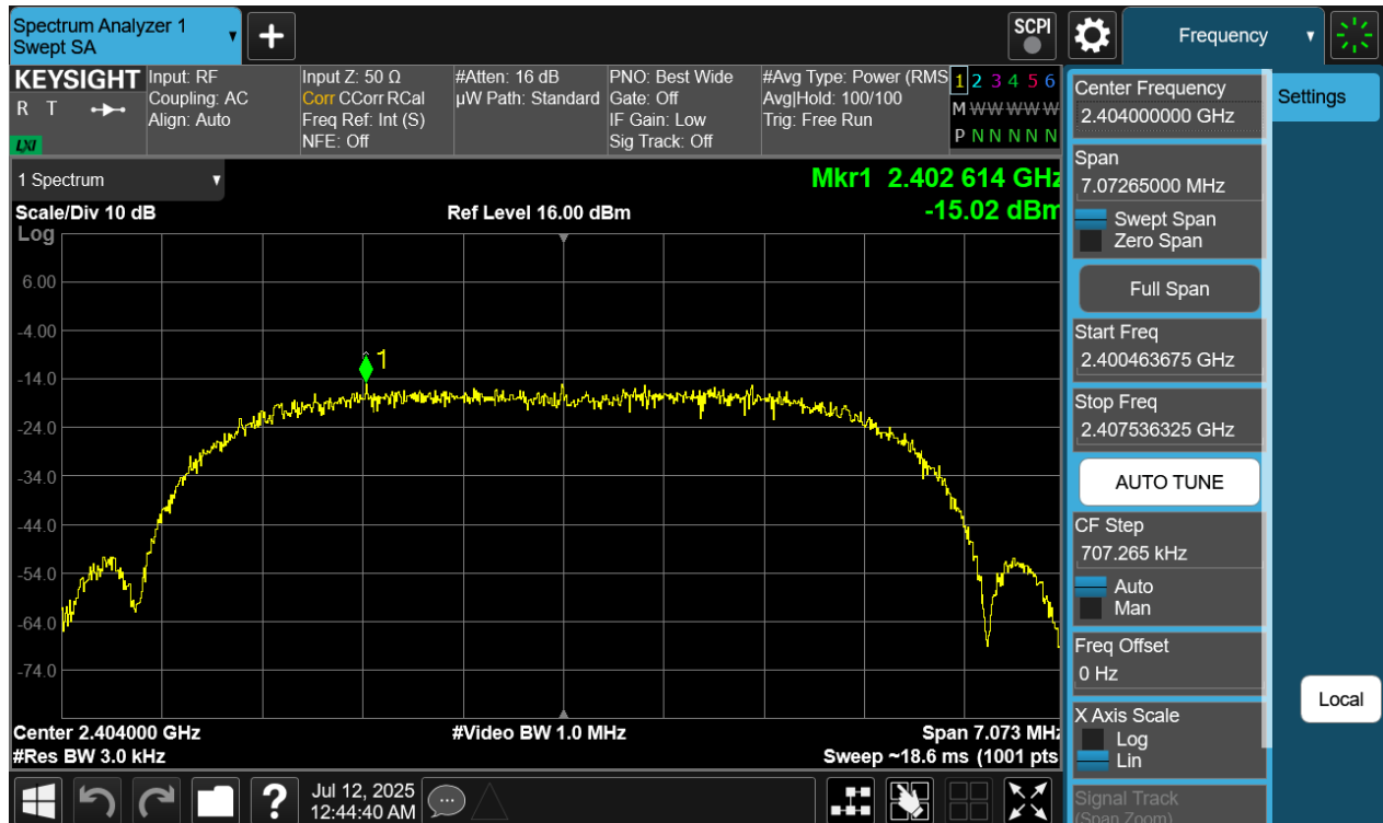
Plot 7-206. Power Spectral Density Plot Tx BF Primary Antenna WF7 (Bluetooth (XHDRPM6), 6Mbps, iPA – Ch. 1)
