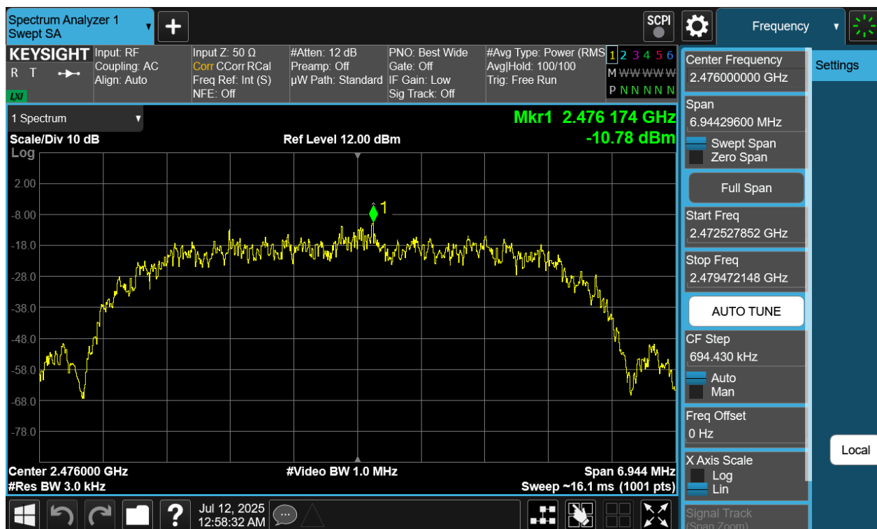
Plot 7-186. Power Spectral Density Plot Tx BF Primary Antenna WF7 (Bluetooth (HDR8), 8Mbps, iPA – Ch. 73)
