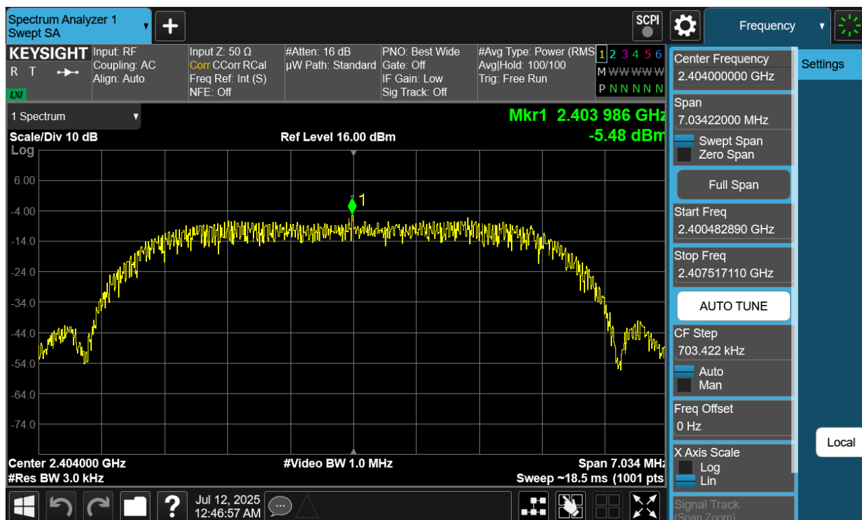
Plot 7-212. Power Spectral Density Plot Tx BF Primary Antenna WF7 (Bluetooth (HDRPM16), 16Mbps, ePA – Ch. 1)
