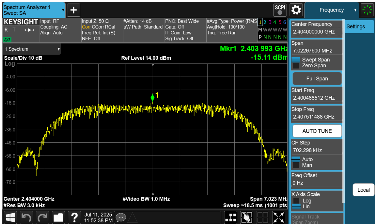
Plot 7-217. Power Spectral Density Plot Tx BF Primary Antenna WF8 (Bluetooth (HDRPM16), 16Mbps, iPA – Ch. 1)
