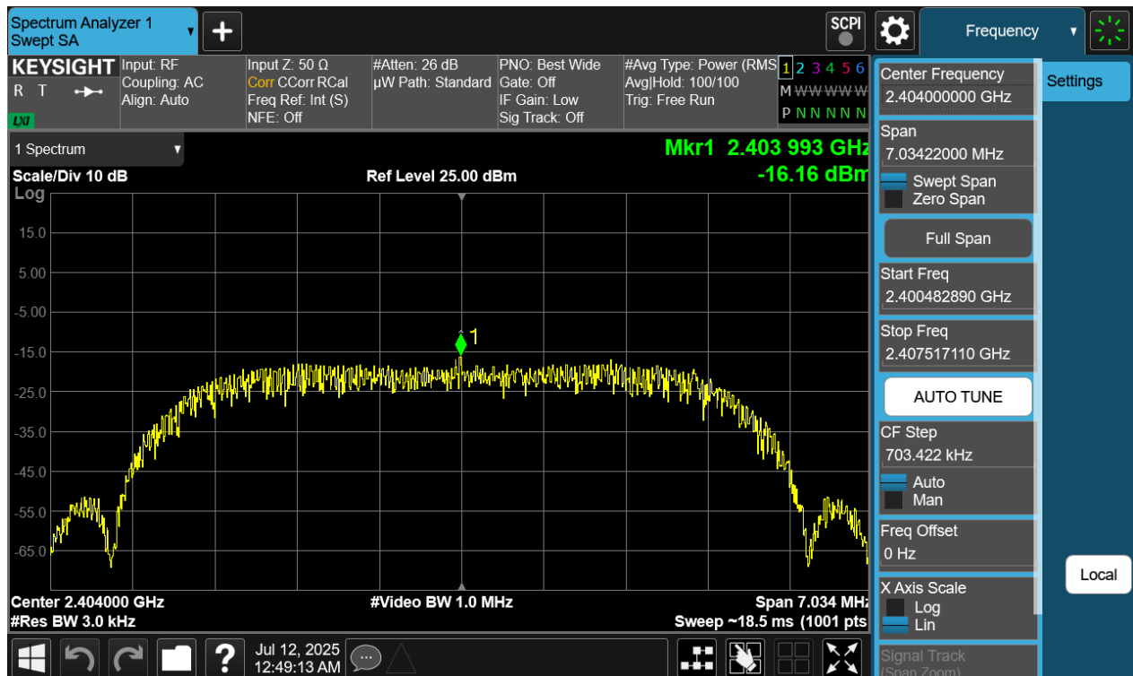
Plot 7-218. Power Spectral Density Plot Tx BF Primary Antenna WF7 (Bluetooth (HDRPM16), 16Mbps, iPA – Ch. 1)
