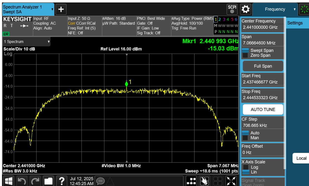
Plot 7-208. Power Spectral Density Plot TxBF Primary Antenna WF7 (Bluetooth (XHDRPM6), 6Mbps, iPA – Ch. 38)
