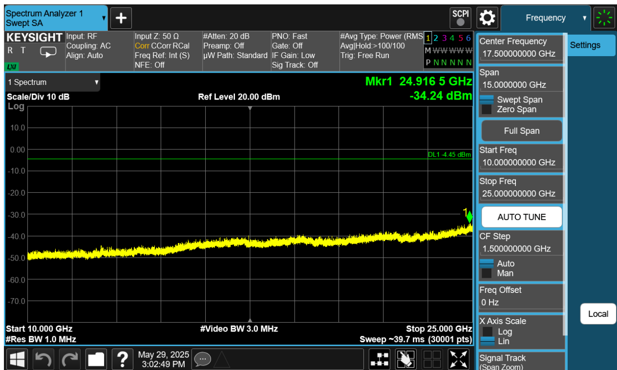
Plot 7-432. Conducted Spurious Plot Antenna WF9 (Bluetooth (HDT2), 2Mbps, ePA – Ch. 73)
