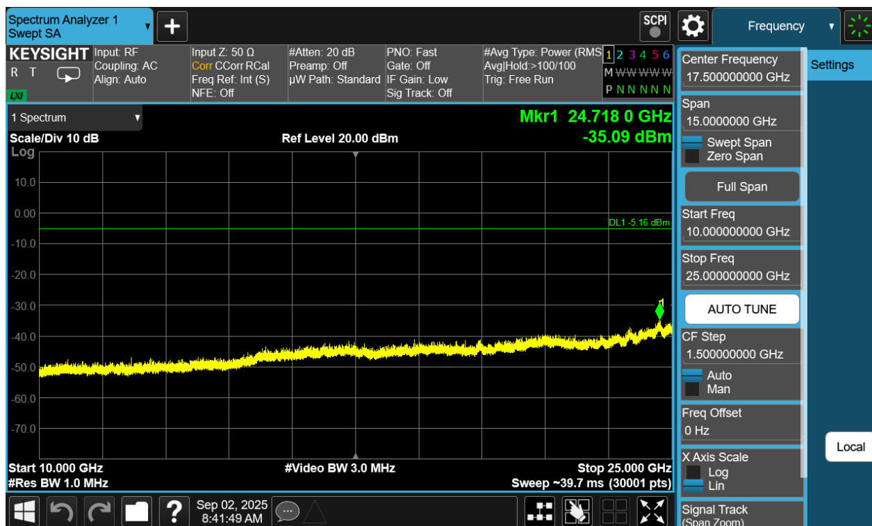
Plot 7-370. Conducted Spurious Plot Antenna WF8 (Bluetooth (HDT2), 2Mbps, ePA – Ch. 37)
