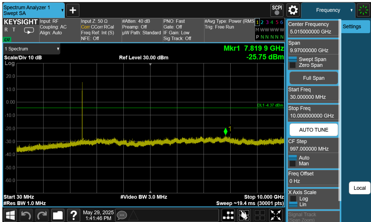
Plot 7-401. Conducted Spurious Plot Antenna WF7 (Bluetooth (HDT2), 2Mbps, ePA – Ch. 73)
