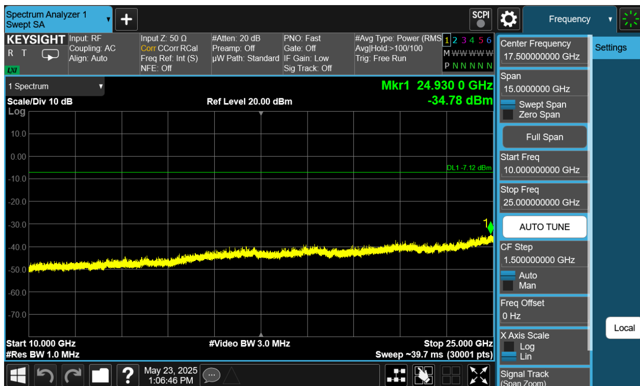
Plot 7-378. Conducted Spurious Plot Antenna WF7 (Bluetooth (HDR4), 4 Mbps, ePA – Ch. 73)
