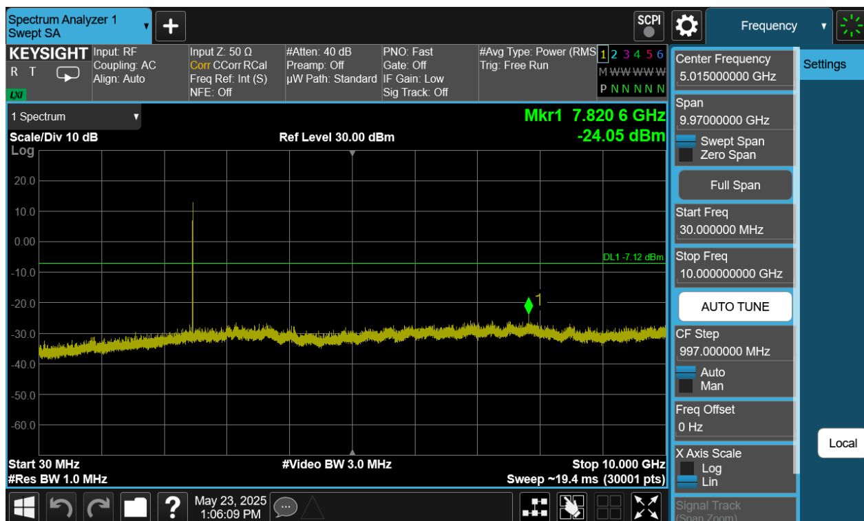
Plot 7-377. Conducted Spurious Plot Antenna WF7 (Bluetooth (HDR4), 4 Mbps, ePA – Ch. 73)
