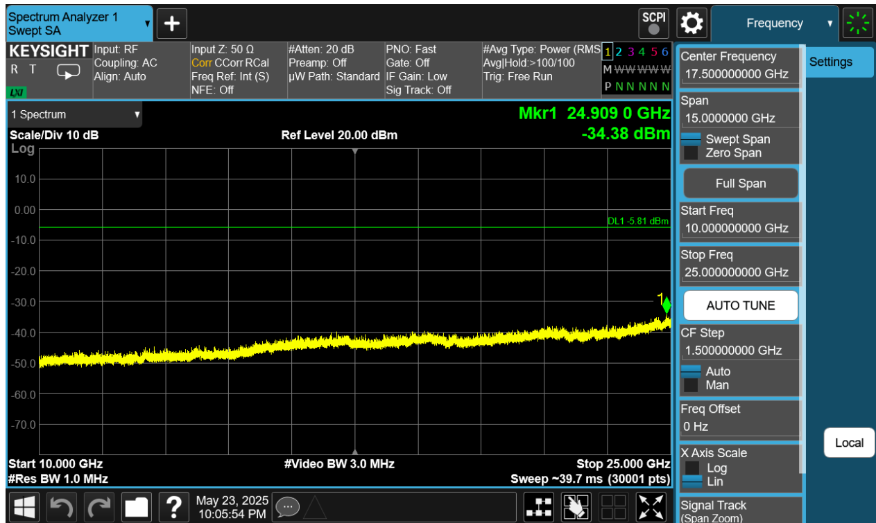
Plot 7-406. Conducted Spurious Plot Antenna WF9 (Bluetooth (HDR4), 4 Mbps, ePA – Ch. 38)
