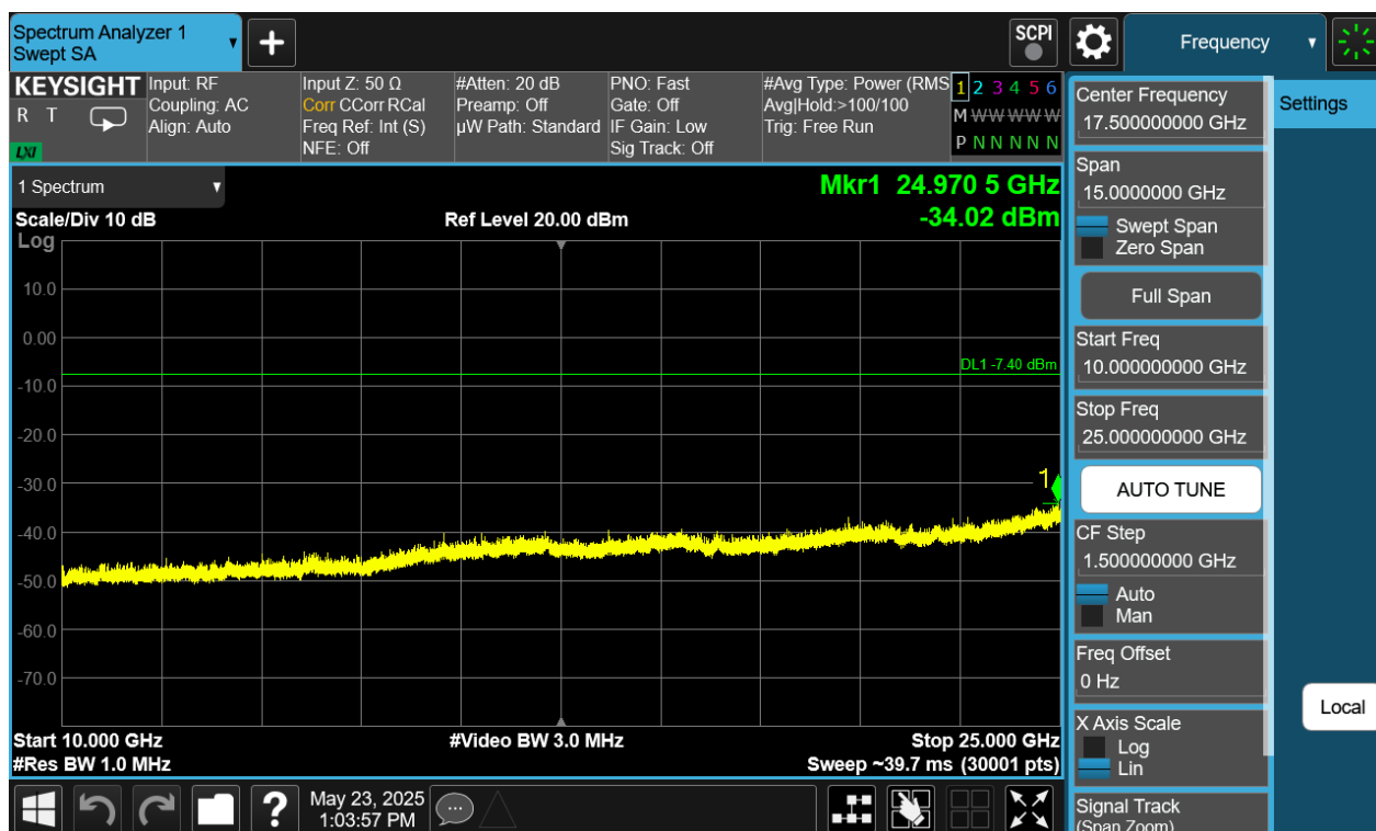
Plot 7-374. Conducted Spurious Plot Antenna WF7 (Bluetooth (HDR4), 4 Mbps, ePA – Ch. 1)
