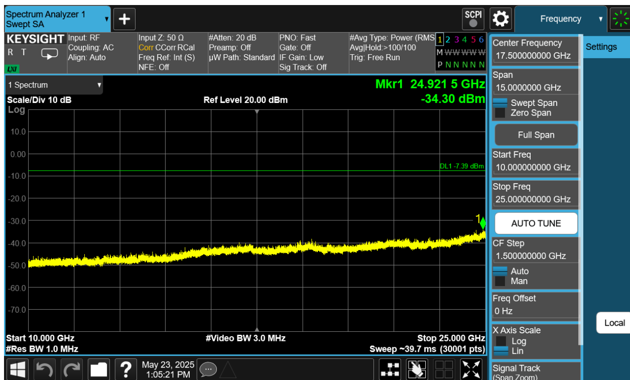
Plot 7-376. Conducted Spurious Plot Antenna WF7 (Bluetooth (HDR4), 4 Mbps, ePA – Ch. 38)
