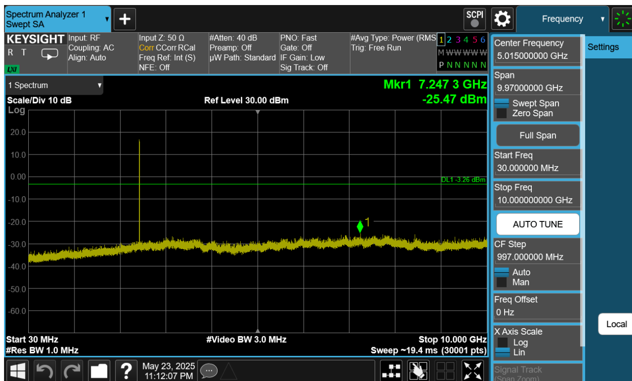
Plot 7-411. Conducted Spurious Plot Antenna WF9 (Bluetooth (HDRPS2), 8Mbps, ePA – Ch. 38)
