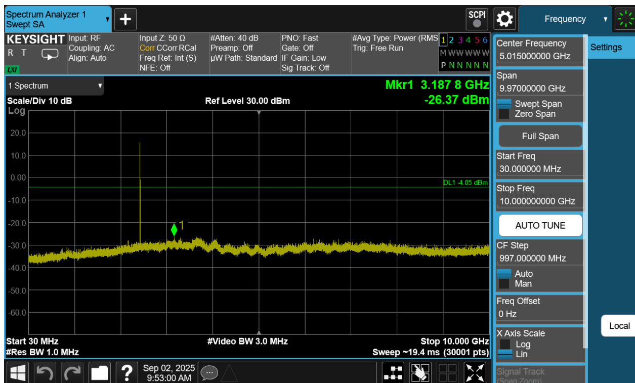
Plot 7-429. Conducted Spurious Plot Antenna WF9 (Bluetooth (HDT2), 2Mbps, ePA – Ch. 37)
