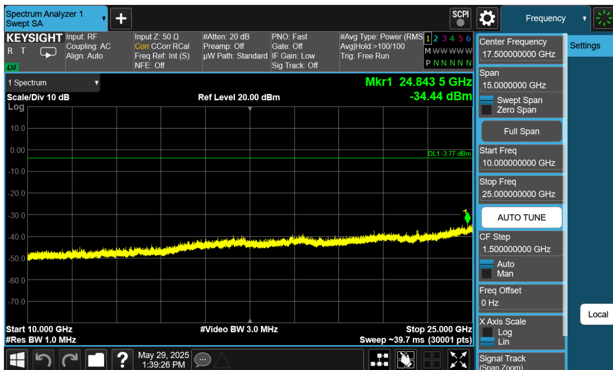
Plot 7-398. Conducted Spurious Plot Antenna WF7 (Bluetooth (HDT2), 2Mbps, ePA – Ch. 1)
