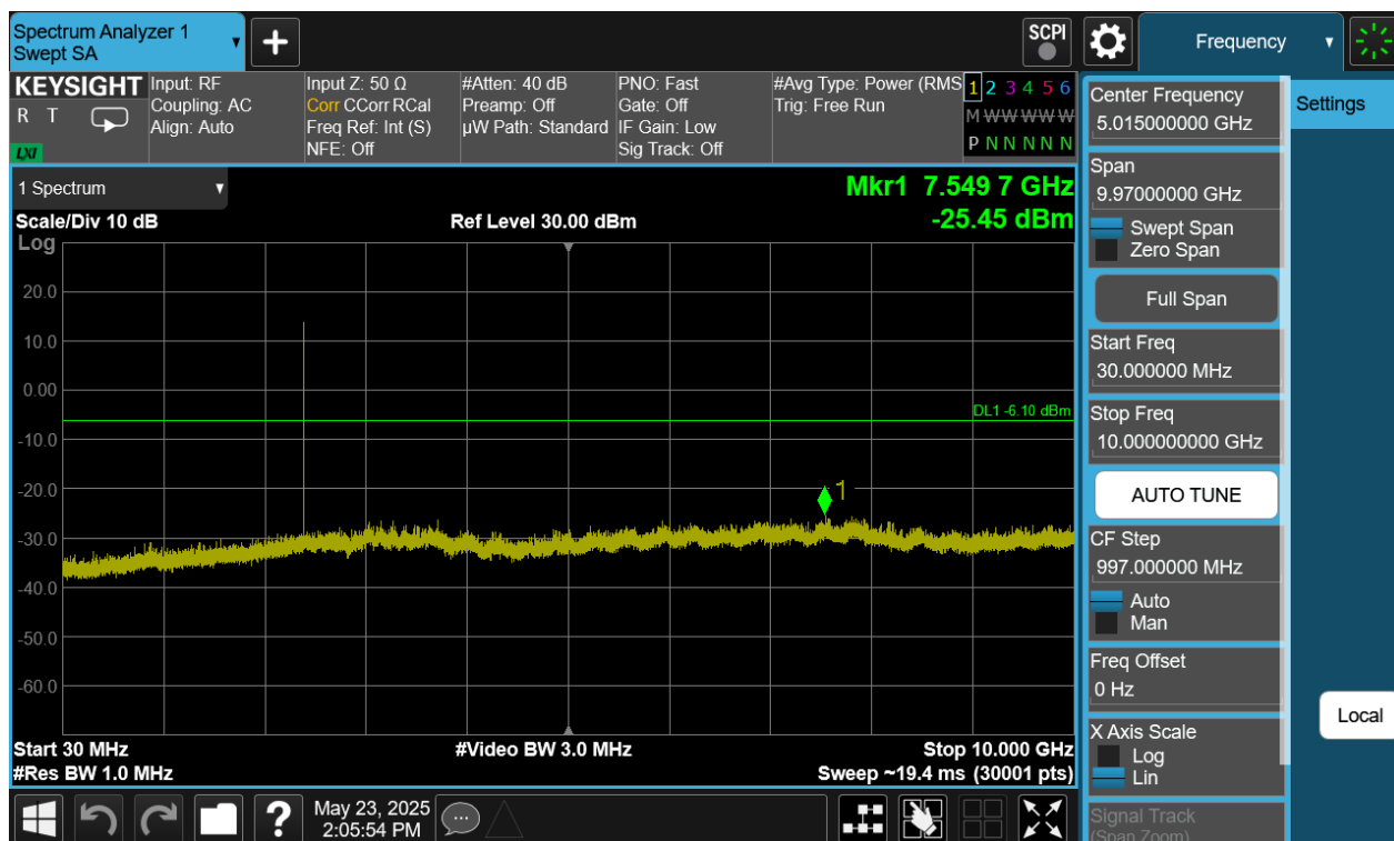
Plot 7-379. Conducted Spurious Plot Antenna WF7 (Bluetooth (HDRPS2), 8Mbps, ePA – Ch. 1)
