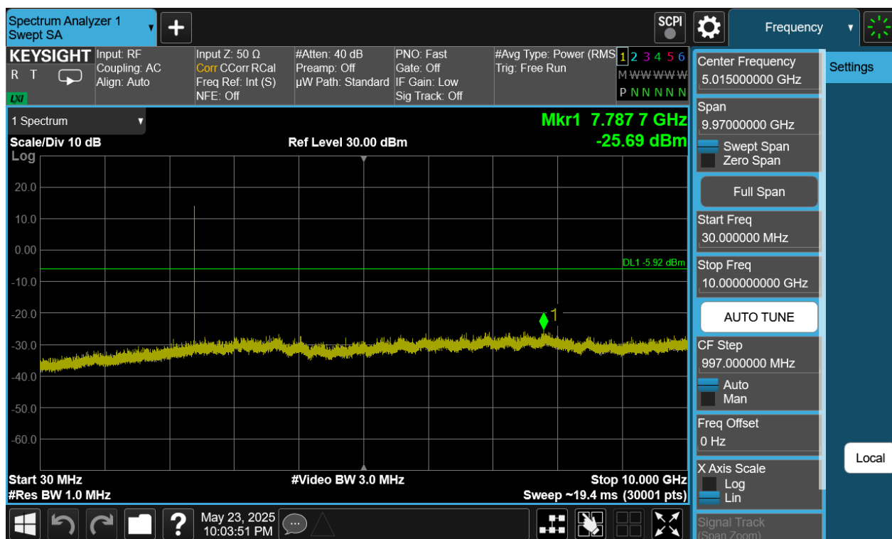
Plot 7-403. Conducted Spurious Plot Antenna WF9 (Bluetooth (HDR4), 4 Mbps, ePA – Ch. 1)
