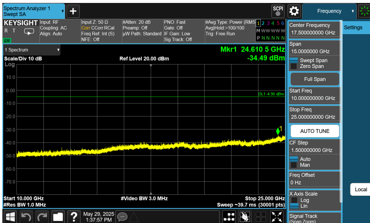
Plot 7-396. Conducted Spurious Plot Antenna WF7 (Bluetooth (HDRPM16), 16Mbps, ePA – Ch. 73)
