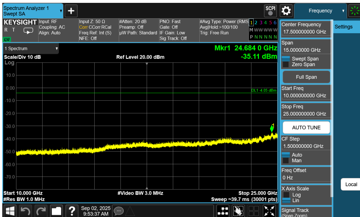
Plot 7-430. Conducted Spurious Plot Antenna WF9 (Bluetooth (HDT2), 2Mbps, ePA – Ch. 37)
