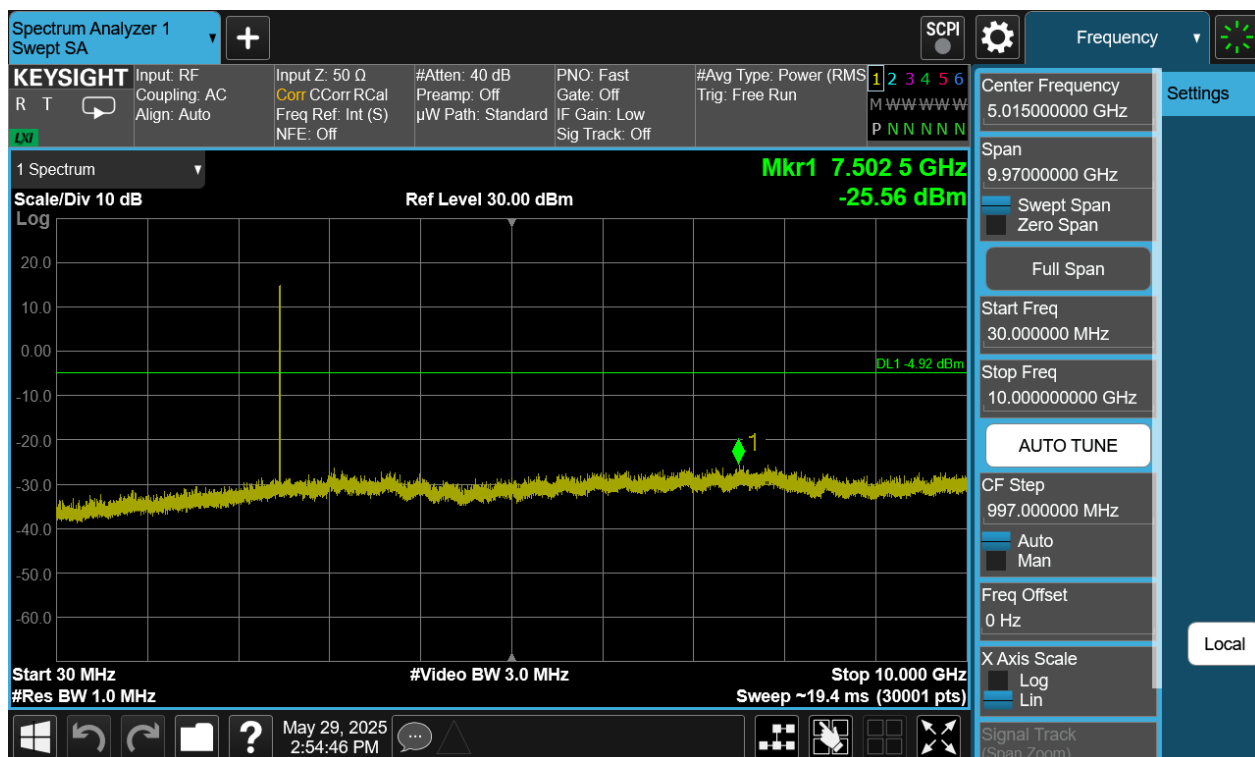
Plot 7-419. Conducted Spurious Plot Antenna WF9 (Bluetooth (XHDRPM6), 6Mbps, ePA – Ch. 73)
