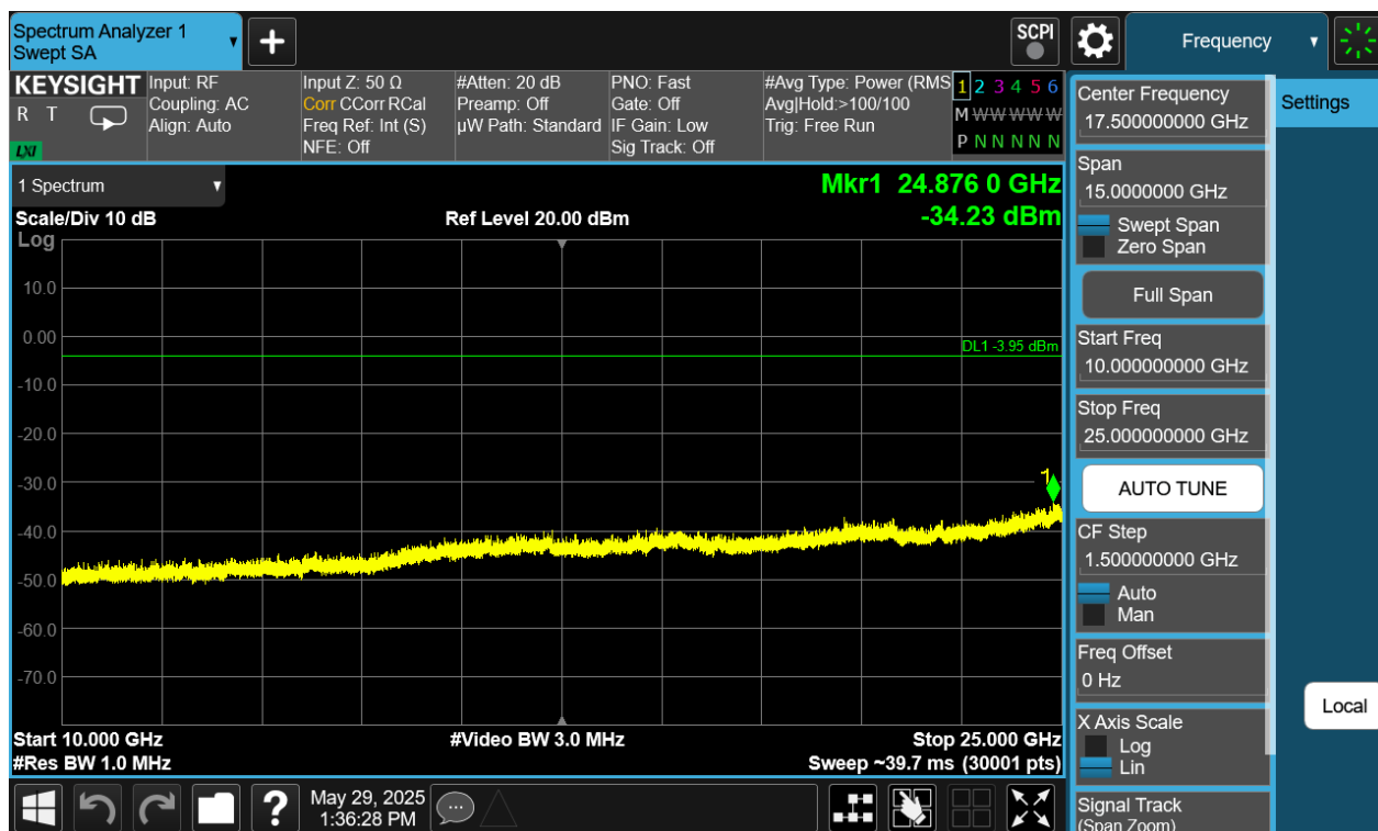
Plot 7-392. Conducted Spurious Plot Antenna WF7 (Bluetooth (HDRPM16), 16Mbps, ePA – Ch. 1)
