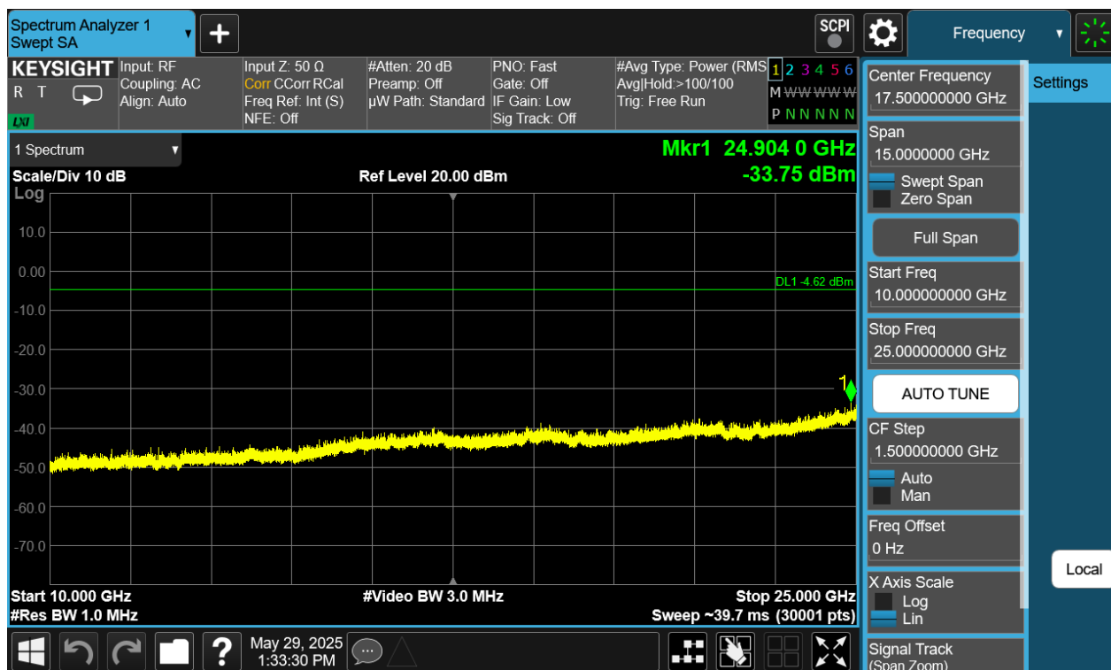
Plot 7-386. Conducted Spurious Plot Antenna WF7 (Bluetooth (XHDRPM6), 6Mbps, ePA – Ch. 1)
