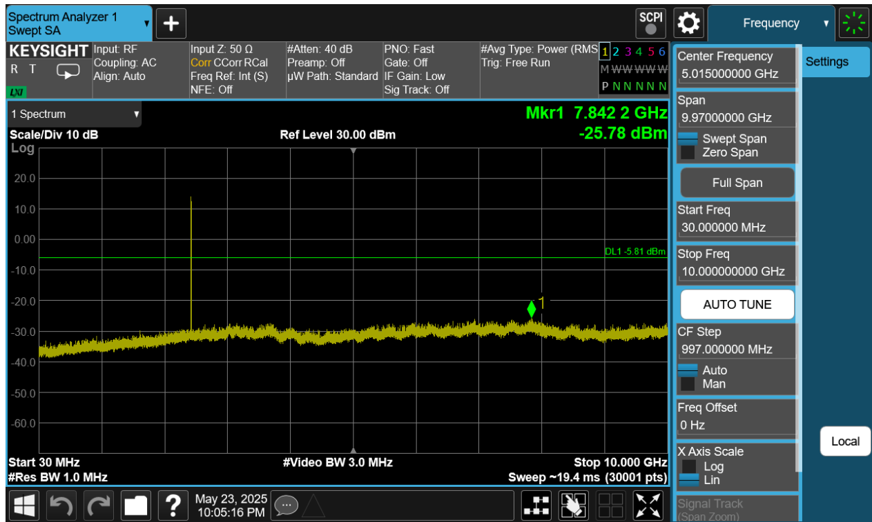
Plot 7-405. Conducted Spurious Plot Antenna WF9 (Bluetooth (HDR4), 4 Mbps, ePA – Ch. 38)
