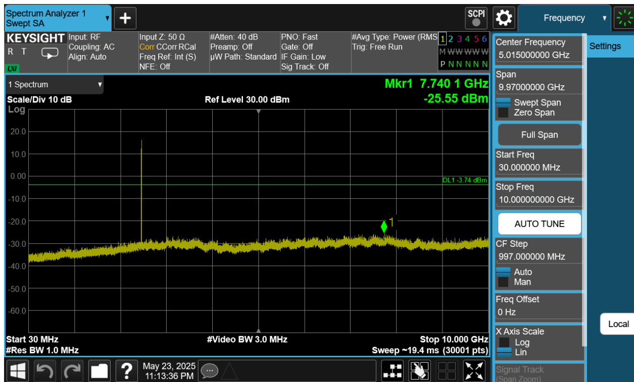
Plot 7-413. Conducted Spurious Plot Antenna WF9 (Bluetooth (HDRPS2), 8Mbps, ePA – Ch. 73)
