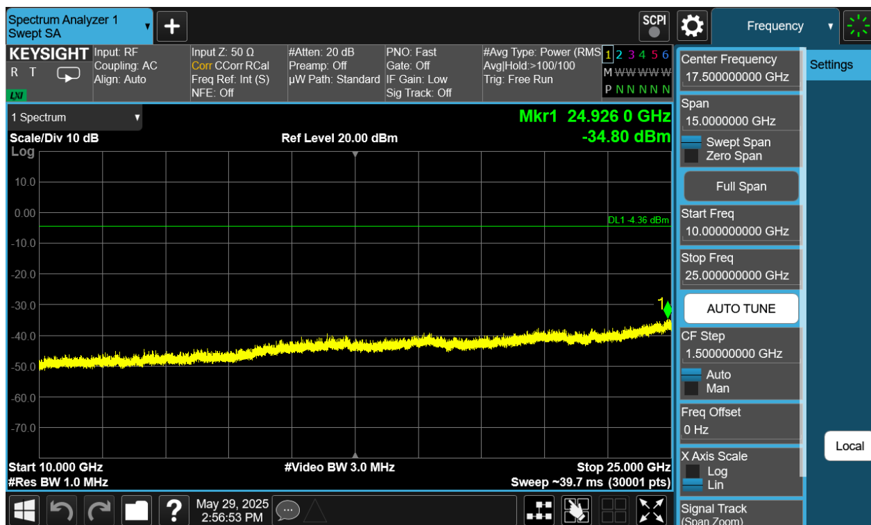
Plot 7-422. Conducted Spurious Plot Antenna WF9 (Bluetooth (HDRPM16), 16Mbps, ePA – Ch. 1)
