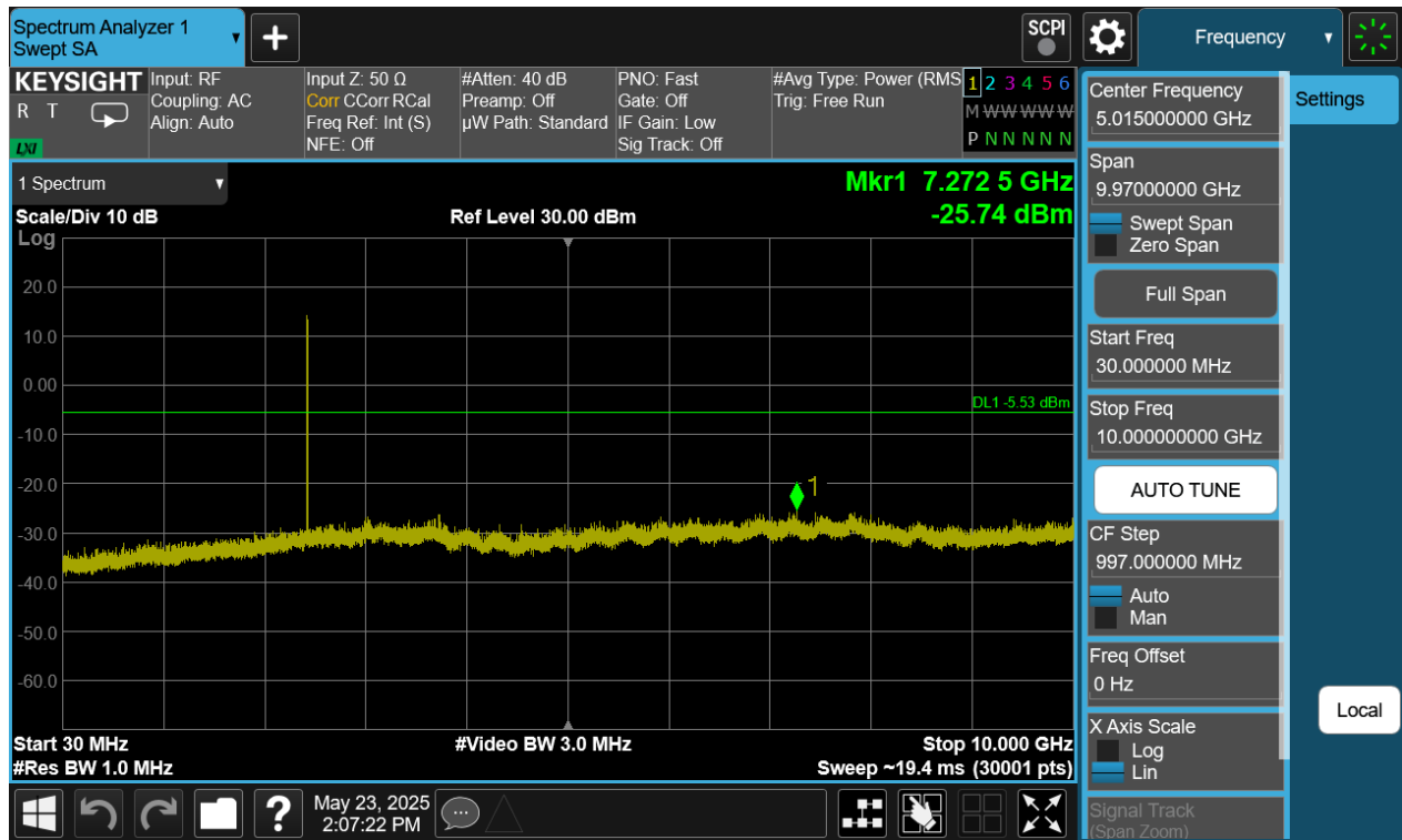
Plot 7-381. Conducted Spurious Plot Antenna WF7 (Bluetooth (HDRPS2), 8Mbps, ePA – Ch. 38)
