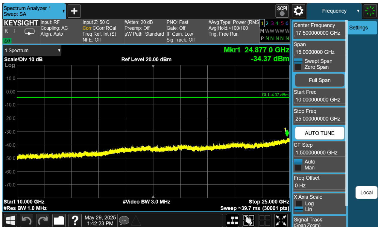
Plot 7-402. Conducted Spurious Plot Antenna WF7 (Bluetooth (HDT2), 2Mbps, ePA – Ch. 73)
