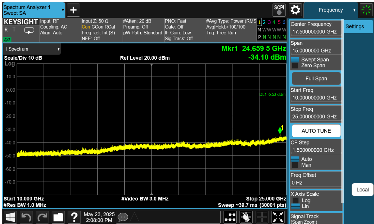
Plot 7-382. Conducted Spurious Plot Antenna WF7 (Bluetooth (HDRPS2), 8Mbps, ePA – Ch. 38)
