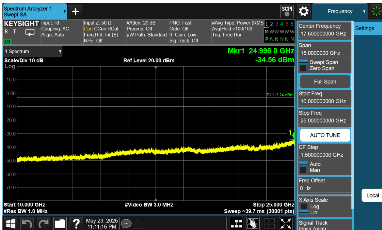
Plot 7-410. Conducted Spurious Plot Antenna WF9 (Bluetooth (HDRPS2), 8Mbps, ePA – Ch. 1)
