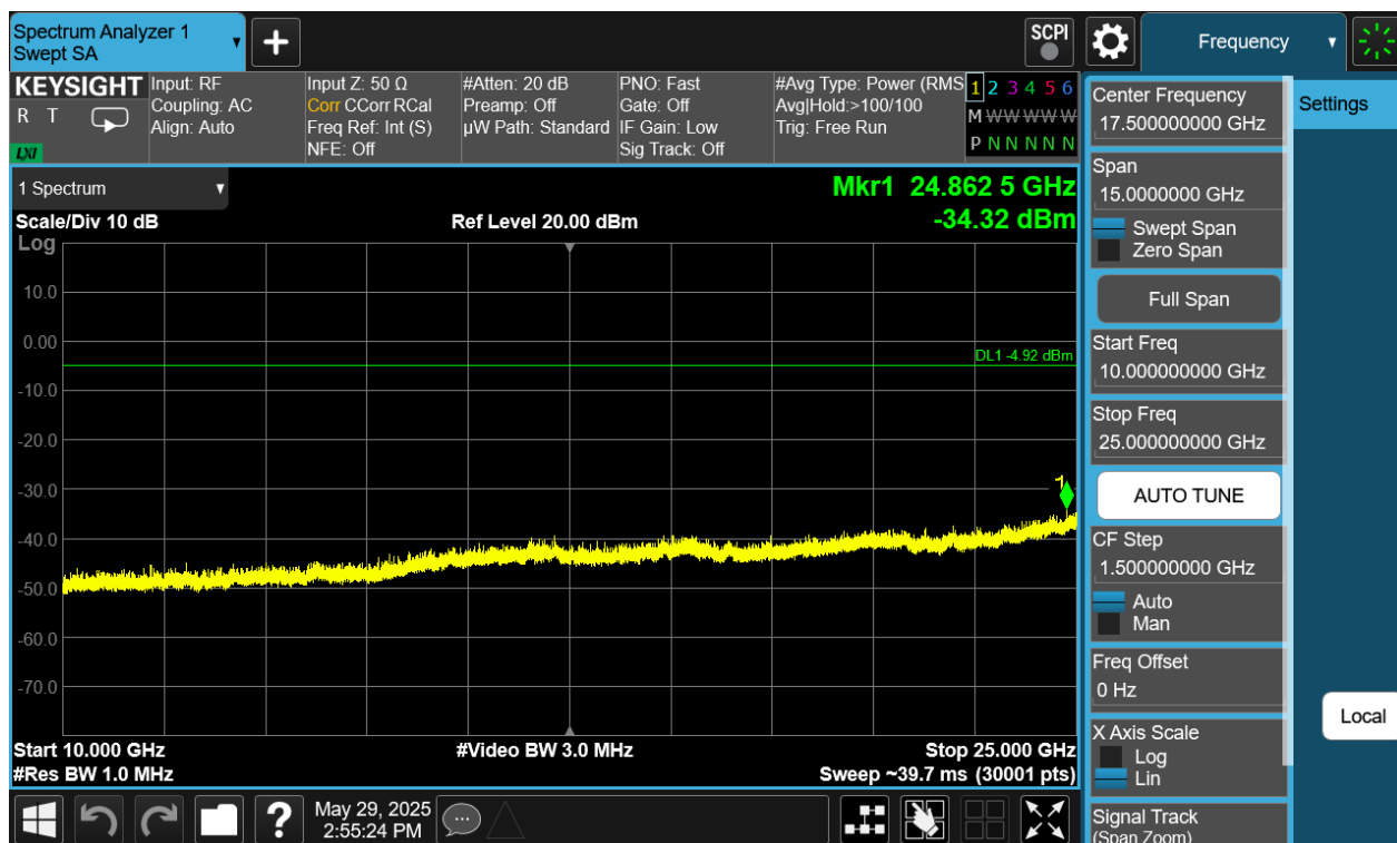
Plot 7-420. Conducted Spurious Plot Antenna WF9 (Bluetooth (XHDRPM6), 6Mbps, ePA – Ch. 73)
