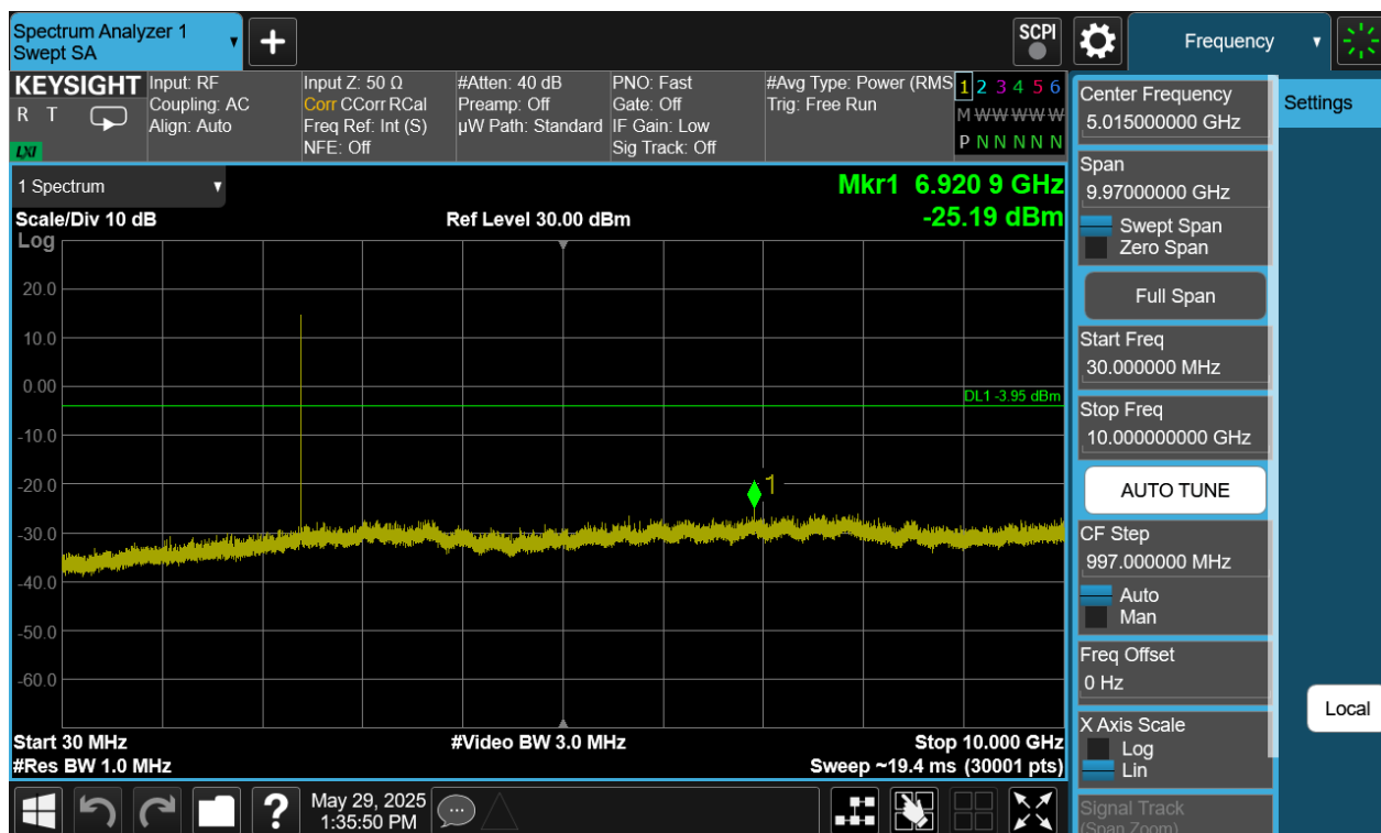
Plot 7-391. Conducted Spurious Plot Antenna WF7 (Bluetooth (HDRPM16), 16Mbps, ePA – Ch. 1)
