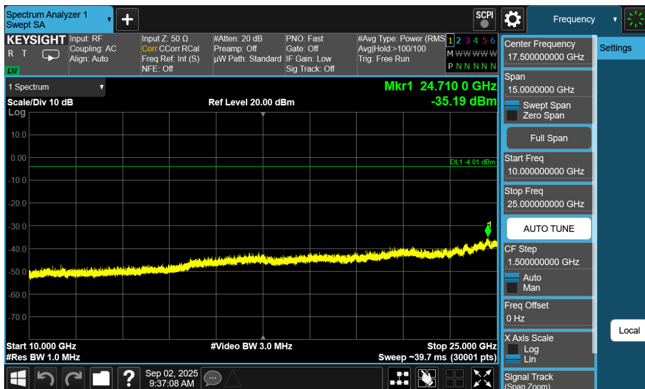
Plot 7-400. Conducted Spurious Plot Antenna WF7 (Bluetooth (HDT2), 2Mbps, ePA – Ch. 37)
