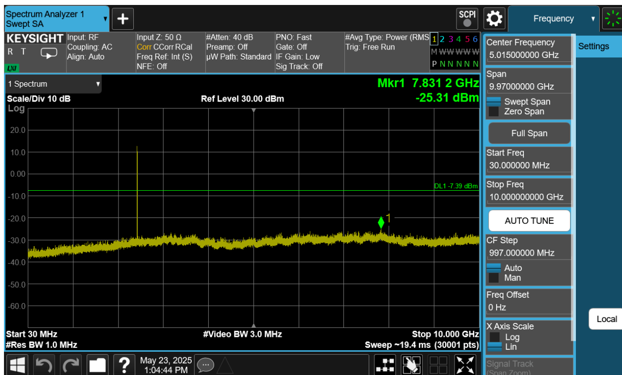
Plot 7-375. Conducted Spurious Plot Antenna WF7 (Bluetooth (HDR4), 4 Mbps, ePA – Ch. 38)
