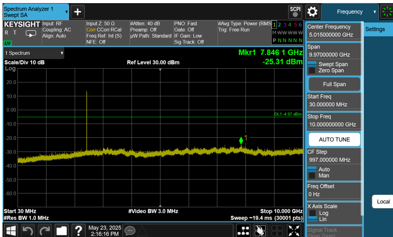
Plot 7-393. Conducted Spurious Plot Antenna WF7 (Bluetooth (HDRPM16), 16Mbps, ePA – Ch. 38)
