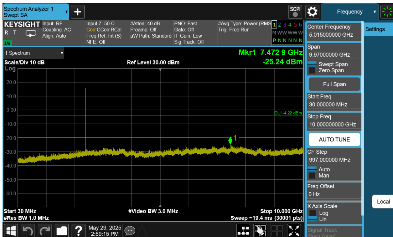
Plot 7-427. Conducted Spurious Plot Antenna WF9 (Bluetooth (HDT2), 2Mbps, ePA – Ch. 1)
