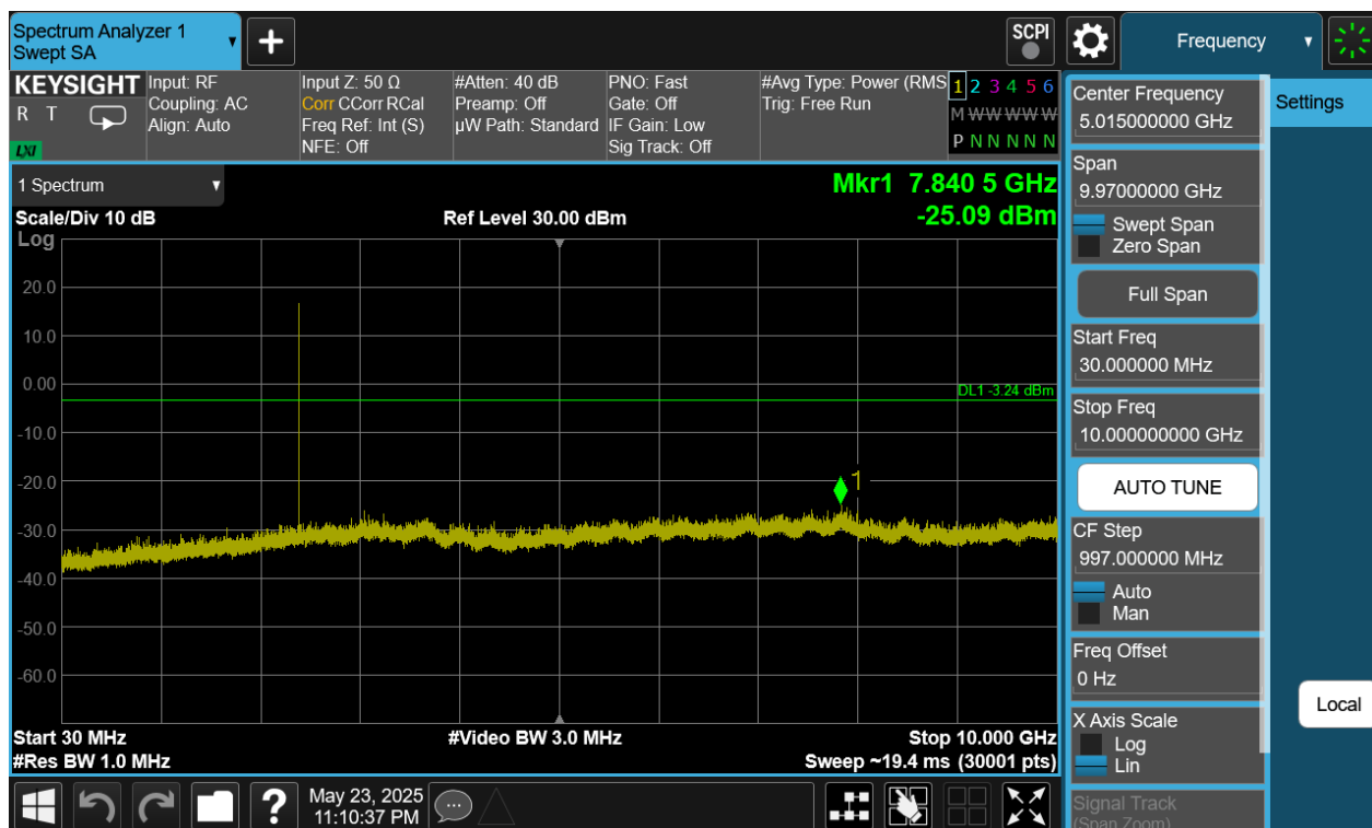
Plot 7-409. Conducted Spurious Plot Antenna WF9 (Bluetooth (HDRPS2), 8Mbps, ePA – Ch. 1)
