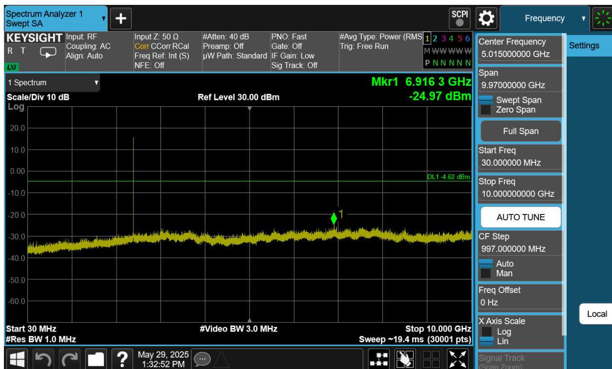
Plot 7-385. Conducted Spurious Plot Antenna WF7 (Bluetooth (XHDRPM6), 6Mbps, ePA – Ch. 1)
