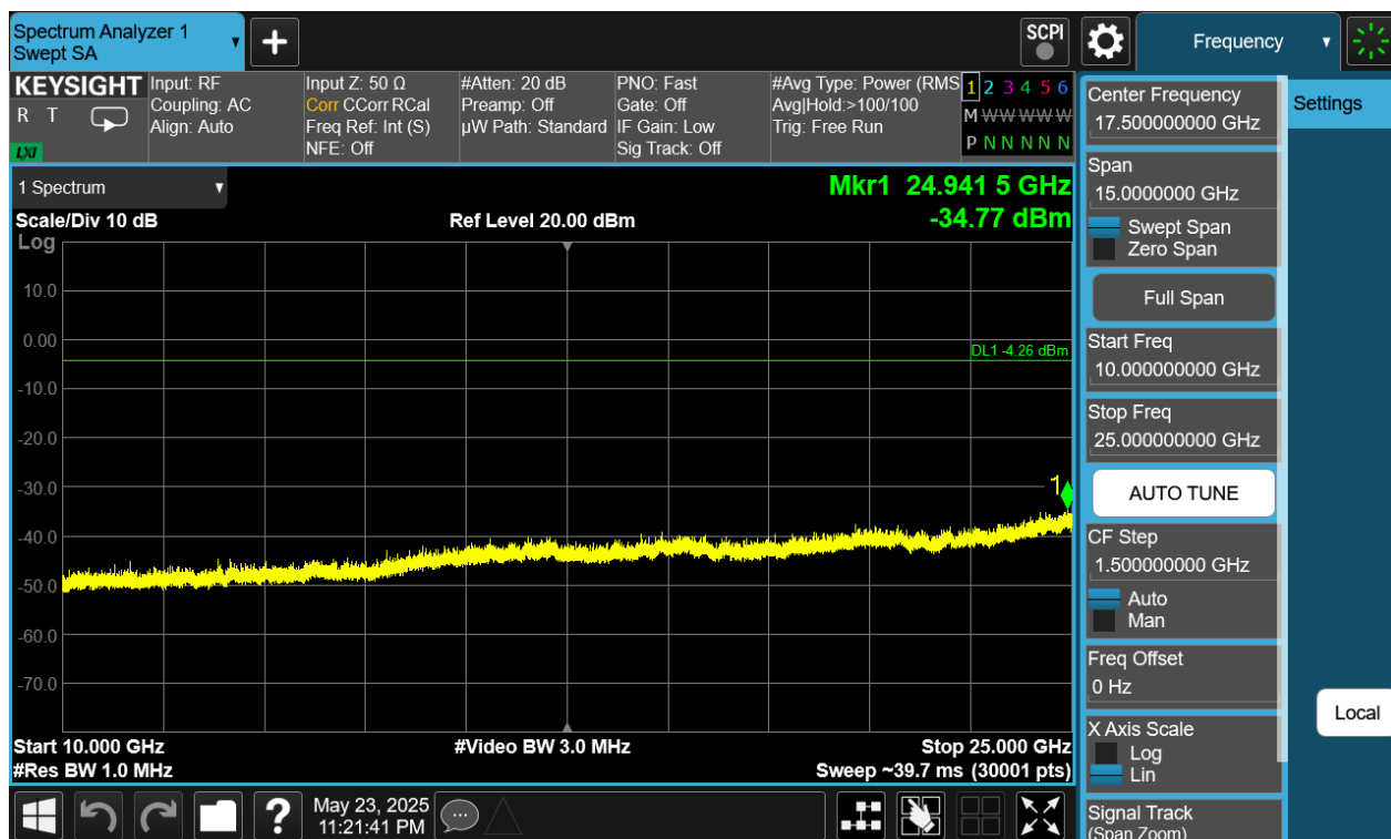
Plot 7-424. Conducted Spurious Plot Antenna WF9 (Bluetooth (HDRPM16), 16Mbps, ePA – Ch. 38)
