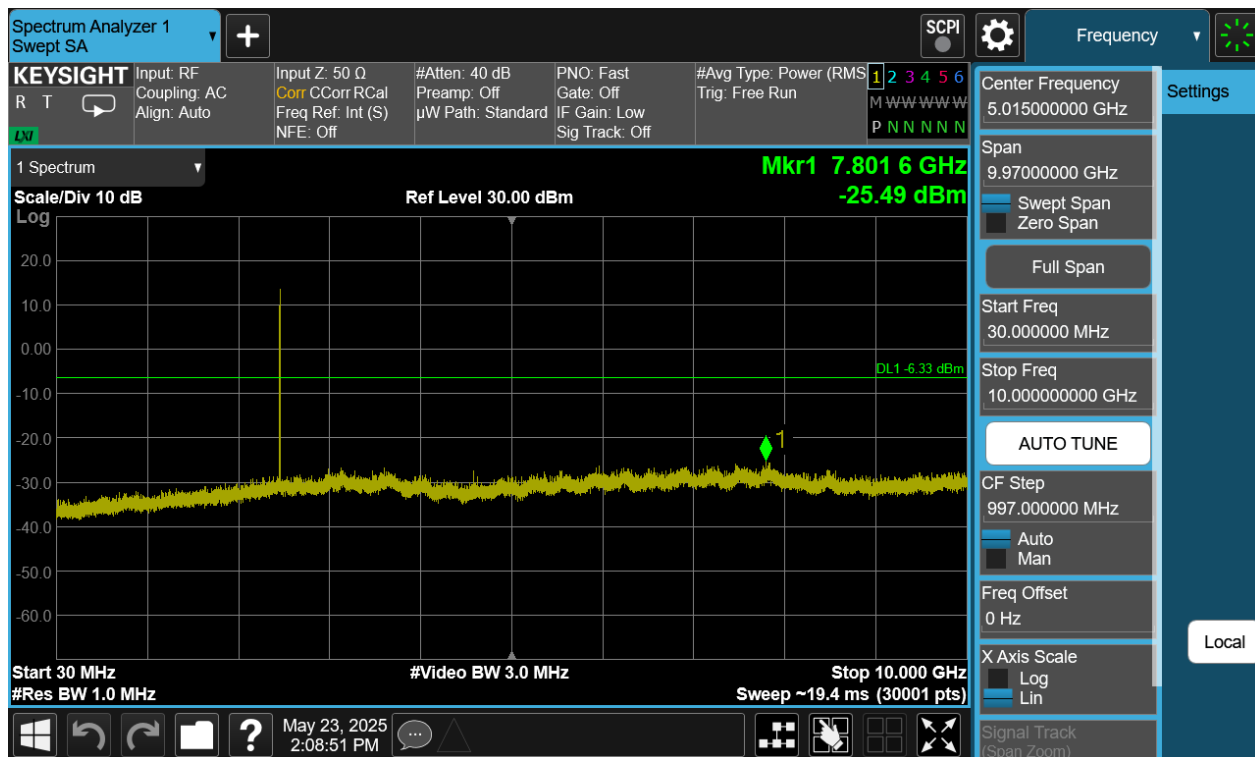
Plot 7-383. Conducted Spurious Plot Antenna WF7 (Bluetooth (HDRPS2), 8Mbps, ePA – Ch. 73)
