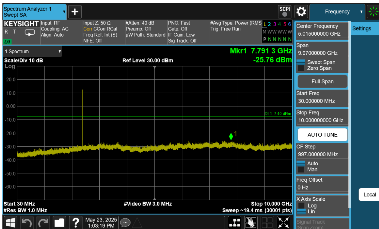
Plot 7-373. Conducted Spurious Plot Antenna WF7 (Bluetooth (HDR4), 4 Mbps, ePA – Ch. 1)
