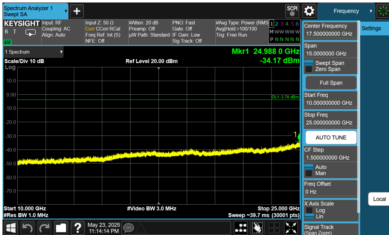
Plot 7-414. Conducted Spurious Plot Antenna WF9 (Bluetooth (HDRPS2), 8Mbps, ePA – Ch. 73)
