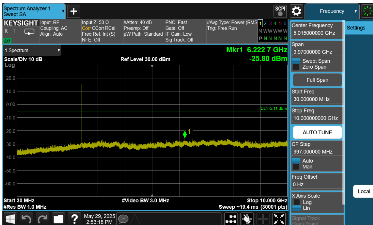
Plot 7-415. Conducted Spurious Plot Antenna WF9 (Bluetooth (XHDRPM6), 6Mbps, ePA – Ch. 1)
