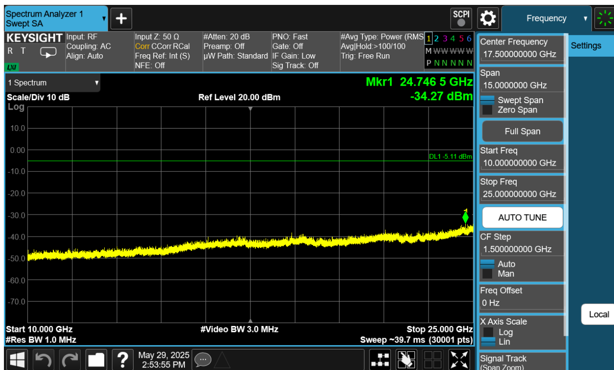
Plot 7-416. Conducted Spurious Plot Antenna WF9 (Bluetooth (XHDRPM6), 6Mbps, ePA – Ch. 1)
