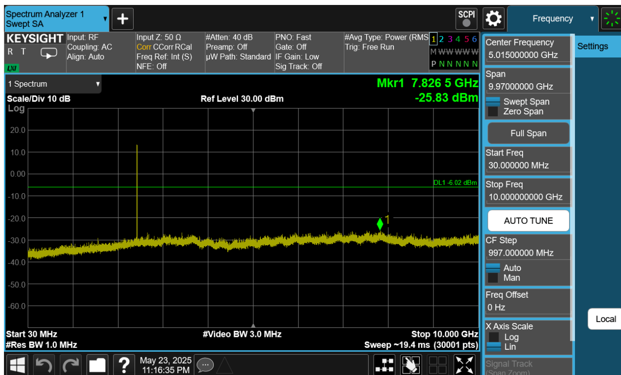
Plot 7-417. Conducted Spurious Plot Antenna WF9 (Bluetooth (XHDRPM6), 6Mbps, ePA – Ch. 38)
