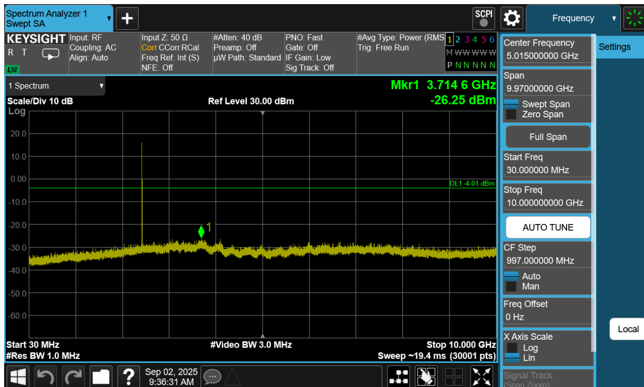
Plot 7-399. Conducted Spurious Plot Antenna WF7 (Bluetooth (HDT2), 2Mbps, ePA – Ch. 37)
