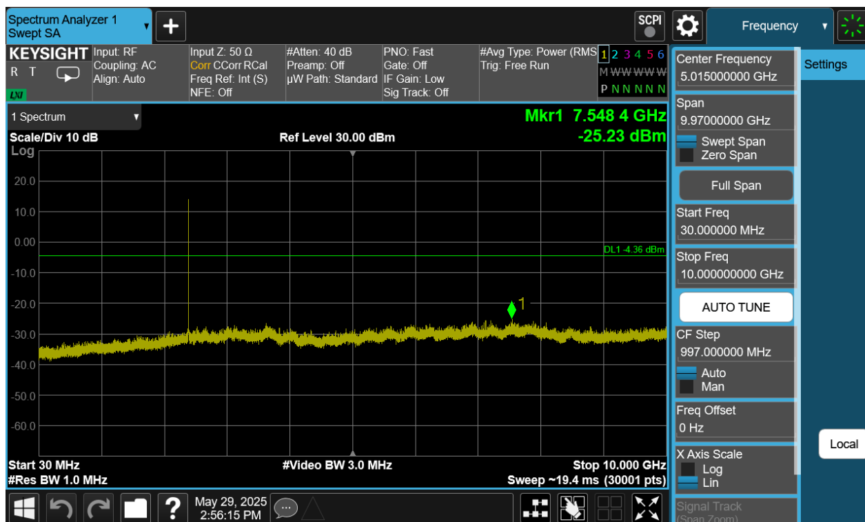
Plot 7-421. Conducted Spurious Plot Antenna WF9 (Bluetooth (HDRPM16), 16Mbps, ePA – Ch. 1)
