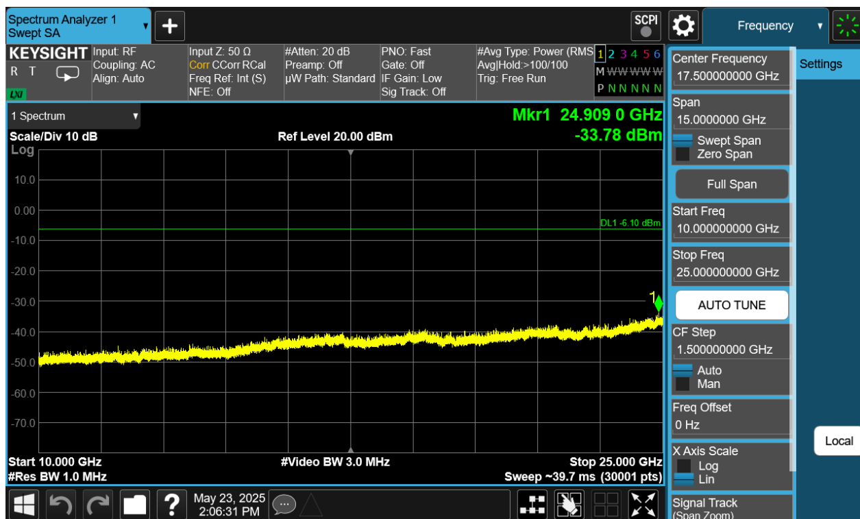
Plot 7-380. Conducted Spurious Plot Antenna WF7 (Bluetooth (HDRPS2), 8Mbps, ePA – Ch. 1)
