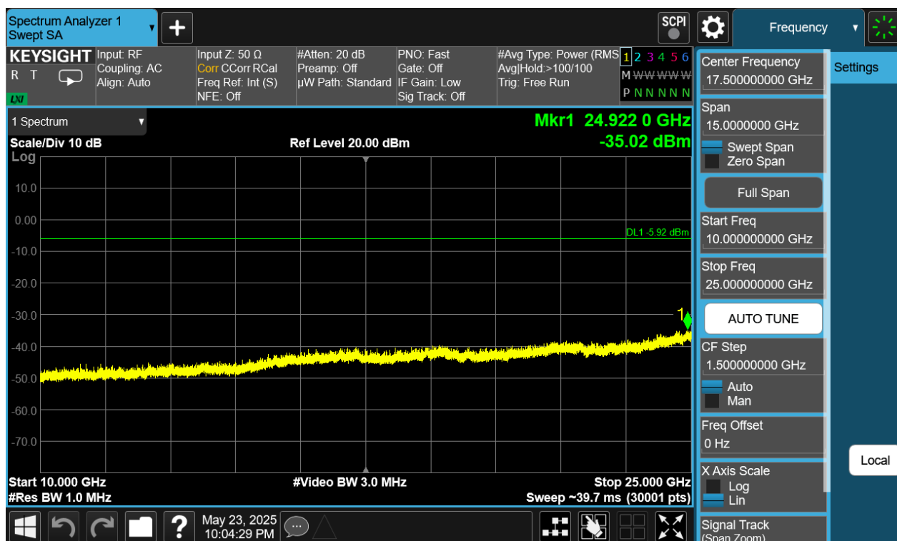
Plot 7-404. Conducted Spurious Plot Antenna WF9 (Bluetooth (HDR4), 4 Mbps, ePA – Ch. 1)
