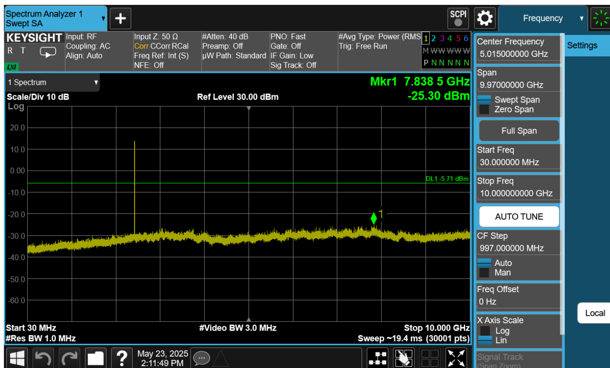
Plot 7-387. Conducted Spurious Plot Antenna WF7 (Bluetooth (XHDRPM6), 6Mbps, ePA – Ch. 38)
