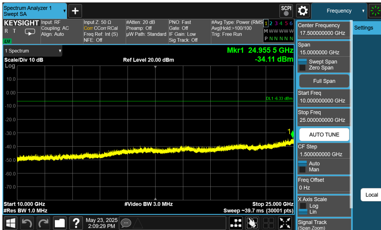
Plot 7-384. Conducted Spurious Plot Antenna WF7 (Bluetooth (HDRPS2), 8Mbps, ePA – Ch. 73)
