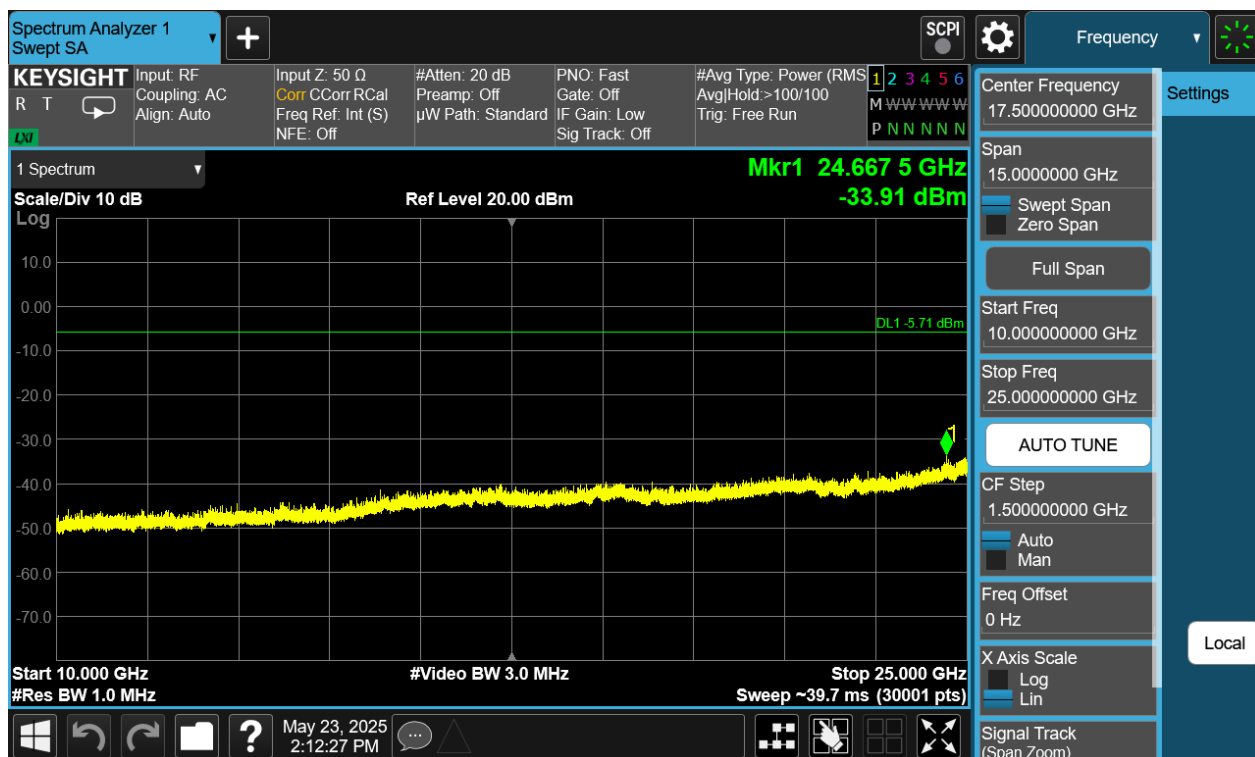
Plot 7-388. Conducted Spurious Plot Antenna WF7 (Bluetooth (XHDRPM6), 6Mbps, ePA – Ch. 38)
