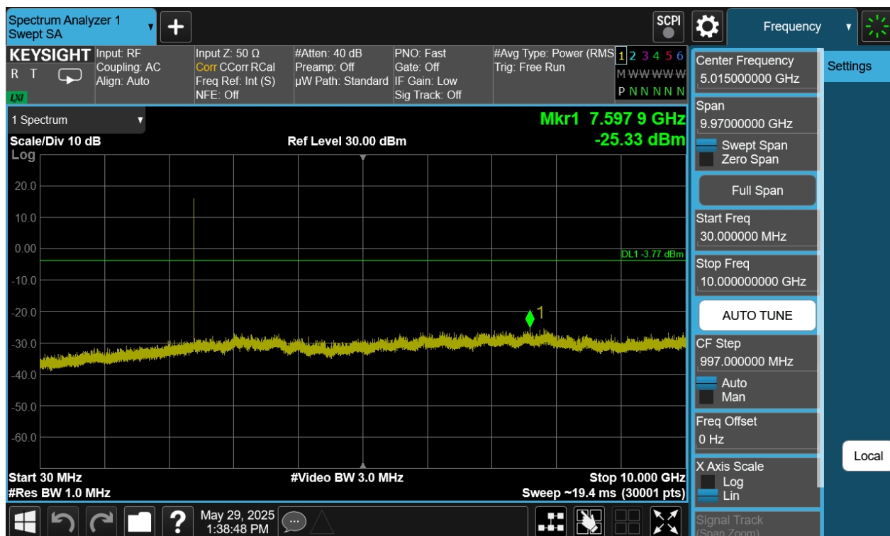
Plot 7-397. Conducted Spurious Plot Antenna WF7 (Bluetooth (HDT2), 2Mbps, ePA – Ch. 1)
