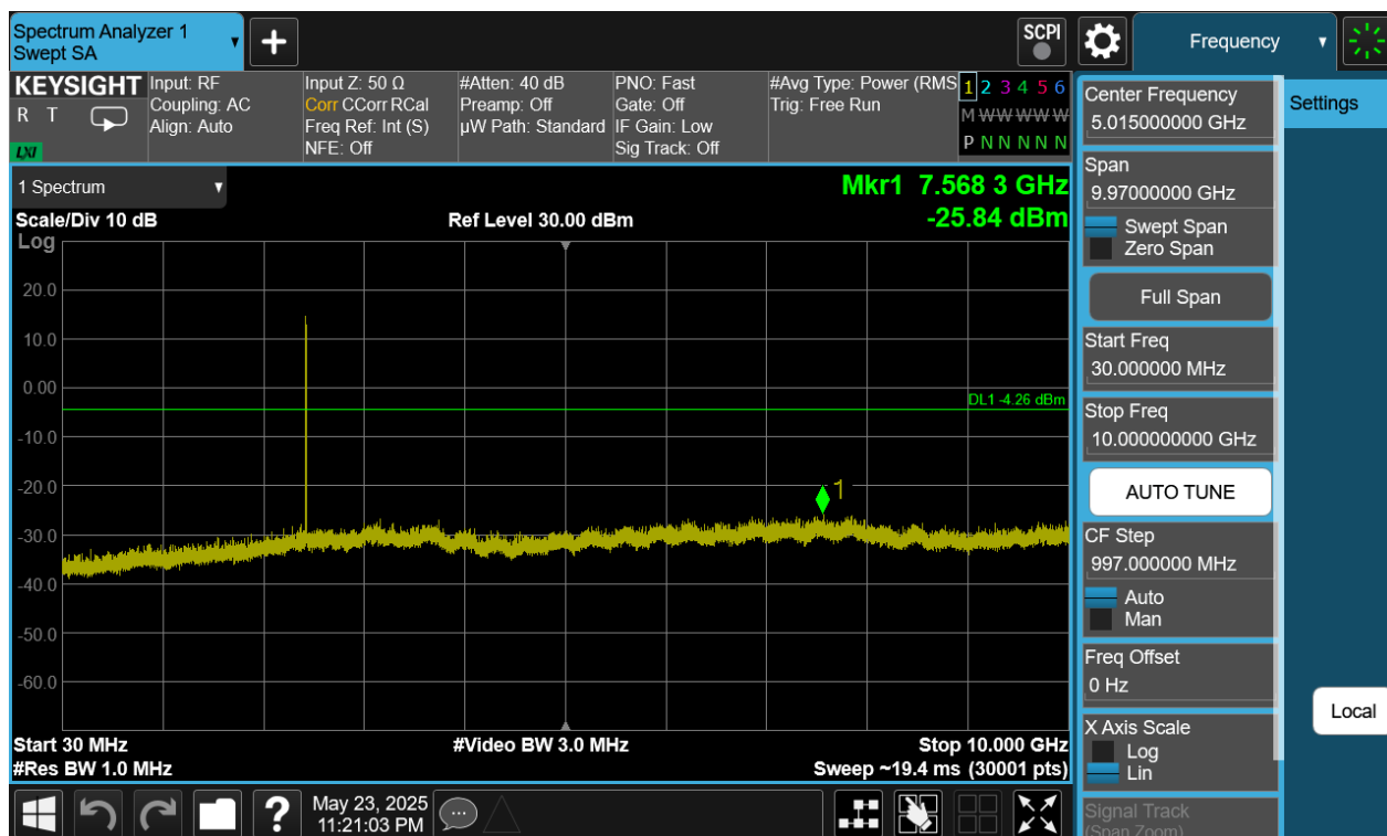
Plot 7-423. Conducted Spurious Plot Antenna WF9 (Bluetooth (HDRPM16), 16Mbps, ePA – Ch. 38)
