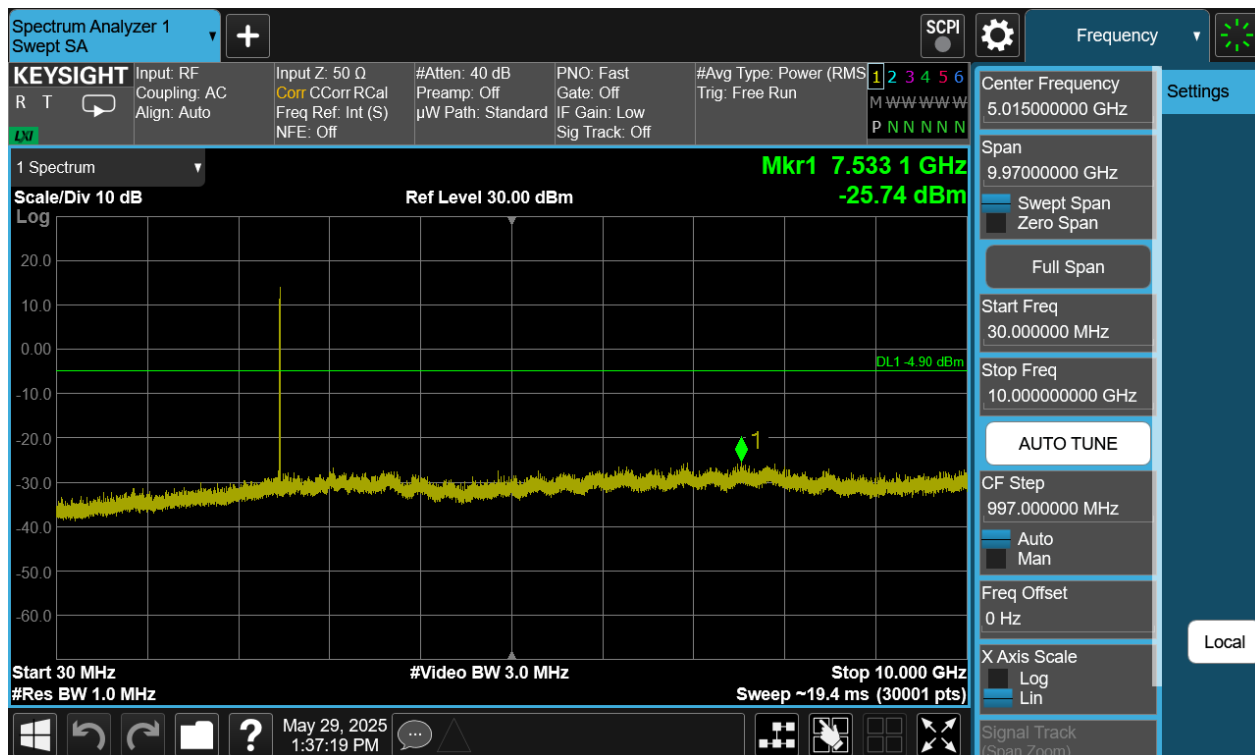
Plot 7-395. Conducted Spurious Plot Antenna WF7 (Bluetooth (HDRPM16), 16Mbps, ePA – Ch. 73)
