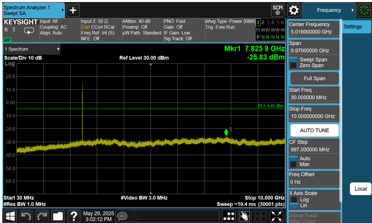
Plot 7-431. Conducted Spurious Plot Antenna WF9 (Bluetooth (HDT2), 2Mbps, ePA – Ch. 73)
