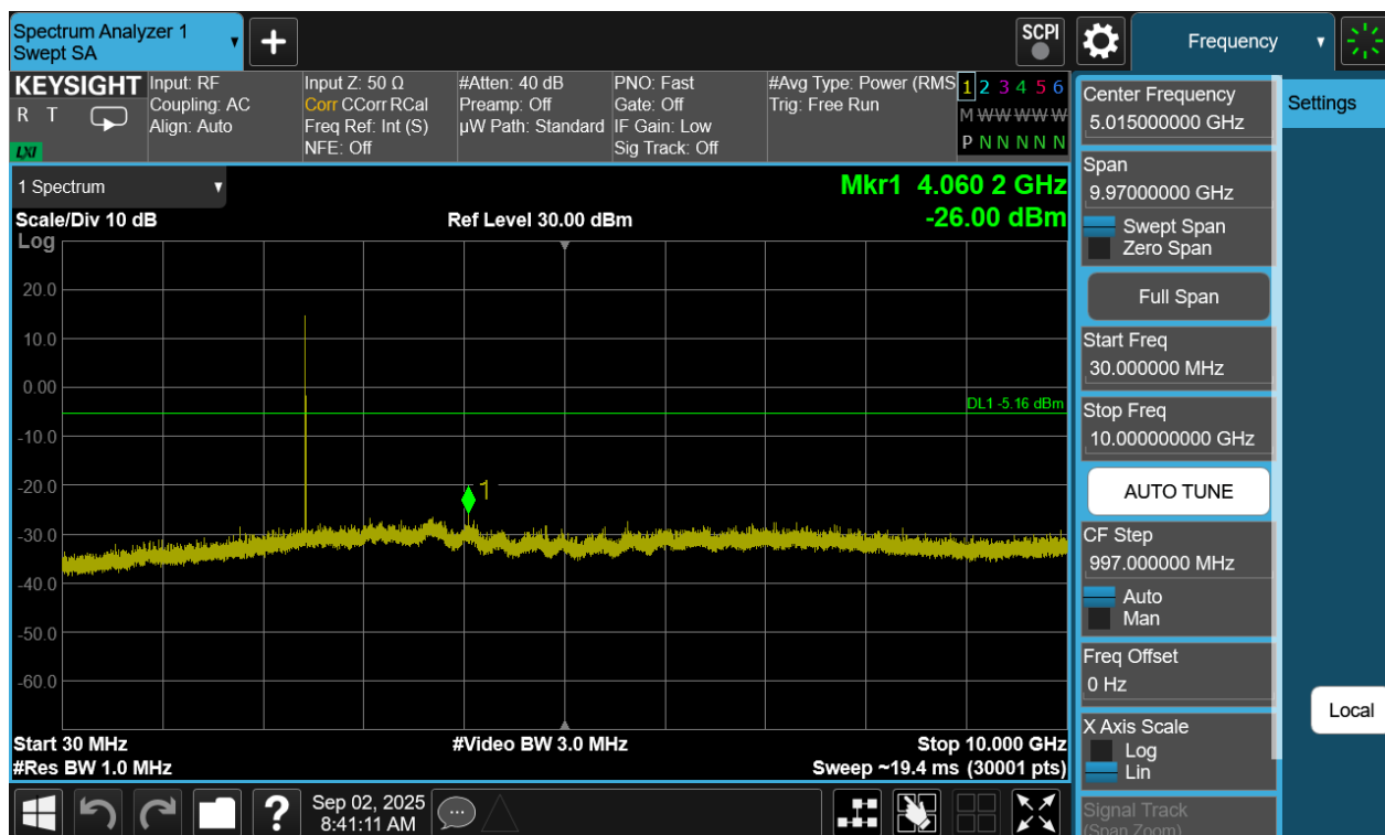
Plot 7-369. Conducted Spurious Plot Antenna WF8 (Bluetooth (HDT2), 2Mbps, ePA – Ch. 37)
