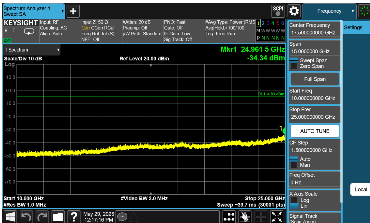
Plot 7-372. Conducted Spurious Plot Antenna WF8 (Bluetooth (HDT2), 2Mbps, ePA – Ch. 73)
