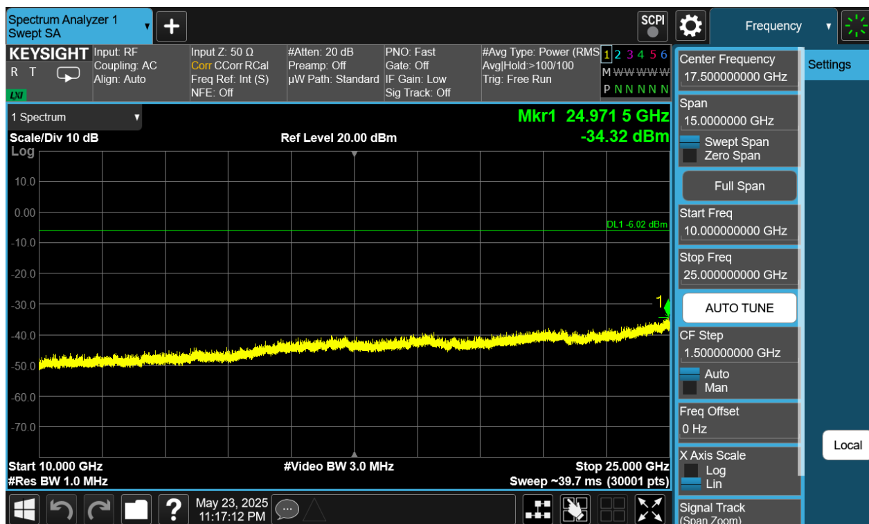
Plot 7-418. Conducted Spurious Plot Antenna WF9 (Bluetooth (XHDRPM6), 6Mbps, ePA – Ch. 38)
