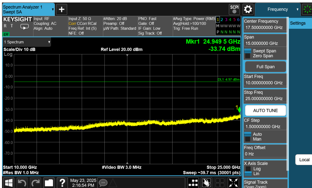
Plot 7-394. Conducted Spurious Plot Antenna WF7 (Bluetooth (HDRPM16), 16Mbps, ePA – Ch. 38)
