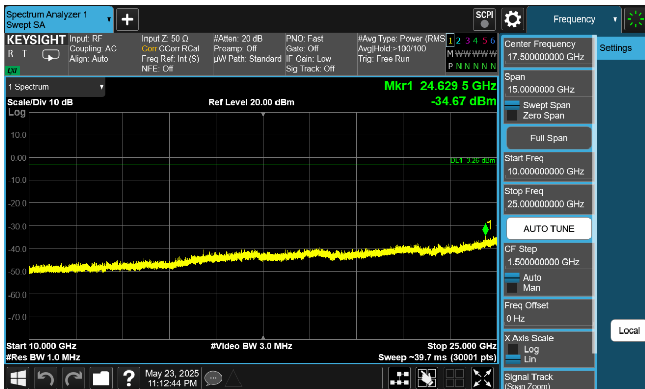
Plot 7-412. Conducted Spurious Plot Antenna WF9 (Bluetooth (HDRPS2), 8Mbps, ePA – Ch. 38)
