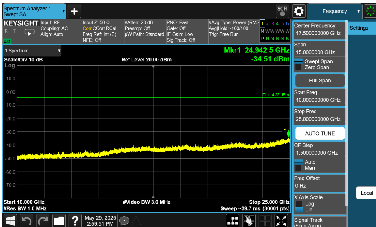
Plot 7-428. Conducted Spurious Plot Antenna WF9 (Bluetooth (HDT2), 2Mbps, ePA – Ch. 1)
