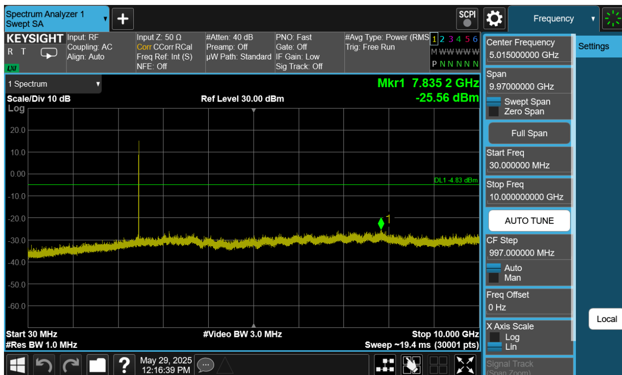
Plot 7-371. Conducted Spurious Plot Antenna WF8 (Bluetooth (HDT2), 2Mbps, ePA – Ch. 73)
