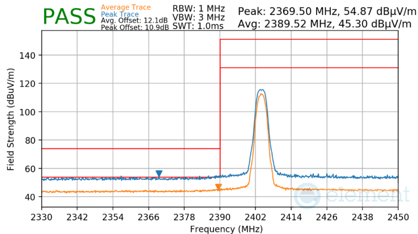
Plot 7-477. Radiated Restricted Lower Band Edge Measurement TxBF Primary
