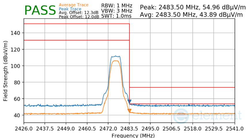
Plot 7-462. Radiated Restricted Upper Band Edge Measurement Antenna WF7
