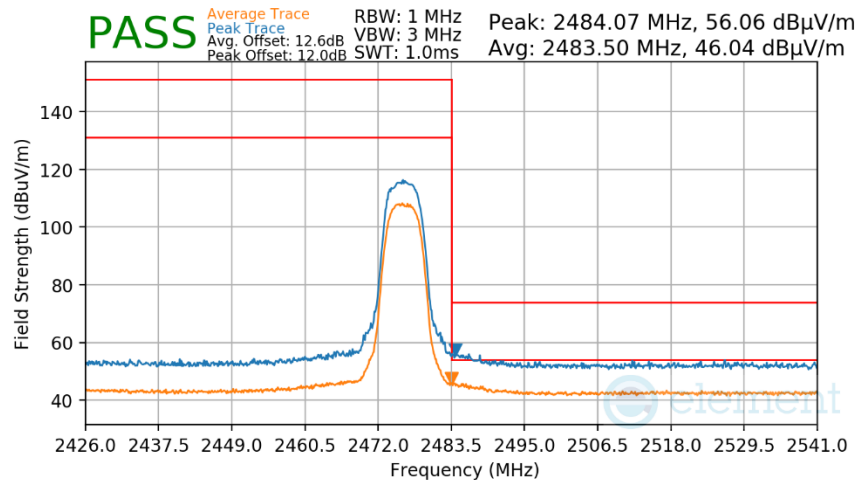
Plot 7-451. Radiated Restricted Upper Band Edge Measurement Antenna WF8
