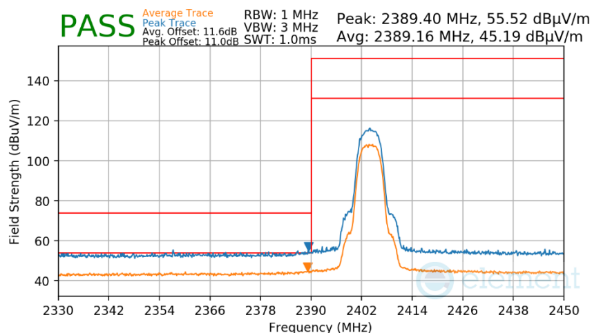
Plot 7-481. Radiated Restricted Lower Band Edge Measurement TxBF Primary
