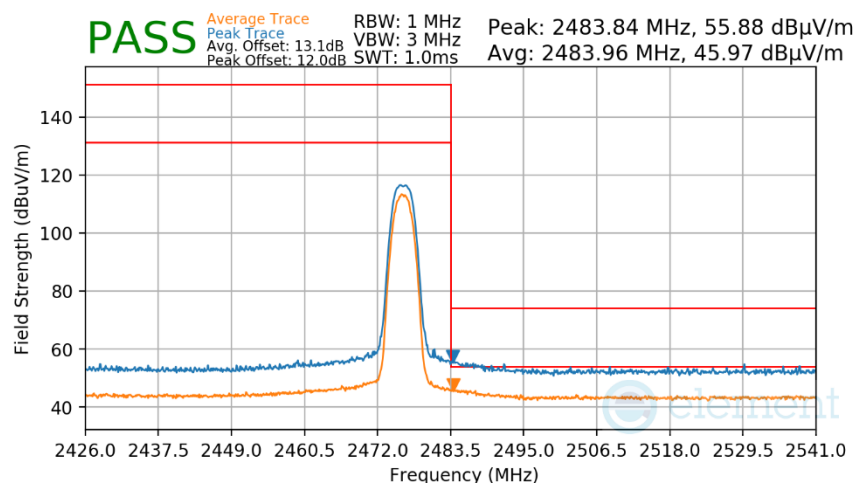
Plot 7-447. Radiated Restricted Upper Band Edge Measurement Antenna WF8
