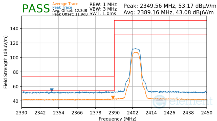
Plot 7-444. Radiated Restricted Lower Band Edge Measurement Antenna WF8
