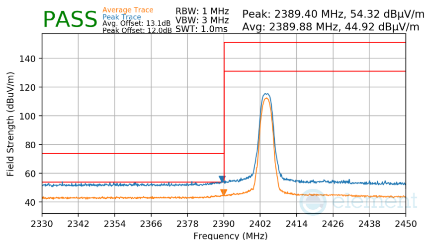
Plot 7-441. Radiated Restricted Lower Band Edge Measurement Antenna WF8
