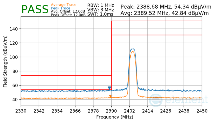
Plot 7-467. Radiated Restricted Lower Band Edge Measurement Antenna WF9
