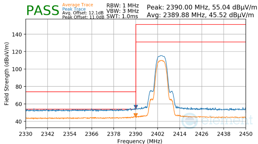
Plot 7-478. Radiated Restricted Lower Band Edge Measurement TxBF Primary
