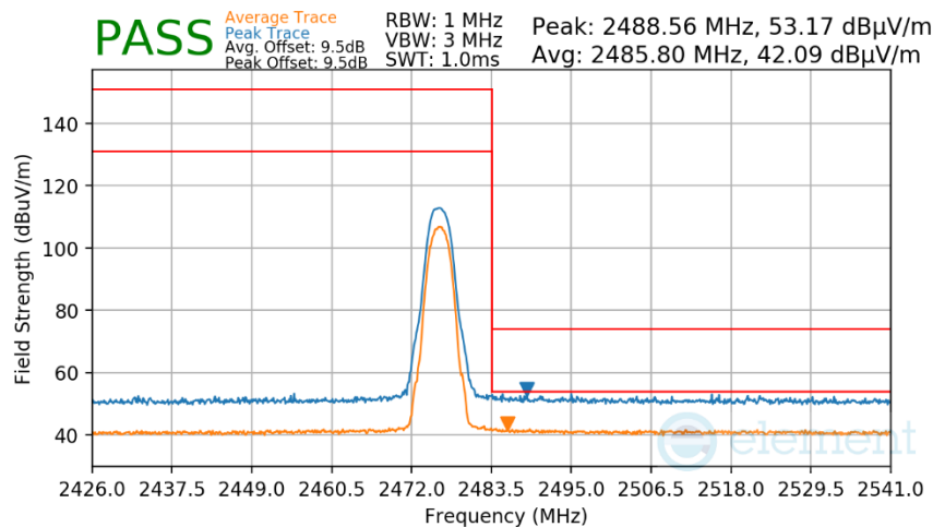
Plot 7-476. Radiated Restricted Upper Band Edge Measurement Antenna WF9
