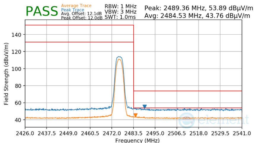
Plot 7-449. Radiated Restricted Upper Band Edge Measurement Antenna WF8
