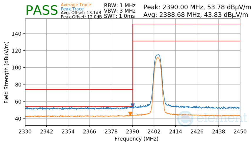
Plot 7-453. Radiated Restricted Lower Band Edge Measurement Antenna WF7
