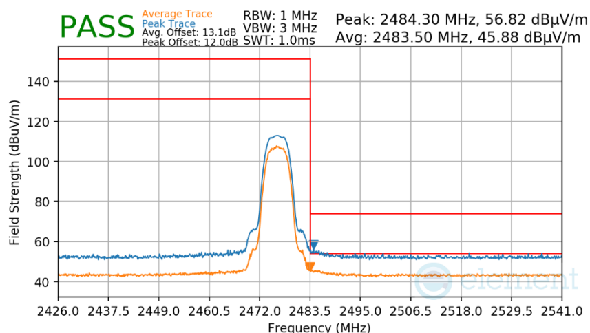
Plot 7-472. Radiated Restricted Upper Band Edge Measurement Antenna WF9
