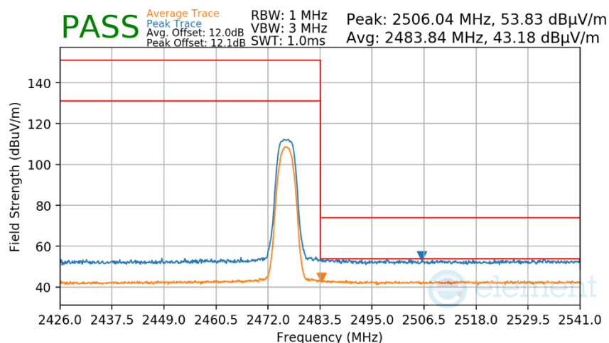
Plot 7-473. Radiated Restricted Upper Band Edge Measurement Antenna WF9
