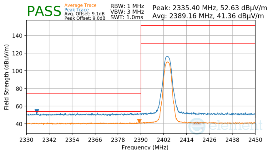
Plot 7-482. Radiated Restricted Lower Band Edge Measurement TxBF Primary
