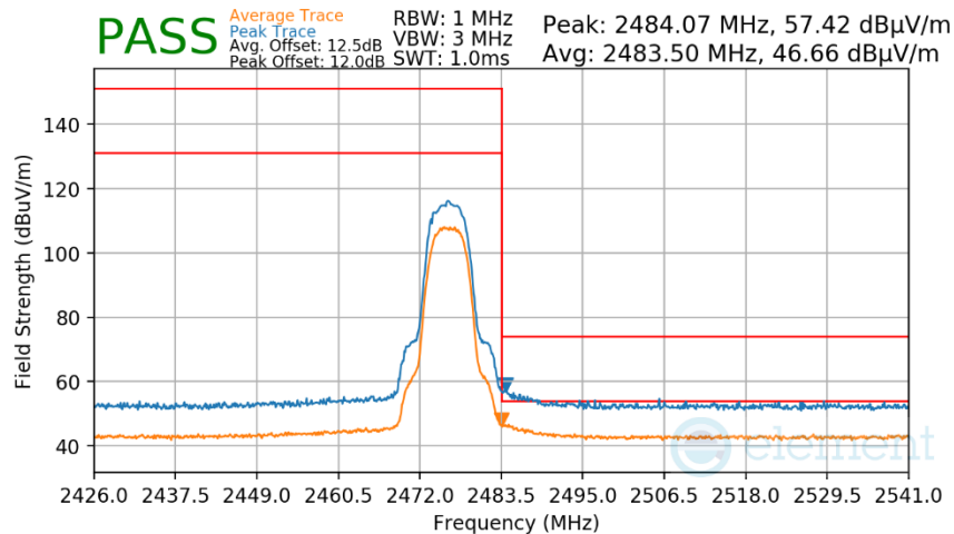
Plot 7-463. Radiated Restricted Upper Band Edge Measurement Antenna WF7
