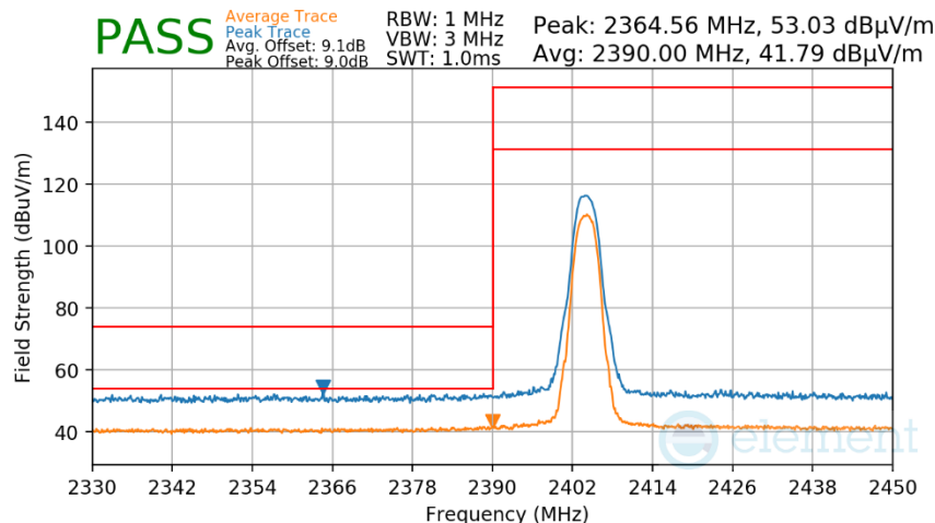
Plot 7-446. Radiated Restricted Lower Band Edge Measurement Antenna WF8
