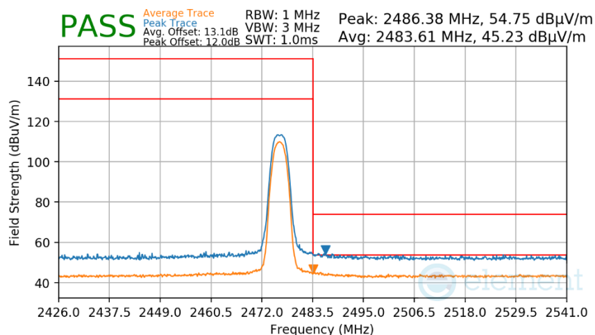
Plot 7-471. Radiated Restricted Upper Band Edge Measurement Antenna WF9
