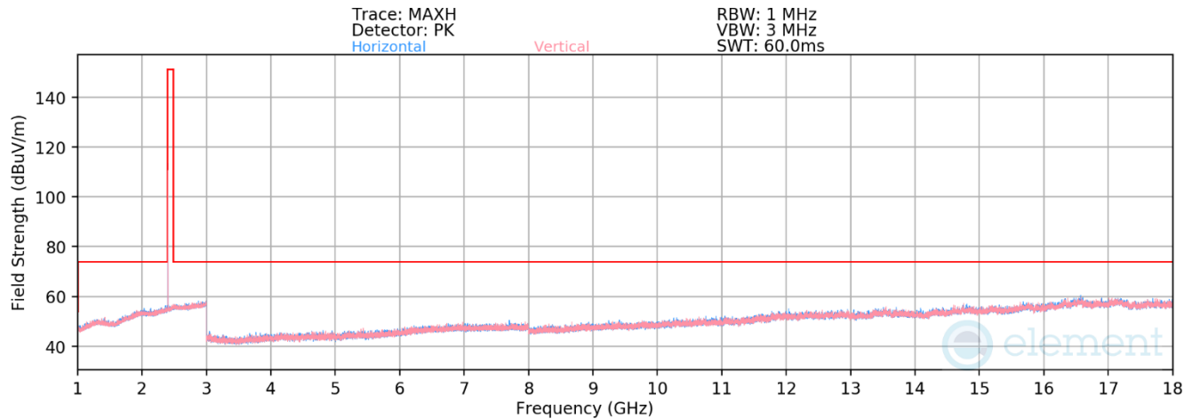
Plot 7-433. Radiated Spurious Emissions 1-18GHz TxBF Primary (4Mbps, HDR4, ePA – Ch. 1)
