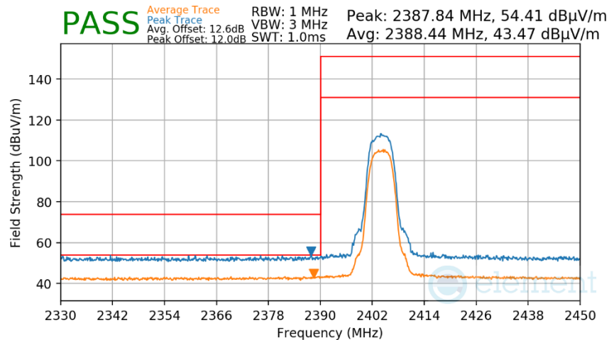
Plot 7-469. Radiated Restricted Lower Band Edge Measurement Antenna WF9
