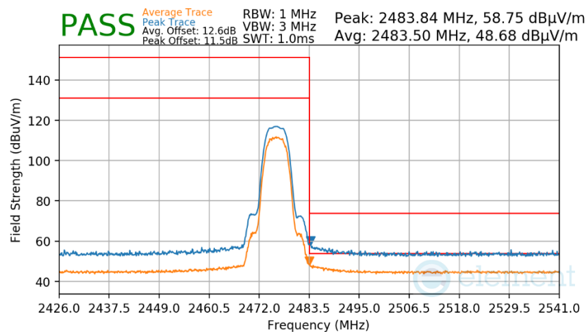
Plot 7-484. Radiated Restricted Upper Band Edge Measurement TxBF Primary
