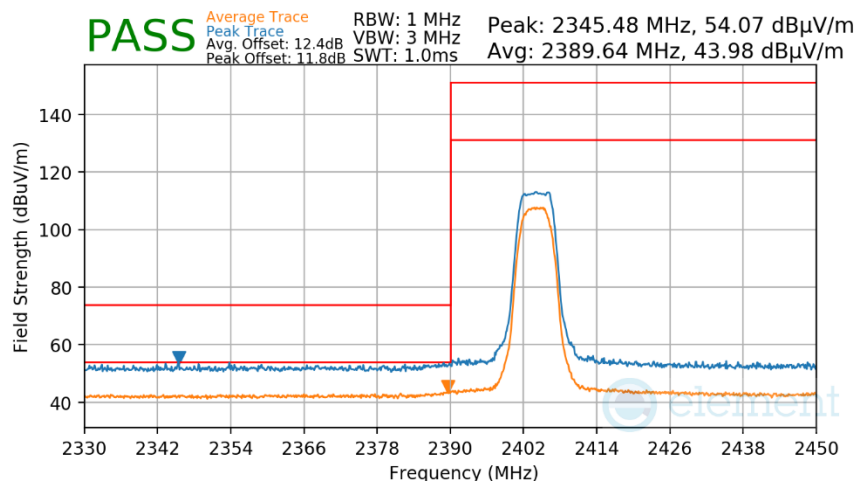
Plot 7-456. Radiated Restricted Lower Band Edge Measurement Antenna WF7
