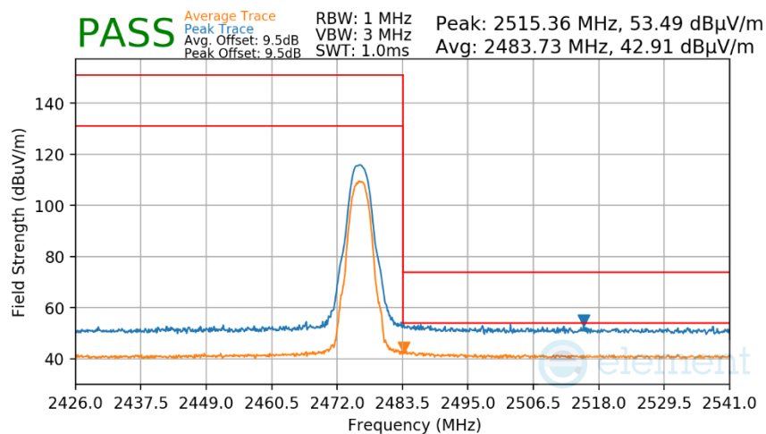
Plot 7-464. Radiated Restricted Upper Band Edge Measurement Antenna WF7
