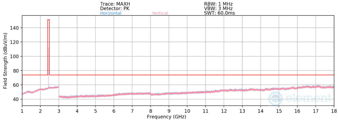
Plot 7-438. Radiated Spurious Emissions 1-18GHz TxBF Diversity (4Mbps, HDR4, ePA – Ch. 38)
