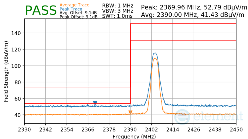
Plot 7-458. Radiated Restricted Lower Band Edge Measurement Antenna WF7
