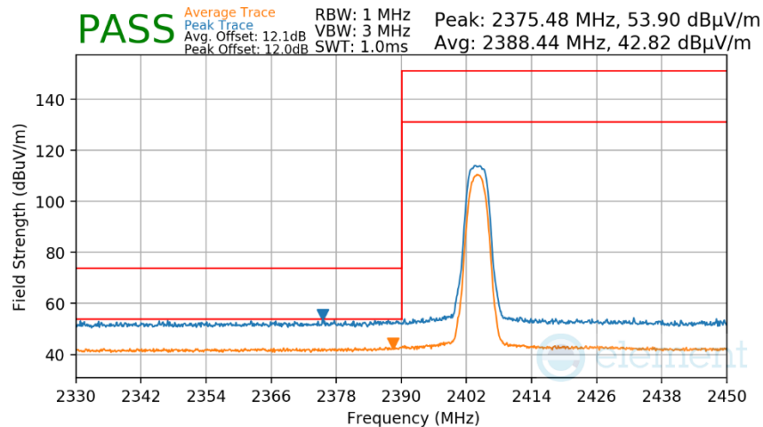
Plot 7-443. Radiated Restricted Lower Band Edge Measurement Antenna WF8
