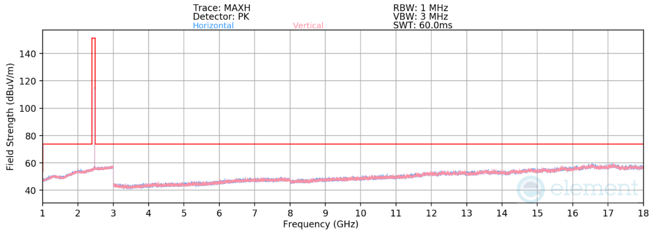
Plot 7-436. Radiated Spurious Emissions 1-18GHz TxBF Primary (4Mbps, HDR4, ePA – Ch. 73)
