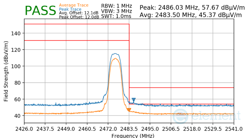
Plot 7-448. Radiated Restricted Upper Band Edge Measurement Antenna WF8
