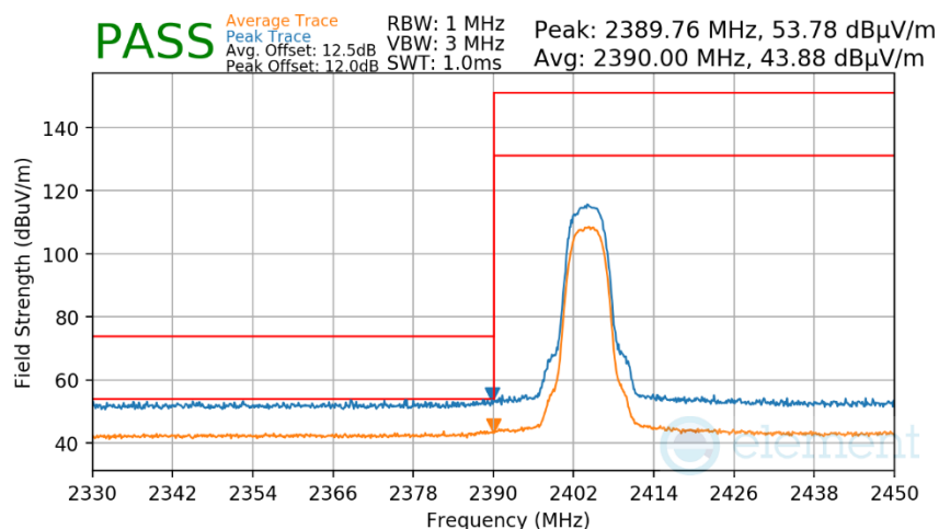
Plot 7-457. Radiated Restricted Lower Band Edge Measurement Antenna WF7
