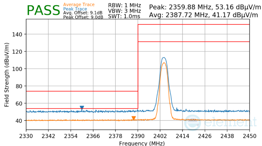
Plot 7-470. Radiated Restricted Lower Band Edge Measurement Antenna WF9
