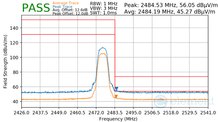
Plot 7-475. Radiated Restricted Upper Band Edge Measurement Antenna WF9
