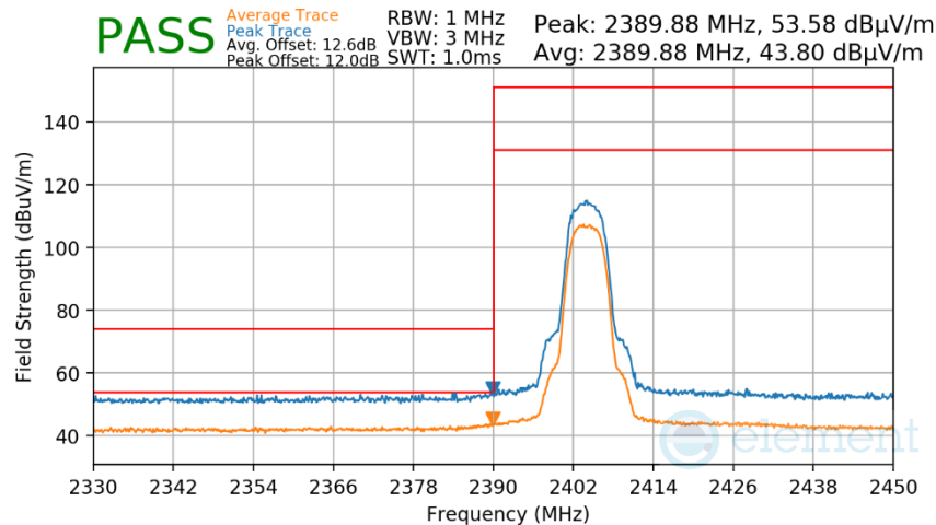
Plot 7-445. Radiated Restricted Lower Band Edge Measurement Antenna WF8
