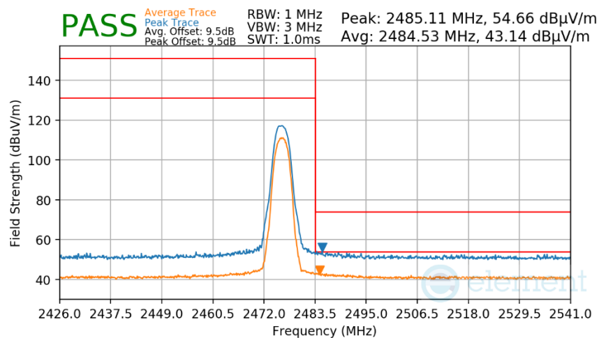
Plot 7-452. Radiated Restricted Upper Band Edge Measurement Antenna WF8
