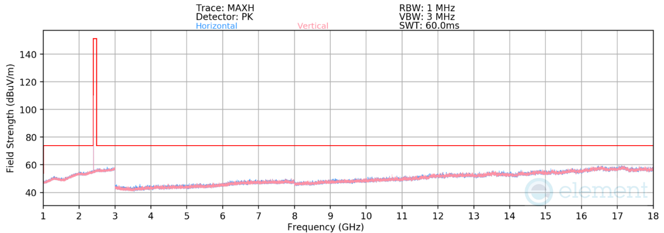
Plot 7-437. Radiated Spurious Emissions 1-18GHz TxBF Diversity (4Mbps, HDR4, ePA – Ch. 1)
