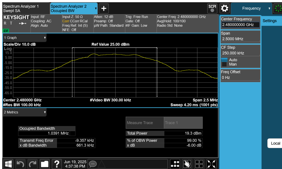
Plot 7-30. 6dB BW & 99% OBW Plot Antenna WF9 (Bluetooth (LE), 500kbps, ePA – Ch. 39)
