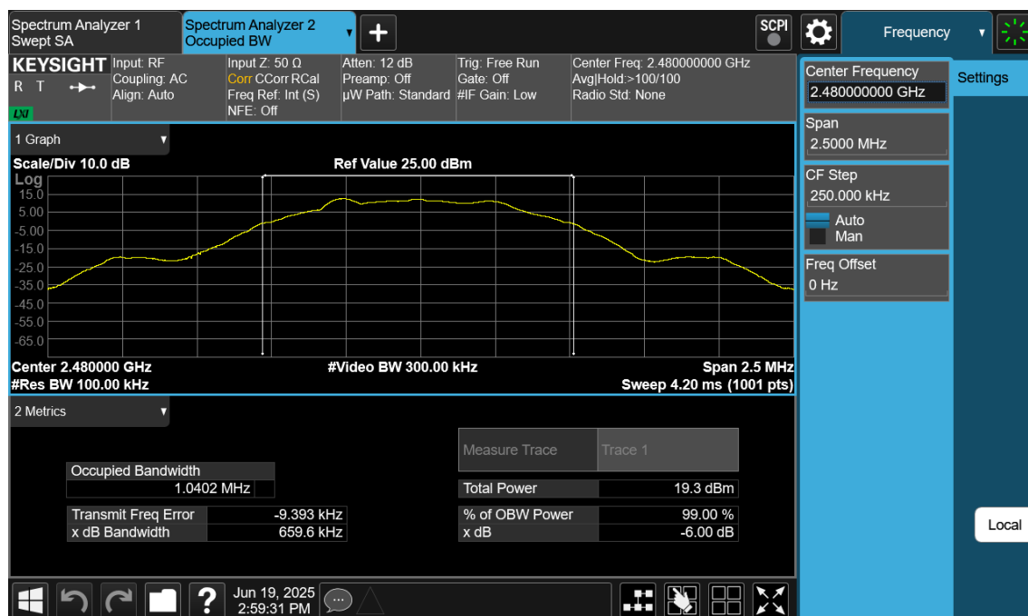
Plot 7-18. 6dB BW & 99% OBW Plot Antenna WF7 (Bluetooth (LE), 500kbps, ePA – Ch. 39)
