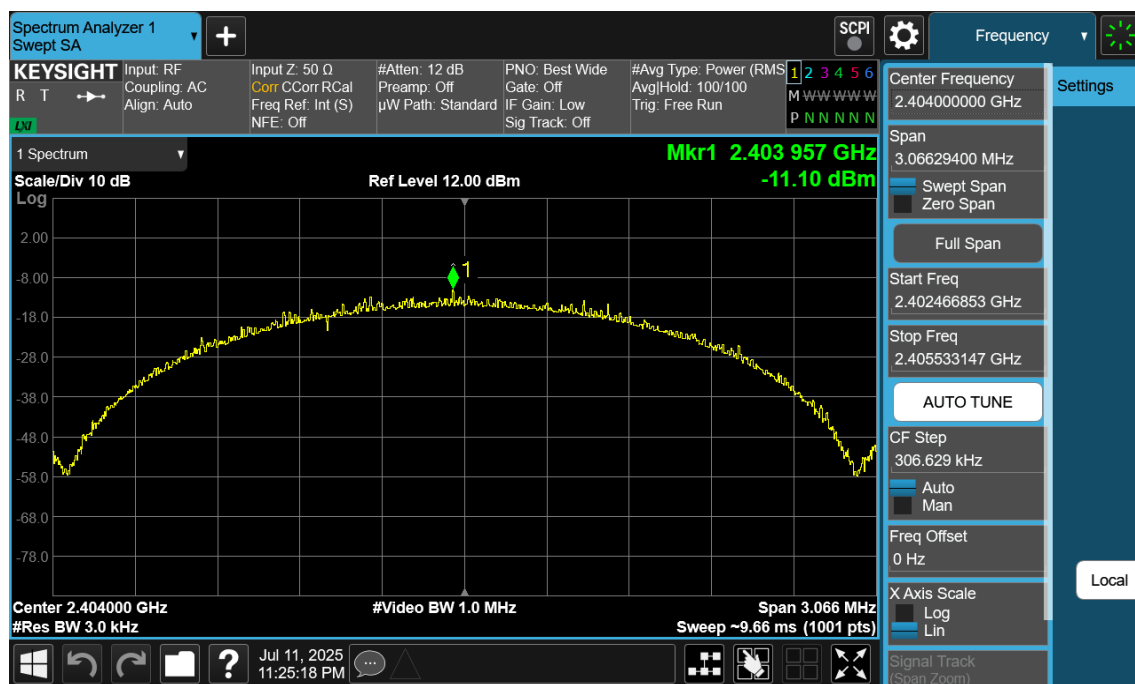
Plot 7-58. Power Spectral Density Plot Antenna WF8 (Bluetooth (LE), 2Mbps, iPA – Ch. 1)
