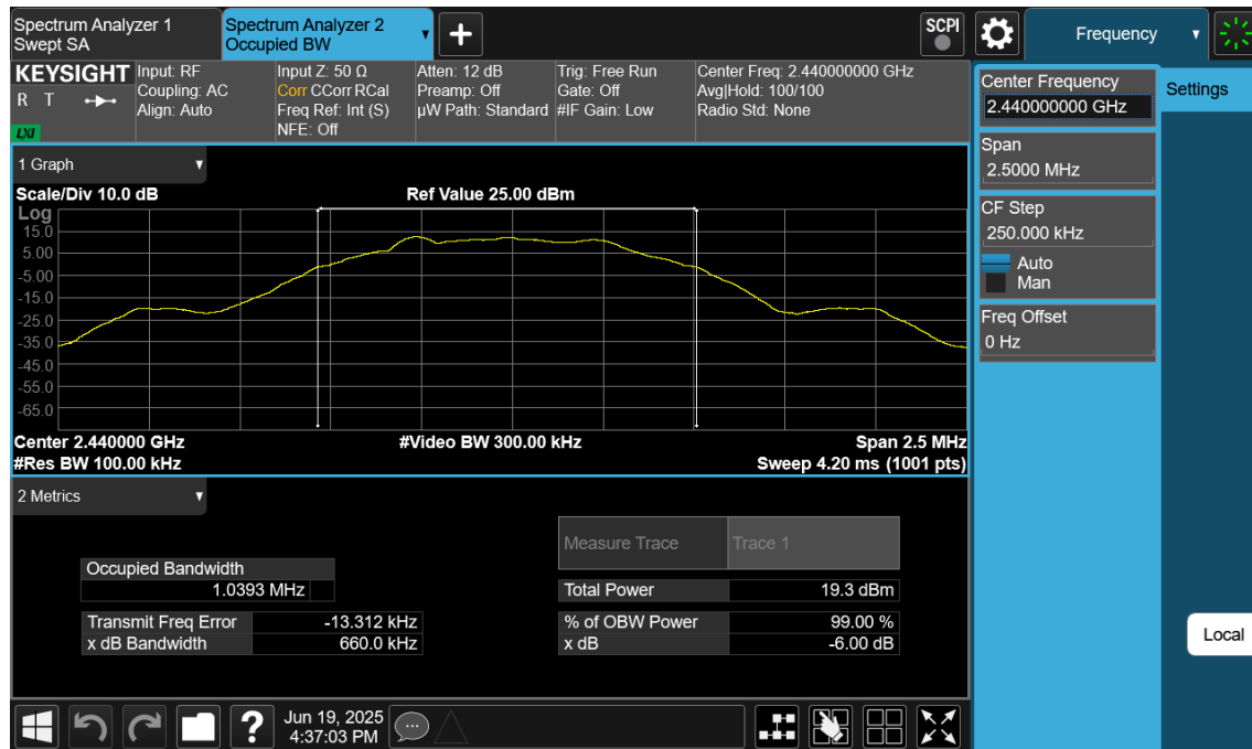
Plot 7-29.6dB BW & 99% OBW Plot Antenna WF9 (Bluetooth (LE), 500kbps, ePA – Ch. 19)
