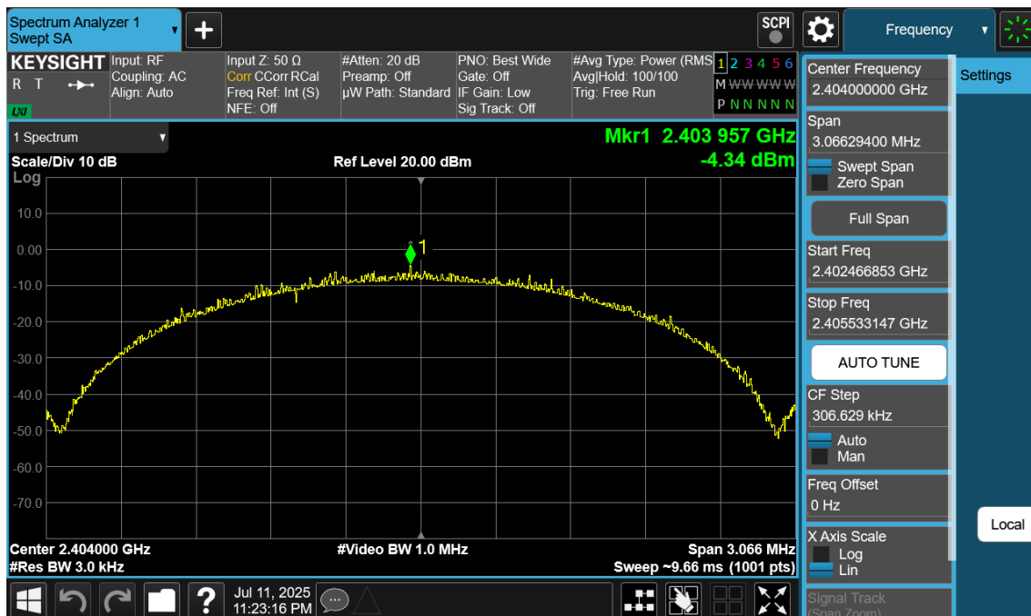
Plot 7-55. Power Spectral Density Plot Antenna WF8 (Bluetooth (LE), 2Mbps, ePA – Ch. 1)
