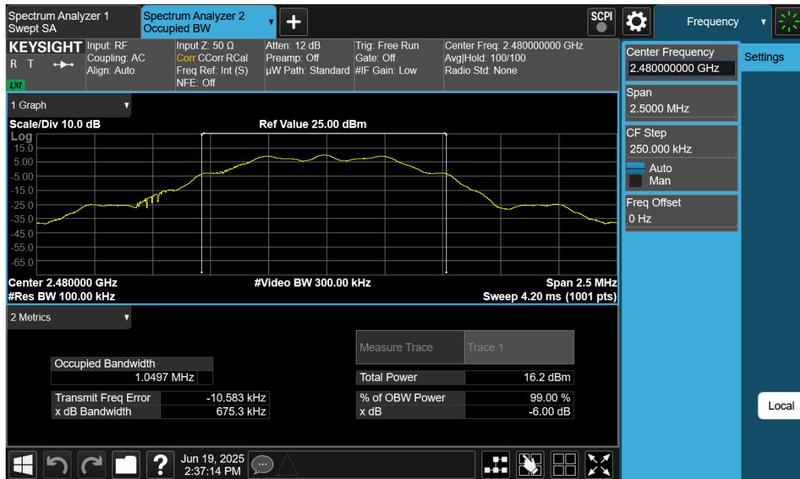
Plot 7-3. 6dB BW & 99% OBW Plot Antenna WF8 (Bluetooth (LE), 125kbps, ePA – Ch. 39)
