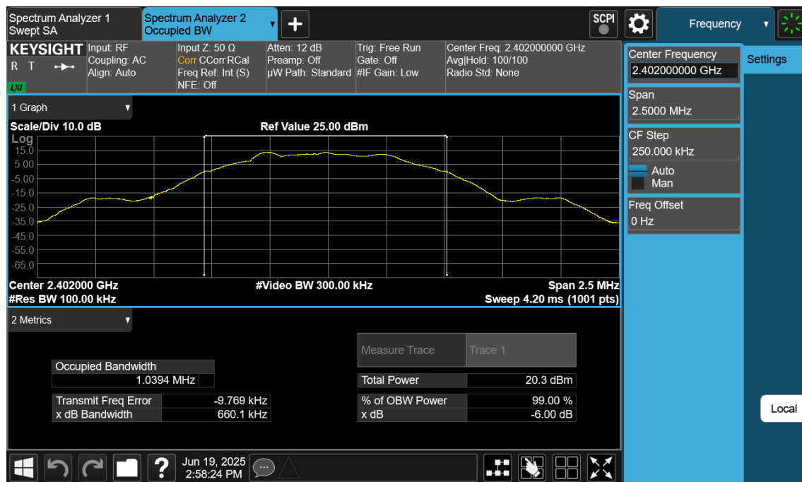
Plot 7-16. 6dB BW & 99% OBW Plot Antenna WF7 (Bluetooth (LE), 500kbps, ePA – Ch. 0)
