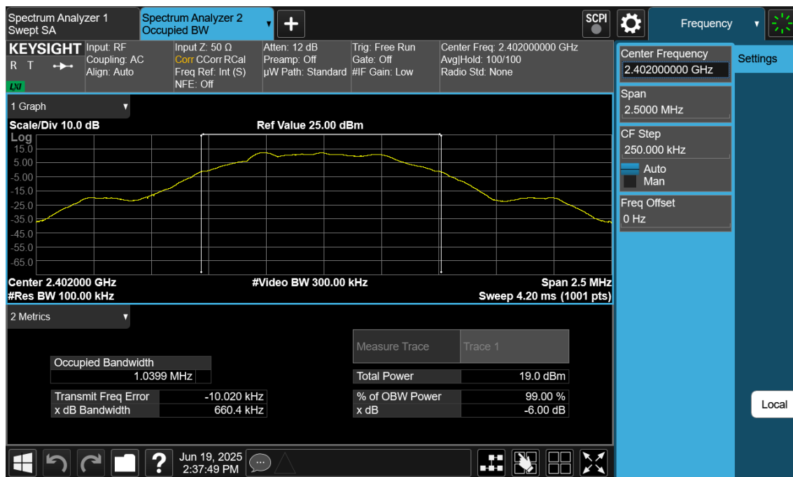
Plot 7-4. 6dB BW & 99% OBW Plot Antenna WF8 (Bluetooth (LE), 500kbps, ePA – Ch. 0)
