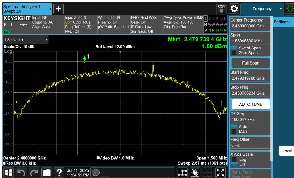
Plot 7-48. Power Spectral Density Plot Antenna WF8 (Bluetooth (LE), 500kbps, iPA – Ch. 39)
