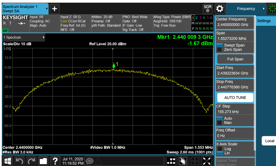
Plot 7-50. Power Spectral Density Plot Antenna WF8 (Bluetooth (LE), 1Mbps, ePA – Ch. 19)
