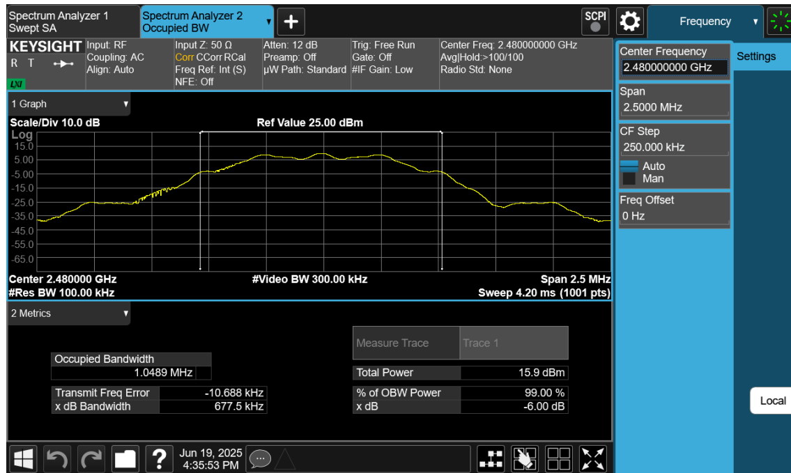
Plot 7-27. 6dB BW & 99% OBW Plot Antenna WF9 (Bluetooth (LE), 125kbps, ePA – Ch. 39)
