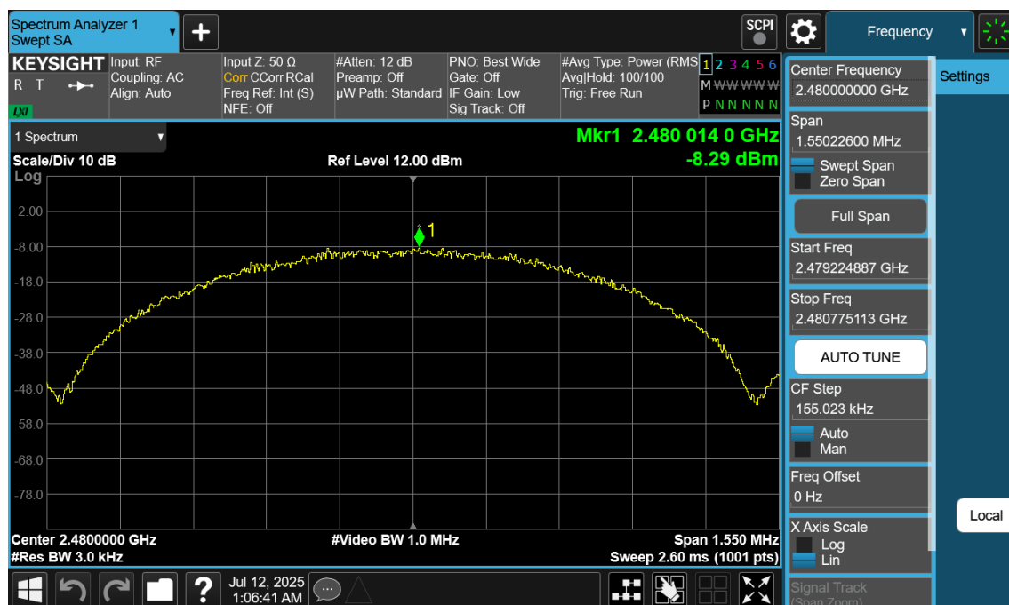
Plot 7-102. Power Spectral Density Plot Antenna WF9 (Bluetooth (LE), 1Mbps, iPA – Ch. 39)
