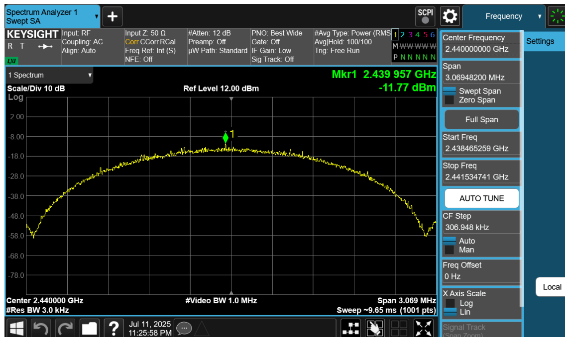
Plot 7-59. Power Spectral Density Plot Antenna WF8 (Bluetooth (LE), 2Mbps, iPA – Ch. 19)
