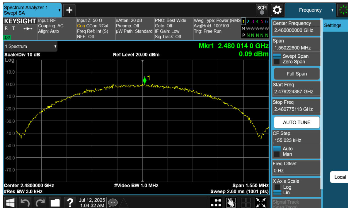
Plot 7-99. Power Spectral Density Plot Antenna WF9 (Bluetooth (LE), 1Mbps, ePA – Ch. 39)
