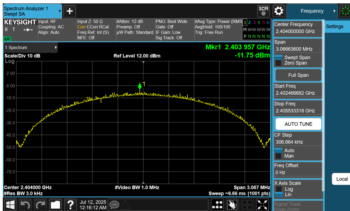
Plot 7-82. Power Spectral Density Plot Antenna WF7 (Bluetooth (LE), 2Mbps, iPA – Ch. 1)
