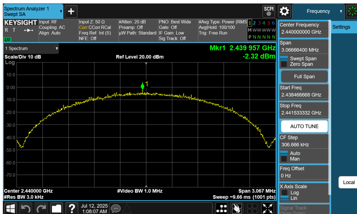
Plot 7-104. Power Spectral Density Plot Antenna WF9 (Bluetooth (LE), 2Mbps, ePA – Ch. 19)
