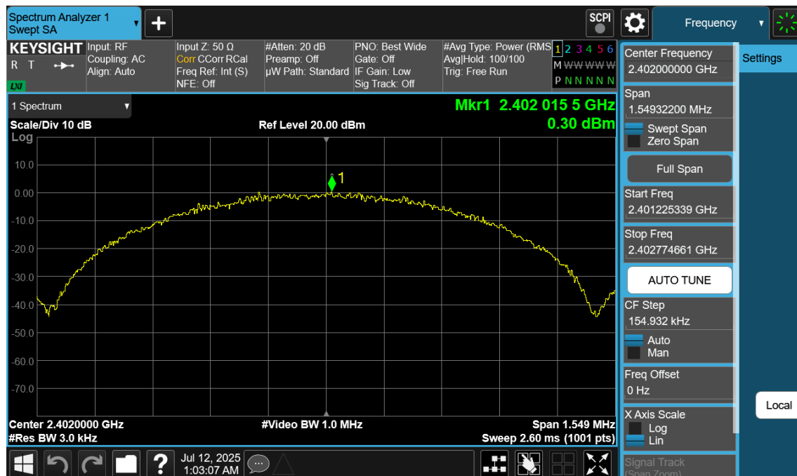
Plot 7-97. Power Spectral Density Plot Antenna WF9 (Bluetooth (LE), 1Mbps, ePA – Ch. 0)
