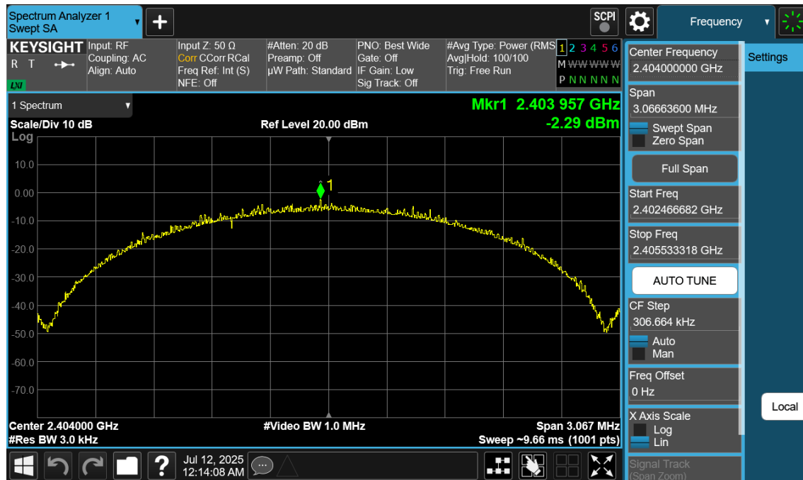
Plot 7-79. Power Spectral Density Plot Antenna WF7 (Bluetooth (LE), 2Mbps, ePA – Ch. 1)
