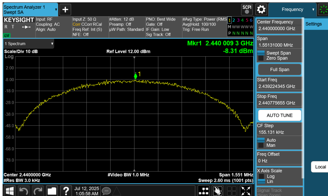
Plot 7-101. Power Spectral Density Plot Antenna WF9 (Bluetooth (LE), 1Mbps, iPA – Ch. 19)
