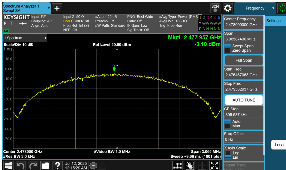
Plot 7-81. Power Spectral Density Plot Antenna WF7 (Bluetooth (LE), 2Mbps, ePA – Ch. 38)
