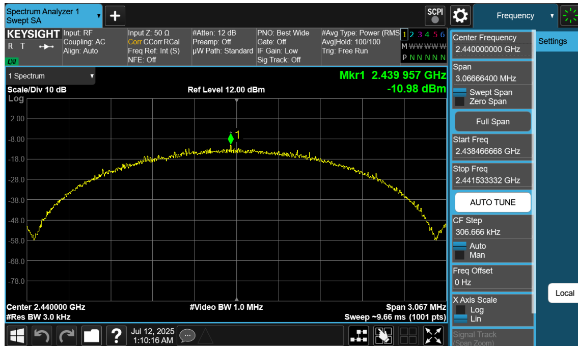
Plot 7-107. Power Spectral Density Plot Antenna WF9 (Bluetooth (LE), 2Mbps, iPA – Ch. 19)
