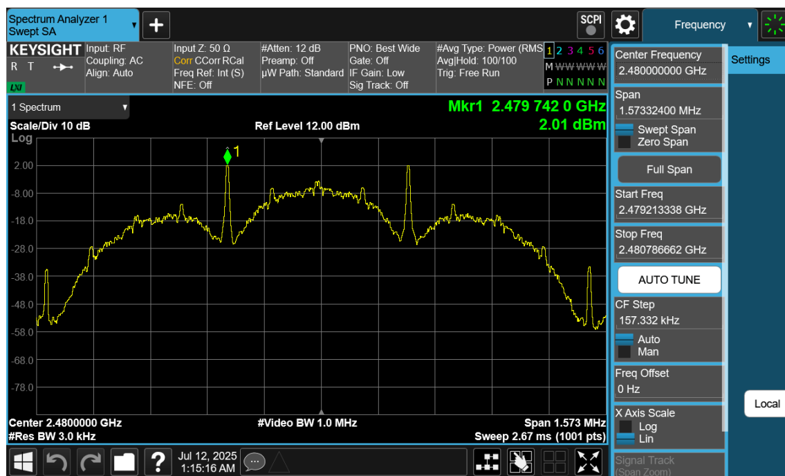
Plot 7-90. Power Spectral Density Plot Antenna WF9 (Bluetooth (LE), 125kbps, iPA – Ch. 39)
