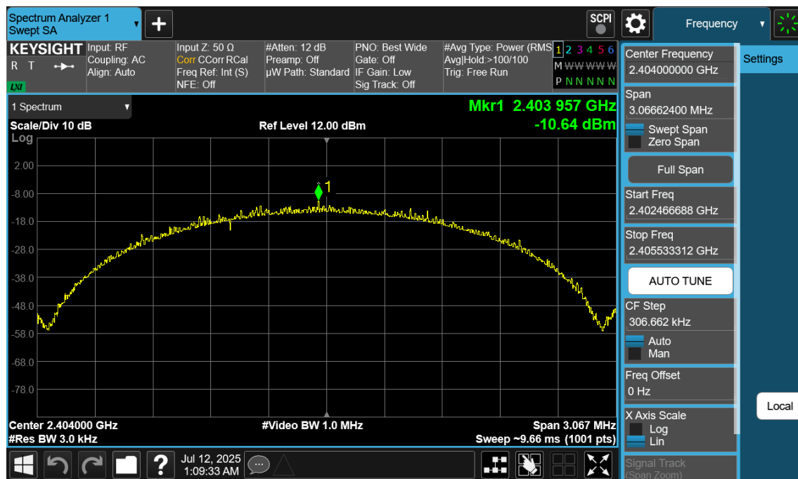
Plot 7-106. Power Spectral Density Plot Antenna WF9 (Bluetooth (LE), 2Mbps, iPA – Ch. 1)
