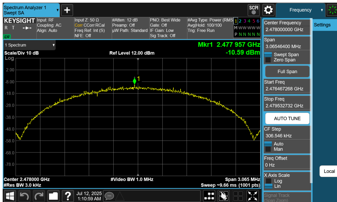
Plot 7-108. Power Spectral Density Plot Antenna WF9 (Bluetooth (LE), 2Mbps, iPA – Ch. 38)
