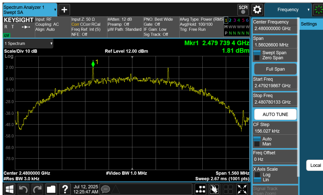
Plot 7-72. Power Spectral Density Plot Antenna WF7 (Bluetooth (LE), 500kbps, iPA – Ch. 39)
