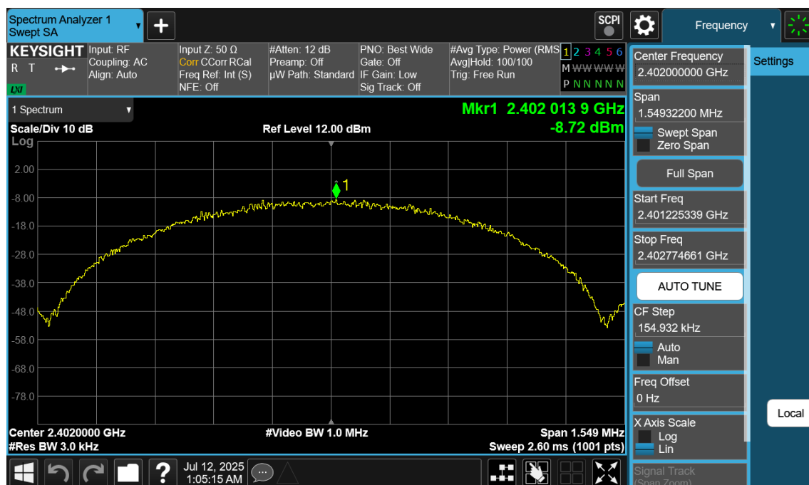
Plot 7-100. Power Spectral Density Plot Antenna WF9 (Bluetooth (LE), 1Mbps, iPA – Ch. 0)
