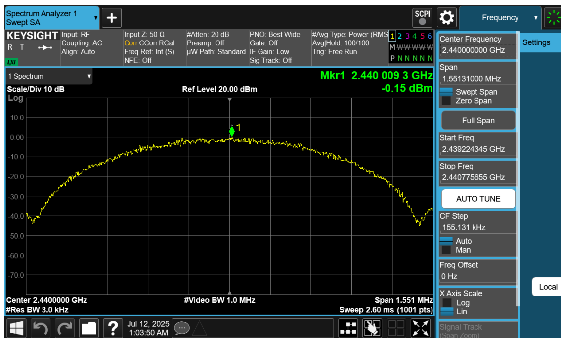
Plot 7-98. Power Spectral Density Plot Antenna WF9 (Bluetooth (LE), 1Mbps, ePA – Ch. 19)
