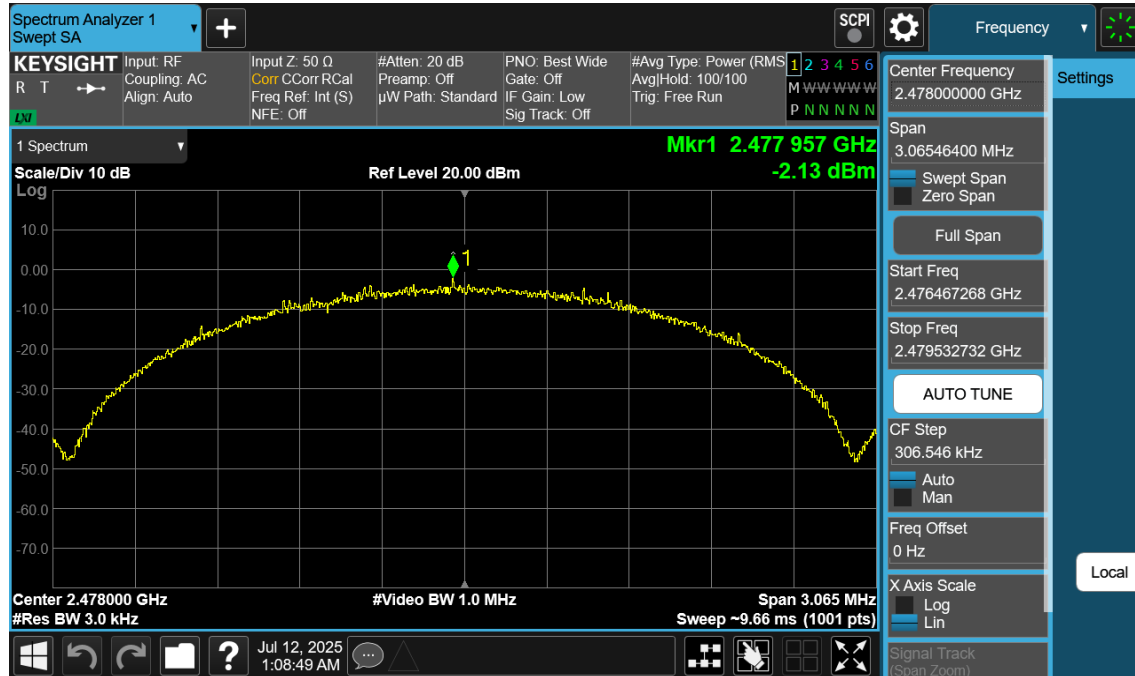
Plot 7-105. Power Spectral Density Plot Antenna WF9 (Bluetooth (LE), 2Mbps, ePA – Ch. 38)
