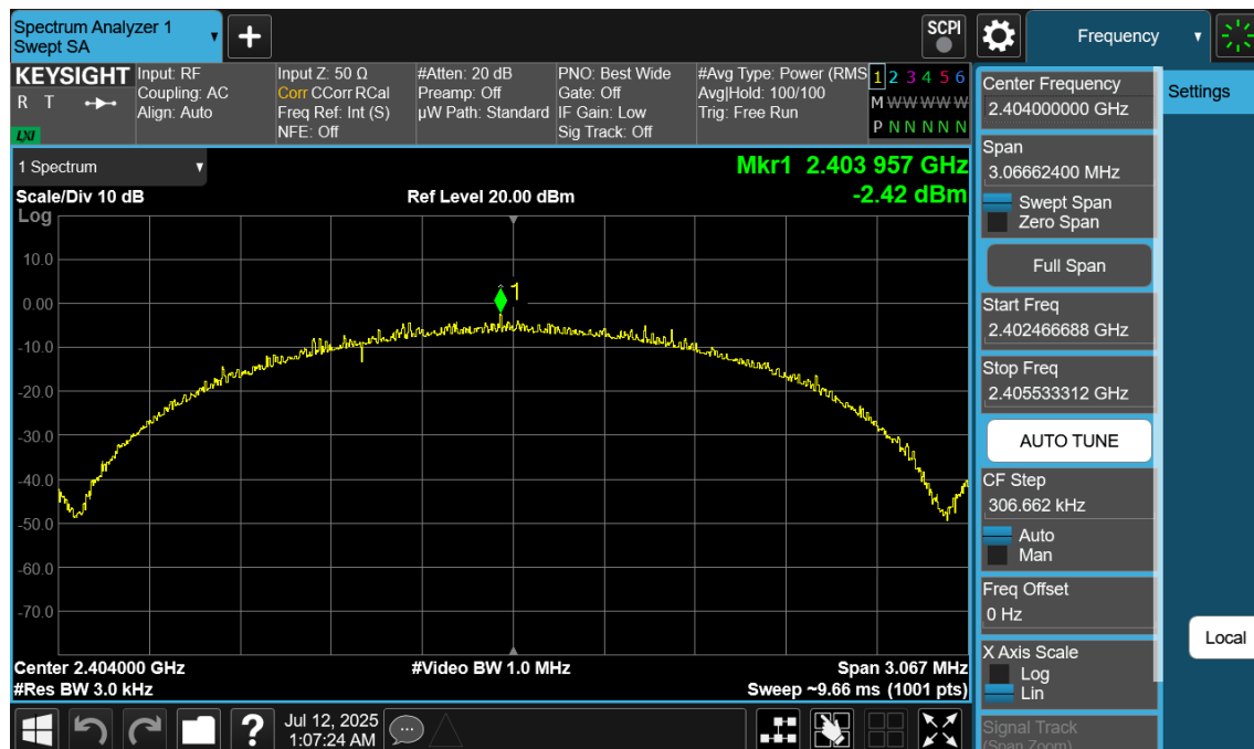
Plot 7-103. Power Spectral Density Plot Antenna WF9 (Bluetooth (LE), 2Mbps, ePA – Ch. 1)
