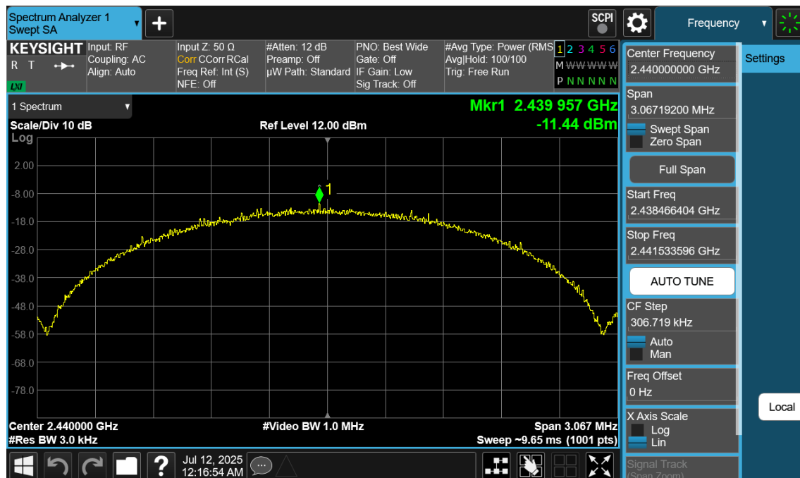
Plot 7-83. Power Spectral Density Plot Antenna WF7 (Bluetooth (LE), 2Mbps, iPA – Ch. 19)
