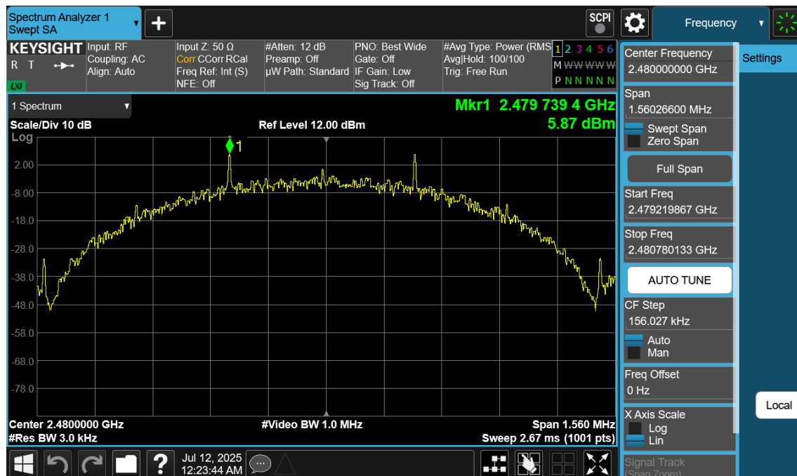
Plot 7-69. Power Spectral Density Plot Antenna WF7 (Bluetooth (LE), 500kbps, ePA – Ch. 39)
