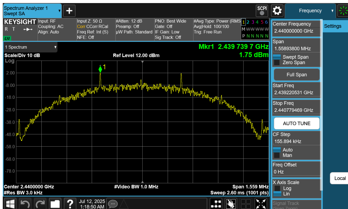
Plot 7-95. Power Spectral Density Plot Antenna WF9 (Bluetooth (LE), 500kbps, iPA – Ch. 19)
