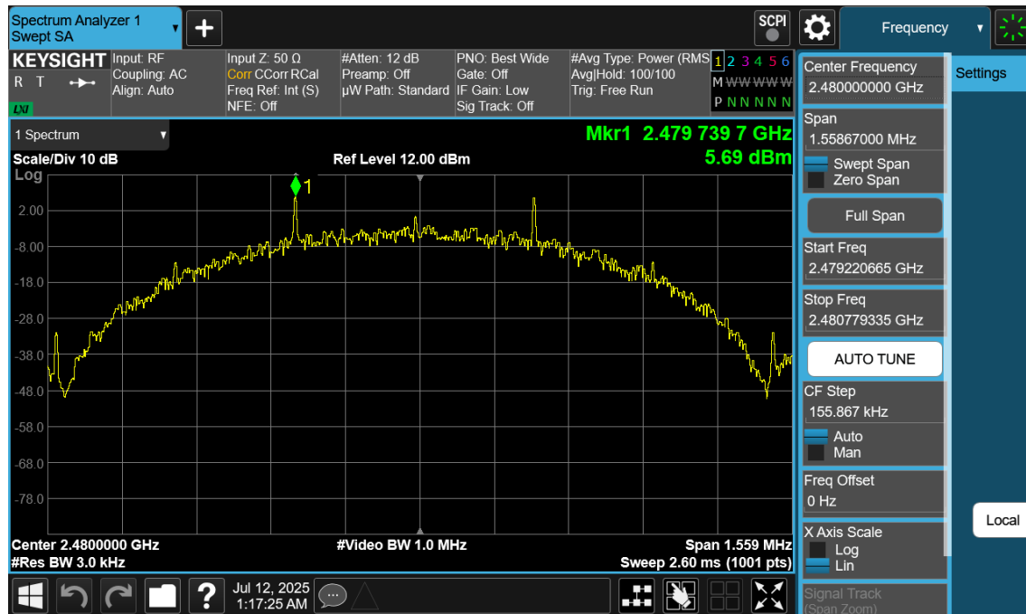
Plot 7-93. Power Spectral Density Plot Antenna WF9 (Bluetooth (LE), 500kbps, ePA – Ch. 39)
