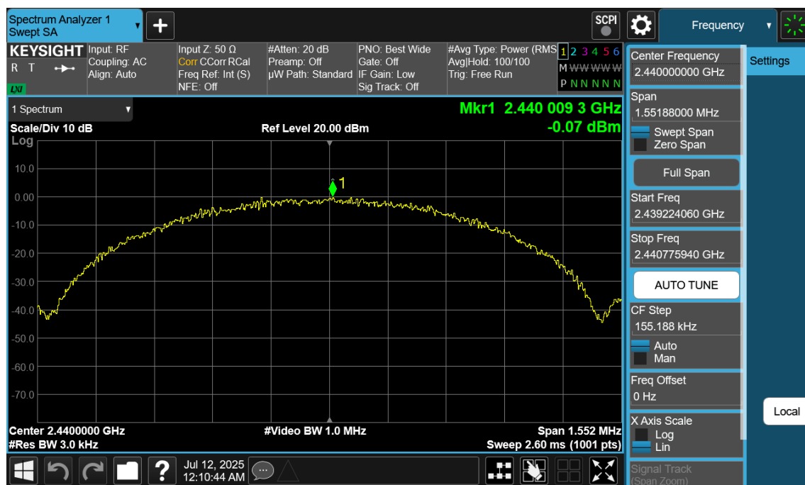
Plot 7-74. Power Spectral Density Plot Antenna WF7 (Bluetooth (LE), 1Mbps, ePA – Ch. 19)
