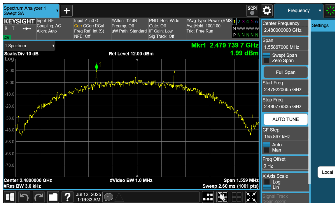
Plot 7-96. Power Spectral Density Plot Antenna WF9 (Bluetooth (LE), 500kbps, iPA – Ch. 39)
