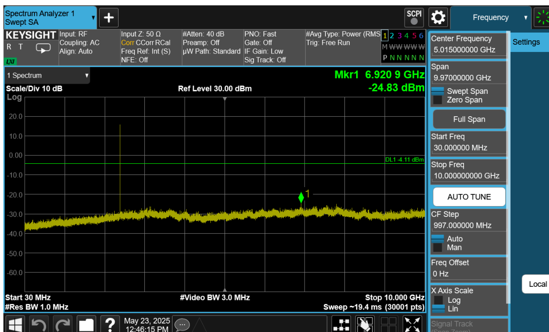
Plot 7-235. Conducted Spurious Plot Antenna WF7 (Bluetooth (LE), 1Mbps, ePA – Ch. 0)
