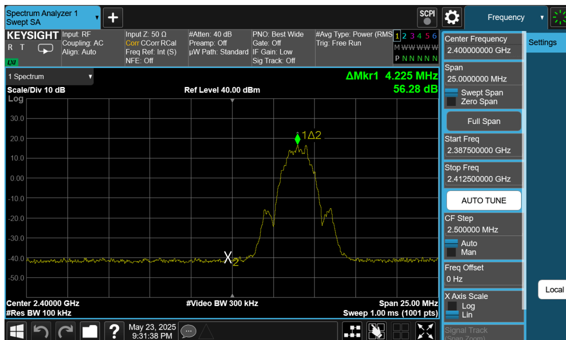
Plot 7-227. Band Edge Plot Antenna WF9 (Bluetooth (LE), 2Mbps, ePA – Ch. 1)
