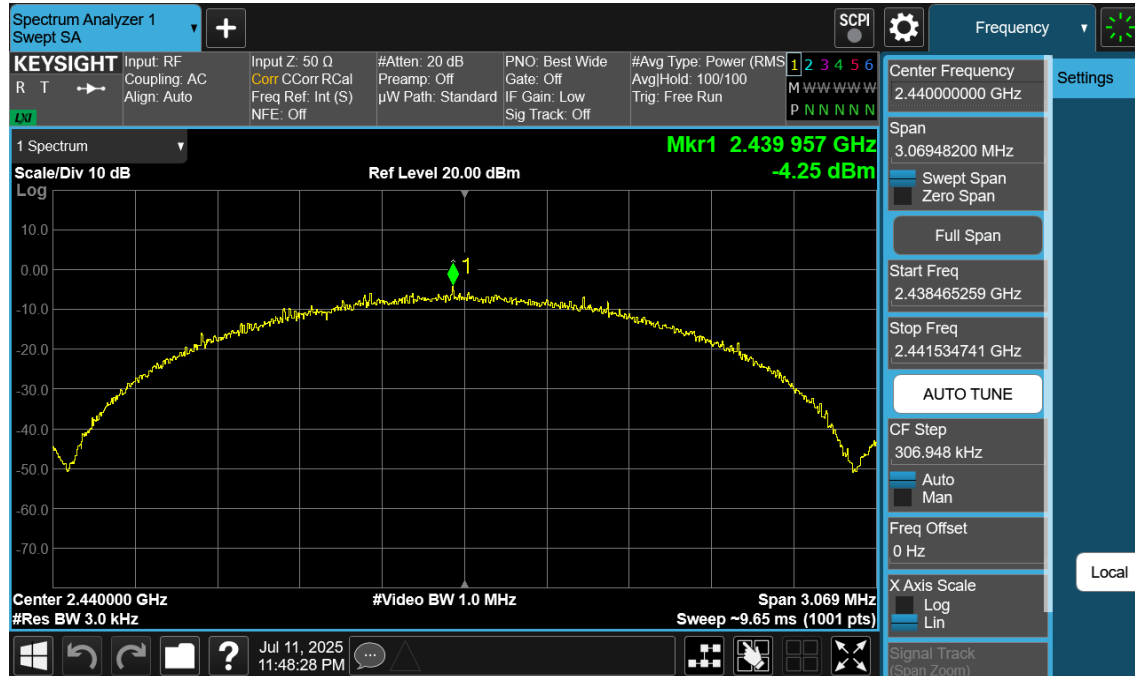
Plot 7-195. Power Spectral Density Plot Antenna WF8 (Bluetooth (LE), 2Mbps, ePA – Ch. 19)
