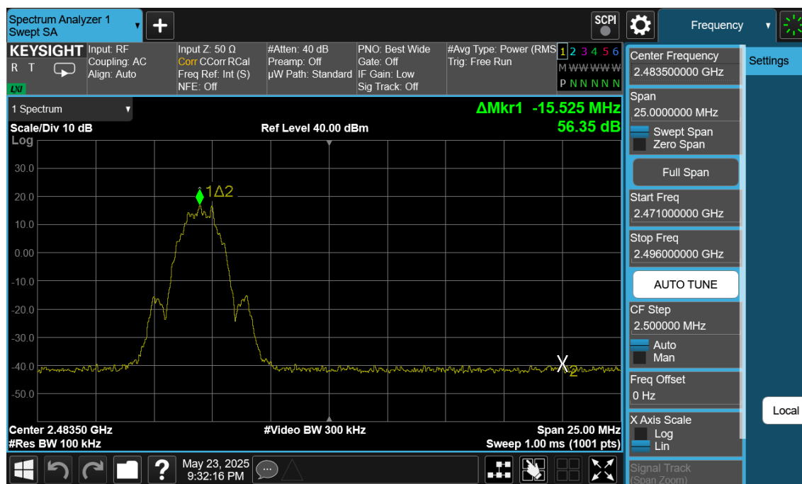
Plot 7-228. Band Edge Plot Antenna WF9 (Bluetooth (LE), 2Mbps, ePA – Ch. 38)
