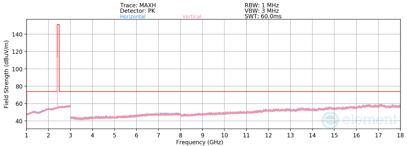
Plot 7-251. Radiated Spurious Emissions 1-18GHz TxBF Diversity (1Mbps, ePA – Ch. 0)
