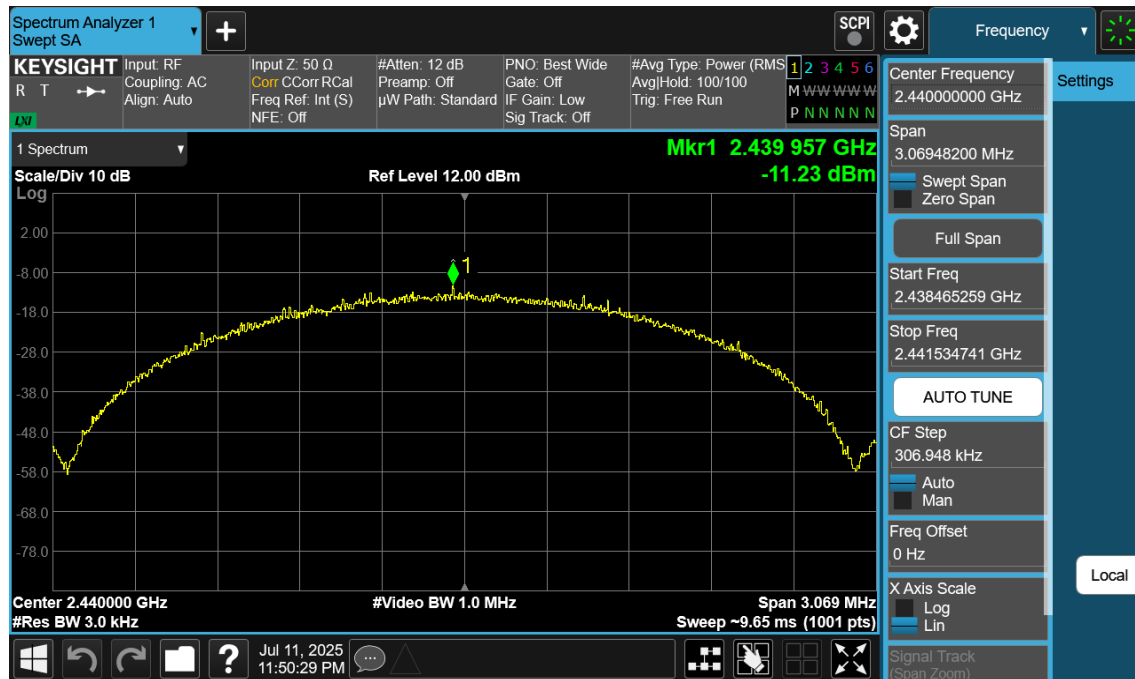
Plot 7-201. Power Spectral Density Plot Antenna WF8 (Bluetooth (LE), 2Mbps, iPA – Ch. 19)
