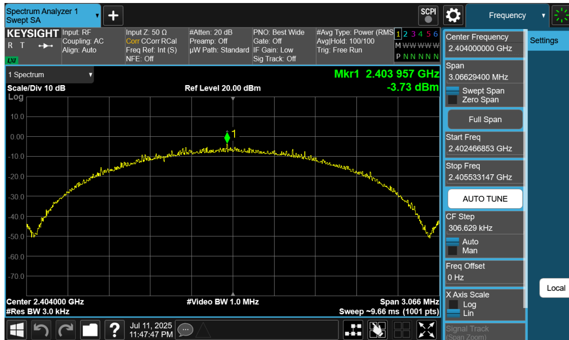
Plot 7-193. Power Spectral Density Plot Antenna WF8 (Bluetooth (LE), 2Mbps, ePA – Ch. 1)
