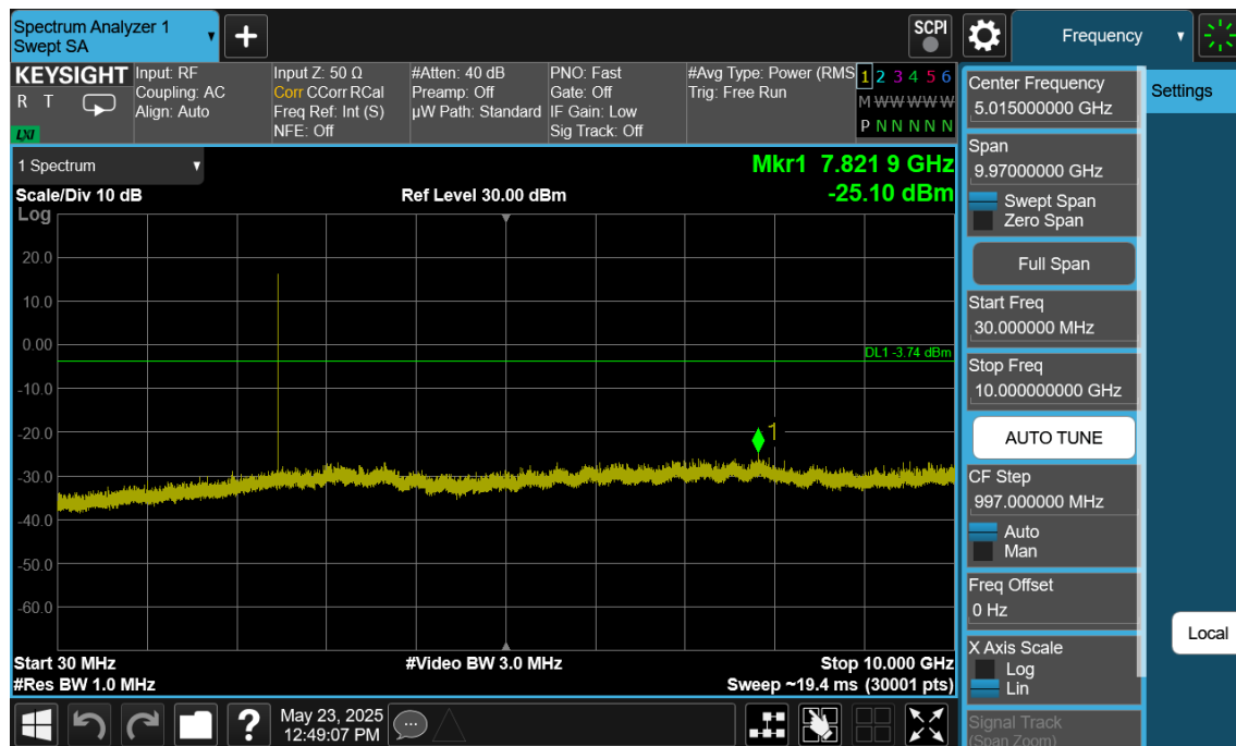
Plot 7-239. Conducted Spurious Plot Antenna WF7 (Bluetooth (LE), 1Mbps, ePA – Ch. 39)
