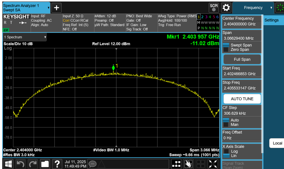
Plot 7-199. Power Spectral Density Plot Antenna WF8 (Bluetooth (LE), 2Mbps, iPA – Ch. 1)
