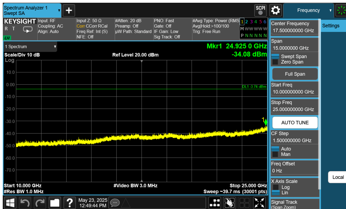
Plot 7-240. Conducted Spurious Plot Antenna WF7 (Bluetooth (LE), 1Mbps, ePA – Ch. 39)
