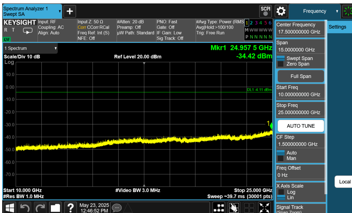
Plot 7-236. Conducted Spurious Plot Antenna WF7 (Bluetooth (LE), 1Mbps, ePA – Ch. 0)
