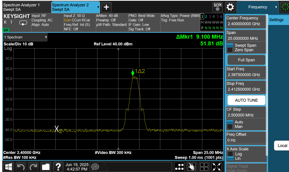
Plot 7-223. Band Edge Plot Antenna WF9 (Bluetooth (LE), 500kbps, ePA – Ch.0)
