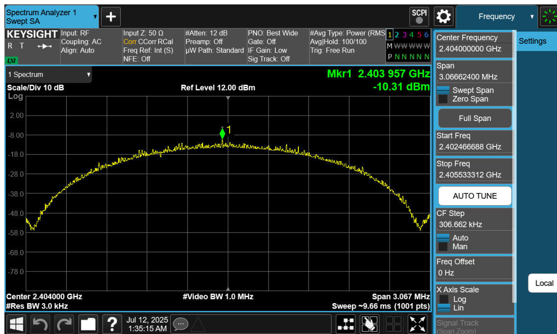
Plot 7-200. Power Spectral Density Plot Antenna WF9 (Bluetooth (LE), 2Mbps, iPA – Ch. 1)
