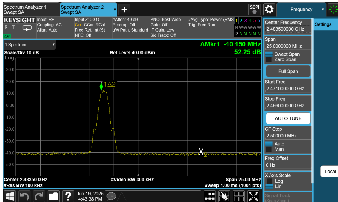
Plot 7-224. Band Edge Plot Antenna WF9 (Bluetooth (LE), 500kbps, ePA – Ch. 39)
