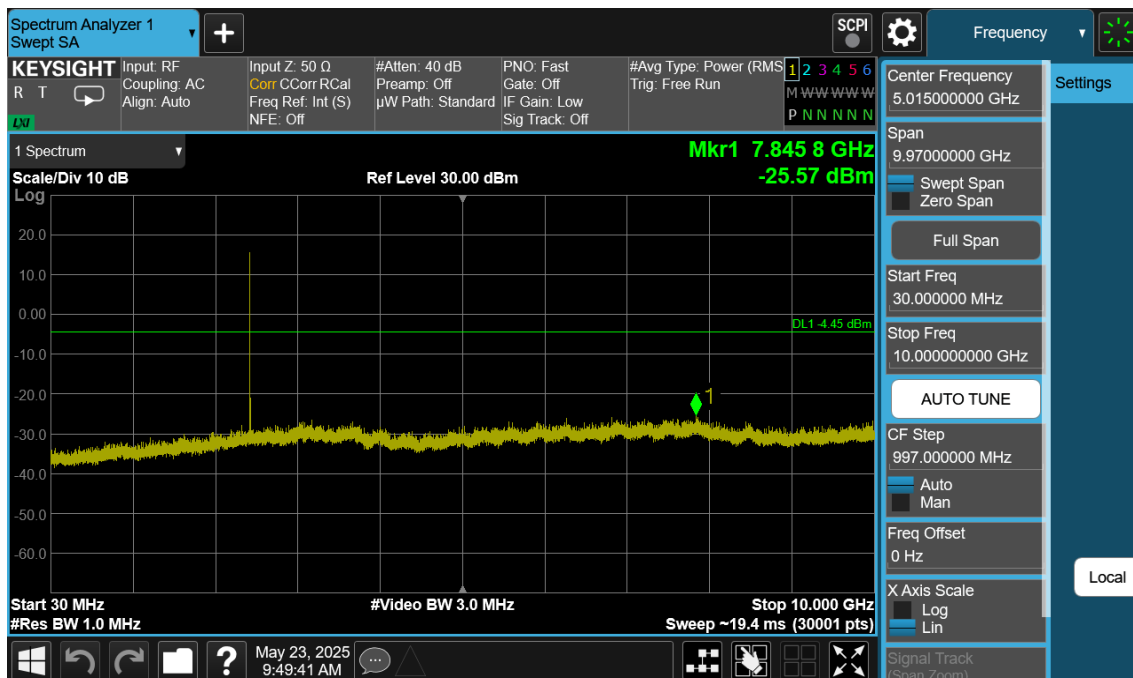
Plot 7-231. Conducted Spurious Plot Antenna WF8 (Bluetooth (LE), 1Mbps, ePA – Ch. 19)
