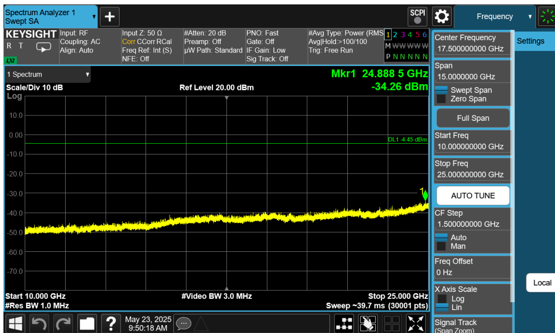
Plot 7-232. Conducted Spurious Plot Antenna WF8 (Bluetooth (LE), 1Mbps, ePA – Ch. 19)
