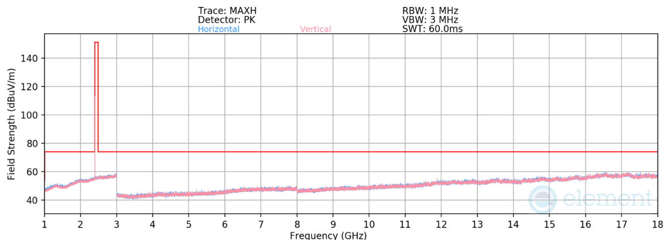
Plot 7-247. Radiated Spurious Emissions 1-18GHz TxBF Primary (1Mbps, ePA – Ch. 0)
