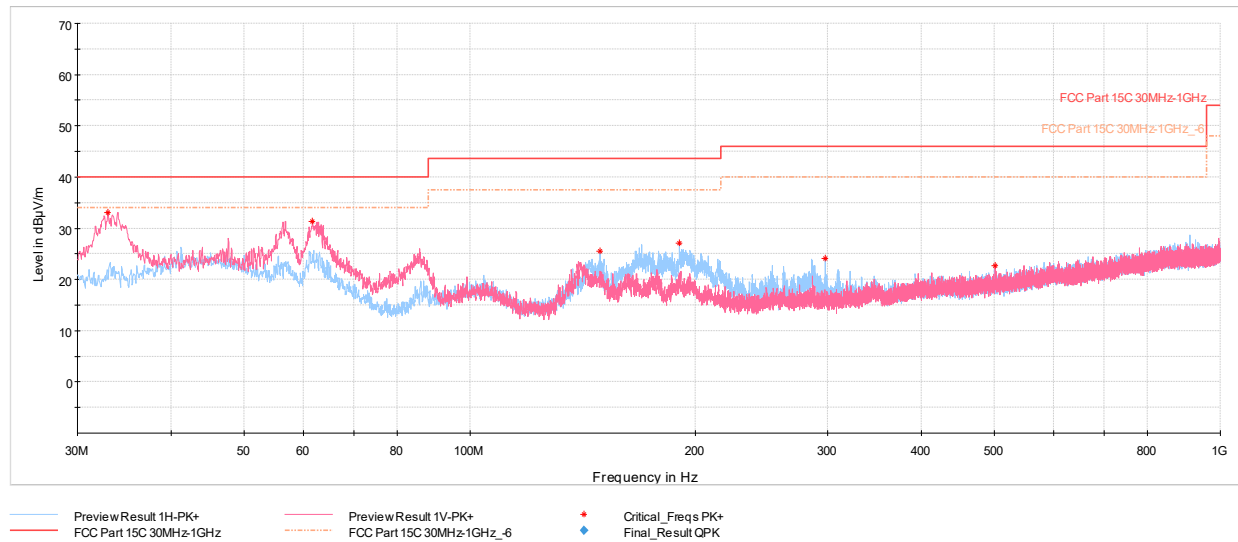
Plot 7-276. Radiated Spurious Emissions Below 1GHz TxBF Diversity (1Mbps, ePA – Ch.19, Pol. H & V, with AC/DC Adapter)
