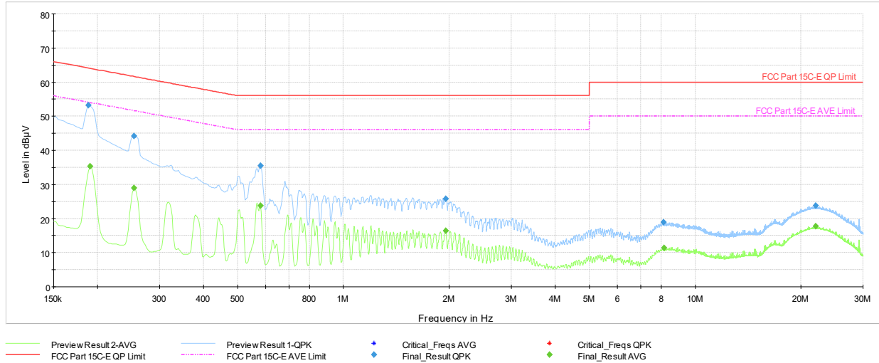
Plot 7-280. AC Line Conducted Plot with Bluetooth LE Tx/BF Diversity (N, 1Mbps ePA – Ch.19, with AC/DC Adapter)
