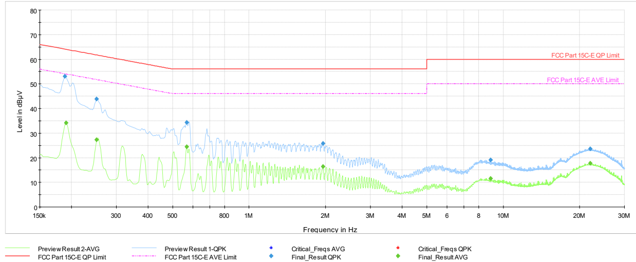
Plot 7-278. AC Line Conducted Plot with Bluetooth LE Tx BF Primary (N, 1Mbps ePA – Ch.19, with AC/DC Adapter)
