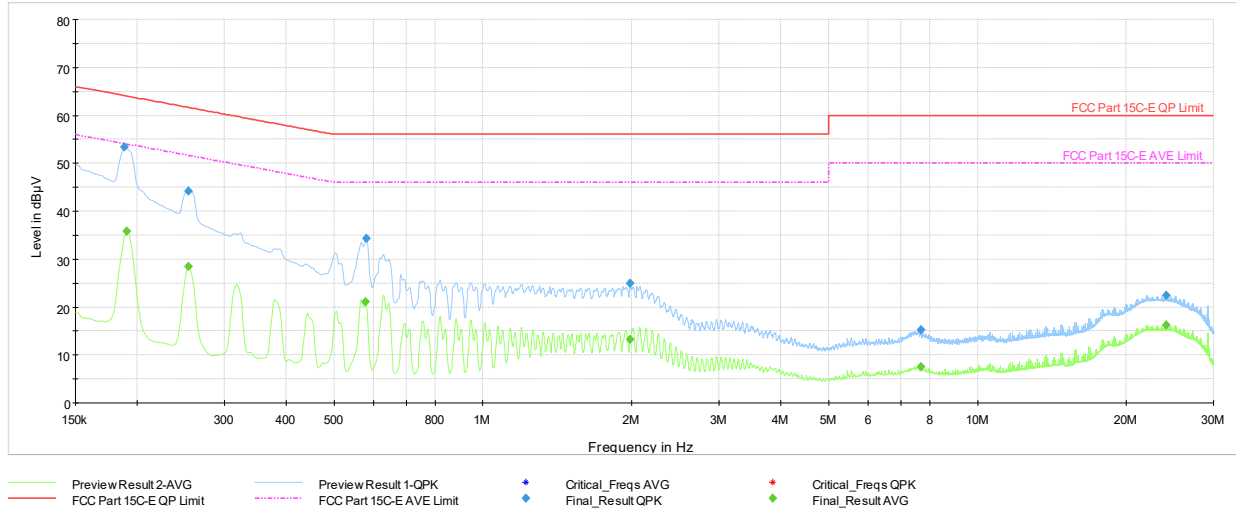
Plot 7-279. AC Line Conducted Plot with Bluetooth LE Tx BF Diversity (L1, 1Mbps ePA – Ch.19 with AC/DC Adapter)
