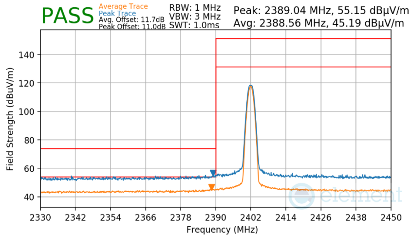
Plot 7-267. Radiated Restricted Lower Band Edge Measurement TxBF Primary (Average & Peak)
