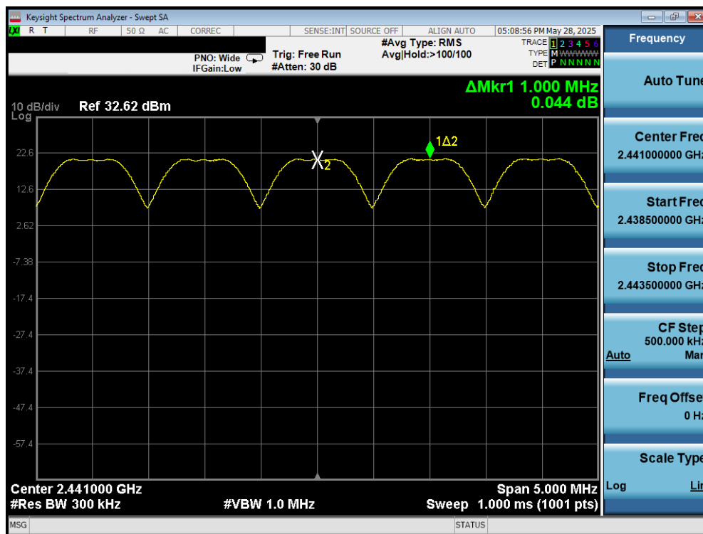
Plot 7-47. Channel Spacing Plot Antenna WF9 (Bluetooth, GFSK, ePA)
