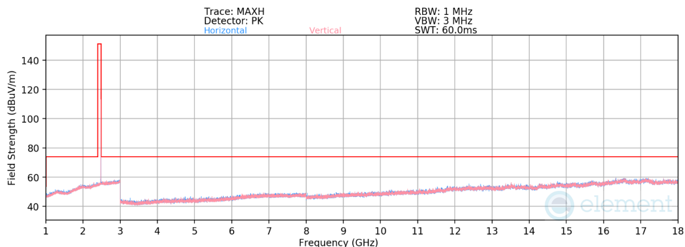
Plot 7-90. Radiated Spurious Emissions above 1GHz TxBF Primary (BT GFSK ePA – Ch. 78)
