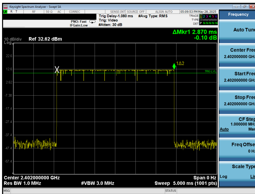
Plot 7-53. Time of Occupancy Plot Antenna WF9 (Bluetooth, GFSK, ePA)
