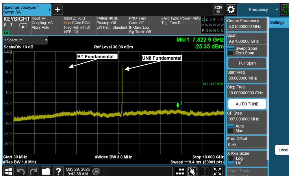
Plot 7-85. Conducted Simultaneous Tx Spurious Plot Antenna WF7 (Bluetooth + UNII)
