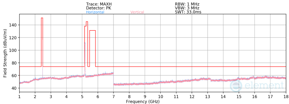
Plot 7-95. Radiated Spurious Emissions above 1GHz – Simultaneous Transmission
