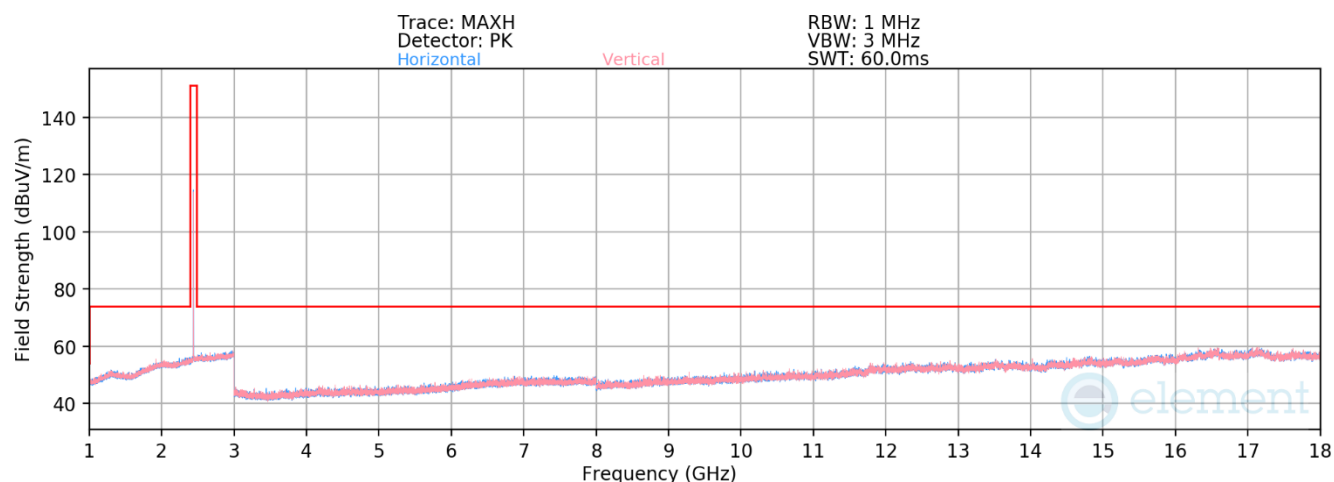
Plot 7-92. Radiated Spurious Emissions above 1GHz Tx BF Diversity (BT GFSK ePA – Ch. 39)
