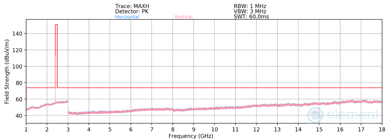
Plot 7-87. Radiated Spurious Emissions above 1GHz TxBF Primary (BT GFSK ePA – Ch. 0)
