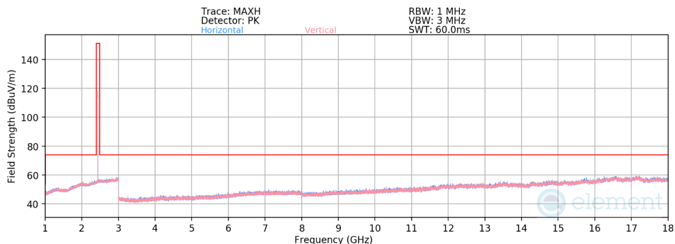
Plot 7-88. Radiated Spurious Emissions above 1GHz TxBF Primary (BT GFSK ePA – Ch. 39)
