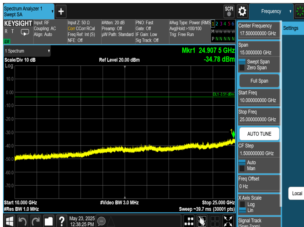
Plot 7-74. Conducted Spurious Plot Antenna WF7 (Bluetooth, GFSK, ePA – Ch. 0)
