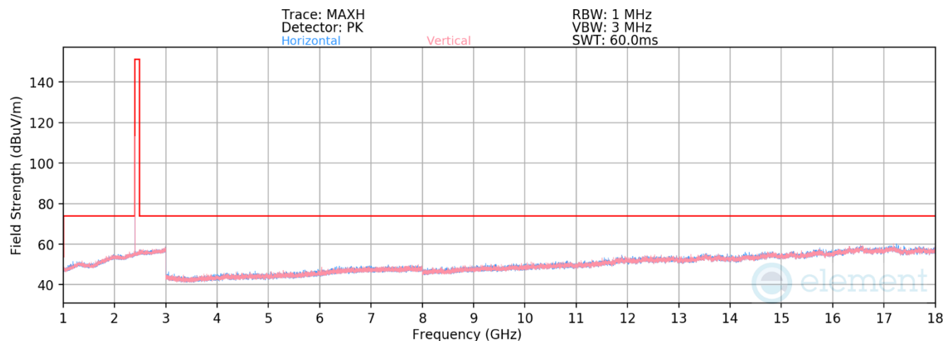
Plot 7-91. Radiated Spurious Emissions above 1GHz TxBF Diversity (BT GFSK ePA – Ch. 0)
