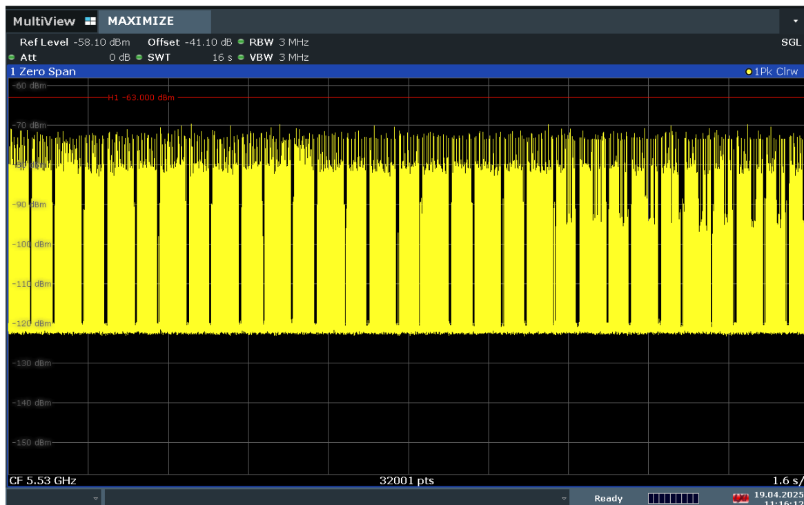
Figure 9-7. 5530MHz - Channel Loading - Mode 3 (80MHz)
