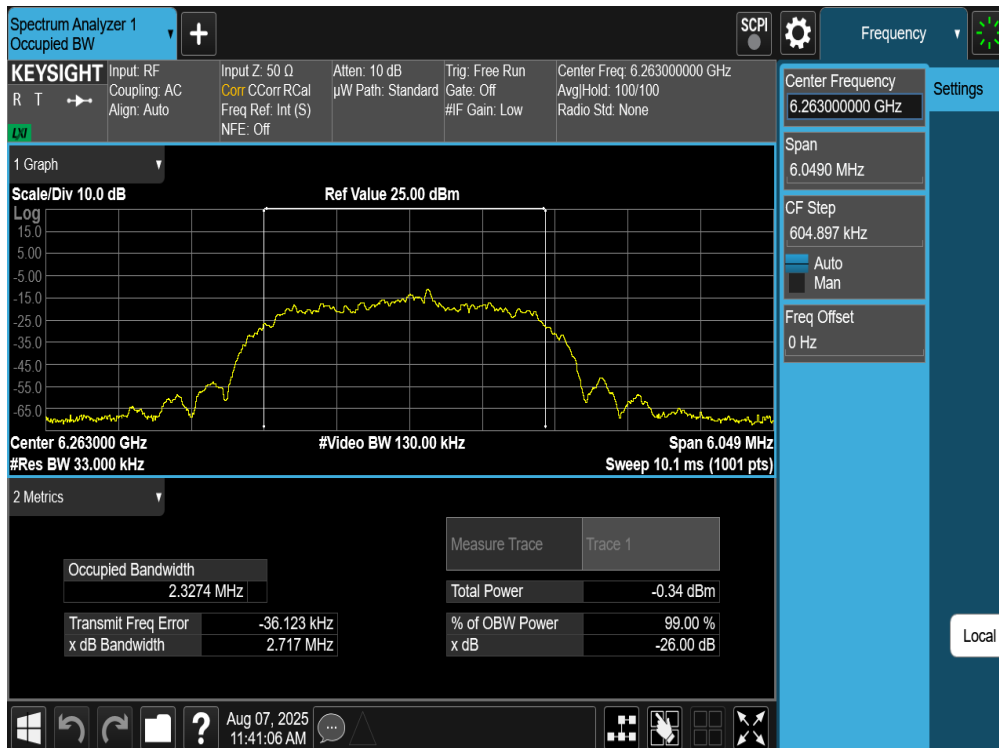
Plot 7-4. 26dB BW & 99% OBW Antenna WF5B (NB UNII HDR4, ePA- 6263MHz)
