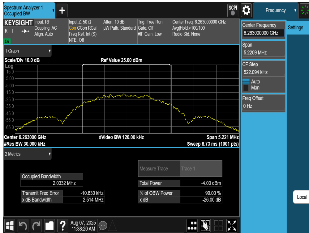
Plot 7-3. 26dB BW & 99% OBW Antenna WF5B (NB UNII LE2M, ePA- 6263MHz)
