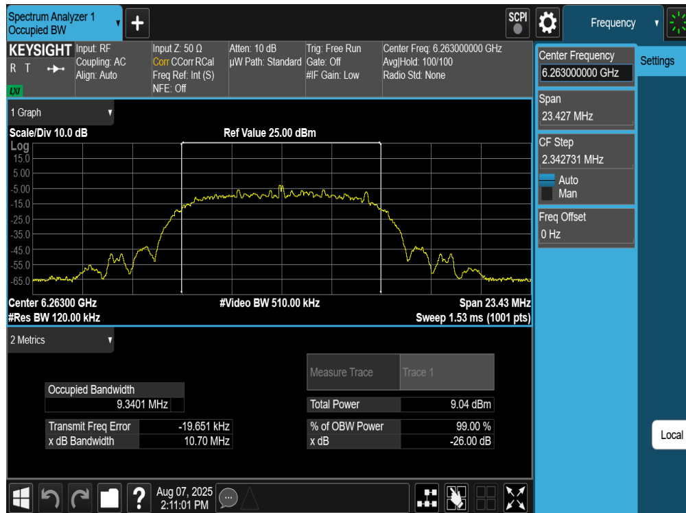
Plot 7-22. 26dB BW & 99% OBW Antenna WF8 (NB UNII HDRPL12, ePA- 6263MHz)
