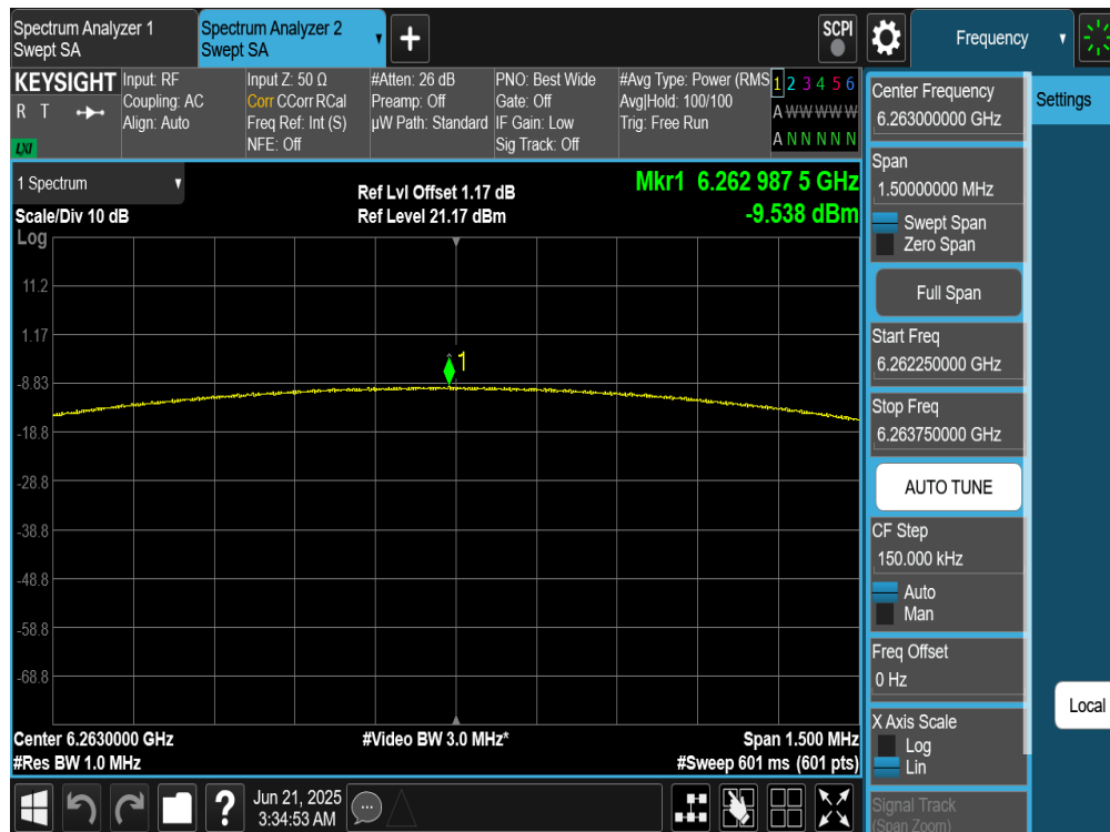
Plot 7-40. PSD Antenna WF5B (NB UNII BDR, ePA – 6263MHz)
