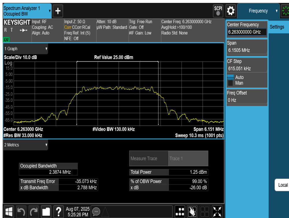
Plot 7-39. 26dB BW & 99% OBW Antenna WF7 (NB UNII HDT6, ePA– 6263MHz)
