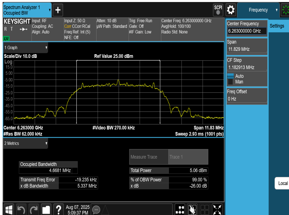
Plot 7-34. 26dB BW & 99% OBW Antenna WF7 (NB UNII HDRPM16, ePA– 6263MHz)
