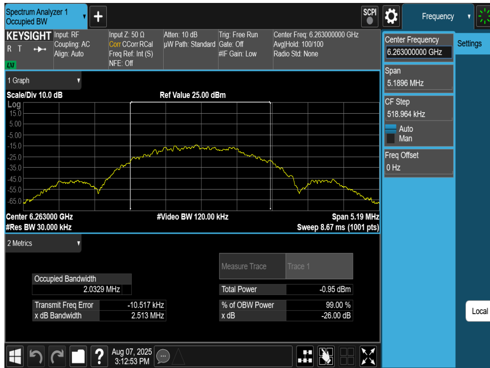
Plot 7-16. 26dB BW & 99% OBW Antenna WF8 (NB UNII LE2M, ePA- 6263MHz)
