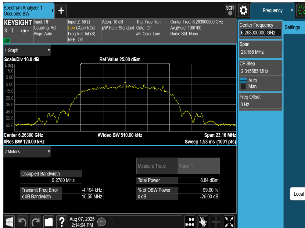
Plot 7-23. 26dB BW & 99% OBW Antenna WF8 (NB UNII HDRPL32, ePA- 6263MHz)
