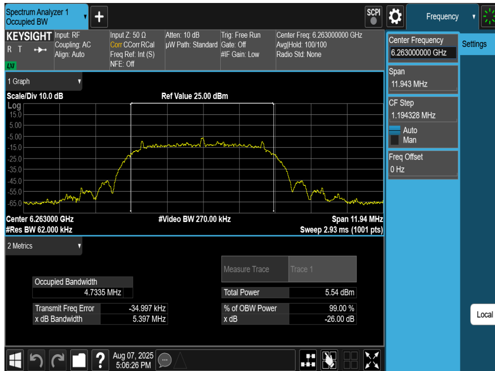
Plot 7-33. 26dB BW & 99% OBW Antenna WF7 (NB UNII XHDRPM6, ePA– 6263MHz)
