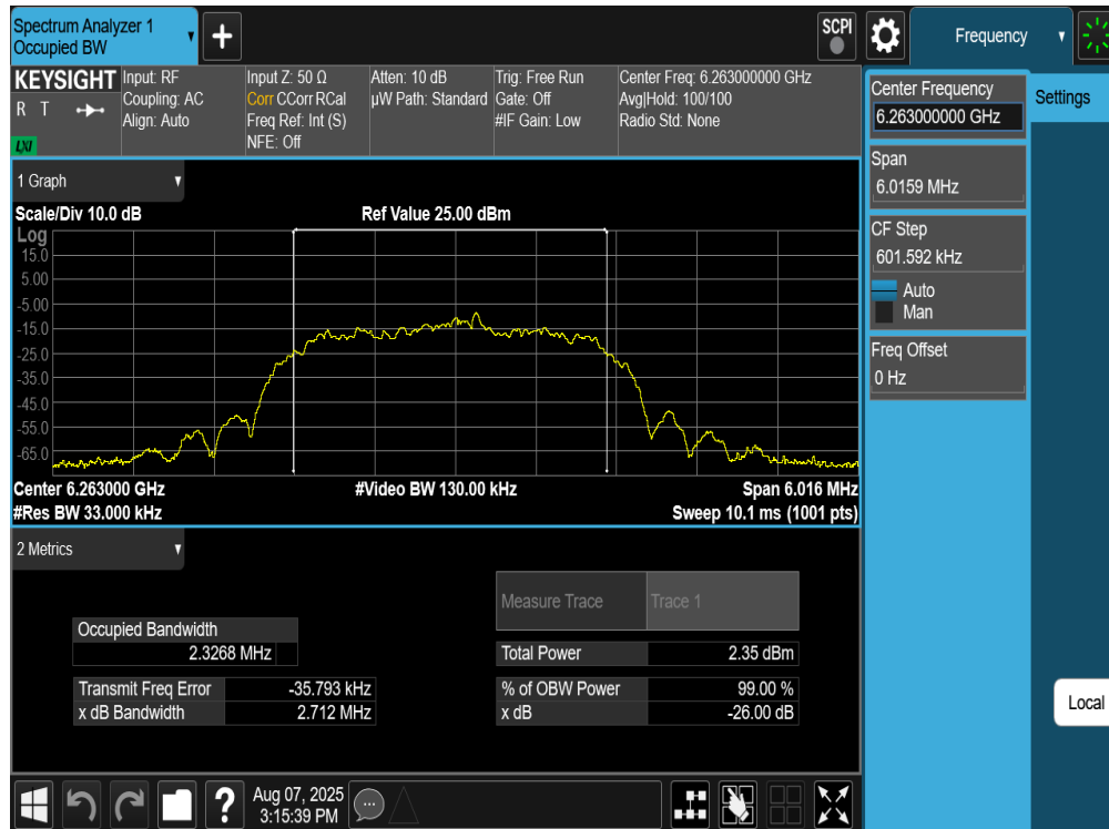
Plot 7-17. 26dB BW & 99% OBW Antenna WF8 (NB UNII HDR4, ePA- 6263MHz)
