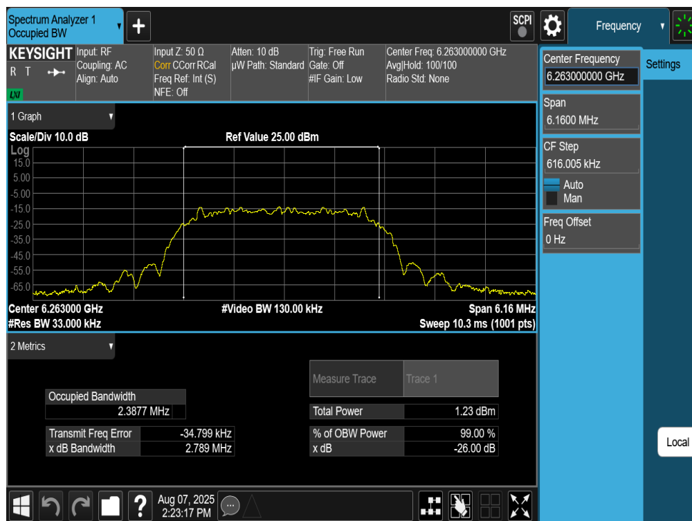
Plot 7-26. 26dB BW & 99% OBW Antenna WF8 (NB UNII HDT6, ePA– 6263MHz)
