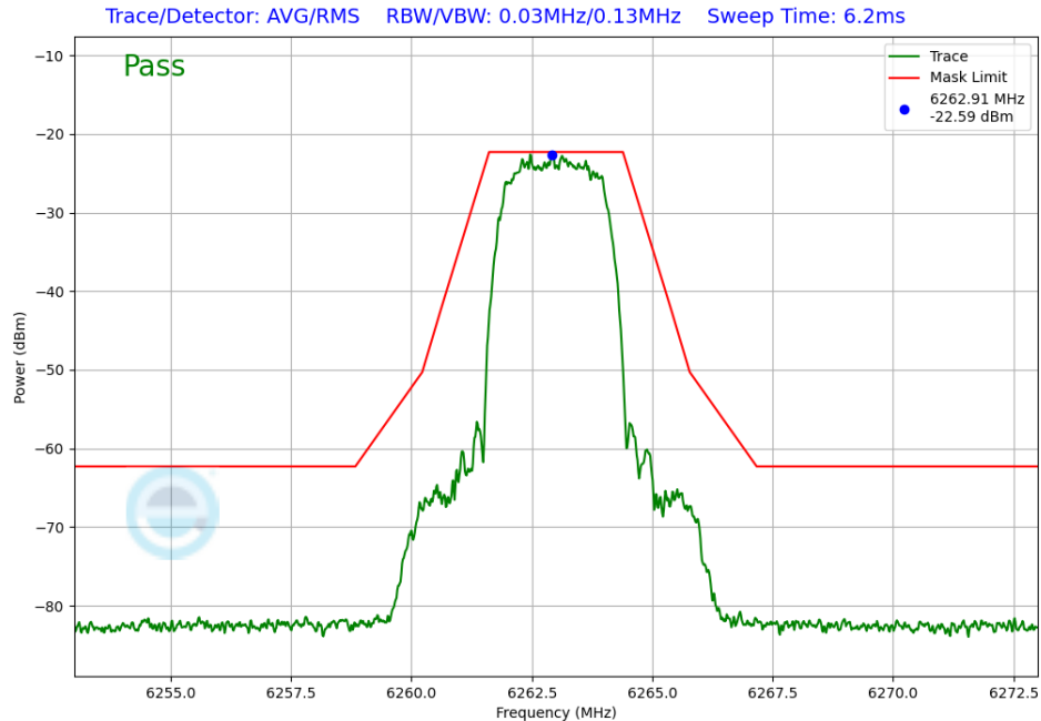
Plot 7-273. In-Band Emission Antenna WF8 (NB UNII HDT6, iPA – 6263MHz)
