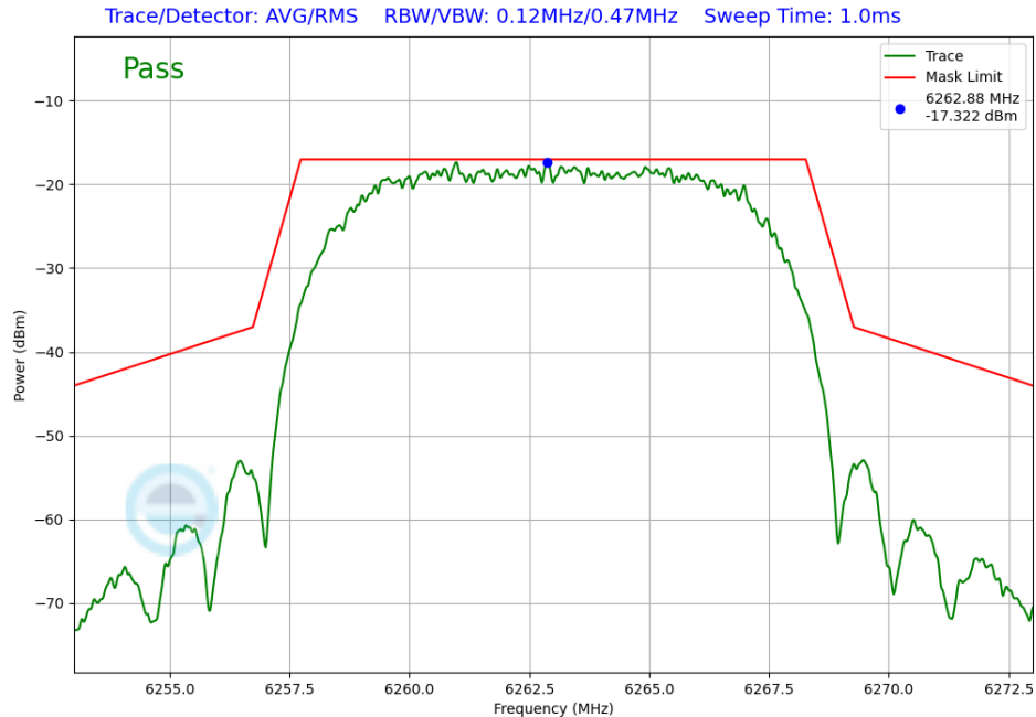
Plot 7-267. In-Band Emission Antenna WF8 (NB UNII HDRPL32, iPA – 6263MHz)
