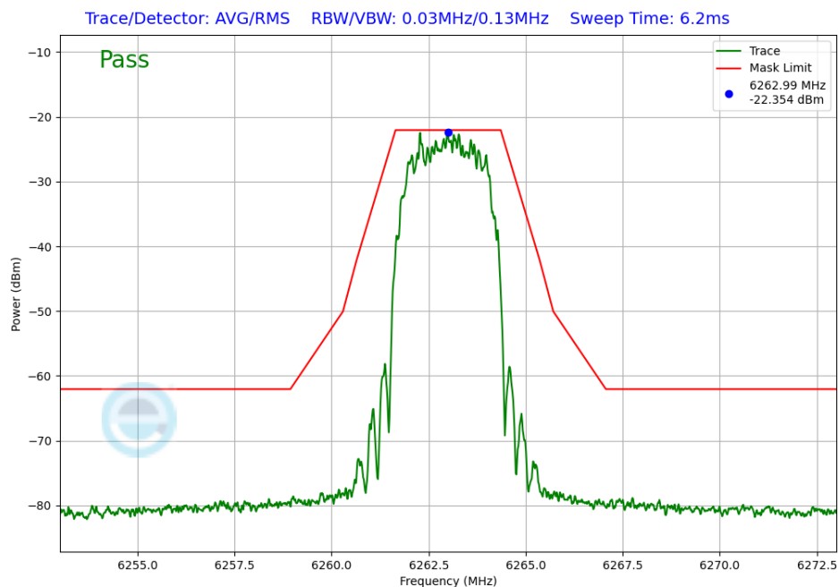
Plot 7-280. In-Band Emission Antenna WF7 (NB UNII HDR4, ePA – 6263MHz)
