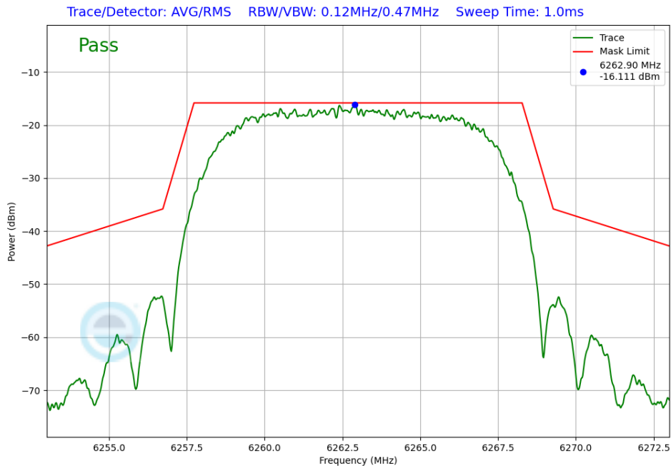
Plot 7-292. In-Band Emission Antenna WF7 (NB UNII HDRPL32, ePA – 6263MHz)
