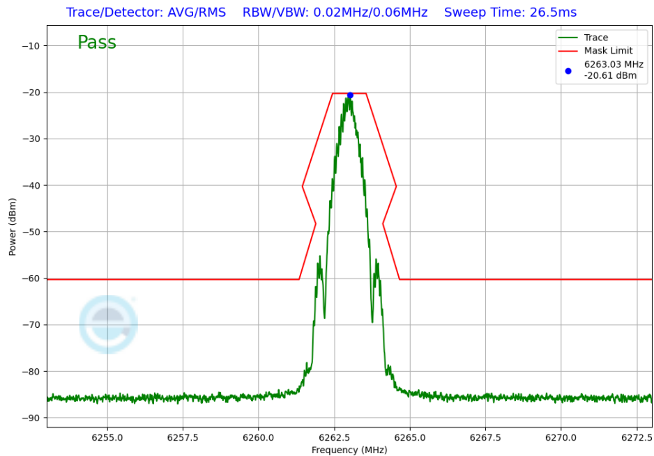
Plot 7-275. In-Band Emission Antenna WF7 (NB UNII BDR, iPA – 6263MHz)
