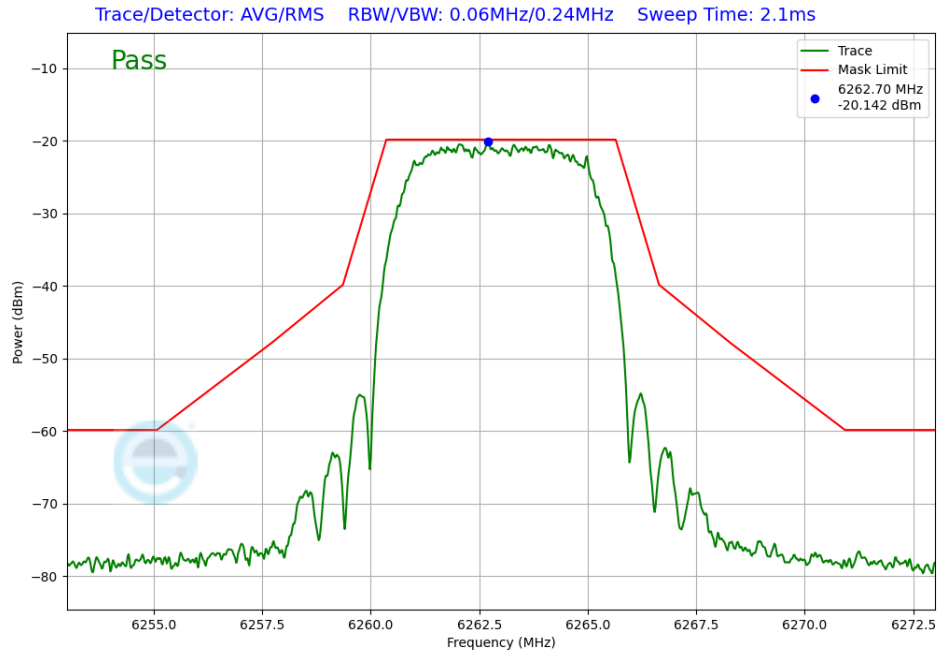
Plot 7-263. In-Band Emission Antenna WF8 (NB UNII HDRPM16, iPA – 6263MHz)
