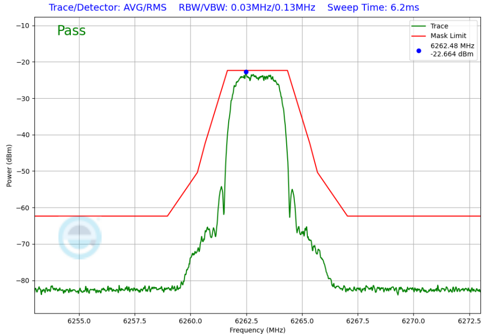
Plot 7-259. In-Band Emission Antenna WF8 (NB UNII HDRPS2, iPA – 6263MHz)
