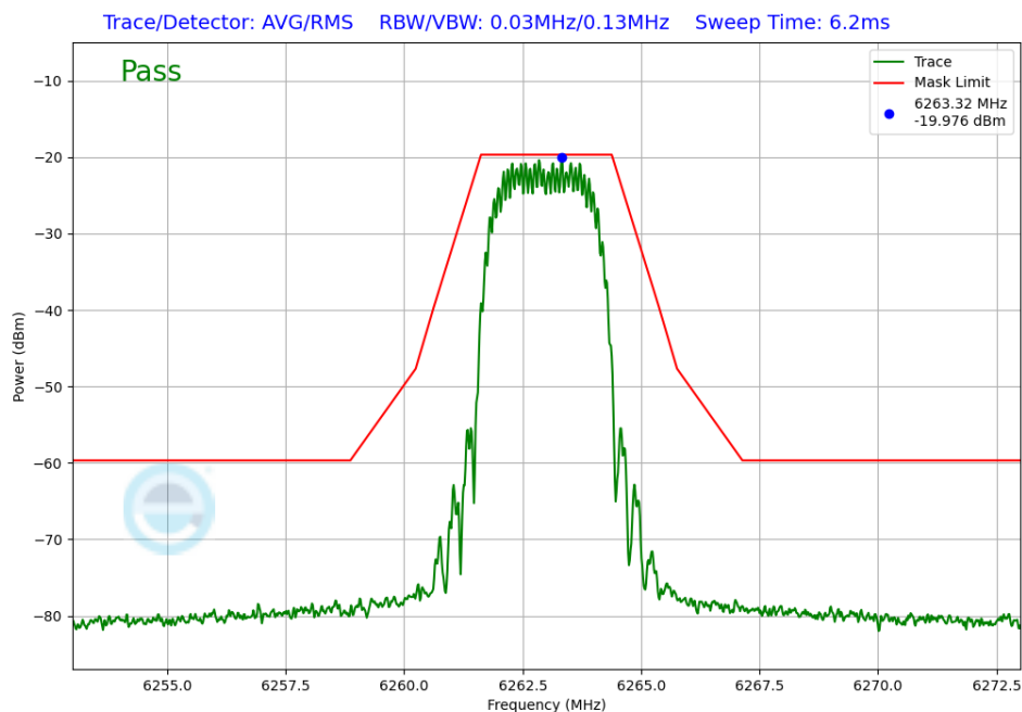
Plot 7-294. In-Band Emission Antenna WF7 (NB UNII HDT2, ePA – 6263MHz)
