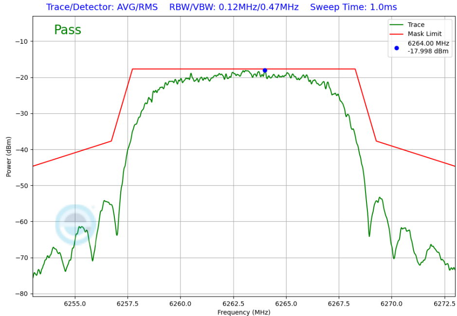
Plot 7-293. In-Band Emission Antenna WF7 (NB UNII HDRPL32, iPA – 6263MHz)
