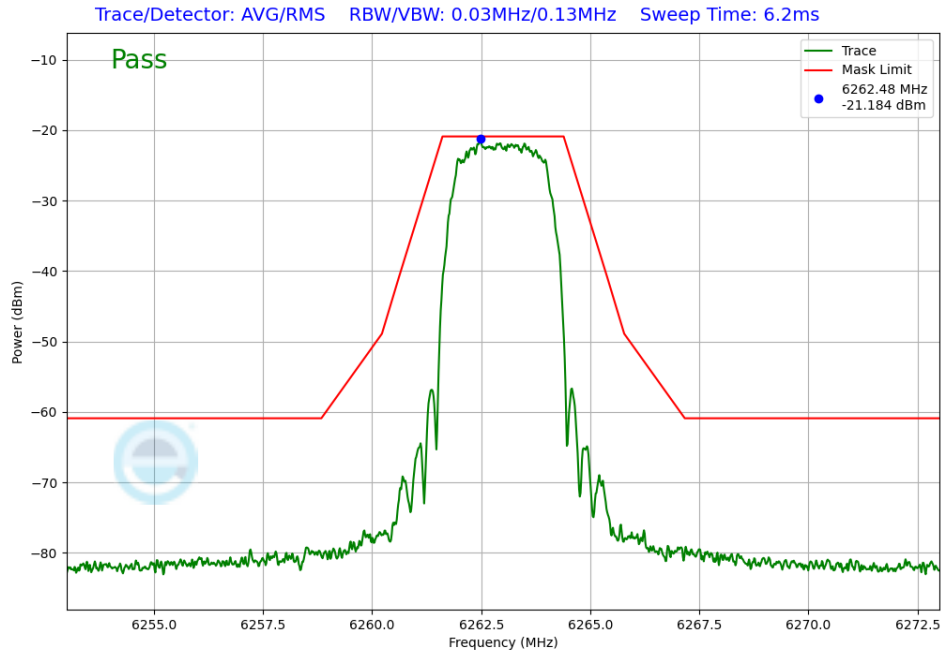
Plot 7-299. In-Band Emission Antenna WF7 (NB UNII HDT6, iPA – 6263MHz)
