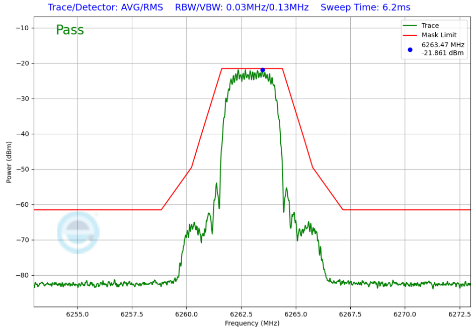
Plot 7-271. In-Band Emission Antenna WF8 (NB UNII HDT4, iPA – 6263MHz)
