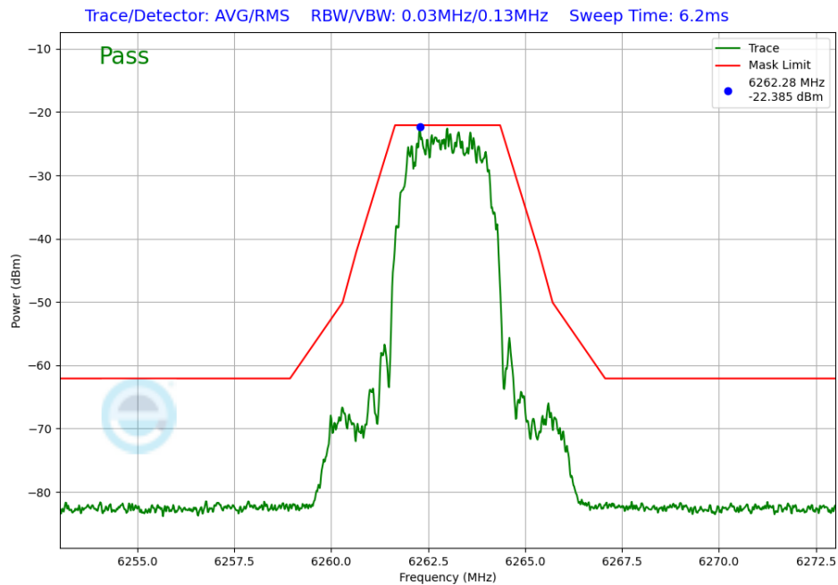
Plot 7-255. In-Band Emission Antenna WF8 (NB UNII HDR4, iPA – 6263MHz)
