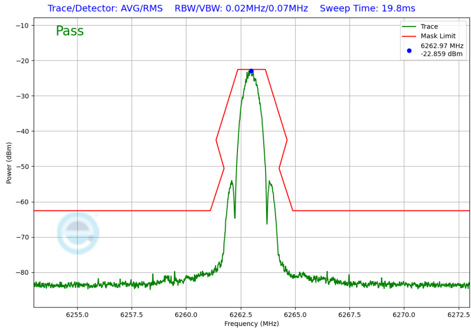
Plot 7-276. In-Band Emission Antenna WF7 (NB UNII LE1M, ePA – 6263MHz)
