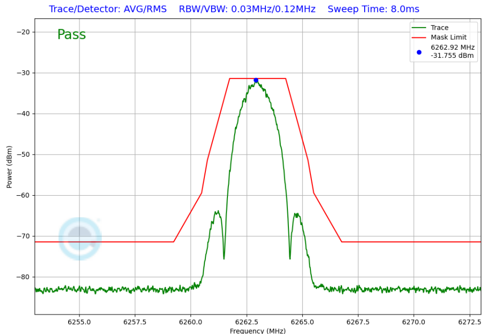
Plot 7-311. In-Band Emission TxBF Primary Antenna WF8 (NB UNII LE2M, iPA – 6263MHz)
