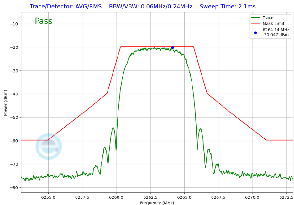
Plot 7-260. In-Band Emission Antenna WF8 (NB UNII XHDRPM6, ePA – 6263MHz)
