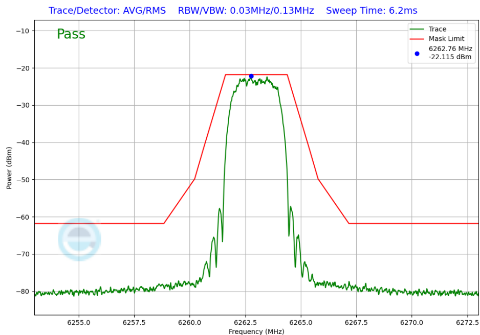
Plot 7-272. In-Band Emission Antenna WF8 (NB UNII HDT6, ePA – 6263MHz)
