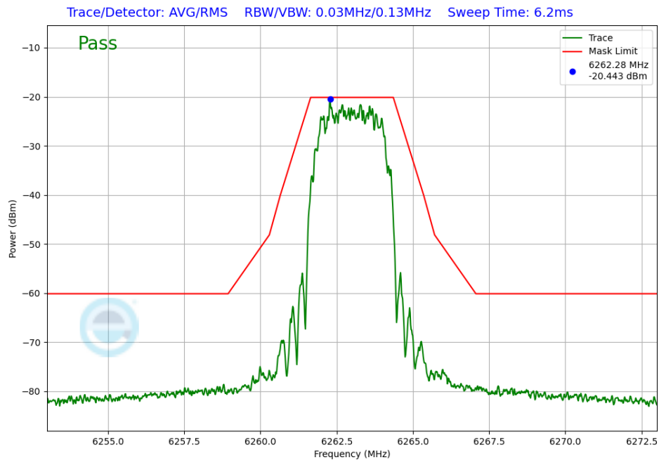
Plot 7-281. In-Band Emission Antenna WF7 (NB UNII HDR4, iPA – 6263MHz)
