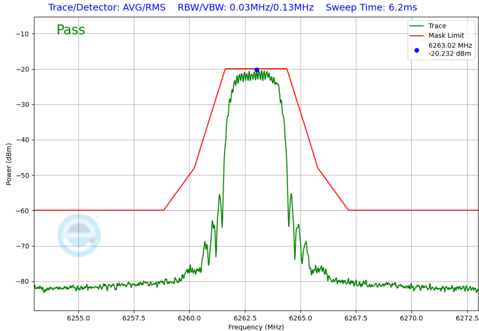
Plot 7-297. In-Band Emission Antenna WF7 (NB UNII HDT4, iPA – 6263MHz)
