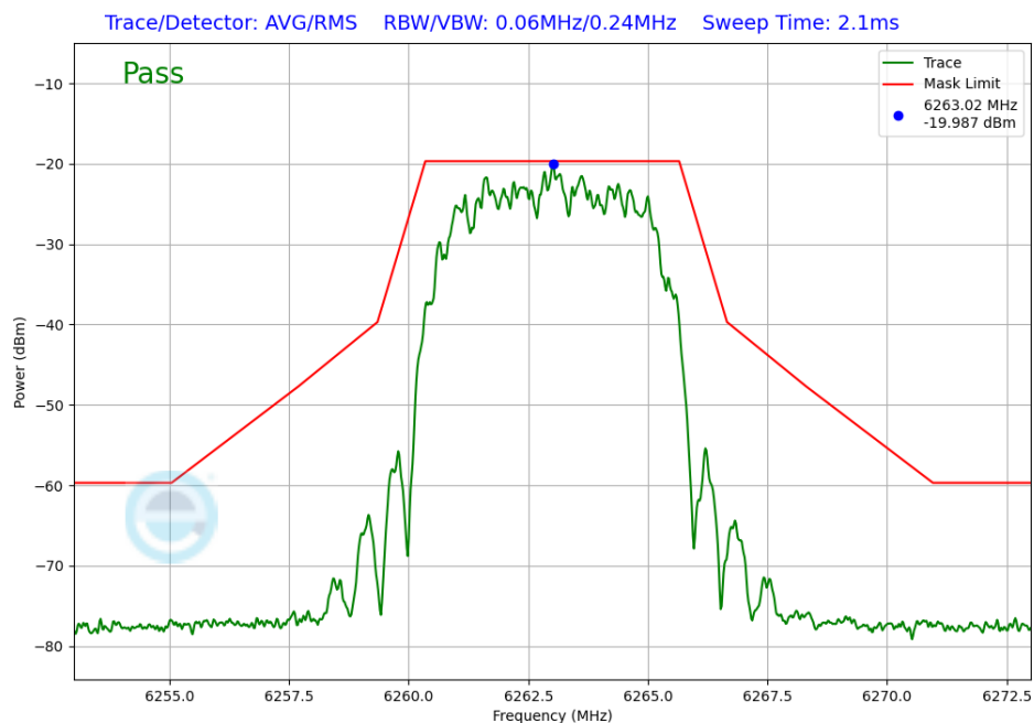
Plot 7-256. In-Band Emission Antenna WF8 (NB UNII HDR8, ePA – 6263MHz)
