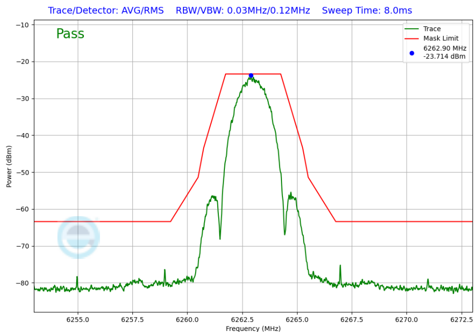
Plot 7-252. In-Band Emission Antenna WF8 (NB UNII LE2M, ePA – 6263MHz)
