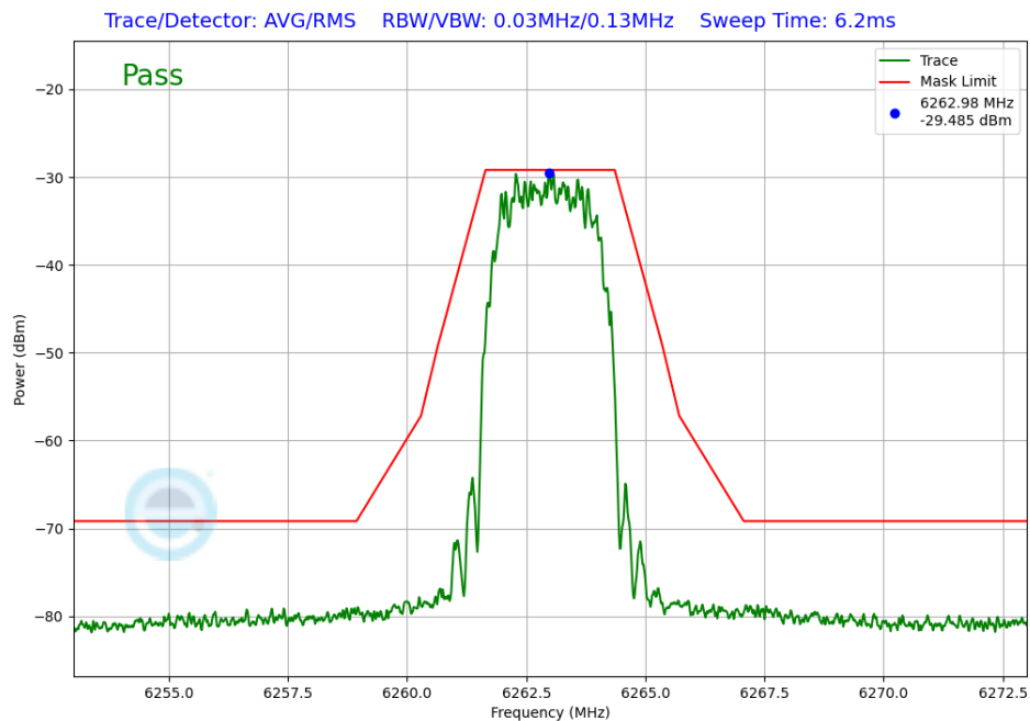
Plot 7-313. In-Band Emission TxBF Primary Antenna WF8 (NB UNII HDR4, ePA – 6263MHz)
