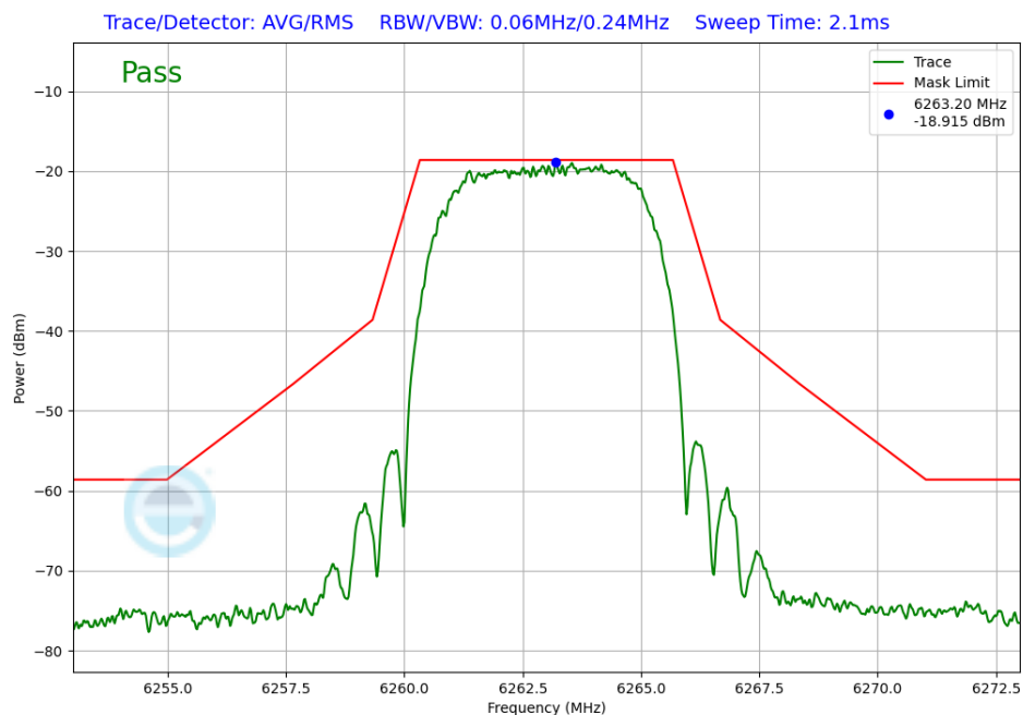
Plot 7-286. In-Band Emission Antenna WF7 (NB UNII XHDRPM6, ePA – 6263MHz)
