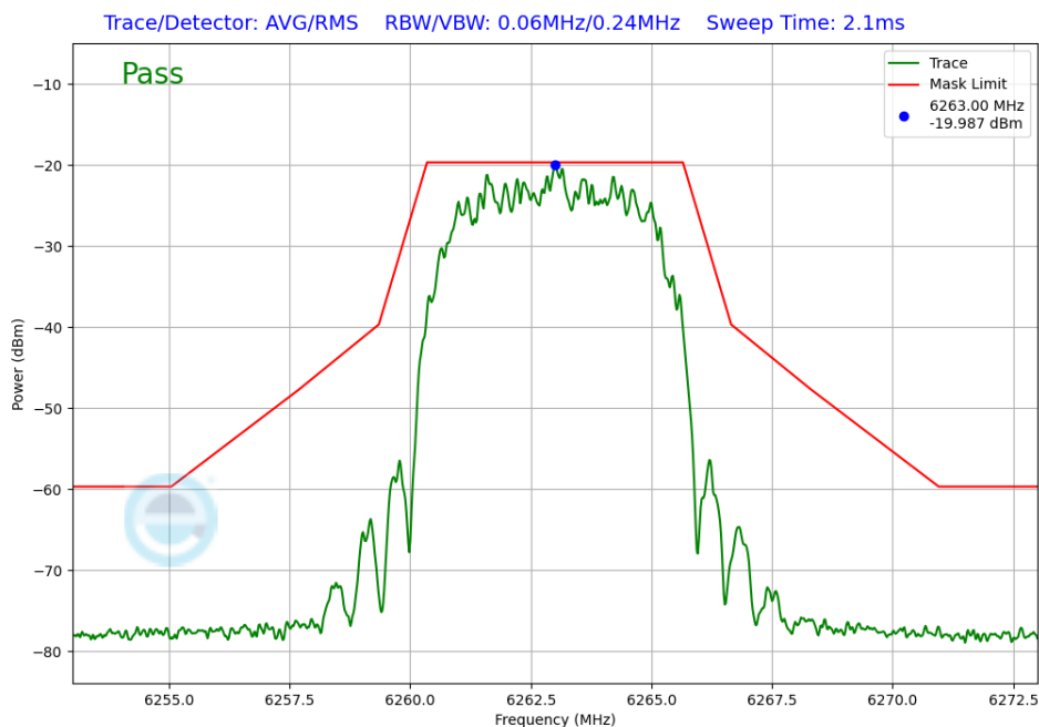
Plot 7-282. In-Band Emission Antenna WF7 (NB UNII HDR8, ePA – 6263MHz)
