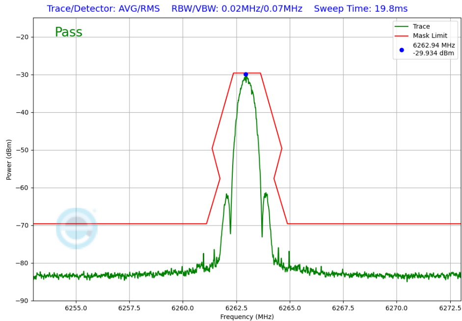
Plot 7-305. In-Band Emission TxBF Primary Antenna WF8 (NB UNII LE1M, ePA – 6263MHz)
