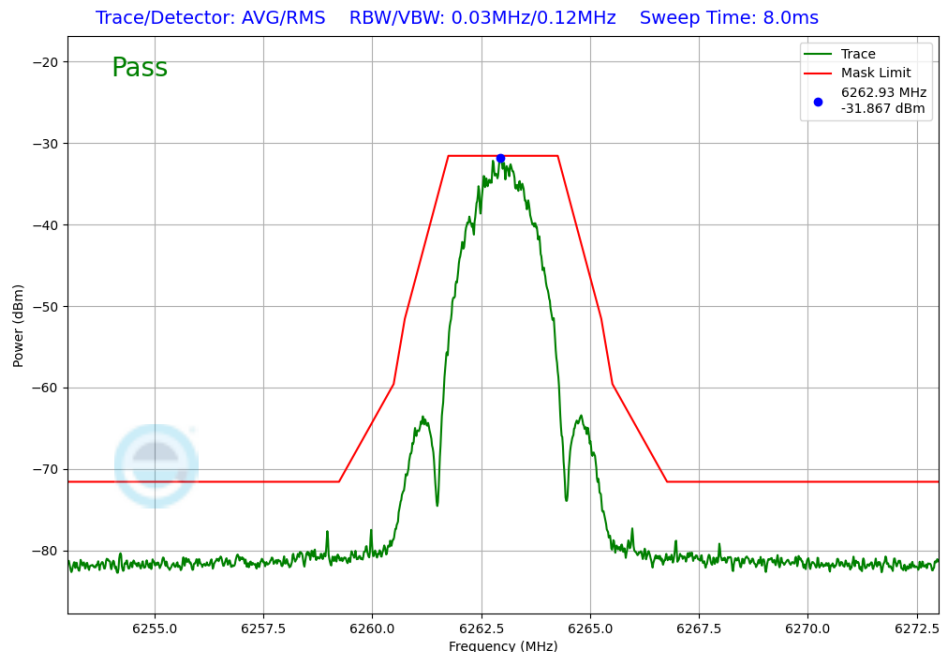
Plot 7-309. In-Band Emission TxBF Primary Antenna WF8 (NB UNII LE2M, ePA – 6263MHz)
