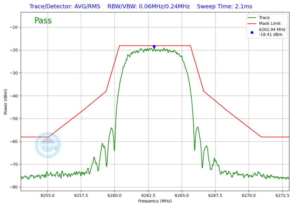
Plot 7-262. In-Band Emission Antenna WF8 (NB UNII HDRPM16, ePA – 6263MHz)
