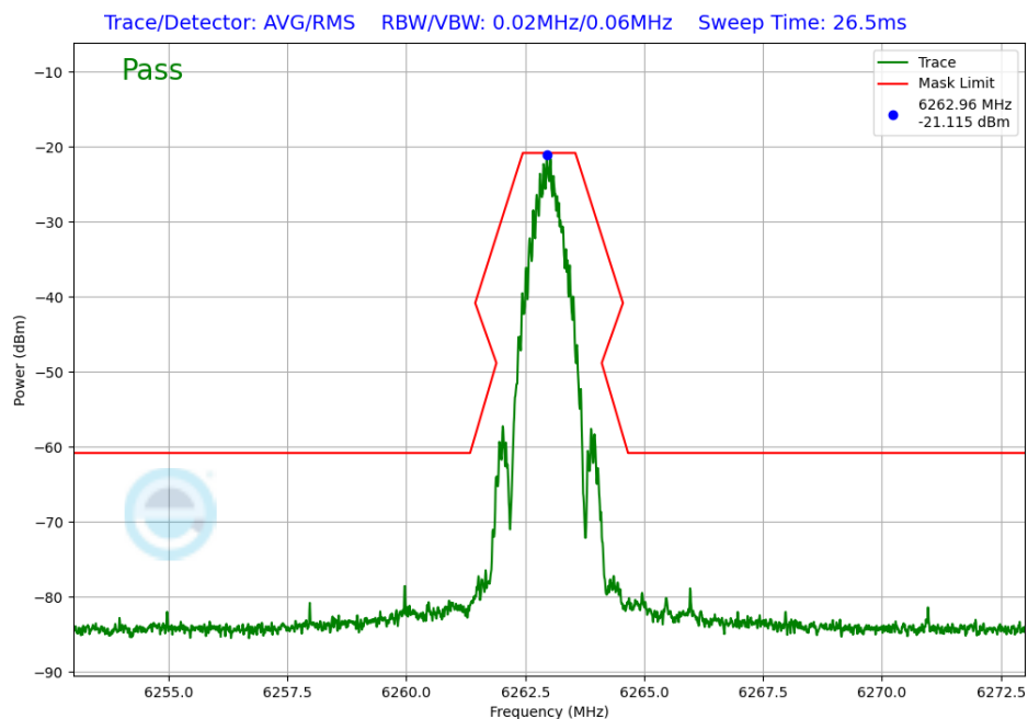
Plot 7-274. In-Band Emission Antenna WF7 (NB UNII BDR, ePA – 6263MHz)
