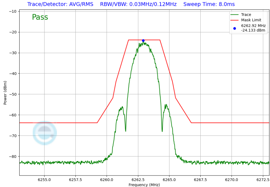
Plot 7-253. In-Band Emission Antenna WF8 (NB UNII LE2M, iPA – 6263MHz)
