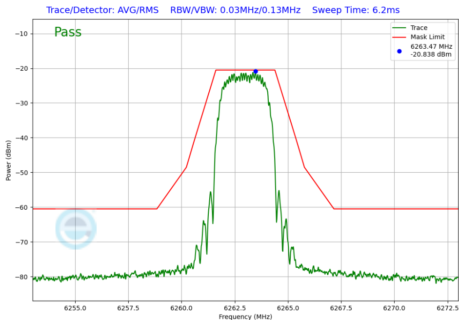
Plot 7-296. In-Band Emission Antenna WF7 (NB UNII HDT4, ePA – 6263MHz)
