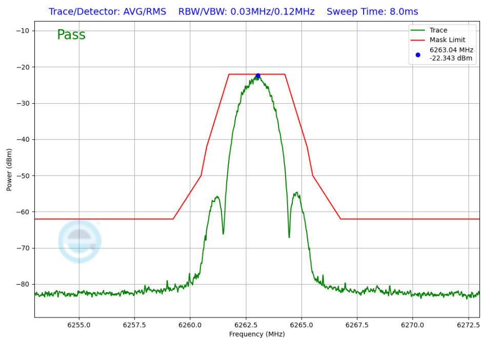
Plot 7-279. In-Band Emission Antenna WF7 (NB UNII LE2M, iPA – 6263MHz)
