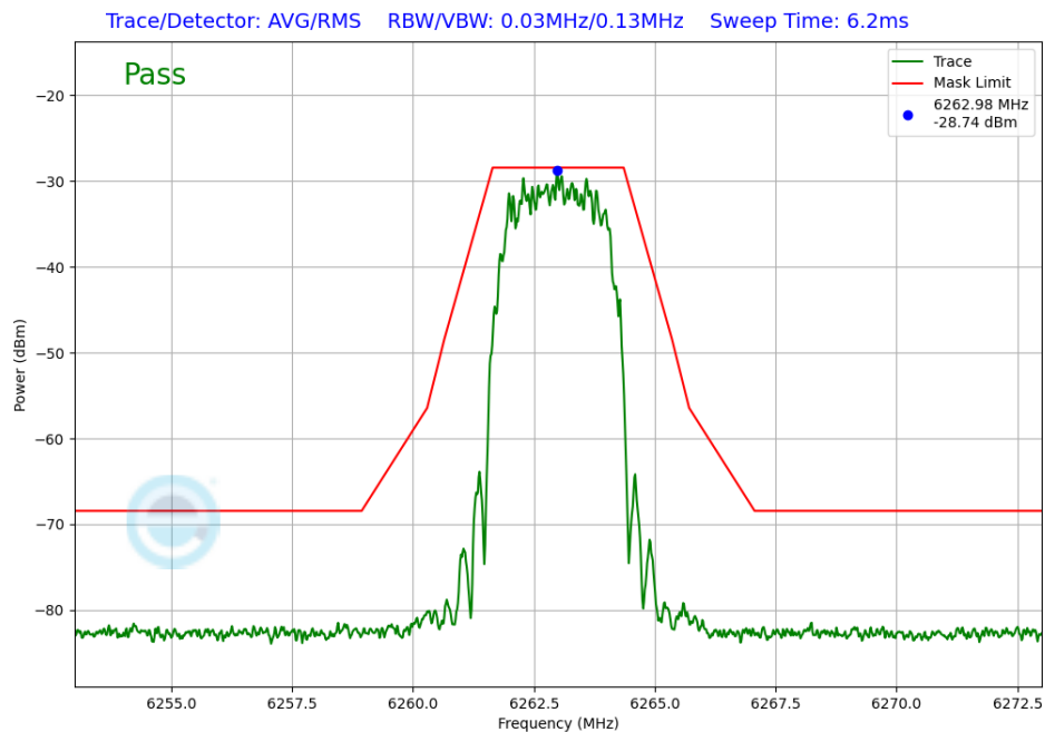
Plot 7-315. In-Band Emission TxBF Primary Antenna WF8 (NB UNII HDR4, iPA – 6263MHz)
