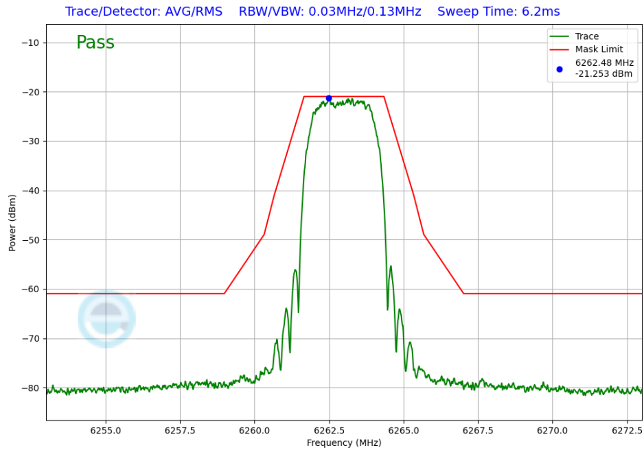
Plot 7-284. In-Band Emission Antenna WF7 (NB UNII HDRPS2, ePA – 6263MHz)
