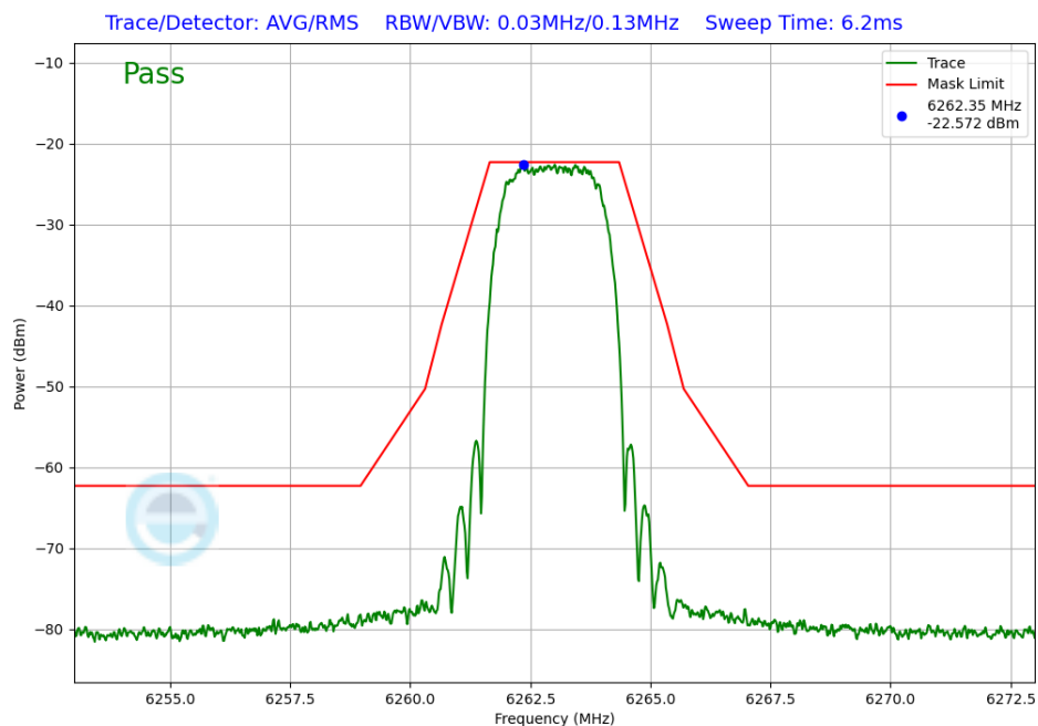
Plot 7-258. In-Band Emission Antenna WF8 (NB UNII HDRPS2, ePA – 6263MHz)
