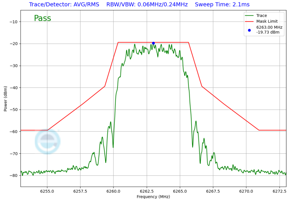
Plot 7-257. In-Band Emission Antenna WF8 (NB UNII HDR8, iPA – 6263MHz)
