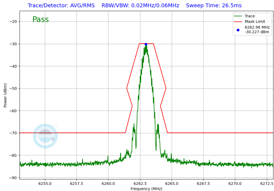
Plot 7-301. In-Band Emission TxBF Primary Antenna WF8 (NB UNII BDR, ePA – 6263MHz)
