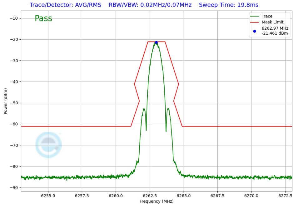
Plot 7-277. In-Band Emission Antenna WF7 (NB UNII LE1M, iPA – 6263MHz)
