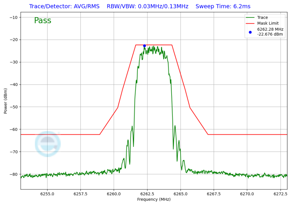
Plot 7-254. In-Band Emission Antenna WF8 (NB UNII HDR4, ePA – 6263MHz)
