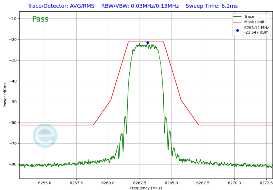
Plot 7-298. In-Band Emission Antenna WF7 (NB UNII HDT6, ePA – 6263MHz)
