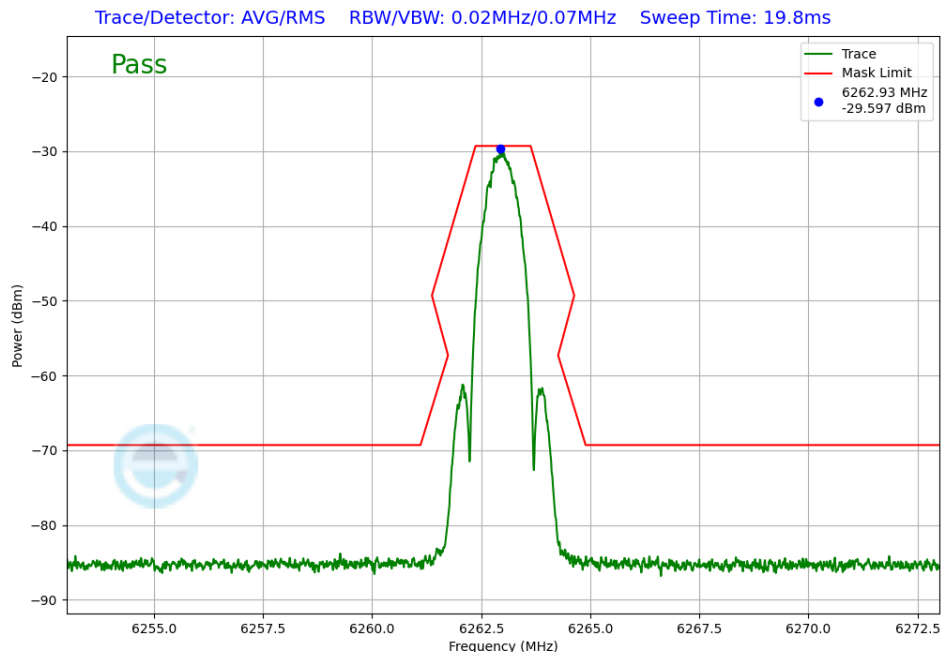
Plot 7-307. In-Band Emission TxBF Primary Antenna WF8 (NB UNII LE1M, iPA – 6263MHz)
