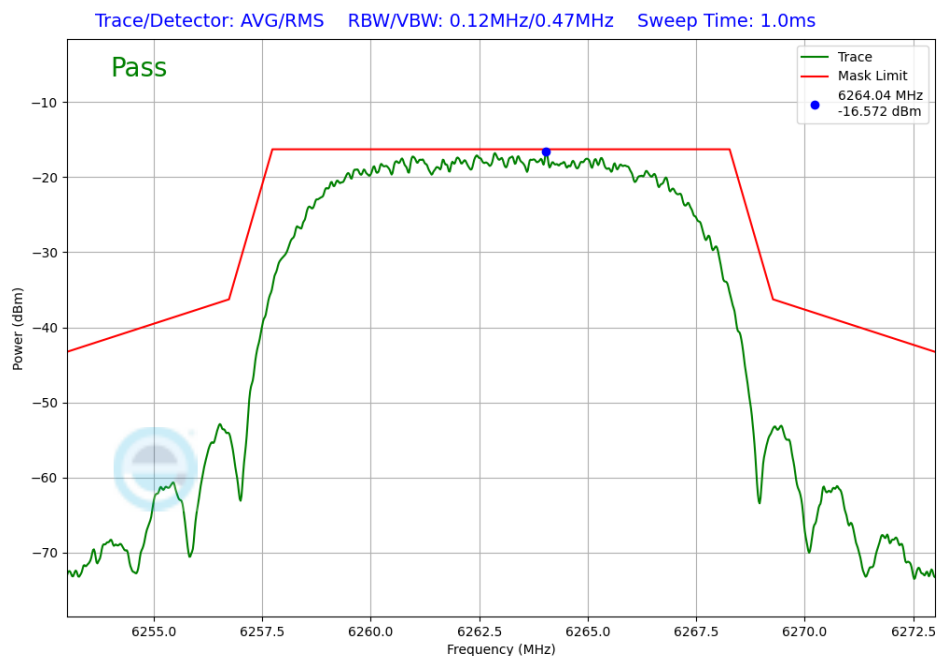
Plot 7-266. In-Band Emission Antenna WF8 (NB UNII HDRPL32, ePA – 6263MHz)
