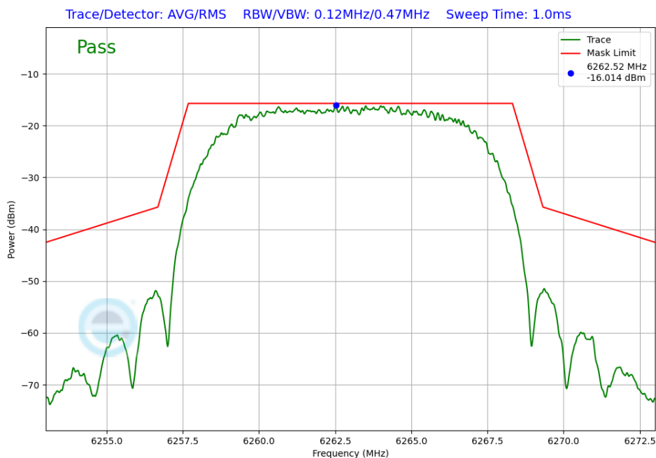
Plot 7-290. In-Band Emission Antenna WF7 (NB UNII HDRPL12, ePA – 6263MHz)
