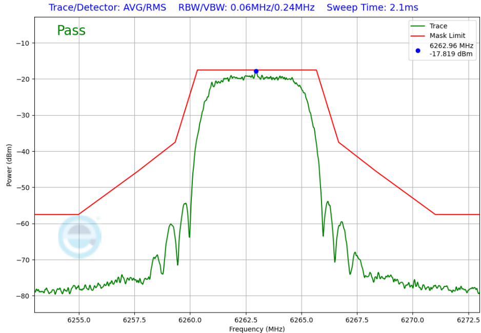
Plot 7-287. In-Band Emission Antenna WF7 (NB UNII XHDRPM6, iPA – 6263MHz)
