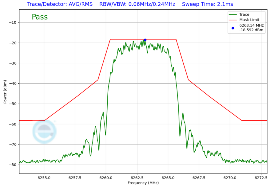
Plot 7-283. In-Band Emission Antenna WF7 (NB UNII HDR8, iPA – 6263MHz)
