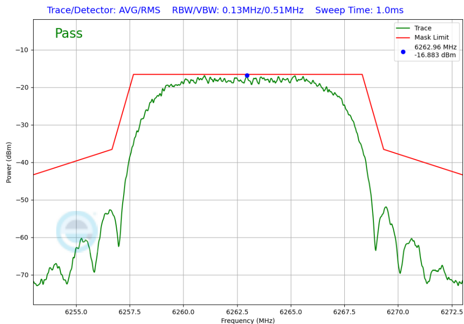
Plot 7-264. In-Band Emission Antenna WF8 (NB UNII HDRPL12, ePA – 6263MHz)
