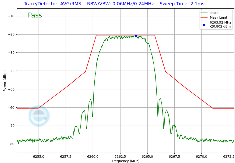
Plot 7-261. In-Band Emission Antenna WF8 (NB UNII XHDRPM6, iPA – 6263MHz)
