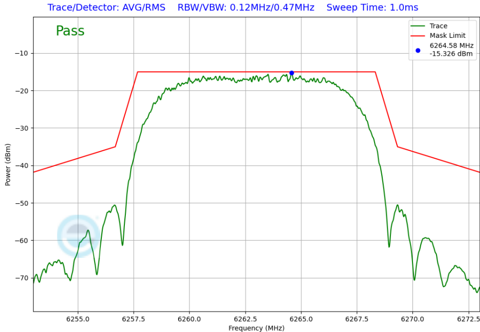
Plot 7-291. In-Band Emission Antenna WF7 (NB UNII HDRPL12, iPA – 6263MHz)
