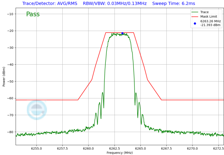
Plot 7-285. In-Band Emission Antenna WF7 (NB UNII HDRPS2, iPA – 6263MHz)
