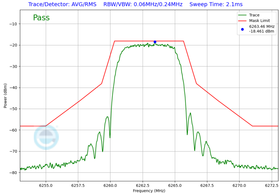
Plot 7-289. In-Band Emission Antenna WF7 (NB UNII HDRPM16, iPA – 6263MHz)
