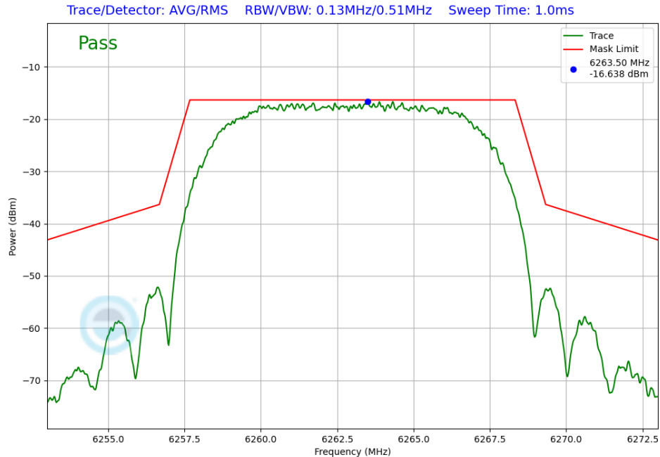
Plot 7-265. In-Band Emission Antenna WF8 (NB UNII HDRPL12, iPA – 6263MHz)
