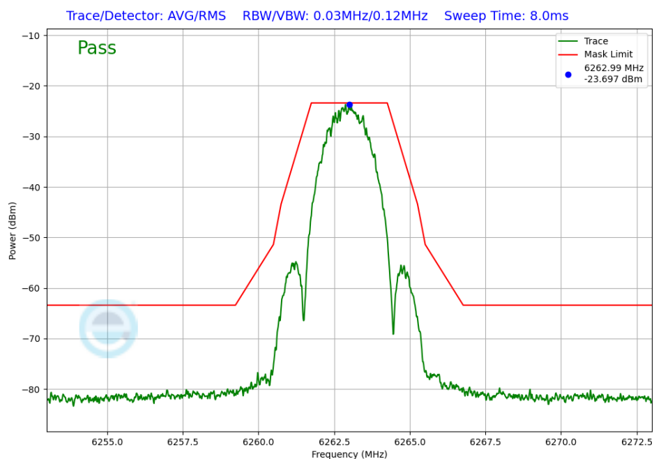
Plot 7-278. In-Band Emission Antenna WF7 (NB UNII LE2M, ePA – 6263MHz)
