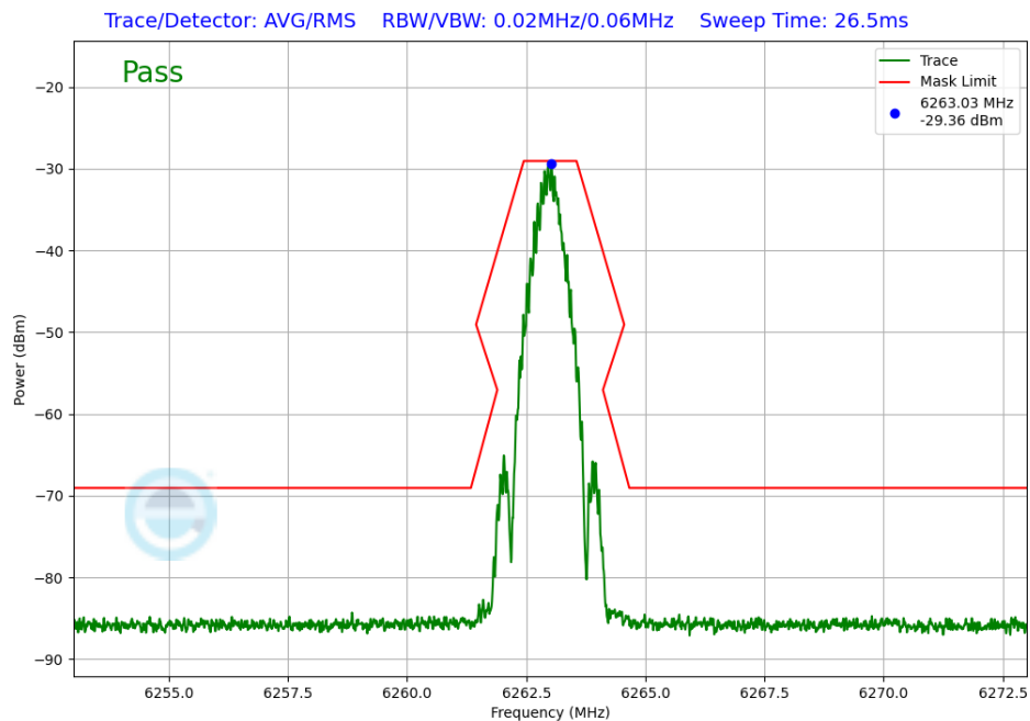
Plot 7-303. In-Band Emission TxBF Primary Antenna WF8 (NB UNII BDR, iPA – 6263MHz)
