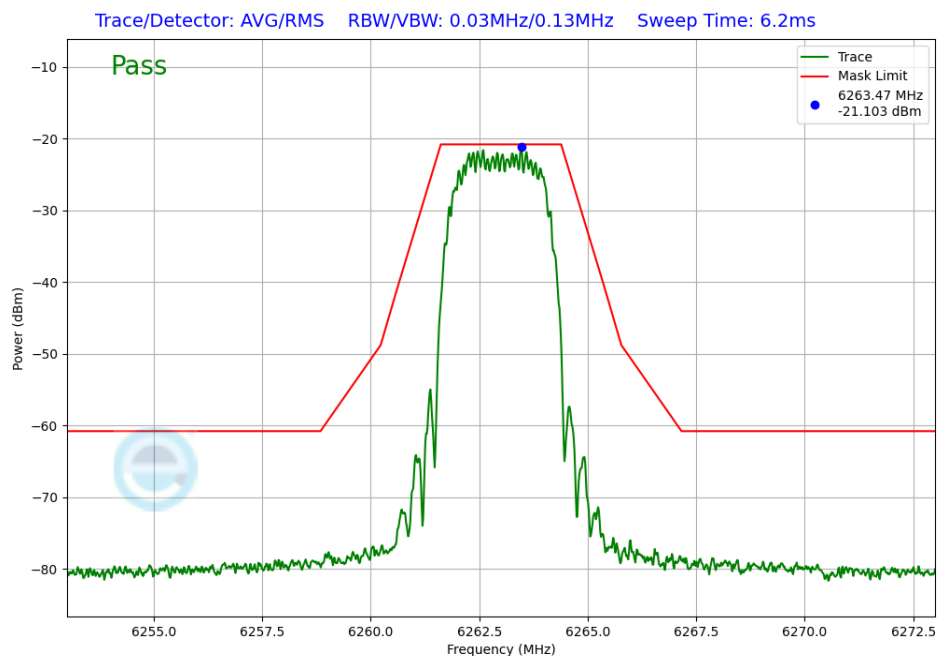
Plot 7-270. In-Band Emission Antenna WF8 (NB UNII HDT4, ePA – 6263MHz)
