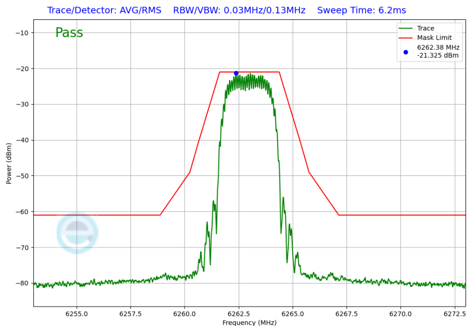
Plot 7-268. In-Band Emission Antenna WF8 (NB UNII HDT2, ePA – 6263MHz)
