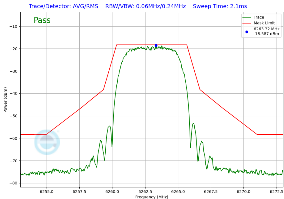
Plot 7-288. In-Band Emission Antenna WF7 (NB UNII HDRPM16, ePA – 6263MHz)
