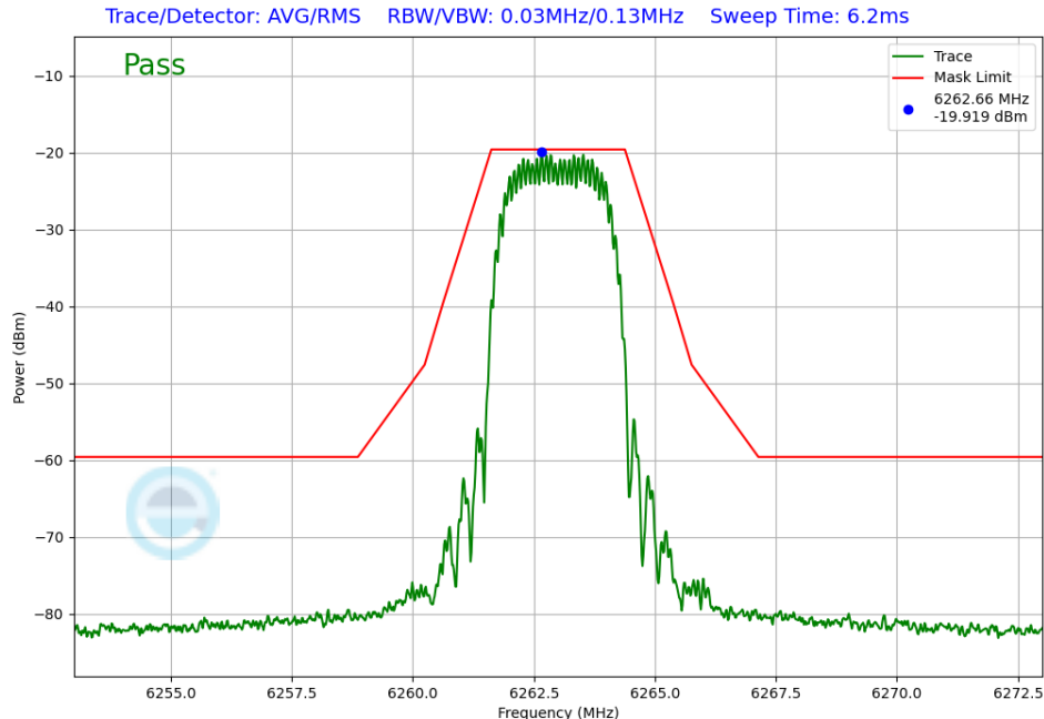
Plot 7-295. In-Band Emission Antenna WF7 (NB UNII HDT2, iPA – 6263MHz)
