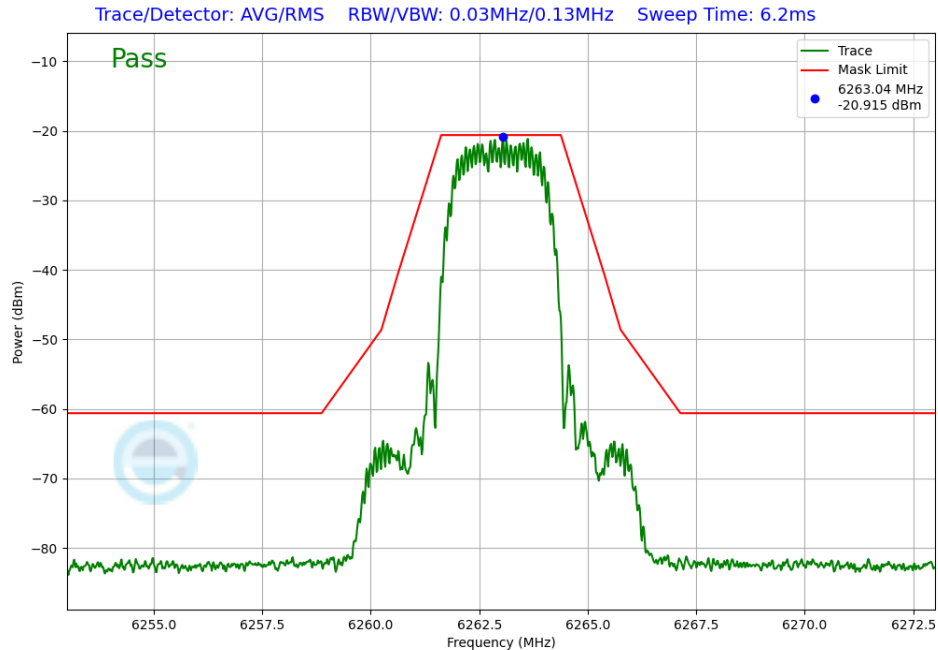
Plot 7-269. In-Band Emission Antenna WF8 (NB UNII HDT2, iPA – 6263MHz)
