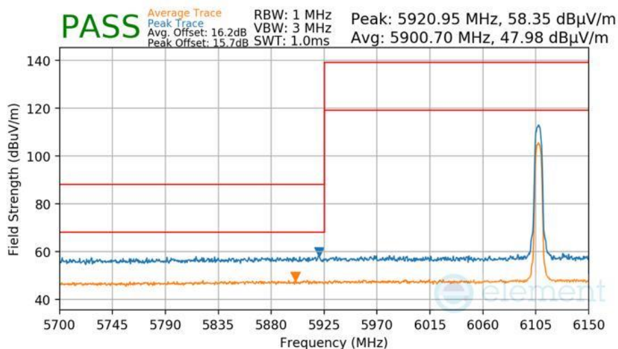
Plot 7-453 Radiated Lower Band Edge Measurement Antenna WF8
