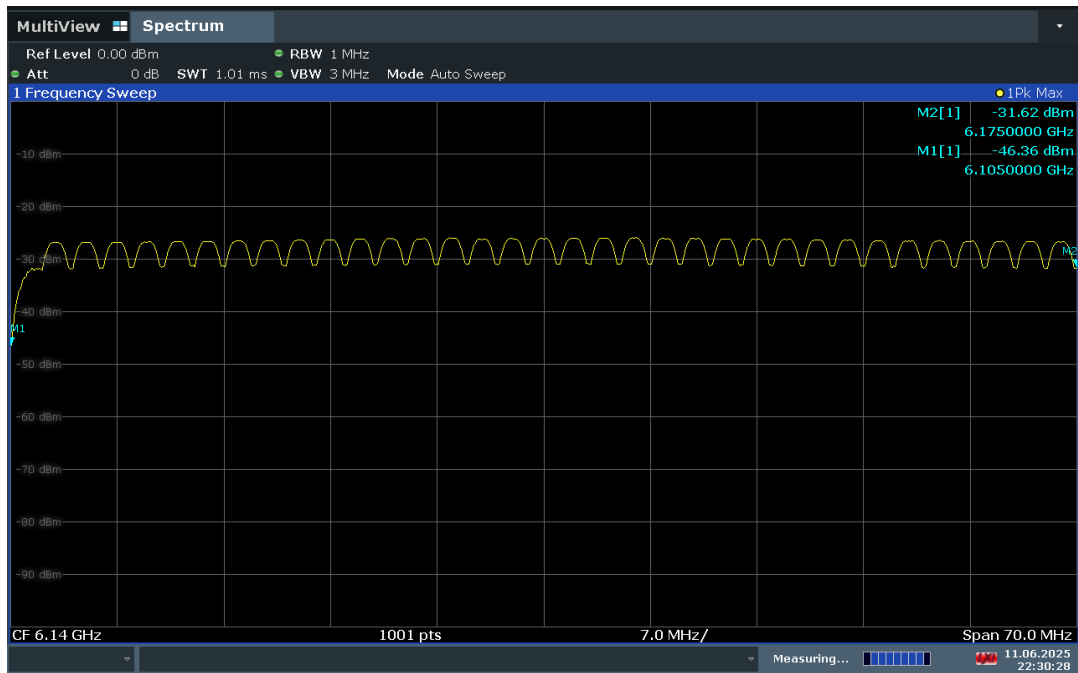
Plot 7-406. Before AWGN Signal Injected
