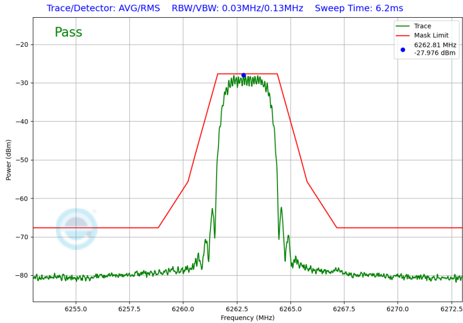
Plot 7-396. In-Band Emission TxBF Diversity Antenna WF8 (NB UNII HDT4, ePA – 6263MHz)
