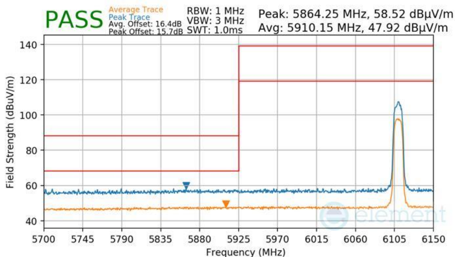
Plot 7-466 Radiated Lower Band Edge Measurement Antenna WF7
