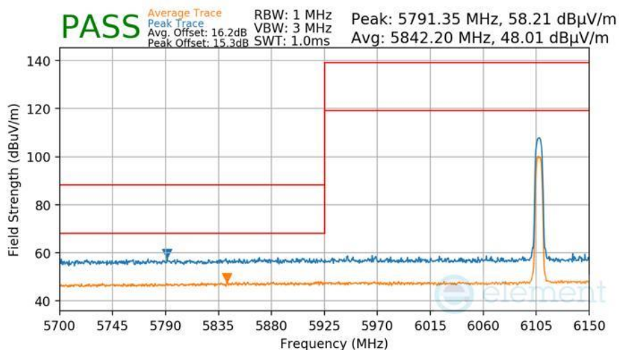
Plot 7-464 Radiated Lower Band Edge Measurement Antenna WF7
