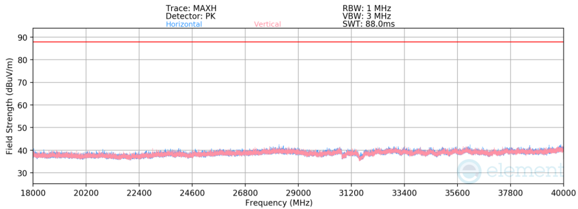
Plot 7-417. Radiated Spurious Emissions Above 18GHz TxBF Primary (HDR4 ePA – 6263MHz)
