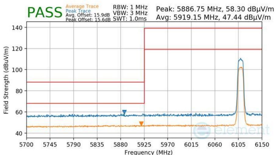
Plot 7-454 Radiated Lower Band Edge Measurement Antenna WF8
