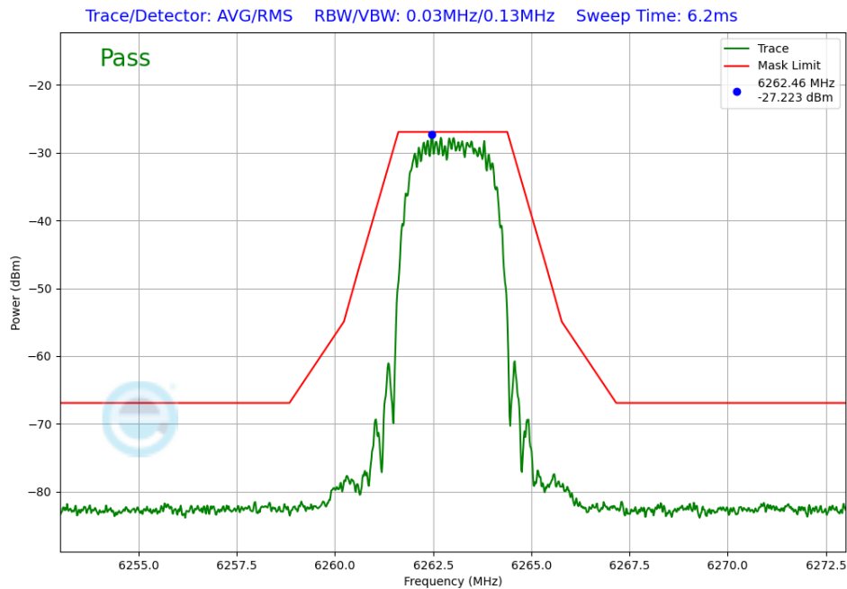
Plot 7-399. In-Band Emission TxBF Diversity Antenna WF7 (NB UNII HDT4, iPA – 6263MHz)
