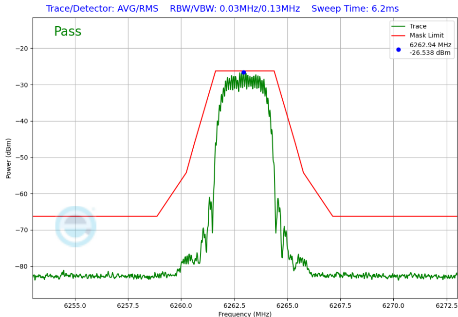
Plot 7-395. In-Band Emission TxBF Diversity Antenna WF7 (NB UNII HDT2, iPA – 6263MHz)
