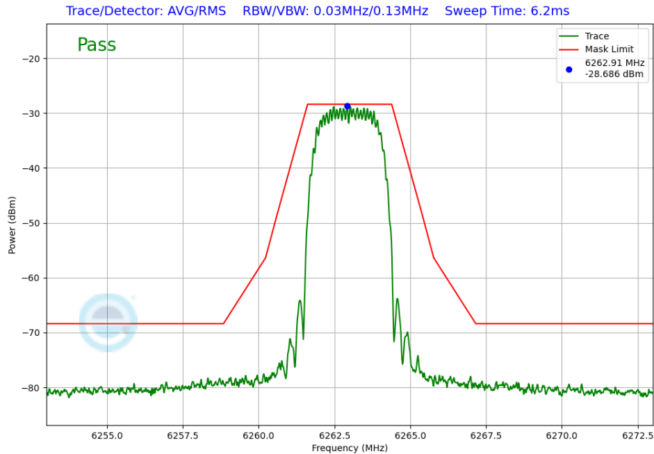
Plot 7-397. In-Band Emission TxBF Diversity Antenna WF7 (NB UNII HDT4, ePA – 6263MHz)
