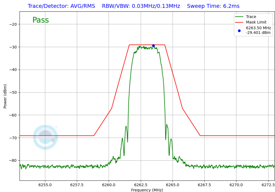
Plot 7-402. In-Band Emission TxBF Diversity Antenna WF8 (NB UNII HDT6, iPA – 6263MHz)
