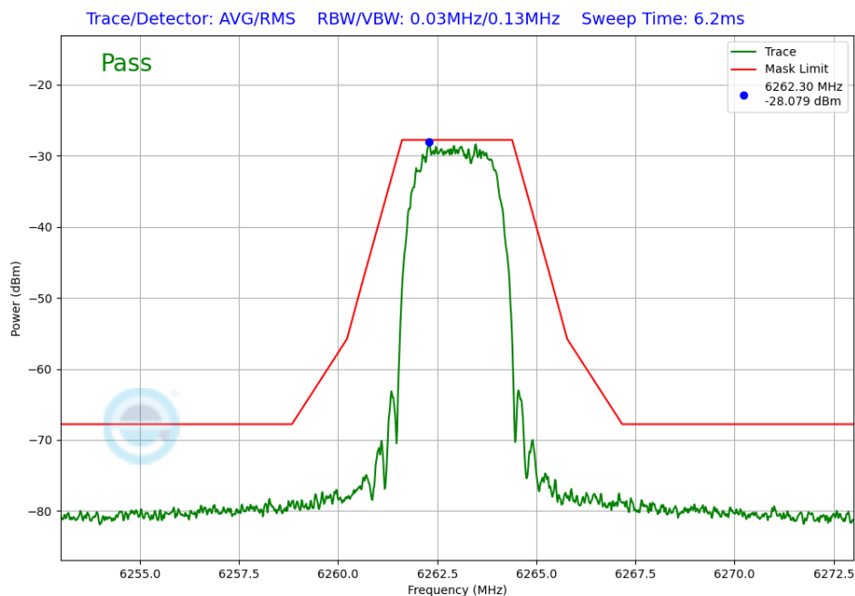
Plot 7-400. In-Band Emission TxBF Diversity Antenna WF8 (NB UNII HDT6, ePA – 6263MHz)
