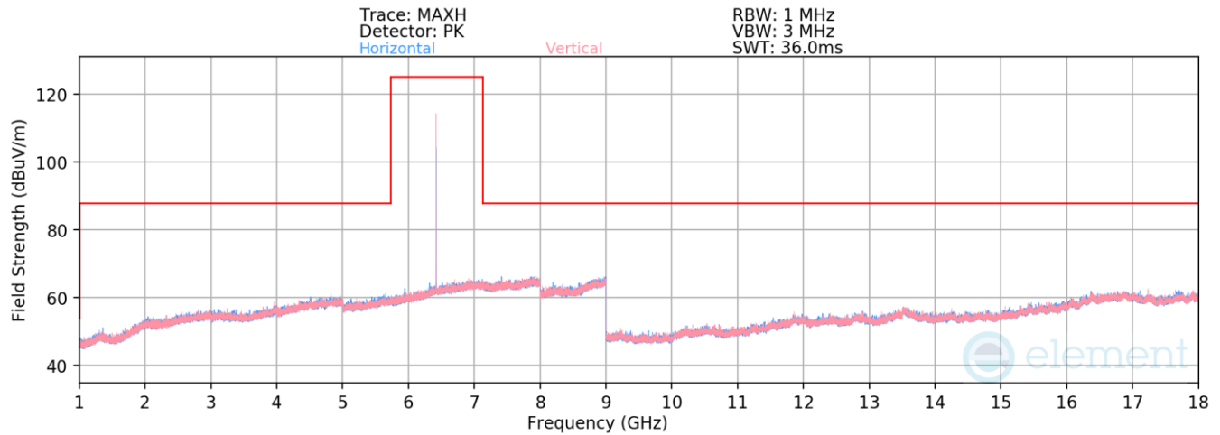
Plot 7-426. Radiated Spurious Emissions 1-18GHz TxBF Diversity (BDR GFSK ePA – 6420MHz)
