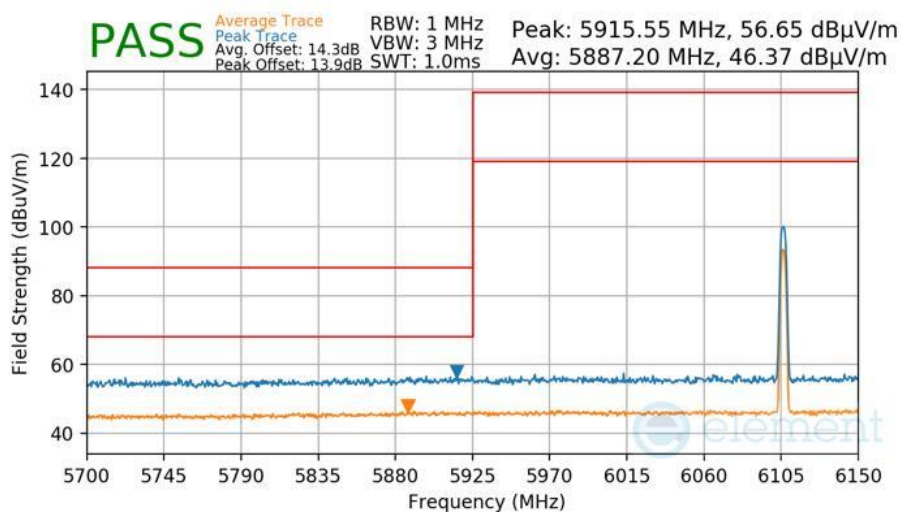
Plot 7-467 Radiated Lower Band Edge Measurement Antenna WF7
