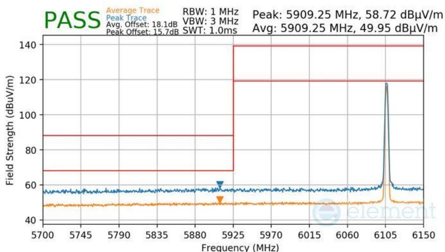
Plot 7-448 Radiated Lower Band Edge Measurement Antenna WF8
