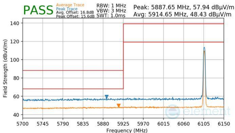
Plot 7-449 Radiated Lower Band Edge Measurement Antenna WF8
