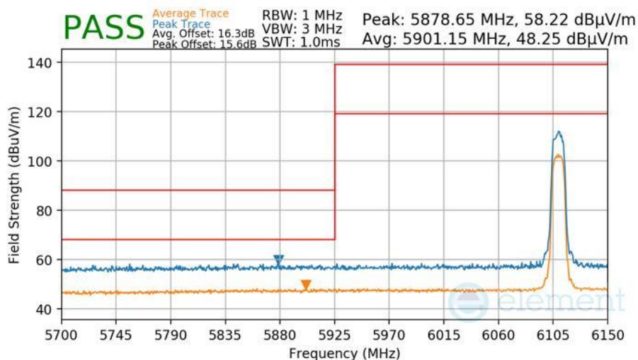
Plot 7-455 Radiated Lower Band Edge Measurement Antenna WF8
