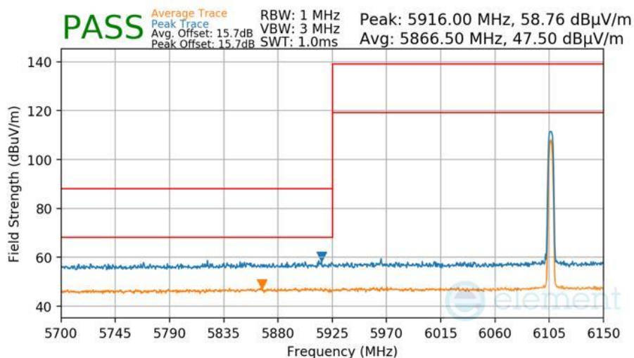
Plot 7-451 Radiated Lower Band Edge Measurement Antenna WF8
