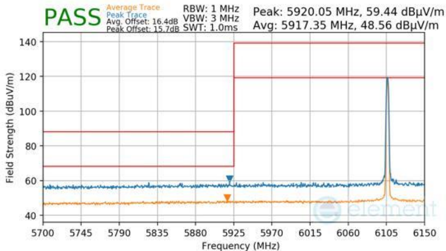
Plot 7-480 Radiated Lower Band Edge Measurement TxBF Diversity
