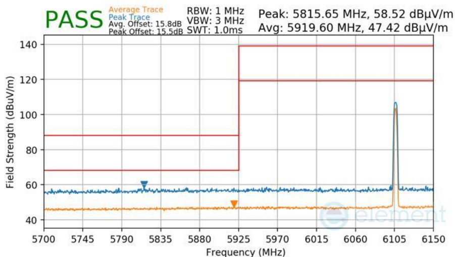
Plot 7-462 Radiated Lower Band Edge Measurement Antenna WF7
