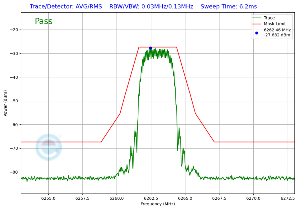
Plot 7-394. In-Band Emission TxBF Diversity Antenna WF8 (NB UNII HDT2, iPA – 6263MHz)
