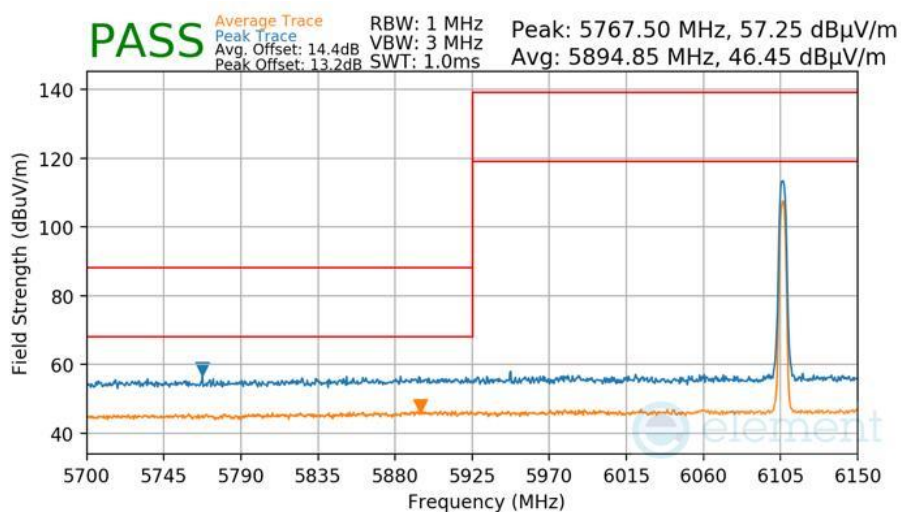
Plot 7-456 Radiated Lower Band Edge Measurement Antenna WF8
