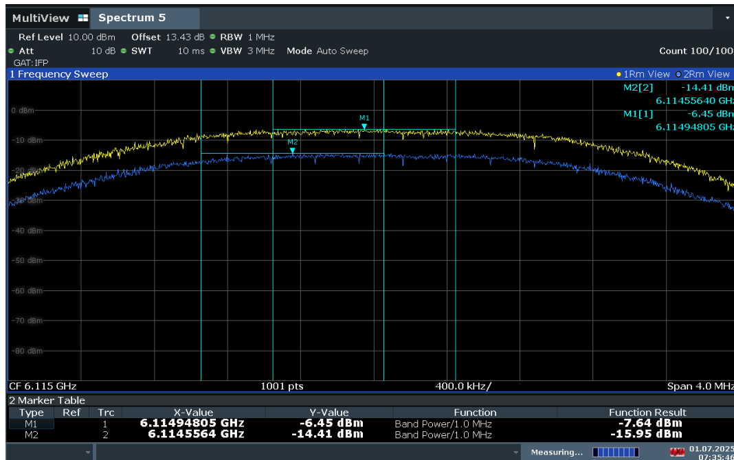
Plot 7-408. Power Density Plot 6115MHz Antenna WF5B
