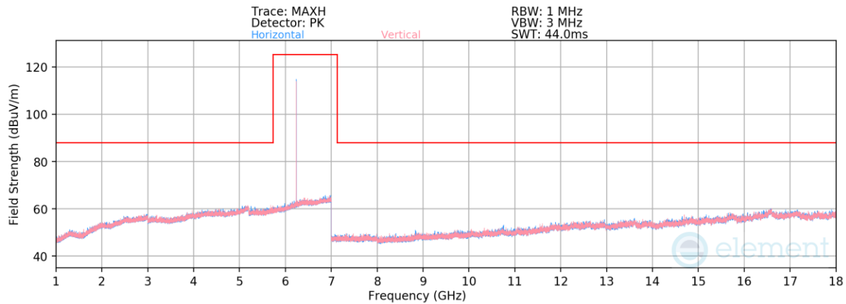
Plot 7-416. Radiated Spurious Emissions 1-18GHz TxBF Primary (HDR4 GFSK ePA – 6263MHz)
