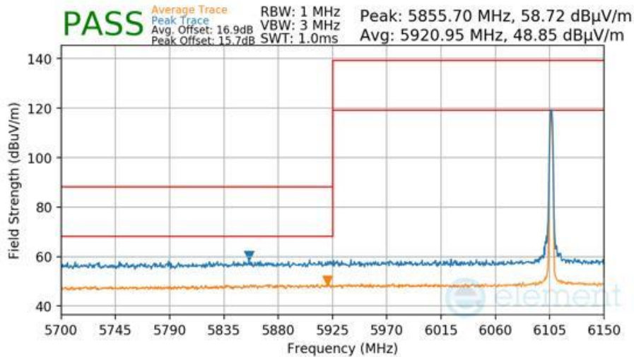
Plot 7-479 Radiated Lower Band Edge Measurement TxBF Diversity
