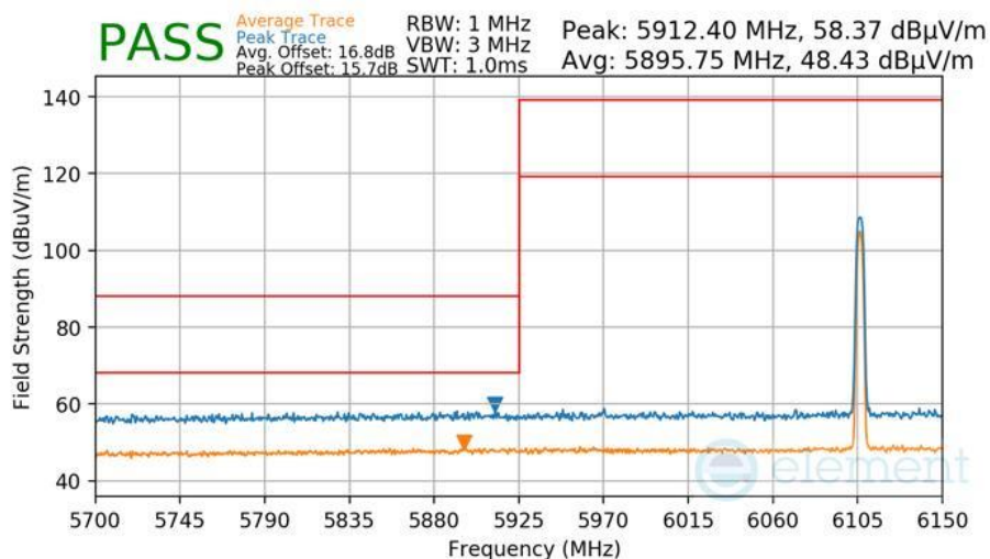
Plot 7-460 Radiated Lower Band Edge Measurement Antenna WF7
