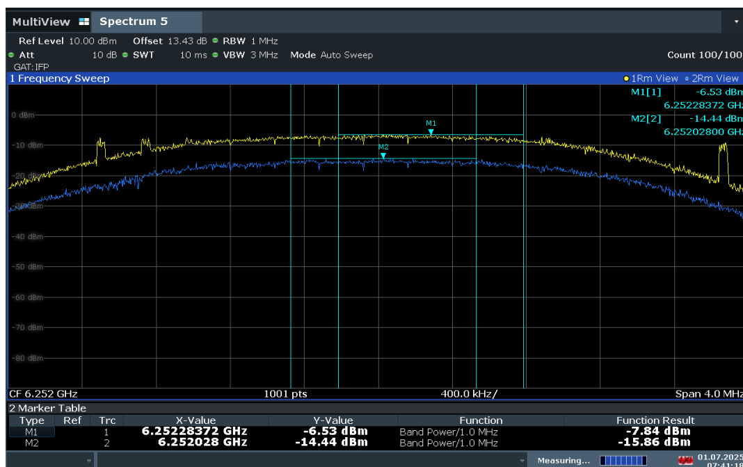
Plot 7-409. Power Density Plot – 6252MHz Antenna WF5B
