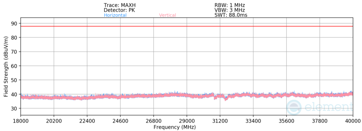
Plot 7-425. Radiated Spurious Emissions Above 18GHz TxBF Diversity (BDR GFSK ePA – 6263MHz)
