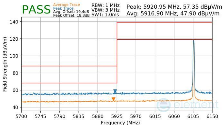
Plot 7-435 Radiated Lower Band Edge Measurement Antenna WF5B
