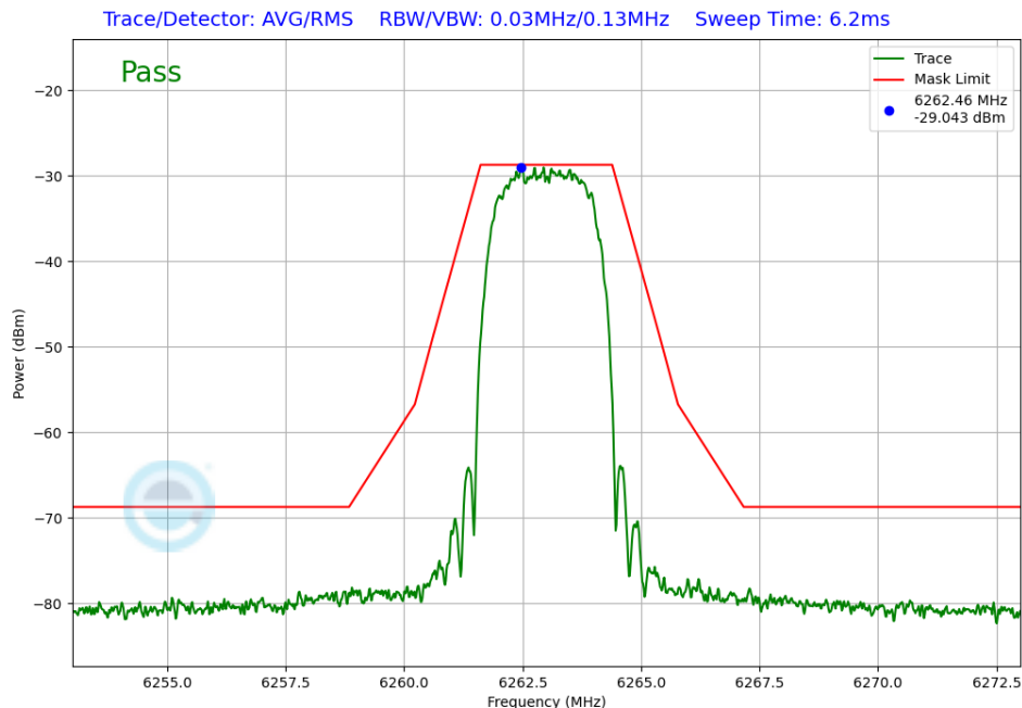
Plot 7-401. In-Band Emission TxBF Diversity Antenna WF7 (NB UNII HDT6, ePA – 6263MHz)
