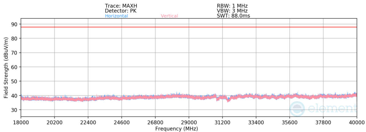
Plot 7-413. Radiated Spurious Emissions Above 18GHz TxBF Primary (BDR GFSK ePA – 6263MHz)
