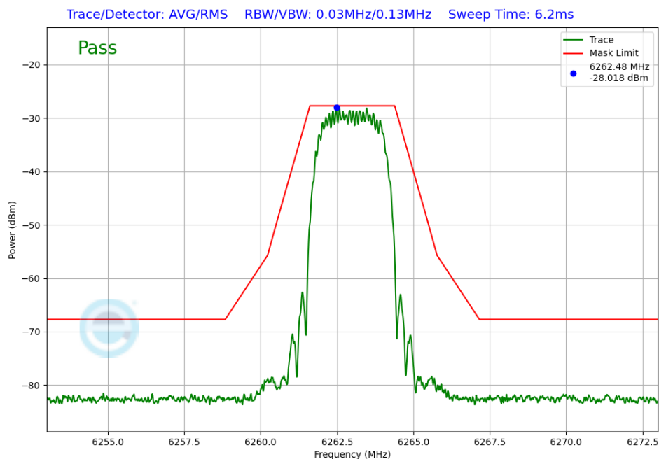
Plot 7-398. In-Band Emission TxBF Diversity Antenna WF8 (NB UNII HDT4, iPA – 6263MHz)
