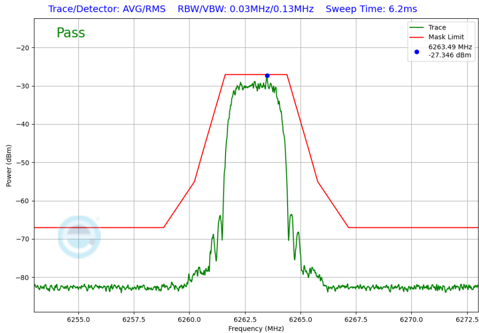
Plot 7-403. In-Band Emission TxBF Diversity Antenna WF7 (NB UNII HDT6, iPA – 6263MHz)
