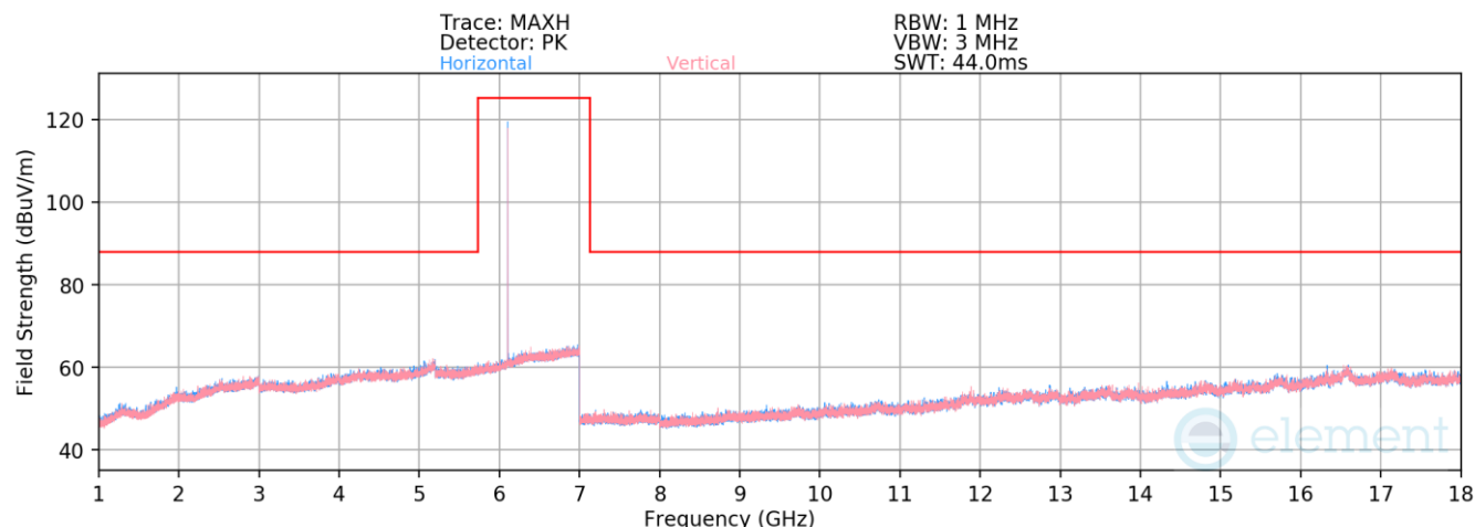
Plot 7-419. Radiated Spurious Emissions 1-18GHz TxBF Primary (LE1M ePA – 6106MHz)
