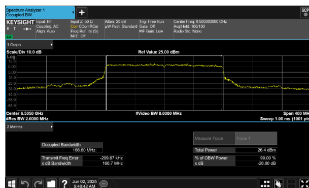
Plot 7-76 26dB BW & 99% OBW Antenna WF7 (160MHz BW 802.11be(SU) - Ch.111)
