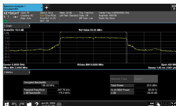
Plot 7-84 26dB BW & 99% OBW Antenna WF7 (160MHz BW 802.11be(SU) - Ch.207)
