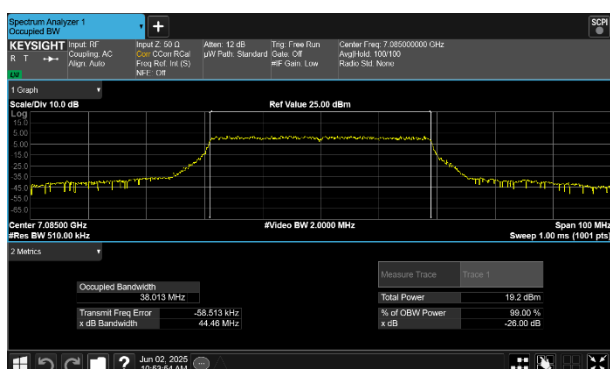
Plot 7-82 26dB BW & 99% OBW Antenna WF7 (40MHz BW 802.11be(SU) - Ch.227)
