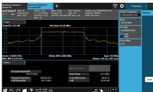
Plot 7-2 26dB BW & 99% OBW Antenna WF5B (40MHz BW 802.11be(SU) - Ch.3)
