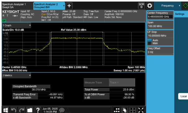
Plot 7-6 26dB BW & 99% OBW Antenna WF5B (40MHz BW 802.11be(SU) - Ch.107)
