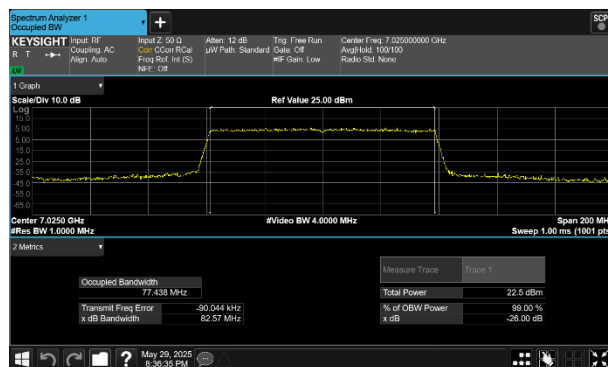
Plot 7-27 26dB BW & 99% OBW Antenna WF5B (80MHz BW 802.11be(SU) - Ch.215)
