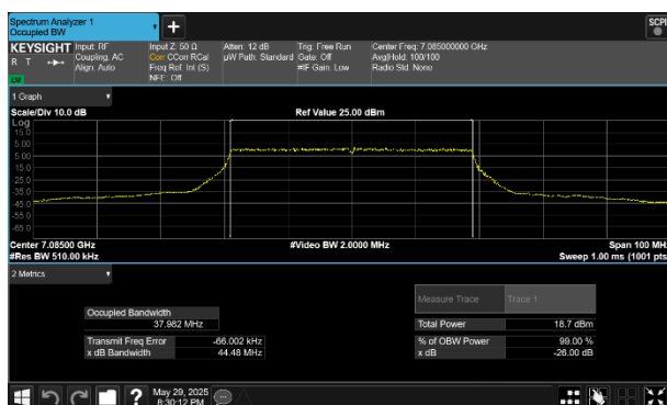
Plot 7-26 26dB BW & 99% OBW Antenna WF5B (40MHz BW 802.11be(SU) - Ch.227)
