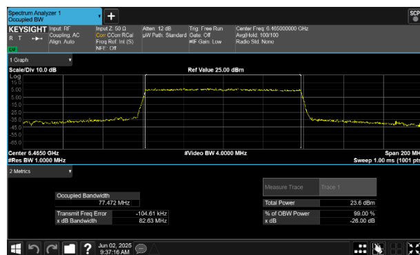
Plot 7-75 26dB BW & 99% OBW Antenna WF7 (80MHz BW 802.11be(SU) - Ch.103)
