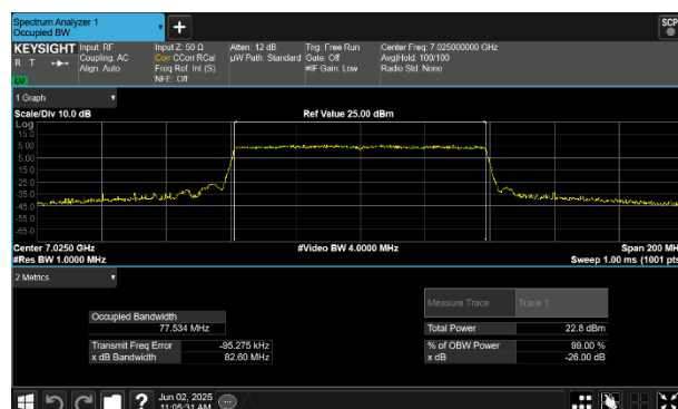
Plot 7-83 26dB BW & 99% OBW Antenna WF7 (80MHz BW 802.11be(SU) - Ch.215)
