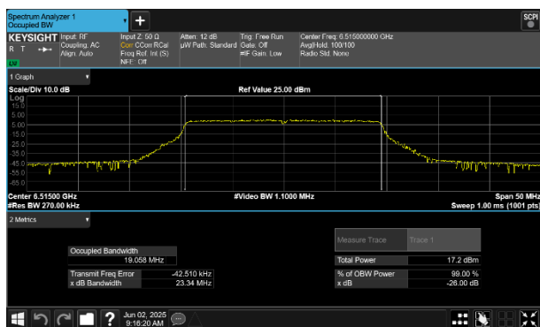
Plot 7-73 26dB BW & 99% OBW Antenna WF7 (20MHz BW 802.11be(SU) - Ch.113)
