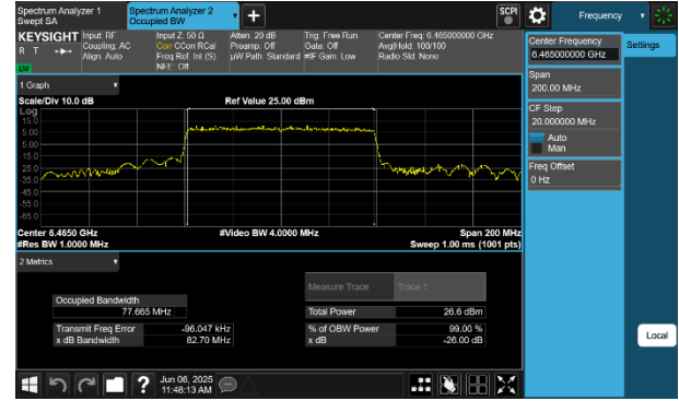
Plot 7-63 26dB BW & 99% OBW Antenna WF7 (80MHz BW 802.11be(SU) - Ch.103)
