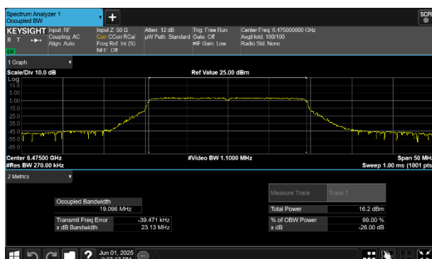
Plot 7-45 26dB BW & 99% OBW Antenna WF8 (20MHz BW 802.11be(SU) - Ch.105)
