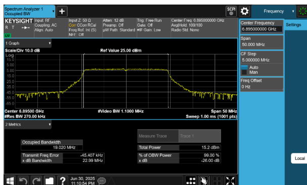
Plot 7-25 26dB BW & 99% OBW Antenna WF5B (20MHz BW 802.11be(SU) - Ch.189)
