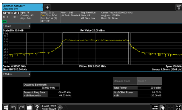
Plot 7-74 26dB BW & 99% OBW Antenna WF7 (40MHz BW 802.11be(SU) - Ch.115)
