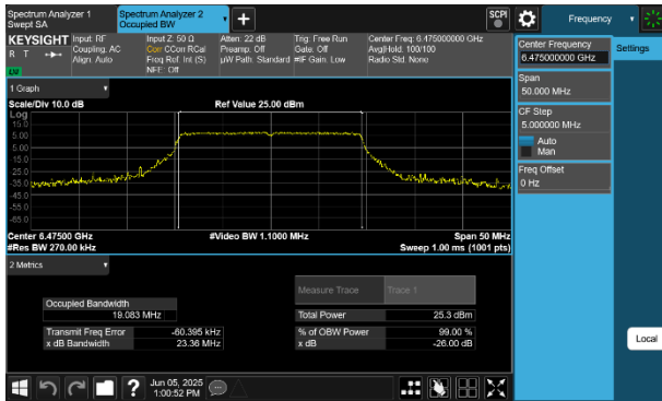
Plot 7-5 26dB BW & 99% OBW Antenna WF5B (20MHz BW 802.11be(SU) - Ch.105)
