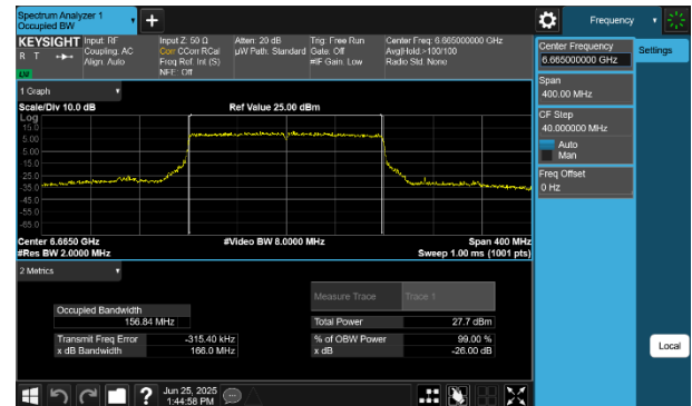
Plot 7-40 26dB BW & 99% OBW Antenna WF8 (160MHz BW 802.11be(SU) - Ch.143)
