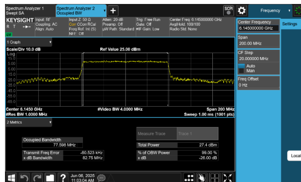
Plot 7-59 26dB BW & 99% OBW Antenna WF7 (80MHz BW 802.11be(SU) - Ch.39)
