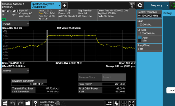
Plot 7-62 26dB BW & 99% OBW Antenna WF7 (40MHz BW 802.11be(SU) - Ch.99)
