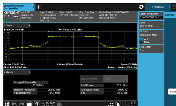
Plot 7-60 26dB BW & 99% OBW Antenna WF7 (160MHz BW 802.11be(SU) - Ch.79)
