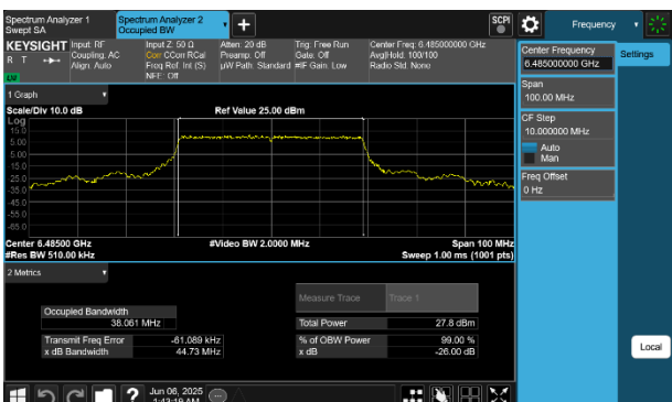
Plot 7-34 26dB BW & 99% OBW Antenna WF8 (40MHz BW 802.11be(SU) - Ch.107)
