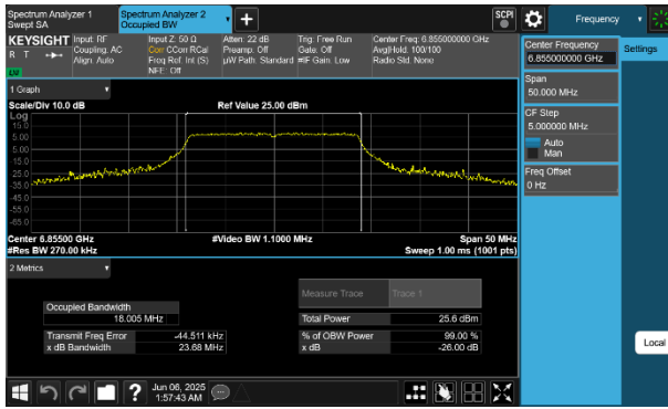
Plot 7-37 26dB BW & 99% OBW Antenna WF8 (20MHz BW 802.11a - Ch.181)
