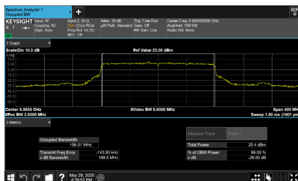
Plot 7-28 26dB BW & 99% OBW Antenna WF5B (160MHz BW 802.11be(SU) - Ch.207)
