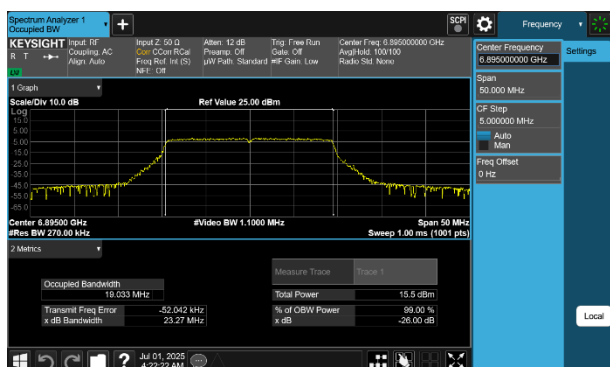
Plot 7-81 26dB BW & 99% OBW Antenna WF7 (20MHz BW 802.11be(SU) - Ch.189)
