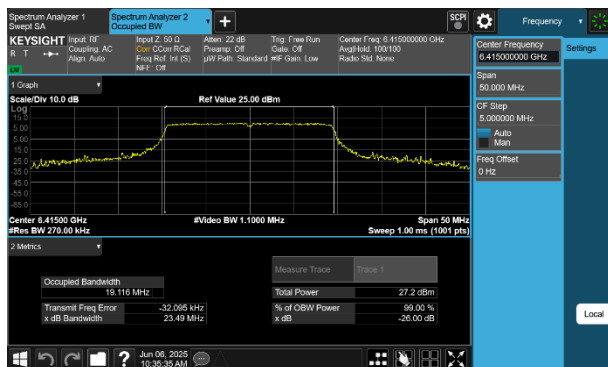
Plot 7-57 26dB BW & 99% OBW Antenna WF7 (20MHz BW 802.11be(SU) - Ch.93)
