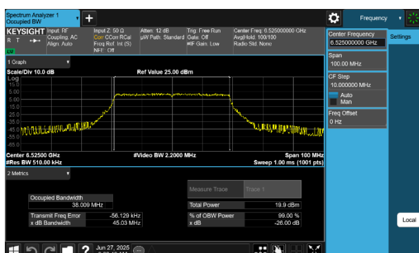
Plot 7-46 26dB BW & 99% OBW Antenna WF8 (40MHz BW 802.11be(SU) - Ch.115)
