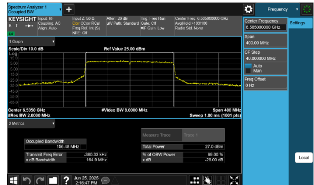
Plot 7-64 26dB BW & 99% OBW Antenna WF7 (160MHz BW 802.11be(SU) - Ch.111)
