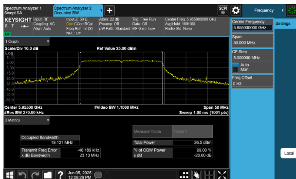
Plot 7-1 26dB BW & 99% OBW Antenna WF5B (20MHz BW 802.11be(SU) - Ch.1)
