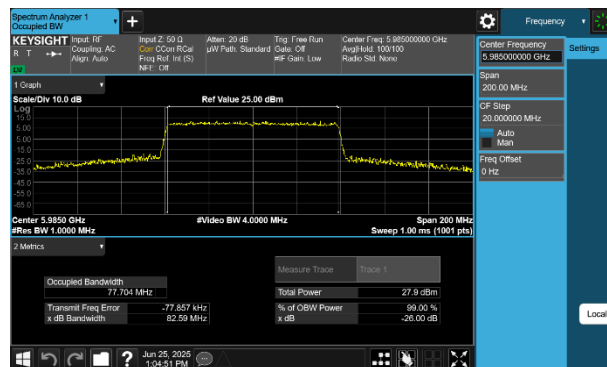
Plot 7-3 26dB BW & 99% OBW Antenna WF5B (80MHz BW 802.11be(SU) - Ch.7)
