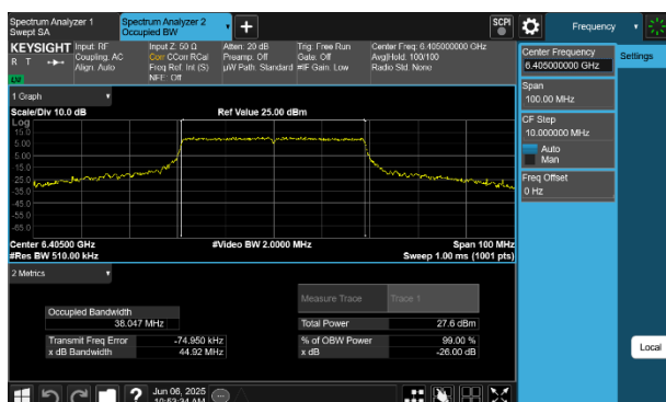
Plot 7-58 26dB BW & 99% OBW Antenna WF7 (40MHz BW 802.11be(SU) - Ch.91)
