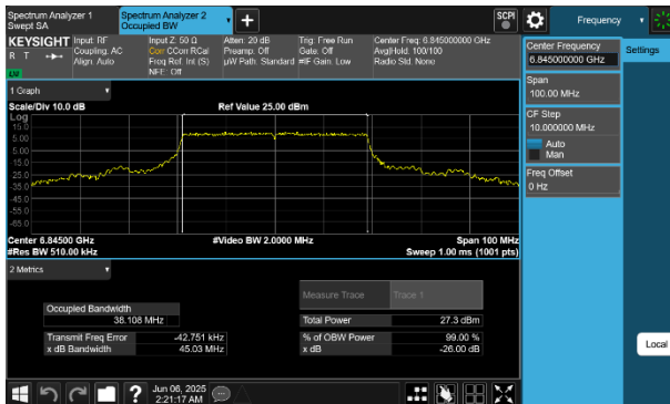
Plot 7-38 26dB BW & 99% OBW Antenna WF8 (40MHz BW 802.11be(SU) - Ch.179)
