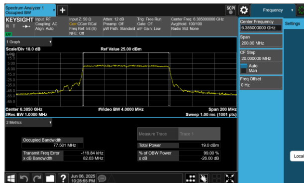
Plot 7-3 26dB BW & 99% OBW Antenna WF5B (80MHz BW 802.11be(SU) - Ch.87)
