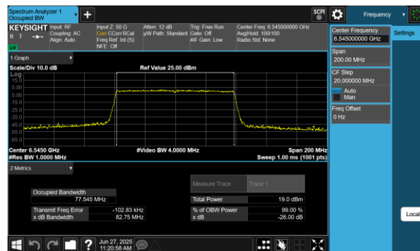
Plot 7-27 26dB BW & 99% OBW Antenna WF8 (80MHz BW 802.11be(SU) - Ch.119)
