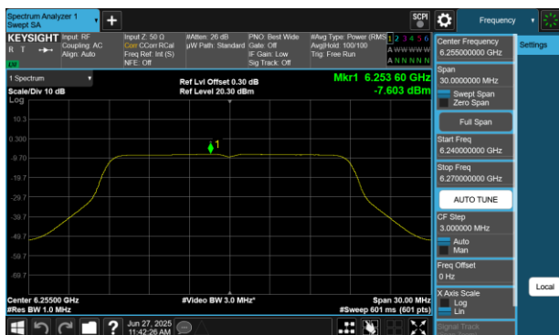
Plot 7-65 PSD Antenna WF8 (20MHz BW 802.11a - Ch.61)
