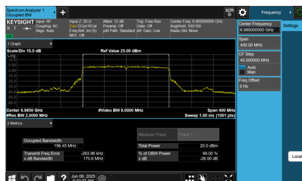
Plot 7-48 26dB BW & 99% OBW Antenna WF7 (160MHz BW 802.11be(SU) - Ch.207)
