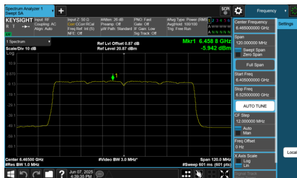
Plot 7-71 PSD Antenna WF8 (80MHz BW 802.11be(SU) - Ch.103)
