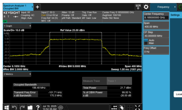
Plot 7-4 26dB BW & 99% OBW Antenna WF5B (160MHz BW 802.11be(SU) - Ch.47)
