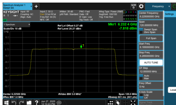
Plot 7-67 PSD Antenna WF8 (80MHz BW 802.11be(SU) - Ch.55)
