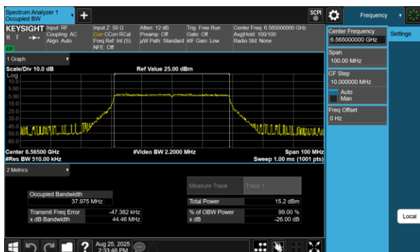
Plot 7-26 26dB BW & 99% OBW Antenna WF8 (40MHz BW 802.11be(SU) - Ch.123)
