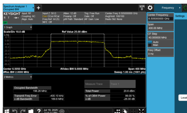
Plot 7-40 26dB BW & 99% OBW Antenna WF7 (160MHz BW 802.11be(SU) - Ch.111)
