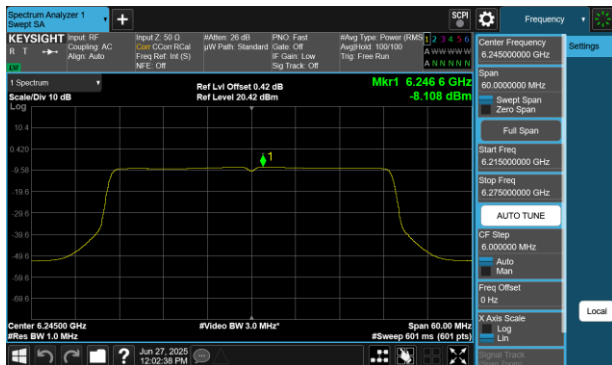
Plot 7-66 PSD Antenna WF8 (40MHz BW 802.11be(SU) - Ch.59)
