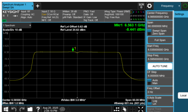
Plot 7-58 PSD Antenna WF5B (40MHz BW 802.11be(SU) - Ch.123)
