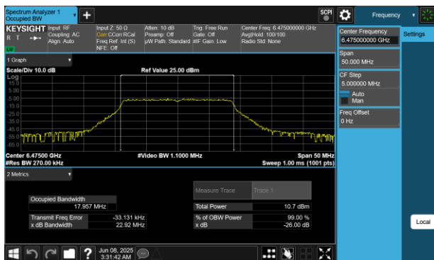
Plot 7-37 26dB BW & 99% OBW Antenna WF7 (20MHz BW 802.11a - Ch.105)
