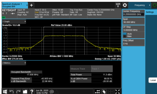
Plot 7-1 26dB BW & 99% OBW Antenna WF5B (20MHz BW 802.11a - Ch.61)
