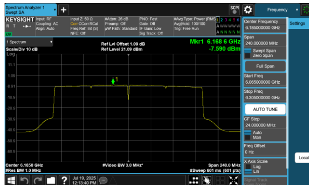
Plot 7-68 PSD Antenna WF8 (160MHz BW 802.11be(SU) - Ch.47)
