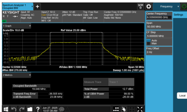
Plot 7-25 26dB BW & 99% OBW Antenna WF8 (20MHz BW 802.11be(SU) - Ch.117)
