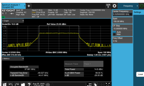
Plot 7-38 26dB BW & 99% OBW Antenna WF7 (40MHz BW 802.11be(SU) - Ch.115)
