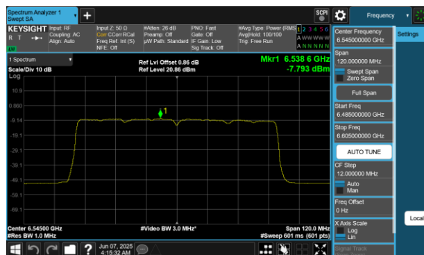
Plot 7-59 PSD Antenna WF5B (80MHz BW 802.11be(SU) - Ch.119)
