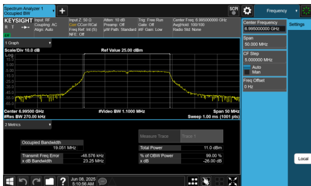
Plot 7-45 26dB BW & 99% OBW Antenna WF7 (20MHz BW 802.11be(SU) - Ch.209)
