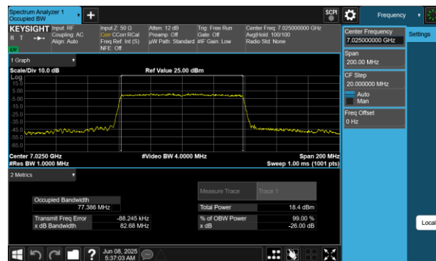
Plot 7-47 26dB BW & 99% OBW Antenna WF7 (80MHz BW 802.11be(SU) - Ch.215)
