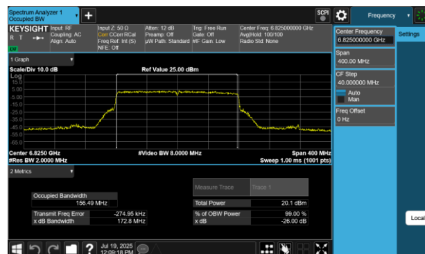
Plot 7-28 26dB BW & 99% OBW Antenna WF8 (160MHz BW 802.11be(SU) - Ch.175)
