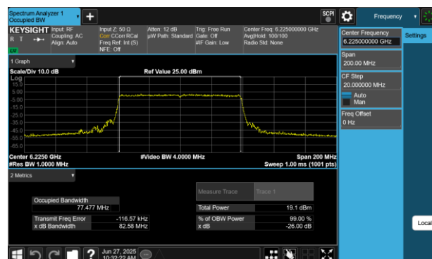
Plot 7-19 26dB BW & 99% OBW Antenna WF8 (80MHz BW 802.11be(SU) - Ch.55)
