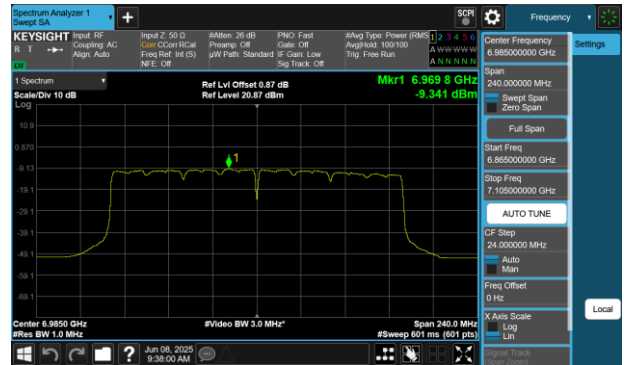
Plot 7-96 PSD Antenna WF7 (160MHz BW 802.11be(SU) - Ch.207)
