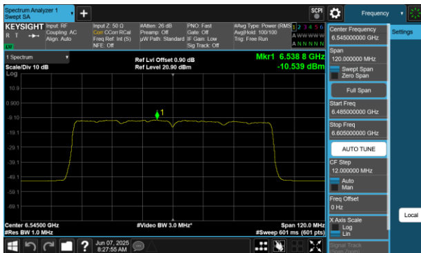
Plot 7-115 PSD SDM Primary Antenna WF5B (80MHz BW 802.11be(SU) - Ch.119)
