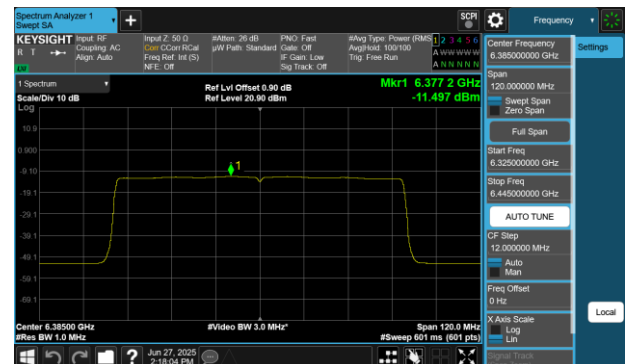
Plot 7-103 PSD SDM Primary Antenna WF8 (80MHz BW 802.11be(SU) - Ch.87)
