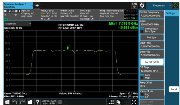
Plot 7-159 PSD SDM Diversity Antenna WF7 (80MHz BW 802.11be(SU) - Ch.215)
