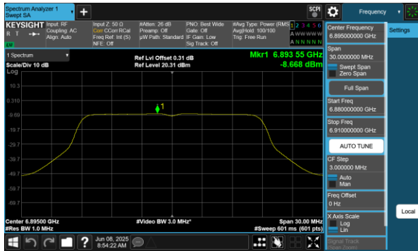
Plot 7-93 PSD Antenna WF7 (20MHz BW 802.11a - Ch.189)
