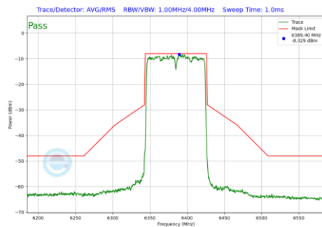
Plot 7-163 In-Band Emission Plot Antenna WF5B (80MHz BW 802.11be(SU) (UNII Band 5) - Ch.87)
