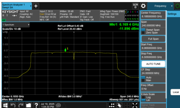
Plot 7-132 PSD SDM Diversity Antenna WF8 (160MHz BW 802.11be(SU) - Ch.47)
