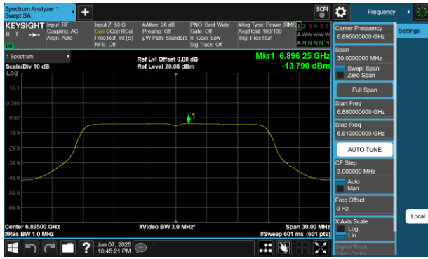
Plot 7-153 PSD CDD Diversity Antenna WF8 (20MHz BW 802.11a - Ch.189)
