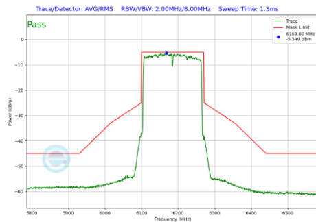
Plot 7-164 In-Band Emission Plot Antenna WF5B (160MHz BW 802.11be(SU) (UNII Band 5) - Ch.47)
