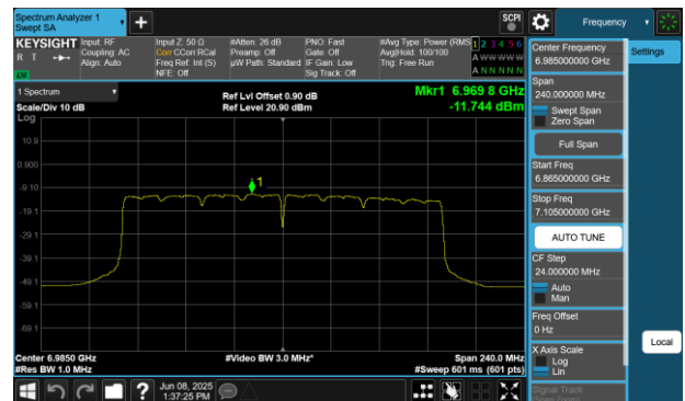
Plot 7-160 PSD SDM Diversity Antenna WF7 (160MHz BW 802.11be(SU) - Ch.207)
