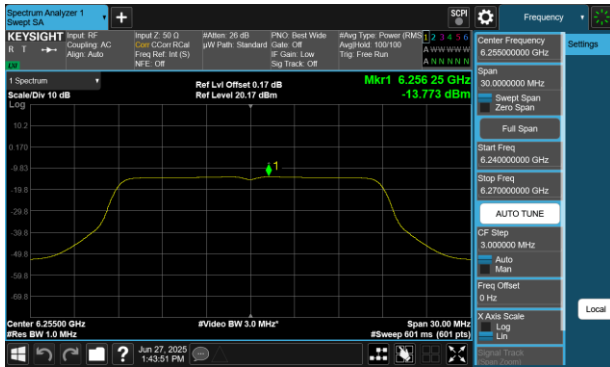
Plot 7-129 PSD CDD Diversity Antenna WF8 (20MHz BW 802.11a - Ch.61)
