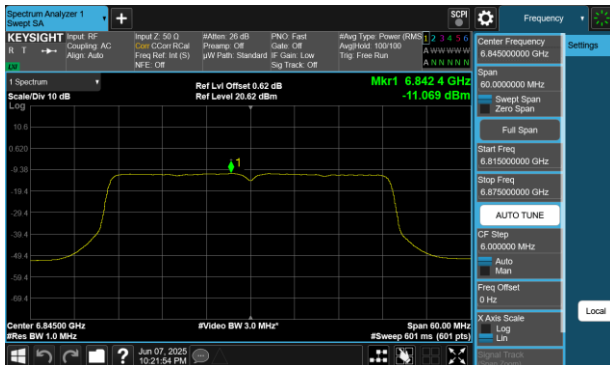
Plot 7-146 PSD SDM Diversity Antenna WF8 (40MHz BW 802.11be(SU) - Ch.179)
