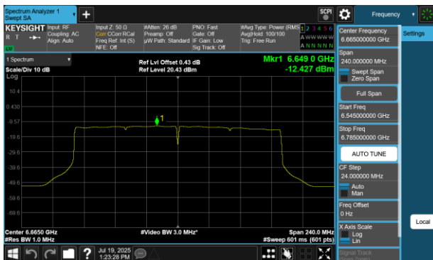
Plot 7-148 PSD SDM Diversity Antenna WF8 (160MHz BW 802.11be(SU) - Ch.143)
