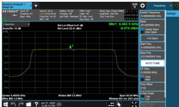
Plot 7-86 PSD Antenna WF7 (40MHz BW 802.11be(SU) - Ch.107)
