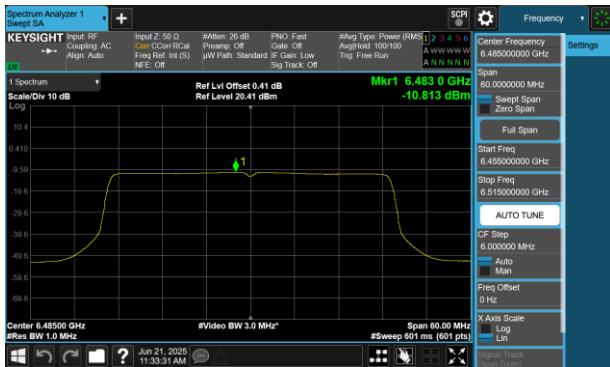
Plot 7-106 PSD SDM Primary Antenna WF5B (40MHz BW 802.11be(SU) - Ch.107)
