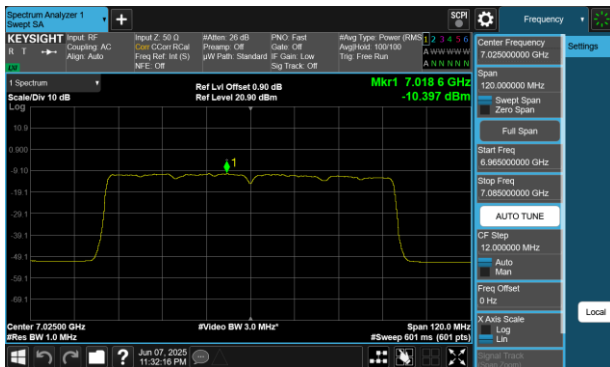
Plot 7-155 PSD SDM Diversity Antenna WF8 (80MHz BW 802.11be(SU) - Ch.215)
