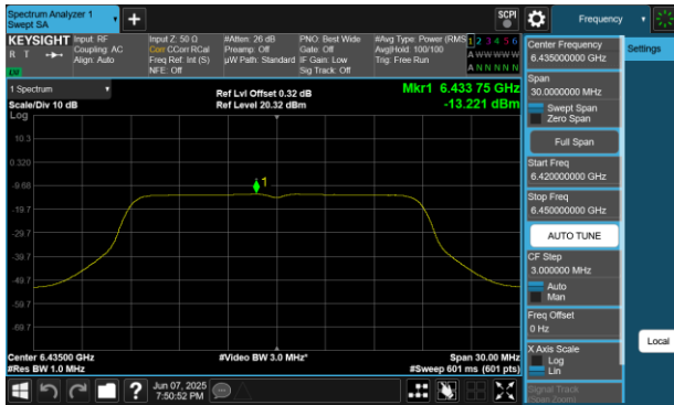
Plot 7-137 PSD CDD Diversity Antenna WF8 (20MHz BW 802.11a - Ch.97)
