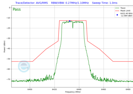
Plot 7-165 In-Band Emission Plot Antenna WF5B (20MHz BW 802.11a (UNII Band 6) - Ch.97)
