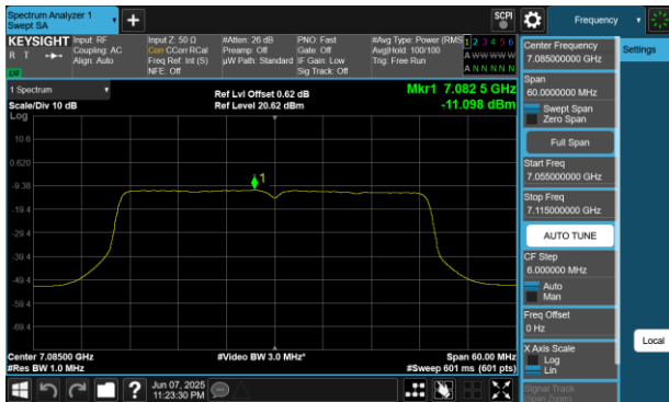
Plot 7-154 PSD SDM Diversity Antenna WF8 (40MHz BW 802.11be(SU) - Ch.227)
