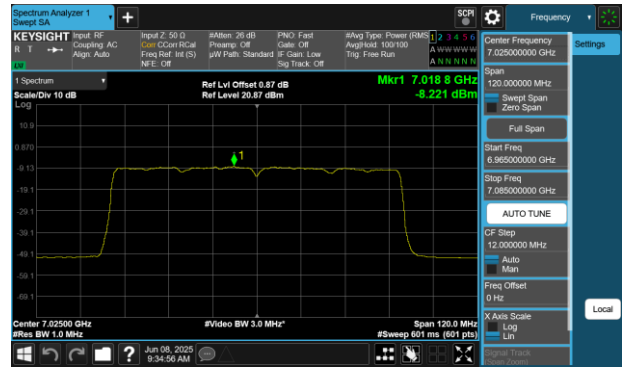
Plot 7-95 PSD Antenna WF7 (80MHz BW 802.11be(SU) - Ch.215)
