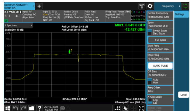
Plot 7-120 PSD SDM Primary Antenna WF8 (160MHz BW 802.11be(SU) - Ch.143)
