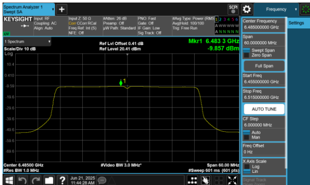
Plot 7-138 PSD SDM Diversity Antenna WF8 (40MHz BW 802.11be(SU) - Ch.107)
