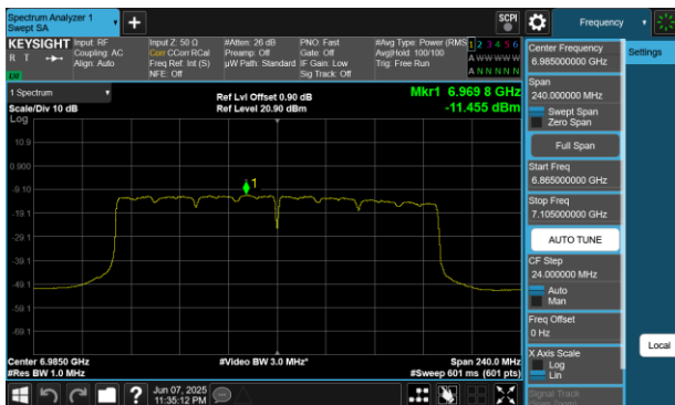
Plot 7-156 PSD SDM Diversity Antenna WF8 (160MHz BW 802.11be(SU) - Ch.207)
