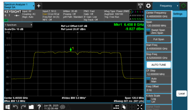
Plot 7-143 PSD SDM Diversity Antenna WF7 (80MHz BW 802.11be(SU) - Ch.103)
