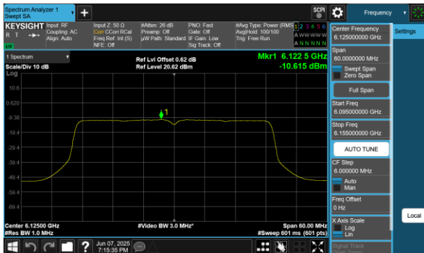
Plot 7-130 PSD SDM Diversity Antenna WF8 (40MHz BW 802.11be(SU) - Ch.35)
