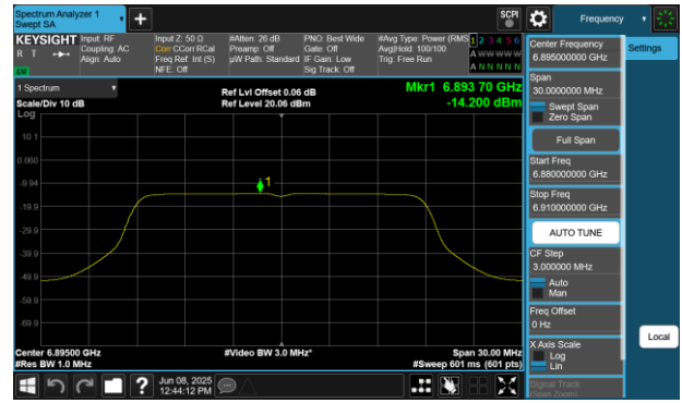
Plot 7-157 PSD CDD Diversity Antenna WF7 (20MHz BW 802.11a - Ch.189)
