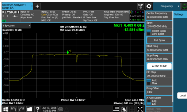
Plot 7-140 PSD SDM Diversity Antenna WF8 (160MHz BW 802.11be(SU) - Ch.111)
