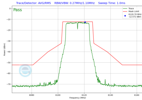
Plot 7-161 In-Band Emission Plot Antenna WF5B (20MHz BW 802.11a (UNII Band 5) - Ch.33)
