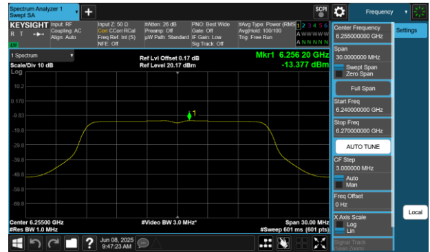
Plot 7-133 PSD CDD Diversity Antenna WF7 (20MHz BW 802.11a - Ch.61)
