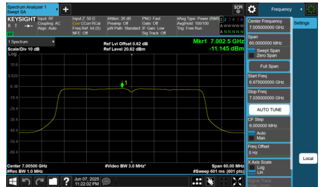
Plot 7-126 PSD SDM Primary Antenna WF8 (40MHz BW 802.11be(SU) - Ch.211)
