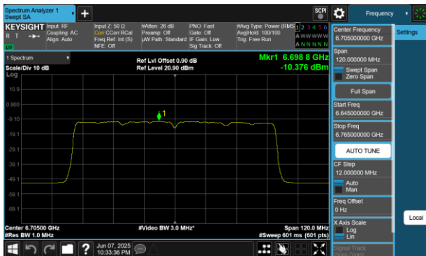
Plot 7-147 PSD SDM Diversity Antenna WF8 (80MHz BW 802.11be(SU) - Ch.151)
