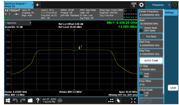
Plot 7-109 PSD CDD Primary Antenna WF8 (20MHz BW 802.11a - Ch.97)
