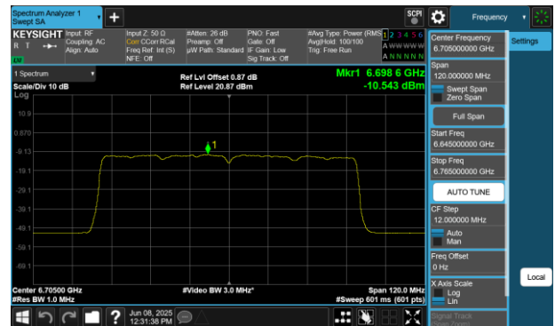
Plot 7-151 PSD SDM Diversity Antenna WF7 (80MHz BW 802.11be(SU) - Ch.151)
