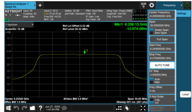
Plot 7-101 PSD CDD Primary Antenna WF8 (20MHz BW 802.11a - Ch.61)
