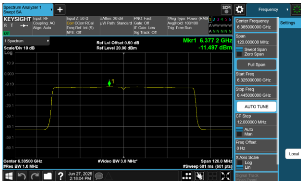
Plot 7-131 PSD SDM Diversity Antenna WF8 (80MHz BW 802.11be(SU) - Ch.87)
