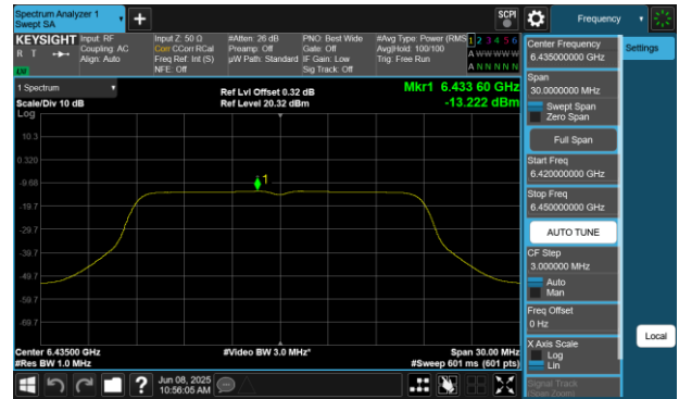
Plot 7-141 PSD CDD Diversity Antenna WF7 (20MHz BW 802.11a - Ch.97)
