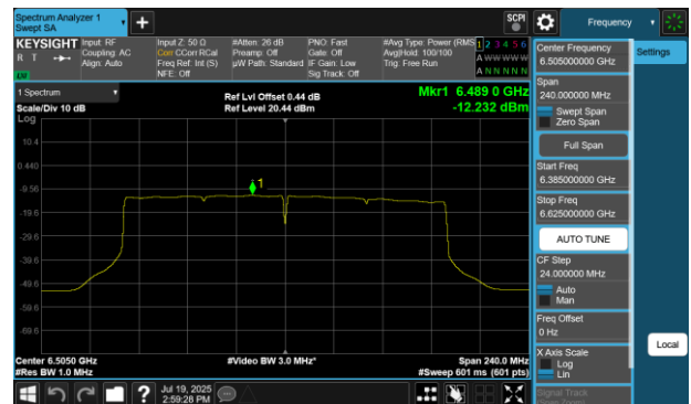
Plot 7-144 PSD SDM Diversity Antenna WF7 (160MHz BW 802.11be(SU) - Ch.111)
