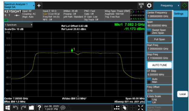
Plot 7-158 PSD SDM Diversity Antenna WF7 (40MHz BW 802.11be(SU) - Ch.227)
