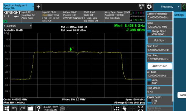
Plot 7-87 PSD Antenna WF7 (80MHz BW 802.11be(SU) - Ch.103)
