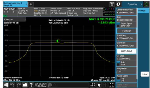
Plot 7-149 PSD CDD Diversity Antenna WF7 (20MHz BW 802.11a - Ch.149)
