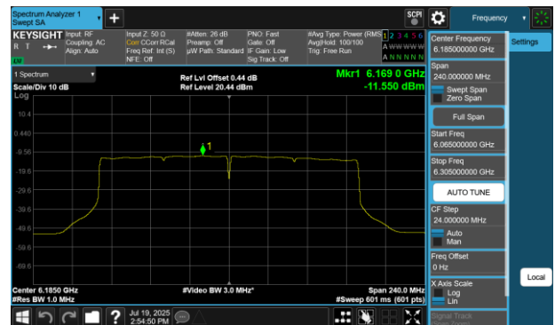
Plot 7-136 PSD SDM Diversity Antenna WF7 (160MHz BW 802.11be(SU) - Ch.47)
