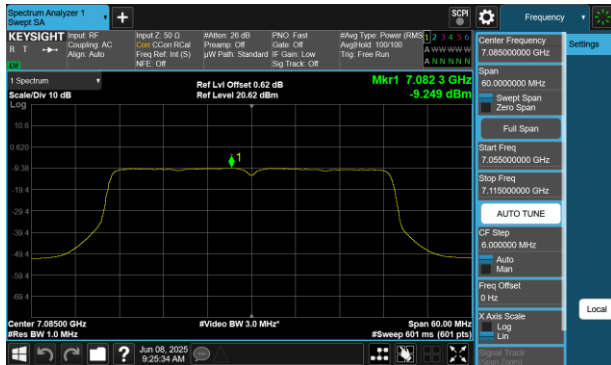
Plot 7-94 PSD Antenna WF7 (40MHz BW 802.11be(SU) - Ch.227)
