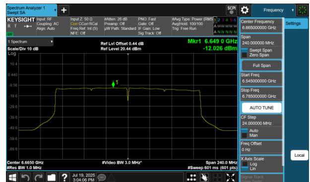
Plot 7-152 PSD SDM Diversity Antenna WF7 (160MHz BW 802.11be(SU) - Ch.143)
