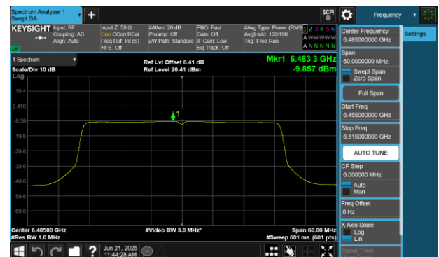
Plot 7-110 PSD SDM Primary Antenna WF8 (40MHz BW 802.11be(SU) - Ch.107)
