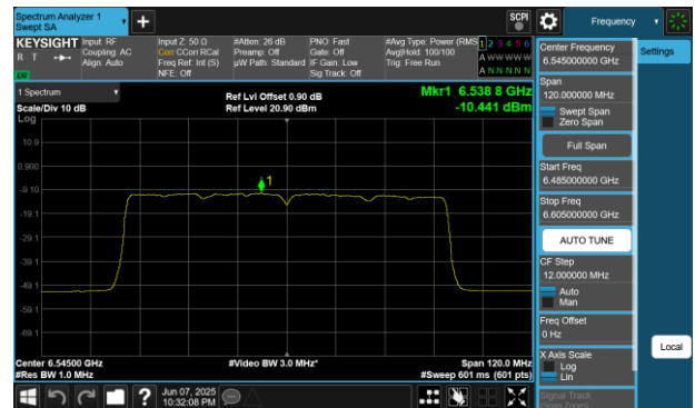
Plot 7-119 PSD SDM Primary Antenna WF8 (80MHz BW 802.11be(SU) - Ch.119)
