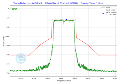
Plot 7-162 In-Band Emission Plot Antenna WF5B (40MHz BW 802.11be(SU) (UNII Band 5) - Ch.91)
