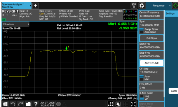
Plot 7-139 PSD SDM Diversity Antenna WF8 (80MHz BW 802.11be(SU) - Ch.103)
