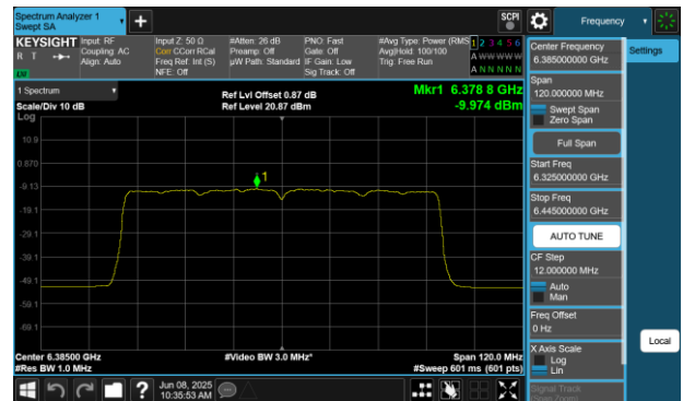
Plot 7-135 PSD SDM Diversity Antenna WF7 (80MHz BW 802.11be(SU) - Ch.87)
