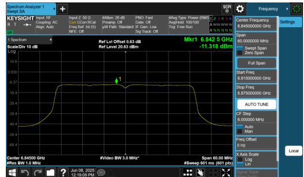
Plot 7-150 PSD SDM Diversity Antenna WF7 (40MHz BW 802.11be(SU) - Ch.179)
