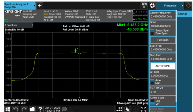
Plot 7-142 PSD SDM Diversity Antenna WF7 (40MHz BW 802.11be(SU) - Ch.107)
