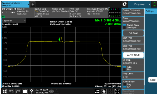
Plot 7-194 PSD SDM Primary Antenna WF5B (40MHz BW 802.11be(SU) - Ch.3)
