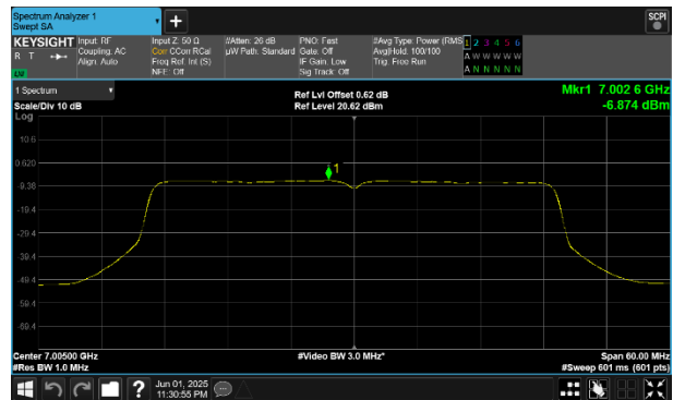
Plot 7-222 PSD SDM Primary Antenna WF8 (40MHz BW 802.11be(SU) - Ch.211)
