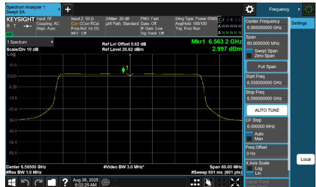
Plot 7-190 PSD CDD Primary Antenna WF8 (40MHz BW 802.11be(SU) - Ch.123)
