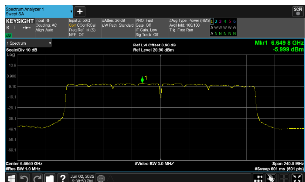
Plot 7-272 PSD SDM Diversity Antenna WF7 (160MHz BW 802.11be(SU) - Ch.143)
