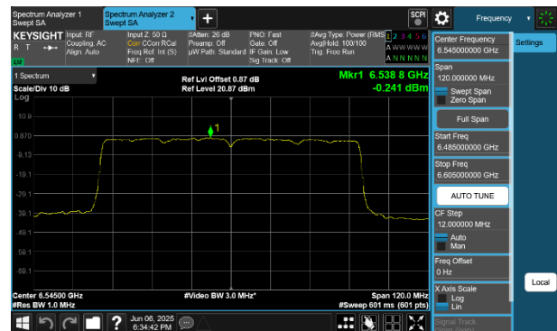
Plot 7-247 PSD CDD Diversity Antenna WF7 (80MHz BW 802.11be(SU) - Ch.119)
