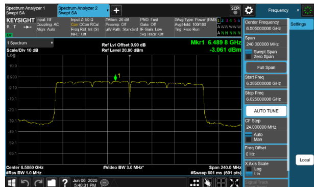
Plot 7-240 PSD CDD Diversity Antenna WF7 (160MHz BW 802.11be(SU) - Ch.111)
