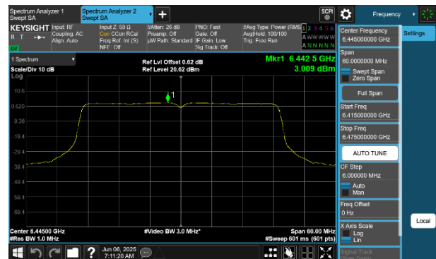
Plot 7-182 PSD CDD Primary Antenna WF8 (40MHz BW 802.11be(SU) - Ch.99)
