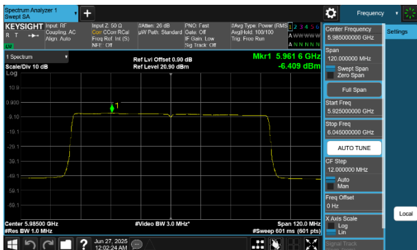
Plot 7-195 PSD SDM Primary Antenna WF5B (80MHz BW 802.11be(SU) - Ch.7)
