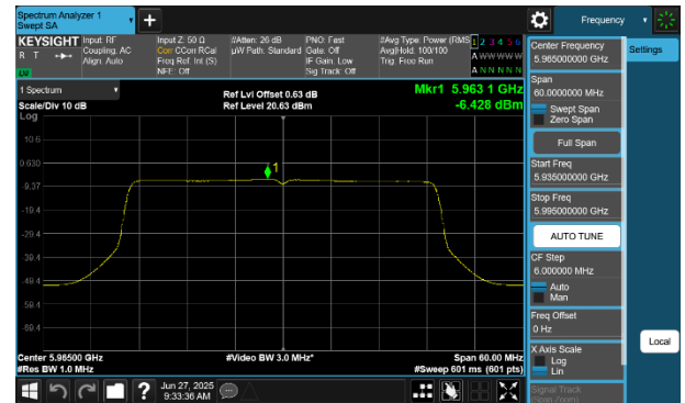
Plot 7-254 PSD SDM Diversity Antenna WF7 (40MHz BW 802.11be(SU) - Ch.3)
