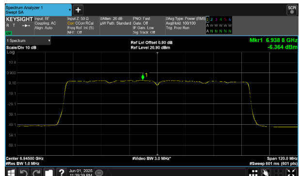
Plot 7-223 PSD SDM Primary Antenna WF8 (80MHz BW 802.11be(SU) - Ch.199)
