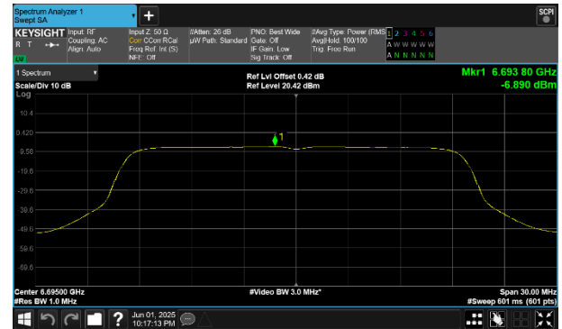
Plot 7-213 PSD SDM Primary Antenna WF8 (20MHz BW 802.11be(SU) - Ch.149)
