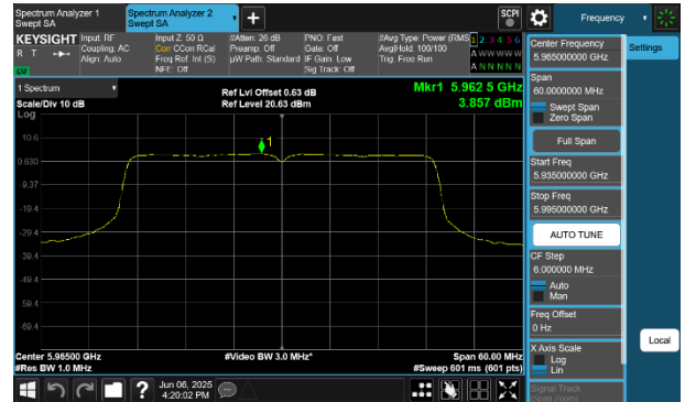
Plot 7-230 PSD CDD Diversity Antenna WF7 (40MHz BW 802.11be(SU) - Ch.3)
