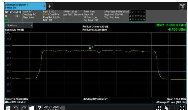
Plot 7-215 PSD SDM Primary Antenna WF8 (80MHz BW 802.11be(SU) - Ch.151)
