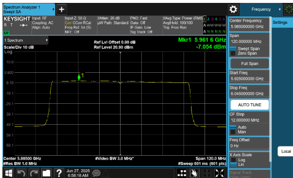
Plot 7-251 PSD SDM Diversity Antenna WF8 (80MHz BW 802.11be(SU) - Ch.7)
