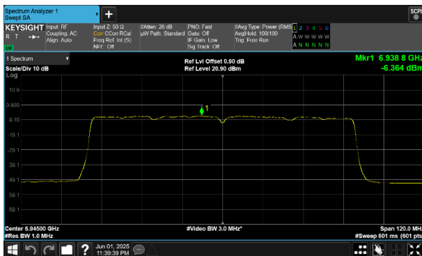
Plot 7-275 PSD SDM Diversity Antenna WF8 (80MHz BW 802.11be(SU) - Ch.199)
