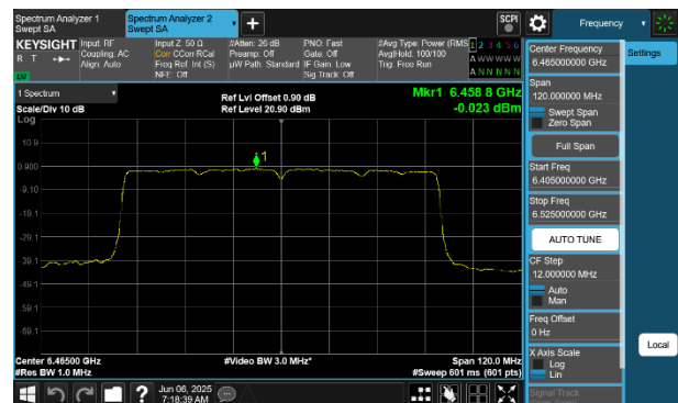
Plot 7-183 PSD CDD Primary Antenna WF8 (80MHz BW 802.11be(SU) - Ch.103)
