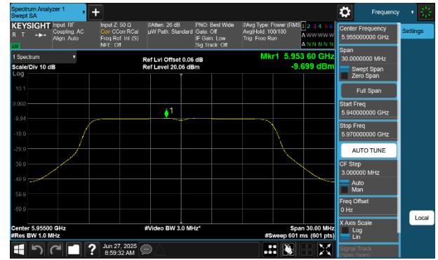
Plot 7-253 PSD CDD Diversity Antenna WF7 (20MHz BW 802.11a - Ch.1)
