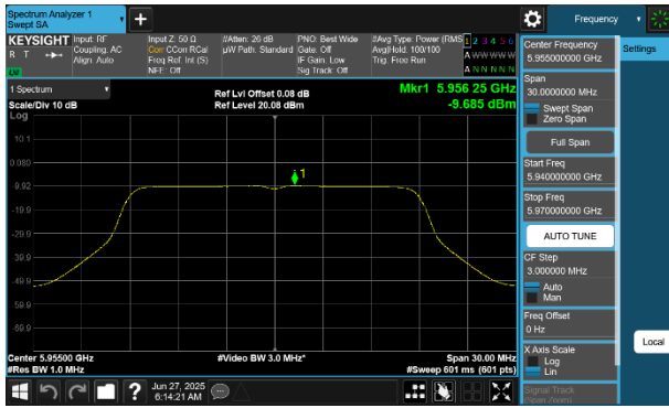
Plot 7-249 PSD CDD Diversity Antenna WF8 (20MHz BW 802.11a - Ch.1)
