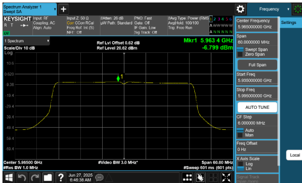
Plot 7-250 PSD SDM Diversity Antenna WF8 (40MHz BW 802.11be(SU) - Ch.3)
