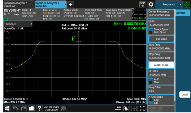
Plot 7-189 PSD CDD Primary Antenna WF8 (20MHz BW 802.11a - Ch.181)
