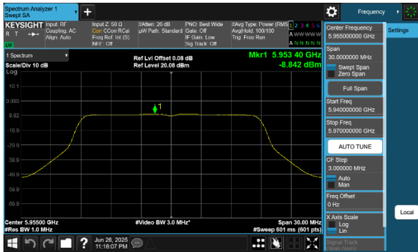
Plot 7-193 PSD CDD Primary Antenna WF5B (20MHz BW 802.11a - Ch.1)
