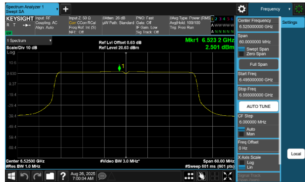
Plot 7-238 PSD CDD Diversity Antenna WF7 (40MHz BW 802.11be(SU) - Ch.115)
