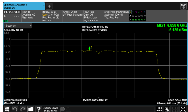
Plot 7-271 PSD SDM Diversity Antenna WF7 (80MHz BW 802.11be(SU) - Ch.183)
