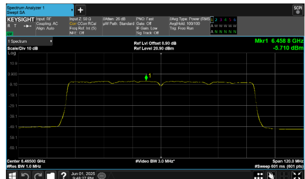
Plot 7-207 PSD SDM Primary Antenna WF8 (80MHz BW 802.11be(SU) - Ch.103)
