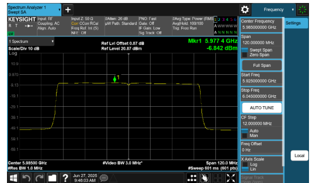
Plot 7-255 PSD SDM Diversity Antenna WF7 (80MHz BW 802.11be(SU) - Ch.7)
