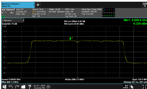
Plot 7-267 PSD SDM Diversity Antenna WF8 (80MHz BW 802.11be(SU) - Ch.183)
