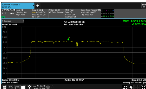
Plot 7-268 PSD SDM Diversity Antenna WF8 (160MHz BW 802.11be(SU) - Ch.143)
