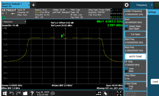
Plot 7-242 PSD CDD Diversity Antenna WF8 (40MHz BW 802.11be(SU) - Ch.123)
