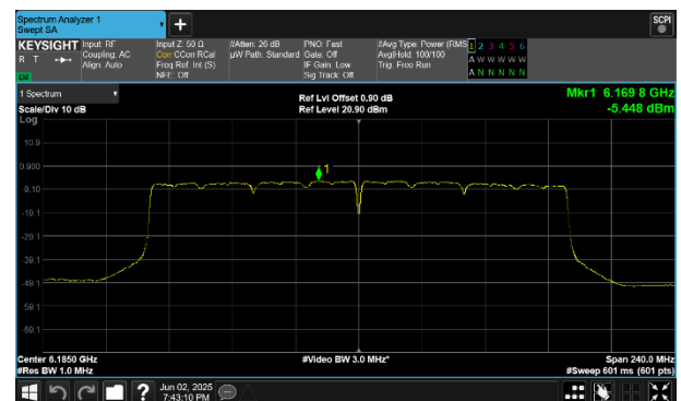
Plot 7-256 PSD SDM Diversity Antenna WF7 (160MHz BW 802.11be(SU) - Ch.47)
