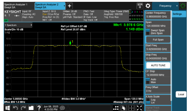
Plot 7-231 PSD CDD Diversity Antenna WF7 (80MHz BW 802.11be(SU) - Ch.7)
