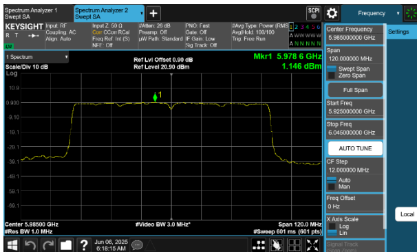
Plot 7-227 PSD CDD Diversity Antenna WF8 (80MHz BW 802.11be(SU) - Ch.7)
