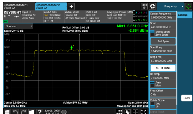
Plot 7-192 PSD CDD Primary Antenna WF8 (160MHz BW 802.11be(SU) - Ch.143)
