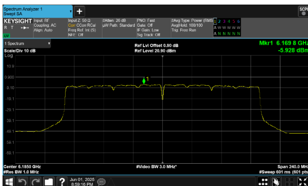
Plot 7-252 PSD SDM Diversity Antenna WF8 (160MHz BW 802.11be(SU) - Ch.47)
