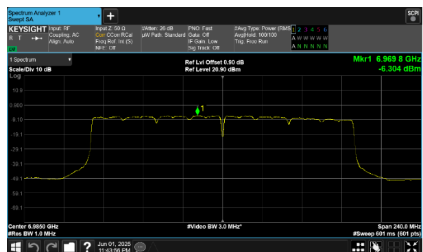
Plot 7-224 PSD SDM Primary Antenna WF8 (160MHz BW 802.11be(SU) - Ch.207)
