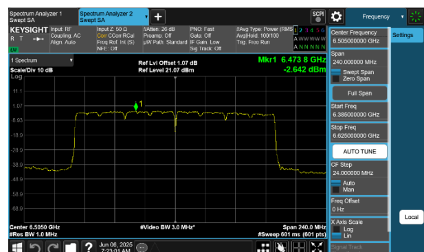
Plot 7-184 PSD CDD Primary Antenna WF8 (160MHz BW 802.11be(SU) - Ch.111)
