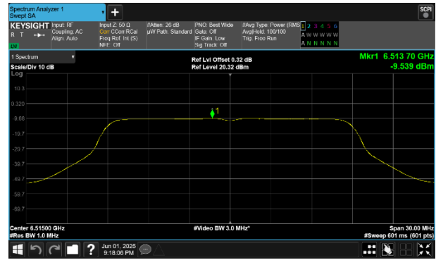
Plot 7-205 PSD CDD Primary Antenna WF8 (20MHz BW 802.11a - Ch.113)
