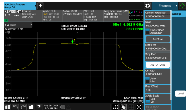
Plot 7-246 PSD CDD Diversity Antenna WF7 (40MHz BW 802.11be(SU) - Ch.123)
