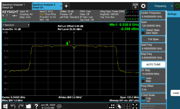
Plot 7-243 PSD CDD Diversity Antenna WF8 (80MHz BW 802.11be(SU) - Ch.119)
