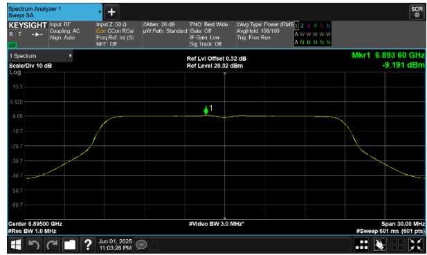
Plot 7-221 PSD CDD Primary Antenna WF8 (20MHz BW 802.11a - Ch.189)
