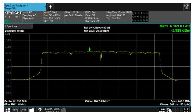
Plot 7-200 PSD SDM Primary Antenna WF8 (160MHz BW 802.11be(SU) - Ch.47)
