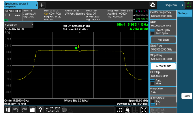
Plot 7-198 PSD SDM Primary Antenna WF8 (40MHz BW 802.11be(SU) - Ch.3)
