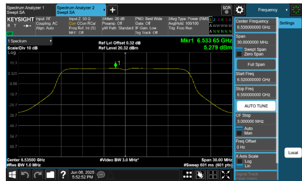
Plot 7-245 PSD CDD Diversity Antenna WF7 (20MHz BW 802.11a - Ch.117)
