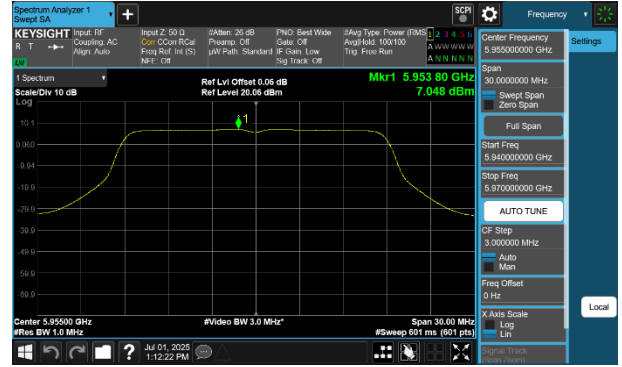
Plot 7-229 PSD CDD Diversity Antenna WF7 (20MHz BW 802.11a - Ch.1)
