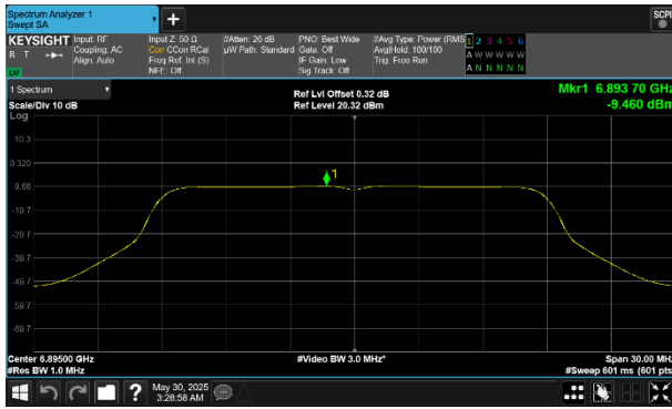
Plot 7-217 PSD CDD Primary Antenna WF5B (20MHz BW 802.11a - Ch.189)
