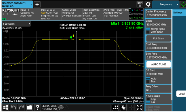
Plot 7-225 PSD CDD Diversity Antenna WF8 (20MHz BW 802.11a - Ch.1)
