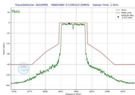
Plot 7-290 In-Band Emission Plot Antenna WF5B (40MHz BW 802.11be(SU) (UNII Band 7) - Ch.179)
