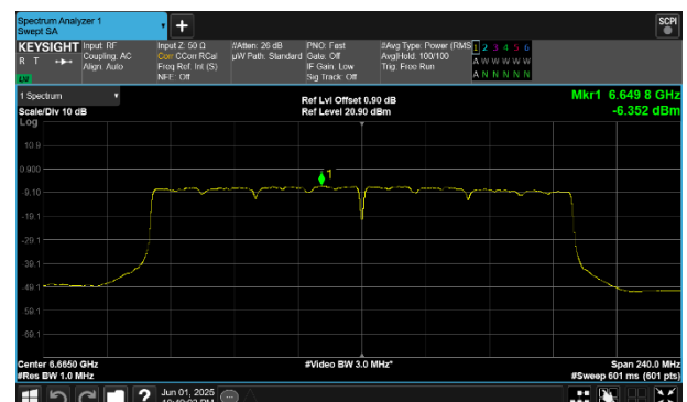
Plot 7-216 PSD SDM Primary Antenna WF8 (160MHz BW 802.11be(SU) - Ch.143)
