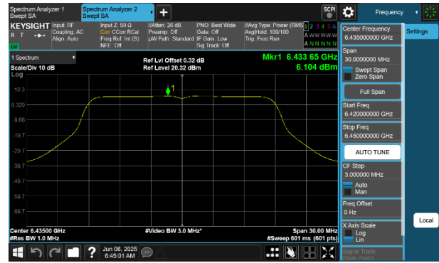
Plot 7-181 PSD CDD Primary Antenna WF8 (20MHz BW 802.11a - Ch.97)
