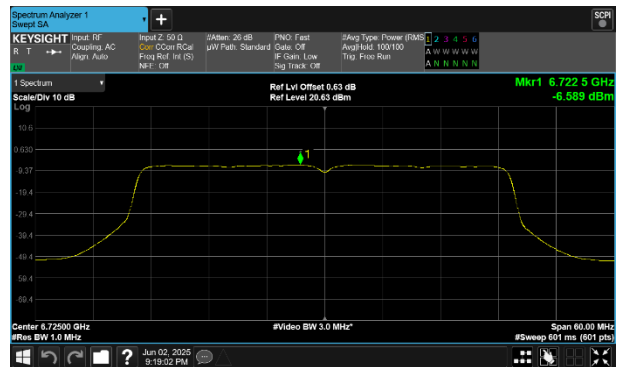
Plot 7-270 PSD SDM Diversity Antenna WF7 (40MHz BW 802.11be(SU) - Ch.155)
