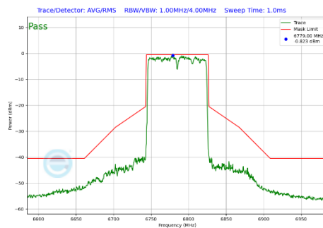
Plot 7-291 In-Band Emission Plot Antenna WF5B (80MHz BW 802.11be(SU) (UNII Band 7) - Ch.167)
