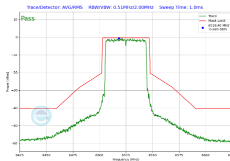
Plot 7-286 In-Band Emission Plot Antenna WF5B (40MHz BW 802.11be(SU) (UNII Band 6) - Ch.115)
