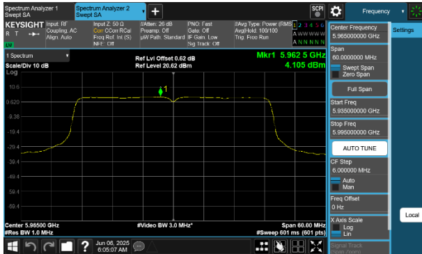
Plot 7-226 PSD CDD Diversity Antenna WF8 (40MHz BW 802.11be(SU) - Ch.3)
