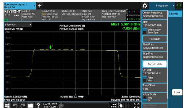
Plot 7-199 PSD SDM Primary Antenna WF8 (80MHz BW 802.11be(SU) - Ch.7)
