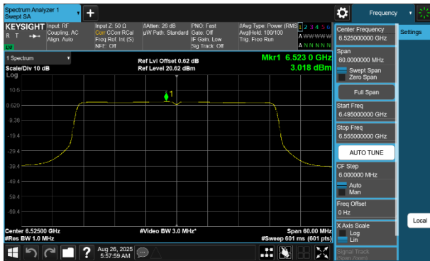
Plot 7-234 PSD CDD Diversity Antenna WF8 (40MHz BW 802.11be(SU) - Ch.115)
