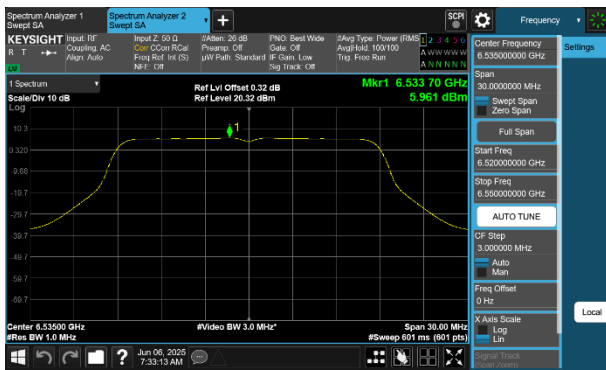
Plot 7-241 PSD CDD Diversity Antenna WF8 (20MHz BW 802.11a - Ch.117)
