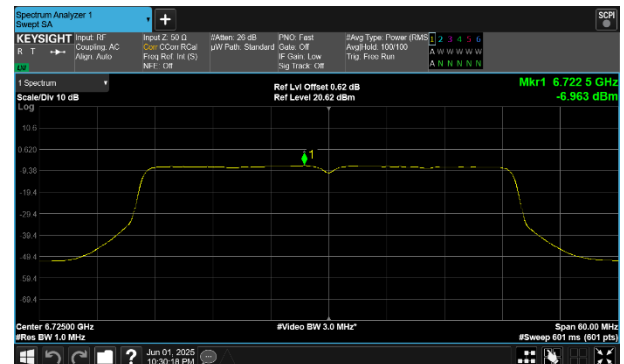
Plot 7-214 PSD SDM Primary Antenna WF8 (40MHz BW 802.11be(SU) - Ch.155)
