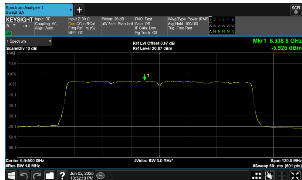
Plot 7-279 PSD SDM Diversity Antenna WF7 (80MHz BW 802.11be(SU) - Ch.199)
