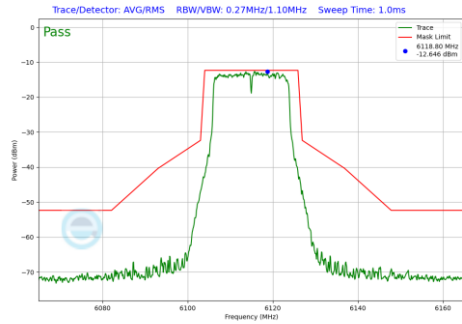
Plot 7-193 In-Band Emission Plot Antenna WF7 (20MHz BW 802.11a (UNII Band 5) - Ch.33)
