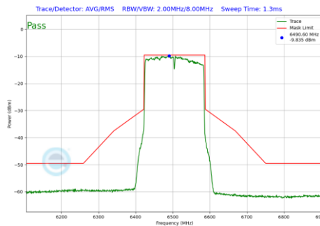
Plot 7-252 In-Band Emission Plot SDM Diversity Antenna WF8 (160MHz BW 802.11be(SU) (UNII Band 6) - Ch.111)
