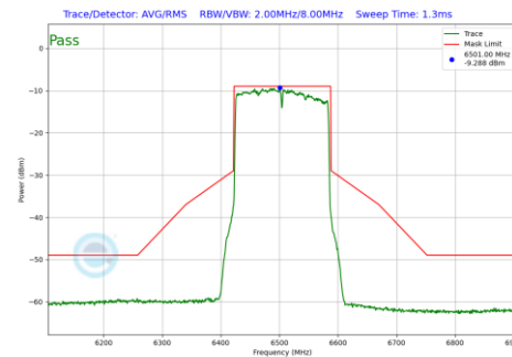
Plot 7-256 In-Band Emission Plot SDM Diversity Antenna WF7 (160MHz BW 802.11be(SU) (UNII Band 6) - Ch.111)
