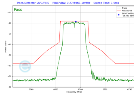
Plot 7-229 In-Band Emission Plot CDD Primary Antenna WF8 (20MHz BW 802.11a (UNII Band 7) - Ch.149)
