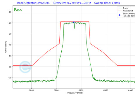
Plot 7-269 In-Band Emission Plot CDD Diversity Antenna WF7 (20MHz BW 802.11a (UNII Band 8) - Ch.189)
