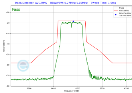
Plot 7-257 In-Band Emission Plot CDD Diversity Antenna WF8 (20MHz BW 802.11a (UNII Band 7) - Ch.149)
