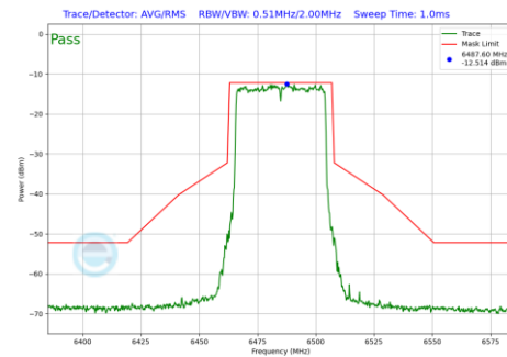
Plot 7-222 In-Band Emission Plot SDM Primary Antenna WF8 (40MHz BW 802.11be(SU) (UNII Band 6) - Ch.107)
