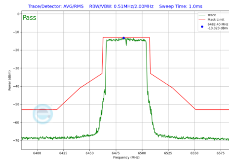
Plot 7-254 In-Band Emission Plot SDM Diversity Antenna WF7 (40MHz BW 802.11be(SU) (UNII Band 6) - Ch.107)
