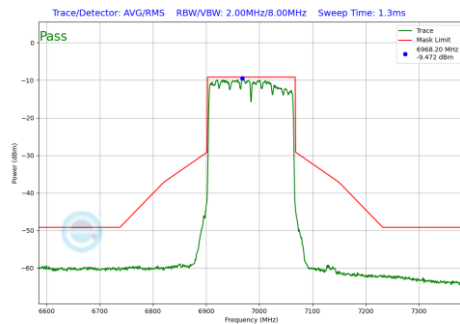
Plot 7-268 In-Band Emission Plot SDM Diversity Antenna WF8 (160MHz BW 802.11be(SU) (UNII Band 8) - Ch.207)
