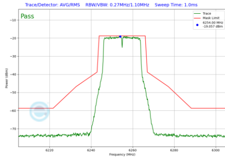
Plot 7-241 In-Band Emission Plot CDD Diversity Antenna WF8 (20MHz BW 802.11a (UNII Band 5) - Ch.61)
