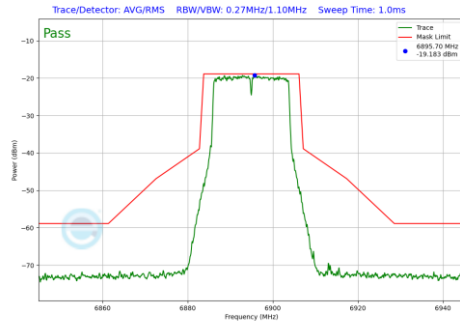
Plot 7-265 In-Band Emission Plot CDD Diversity Antenna WF8 (20MHz BW 802.11a (UNII Band 8) - Ch.189)
