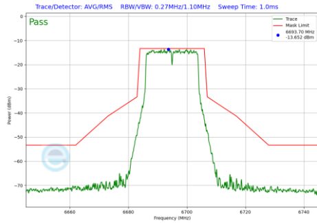
Plot 7-201 In-Band Emission Plot Antenna WF7 (20MHz BW 802.11a (UNII Band 7) - Ch.149)
