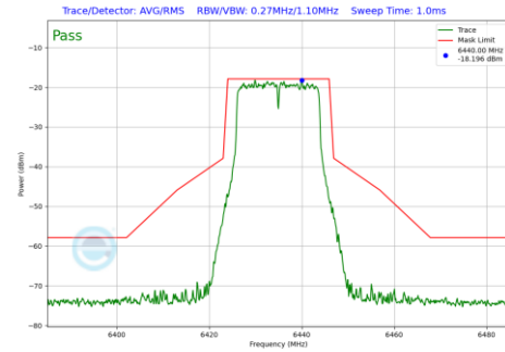
Plot 7-253 In-Band Emission Plot CDD Diversity Antenna WF7 (20MHz BW 802.11a (UNII Band 6) - Ch.97)
