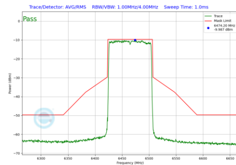
Plot 7-255 In-Band Emission Plot SDM Diversity Antenna WF7 (80MHz BW 802.11be(SU) (UNII Band 6) - Ch.103)
