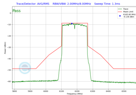
Plot 7-216 In-Band Emission Plot SDM Primary Antenna WF8 (160MHz BW 802.11be(SU) (UNII Band 5) - Ch.47)
