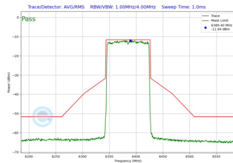
Plot 7-215 In-Band Emission Plot SDM Primary Antenna WF8 (80MHz BW 802.11be(SU) (UNII Band 5) - Ch.87)
