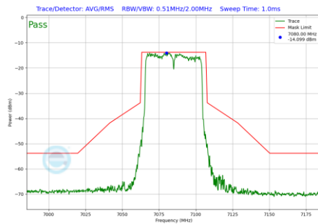
Plot 7-266 In-Band Emission Plot SDM Diversity Antenna WF8 (40MHz BW 802.11be(SU) (UNII Band 8) - Ch.227)
