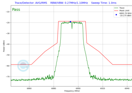
Plot 7-233 In-Band Emission Plot SDM Primary Antenna WF5B (20MHz BW 802.11a (UNII Band 8) - Ch.189)
