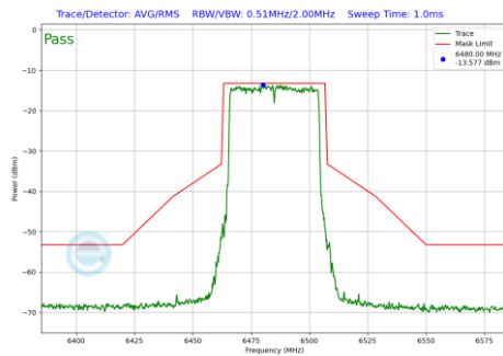
Plot 7-218 In-Band Emission Plot SDM Primary Antenna WF5B (40MHz BW 802.11be(SU) (UNII Band 6) - Ch.107)
