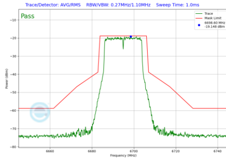
Plot 7-225 In-Band Emission Plot CDD Primary Antenna WF5B (20MHz BW 802.11a (UNII Band 7) - Ch.149)
