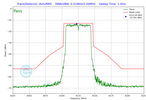
Plot 7-214 In-Band Emission Plot SDM Primary Antenna WF8 (40MHz BW 802.11be(SU) (UNII Band 5) - Ch.35)
