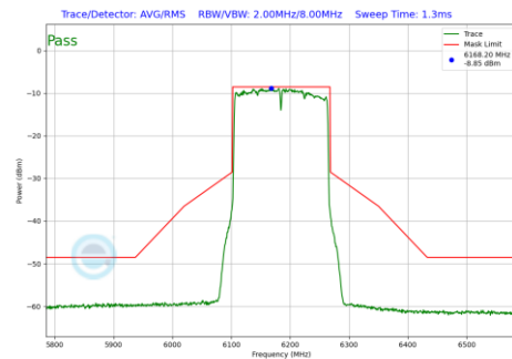
Plot 7-248 In-Band Emission Plot SDM Diversity Antenna WF7 (160MHz BW 802.11be(SU) (UNII Band 5) - Ch.47)
