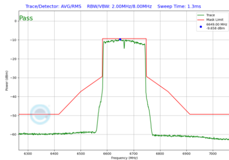
Plot 7-260 In-Band Emission Plot SDM Diversity Antenna WF8 (160MHz BW 802.11be(SU) (UNII Band 7) - Ch.143)
