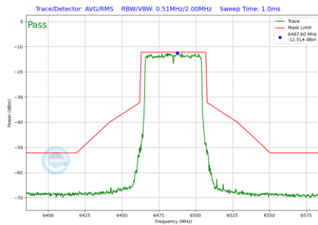
Plot 7-250 In-Band Emission Plot SDM Diversity Antenna WF8 (40MHz BW 802.11be(SU) (UNII Band 6) - Ch.107)
