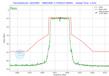
Plot 7-182 In-Band Emission Plot Antenna WF8 (40MHz BW 802.11be(SU) (UNII Band 6) - Ch.107)
