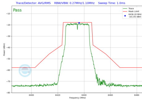
Plot 7-249 In-Band Emission Plot CDD Diversity Antenna WF8 (20MHz BW 802.11a (UNII Band 6) - Ch.97)
