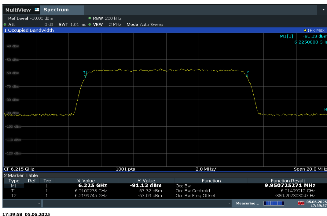
Plot 7-273. AWGN Signal – UNII 5 – 20MHz
