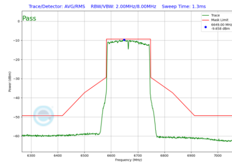
Plot 7-232 In-Band Emission Plot SDM Primary Antenna WF8 (160MHz BW 802.11be(SU) (UNII Band 7) - Ch.143)
