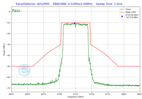
Plot 7-186 In-Band Emission Plot Antenna WF8 (40MHz BW 802.11be(SU) (UNII Band 7) - Ch.155)
