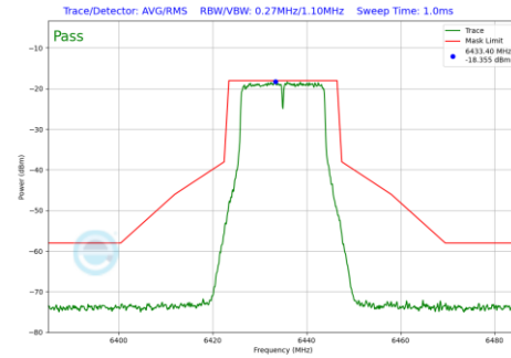
Plot 7-221 In-Band Emission Plot CDD Primary Antenna WF8 (20MHz BW 802.11a (UNII Band 6) - Ch.97)
