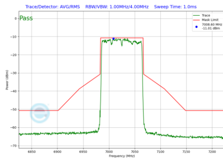
Plot 7-267 In-Band Emission Plot SDM Diversity Antenna WF8 (80MHz BW 802.11be(SU) (UNII Band 8) - Ch.215)
