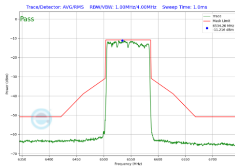
Plot 7-227 In-Band Emission Plot SDM Primary Antenna WF5B (80MHz BW 802.11be(SU) (UNII Band 7) - Ch.119)
