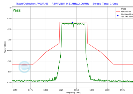
Plot 7-262 In-Band Emission Plot SDM Diversity Antenna WF7 (40MHz BW 802.11be(SU) (UNII Band 7) - Ch.179)
