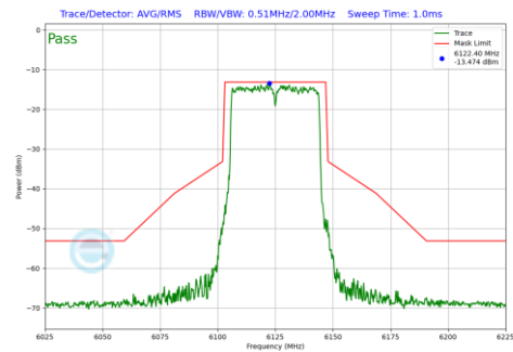
Plot 7-246 In-Band Emission Plot SDM Diversity Antenna WF7 (40MHz BW 802.11be(SU) (UNII Band 5) - Ch.35)
