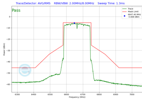
Plot 7-188 In-Band Emission Plot Antenna WF8 (160MHz BW 802.11be(SU) (UNII Band 7) - Ch.143)
