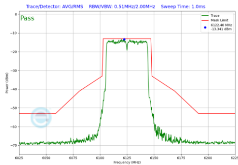
Plot 7-242 In-Band Emission Plot SDM Diversity Antenna WF8 (40MHz BW 802.11be(SU) (UNII Band 5) - Ch.35)
