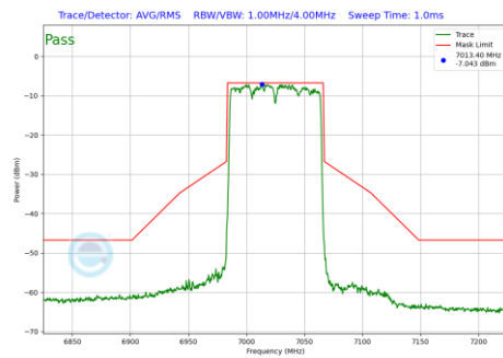
Plot 7-191 In-Band Emission Plot Antenna WF8 (80MHz BW 802.11be(SU) (UNII Band 8) - Ch.215)
