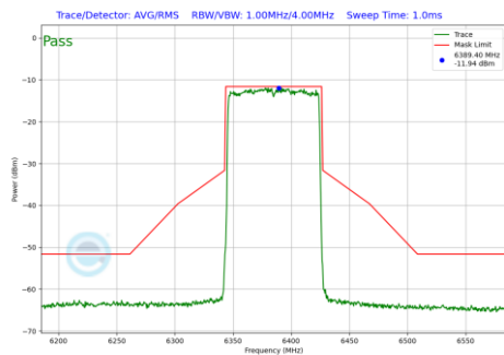
Plot 7-243 In-Band Emission Plot SDM Diversity Antenna WF8 (80MHz BW 802.11be(SU) (UNII Band 5) - Ch.87)
