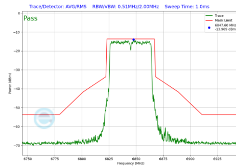
Plot 7-230 In-Band Emission Plot SDM Primary Antenna WF8 (40MHz BW 802.11be(SU) (UNII Band 7) - Ch.179)
