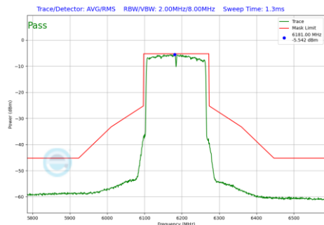
Plot 7-196 In-Band Emission Plot Antenna WF7 (160MHz BW 802.11be(SU) (UNII Band 5) - Ch.47)
