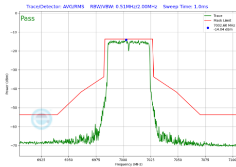
Plot 7-234 In-Band Emission Plot SDM Primary Antenna WF5B (40MHz BW 802.11be(SU) (UNII Band 8) - Ch.211)
