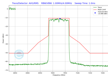
Plot 7-235 In-Band Emission Plot SDM Primary Antenna WF5B (80MHz BW 802.11be(SU) (UNII Band 8) - Ch.215)
