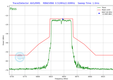
Plot 7-258 In-Band Emission Plot SDM Diversity Antenna WF8 (40MHz BW 802.11be(SU) (UNII Band 7) - Ch.179)
