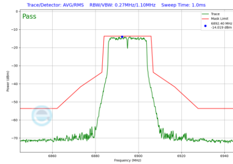
Plot 7-205 In-Band Emission Plot Antenna WF7 (20MHz BW 802.11a (UNII Band 8) - Ch.189)
