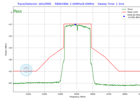
Plot 7-224 In-Band Emission Plot SDM Primary Antenna WF8 (160MHz BW 802.11be(SU) (UNII Band 6) - Ch.111)
