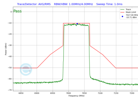
Plot 7-271 In-Band Emission Plot SDM Diversity Antenna WF7 (80MHz BW 802.11be(SU) (UNII Band 8) - Ch.215)
