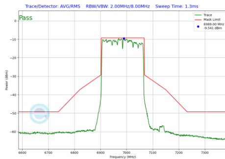
Plot 7-236 In-Band Emission Plot SDM Primary Antenna WF5B (160MHz BW 802.11be(SU) (UNII Band 8) - Ch.207)
