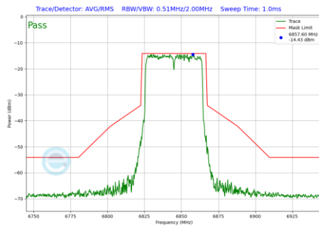
Plot 7-226 In-Band Emission Plot SDM Primary Antenna WF5B (40MHz BW 802.11be(SU) (UNII Band 7) - Ch.179)
