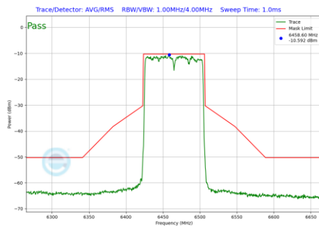
Plot 7-219 In-Band Emission Plot SDM Primary Antenna WF5B (80MHz BW 802.11be(SU) (UNII Band 6) - Ch.103)
