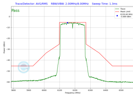
Plot 7-180 In-Band Emission Plot Antenna WF8 (160MHz BW 802.11be(SU) (UNII Band 5) - Ch.47)
