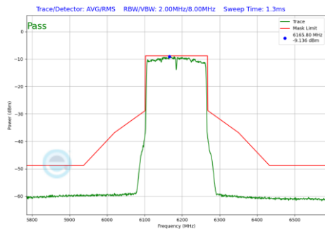
Plot 7-244 In-Band Emission Plot SDM Diversity Antenna WF8 (160MHz BW 802.11be(SU) (UNII Band 5) - Ch.47)
