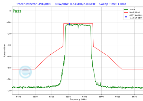
Plot 7-170 In-Band Emission Plot Antenna WF5B (40MHz BW 802.11be(SU) (UNII Band 7) - Ch.123)
