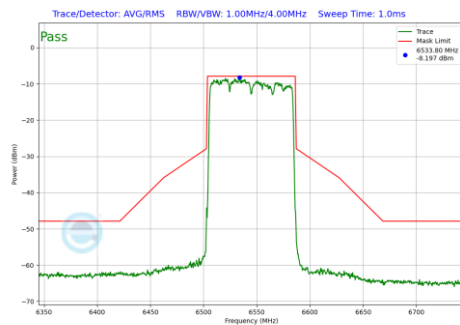
Plot 7-171 In-Band Emission Plot Antenna WF5B (80MHz BW 802.11be(SU) (UNII Band 7) - Ch.119)
