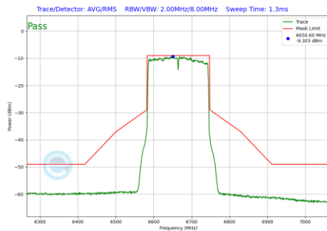
Plot 7-228 In-Band Emission Plot SDM Primary Antenna WF5B (160MHz BW 802.11be(SU) (UNII Band 7) - Ch.143)
