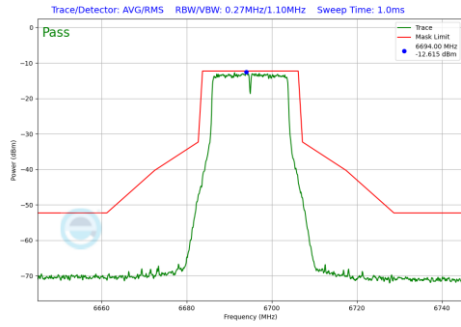
Plot 7-185 In-Band Emission Plot Antenna WF8 (20MHz BW 802.11a (UNII Band 7) - Ch.149)
