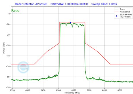
Plot 7-203 In-Band Emission Plot Antenna WF7 (80MHz BW 802.11be(SU) (UNII Band 7) - Ch.119)
