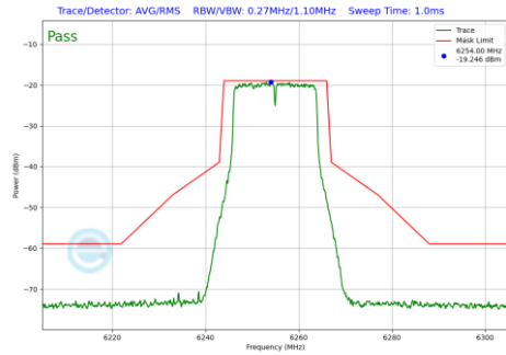
Plot 7-209 In-Band Emission Plot CDD Primary Antenna WF5B (20MHz BW 802.11a (UNII Band 5) - Ch.61)
