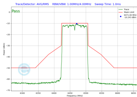
Plot 7-251 In-Band Emission Plot SDM Diversity Antenna WF8 (80MHz BW 802.11be(SU) (UNII Band 6) - Ch.103)
