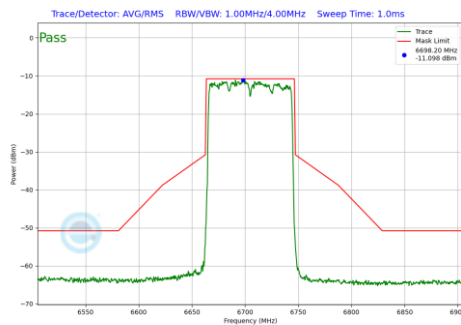
Plot 7-259 In-Band Emission Plot SDM Diversity Antenna WF8 (80MHz BW 802.11be(SU) (UNII Band 7) - Ch.151)
