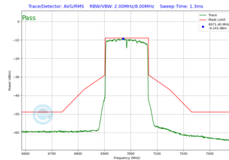
Plot 7-272 In-Band Emission Plot SDM Diversity Antenna WF7 (160MHz BW 802.11be(SU) (UNII Band 8) - Ch.207)
