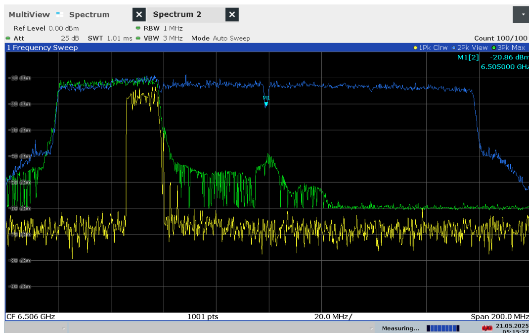
Plot 7-306. 160MHz Bandwidth, AWGN Signal Injected – 6505MHz
