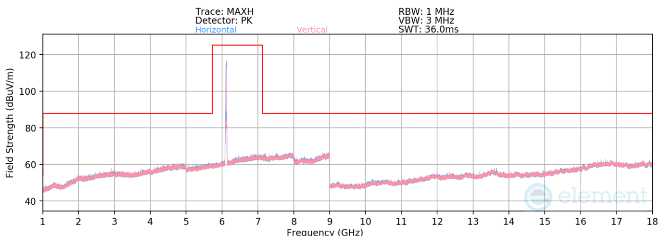
Plot 7-310. Radiated Spurious Emissions 1-18GHz SDM Primary (802.11be – Ch. 33)
