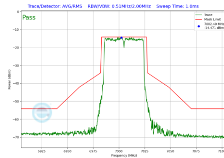
Plot 7-238 In-Band Emission Plot SDM Primary Antenna WF8 (40MHz BW 802.11be(SU) (UNII Band 8) - Ch.211)
