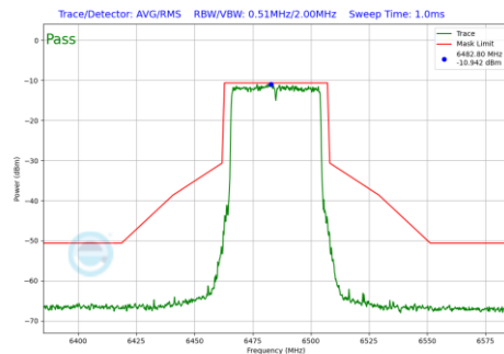
Plot 7-198 In-Band Emission Plot Antenna WF7 (40MHz BW 802.11be(SU) (UNII Band 6) - Ch.107)
