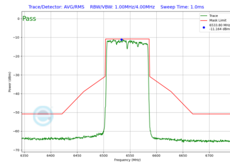
Plot 7-231 In-Band Emission Plot SDM Primary Antenna WF8 (80MHz BW 802.11be(SU) (UNII Band 7) - Ch.119)
