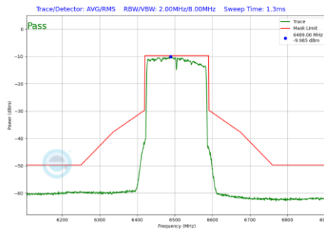
Plot 7-220 In-Band Emission Plot SDM Primary Antenna WF5B (160MHz BW 802.11be(SU) (UNII Band 6) - Ch.111)
