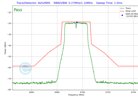
Plot 7-261 In-Band Emission Plot CDD Diversity Antenna WF7 (20MHz BW 802.11a (UNII Band 7) - Ch.149)
