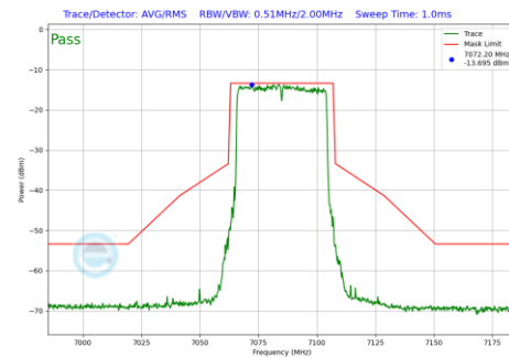
Plot 7-270 In-Band Emission Plot SDM Diversity Antenna WF7 (40MHz BW 802.11be(SU) (UNII Band 8) - Ch.227)
