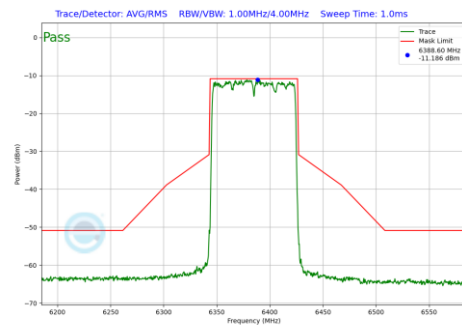
Plot 7-247 In-Band Emission Plot SDM Diversity Antenna WF7 (80MHz BW 802.11be(SU) (UNII Band 5) - Ch.87)
