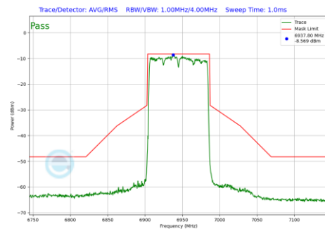
Plot 7-175 In-Band Emission Plot Antenna WF5B (80MHz BW 802.11be(SU) (UNII Band 8) - Ch.199)
