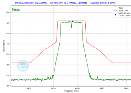
Plot 7-217 In-Band Emission Plot CDD Primary Antenna WF5B (20MHz BW 802.11a (UNII Band 6) - Ch.97)
