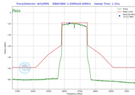
Plot 7-264 In-Band Emission Plot SDM Diversity Antenna WF7 (160MHz BW 802.11be(SU) (UNII Band 7) - Ch.143)
