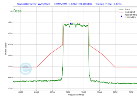
Plot 7-239 In-Band Emission Plot SDM Primary Antenna WF8 (80MHz BW 802.11be(SU) (UNII Band 8) - Ch.215)
