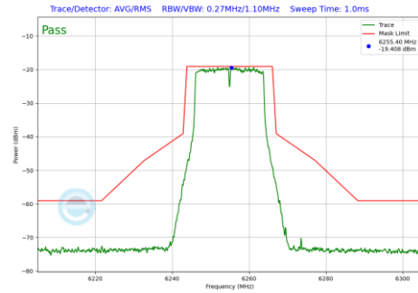
Plot 7-213 In-Band Emission Plot CDD Primary Antenna WF8 (20MHz BW 802.11a (UNII Band 5) - Ch.61)
