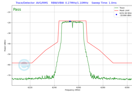
Plot 7-245 In-Band Emission Plot CDD Diversity Antenna WF7 (20MHz BW 802.11a (UNII Band 5) - Ch.61)
