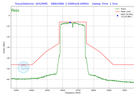
Plot 7-204 In-Band Emission Plot Antenna WF7 (160MHz BW 802.11be(SU) (UNII Band 7) - Ch.143)
