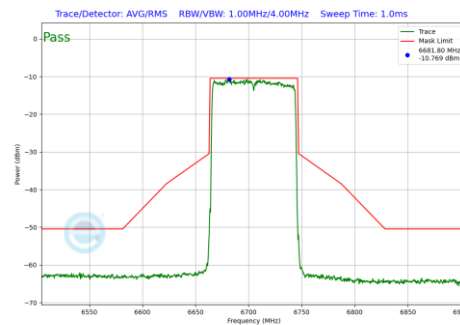
Plot 7-263 In-Band Emission Plot SDM Diversity Antenna WF7 (80MHz BW 802.11be(SU) (UNII Band 7) - Ch.151)
