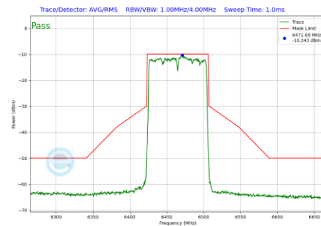
Plot 7-223 In-Band Emission Plot SDM Primary Antenna WF8 (80MHz BW 802.11be(SU) (UNII Band 6) - Ch.103)
