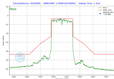
Plot 7-472 In-Band Emission Plot SDM Diversity Antenna WF8 (160MHz BW 802.11be(SU) (UNII Band 7) - Ch.143)
