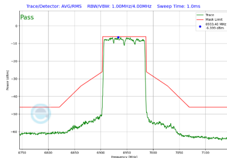
Plot 7-459 In-Band Emission Plot SDM Diversity Antenna WF7 (80MHz BW 802.11be(SU) (UNII Band 8) - Ch.199)
