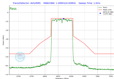
Plot 7-471 In-Band Emission Plot SDM Diversity Antenna WF8 (80MHz BW 802.11be(SU) (UNII Band 7) - Ch.183)
