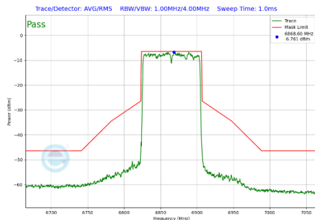
Plot 7-455 In-Band Emission Plot SDM Diversity Antenna WF7 (80MHz BW 802.11be(SU) (UNII Band 7) - Ch.183)
