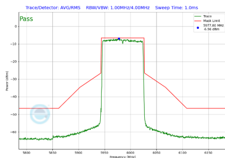
Plot 7-463 In-Band Emission Plot SDM Diversity Antenna WF8 (80MHz BW 802.11be(SU) (UNII Band 5) - Ch.7)
