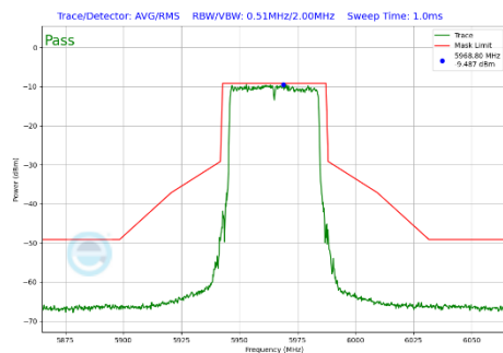
Plot 7-462 In-Band Emission Plot SDM Diversity Antenna WF8 (40MHz BW 802.11be(SU) (UNII Band 5) - Ch.3)
