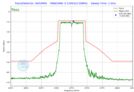
Plot 7-470 In-Band Emission Plot SDM Diversity Antenna WF8 (40MHz BW 802.11be(SU) (UNII Band 7) - Ch.155)
