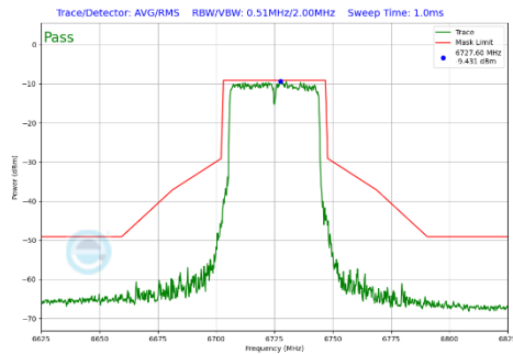
Plot 7-454 In-Band Emission Plot SDM Diversity Antenna WF7 (40MHz BW 802.11be(SU) (UNII Band 7) - Ch.155)
