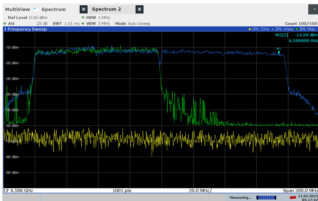
Plot 7-511. 160MHz Bandwidth, AWGN Signal Injected – 6580MHz
