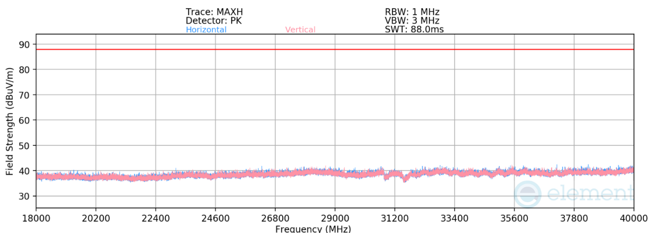
Plot 7-542. Radiated Spurious Emissions 18-40GHz SDM Diversity (802.11be – Ch. 209)
