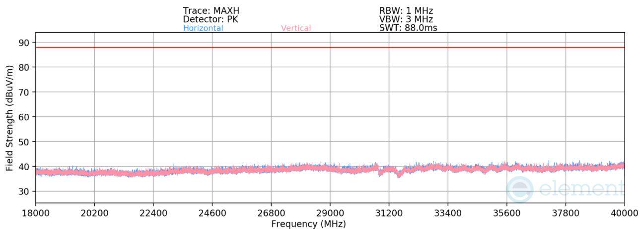
Plot 7-530. Radiated Spurious Emissions 18-40GHz CDD Diversity (802.11be – Ch. 45)
