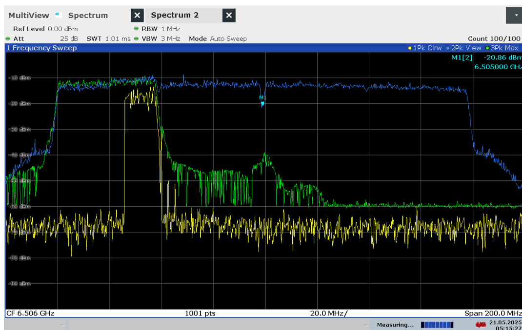
Plot 7-510. 160MHz Bandwidth, AWGN Signal Injected – 6505MHz
