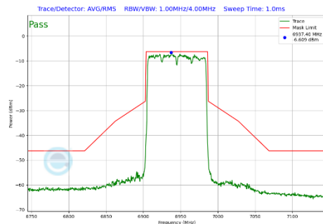
Plot 7-475 In-Band Emission Plot SDM Diversity Antenna WF8 (80MHz BW 802.11be(SU) (UNII Band 8) - Ch.199)
