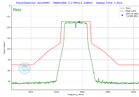
Plot 7-461 In-Band Emission Plot CDD Diversity Antenna WF8 (20MHz BW 802.11a (UNII Band 5) - Ch.1)
