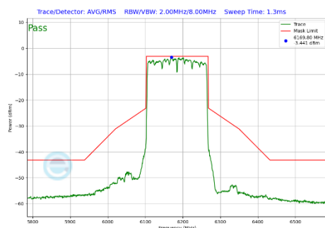
Plot 7-464 In-Band Emission Plot SDM Diversity Antenna WF8 (160MHz BW 802.11be(SU) (UNII Band 5) - Ch.47)
