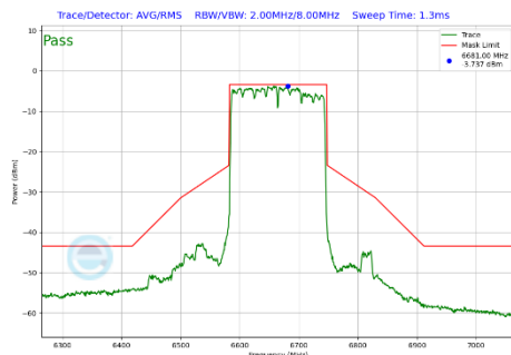
Plot 7-456 In-Band Emission Plot SDM Diversity Antenna WF7 (160MHz BW 802.11be(SU) (UNII Band 7) - Ch.143)
