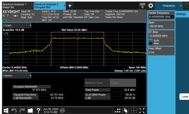
Plot 7-20 26dB BW & 99% OBW Antenna WF5B (40MHz BW 802.11be(RU) RU484 Index65 - Ch.99)
