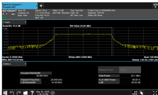
Plot 7-42 26dB BW & 99% OBW Antenna WF5B (40MHz BW 802.11be(RU) RU484 Index65 - Ch.43)
