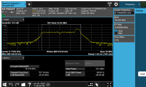
Plot 7-1 26dB BW & 99% OBW Antenna WF5B (20MHz BW 802.11be(RU) RU26 Index8 - Ch.45)
