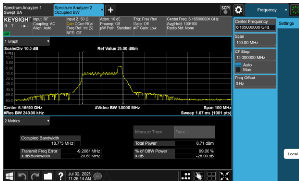
Plot 7-35 26dB BW & 99% OBW Antenna WF5B (40MHz BW 802.11be(RU) RU26 Index8 - Ch.43)
