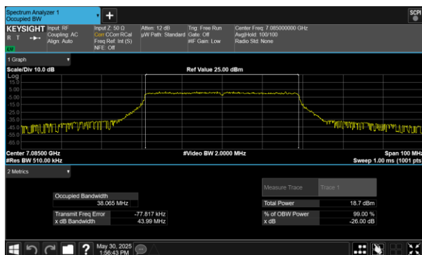
Plot 7-75 26dB BW & 99% OBW Antenna WF5B (40MHz BW 802.11be(RU) RU484 Index65 - Ch.227)
