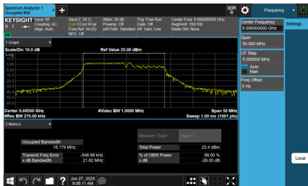
Plot 7-27 26dB BW & 99% OBW Antenna WF5B (20MHz BW 802.11be(RU) RU106+26 Index82 - Ch.149)
