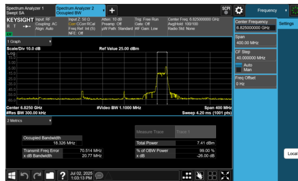
Plot 7-59 26dB BW & 99% OBW Antenna WF5B (160MHz BW 802.11be(RU) RU26 Index36 - Ch.175)
