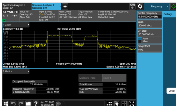
Plot 7-28 26dB BW & 99% OBW Antenna WF5B (80MHz BW 802.11be(RU) RU484+242 Index92 - Ch.119)
