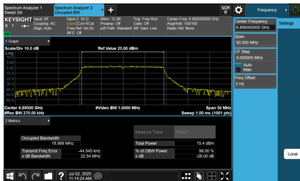
Plot 7-74 26dB BW & 99% OBW Antenna WF5B (20MHz BW 802.11be(RU) RU242 Index61 - Ch.189)
