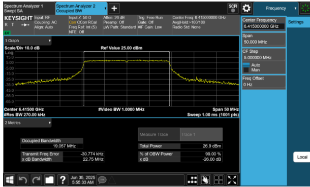
Plot 7-8 26dB BW & 99% OBW Antenna WF5B (20MHz BW 802.11be(RU) RU242 Index61 - Ch.93)
