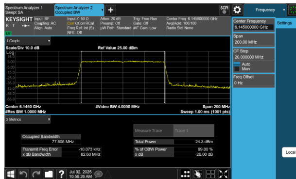
Plot 7-43 26dB BW & 99% OBW Antenna WF5B (80MHz BW 802.11be(RU) RU996 Index67 - Ch.39)
