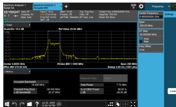
Plot 7-58 26dB BW & 99% OBW Antenna WF5B (80MHz BW 802.11be(RU) RU26 Index0 - Ch.183)
