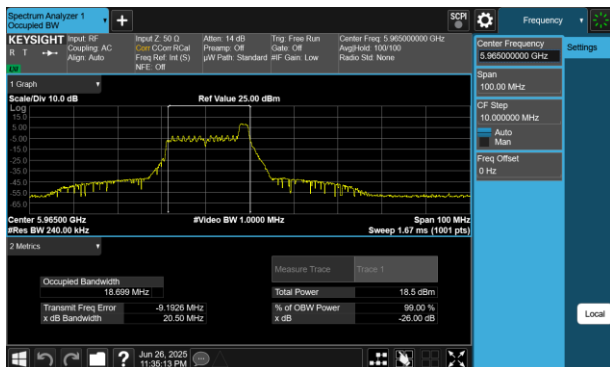
Plot 7-2 26dB BW & 99% OBW Antenna WF5B (40MHz BW 802.11be(RU) RU26 Index8 - Ch.3)
