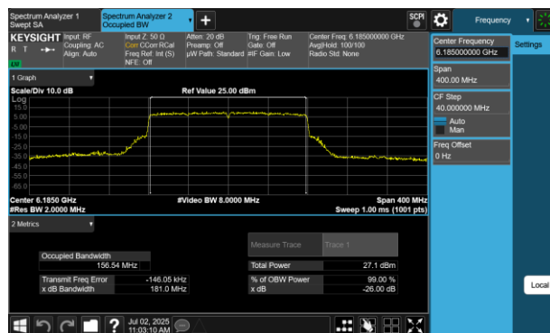
Plot 7-44 26dB BW & 99% OBW Antenna WF5B (160MHz BW 802.11be(RU) RU996X2 Index68 - Ch.47)
