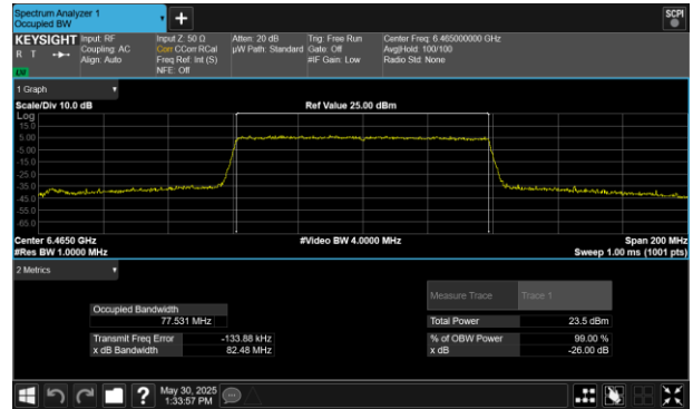
Plot 7-54 26dB BW & 99% OBW Antenna WF5B (80MHz BW 802.11be(RU) RU996 Index67 - Ch.103)
