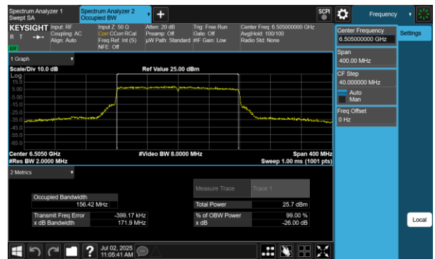
Plot 7-55 26dB BW & 99% OBW Antenna WF5B (160MHz BW 802.11be(RU) RU996X2 Index68 - Ch.111)
