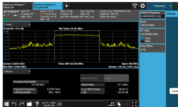
Plot 7-29 26dB BW & 99% OBW Antenna WF5B (160MHz BW 802.11be(RU) RU996+484+242 Index96 - Ch.143)
