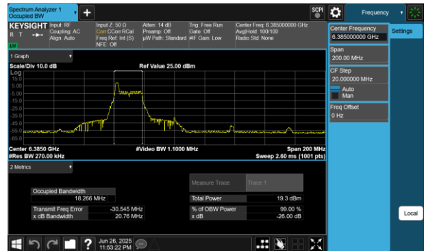
Plot 7-3 26dB BW & 99% OBW Antenna WF5B (80MHz BW 802.11be(RU) RU26 Index0 - Ch.87)
