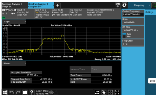
Plot 7-46 26dB BW & 99% OBW Antenna WF5B (40MHz BW 802.11be(RU) RU26 Index8 - Ch.107)
