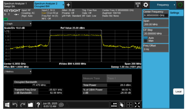
Plot 7-10 26dB BW & 99% OBW Antenna WF5B (80MHz BW 802.11be(RU) RU996 Index67 - Ch.87)
