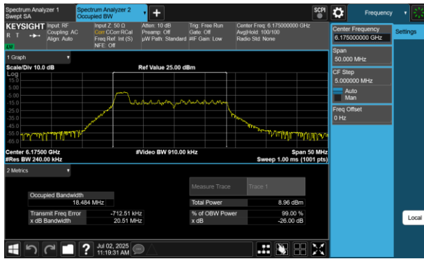
Plot 7-34 26dB BW & 99% OBW Antenna WF5B (20MHz BW 802.11be(RU) RU26 Index0 - Ch.45)
