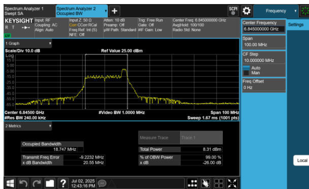
Plot 7-57 26dB BW & 99% OBW Antenna WF5B (40MHz BW 802.11be(RU) RU26 Index8 - Ch.179)
