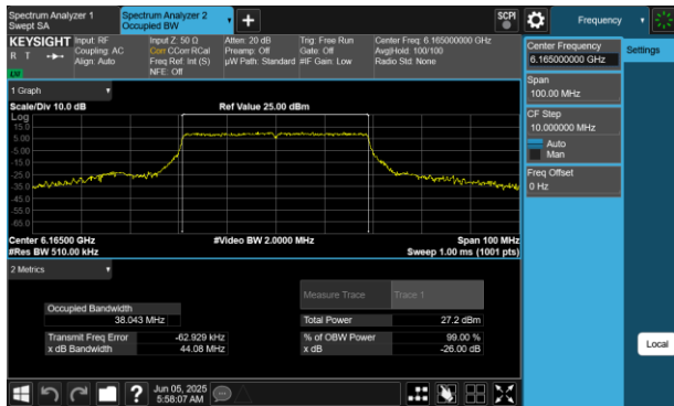
Plot 7-9 26dB BW & 99% OBW Antenna WF5B (40MHz BW 802.11be(RU) RU484 Index65 - Ch.43)
