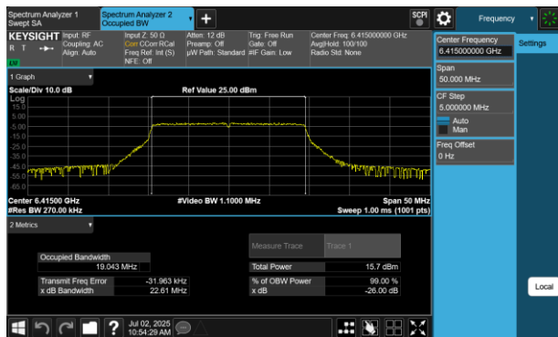
Plot 7-41 26dB BW & 99% OBW Antenna WF5B (20MHz BW 802.11be(RU) RU242 Index61 - Ch.93)
