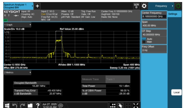
Plot 7-4 26dB BW & 99% OBW Antenna WF5B (160MHz BW 802.11be(RU) RU26 Index17 - Ch.47)
