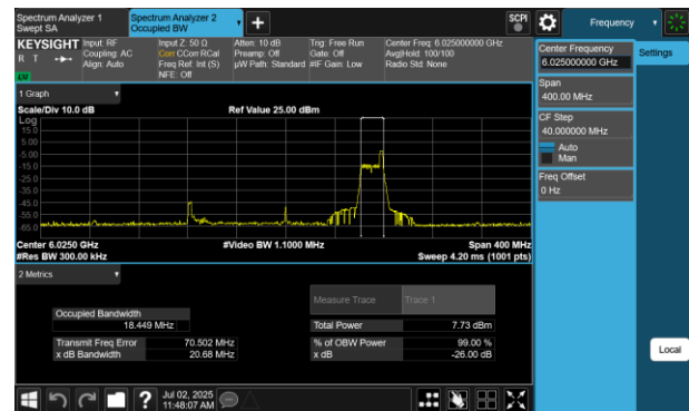
Plot 7-37 26dB BW & 99% OBW Antenna WF5B (160MHz BW 802.11be(RU) RU26 Index36 - Ch.15)
