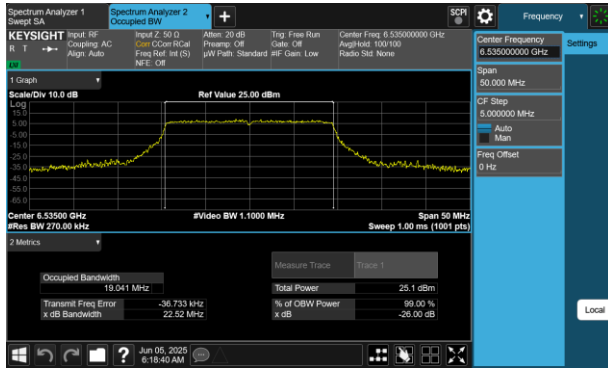
Plot 7-30 26dB BW & 99% OBW Antenna WF5B (20MHz BW 802.11be(RU) RU242 Index61 - Ch.117)
