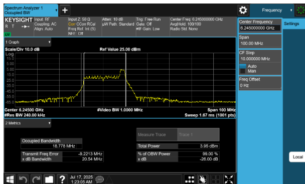
Plot 7-46 26dB BW & 99% OBW Antenna WF8 (40MHz BW 802.11be(RU) RU26 Index8 - Ch.59)
