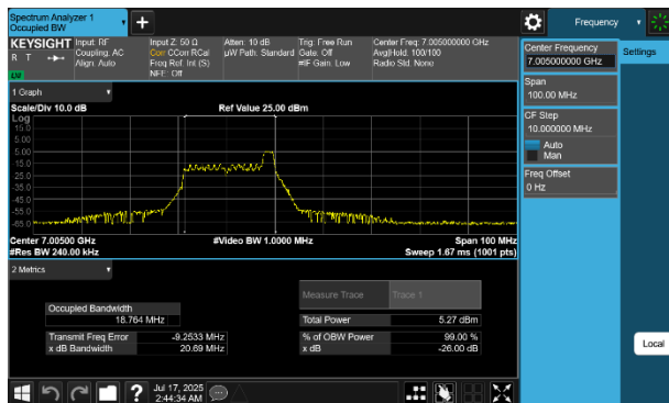
Plot 7-79 26dB BW & 99% OBW Antenna WF8 (40MHz BW 802.11be(RU) RU26 Index8 - Ch.211)
