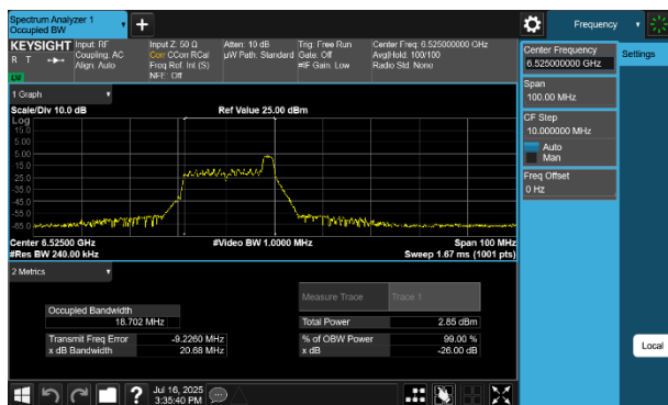
Plot 7-13 26dB BW & 99% OBW Antenna WF5B (40MHz BW 802.11be(RU) RU26 Index8 - Ch.115)
