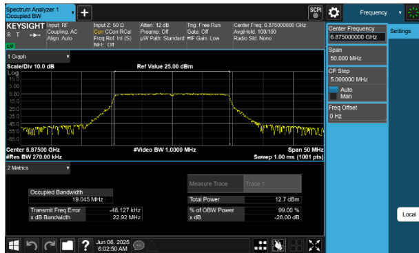
Plot 7-74 26dB BW & 99% OBW Antenna WF8 (20MHz BW 802.11be(RU) RU242 Index61 - Ch.185)
