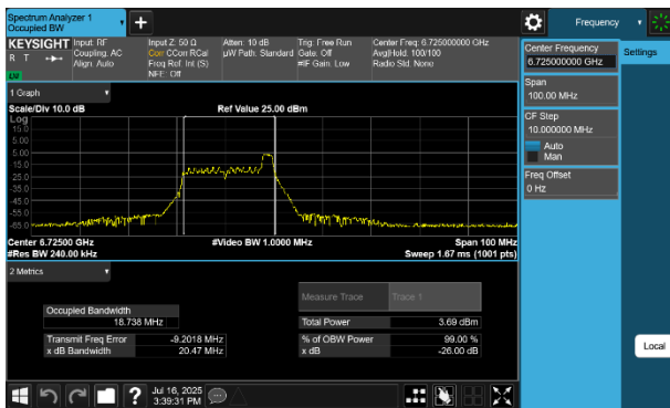
Plot 7-24 26dB BW & 99% OBW Antenna WF5B (40MHz BW 802.11be(RU) RU26 Index8 - Ch.155)
