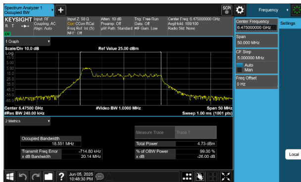
Plot 7-12 26dB BW & 99% OBW Antenna WF5B (20MHz BW 802.11be(RU) RU26 Index0 - Ch.105)
