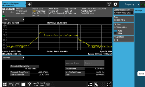
Plot 7-45 26dB BW & 99% OBW Antenna WF8 (20MHz BW 802.11be(RU) RU26 Index0 - Ch.93)
