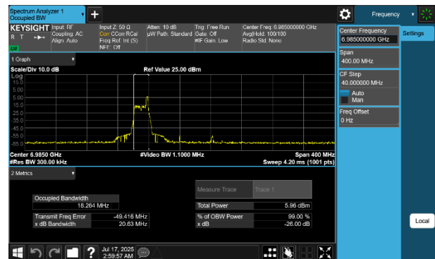
Plot 7-81 26dB BW & 99% OBW Antenna WF8 (160MHz BW 802.11be(RU) RU26 Index17 - Ch.207)
