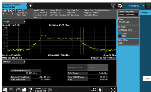
Plot 7-67 26dB BW & 99% OBW Antenna WF8 (20MHz BW 802.11be(RU) RU26 Index0 - Ch.149)
