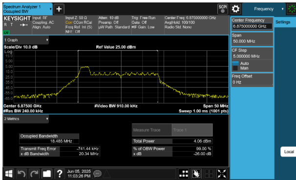
Plot 7-23 26dB BW & 99% OBW Antenna WF5B (20MHz BW 802.11be(RU) RU26 Index0 - Ch.185)
