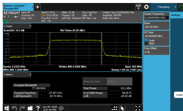
Plot 7-10 26dB BW & 99% OBW Antenna WF5B (80MHz BW 802.11be(RU) RU996 Index67 - Ch.55)
