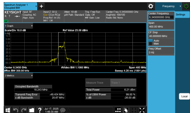
Plot 7-48 26dB BW & 99% OBW Antenna WF8 (160MHz BW 802.11be(RU) RU26 Index17 - Ch.79)
