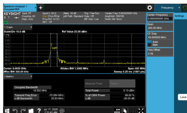
Plot 7-70 26dB BW & 99% OBW Antenna WF8 (160MHz BW 802.11be(RU) RU26 Index0 - Ch.143)
