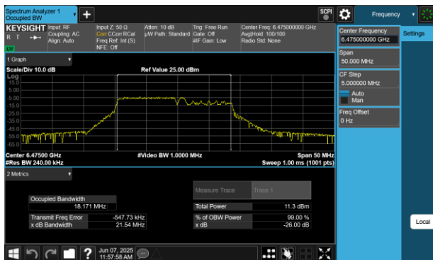
Plot 7-60 26dB BW & 99% OBW Antenna WF8 (20MHz BW 802.11be(RU) RU106+26 Index82 - Ch.105)
