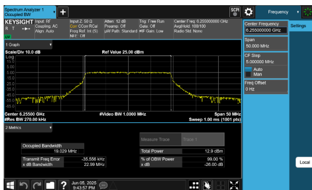
Plot 7-8 26dB BW & 99% OBW Antenna WF5B (20MHz BW 802.11be(RU) RU242 Index61 - Ch.61)
