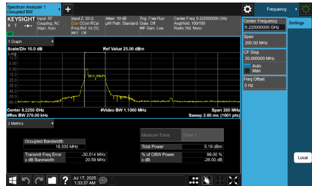
Plot 7-47 26dB BW & 99% OBW Antenna WF8 (80MHz BW 802.11be(RU) RU26 Index0 - Ch.55)
