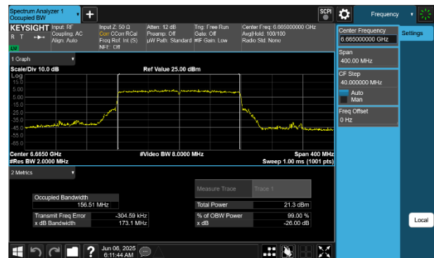
Plot 7-77 26dB BW & 99% OBW Antenna WF8 (160MHz BW 802.11be(RU) RU996X2 Index68 - Ch.143)
