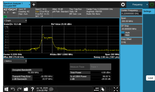
Plot 7-3 26dB BW & 99% OBW Antenna WF5B (80MHz BW 802.11be(RU) RU26 Index0 - Ch.55)
