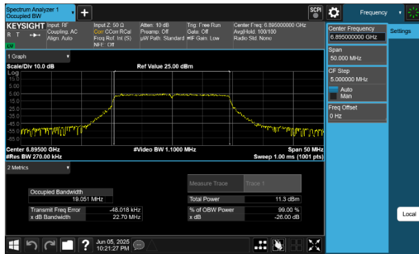
Plot 7-41 26dB BW & 99% OBW Antenna WF5B (20MHz BW 802.11be(RU) RU242 Index61 - Ch.189)
