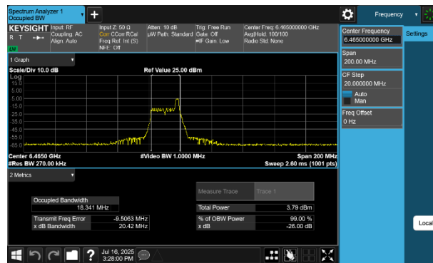
Plot 7-14 26dB BW & 99% OBW Antenna WF5B (80MHz BW 802.11be(RU) RU26 Index17 - Ch.103)
