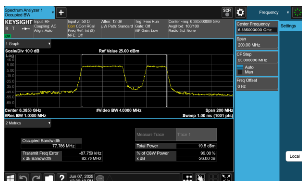
Plot 7-50 26dB BW & 99% OBW Antenna WF8 (80MHz BW 802.11be(RU) RU484+242 Index92 - Ch.87)
