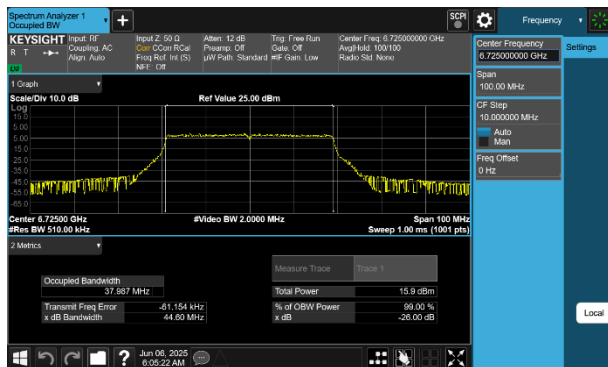
Plot 7-75 26dB BW & 99% OBW Antenna WF8 (40MHz BW 802.11be(RU) RU484 Index65 - Ch.155)
