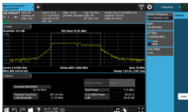
Plot 7-49 26dB BW & 99% OBW Antenna WF8 (20MHz BW 802.11be(RU) RU106+26 Index82 - Ch.93)
