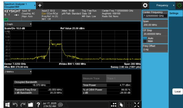
Plot 7-80 26dB BW & 99% OBW Antenna WF8 (80MHz BW 802.11be(RU) RU26 Index0 - Ch.215)
