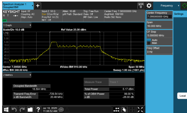
Plot 7-78 26dB BW & 99% OBW Antenna WF8 (20MHz BW 802.11be(RU) RU26 Index0 - Ch.229)
