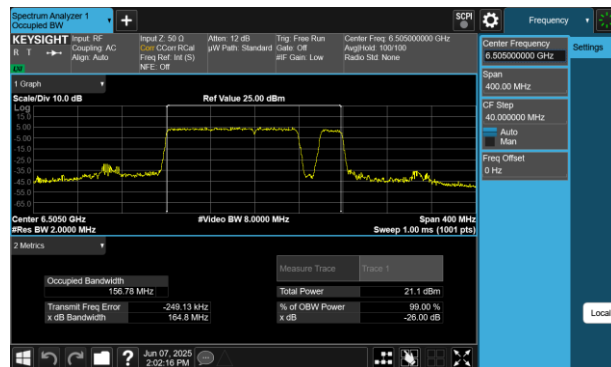
Plot 7-62 26dB BW & 99% OBW Antenna WF8 (160MHz BW 802.11be(RU) RU996+484+242 Index98 - Ch.111)
