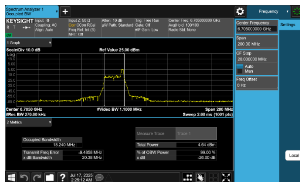
Plot 7-69 26dB BW & 99% OBW Antenna WF8 (80MHz BW 802.11be(RU) RU26 Index17 - Ch.151)
