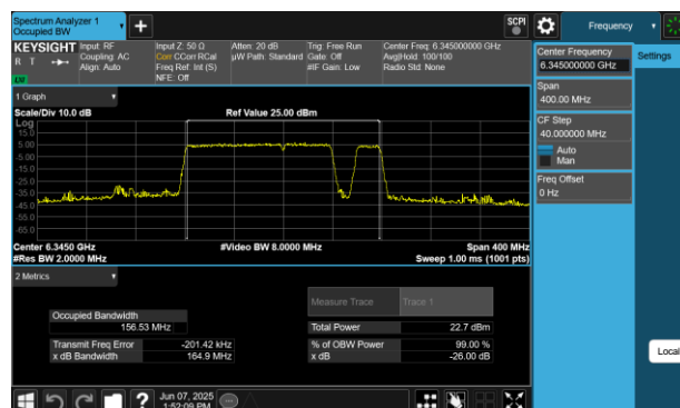
Plot 7-51 26dB BW & 99% OBW Antenna WF8 (160MHz BW 802.11be(RU) RU996+484+242 Index98 - Ch.79)
