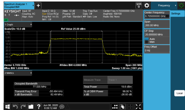
Plot 7-76 26dB BW & 99% OBW Antenna WF8 (80MHz BW 802.11be(RU) RU996 Index67 - Ch.151)
