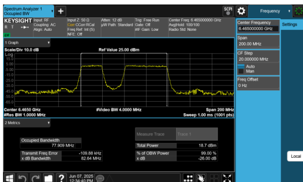
Plot 7-61 26dB BW & 99% OBW Antenna WF8 (80MHz BW 802.11be(RU) RU484+242 Index91 - Ch.103)
