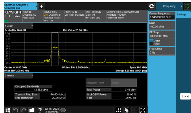
Plot 7-4 26dB BW & 99% OBW Antenna WF5B (160MHz BW 802.11be(RU) RU26 Index0 - Ch.79)
