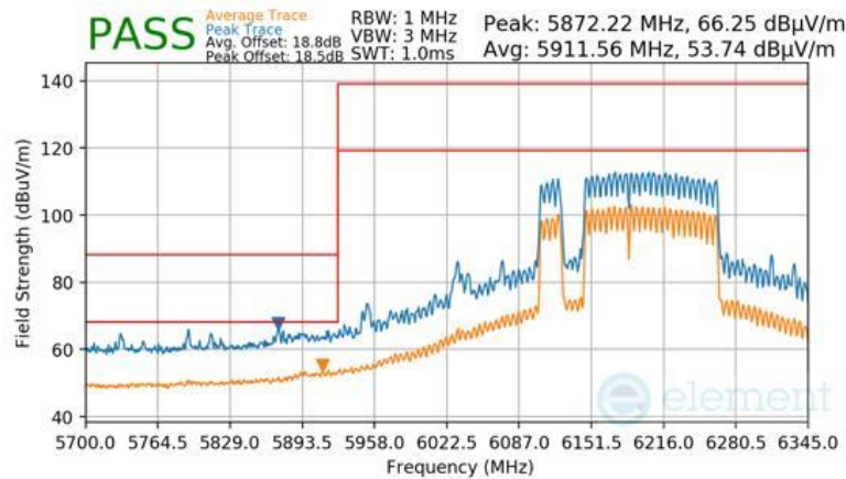
Plot 7-1075 SDM Primary Radiated Lower Band Edge (Peak & Average – UNII Band 5) - RU996+484+242 (L)
