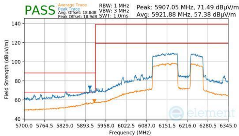
Plot 7-1006 Antenna WF7 Radiated Lower Band Edge (Peak & Average – UNII Band 5) - RU996+484 (H)
