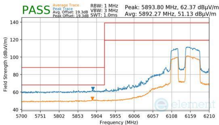
Plot 7-992 Antenna WF7 Radiated Lower Band Edge (Peak & Average – UNII Band 5) - RU484+242
