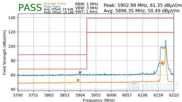
Plot 7-988 Antenna WF7 Radiated Lower Band Edge (Peak & Average – UNII Band 5) - RU26
