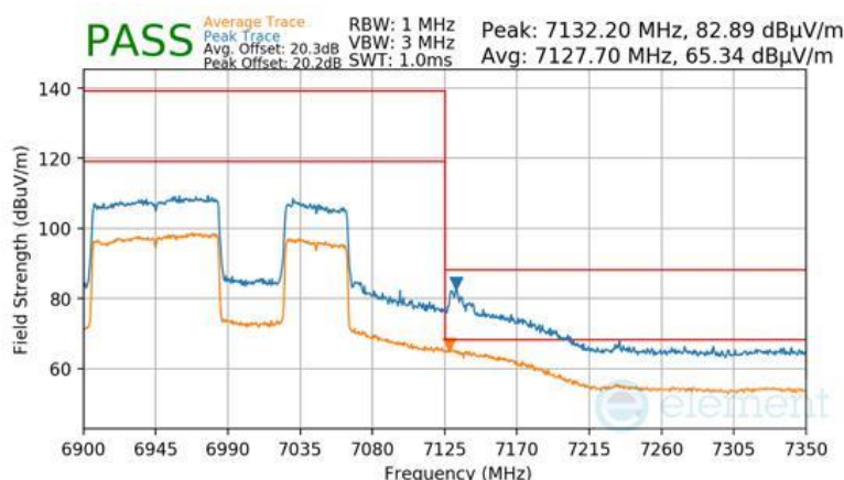
Plot 7-1010 Antenna WF7 Radiated Upper Band Edge (Peak & Average – UNII Band 8) - RU996+484 (H)
