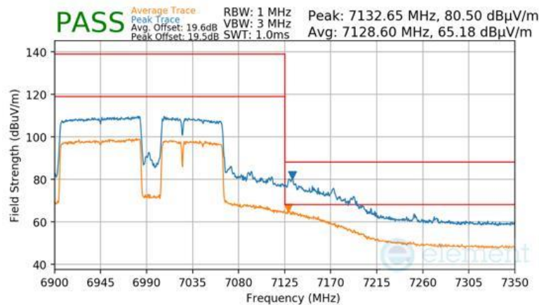
Plot 7-961 Antenna WF8 Radiated Upper Band Edge (Peak & Average – UNII Band 8) - RU996+484+242 (H)
