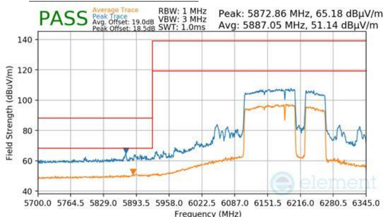
Plot 7-956 Antenna WF8 Radiated Lower Band Edge (Peak & Average – UNII Band 5) - RU996+484+242 (H)
