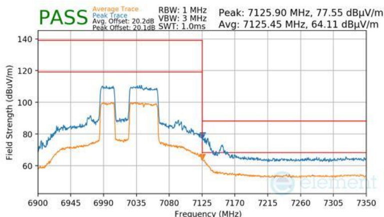
Plot 7-996 Antenna WF7 Radiated Upper Band Edge (Peak & Average – UNII Band 8) - RU484+242
