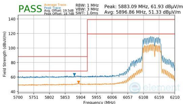
Plot 7-1054 SDM Primary Radiated Lower Band Edge (Peak & Average – UNII Band 5) - RU484+242
