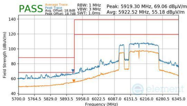
Plot 7-1015 Antenna WF7 Radiated Lower Band Edge (Peak & Average – UNII Band 5) - RU996+484+242 (L)
