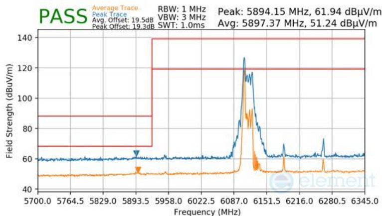
Plot 7-1061 SDM Primary Radiated Lower Band Edge (Peak & Average – UNII Band 5) - RU26
