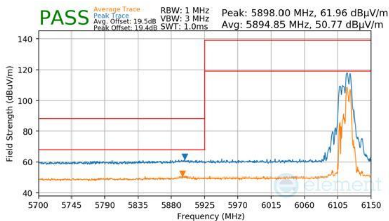
Plot 7-1036 SDM Primary Radiated Lower Band Edge (Peak & Average – UNII Band 5) - RU52+26
