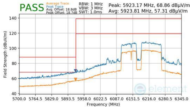
Plot 7-1019 Antenna WF7 Radiated Lower Band Edge (Peak & Average – UNII Band 5) - RU996+484+242 (L)
