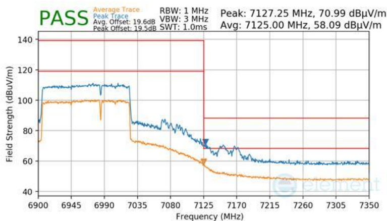
Plot 7-951 Antenna WF8 Radiated Upper Band Edge (Peak & Average – UNII Band 8) - RU996+484 (H)
