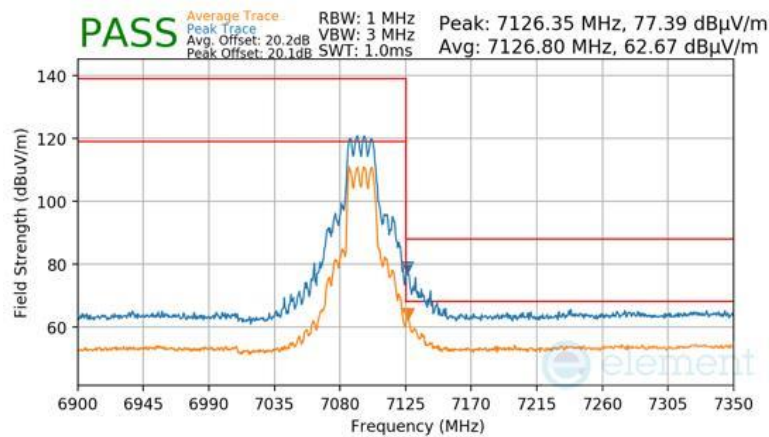
Plot 7-1040 SDM Primary Radiated Upper Band Edge (Peak & Average – UNII Band 8) - RU242
