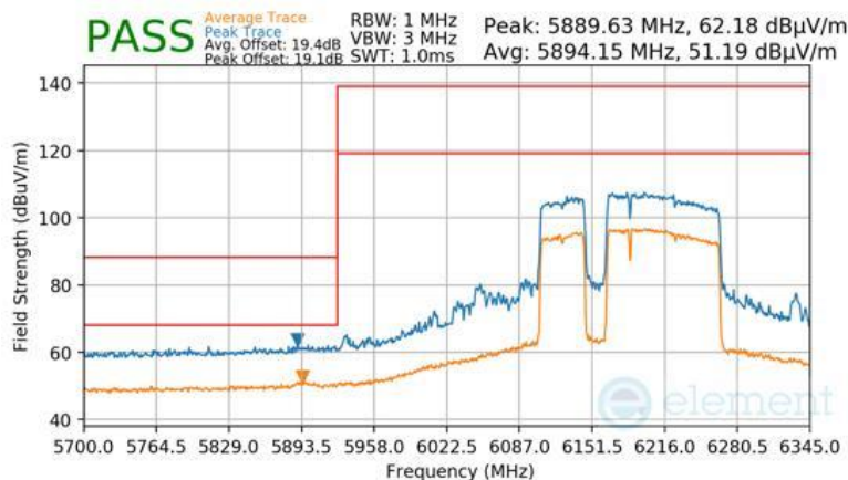
Plot 7-957 Antenna WF8 Radiated Lower Band Edge (Peak & Average – UNII Band 5) - RU996+484+242 (L)
