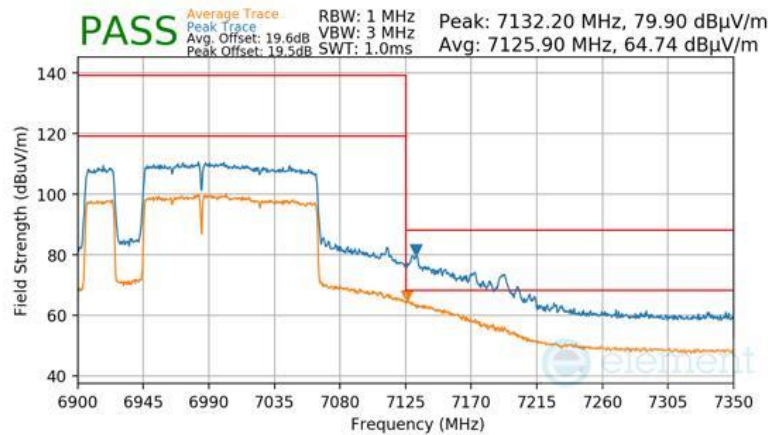
Plot 7-963 Antenna WF8 Radiated Upper Band Edge (Peak & Average – UNII Band 8) - RU996+484+242 (L)
