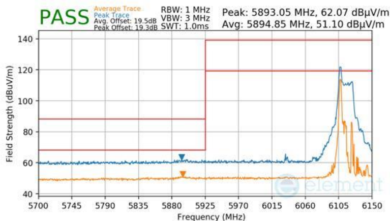
Plot 7-981 Antenna WF7 Radiated Lower Band Edge (Peak & Average – UNII Band 5) - RU26
