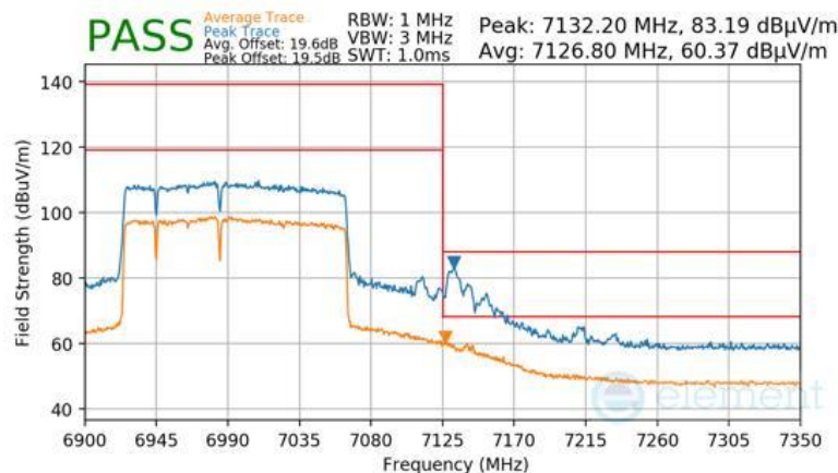
Plot 7-962 Antenna WF8 Radiated Upper Band Edge (Peak & Average – UNII Band 8) - RU996+484+242 (L)
