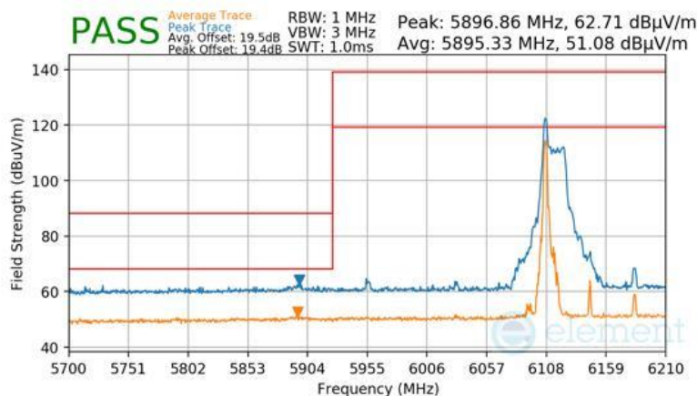
Plot 7-987 Antenna WF7 Radiated Lower Band Edge (Peak & Average – UNII Band 5) - RU26
