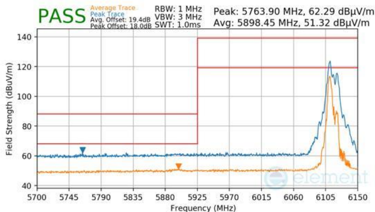
Plot 7-1035 SDM Primary Radiated Lower Band Edge (Peak & Average – UNII Band 5) - RU52+26
