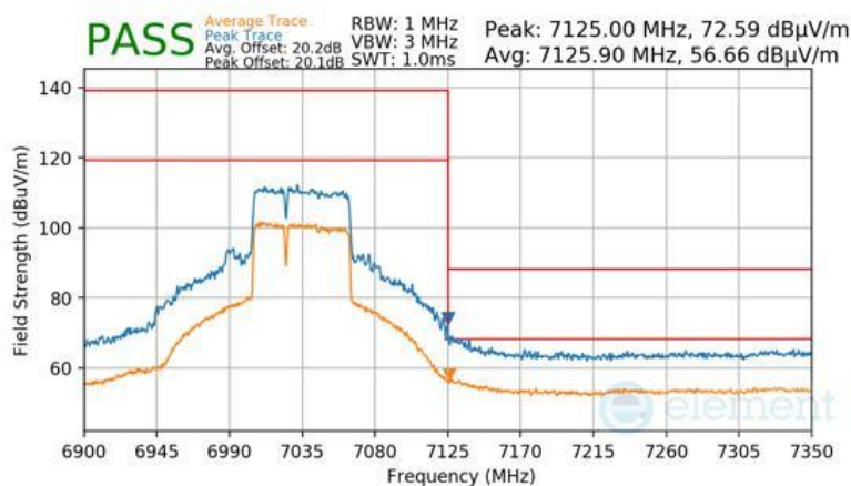
Plot 7-995 Antenna WF7 Radiated Upper Band Edge (Peak & Average – UNII Band 8) - RU484+242
