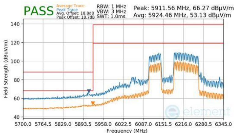
Plot 7-1067 SDM Primary Radiated Lower Band Edge (Peak & Average – UNII Band 5) - RU996+484 (L)
