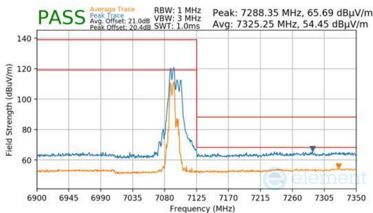
Plot 7-1097 SDM Diversity Radiated Upper Band Edge (Peak & Average – UNII Band 8) - RU52+26
