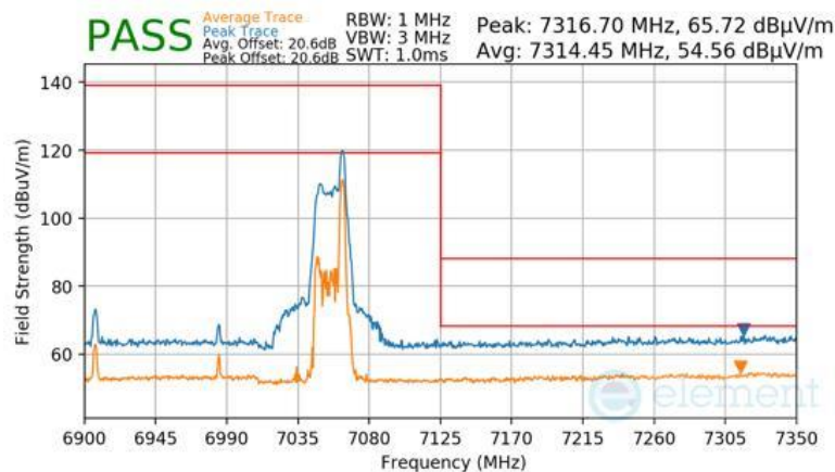
Plot 7-1004 Antenna WF7 Radiated Upper Band Edge (Peak & Average – UNII Band 8) - RU26
