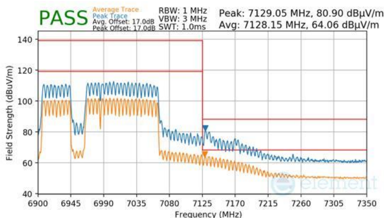
Plot 7-1085 SDM Primary Radiated Upper Band Edge (Peak & Average – UNII Band 8) - RU996+484+242 (L)
