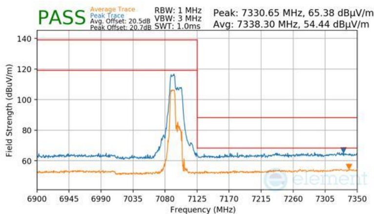
Plot 7-977 Antenna WF7 Radiated Upper Band Edge (Peak & Average – UNII Band 8) - RU52+26
