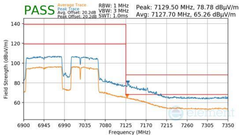
Plot 7-1021 Antenna WF7 Radiated Upper Band Edge (Peak & Average – UNII Band 8) - RU996+484+242 (H)
