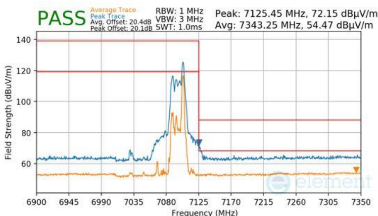
Plot 7-1044 SDM Primary Radiated Upper Band Edge (Peak & Average – UNII Band 8) - RU26
