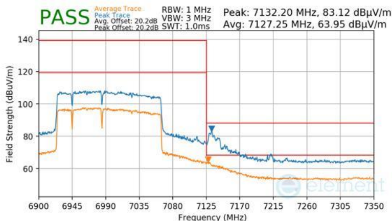
Plot 7-1022 Antenna WF7 Radiated Upper Band Edge (Peak & Average – UNII Band 8) - RU996+484+242 (L)
