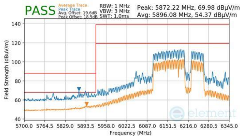
Plot 7-1076 SDM Primary Radiated Lower Band Edge (Peak & Average – UNII Band 5) - RU996+484+242 (H)
