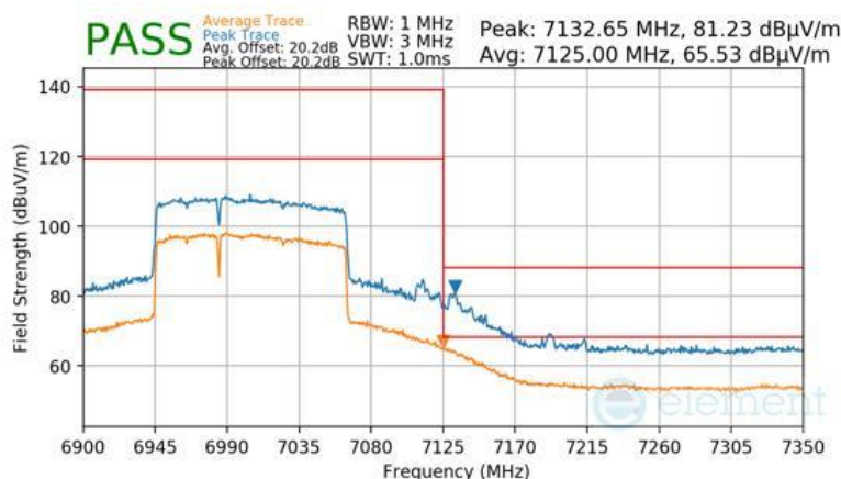
Plot 7-1009 Antenna WF7 Radiated Upper Band Edge (Peak & Average – UNII Band 8) - RU996+484 (L)
