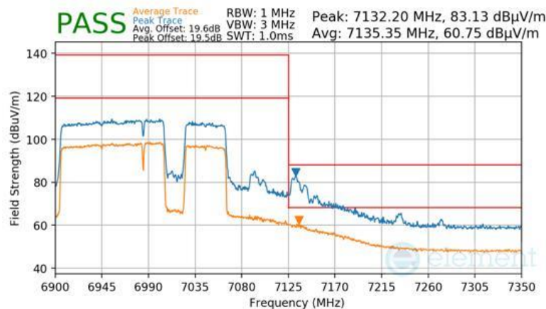
Plot 7-964 Antenna WF8 Radiated Upper Band Edge (Peak & Average – UNII Band 8) - RU996+484+242 (H)
