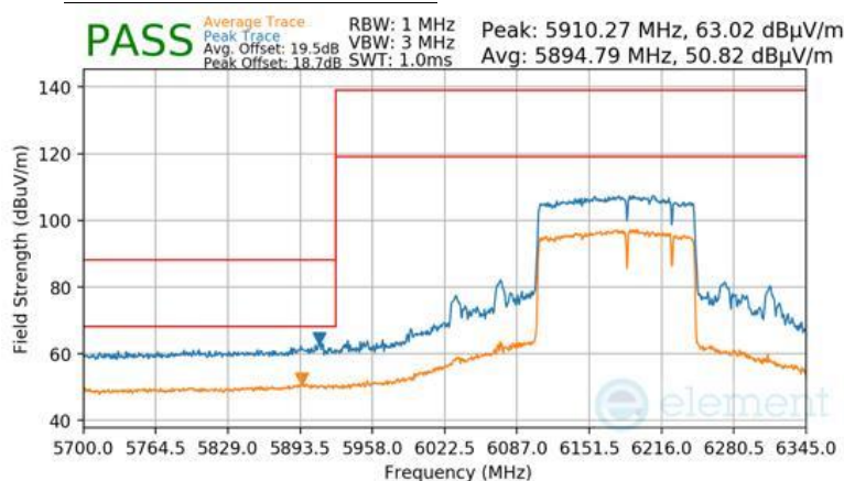
Plot 7-960 Antenna WF8 Radiated Lower Band Edge (Peak & Average – UNII Band 5) - RU996+484+242 (H)
