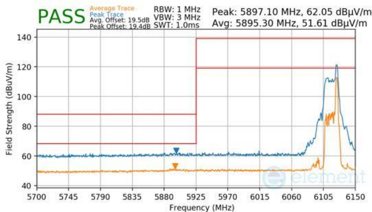
Plot 7-972 Antenna WF7 Radiated Lower Band Edge (Peak & Average – UNII Band 5) - RU26
