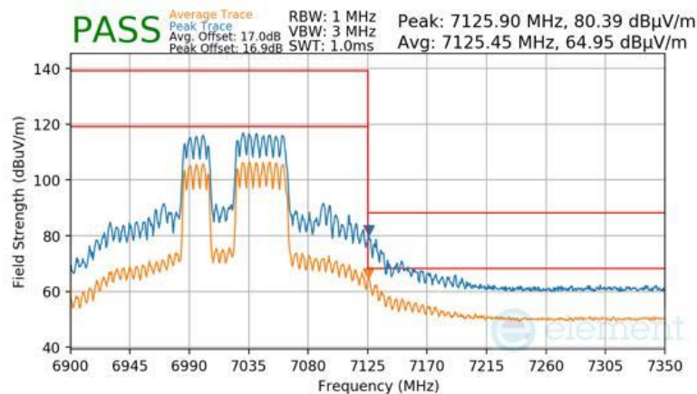
Plot 7-1056 SDM Primary Radiated Upper Band Edge (Peak & Average – UNII Band 8) - RU484+242
