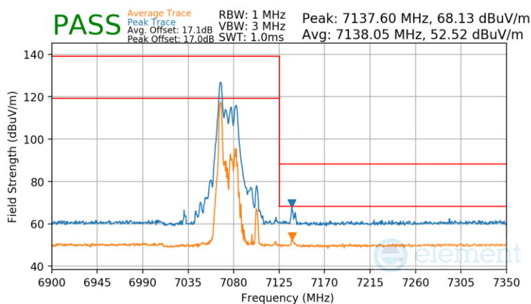
Plot 7-1043 SDM Primary Radiated Upper Band Edge (Peak & Average – UNII Band 8) - RU26
