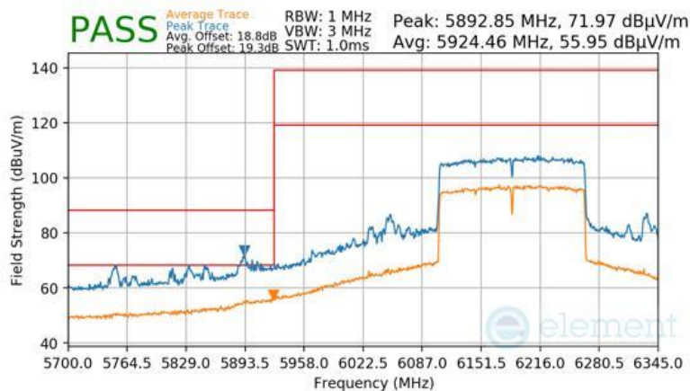
Plot 7-1029 Antenna WF7 Radiated Lower Band Edge (Peak & Average – UNII Band 5) - RU996X2
