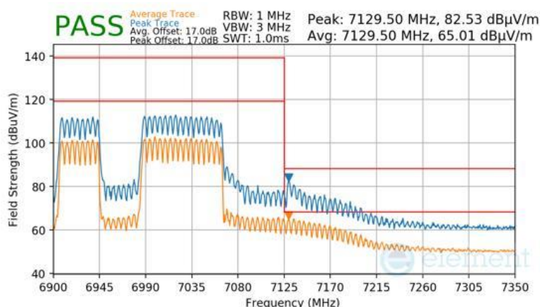
Plot 7-1072 SDM Primary Radiated Upper Band Edge (Peak & Average – UNII Band 8) - RU996+484 (L)
