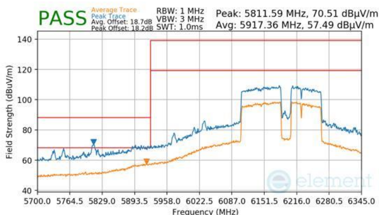
Plot 7-1014 Antenna WF7 Radiated Lower Band Edge (Peak & Average – UNII Band 5) - RU996+484+242 (H)
