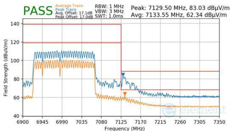
Plot 7-1082 SDM Primary Radiated Upper Band Edge (Peak & Average – UNII Band 8) - RU996+484+242 (L)
