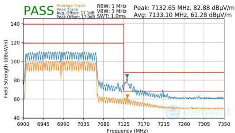
Plot 7-1090 SDM Primary Radiated Upper Band Edge (Peak & Average – UNII Band 8) - RU996X2
