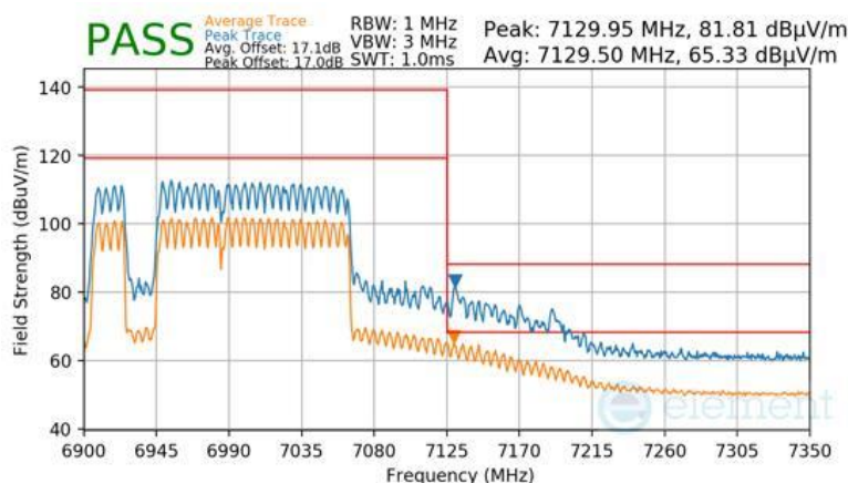
Plot 7-1083 SDM Primary Radiated Upper Band Edge (Peak & Average – UNII Band 8) - RU996+484+242 (L)
