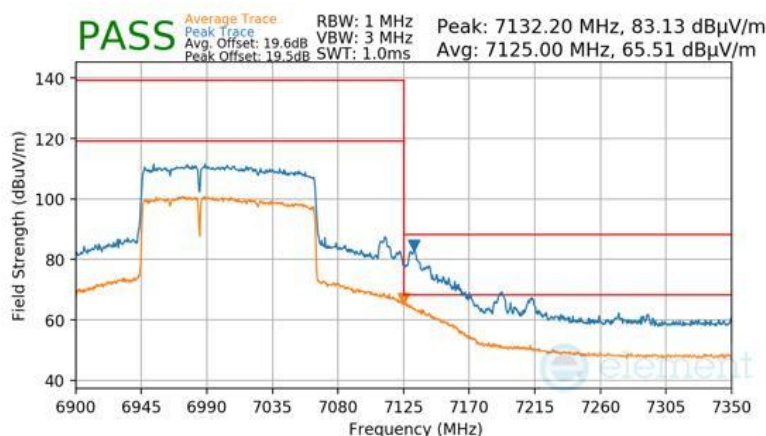
Plot 7-949 Antenna WF8 Radiated Upper Band Edge (Peak & Average – UNII Band 8) - RU996+484 (L)
