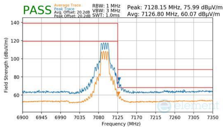
Plot 7-1100 SDM Diversity Radiated Upper Band Edge (Peak & Average – UNII Band 8) - RU242
