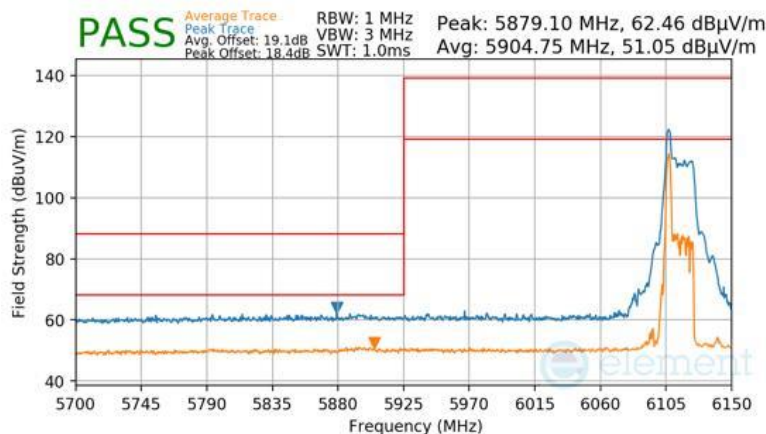
Plot 7-971 Antenna WF7 Radiated Lower Band Edge (Peak & Average – UNII Band 5) - RU26
