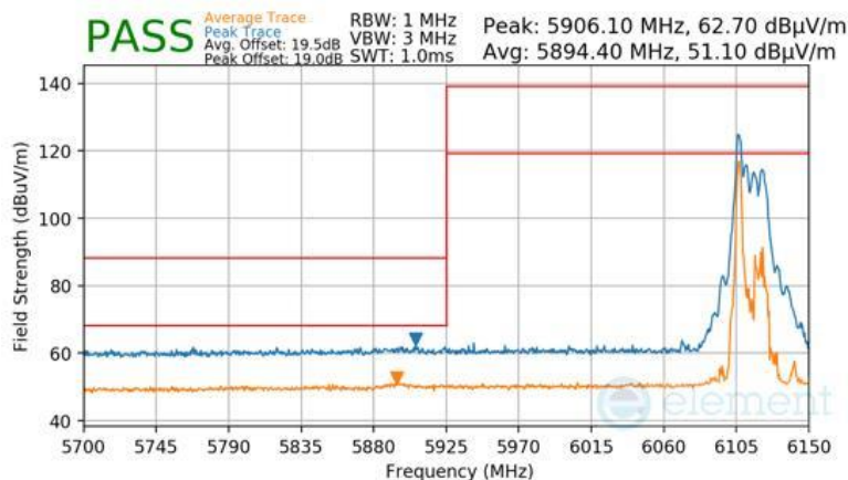
Plot 7-1031 SDM Primary Radiated Lower Band Edge (Peak & Average – UNII Band 5) - RU26
