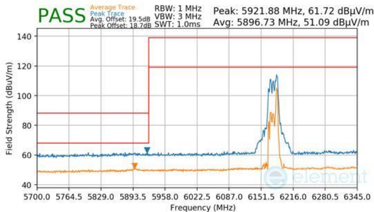
Plot 7-1062 SDM Primary Radiated Lower Band Edge (Peak & Average – UNII Band 5) - RU26
