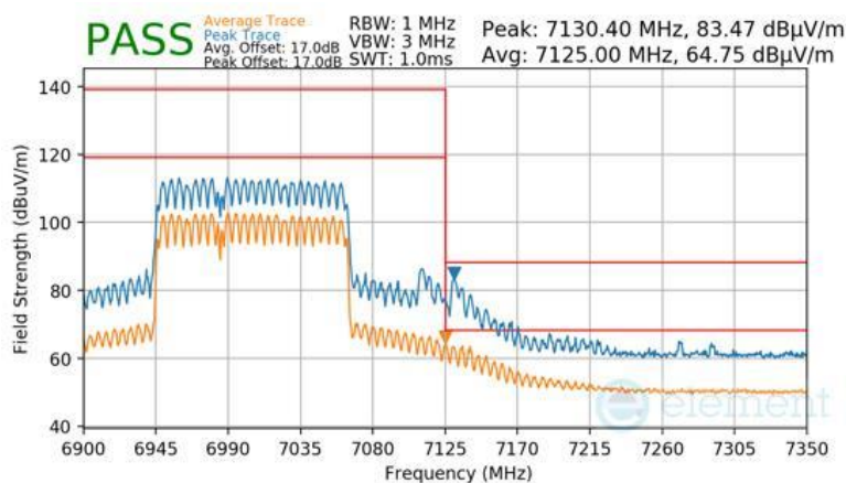
Plot 7-1069 SDM Primary Radiated Upper Band Edge (Peak & Average – UNII Band 8) - RU996+484 (L)
