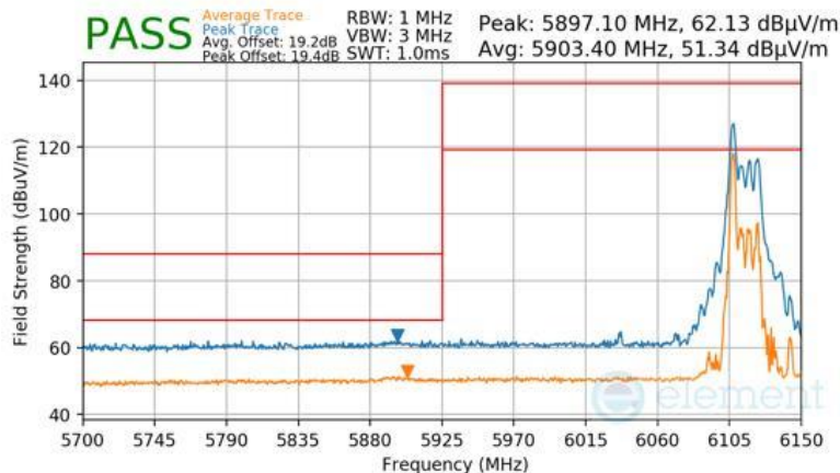
Plot 7-1101 SDM Diversity Radiated Lower Band Edge (Peak & Average – UNII Band 5) - RU26
