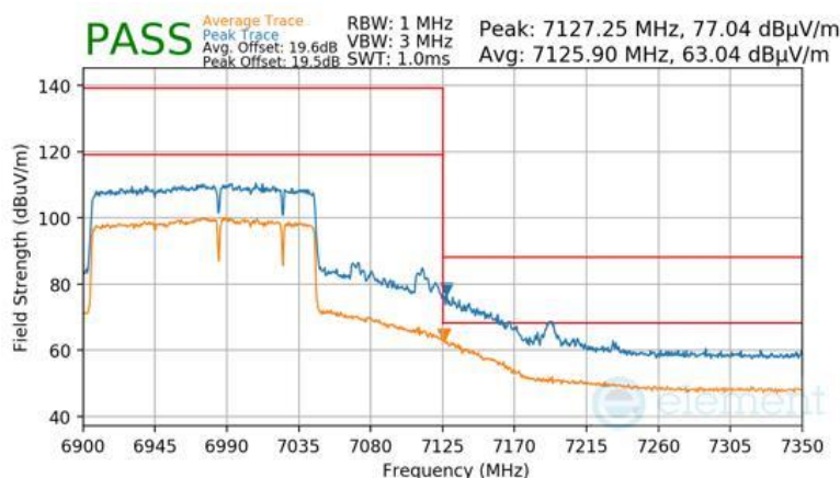
Plot 7-967 Antenna WF8 Radiated Upper Band Edge (Peak & Average – UNII Band 8) - RU996+484+242 (H)
