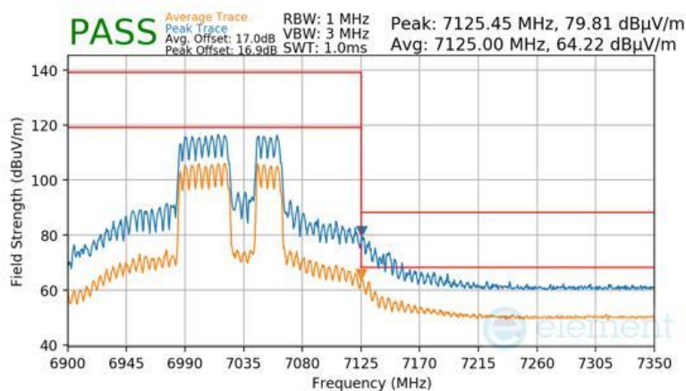
Plot 7-1057 SDM Primary Radiated Upper Band Edge (Peak & Average – UNII Band 8) - RU484+242
