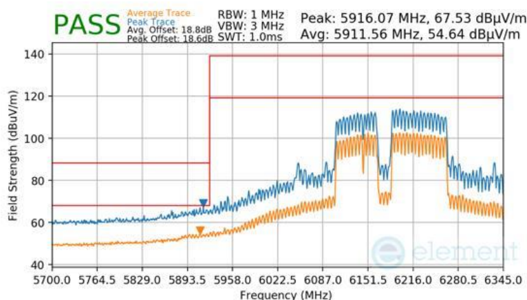
Plot 7-1079 SDM Primary Radiated Lower Band Edge (Peak & Average – UNII Band 5) - RU996+484+242 (L)
