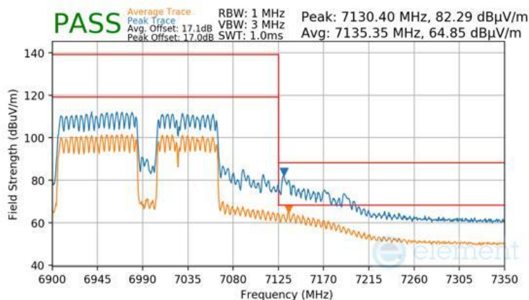
Plot 7-1081 SDM Primary Radiated Upper Band Edge (Peak & Average – UNII Band 8) - RU996+484+242 (H)
