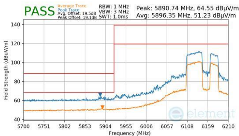
Plot 7-993 Antenna WF7 Radiated Lower Band Edge (Peak & Average – UNII Band 5) - RU484+242
