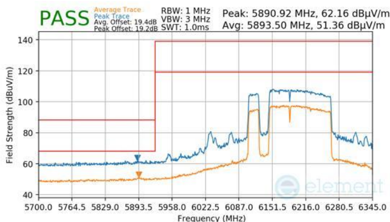
Plot 7-955 Antenna WF8 Radiated Lower Band Edge (Peak & Average – UNII Band 5) - RU996+484+242 (L)
