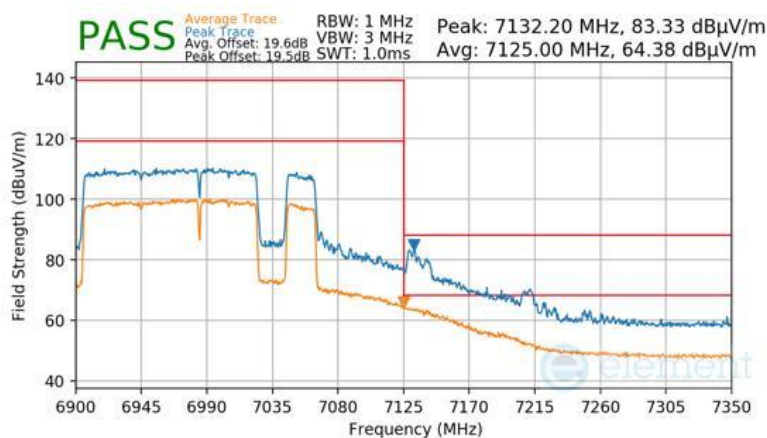
Plot 7-965 Antenna WF8 Radiated Upper Band Edge (Peak & Average – UNII Band 8) - RU996+484+242 (H)
