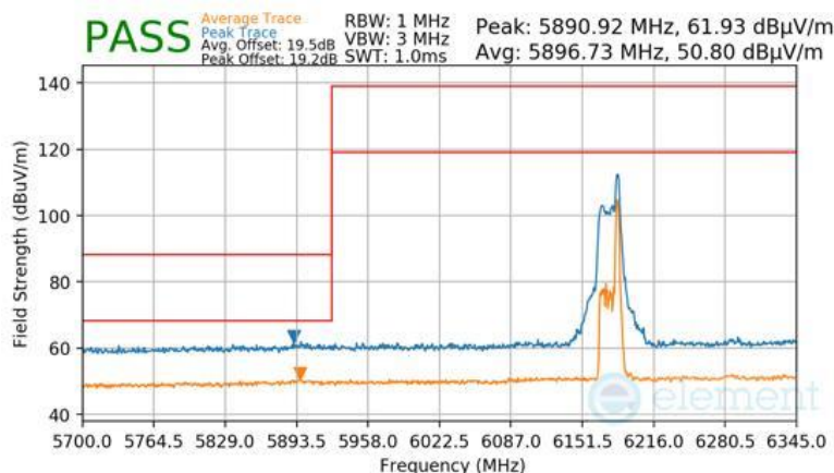
Plot 7-1002 Antenna WF7 Radiated Lower Band Edge (Peak & Average – UNII Band 5) - RU26
