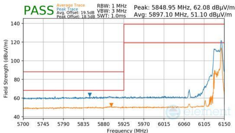
Plot 7-982 Antenna WF7 Radiated Lower Band Edge (Peak & Average – UNII Band 5) - RU26
