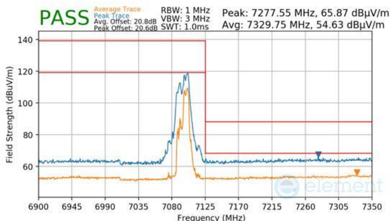
Plot 7-1038 SDM Primary Radiated Upper Band Edge (Peak & Average – UNII Band 8) - RU52+26
