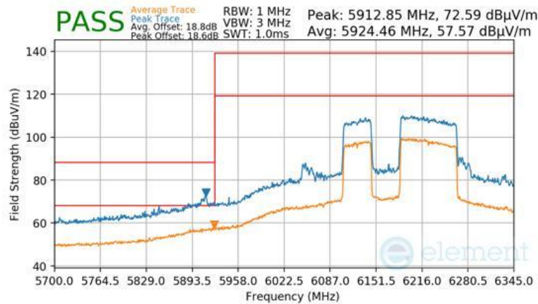
Plot 7-1007 Antenna WF7 Radiated Lower Band Edge (Peak & Average – UNII Band 5) - RU996+484 (L)
