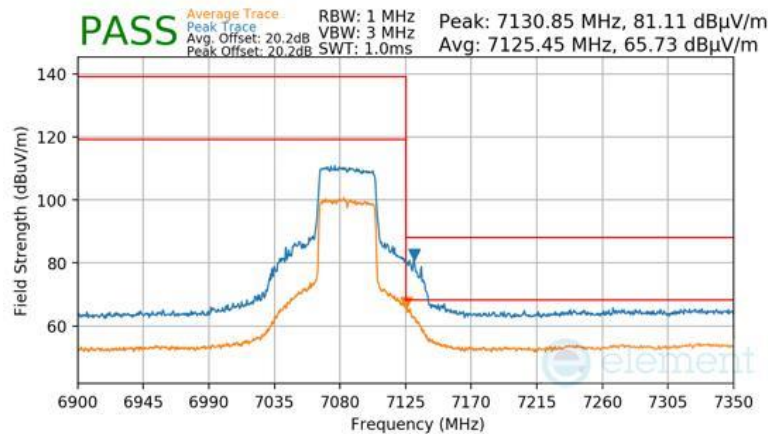
Plot 7-986 Antenna WF7 Radiated Upper Band Edge (Peak & Average – UNII Band 8) - RU484
