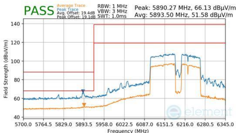
Plot 7-954 Antenna WF8 Radiated Lower Band Edge (Peak & Average – UNII Band 5) - RU996+484+242 (H)
