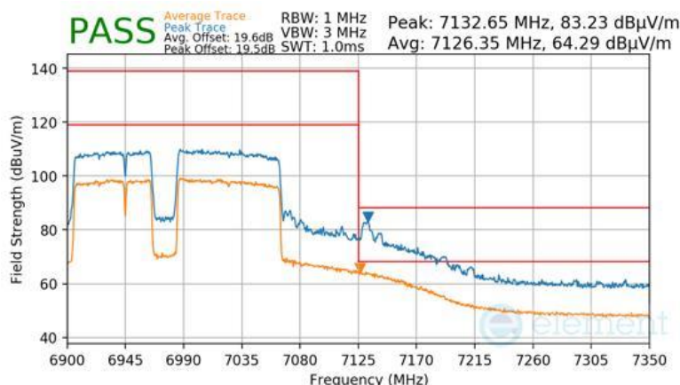
Plot 7-968 Antenna WF8 Radiated Upper Band Edge (Peak & Average – UNII Band 8) - RU996+484+242 (L)
