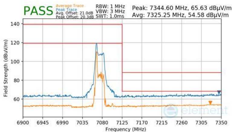
Plot 7-983 Antenna WF7 Radiated Upper Band Edge (Peak & Average – UNII Band 8) - RU26
