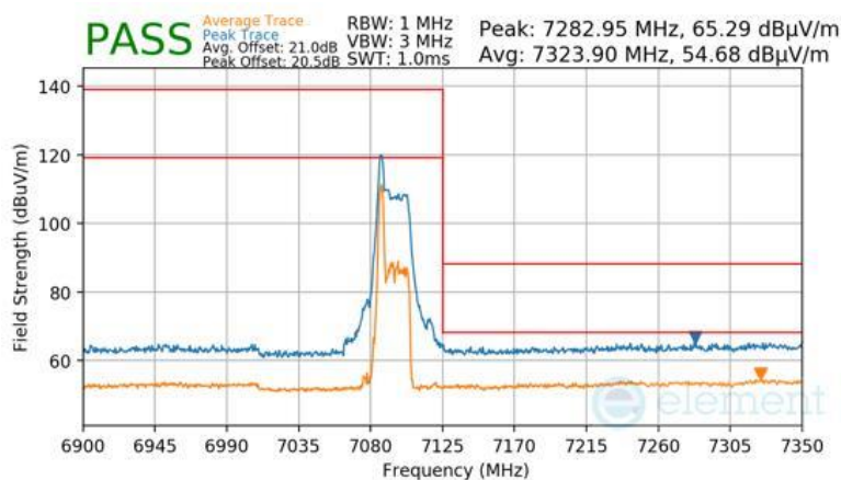
Plot 7-973 Antenna WF7 Radiated Upper Band Edge (Peak & Average – UNII Band 8) - RU26
