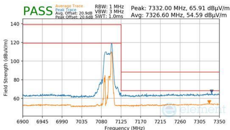
Plot 7-974 Antenna WF7 Radiated Upper Band Edge (Peak & Average – UNII Band 8) - RU26
