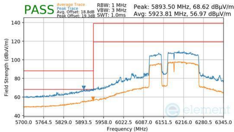
Plot 7-1017 Antenna WF7 Radiated Lower Band Edge (Peak & Average – UNII Band 5) - RU996+484+242 (L)
