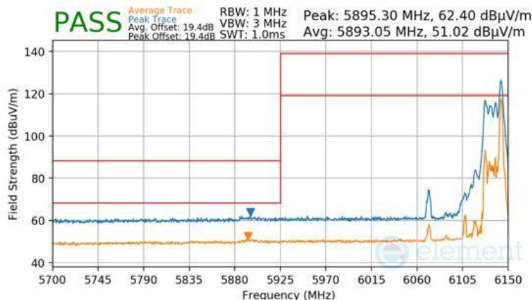
Plot 7-1042 SDM Primary Radiated Lower Band Edge (Peak & Average – UNII Band 5) - RU26
