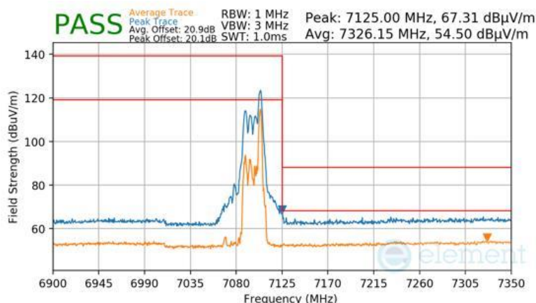
Plot 7-1094 SDM Diversity Radiated Upper Band Edge (Peak & Average – UNII Band 8) - RU26
