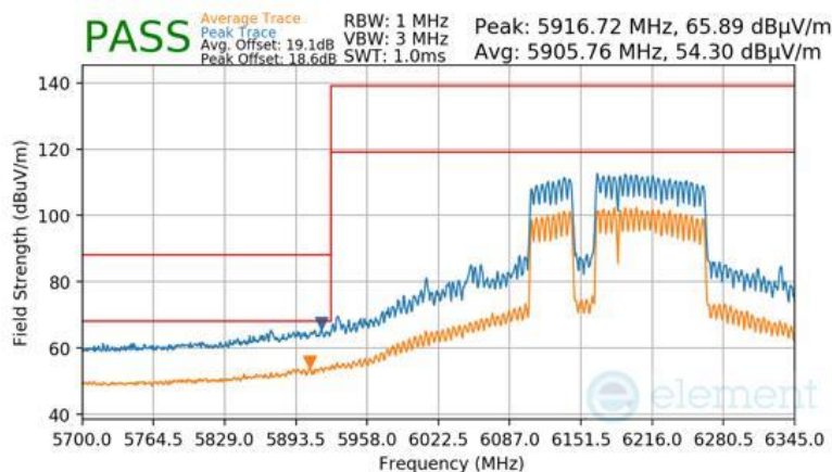
Plot 7-1077 SDM Primary Radiated Lower Band Edge (Peak & Average – UNII Band 5) - RU996+484+242 (L)
