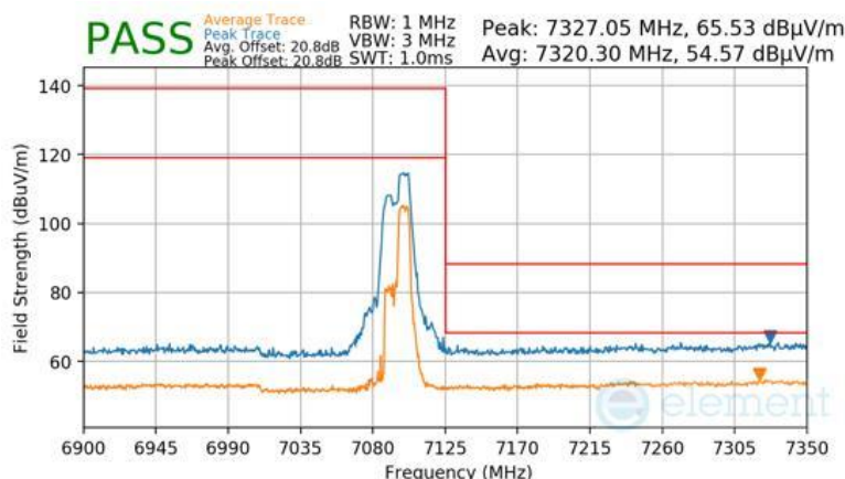
Plot 7-978 Antenna WF7 Radiated Upper Band Edge (Peak & Average – UNII Band 8) - RU52+26
