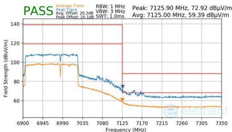
Plot 7-1011 Antenna WF7 Radiated Upper Band Edge (Peak & Average – UNII Band 8) - RU996+484 (H)
