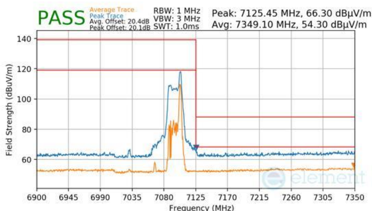
Plot 7-984 Antenna WF7 Radiated Upper Band Edge (Peak & Average – UNII Band 8) - RU26
