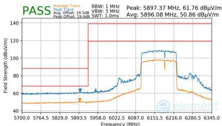
Plot 7-948 Antenna WF8 Radiated Lower Band Edge (Peak & Average – UNII Band 5) - RU996+484 (H)
