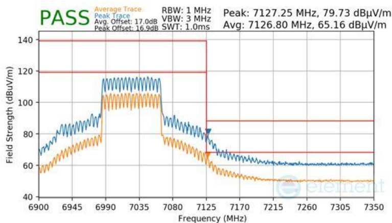
Plot 7-1060 SDM Primary Radiated Upper Band Edge (Peak & Average – UNII Band 8) - RU996
