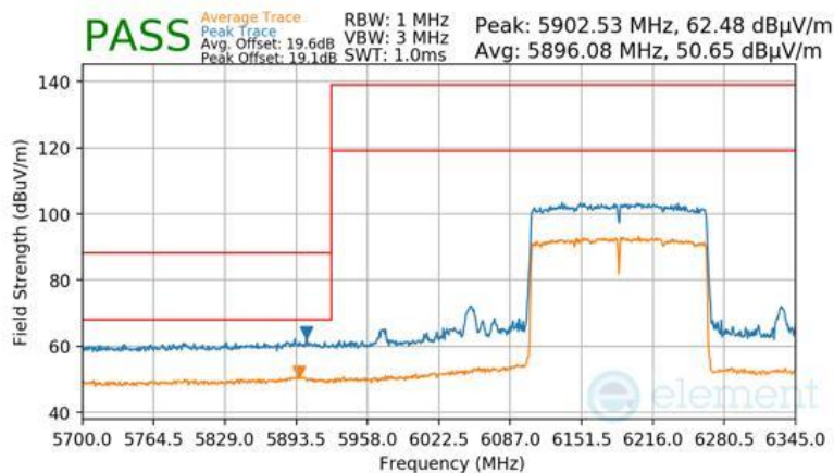
Plot 7-969 Antenna WF8 Radiated Lower Band Edge (Peak & Average – UNII Band 5) - RU996X2
