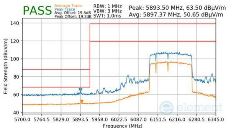
Plot 7-953 Antenna WF8 Radiated Lower Band Edge (Peak & Average – UNII Band 5) - RU996+484+242 (L)
