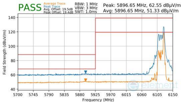
Plot 7-1092 SDM Diversity Radiated Lower Band Edge (Peak & Average – UNII Band 5) - RU26
