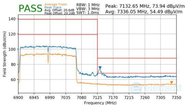
Plot 7-970 Antenna WF8 Radiated Upper Band Edge (Peak & Average – UNII Band 8) - RU996X2
