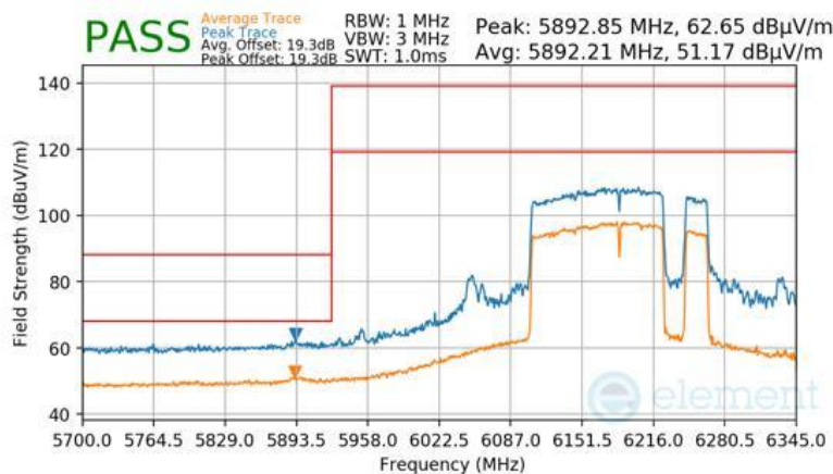
Plot 7-958 Antenna WF8 Radiated Lower Band Edge (Peak & Average – UNII Band 5) - RU996+484+242 (H)
