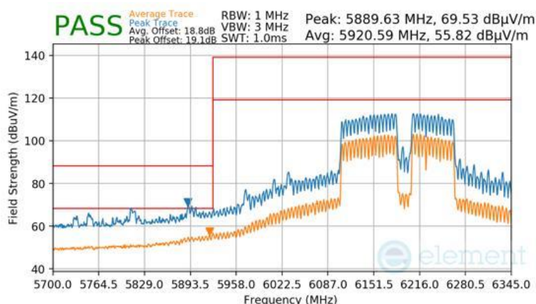
Plot 7-1074 SDM Primary Radiated Lower Band Edge (Peak & Average – UNII Band 5) - RU996+484+242 (H)
