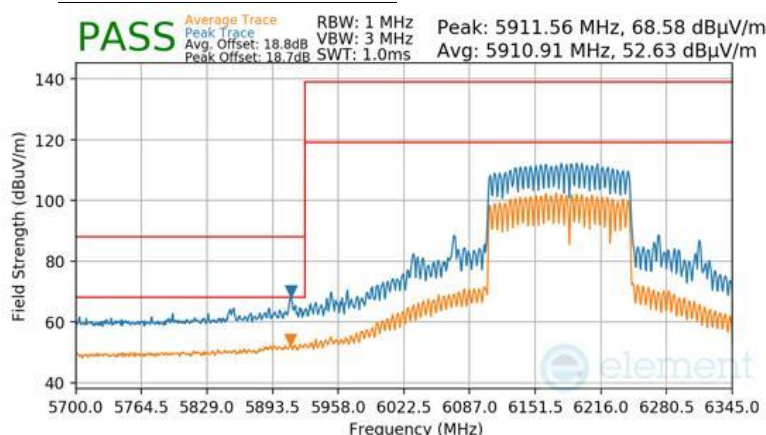
Plot 7-1080 SDM Primary Radiated Lower Band Edge (Peak & Average – UNII Band 5) - RU996+484+242 (H)
