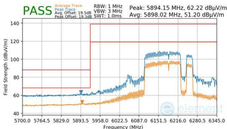
Plot 7-1078 SDM Primary Radiated Lower Band Edge (Peak & Average – UNII Band 5) - RU996+484+242 (H)
