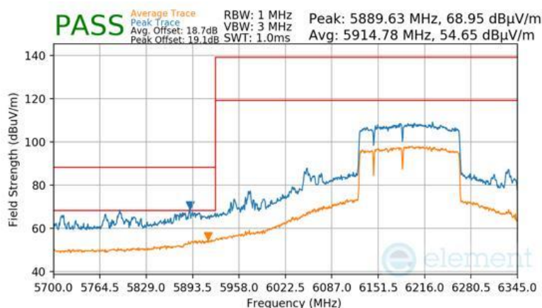
Plot 7-1013 Antenna WF7 Radiated Lower Band Edge (Peak & Average – UNII Band 5) - RU996+484+242 (L)
