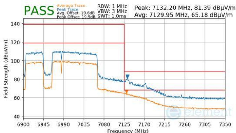
Plot 7-966 Antenna WF8 Radiated Upper Band Edge (Peak & Average – UNII Band 8) - RU996+484+242 (L)
