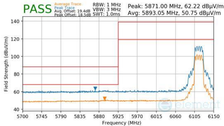
Plot 7-1039 SDM Primary Radiated Lower Band Edge (Peak & Average – UNII Band 5) - RU242
