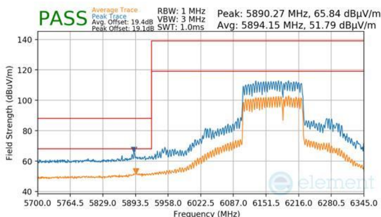
Plot 7-1068 SDM Primary Radiated Lower Band Edge (Peak & Average – UNII Band 5) - RU996+484 (H)
