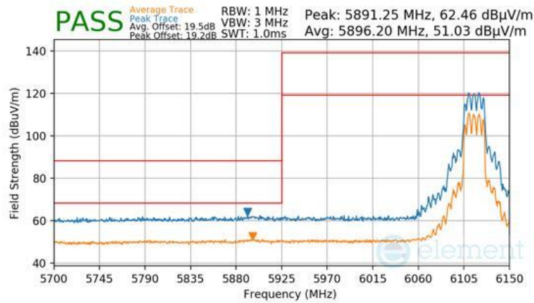
Plot 7-1099 SDM Diversity Radiated Lower Band Edge (Peak & Average – UNII Band 5) - RU242
