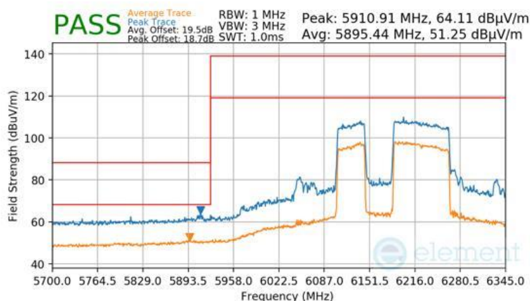
Plot 7-947 Antenna WF8 Radiated Lower Band Edge (Peak & Average – UNII Band 5) - RU996+484 (L)
