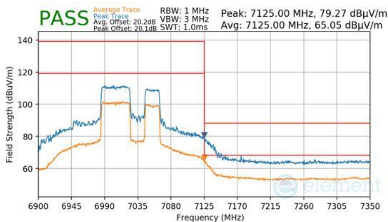
Plot 7-997 Antenna WF7 Radiated Upper Band Edge (Peak & Average – UNII Band 8) - RU484+242
