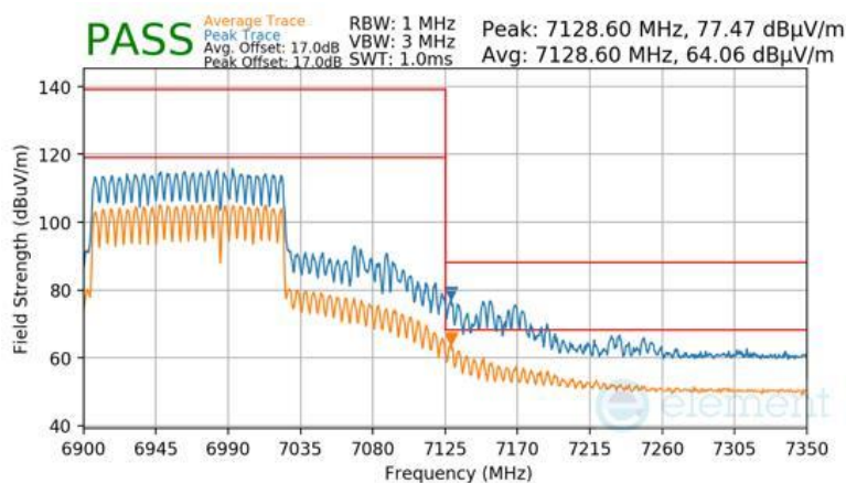
Plot 7-1071 SDM Primary Radiated Upper Band Edge (Peak & Average – UNII Band 8) - RU996+484 (H)
