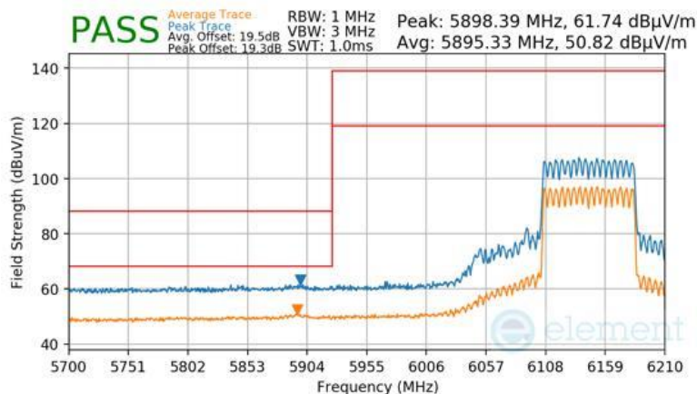
Plot 7-1059 SDM Primary Radiated Lower Band Edge (Peak & Average – UNII Band 5) - RU996
