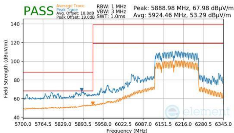
Plot 7-1073 SDM Primary Radiated Lower Band Edge (Peak & Average – UNII Band 5) - RU996+484+242 (L)
