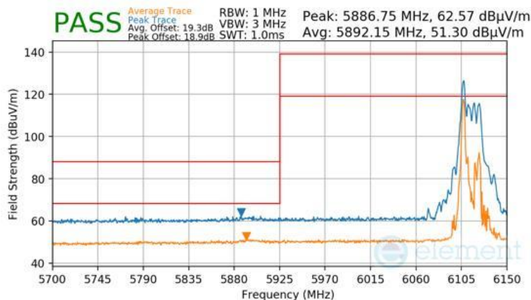
Plot 7-1091 SDM Diversity Radiated Lower Band Edge (Peak & Average – UNII Band 5) - RU26
