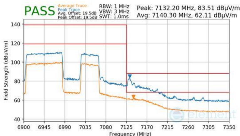
Plot 7-950 Antenna WF8 Radiated Upper Band Edge (Peak & Average – UNII Band 8) - RU996+484 (H)
