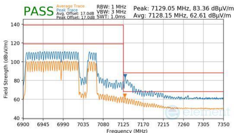
Plot 7-1086 SDM Primary Radiated Upper Band Edge (Peak & Average – UNII Band 8) - RU996+484+242 (H)
