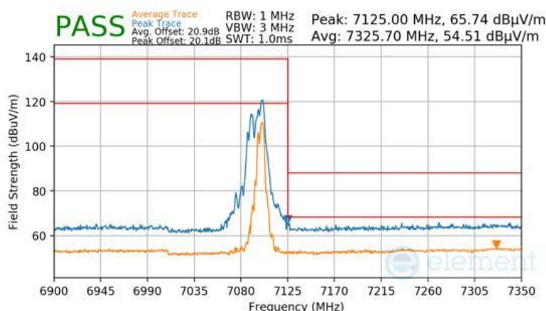
Plot 7-1098 SDM Diversity Radiated Upper Band Edge (Peak & Average – UNII Band 8) - RU52+26
