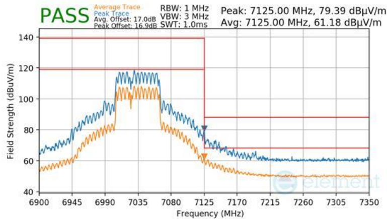
Plot 7-1055 SDM Primary Radiated Upper Band Edge (Peak & Average – UNII Band 8) - RU484+242
