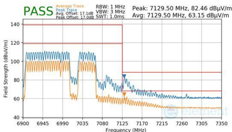
Plot 7-1084 SDM Primary Radiated Upper Band Edge (Peak & Average – UNII Band 8) - RU996+484+242 (H)
