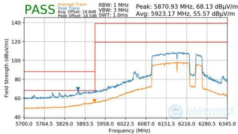
Plot 7-1018 Antenna WF7 Radiated Lower Band Edge (Peak & Average – UNII Band 5) - RU996+484+242 (H)
