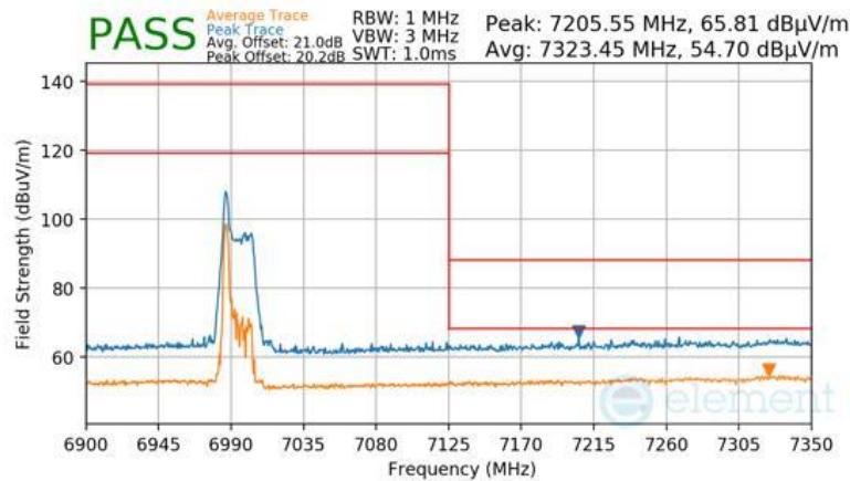
Plot 7-1003 Antenna WF7 Radiated Upper Band Edge (Peak & Average – UNII Band 8) - RU26
