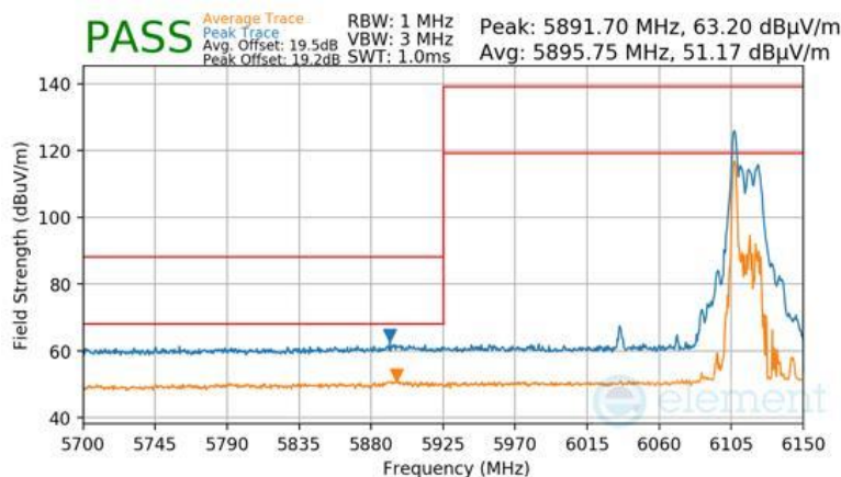
Plot 7-1041 SDM Primary Radiated Lower Band Edge (Peak & Average – UNII Band 5) - RU26
