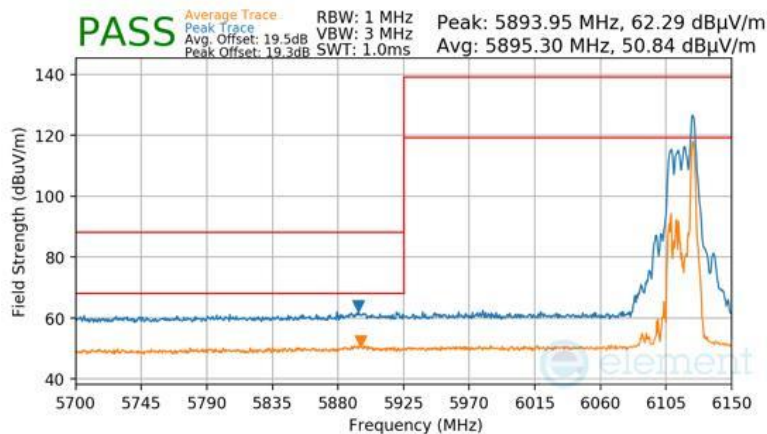
Plot 7-1032 SDM Primary Radiated Lower Band Edge (Peak & Average – UNII Band 5) - RU26
