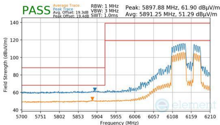
Plot 7-1053 SDM Primary Radiated Lower Band Edge (Peak & Average – UNII Band 5) - RU484+242
