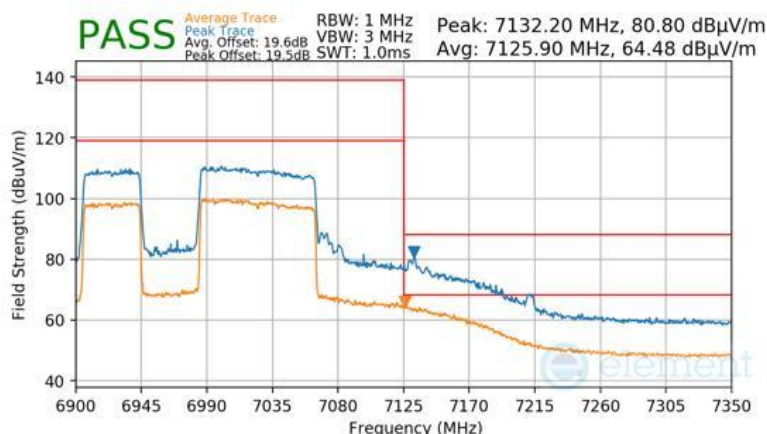
Plot 7-952 Antenna WF8 Radiated Upper Band Edge (Peak & Average – UNII Band 8) - RU996+484 (L)
