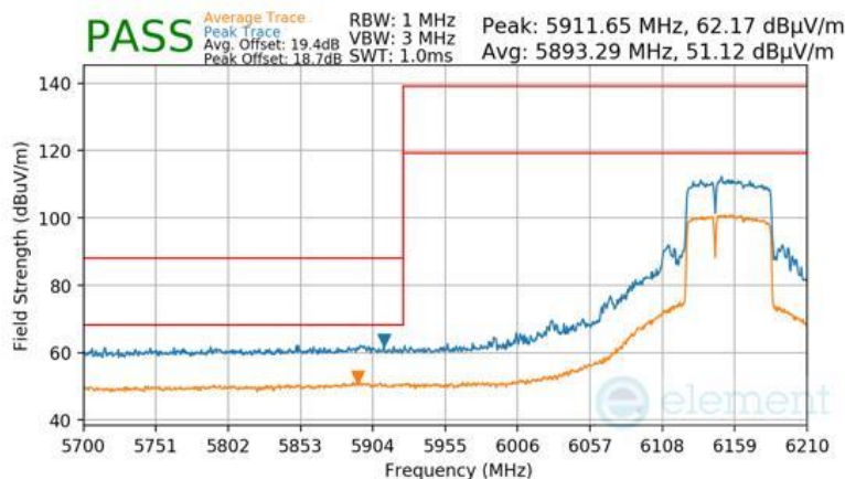
Plot 7-991 Antenna WF7 Radiated Lower Band Edge (Peak & Average – UNII Band 5) - RU484+242
