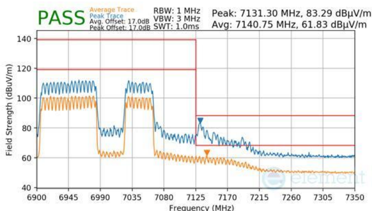
Plot 7-1070 SDM Primary Radiated Upper Band Edge (Peak & Average – UNII Band 8) - RU996+484 (H)
