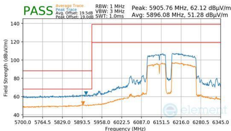
Plot 7-959 Antenna WF8 Radiated Lower Band Edge (Peak & Average – UNII Band 5) - RU996+484+242 (L)
