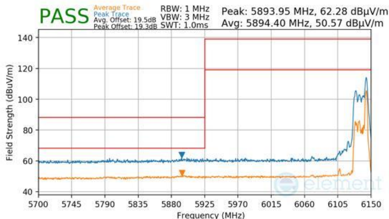
Plot 7-1102 SDM Diversity Radiated Lower Band Edge (Peak & Average – UNII Band 5) - RU26
