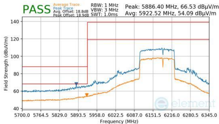
Plot 7-1008 Antenna WF7 Radiated Lower Band Edge (Peak & Average – UNII Band 5) - RU996+484 (H)
