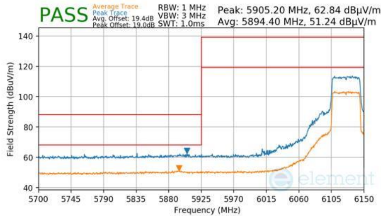
Plot 7-985 Antenna WF7 Radiated Lower Band Edge (Peak & Average – UNII Band 5) - RU484
