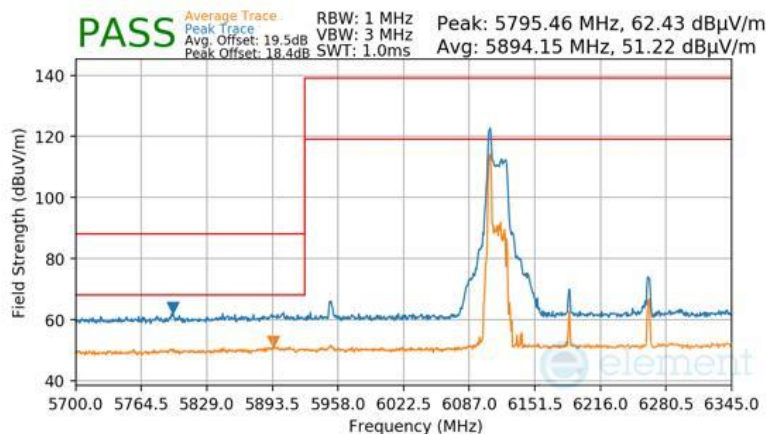
Plot 7-1001 Antenna WF7 Radiated Lower Band Edge (Peak & Average – UNII Band 5) - RU26
