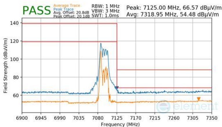
Plot 7-1093 SDM Diversity Radiated Upper Band Edge (Peak & Average – UNII Band 8) - RU26
