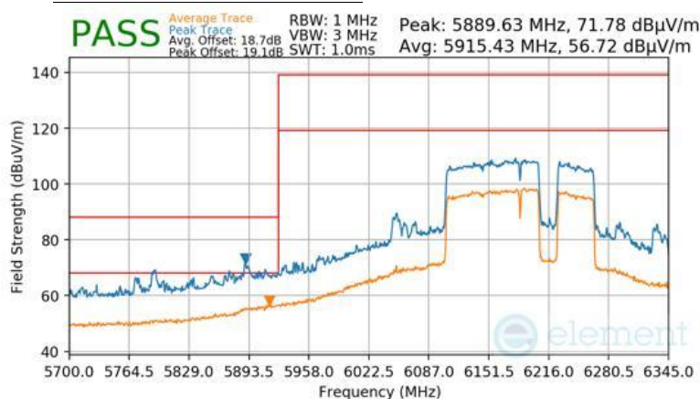
Plot 7-1016 Antenna WF7 Radiated Lower Band Edge (Peak & Average – UNII Band 5) - RU996+484+242 (H)
