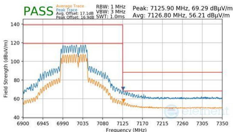
Plot 7-1058 SDM Primary Radiated Upper Band Edge (Peak & Average – UNII Band 8) - RU484+242
