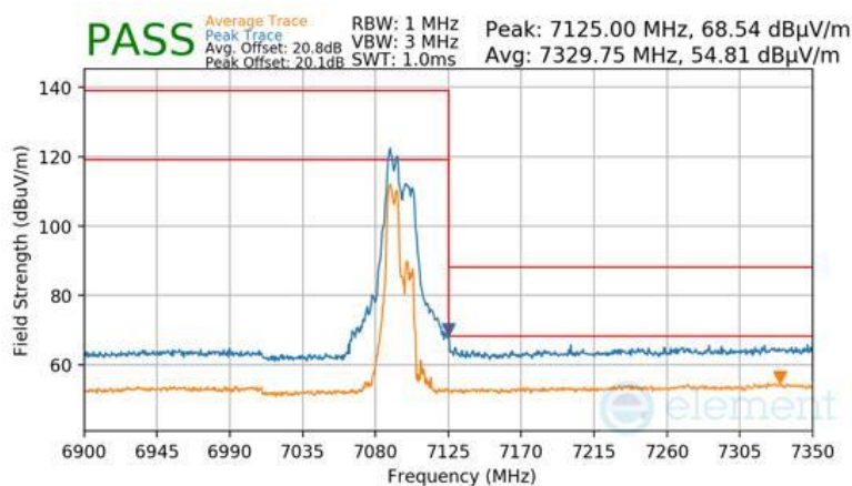
Plot 7-1037 SDM Primary Radiated Upper Band Edge (Peak & Average – UNII Band 8) - RU52+26
