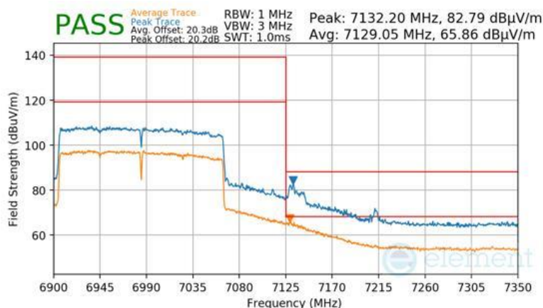
Plot 7-1030 Antenna WF7 Radiated Upper Band Edge (Peak & Average – UNII Band 8) - RU996X2
