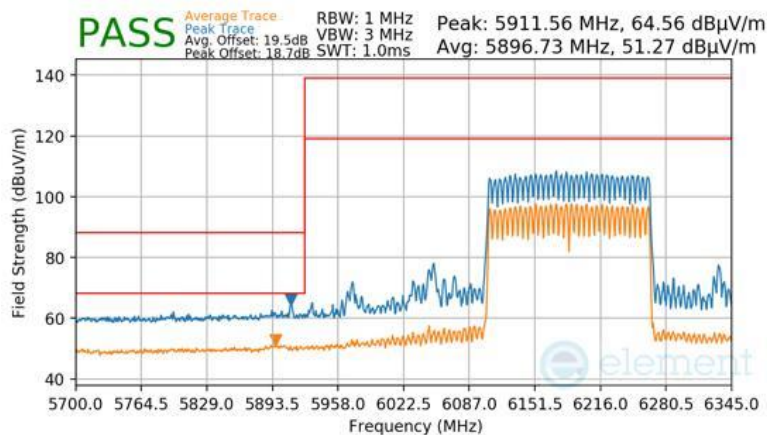
Plot 7-1089 SDM Primary Radiated Lower Band Edge (Peak & Average – UNII Band 5) - RU996X2
