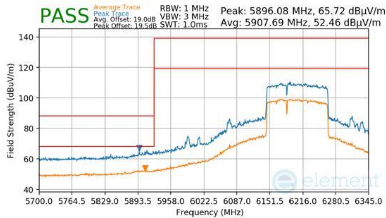
Plot 7-1005 Antenna WF7 Radiated Lower Band Edge (Peak & Average – UNII Band 5) - RU996+484 (L)
