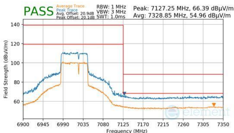
Plot 7-998 Antenna WF7 Radiated Upper Band Edge (Peak & Average – UNII Band 8) - RU484+242
