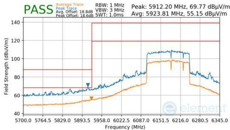
Plot 7-1020 Antenna WF7 Radiated Lower Band Edge (Peak & Average – UNII Band 5) - RU996+484+242 (H)
