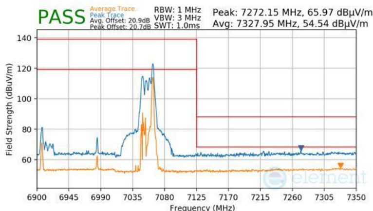
Plot 7-1124 SDM Diversity Radiated Upper Band Edge (Peak & Average – UNII Band 8) - RU26
