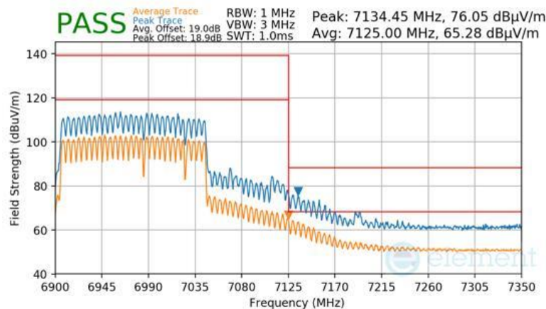
Plot 7-1148 SDM Diversity Radiated Upper Band Edge (Peak & Average – UNII Band 8) - RU996+484+242 (H)
