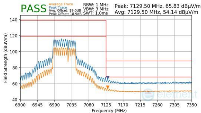
Plot 7-1118 SDM Diversity Radiated Upper Band Edge (Peak & Average – UNII Band 8) - RU484+242
