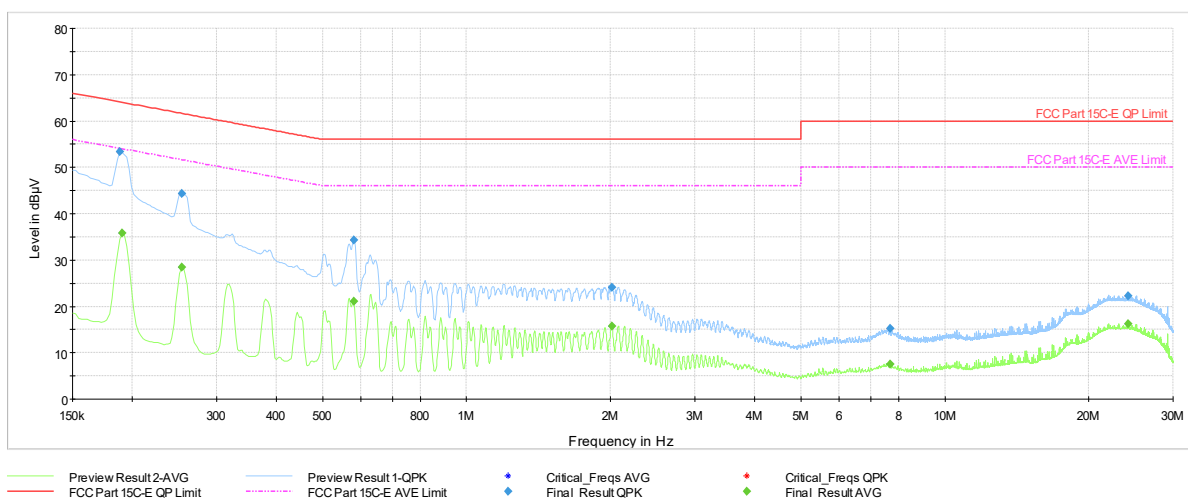
Plot 7-1161. AC Line Conducted Plot with 11be UNII Band 5 SDM Diversity – RU242 – Ch.33 (L1) with Laptop
