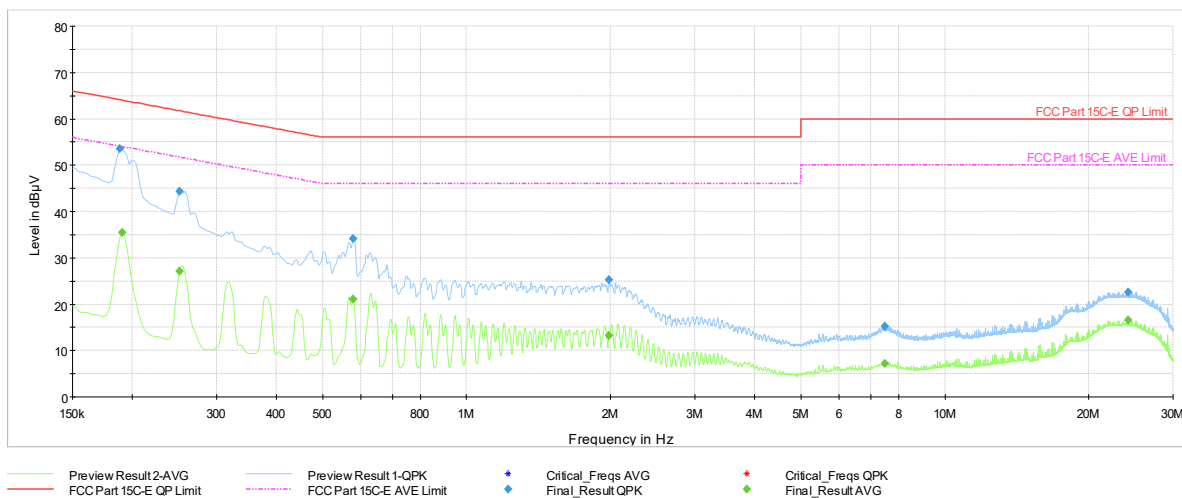
Plot 7-1155. AC Line Conducted Plot with 11be UNII Band 5 SDM Primary – RU26 – Ch.33 (L1) with Laptop
