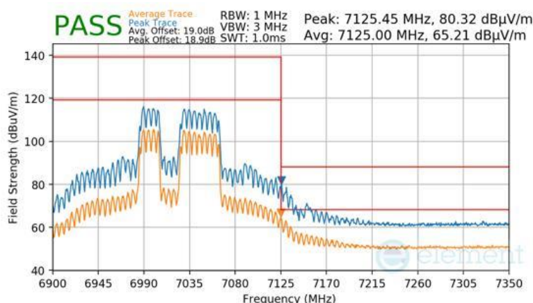
Plot 7-1116 SDM Diversity Radiated Upper Band Edge (Peak & Average – UNII Band 8) - RU484+242
