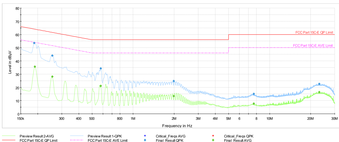
Plot 7-1157. AC Line Conducted Plot with 11be UNII Band 5 SDM Primary – RU242 – Ch.33 (L1) with Laptop
