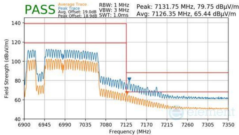
Plot 7-1143 SDM Diversity Radiated Upper Band Edge (Peak & Average – UNII Band 8) - RU996+484+242 (L)
