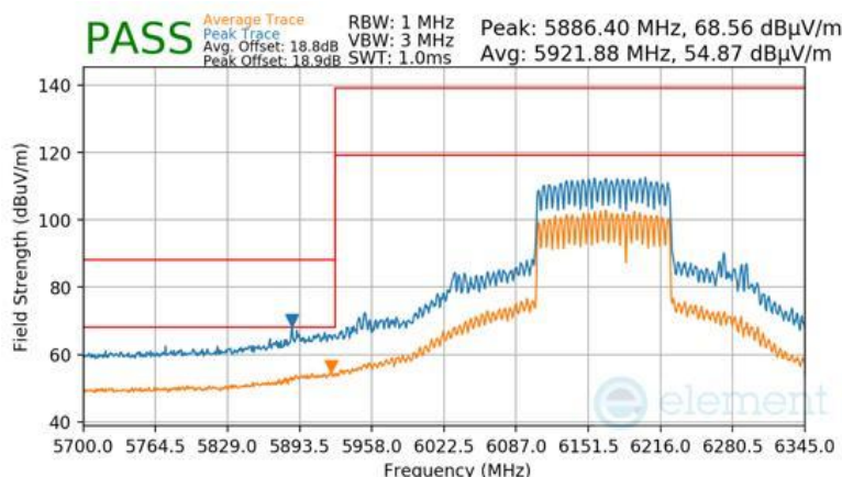
Plot 7-1128 SDM Diversity Radiated Lower Band Edge (Peak & Average – UNII Band 5) - RU996+484 (H)
