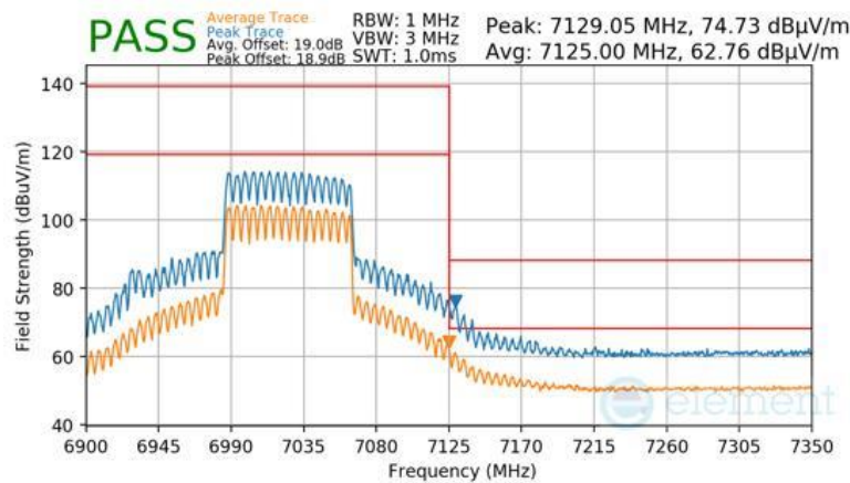
Plot 7-1120 SDM Diversity Radiated Upper Band Edge (Peak & Average – UNII Band 8) - RU996
