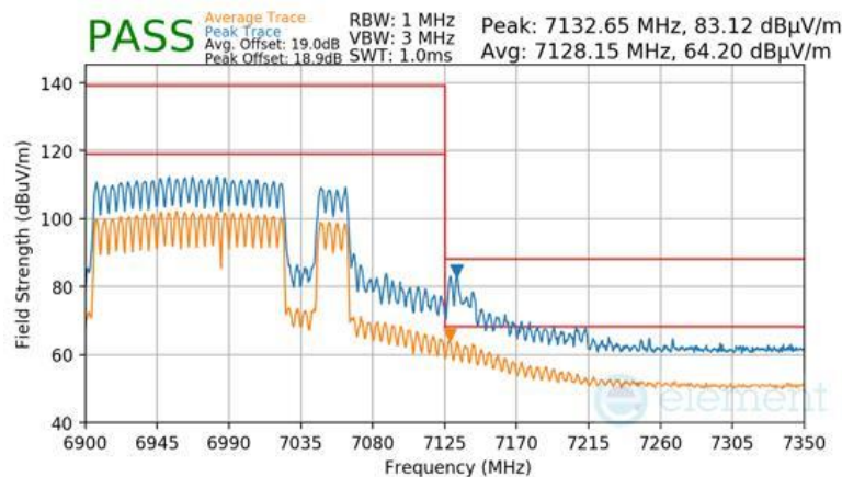
Plot 7-1146 SDM Diversity Radiated Upper Band Edge (Peak & Average – UNII Band 8) - RU996+484+242 (H)
