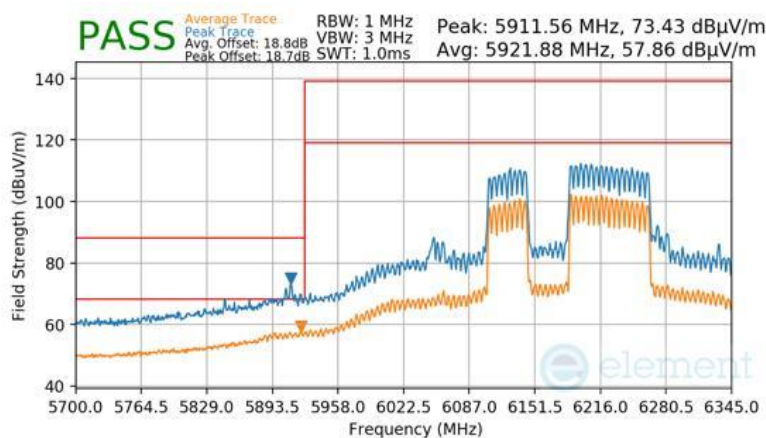
Plot 7-1127 SDM Diversity Radiated Lower Band Edge (Peak & Average – UNII Band 5) - RU996+484 (L)
