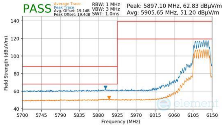
Plot 7-1105 SDM Diversity Radiated Lower Band Edge (Peak & Average – UNII Band 5) - RU484
