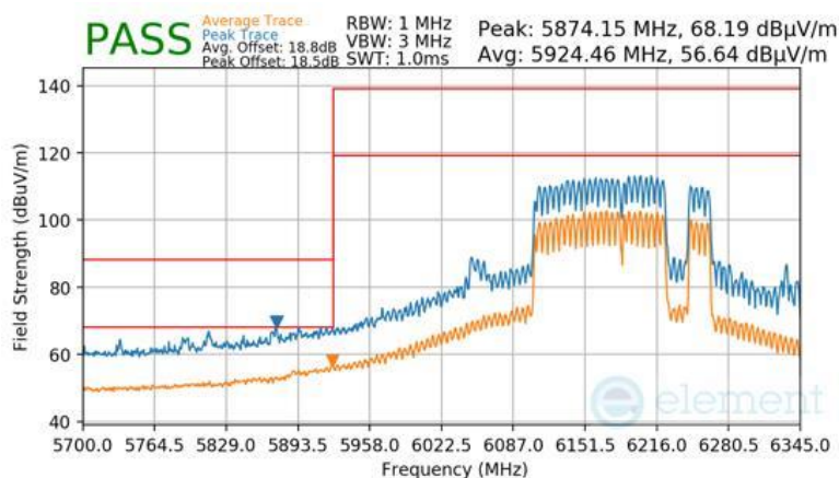
Plot 7-1138 SDM Diversity Radiated Lower Band Edge (Peak & Average – UNII Band 5) - RU996+484+242 (H)
