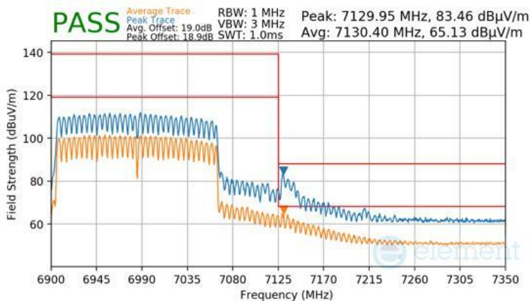
Plot 7-1150 SDM Diversity Radiated Upper Band Edge (Peak & Average – UNII Band 8) - RU996X2
