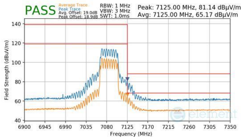
Plot 7-1106 SDM Diversity Radiated Upper Band Edge (Peak & Average – UNII Band 8) - RU484
