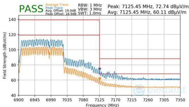
Plot 7-1131 SDM Diversity Radiated Upper Band Edge (Peak & Average – UNII Band 8) - RU996+484 (H)
