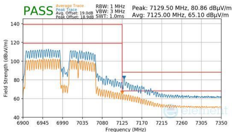
Plot 7-1142 SDM Diversity Radiated Upper Band Edge (Peak & Average – UNII Band 8) - RU996+484+242 (H)
