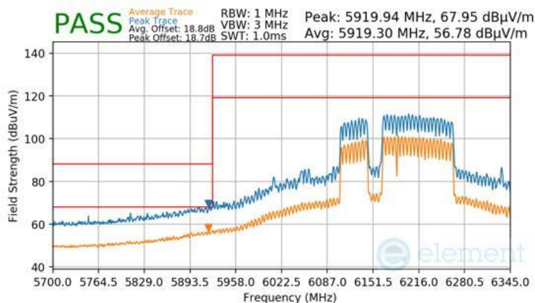
Plot 7-1137 SDM Diversity Radiated Lower Band Edge (Peak & Average – UNII Band 5) - RU996+484+242 (L)
