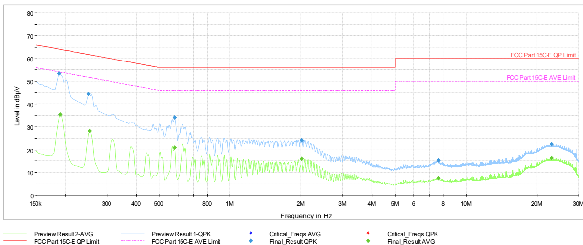
Plot 7-1159. AC Line Conducted Plot with 11be UNII Band 5 SDM Diversity – RU26 – Ch.33 (L1) with Laptop
