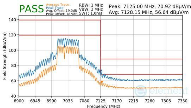
Plot 7-1115 SDM Diversity Radiated Upper Band Edge (Peak & Average – UNII Band 8) - RU484+242
