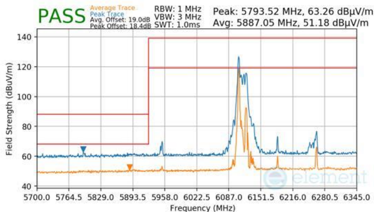
Plot 7-1121 SDM Diversity Radiated Lower Band Edge (Peak & Average – UNII Band 5) - RU26
