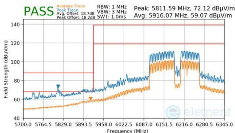
Plot 7-1134 SDM Diversity Radiated Lower Band Edge (Peak & Average – UNII Band 5) - RU996+484+242 (H)
