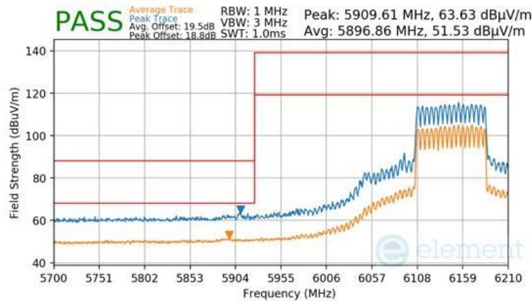
Plot 7-1119 SDM Diversity Radiated Lower Band Edge (Peak & Average – UNII Band 5) - RU996
