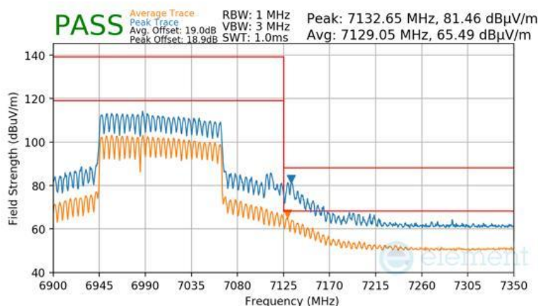
Plot 7-1129 SDM Diversity Radiated Upper Band Edge (Peak & Average – UNII Band 8) - RU996+484 (L)
