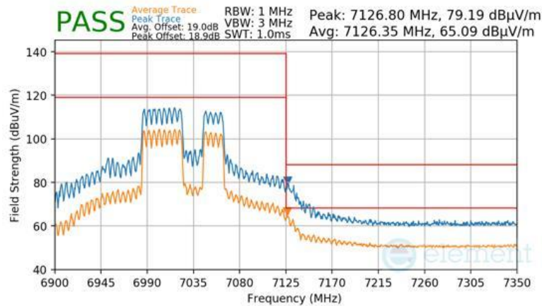
Plot 7-1117 SDM Diversity Radiated Upper Band Edge (Peak & Average – UNII Band 8) - RU484+242
