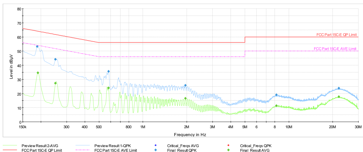
Plot 7-1160. AC Line Conducted Plot with 11be UNII Band 5 SDM Diversity – RU26 – Ch.33 (N) with Laptop
