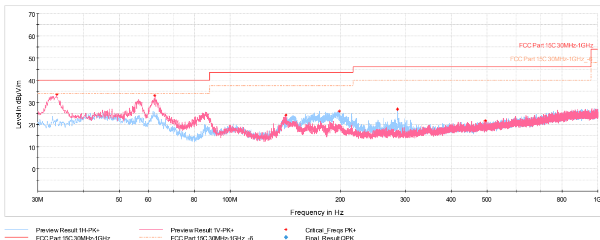
Plot 7-1153. Radiated Spurious Emissions below 1GHz SDM Diversity (802.11be – Ch.61 – RU26) with AC/DC Adapter
