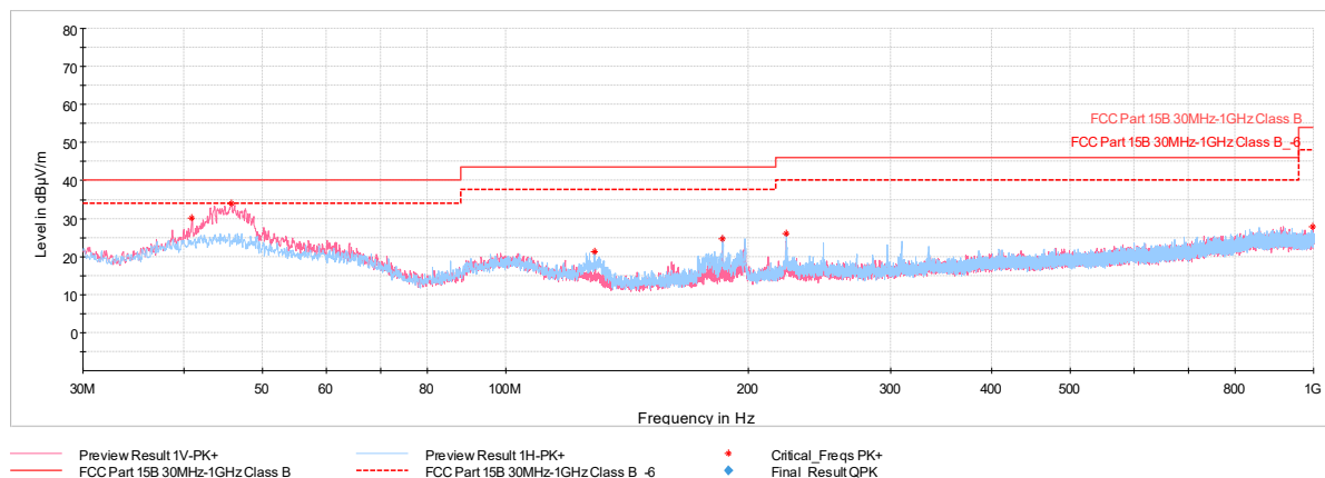
Plot 7-1151. Radiated Spurious Emissions below 1GHz SDM Primary (802.11be – Ch.61 – RU26) with AC/DC Adapter
