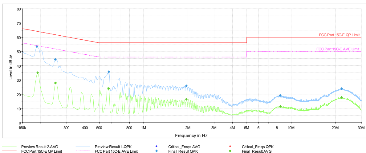
Plot 7-1158. AC Line Conducted Plot with 11be UNII Band 5 SDM Primary – RU242 – Ch.33 (N) with Laptop
