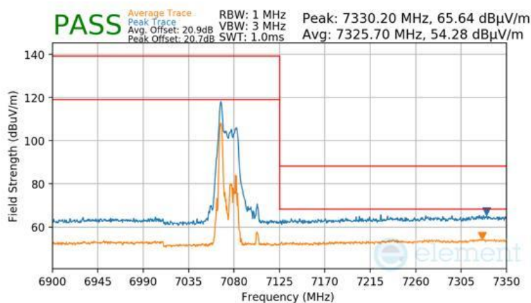
Plot 7-1103 SDM Diversity Radiated Upper Band Edge (Peak & Average – UNII Band 8) - RU26
