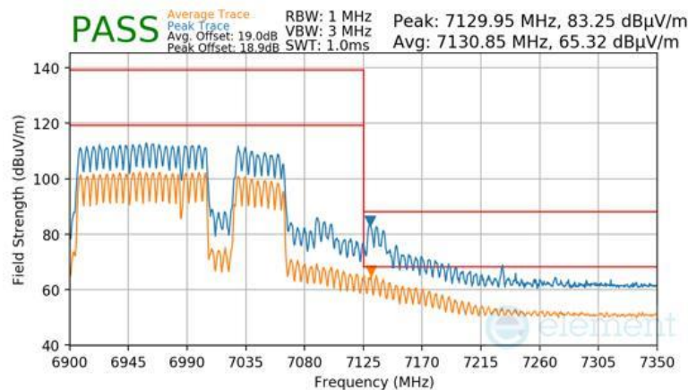
Plot 7-1144 SDM Diversity Radiated Upper Band Edge (Peak & Average – UNII Band 8) - RU996+484+242 (H)
