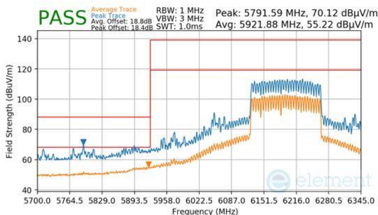
Plot 7-1133 SDM Diversity Radiated Lower Band Edge (Peak & Average – UNII Band 5) - RU996+484+242 (L)
