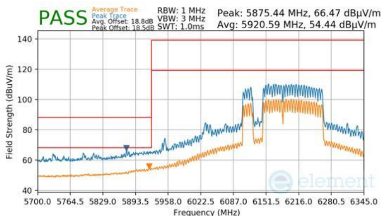
Plot 7-1135 SDM Diversity Radiated Lower Band Edge (Peak & Average – UNII Band 5) - RU996+484+242 (L)
