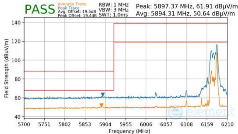
Plot 7-1108 SDM Diversity Radiated Lower Band Edge (Peak & Average – UNII Band 5) - RU26
