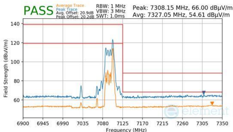
Plot 7-1104 SDM Diversity Radiated Upper Band Edge (Peak & Average – UNII Band 8) - RU26
