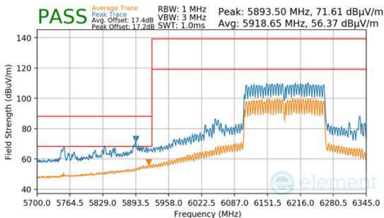
Plot 7-1149 SDM Diversity Radiated Lower Band Edge (Peak & Average – UNII Band 5) - RU996X2
