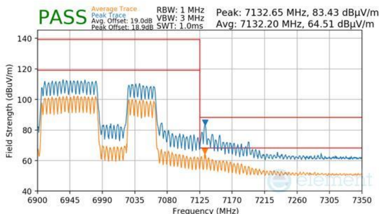
Plot 7-1130 SDM Diversity Radiated Upper Band Edge (Peak & Average – UNII Band 8) - RU996+484 (H)
