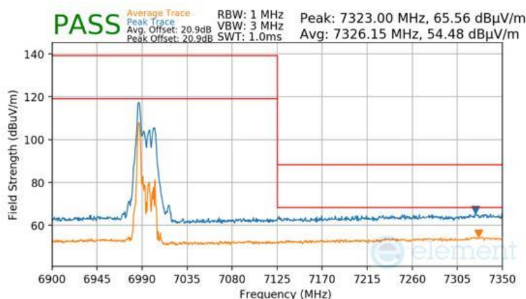
Plot 7-1123 SDM Diversity Radiated Upper Band Edge (Peak & Average – UNII Band 8) - RU26
