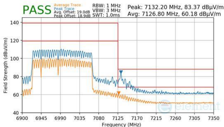
Plot 7-1141 SDM Diversity Radiated Upper Band Edge (Peak & Average – UNII Band 8) - RU996+484+242 (L)
