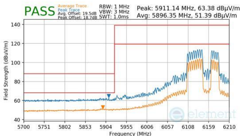
Plot 7-1113 SDM Diversity Radiated Lower Band Edge (Peak & Average – UNII Band 5) - RU484+242
