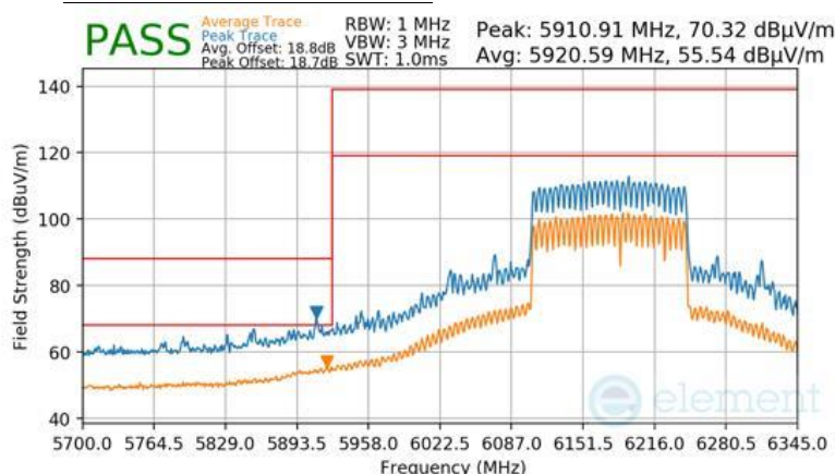
Plot 7-1140 SDM Diversity Radiated Lower Band Edge (Peak & Average – UNII Band 5) - RU996+484+242 (H)
