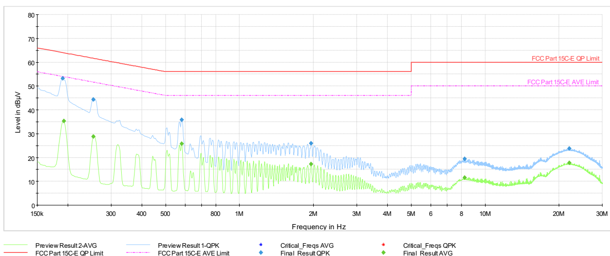
Plot 7-1156. AC Line Conducted Plot with 11be UNII Band 5 SDM Primary – RU26 – Ch.33 (N) with Laptop
