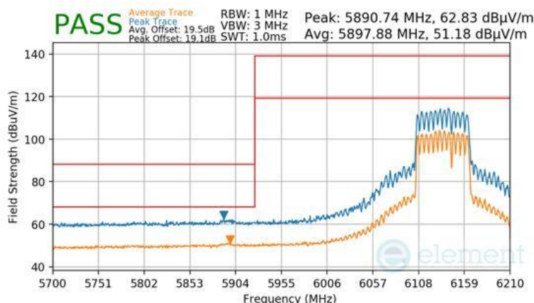
Plot 7-1114 SDM Diversity Radiated Lower Band Edge (Peak & Average – UNII Band 5) - RU484+242
