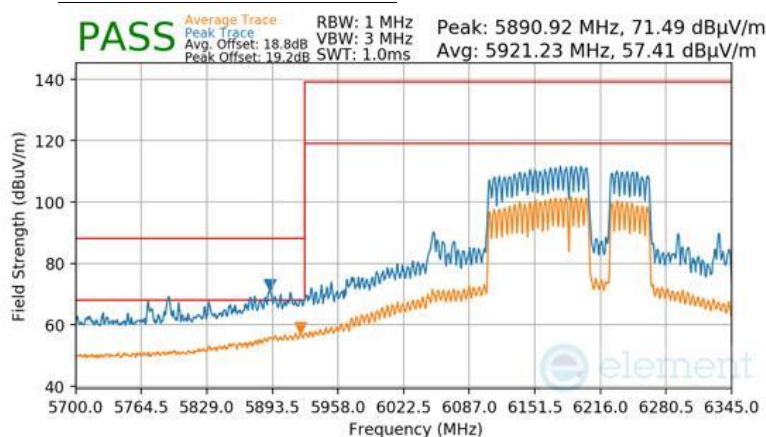
Plot 7-1136 SDM Diversity Radiated Lower Band Edge (Peak & Average – UNII Band 5) - RU996+484+242 (H)
