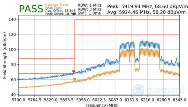
Plot 7-1139 SDM Diversity Radiated Lower Band Edge (Peak & Average – UNII Band 5) - RU996+484+242 (L)
