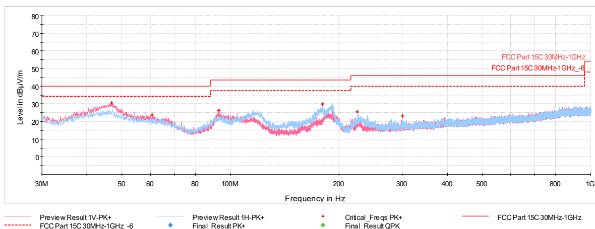
Plot 7-1152. Radiated Spurious Emissions below 1GHz SDM Primary (802.11be – Ch.61 – RU242) with AC/DC Adapter
