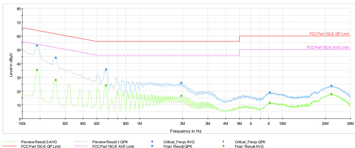
Plot 7-1162. AC Line Conducted Plot with 11be UNII Band 5 SDM Diversity – RU242 – Ch.33 (N) with Laptop
