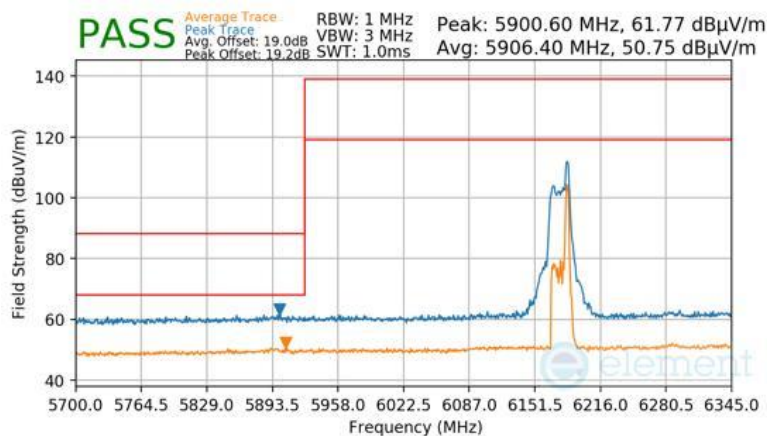
Plot 7-1122 SDM Diversity Radiated Lower Band Edge (Peak & Average – UNII Band 5) - RU26
