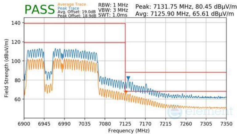
Plot 7-1145 SDM Diversity Radiated Upper Band Edge (Peak & Average – UNII Band 8) - RU996+484+242 (L)
