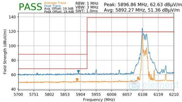
Plot 7-1107 SDM Diversity Radiated Lower Band Edge (Peak & Average – UNII Band 5) - RU26
