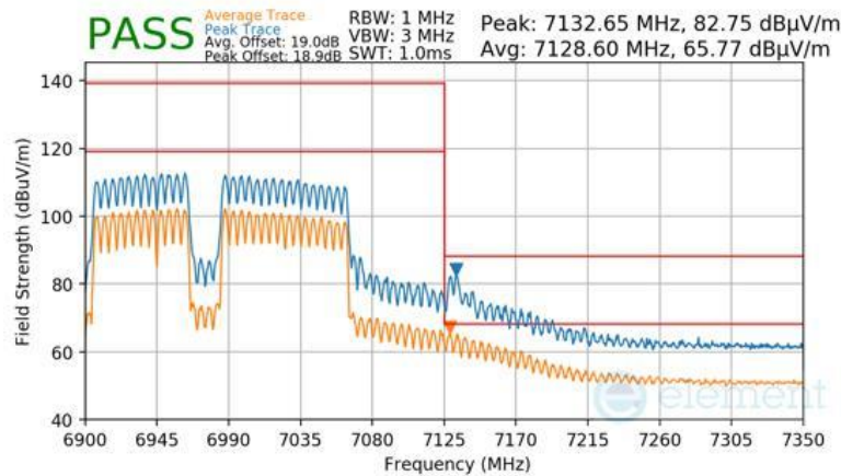
Plot 7-1147 SDM Diversity Radiated Upper Band Edge (Peak & Average – UNII Band 8) - RU996+484+242 (L)
