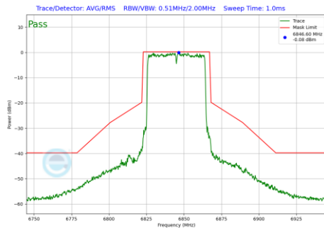
Plot 7-1052 In-Band Emission Plot CDD Primary Antenna WF5B (40MHz BW 802.11be(RU) RU484 Index65 (UNII Band 7) - Ch.179)
