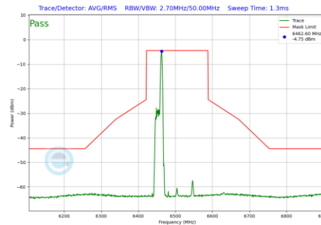
Plot 7-1090 In-Band Emission Plot CDD Primary Antenna WF8 (160MHz BW 802.11be(RU) RU26 Index17 (UNII Band 6) - Ch.111)
