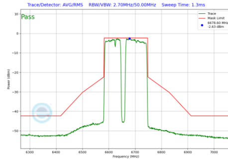
Plot 7-1119 In-Band Emission Plot CDD Primary Antenna WF8 (160MHz BW 802.11be(RU) RU996+484+242 Index99 (UNII Band 7) - Ch.143)
