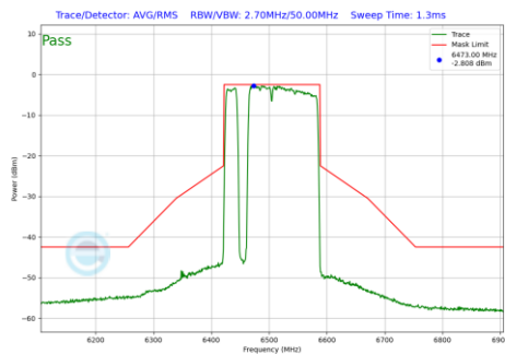
Plot 7-1116 In-Band Emission Plot CDD Primary Antenna WF8 (160MHz BW 802.11be(RU) RU996+484+242 Index97 (UNII Band 6) - Ch.111)
