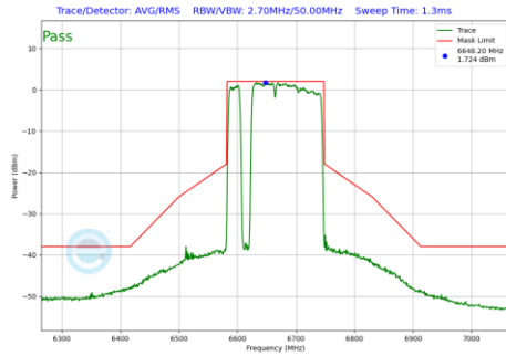
Plot 7-1033 In-Band Emission Plot CDD Primary Antenna WF5B (160MHz BW 802.11be(RU) RU996+484+242 Index97 (UNII Band 7) - Ch.143)
