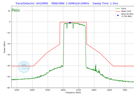
Plot 7-982 In-Band Emission Plot Antenna WF7 (160MHz BW 802.11be(RU) RU996+484+242 Index96 (UNII Band 7) - Ch.143)
