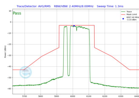
Plot 7-1113 In-Band Emission Plot CDD Primary Antenna WF8 (160MHz BW 802.11be(RU) RU996+484+242 Index97 (UNII Band 5) - Ch.15)
