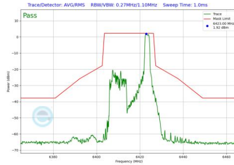
Plot 7-1013 In-Band Emission Plot CDD Primary Antenna WF8 (20MHz BW 802.11be(RU) RU26 Index8 (UNII Band 5) - Ch.93)
