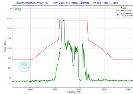
Plot 7-1095 In-Band Emission Plot CDD Primary Antenna WF8 (20MHz BW 802.11be(RU) RU26 Index0 (UNII Band 8) - Ch.189)
