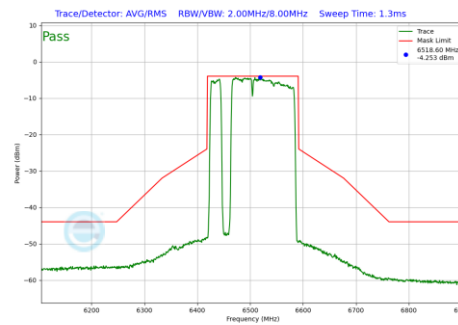
Plot 7-1104 In-Band Emission Plot CDD Primary Antenna WF5B (160MHz BW 802.11be(RU) RU996+484+242 Index97 (UNII Band 6) - Ch.111)
