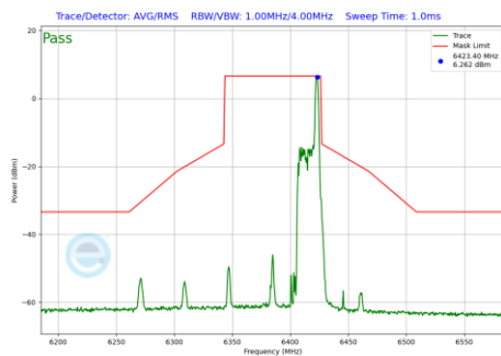
Plot 7-1003 In-Band Emission Plot CDD Primary Antenna WF5B (80MHz BW 802.11be(RU) RU26 Index36 (UNII Band 5) - Ch.87)
