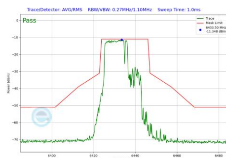
Plot 7-1114 In-Band Emission Plot CDD Primary Antenna WF8 (20MHz BW 802.11be(RU) RU106+26 Index82 (UNII Band 6) - Ch.97)
