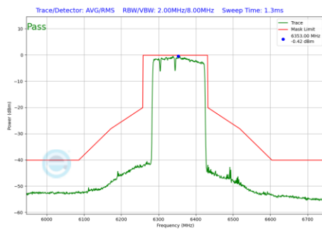
Plot 7-976 In-Band Emission Plot Antenna WF7 (160MHz BW 802.11be(RU) RU996+484+242 Index96 (UNII Band 5) - Ch.79)
