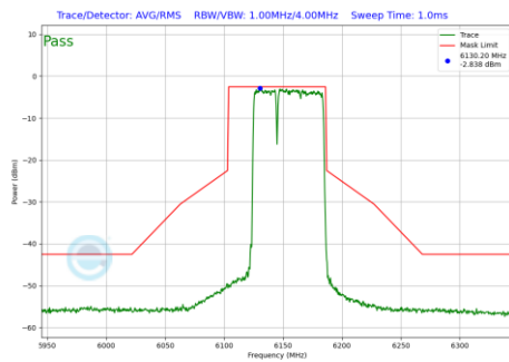
Plot 7-975 In-Band Emission Plot Antenna WF7 (80MHz BW 802.11be(RU) RU484+242 Index90 (UNII Band 5) - Ch.39)
