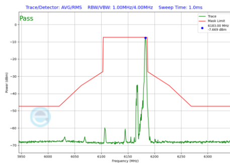
Plot 7-1069 In-Band Emission Plot CDD Primary Antenna WF5B (80MHz BW 802.11be(RU) RU26 Index36 (UNII Band 5) - Ch.39)
