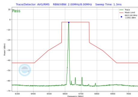
Plot 7-969 In-Band Emission Plot Antenna WF7 (160MHz BW 802.11be(RU) RU26 Index17 (UNII Band 7) - Ch.143)
