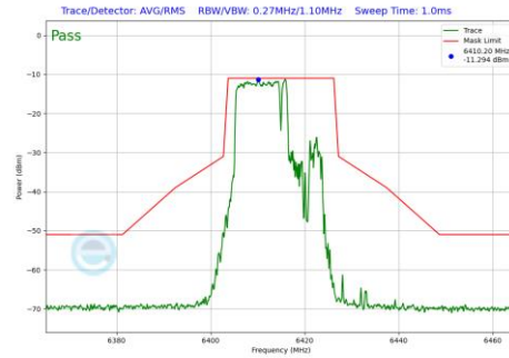
Plot 7-1111 In-Band Emission Plot CDD Primary Antenna WF8 (20MHz BW 802.11be(RU) RU106+26 Index82 (UNII Band 5) - Ch.93)
