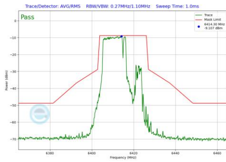
Plot 7-974 In-Band Emission Plot Antenna WF7 (20MHz BW 802.11be(RU) RU106+26 Index82 (UNII Band 5) - Ch.93)
