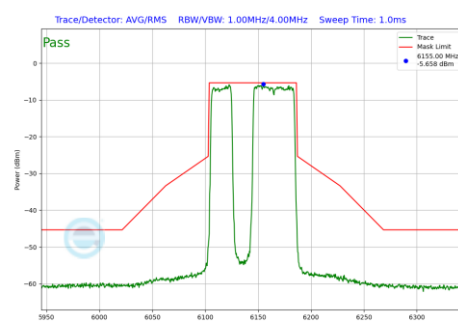
Plot 7-1112 In-Band Emission Plot CDD Primary Antenna WF8 (80MHz BW 802.11be(RU) RU484+242 Index91 (UNII Band 5) - Ch.39)
