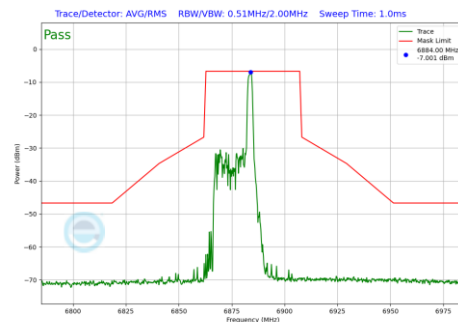
Plot 7-971 In-Band Emission Plot Antenna WF7 (40MHz BW 802.11be(RU) RU26 Index8 (UNII Band 8) - Ch.187)
