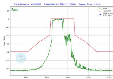
Plot 7-1040 In-Band Emission Plot CDD Primary Antenna WF8 (20MHz BW 802.11be(RU) RU106+26 Index82 (UNII Band 7) - Ch.117)
