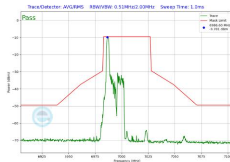
Plot 7-1080 In-Band Emission Plot CDD Primary Antenna WF5B (40MHz BW 802.11be(RU) RU26 Index0 (UNII Band 8) - Ch.211)
