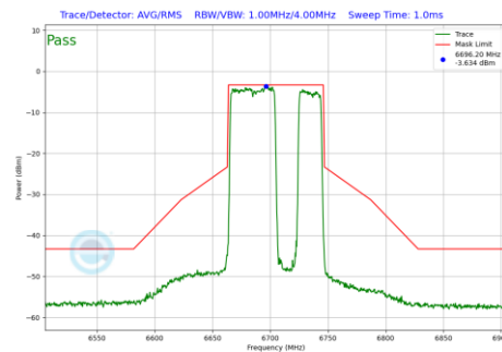
Plot 7-981 In-Band Emission Plot Antenna WF7 (80MHz BW 802.11be(RU) RU484+242 Index92 (UNII Band 7) - Ch.151)
