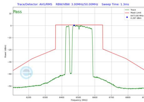
Plot 7-979 In-Band Emission Plot Antenna WF7 (160MHz BW 802.11be(RU) RU996+484+242 Index97 (UNII Band 6) - Ch.111)
