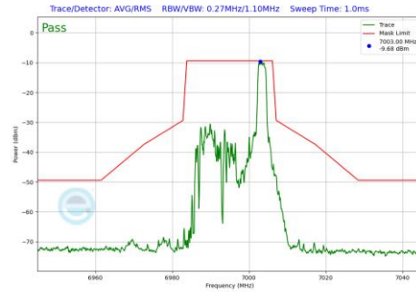
Plot 7-970 In-Band Emission Plot Antenna WF7 (20MHz BW 802.11be(RU) RU26 Index8 (UNII Band 8) - Ch.209)
