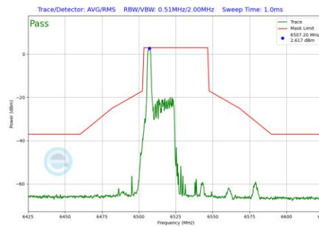
Plot 7-1006 In-Band Emission Plot CDD Primary Antenna WF5B (40MHz BW 802.11be(RU) RU26 Index0 (UNII Band 6) - Ch.115)
