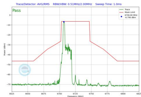
Plot 7-967 In-Band Emission Plot Antenna WF7 (40MHz BW 802.11be(RU) RU26 Index0 (UNII Band 7) - Ch.155)
