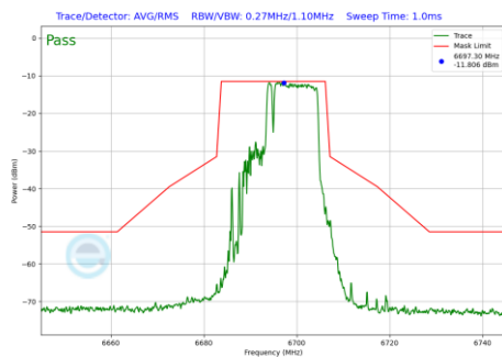
Plot 7-1117 In-Band Emission Plot CDD Primary Antenna WF8 (20MHz BW 802.11be(RU) RU106+26 Index83 (UNII Band 7) - Ch.149)
