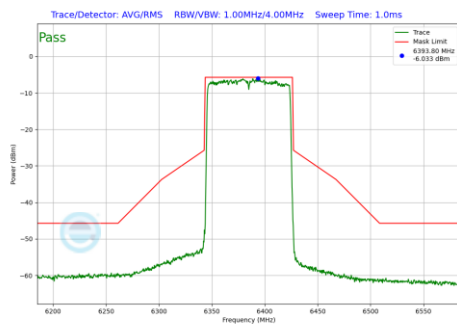
Plot 7-1124 In-Band Emission Plot CDD Primary Antenna WF5B (80MHz BW 802.11be(RU) RU996 Index67 (UNII Band 5) - Ch.87)
