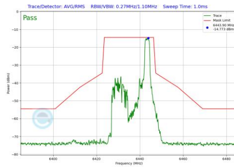
Plot 7-1071 In-Band Emission Plot CDD Primary Antenna WF5B (20MHz BW 802.11be(RU) RU26 Index8 (UNII Band 6) - Ch.97)
