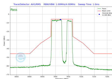
Plot 7-1120 In-Band Emission Plot CDD Primary Antenna WF8 (80MHz BW 802.11be(RU) RU484+242 Index92 (UNII Band 8) - Ch.215)
