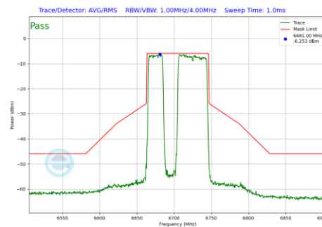
Plot 7-1106 In-Band Emission Plot CDD Primary Antenna WF5B (80MHz BW 802.11be(RU) RU484+242 Index91 (UNII Band 7) - Ch.151)
