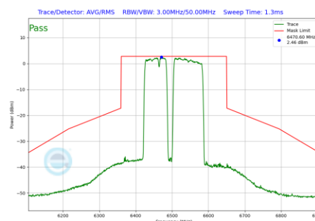
Plot 7-1039 In-Band Emission Plot CDD Primary Antenna WF8 (160MHz BW 802.11be(RU) RU996+484+242 Index99 (UNII Band 6) - Ch.111)
