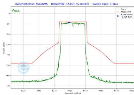
Plot 7-1123 In-Band Emission Plot CDD Primary Antenna WF5B (40MHz BW 802.11be(RU) RU484 Index65 (UNII Band 5) - Ch.91)
