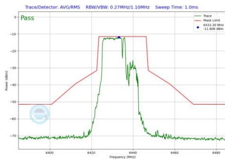
Plot 7-1102 In-Band Emission Plot CDD Primary Antenna WF5B (20MHz BW 802.11be(RU) RU106+26 Index82 (UNII Band 6) - Ch.97)
