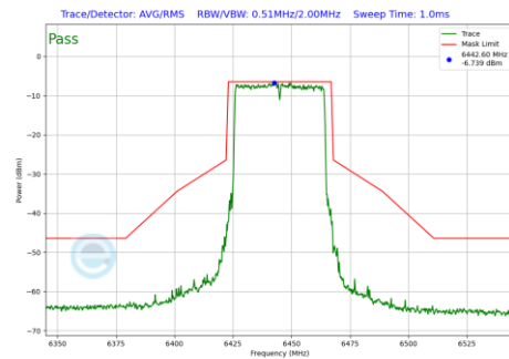
Plot 7-990 In-Band Emission Plot Antenna WF7 (40MHz BW 802.11be(RU) RU484 Index65 (UNII Band 6) - Ch.99)
