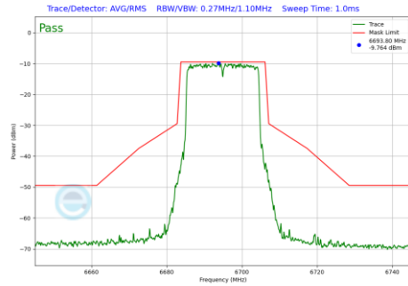
Plot 7-993 In-Band Emission Plot Antenna WF7 (20MHz BW 802.11be(RU) RU242 Index61 (UNII Band 7) - Ch.149)
