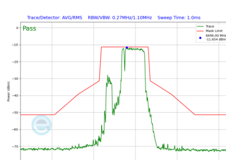
Plot 7-1105 In-Band Emission Plot CDD Primary Antenna WF5B (20MHz BW 802.11be(RU) RU106+26 Index83 (UNII Band 7) - Ch.149)
