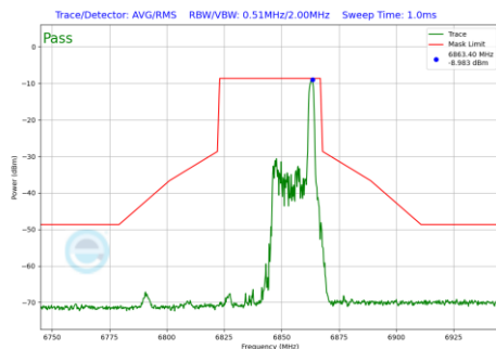
Plot 7-1076 In-Band Emission Plot CDD Primary Antenna WF5B (40MHz BW 802.11be(RU) RU26 Index17 (UNII Band 7) - Ch.179)
