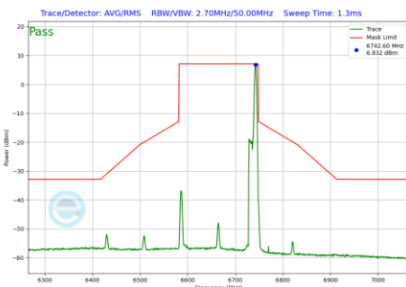
Plot 7-1012 In-Band Emission Plot CDD Primary Antenna WF5B (160MHz BW 802.11be(RU) RU26 Index36 (UNII Band 7) - Ch.143)
