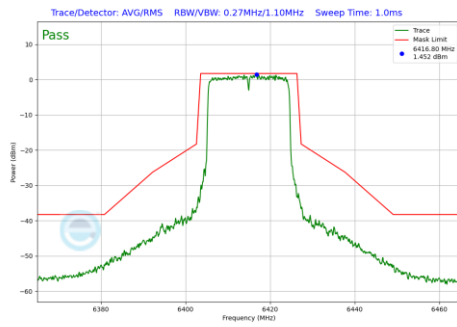
Plot 7-1043 In-Band Emission Plot CDD Primary Antenna WF5B (20MHz BW 802.11be(RU) RU242 Index61 (UNII Band 5) - Ch.93)
