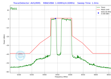
Plot 7-1029 In-Band Emission Plot CDD Primary Antenna WF5B (80MHz BW 802.11be(RU) RU484+242 Index91 (UNII Band 6) - Ch.103)
