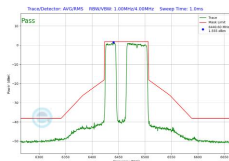
Plot 7-1038 In-Band Emission Plot CDD Primary Antenna WF8 (80MHz BW 802.11be(RU) RU484+242 Index91 (UNII Band 6) - Ch.103)
