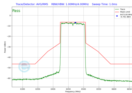
Plot 7-1128 In-Band Emission Plot CDD Primary Antenna WF5B (80MHz BW 802.11be(RU) RU996 Index67 (UNII Band 6) - Ch.103)
