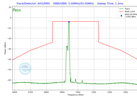
Plot 7-1098 In-Band Emission Plot CDD Primary Antenna WF8 (160MHz BW 802.11be(RU) RU26 Index17 (UNII Band 8) - Ch.207)
