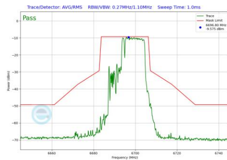
Plot 7-980 In-Band Emission Plot Antenna WF7 (20MHz BW 802.11be(RU) RU106+26 Index83 (UNII Band 7) - Ch.149)
