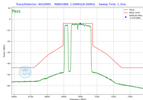
Plot 7-1110 In-Band Emission Plot CDD Primary Antenna WF5B (160MHz BW 802.11be(RU) RU996+484+242 Index97 (UNII Band 8) - Ch.207)
