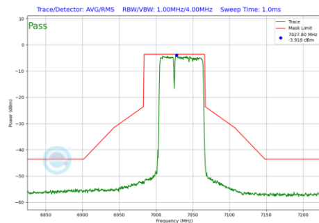
Plot 7-983 In-Band Emission Plot Antenna WF7 (80MHz BW 802.11be(RU) RU484+242 Index90 (UNII Band 8) - Ch.215)
