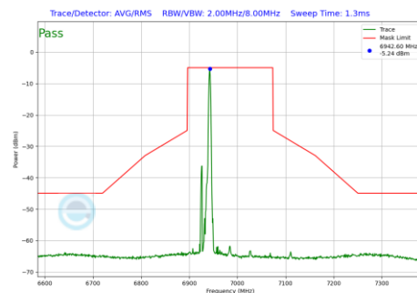
Plot 7-1082 In-Band Emission Plot CDD Primary Antenna WF5B (160MHz BW 802.11be(RU) RU26 Index17 (UNII Band 8) - Ch.207)
