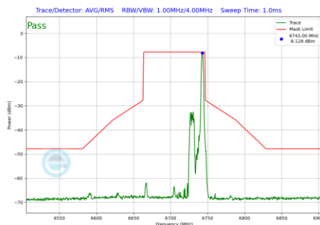
Plot 7-1077 In-Band Emission Plot CDD Primary Antenna WF5B (80MHz BW 802.11be(RU) RU26 Index36 (UNII Band 7) - Ch.151)
