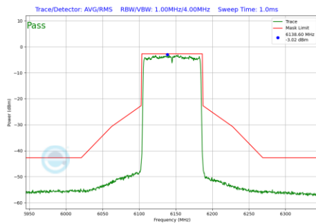
Plot 7-987 In-Band Emission Plot Antenna WF7 (80MHz BW 802.11be(RU) RU996 Index67 (UNII Band 5) - Ch.39)
