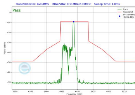
Plot 7-1072 In-Band Emission Plot CDD Primary Antenna WF5B (40MHz BW 802.11be(RU) RU26 Index8 (UNII Band 6) - Ch.99)
