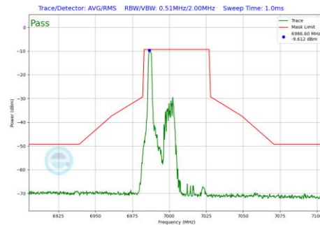
Plot 7-1096 In-Band Emission Plot CDD Primary Antenna WF8 (40MHz BW 802.11be(RU) RU26 Index0 (UNII Band 8) - Ch.211)
