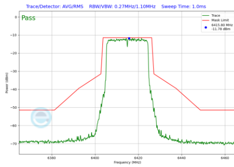
Plot 7-1122 In-Band Emission Plot CDD Primary Antenna WF5B (20MHz BW 802.11be(RU) RU242 Index61 (UNII Band 5) - Ch.93)
