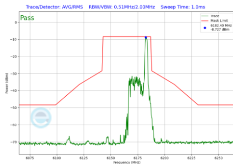
Plot 7-1068 In-Band Emission Plot CDD Primary Antenna WF5B (40MHz BW 802.11be(RU) RU26 Index17 (UNII Band 5) - Ch.43)
