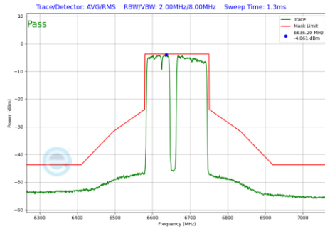
Plot 7-1107 In-Band Emission Plot CDD Primary Antenna WF5B (160MHz BW 802.11be(RU) RU996+484+242 Index99 (UNII Band 7) - Ch.143)
