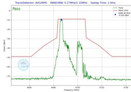
Plot 7-966 In-Band Emission Plot Antenna WF7 (20MHz BW 802.11be(RU) RU26 Index0 (UNII Band 7) - Ch.149)
