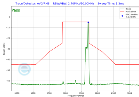
Plot 7-1094 In-Band Emission Plot CDD Primary Antenna WF8 (160MHz BW 802.11be(RU) RU26 Index36 (UNII Band 7) - Ch.143)
