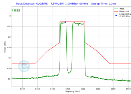
Plot 7-1103 In-Band Emission Plot CDD Primary Antenna WF5B (80MHz BW 802.11be(RU) RU484+242 Index91 (UNII Band 6) - Ch.103)
