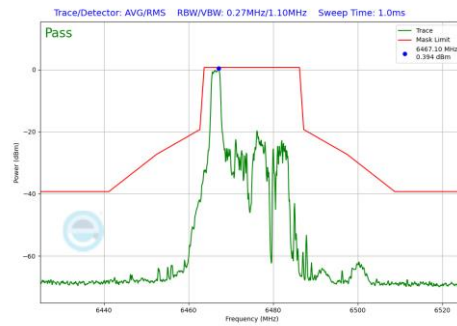
Plot 7-1005 In-Band Emission Plot CDD Primary Antenna WF5B (20MHz BW 802.11be(RU) RU26 Index0 (UNII Band 6) - Ch.105)
