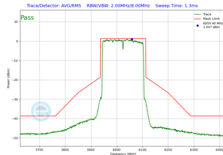
Plot 7-1058 In-Band Emission Plot CDD Primary Antenna WF8 (160MHz BW 802.11be(RU) RU996X2 Index68 (UNII Band 5) - Ch.15)
