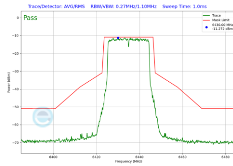
Plot 7-1126 In-Band Emission Plot CDD Primary Antenna WF5B (20MHz BW 802.11be(RU) RU242 Index61 (UNII Band 6) - Ch.97)
