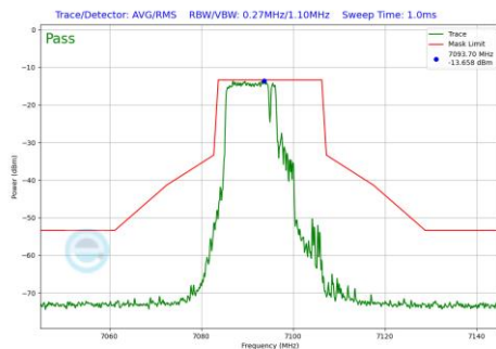
Plot 7-1108 In-Band Emission Plot CDD Primary Antenna WF5B (20MHz BW 802.11be(RU) RU106+26 Index82 (UNII Band 8) - Ch.229)
