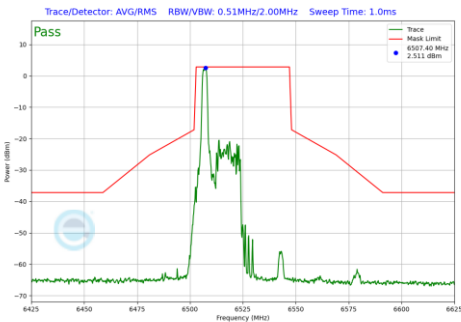
Plot 7-1018 In-Band Emission Plot CDD Primary Antenna WF8 (40MHz BW 802.11be(RU) RU26 Index0 (UNII Band 6) - Ch.115)
