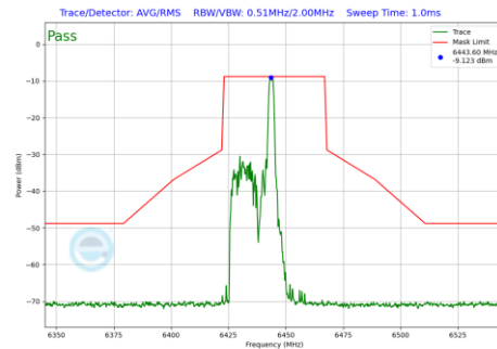
Plot 7-1088 In-Band Emission Plot CDD Primary Antenna WF8 (40MHz BW 802.11be(RU) RU26 Index8 (UNII Band 6) - Ch.99)
