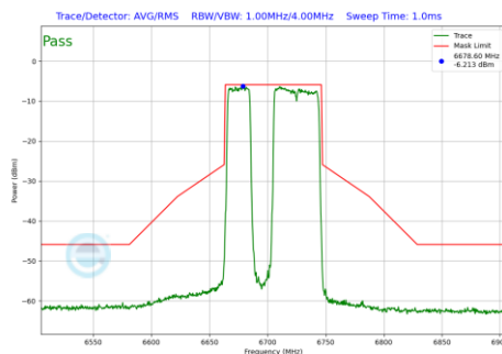
Plot 7-1118 In-Band Emission Plot CDD Primary Antenna WF8 (80MHz BW 802.11be(RU) RU484+242 Index91 (UNII Band 7) - Ch.151)
