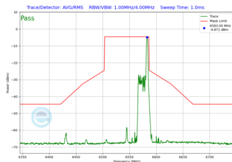
Plot 7-968 In-Band Emission Plot Antenna WF7 (80MHz BW 802.11be(RU) RU26 Index36 (UNII Band 7) - Ch.119)
