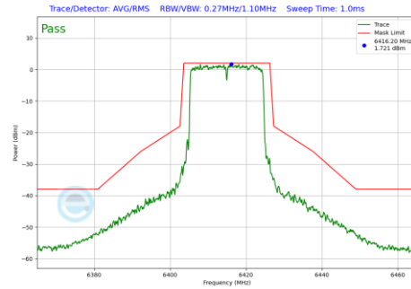
Plot 7-1055 In-Band Emission Plot CDD Primary Antenna WF8 (20MHz BW 802.11be(RU) RU242 Index61 (UNII Band 5) - Ch.93)
