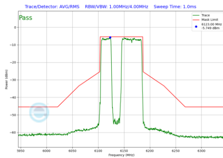
Plot 7-1100 In-Band Emission Plot CDD Primary Antenna WF5B (80MHz BW 802.11be(RU) RU484+242 Index91 (UNII Band 5) - Ch.39)
