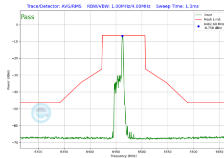
Plot 7-1089 In-Band Emission Plot CDD Primary Antenna WF8 (80MHz BW 802.11be(RU) RU26 Index17 (UNII Band 6) - Ch.103)
