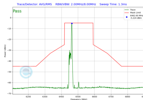
Plot 7-1074 In-Band Emission Plot CDD Primary Antenna WF5B (160MHz BW 802.11be(RU) RU26 Index17 (UNII Band 6) - Ch.111)
