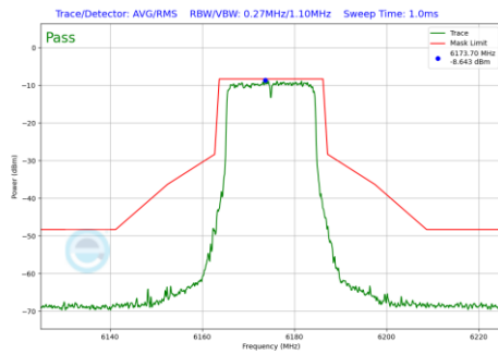
Plot 7-985 In-Band Emission Plot Antenna WF7 (20MHz BW 802.11be(RU) RU242 Index61 (UNII Band 5) - Ch.45)
