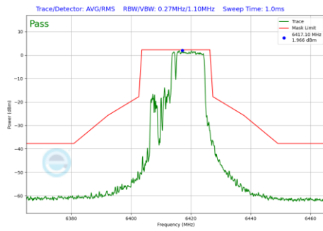
Plot 7-1025 In-Band Emission Plot CDD Primary Antenna WF5B (20MHz BW 802.11be(RU) RU106+26 Index83 (UNII Band 5) - Ch.93)
