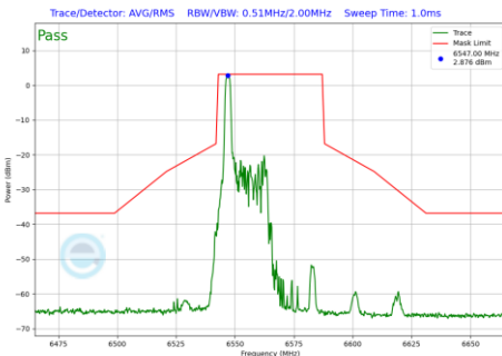
Plot 7-1010 In-Band Emission Plot CDD Primary Antenna WF5B (40MHz BW 802.11be(RU) RU26 Index0 (UNII Band 7) - Ch.123)
