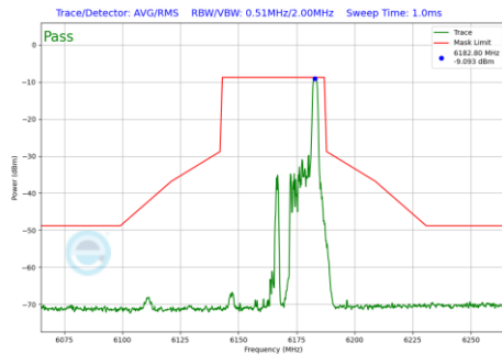
Plot 7-1084 In-Band Emission Plot CDD Primary Antenna WF8 (40MHz BW 802.11be(RU) RU26 Index17 (UNII Band 5) - Ch.43)
