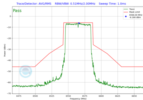
Plot 7-994 In-Band Emission Plot Antenna WF7 (40MHz BW 802.11be(RU) RU484 Index65 (UNII Band 7) - Ch.123)
