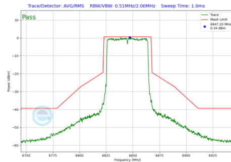
Plot 7-1064 In-Band Emission Plot CDD Primary Antenna WF8 (40MHz BW 802.11be(RU) RU484 Index65 (UNII Band 7) - Ch.179)
