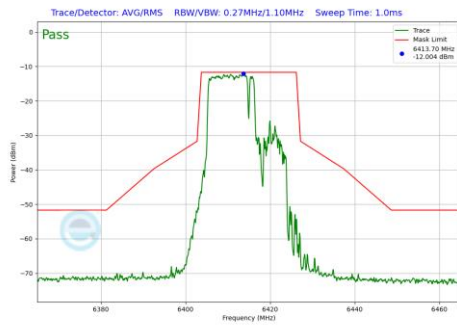
Plot 7-1099 In-Band Emission Plot CDD Primary Antenna WF5B (20MHz BW 802.11be(RU) RU106+26 Index82 (UNII Band 5) - Ch.93)
