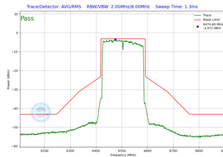
Plot 7-1129 In-Band Emission Plot CDD Primary Antenna WF5B (160MHz BW 802.11be(RU) RU996X2 Index68 (UNII Band 6) - Ch.111)
