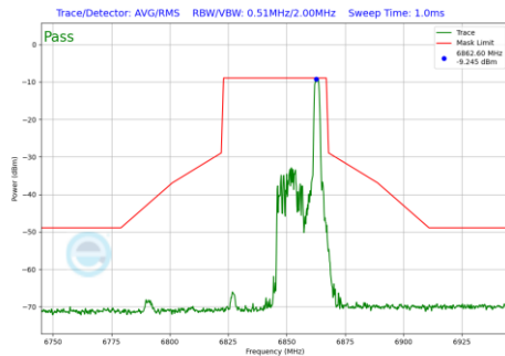
Plot 7-1092 In-Band Emission Plot CDD Primary Antenna WF8 (40MHz BW 802.11be(RU) RU26 Index17 (UNII Band 7) - Ch.179)
