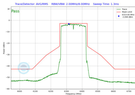
Plot 7-1125 In-Band Emission Plot CDD Primary Antenna WF5B (160MHz BW 802.11be(RU) RU996X2 Index68 (UNII Band 5) - Ch.79)
