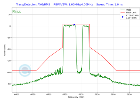
Plot 7-1041 In-Band Emission Plot CDD Primary Antenna WF8 (80MHz BW 802.11be(RU) RU484+242 Index92 (UNII Band 7) - Ch.167)
