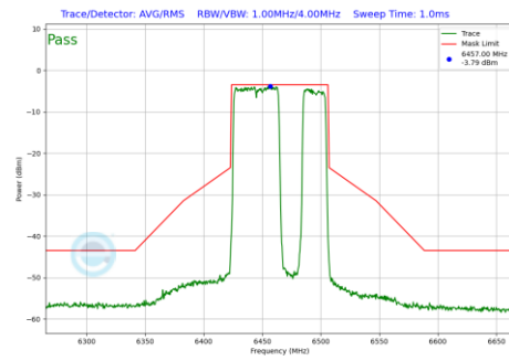
Plot 7-978 In-Band Emission Plot Antenna WF7 (80MHz BW 802.11be(RU) RU484+242 Index92 (UNII Band 6) - Ch.103)
