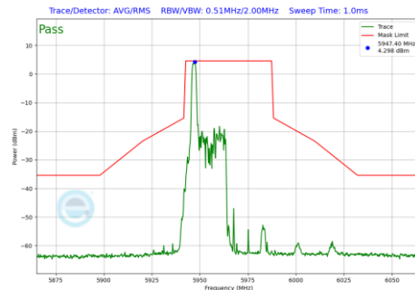
Plot 7-1014 In-Band Emission Plot CDD Primary Antenna WF8 (40MHz BW 802.11be(RU) RU26 Index0 (UNII Band 5) - Ch.3)
