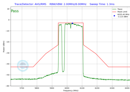
Plot 7-1101 In-Band Emission Plot CDD Primary Antenna WF5B (160MHz BW 802.11be(RU) RU996+484+242 Index97 (UNII Band 5) - Ch.15)
