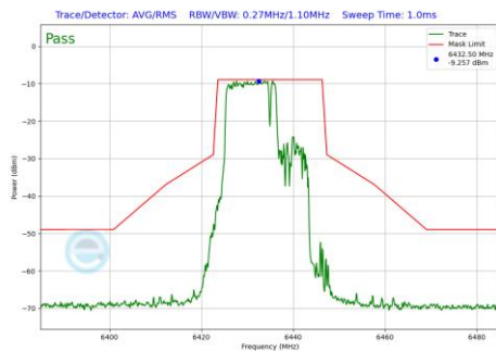
Plot 7-977 In-Band Emission Plot Antenna WF7 (20MHz BW 802.11be(RU) RU106+26 Index82 (UNII Band 6) - Ch.97)
