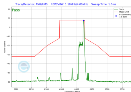
Plot 7-1015 In-Band Emission Plot CDD Primary Antenna WF8 (80MHz BW 802.11be(RU) RU26 Index36 (UNII Band 5) - Ch.87)
