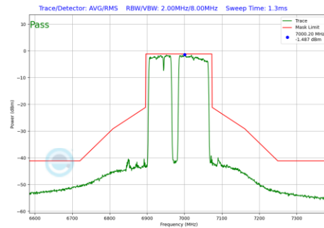
Plot 7-984 In-Band Emission Plot Antenna WF7 (160MHz BW 802.11be(RU) RU996+484+242 Index99 (UNII Band 8) - Ch.207)
