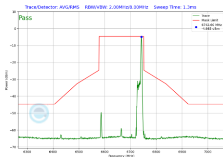
Plot 7-1078 In-Band Emission Plot CDD Primary Antenna WF5B (160MHz BW 802.11be(RU) RU26 Index36 (UNII Band 7) - Ch.143)
