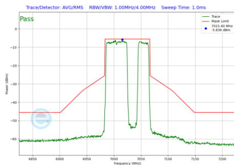
Plot 7-1109 In-Band Emission Plot CDD Primary Antenna WF5B (80MHz BW 802.11be(RU) RU484+242 Index92 (UNII Band 8) - Ch.215)
