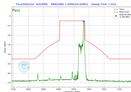
Plot 7-972 In-Band Emission Plot Antenna WF7 (80MHz BW 802.11be(RU) RU26 Index36 (UNII Band 8) - Ch.199)
