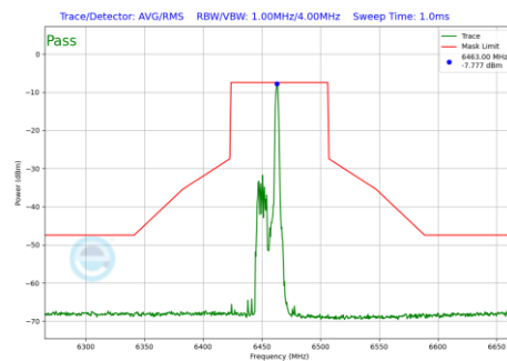
Plot 7-1073 In-Band Emission Plot CDD Primary Antenna WF5B (80MHz BW 802.11be(RU) RU26 Index17 (UNII Band 6) - Ch.103)
