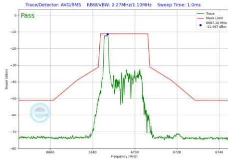
Plot 7-1075 In-Band Emission Plot CDD Primary Antenna WF5B (20MHz BW 802.11be(RU) RU26 Index0 (UNII Band 7) - Ch.149)
