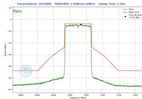
Plot 7-999 In-Band Emission Plot Antenna WF7 (80MHz BW 802.11be(RU) RU996 Index67 (UNII Band 8) - Ch.215)
