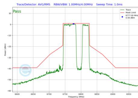
Plot 7-1032 In-Band Emission Plot CDD Primary Antenna WF5B (80MHz BW 802.11be(RU) RU484+242 Index92 (UNII Band 7) - Ch.167)
