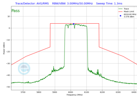
Plot 7-1036 In-Band Emission Plot CDD Primary Antenna WF8 (160MHz BW 802.11be(RU) RU996+484+242 Index96 (UNII Band 5) - Ch.15)
