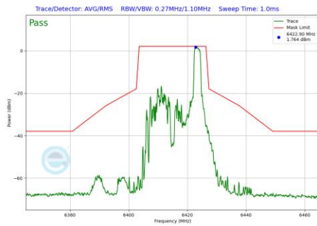
Plot 7-1001 In-Band Emission Plot CDD Primary Antenna WF5B (20MHz BW 802.11be(RU) RU26 Index8 (UNII Band 5) - Ch.93)
