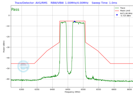
Plot 7-1115 In-Band Emission Plot CDD Primary Antenna WF8 (80MHz BW 802.11be(RU) RU484+242 Index91 (UNII Band 6) - Ch.103)
