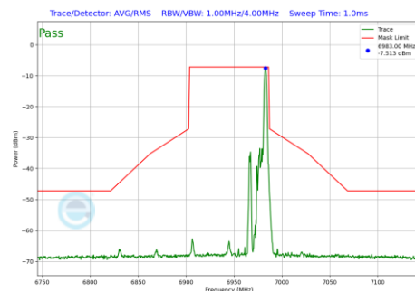
Plot 7-1081 In-Band Emission Plot CDD Primary Antenna WF5B (80MHz BW 802.11be(RU) RU26 Index36 (UNII Band 8) - Ch.199)
