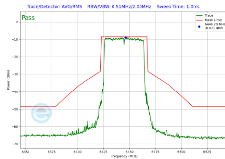
Plot 7-1127 In-Band Emission Plot CDD Primary Antenna WF5B (40MHz BW 802.11be(RU) RU484 Index65 (UNII Band 6) - Ch.99)
