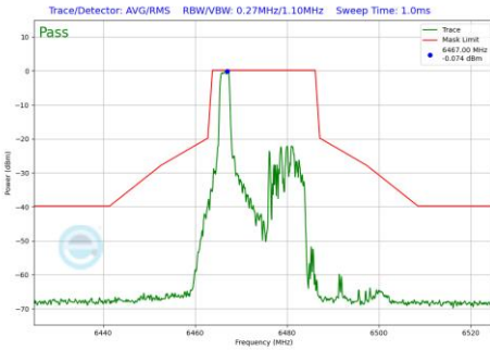
Plot 7-1017 In-Band Emission Plot CDD Primary Antenna WF8 (20MHz BW 802.11be(RU) RU26 Index0 (UNII Band 6) - Ch.105)
