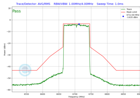
Plot 7-995 In-Band Emission Plot Antenna WF7 (80MHz BW 802.11be(RU) RU996 Index67 (UNII Band 7) - Ch.151)
