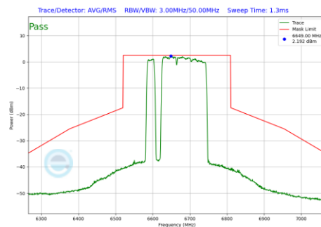
Plot 7-1042 In-Band Emission Plot CDD Primary Antenna WF8 (160MHz BW 802.11be(RU) RU996+484+242 Index97 (UNII Band 7) - Ch.143)
