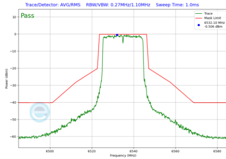
Plot 7-1051 In-Band Emission Plot CDD Primary Antenna WF5B (20MHz BW 802.11be(RU) RU242 Index61 (UNII Band 7) - Ch.117)
