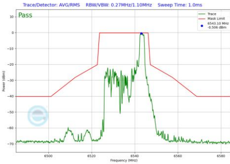
Plot 7-1009 In-Band Emission Plot CDD Primary Antenna WF5B (20MHz BW 802.11be(RU) RU26 Index8 (UNII Band 7) - Ch.117)
