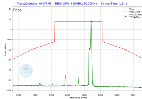
Plot 7-1024 In-Band Emission Plot CDD Primary Antenna WF8 (160MHz BW 802.11be(RU) RU26 Index36 (UNII Band 7) - Ch.143)
