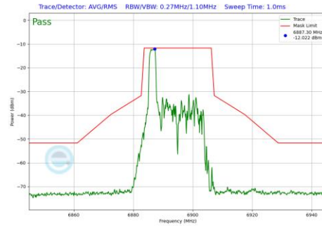
Plot 7-1079 In-Band Emission Plot CDD Primary Antenna WF5B (20MHz BW 802.11be(RU) RU26 Index0 (UNII Band 8) - Ch.189)
