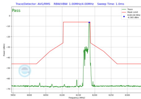
Plot 7-1085 In-Band Emission Plot CDD Primary Antenna WF8 (80MHz BW 802.11be(RU) RU26 Index36 (UNII Band 5) - Ch.39)
