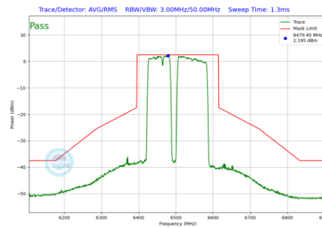
Plot 7-1030 In-Band Emission Plot CDD Primary Antenna WF5B (160MHz BW 802.11be(RU) RU996+484+242 Index99 (UNII Band 6) - Ch.111)
