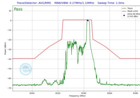
Plot 7-1021 In-Band Emission Plot CDD Primary Antenna WF8 (20MHz BW 802.11be(RU) RU26 Index8 (UNII Band 7) - Ch.117)
