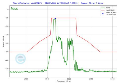
Plot 7-1067 In-Band Emission Plot CDD Primary Antenna WF5B (20MHz BW 802.11be(RU) RU26 Index0 (UNII Band 5) - Ch.1)
