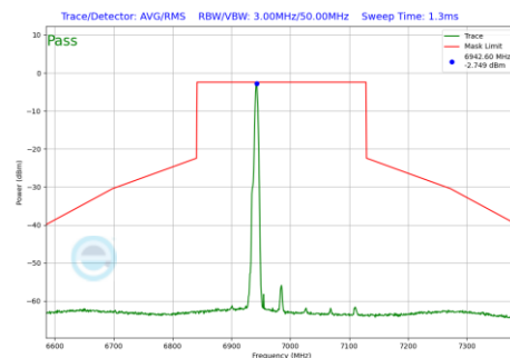
Plot 7-973 In-Band Emission Plot Antenna WF7 (160MHz BW 802.11be(RU) RU26 Index17 (UNII Band 8) - Ch.207)
