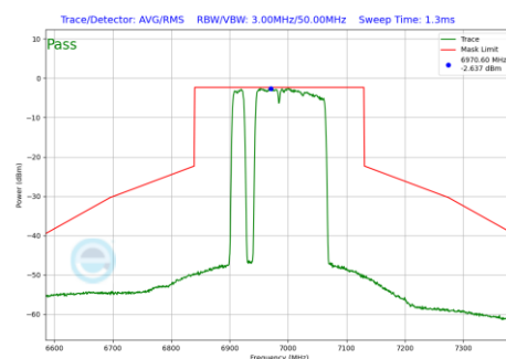
Plot 7-1121 In-Band Emission Plot CDD Primary Antenna WF8 (160MHz BW 802.11be(RU) RU996+484+242 Index97 (UNII Band 8) - Ch.207)
