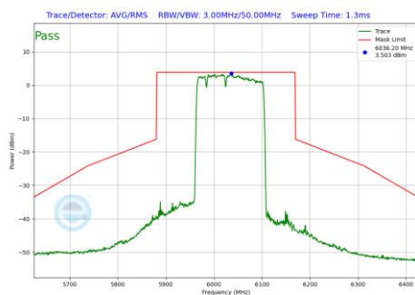
Plot 7-1027 In-Band Emission Plot CDD Primary Antenna WF5B (160MHz BW 802.11be(RU) RU996+484+242 Index96 (UNII Band 5) - Ch.15)
