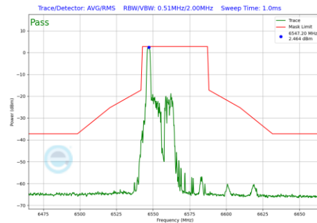
Plot 7-1022 In-Band Emission Plot CDD Primary Antenna WF8 (40MHz BW 802.11be(RU) RU26 Index0 (UNII Band 7) - Ch.123)
