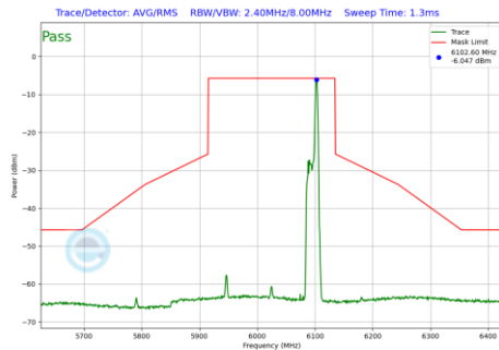
Plot 7-1086 In-Band Emission Plot CDD Primary Antenna WF8 (160MHz BW 802.11be(RU) RU26 Index36 (UNII Band 5) - Ch.15)
