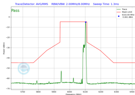
Plot 7-1070 In-Band Emission Plot CDD Primary Antenna WF5B (160MHz BW 802.11be(RU) RU26 Index36 (UNII Band 5) - Ch.15)
