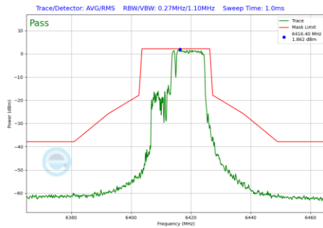
Plot 7-1034 In-Band Emission Plot CDD Primary Antenna WF8 (20MHz BW 802.11be(RU) RU106+26 Index83 (UNII Band 5) - Ch.93)
