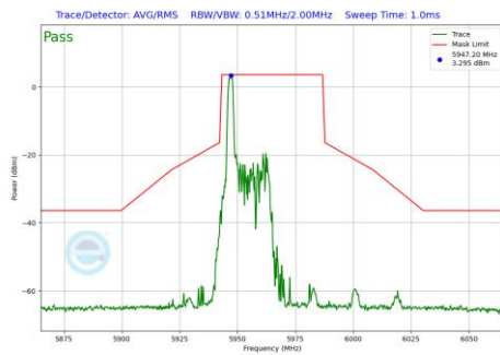
Plot 7-1002 In-Band Emission Plot CDD Primary Antenna WF5B (40MHz BW 802.11be(RU) RU26 Index0 (UNII Band 5) - Ch.3)
