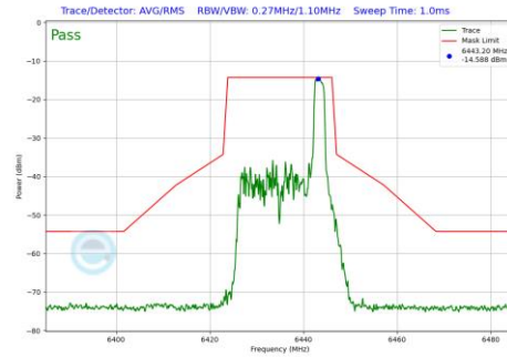
Plot 7-1087 In-Band Emission Plot CDD Primary Antenna WF8 (20MHz BW 802.11be(RU) RU26 Index8 (UNII Band 6) - Ch.97)
