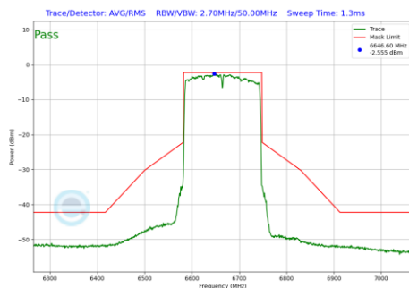
Plot 7-1149 In-Band Emission Plot CDD Primary Antenna WF8 (160MHz BW 802.11be(RU) RU996X2 Index68 (UNII Band 7) - Ch.143)
