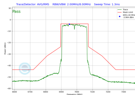
Plot 7-1289 In-Band Emission Plot CDD Diversity Antenna WF7 (160MHz BW 802.11be(RU) RU996X2 Index68 (UNII Band 8) - Ch.207)
