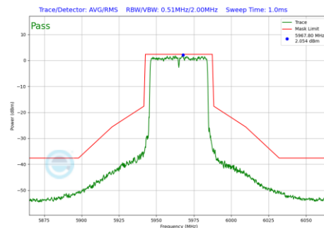
Plot 7-1209 In-Band Emission Plot CDD Diversity Antenna WF8 (40MHz BW 802.11be(RU) RU484 Index65 (UNII Band 5) - Ch.3)
