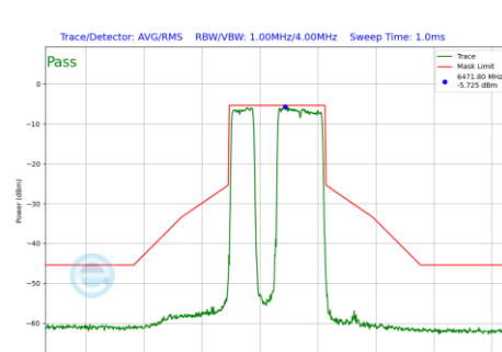
Plot 7-1267 In-Band Emission Plot SDM Diversity Antenna WF8 (80MHz BW 802.11be(RU) RU484+242 Index91 (UNII Band 6) - Ch.103)
