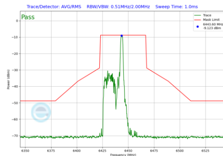
Plot 7-1241 In-Band Emission Plot CDD Diversity Antenna WF8 (40MHz BW 802.11be(RU) RU26 Index8 (UNII Band 6) - Ch.99)
