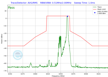
Plot 7-1171 In-Band Emission Plot CDD Diversity Antenna WF8 (40MHz BW 802.11be(RU) RU26 Index17 (UNII Band 6) - Ch.99)
