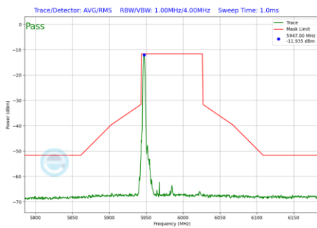
Plot 7-1222 In-Band Emission Plot CDD Diversity Antenna WF7 (80MHz BW 802.11be(RU) RU26 Index0 (UNII Band 5) - Ch.7)
