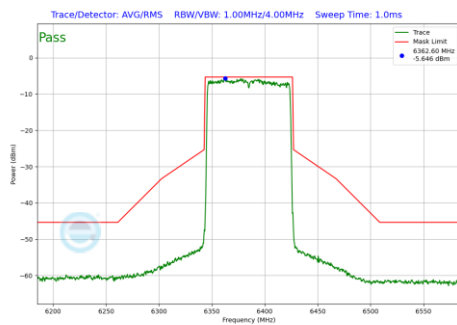
Plot 7-1276 In-Band Emission Plot CDD Diversity Antenna WF7 (80MHz BW 802.11be(RU) RU996 Index67 (UNII Band 5) - Ch.87)
