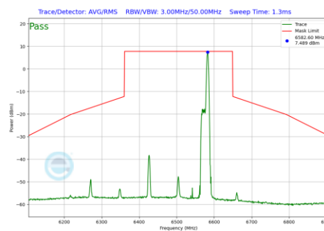
Plot 7-1161 In-Band Emission Plot CDD Diversity Antenna WF7 (160MHz BW 802.11be(RU) RU26 Index36 (UNII Band 6) - Ch.111)
