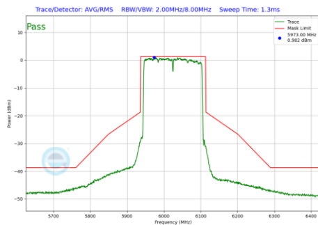
Plot 7-1199 In-Band Emission Plot CDD Diversity Antenna WF7 (160MHz BW 802.11be(RU) RU996X2 Index68 (UNII Band 5) - Ch.15)
