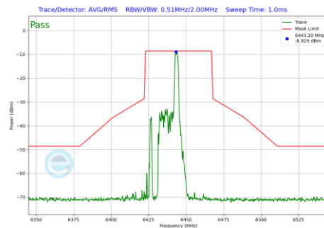
Plot 7-1225 In-Band Emission Plot CDD Diversity Antenna WF7 (40MHz BW 802.11be(RU) RU26 Index8 (UNII Band 6) - Ch.99)
