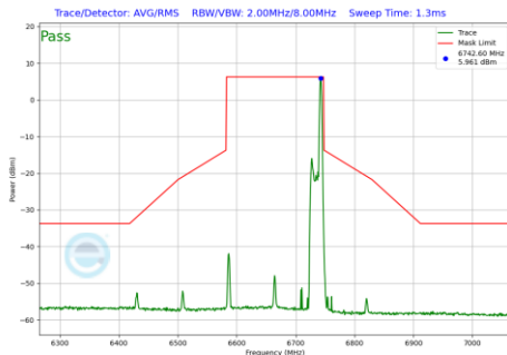
Plot 7-1165 In-Band Emission Plot CDD Diversity Antenna WF7 (160MHz BW 802.11be(RU) RU26 Index36 (UNII Band 7) - Ch.143)
