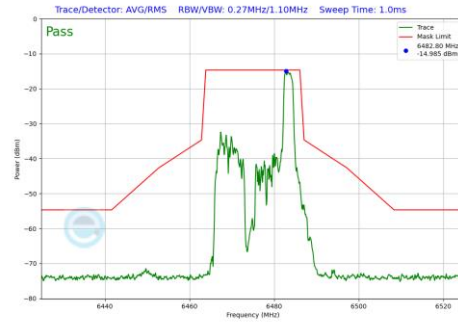
Plot 7-1240 In-Band Emission Plot CDD Diversity Antenna WF8 (20MHz BW 802.11be(RU) RU26 Index8 (UNII Band 6) - Ch.105)
