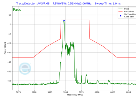
Plot 7-1167 In-Band Emission Plot CDD Diversity Antenna WF8 (40MHz BW 802.11be(RU) RU26 Index0 (UNII Band 5) - Ch.3)
