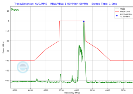
Plot 7-1164 In-Band Emission Plot CDD Diversity Antenna WF7 (80MHz BW 802.11be(RU) RU26 Index36 (UNII Band 7) - Ch.167)
