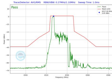
Plot 7-1174 In-Band Emission Plot CDD Diversity Antenna WF8 (20MHz BW 802.11be(RU) RU26 Index0 (UNII Band 7) - Ch.117)
