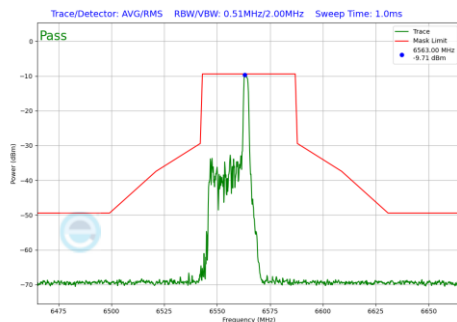
Plot 7-1229 In-Band Emission Plot CDD Diversity Antenna WF7 (40MHz BW 802.11be(RU) RU26 Index8 (UNII Band 7) - Ch.123)
