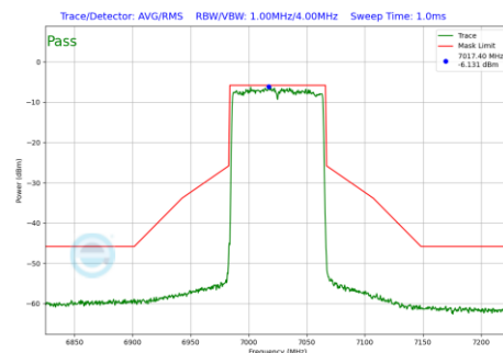
Plot 7-1288 In-Band Emission Plot CDD Diversity Antenna WF7 (80MHz BW 802.11be(RU) RU996 Index67 (UNII Band 8) - Ch.215)
