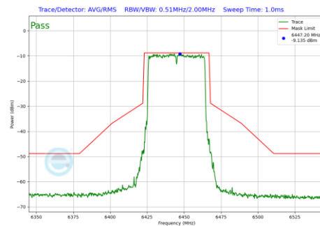
Plot 7-1295 In-Band Emission Plot CDD Diversity Antenna WF8 (40MHz BW 802.11be(RU) RU484 Index65 (UNII Band 6) - Ch.99)
