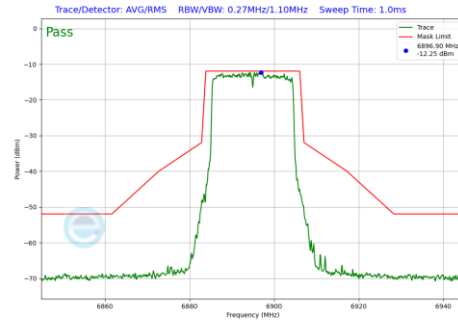
Plot 7-1150 In-Band Emission Plot CDD Primary Antenna WF8 (20MHz BW 802.11be(RU) RU242 Index61 (UNII Band 8) - Ch.189)
