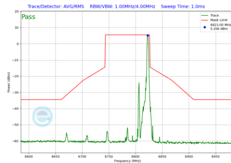
Plot 7-1176 In-Band Emission Plot CDD Diversity Antenna WF8 (80MHz BW 802.11be(RU) RU26 Index36 (UNII Band 7) - Ch.167)
