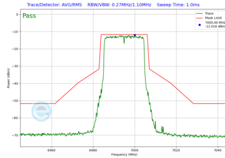
Plot 7-1302 In-Band Emission Plot CDD Diversity Antenna WF8 (20MHz BW 802.11be(RU) RU242 Index61 (UNII Band 8) - Ch.209)
