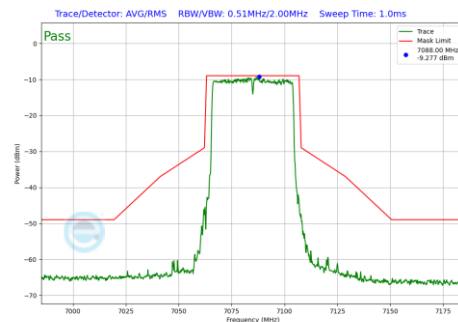
Plot 7-1287 In-Band Emission Plot CDD Diversity Antenna WF7 (40MHz BW 802.11be(RU) RU484 Index65 (UNII Band 8) - Ch.227)
