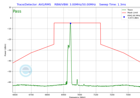
Plot 7-1235 In-Band Emission Plot CDD Diversity Antenna WF7 (160MHz BW 802.11be(RU) RU26 Index17 (UNII Band 8) - Ch.207)
