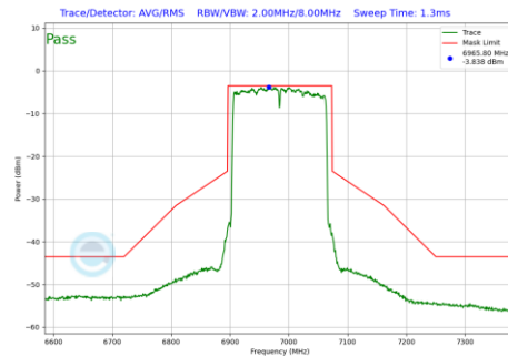
Plot 7-1137 In-Band Emission Plot CDD Primary Antenna WF5B (160MHz BW 802.11be(RU) RU996X2 Index68 (UNII Band 8) - Ch.207)
