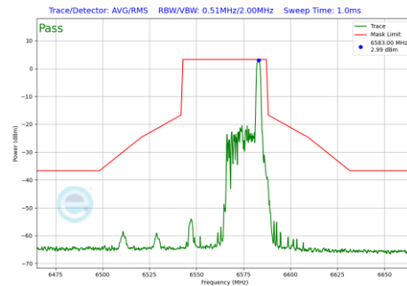
Plot 7-1175 In-Band Emission Plot CDD Diversity Antenna WF8 (40MHz BW 802.11be(RU) RU26 Index17 (UNII Band 7) - Ch.123)
