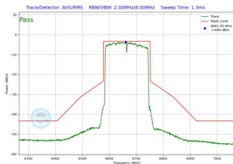
Plot 7-1285 In-Band Emission Plot CDD Diversity Antenna WF7 (160MHz BW 802.11be(RU) RU996X2 Index68 (UNII Band 7) - Ch.143)
