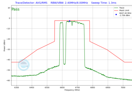
Plot 7-1260 In-Band Emission Plot CDD Diversity Antenna WF7 (160MHz BW 802.11be(RU) RU996+484+242 Index97 (UNII Band 7) - Ch.143)
