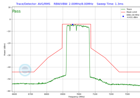
Plot 7-1262 In-Band Emission Plot CDD Diversity Antenna WF7 (160MHz BW 802.11be(RU) RU996+484+242 Index96 (UNII Band 8) - Ch.207)
