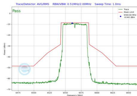
Plot 7-1299 In-Band Emission Plot CDD Diversity Antenna WF8 (40MHz BW 802.11be(RU) RU484 Index65 (UNII Band 7) - Ch.123)
