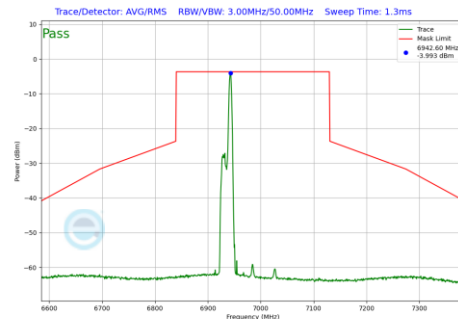
Plot 7-1251 In-Band Emission Plot CDD Diversity Antenna WF8 (160MHz BW 802.11be(RU) RU26 Index17 (UNII Band 8) - Ch.207)
