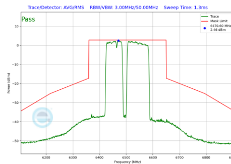
Plot 7-1192 In-Band Emission Plot CDD Diversity Antenna WF8 (160MHz BW 802.11be(RU) RU996+484+242 Index99 (UNII Band 6) - Ch.111)
