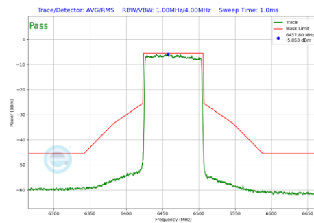
Plot 7-1280 In-Band Emission Plot CDD Diversity Antenna WF7 (80MHz BW 802.11be(RU) RU996 Index67 (UNII Band 6) - Ch.103)
