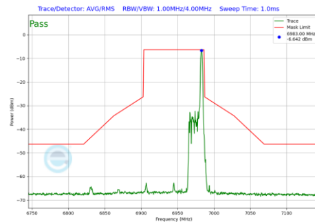
Plot 7-1250 In-Band Emission Plot CDD Diversity Antenna WF8 (80MHz BW 802.11be(RU) RU26 Index36 (UNII Band 8) - Ch.199)
