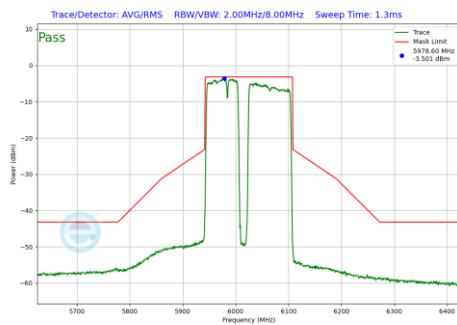
Plot 7-1254 In-Band Emission Plot CDD Diversity Antenna WF7 (160MHz BW 802.11be(RU) RU996+484+242 Index99 (UNII Band 5) - Ch.15)
