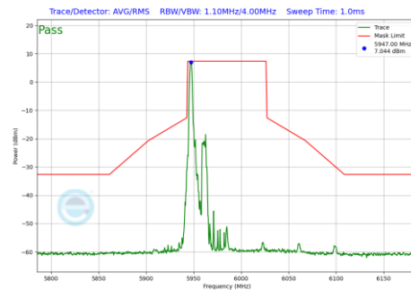
Plot 7-1168 In-Band Emission Plot CDD Diversity Antenna WF8 (80MHz BW 802.11be(RU) RU26 Index0 (UNII Band 5) - Ch.7)
