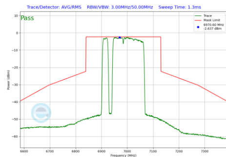
Plot 7-1273 In-Band Emission Plot SDM Diversity Antenna WF8 (160MHz BW 802.11be(RU) RU996+484+242 Index97 (UNII Band 8) - Ch.207)
