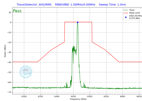
Plot 7-1160 In-Band Emission Plot CDD Diversity Antenna WF7 (80MHz BW 802.11be(RU) RU26 Index17 (UNII Band 6) - Ch.103)
