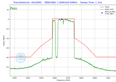
Plot 7-1186 In-Band Emission Plot CDD Diversity Antenna WF7 (160MHz BW 802.11be(RU) RU996+484+242 Index97 (UNII Band 7) - Ch.143)
