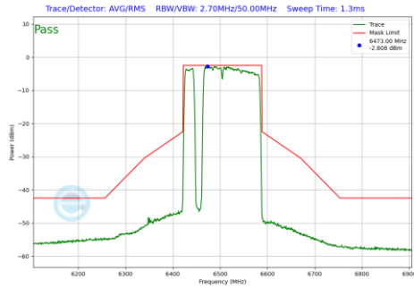
Plot 7-1268 In-Band Emission Plot SDM Diversity Antenna WF8 (160MHz BW 802.11be(RU) RU996+484+242 Index97 (UNII Band 6) - Ch.111)
