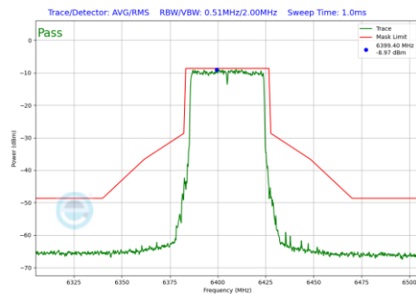
Plot 7-1291 In-Band Emission Plot CDD Diversity Antenna WF8 (40MHz BW 802.11be(RU) RU484 Index65 (UNII Band 5) - Ch.91)
