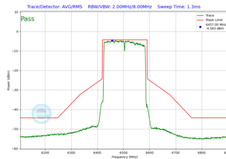
Plot 7-1281 In-Band Emission Plot CDD Diversity Antenna WF7 (160MHz BW 802.11be(RU) RU996X2 Index68 (UNII Band 6) - Ch.111)
