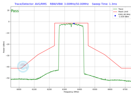
Plot 7-1277 In-Band Emission Plot CDD Diversity Antenna WF7 (160MHz BW 802.11be(RU) RU996X2 Index68 (UNII Band 5) - Ch.79)
