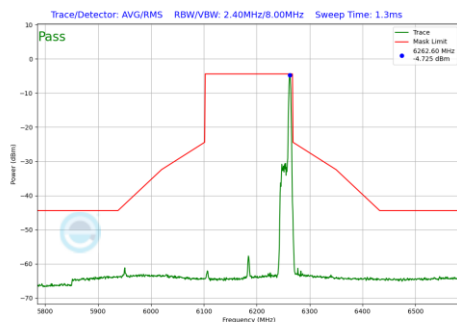
Plot 7-1239 In-Band Emission Plot CDD Diversity Antenna WF8 (160MHz BW 802.11be(RU) RU26 Index36 (UNII Band 5) - Ch.47)
