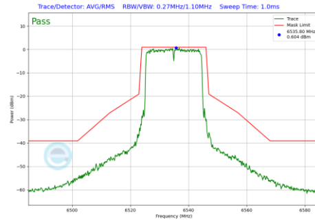
Plot 7-1216 In-Band Emission Plot CDD Diversity Antenna WF8 (20MHz BW 802.11be(RU) RU242 Index61 (UNII Band 7) - Ch.117)
