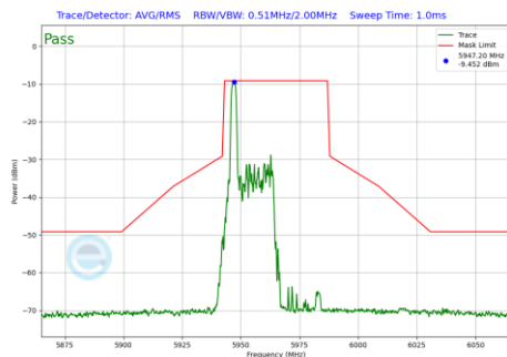
Plot 7-1237 In-Band Emission Plot CDD Diversity Antenna WF8 (40MHz BW 802.11be(RU) RU26 Index0 (UNII Band 5) - Ch.3)
