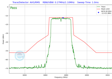
Plot 7-1130 In-Band Emission Plot CDD Primary Antenna WF5B (20MHz BW 802.11be(RU) RU242 Index61 (UNII Band 7) - Ch.185)
