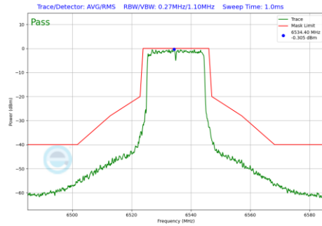
Plot 7-1204 In-Band Emission Plot CDD Diversity Antenna WF7 (20MHz BW 802.11be(RU) RU242 Index61 (UNII Band 7) - Ch.117)
