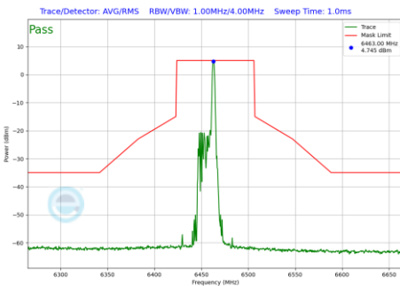
Plot 7-1172 In-Band Emission Plot CDD Diversity Antenna WF8 (80MHz BW 802.11be(RU) RU26 Index17 (UNII Band 6) - Ch.103)
