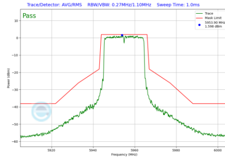
Plot 7-1208 In-Band Emission Plot CDD Diversity Antenna WF8 (20MHz BW 802.11be(RU) RU242 Index61 (UNII Band 5) - Ch.1)
