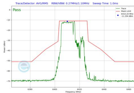
Plot 7-1263 In-Band Emission Plot SDM Diversity Antenna WF8 (20MHz BW 802.11be(RU) RU106+26 Index82 (UNII Band 5) - Ch.93)
