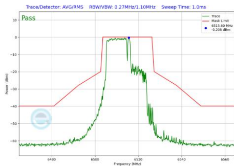
Plot 7-1181 In-Band Emission Plot CDD Diversity Antenna WF7 (20MHz BW 802.11be(RU) RU106+26 Index82 (UNII Band 6) - Ch.113)
