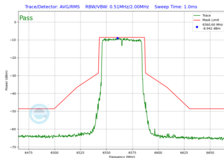
Plot 7-1147 In-Band Emission Plot CDD Primary Antenna WF8 (40MHz BW 802.11be(RU) RU484 Index65 (UNII Band 7) - Ch.123)
