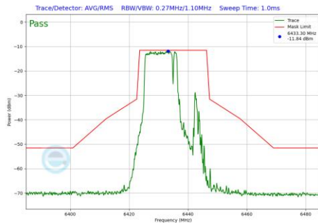
Plot 7-1255 In-Band Emission Plot CDD Diversity Antenna WF7 (20MHz BW 802.11be(RU) RU106+26 Index82 (UNII Band 6) - Ch.97)
