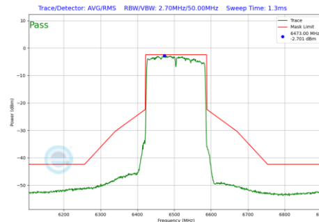
Plot 7-1145 In-Band Emission Plot CDD Primary Antenna WF8 (160MHz BW 802.11be(RU) RU996X2 Index68 (UNII Band 6) - Ch.111)
