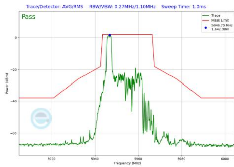
Plot 7-1154 In-Band Emission Plot CDD Diversity Antenna WF7 (20MHz BW 802.11be(RU) RU26 Index0 (UNII Band 5) - Ch.1)
