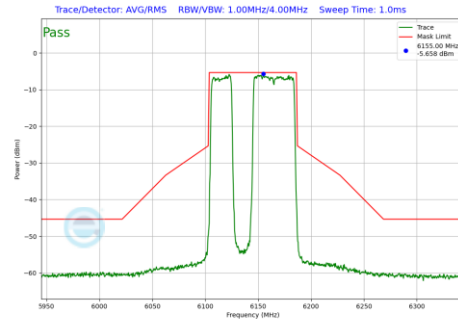
Plot 7-1264 In-Band Emission Plot SDM Diversity Antenna WF8 (80MHz BW 802.11be(RU) RU484+242 Index91 (UNII Band 5) - Ch.39)
