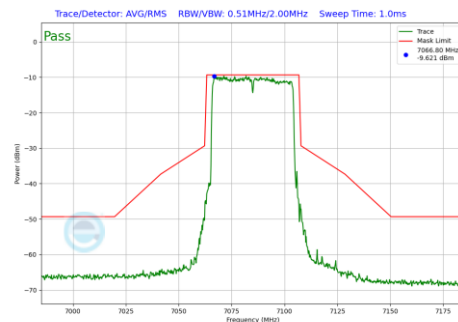
Plot 7-1151 In-Band Emission Plot CDD Primary Antenna WF8 (40MHz BW 802.11be(RU) RU484 Index65 (UNII Band 8) - Ch.227)
