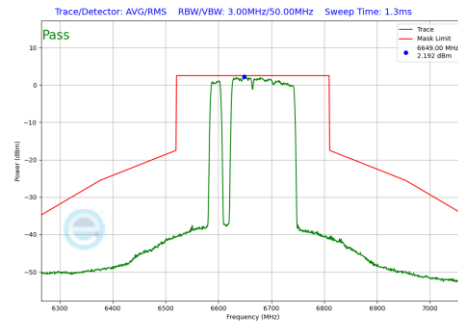
Plot 7-1195 In-Band Emission Plot CDD Diversity Antenna WF8 (160MHz BW 802.11be(RU) RU996+484+242 Index97 (UNII Band 7) - Ch.143)
