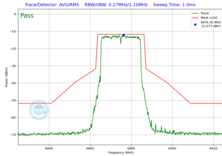
Plot 7-1146 In-Band Emission Plot CDD Primary Antenna WF8 (20MHz BW 802.11be(RU) RU242 Index61 (UNII Band 7) - Ch.185)
