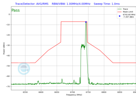
Plot 7-1246 In-Band Emission Plot CDD Diversity Antenna WF8 (80MHz BW 802.11be(RU) RU26 Index36 (UNII Band 7) - Ch.151)
