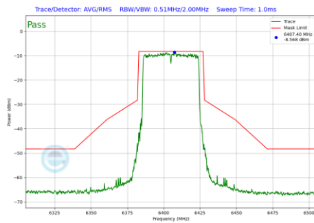
Plot 7-1275 In-Band Emission Plot CDD Diversity Antenna WF7 (40MHz BW 802.11be(RU) RU484 Index65 (UNII Band 5) - Ch.91)
