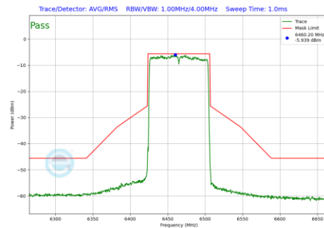
Plot 7-1144 In-Band Emission Plot CDD Primary Antenna WF8 (80MHz BW 802.11be(RU) RU996 Index67 (UNII Band 6) - Ch.103)
