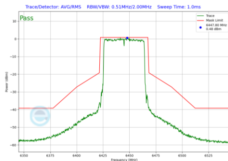
Plot 7-1213 In-Band Emission Plot CDD Diversity Antenna WF8 (40MHz BW 802.11be(RU) RU484 Index65 (UNII Band 6) - Ch.99)
