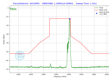
Plot 7-1226 In-Band Emission Plot CDD Diversity Antenna WF7 (80MHz BW 802.11be(RU) RU26 Index36 (UNII Band 6) - Ch.103)
