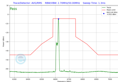
Plot 7-1247 In-Band Emission Plot CDD Diversity Antenna WF8 (160MHz BW 802.11be(RU) RU26 Index17 (UNII Band 7) - Ch.143)
