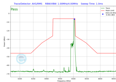
Plot 7-1242 In-Band Emission Plot CDD Diversity Antenna WF8 (80MHz BW 802.11be(RU) RU26 Index36 (UNII Band 6) - Ch.103)
