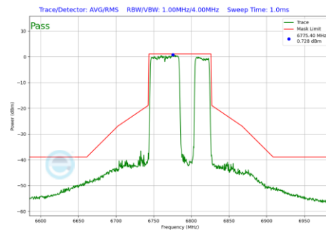
Plot 7-1185 In-Band Emission Plot CDD Diversity Antenna WF7 (80MHz BW 802.11be(RU) RU484+242 Index92 (UNII Band 7) - Ch.167)
