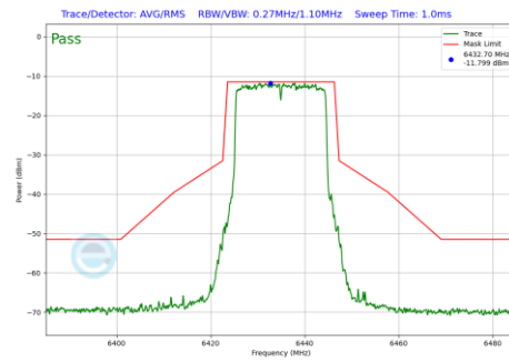
Plot 7-1278 In-Band Emission Plot CDD Diversity Antenna WF7 (20MHz BW 802.11be(RU) RU242 Index61 (UNII Band 6) - Ch.97)
