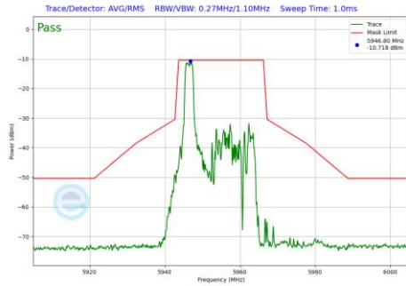
Plot 7-1236 In-Band Emission Plot CDD Diversity Antenna WF8 (20MHz BW 802.11be(RU) RU26 Index0 (UNII Band 5) - Ch.1)
