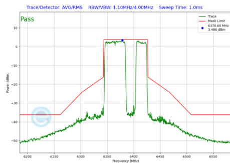
Plot 7-1188 In-Band Emission Plot CDD Diversity Antenna WF8 (80MHz BW 802.11be(RU) RU484+242 Index92 (UNII Band 5) - Ch.87)
