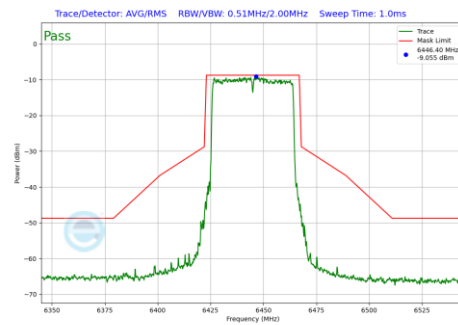
Plot 7-1279 In-Band Emission Plot CDD Diversity Antenna WF7 (40MHz BW 802.11be(RU) RU484 Index65 (UNII Band 6) - Ch.99)
