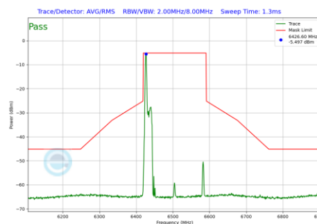
Plot 7-1227 In-Band Emission Plot CDD Diversity Antenna WF7 (160MHz BW 802.11be(RU) RU26 Index0 (UNII Band 6) - Ch.111)
