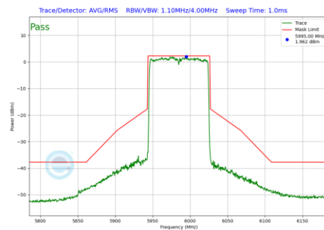
Plot 7-1210 In-Band Emission Plot CDD Diversity Antenna WF8 (80MHz BW 802.11be(RU) RU996 Index67 (UNII Band 5) - Ch.7)
