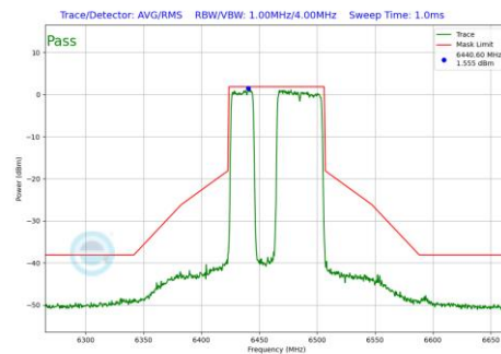
Plot 7-1191 In-Band Emission Plot CDD Diversity Antenna WF8 (80MHz BW 802.11be(RU) RU484+242 Index91 (UNII Band 6) - Ch.103)
