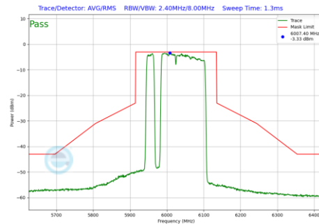
Plot 7-1265 In-Band Emission Plot SDM Diversity Antenna WF8 (160MHz BW 802.11be(RU) RU996+484+242 Index97 (UNII Band 5) - Ch.15)
