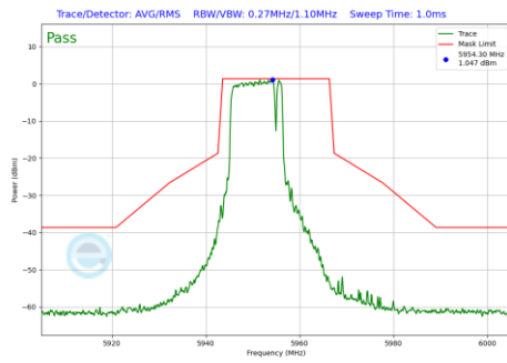
Plot 7-1178 In-Band Emission Plot CDD Diversity Antenna WF7 (20MHz BW 802.11be(RU) RU106+26 Index82 (UNII Band 5) - Ch.1)
