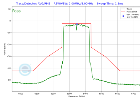
Plot 7-1141 In-Band Emission Plot CDD Primary Antenna WF8 (160MHz BW 802.11be(RU) RU996X2 Index68 (UNII Band 5) - Ch.79)
