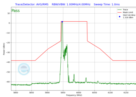
Plot 7-1156 In-Band Emission Plot CDD Diversity Antenna WF7 (80MHz BW 802.11be(RU) RU26 Index0 (UNII Band 5) - Ch.7)
