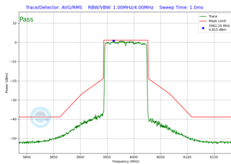
Plot 7-1198 In-Band Emission Plot CDD Diversity Antenna WF7 (80MHz BW 802.11be(RU) RU996 Index67 (UNII Band 5) - Ch.7)
