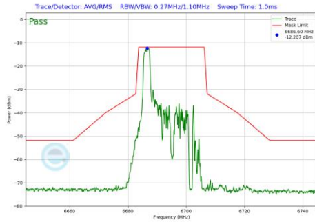
Plot 7-1228 In-Band Emission Plot CDD Diversity Antenna WF7 (20MHz BW 802.11be(RU) RU26 Index0 (UNII Band 7) - Ch.149)
