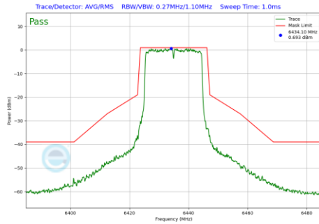
Plot 7-1212 In-Band Emission Plot CDD Diversity Antenna WF8 (20MHz BW 802.11be(RU) RU242 Index61 (UNII Band 6) - Ch.97)
