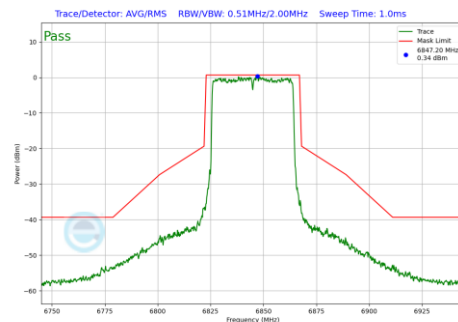
Plot 7-1217 In-Band Emission Plot CDD Diversity Antenna WF8 (40MHz BW 802.11be(RU) RU484 Index65 (UNII Band 7) - Ch.179)
