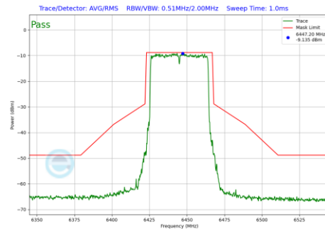
Plot 7-1143 In-Band Emission Plot CDD Primary Antenna WF8 (40MHz BW 802.11be(RU) RU484 Index65 (UNII Band 6) - Ch.99)
