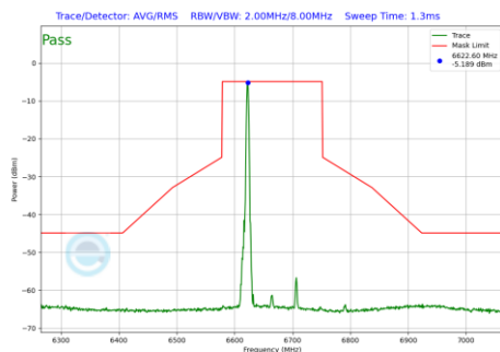
Plot 7-1231 In-Band Emission Plot CDD Diversity Antenna WF7 (160MHz BW 802.11be(RU) RU26 Index17 (UNII Band 7) - Ch.143)
