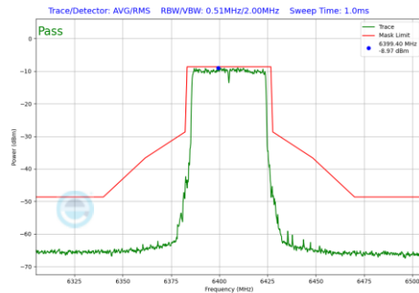
Plot 7-1139 In-Band Emission Plot CDD Primary Antenna WF8 (40MHz BW 802.11be(RU) RU484 Index65 (UNII Band 5) - Ch.91)
