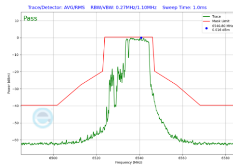
Plot 7-1184 In-Band Emission Plot CDD Diversity Antenna WF7 (20MHz BW 802.11be(RU) RU106+26 Index83 (UNII Band 7) - Ch.117)
