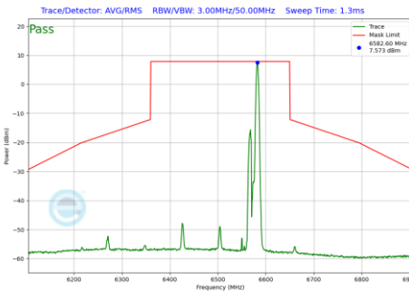
Plot 7-1173 In-Band Emission Plot CDD Diversity Antenna WF8 (160MHz BW 802.11be(RU) RU26 Index36 (UNII Band 6) - Ch.111)
