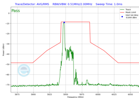
Plot 7-1221 In-Band Emission Plot CDD Diversity Antenna WF7 (40MHz BW 802.11be(RU) RU26 Index0 (UNII Band 5) - Ch.3)
