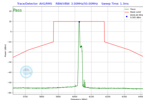
Plot 7-1169 In-Band Emission Plot CDD Diversity Antenna WF8 (160MHz BW 802.11be(RU) RU26 Index0 (UNII Band 5) - Ch.15)
