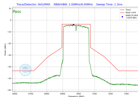
Plot 7-1305 In-Band Emission Plot CDD Diversity Antenna WF8 (160MHz BW 802.11be(RU) RU996X2 Index68 (UNII Band 8) - Ch.207)
