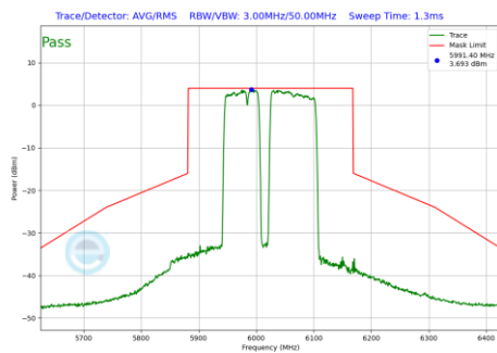
Plot 7-1180 In-Band Emission Plot CDD Diversity Antenna WF7 (160MHz BW 802.11be(RU) RU996+484+242 Index99 (UNII Band 5) - Ch.15)
