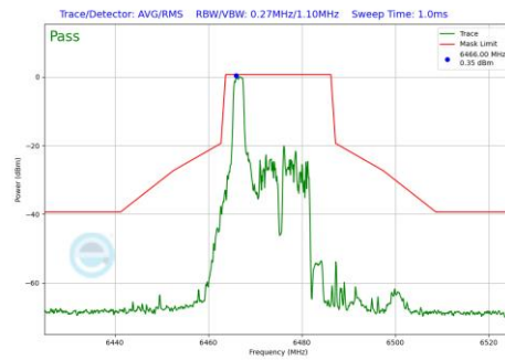
Plot 7-1158 In-Band Emission Plot CDD Diversity Antenna WF7 (20MHz BW 802.11be(RU) RU26 Index0 (UNII Band 6) - Ch.105)
