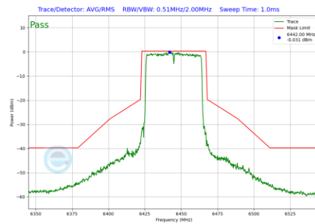
Plot 7-1201 In-Band Emission Plot CDD Diversity Antenna WF7 (40MHz BW 802.11be(RU) RU484 Index65 (UNII Band 6) - Ch.99)
