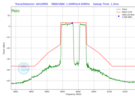
Plot 7-1179 In-Band Emission Plot CDD Diversity Antenna WF7 (80MHz BW 802.11be(RU) RU484+242 Index92 (UNII Band 5) - Ch.7)
