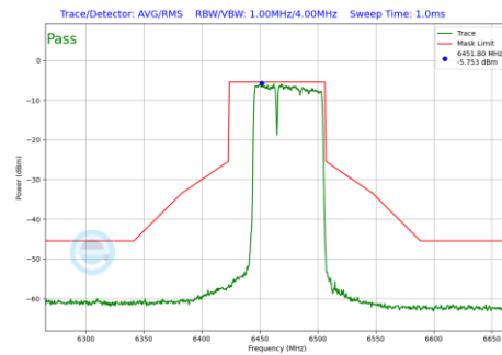
Plot 7-1256 In-Band Emission Plot CDD Diversity Antenna WF7 (80MHz BW 802.11be(RU) RU484+242 Index90 (UNII Band 6) - Ch.103)
