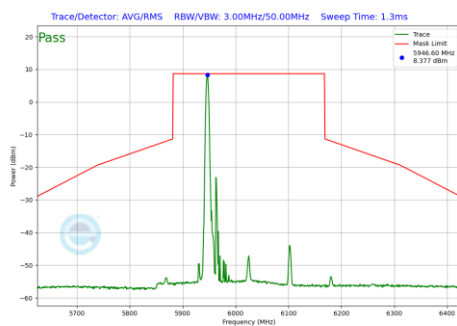
Plot 7-1157 In-Band Emission Plot CDD Diversity Antenna WF7 (160MHz BW 802.11be(RU) RU26 Index0 (UNII Band 5) - Ch.15)
