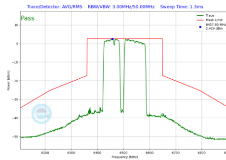
Plot 7-1183 In-Band Emission Plot CDD Diversity Antenna WF7 (160MHz BW 802.11be(RU) RU996+484+242 Index99 (UNII Band 6) - Ch.111)
