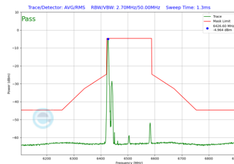
Plot 7-1243 In-Band Emission Plot CDD Diversity Antenna WF8 (160MHz BW 802.11be(RU) RU26 Index0 (UNII Band 6) - Ch.111)
