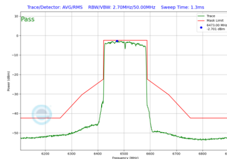
Plot 7-1297 In-Band Emission Plot CDD Diversity Antenna WF8 (160MHz BW 802.11be(RU) RU996X2 Index68 (UNII Band 6) - Ch.111)
