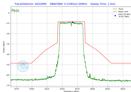
Plot 7-1283 In-Band Emission Plot CDD Diversity Antenna WF7 (40MHz BW 802.11be(RU) RU484 Index65 (UNII Band 7) - Ch.123)
