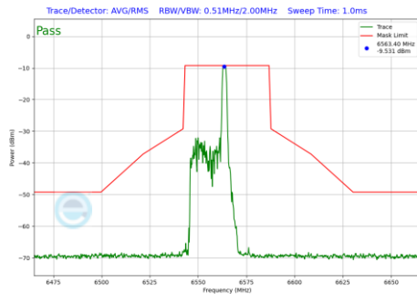
Plot 7-1245 In-Band Emission Plot CDD Diversity Antenna WF8 (40MHz BW 802.11be(RU) RU26 Index8 (UNII Band 7) - Ch.123)
