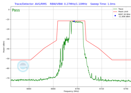
Plot 7-1269 In-Band Emission Plot SDM Diversity Antenna WF8 (20MHz BW 802.11be(RU) RU106+26 Index83 (UNII Band 7) - Ch.149)
