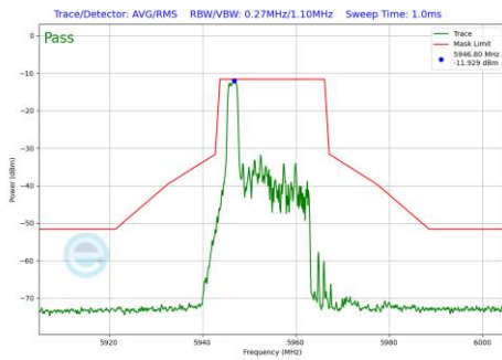
Plot 7-1220 In-Band Emission Plot CDD Diversity Antenna WF7 (20MHz BW 802.11be(RU) RU26 Index0 (UNII Band 5) - Ch.1)
