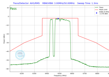
Plot 7-1257 In-Band Emission Plot CDD Diversity Antenna WF7 (160MHz BW 802.11be(RU) RU996+484+242 Index97 (UNII Band 6) - Ch.111)
