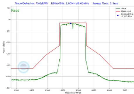
Plot 7-1133 In-Band Emission Plot CDD Primary Antenna WF5B (160MHz BW 802.11be(RU) RU996X2 Index68 (UNII Band 7) - Ch.143)
