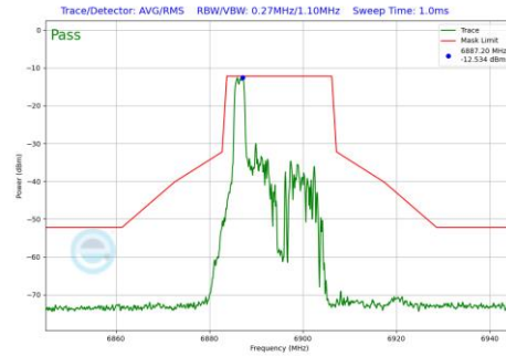
Plot 7-1232 In-Band Emission Plot CDD Diversity Antenna WF7 (20MHz BW 802.11be(RU) RU26 Index0 (UNII Band 8) - Ch.189)
