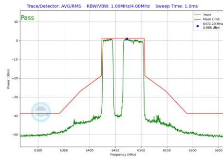
Plot 7-1182 In-Band Emission Plot CDD Diversity Antenna WF7 (80MHz BW 802.11be(RU) RU484+242 Index91 (UNII Band 6) - Ch.103)
