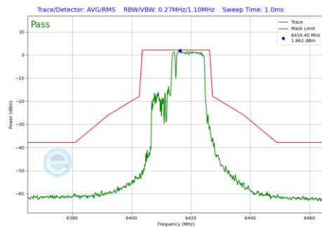
Plot 7-1187 In-Band Emission Plot CDD Diversity Antenna WF8 (20MHz BW 802.11be(RU) RU106+26 Index83 (UNII Band 5) - Ch.93)
