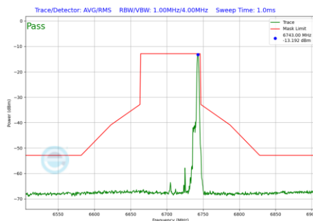
Plot 7-1230 In-Band Emission Plot CDD Diversity Antenna WF7 (80MHz BW 802.11be(RU) RU26 Index36 (UNII Band 7) - Ch.151)
