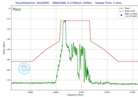
Plot 7-1244 In-Band Emission Plot CDD Diversity Antenna WF8 (20MHz BW 802.11be(RU) RU26 Index0 (UNII Band 7) - Ch.149)
