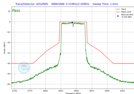
Plot 7-1205 In-Band Emission Plot CDD Diversity Antenna WF7 (40MHz BW 802.11be(RU) RU484 Index65 (UNII Band 7) - Ch.179)
