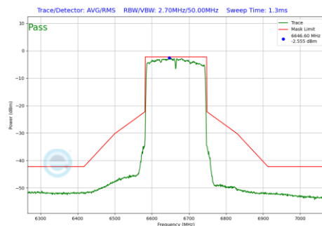
Plot 7-1301 In-Band Emission Plot CDD Diversity Antenna WF8 (160MHz BW 802.11be(RU) RU996X2 Index68 (UNII Band 7) - Ch.143)
