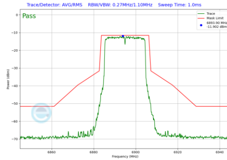
Plot 7-1134 In-Band Emission Plot CDD Primary Antenna WF5B (20MHz BW 802.11be(RU) RU242 Index61 (UNII Band 8) - Ch.189)
