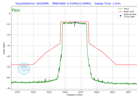
Plot 7-1131 In-Band Emission Plot CDD Primary Antenna WF5B (40MHz BW 802.11be(RU) RU484 Index65 (UNII Band 7) - Ch.123)
