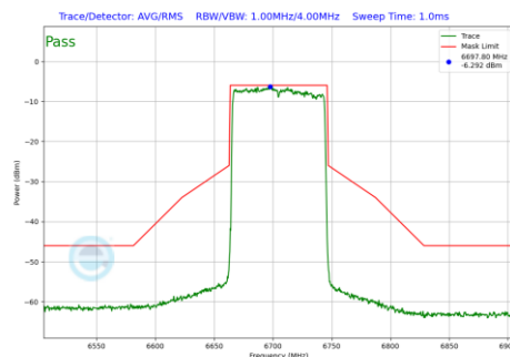
Plot 7-1300 In-Band Emission Plot CDD Diversity Antenna WF8 (80MHz BW 802.11be(RU) RU996 Index67 (UNII Band 7) - Ch.151)
