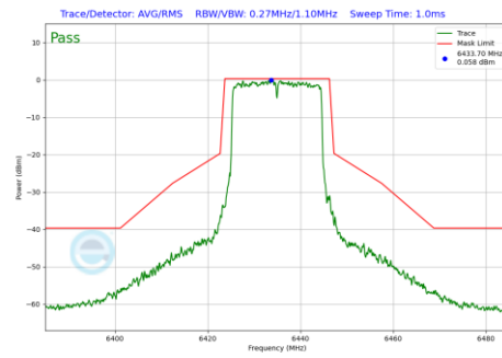
Plot 7-1200 In-Band Emission Plot CDD Diversity Antenna WF7 (20MHz BW 802.11be(RU) RU242 Index61 (UNII Band 6) - Ch.97)
