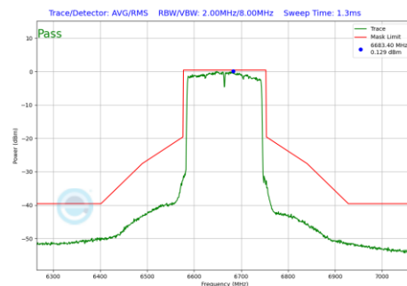
Plot 7-1219 In-Band Emission Plot CDD Diversity Antenna WF8 (160MHz BW 802.11be(RU) RU996X2 Index68 (UNII Band 7) - Ch.143)
