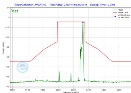
Plot 7-1223 In-Band Emission Plot CDD Diversity Antenna WF7 (160MHz BW 802.11be(RU) RU26 Index36 (UNII Band 5) - Ch.47)
