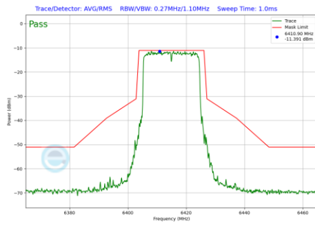
Plot 7-1274 In-Band Emission Plot CDD Diversity Antenna WF7 (20MHz BW 802.11be(RU) RU242 Index61 (UNII Band 5) - Ch.93)
