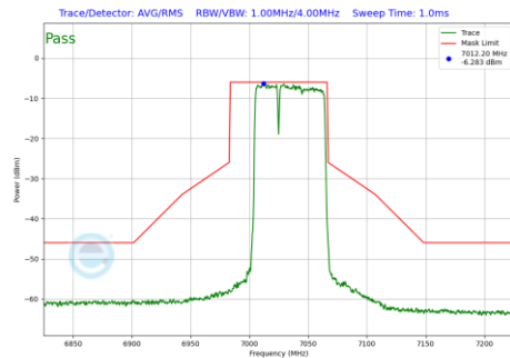
Plot 7-1261 In-Band Emission Plot CDD Diversity Antenna WF7 (80MHz BW 802.11be(RU) RU484+242 Index90 (UNII Band 8) - Ch.215)
