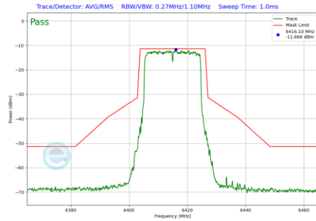
Plot 7-1138 In-Band Emission Plot CDD Primary Antenna WF8 (20MHz BW 802.11be(RU) RU242 Index61 (UNII Band 5) - Ch.93)
