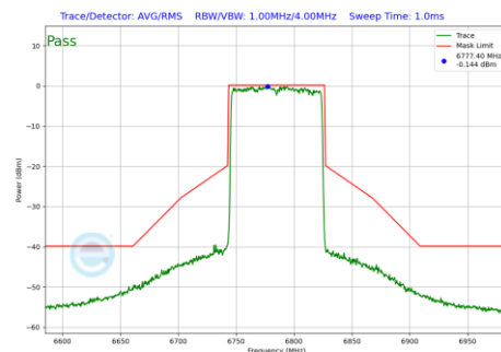
Plot 7-1218 In-Band Emission Plot CDD Diversity Antenna WF8 (80MHz BW 802.11be(RU) RU996 Index67 (UNII Band 7) - Ch.167)
