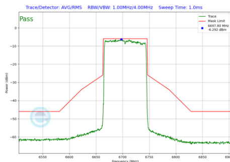
Plot 7-1148 In-Band Emission Plot CDD Primary Antenna WF8 (80MHz BW 802.11be(RU) RU996 Index67 (UNII Band 7) - Ch.151)
