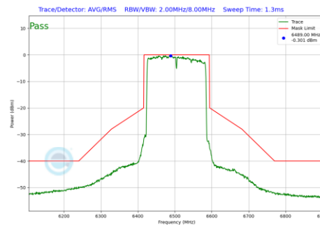
Plot 7-1203 In-Band Emission Plot CDD Diversity Antenna WF7 (160MHz BW 802.11be(RU) RU996X2 Index68 (UNII Band 6) - Ch.111)
