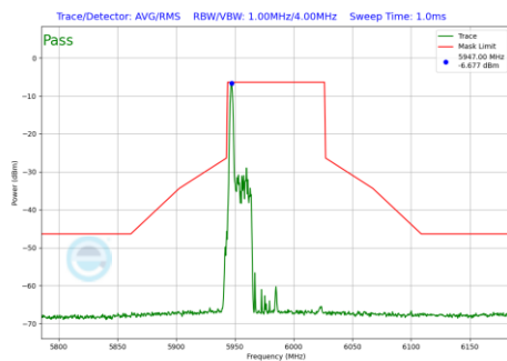
Plot 7-1238 In-Band Emission Plot CDD Diversity Antenna WF8 (80MHz BW 802.11be(RU) RU26 Index0 (UNII Band 5) - Ch.7)
