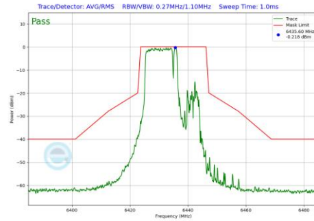
Plot 7-1190 In-Band Emission Plot CDD Diversity Antenna WF8 (20MHz BW 802.11be(RU) RU106+26 Index82 (UNII Band 6) - Ch.97)
