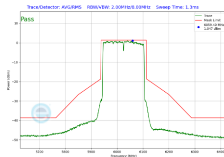
Plot 7-1211 In-Band Emission Plot CDD Diversity Antenna WF8 (160MHz BW 802.11be(RU) RU996X2 Index68 (UNII Band 5) - Ch.15)
