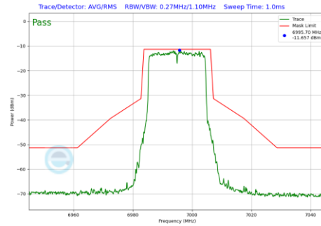
Plot 7-1286 In-Band Emission Plot CDD Diversity Antenna WF7 (20MHz BW 802.11be(RU) RU242 Index61 (UNII Band 8) - Ch.209)
