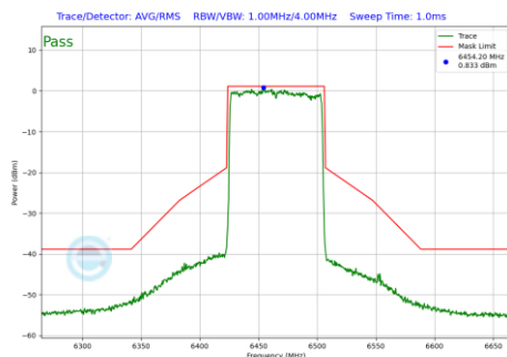
Plot 7-1214 In-Band Emission Plot CDD Diversity Antenna WF8 (80MHz BW 802.11be(RU) RU996 Index67 (UNII Band 6) - Ch.103)
