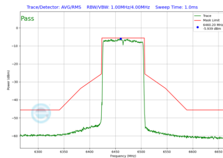
Plot 7-1296 In-Band Emission Plot CDD Diversity Antenna WF8 (80MHz BW 802.11be(RU) RU996 Index67 (UNII Band 6) - Ch.103)
