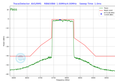
Plot 7-1206 In-Band Emission Plot CDD Diversity Antenna WF7 (80MHz BW 802.11be(RU) RU996 Index67 (UNII Band 7) - Ch.167)
