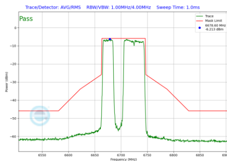
Plot 7-1270 In-Band Emission Plot SDM Diversity Antenna WF8 (80MHz BW 802.11be(RU) RU484+242 Index91 (UNII Band 7) - Ch.151)
