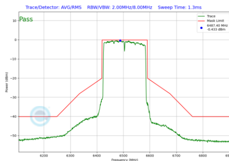
Plot 7-1215 In-Band Emission Plot CDD Diversity Antenna WF8 (160MHz BW 802.11be(RU) RU996X2 Index68 (UNII Band 6) - Ch.111)
