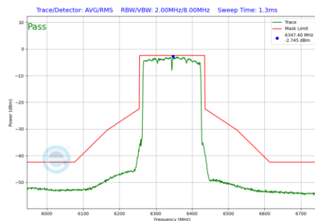
Plot 7-1293 In-Band Emission Plot CDD Diversity Antenna WF8 (160MHz BW 802.11be(RU) RU996X2 Index68 (UNII Band 5) - Ch.79)
