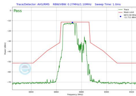
Plot 7-1258 In-Band Emission Plot CDD Diversity Antenna WF7 (20MHz BW 802.11be(RU) RU106+26 Index82 (UNII Band 7) - Ch.185)
