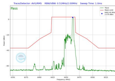
Plot 7-1159 In-Band Emission Plot CDD Diversity Antenna WF7 (40MHz BW 802.11be(RU) RU26 Index17 (UNII Band 6) - Ch.99)
