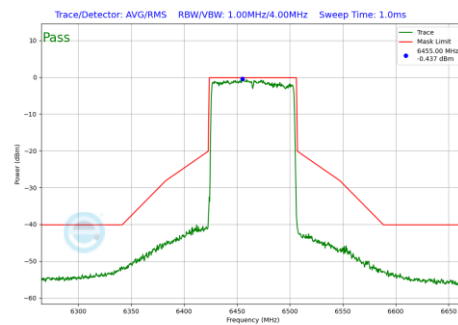
Plot 7-1202 In-Band Emission Plot CDD Diversity Antenna WF7 (80MHz BW 802.11be(RU) RU996 Index67 (UNII Band 6) - Ch.103)
