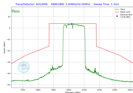
Plot 7-1189 In-Band Emission Plot CDD Diversity Antenna WF8 (160MHz BW 802.11be(RU) RU996+484+242 Index96 (UNII Band 5) - Ch.15)
