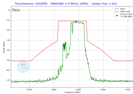
Plot 7-1252 In-Band Emission Plot CDD Diversity Antenna WF7 (20MHz BW 802.11be(RU) RU106+26 Index83 (UNII Band 5) - Ch.45)
