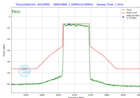
Plot 7-1284 In-Band Emission Plot CDD Diversity Antenna WF7 (80MHz BW 802.11be(RU) RU996 Index67 (UNII Band 7) - Ch.151)
