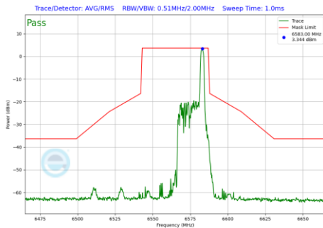
Plot 7-1163 In-Band Emission Plot CDD Diversity Antenna WF7 (40MHz BW 802.11be(RU) RU26 Index17 (UNII Band 7) - Ch.123)
