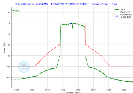
Plot 7-1207 In-Band Emission Plot CDD Diversity Antenna WF7 (160MHz BW 802.11be(RU) RU996X2 Index68 (UNII Band 7) - Ch.143)
