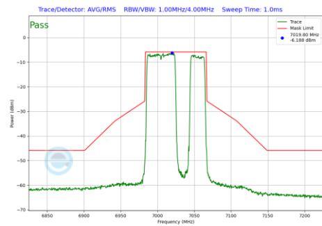
Plot 7-1272 In-Band Emission Plot SDM Diversity Antenna WF8 (80MHz BW 802.11be(RU) RU484+242 Index92 (UNII Band 8) - Ch.215)
