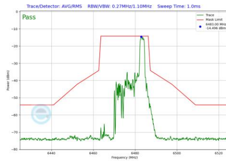
Plot 7-1224 In-Band Emission Plot CDD Diversity Antenna WF7 (20MHz BW 802.11be(RU) RU26 Index8 (UNII Band 6) - Ch.105)
