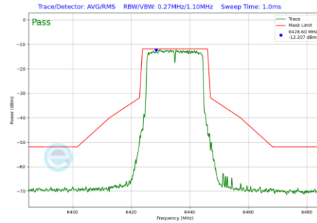
Plot 7-1142 In-Band Emission Plot CDD Primary Antenna WF8 (20MHz BW 802.11be(RU) RU242 Index61 (UNII Band 6) - Ch.97)
