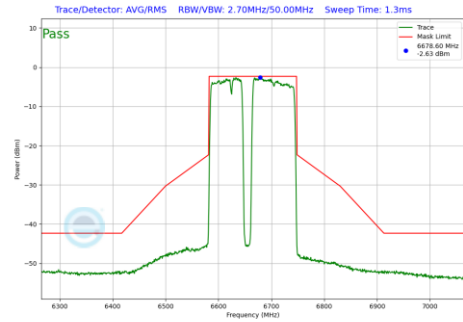
Plot 7-1271 In-Band Emission Plot SDM Diversity Antenna WF8 (160MHz BW 802.11be(RU) RU996+484+242 Index99 (UNII Band 7) - Ch.143)
