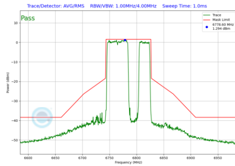
Plot 7-1194 In-Band Emission Plot CDD Diversity Antenna WF8 (80MHz BW 802.11be(RU) RU484+242 Index92 (UNII Band 7) - Ch.167)
