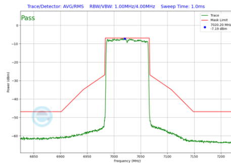
Plot 7-1136 In-Band Emission Plot CDD Primary Antenna WF5B (80MHz BW 802.11be(RU) RU996 Index67 (UNII Band 8) - Ch.215)
