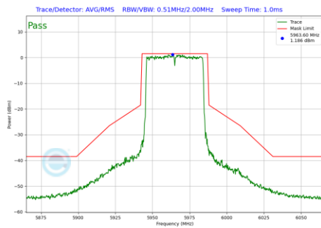
Plot 7-1197 In-Band Emission Plot CDD Diversity Antenna WF7 (40MHz BW 802.11be(RU) RU484 Index65 (UNII Band 5) - Ch.3)
