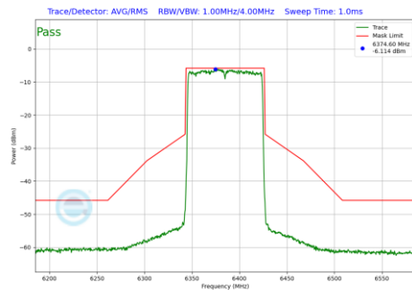
Plot 7-1140 In-Band Emission Plot CDD Primary Antenna WF8 (80MHz BW 802.11be(RU) RU996 Index67 (UNII Band 5) - Ch.87)
