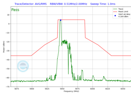
Plot 7-1155 In-Band Emission Plot CDD Diversity Antenna WF7 (40MHz BW 802.11be(RU) RU26 Index0 (UNII Band 5) - Ch.3)
