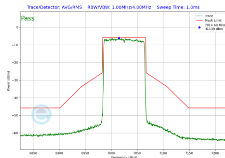
Plot 7-1152 In-Band Emission Plot CDD Primary Antenna WF8 (80MHz BW 802.11be(RU) RU996 Index67 (UNII Band 8) - Ch.215)
