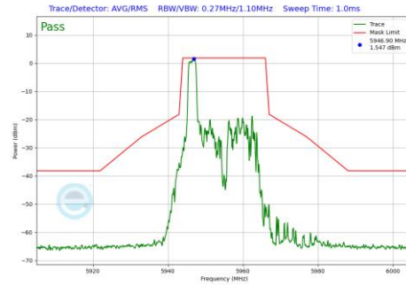
Plot 7-1166 In-Band Emission Plot CDD Diversity Antenna WF8 (20MHz BW 802.11be(RU) RU26 Index0 (UNII Band 5) - Ch.1)
