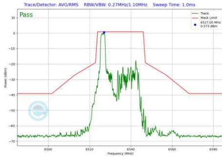
Plot 7-1162 In-Band Emission Plot CDD Diversity Antenna WF7 (20MHz BW 802.11be(RU) RU26 Index0 (UNII Band 7) - Ch.117)
