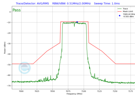
Plot 7-1135 In-Band Emission Plot CDD Primary Antenna WF5B (40MHz BW 802.11be(RU) RU484 Index65 (UNII Band 8) - Ch.227)
