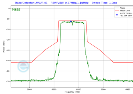
Plot 7-1282 In-Band Emission Plot CDD Diversity Antenna WF7 (20MHz BW 802.11be(RU) RU242 Index61 (UNII Band 7) - Ch.185)
