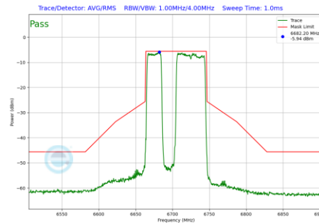
Plot 7-1259 In-Band Emission Plot CDD Diversity Antenna WF7 (80MHz BW 802.11be(RU) RU484+242 Index91 (UNII Band 7) - Ch.151)
