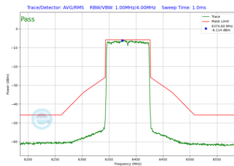
Plot 7-1292 In-Band Emission Plot CDD Diversity Antenna WF8 (80MHz BW 802.11be(RU) RU996 Index67 (UNII Band 5) - Ch.87)
