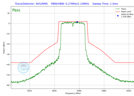
Plot 7-1196 In-Band Emission Plot CDD Diversity Antenna WF7 (20MHz BW 802.11be(RU) RU242 Index61 (UNII Band 5) - Ch.1)
