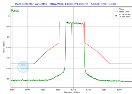
Plot 7-1253 In-Band Emission Plot CDD Diversity Antenna WF7 (80MHz BW 802.11be(RU) RU484+242 Index90 (UNII Band 5) - Ch.39)
