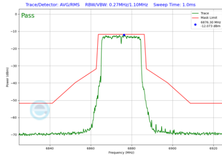
Plot 7-1298 In-Band Emission Plot CDD Diversity Antenna WF8 (20MHz BW 802.11be(RU) RU242 Index61 (UNII Band 7) - Ch.185)
