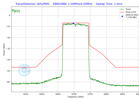
Plot 7-1132 In-Band Emission Plot CDD Primary Antenna WF5B (80MHz BW 802.11be(RU) RU996 Index67 (UNII Band 7) - Ch.151)
