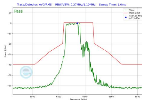
Plot 7-1193 In-Band Emission Plot CDD Diversity Antenna WF8 (20MHz BW 802.11be(RU) RU106+26 Index82 (UNII Band 7) - Ch.117)
