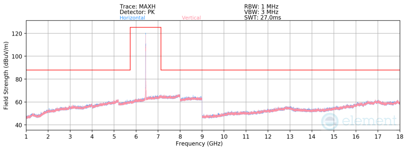
Plot 7-1345. Radiated Spurious Emissions above 1GHz CDD Primary (802.11be – Ch. 97 – RU26)
