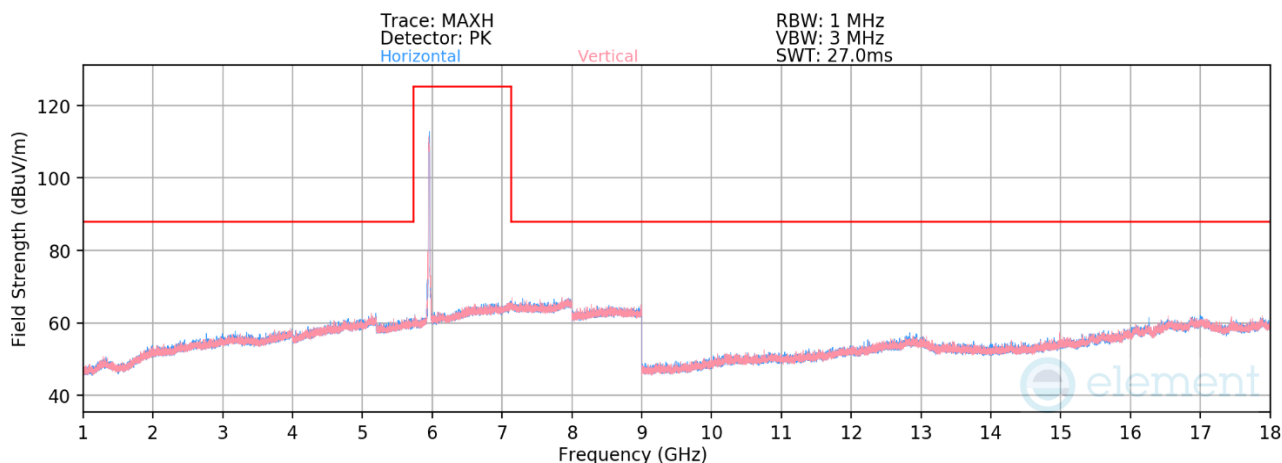
Plot 7-1357. Radiated Spurious Emissions above 1GHz CDD Primary (802.11be – Ch. 1 – RU242)
