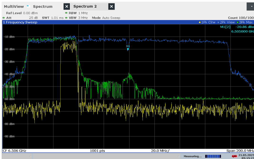
Plot 7-1339. 160MHz Bandwidth, AWGN Signal Injected – 6505Mhz
