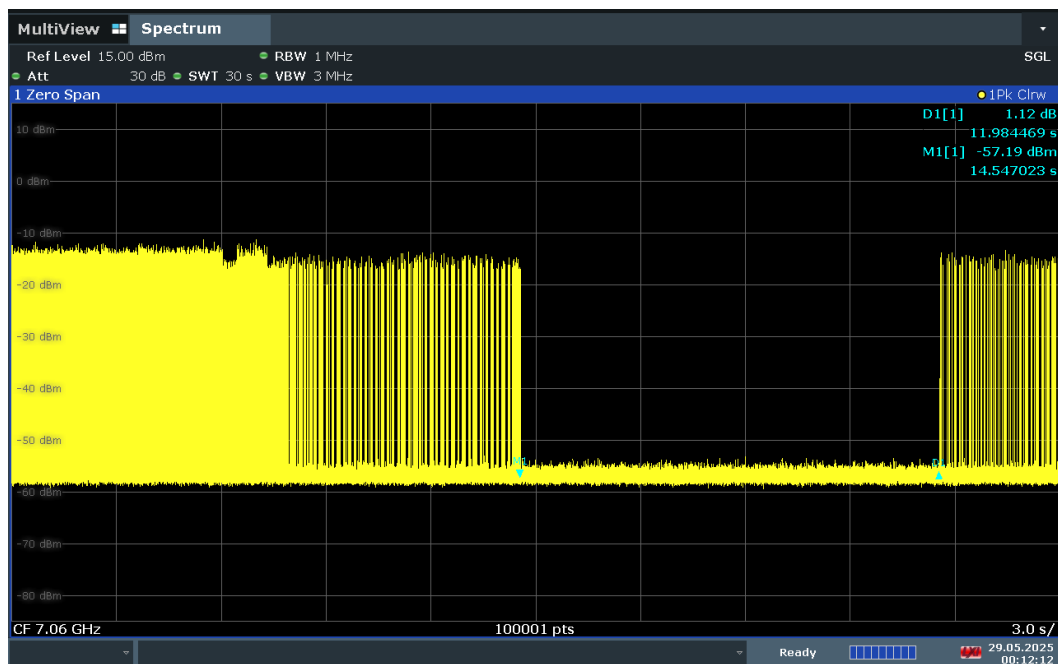
Plot 7-1337. Contention Based Protocol Timing Plot – UNII 8 – 160MHz Channel 207 – High
