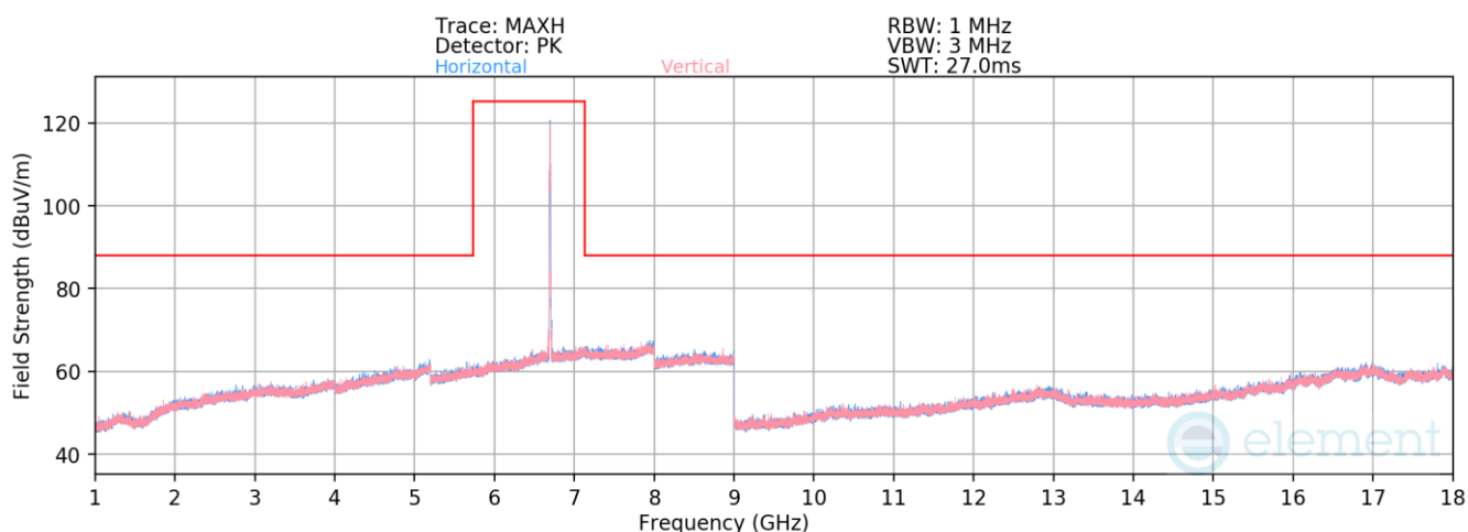
Plot 7-1350. Radiated Spurious Emissions above 1GHz CDD Primary (802.11be – Ch. 149 – RU26)
