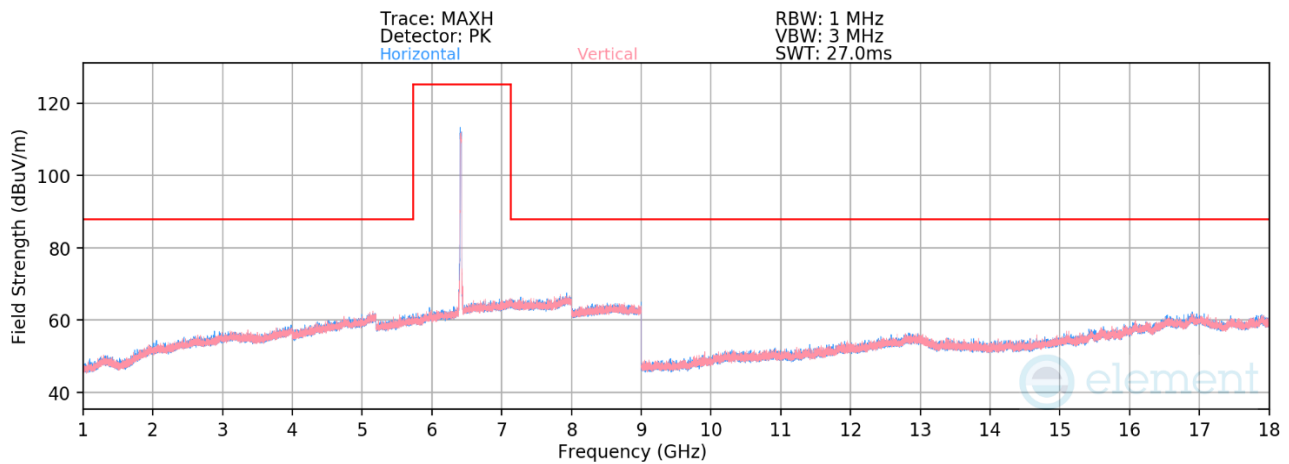
Plot 7-1360. Radiated Spurious Emissions above 1GHz CDD Primary (802.11be – Ch. 93 – RU242)
