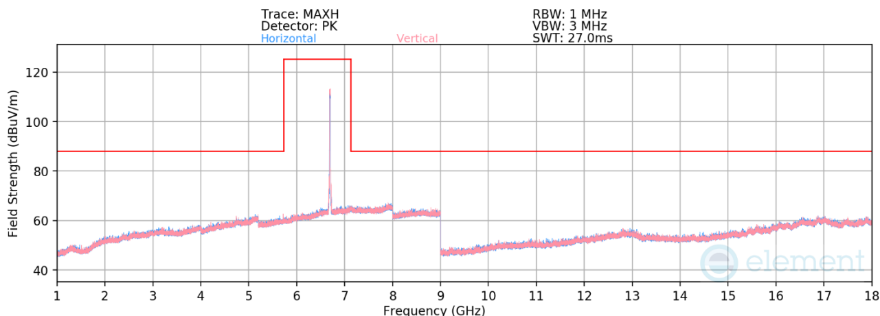
Plot 7-1366. Radiated Spurious Emissions above 1GHz CDD Primary (802.11be – Ch. 149 – RU242)
