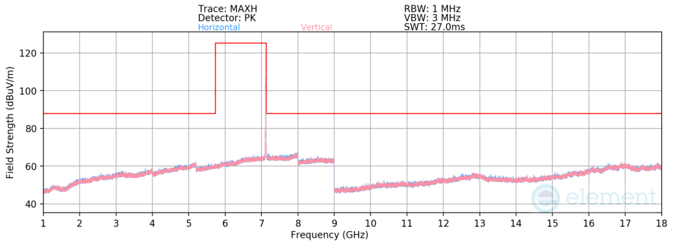
Plot 7-1356. Radiated Spurious Emissions above 1GHz CDD Primary (802.11be – Ch. 229 – RU26)
