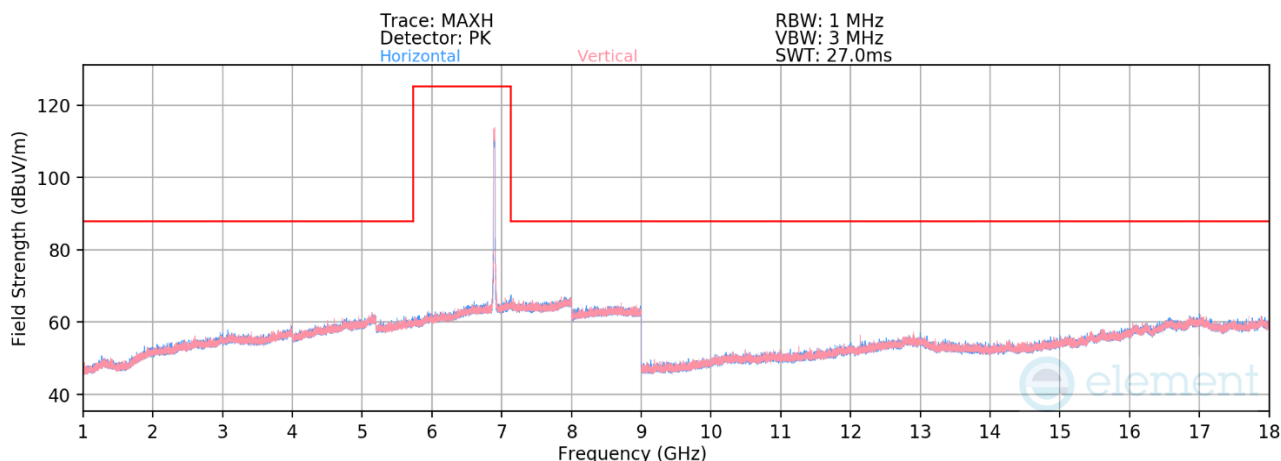
Plot 7-1369. Radiated Spurious Emissions above 1GHz SDM Primary (802.11be – Ch. 189 – RU242)
