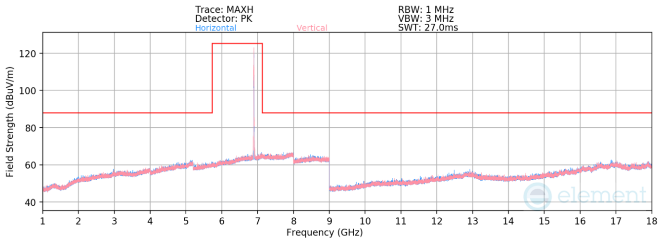
Plot 7-1353. Radiated Spurious Emissions above 1GHz CDD Primary (802.11be – Ch. 189 – RU26)
