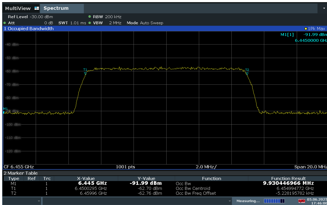
Plot 7-1310. AWGN Signal – UNII 6 – 20MHz
