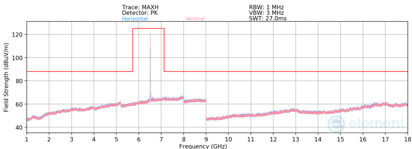
Plot 7-1348. Radiated Spurious Emissions above 1GHz CDD Primary (802.11be – Ch. 113 – RU26)
