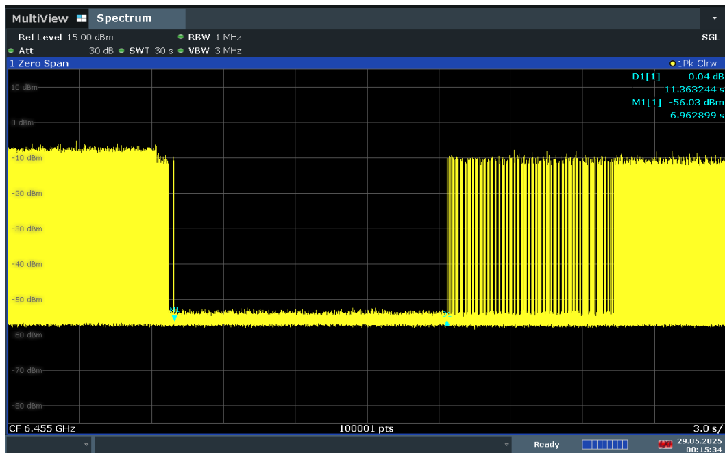
Plot 7-1326. Contention Based Protocol Timing Plot – UNII 6 – 20MHz Channel 101
