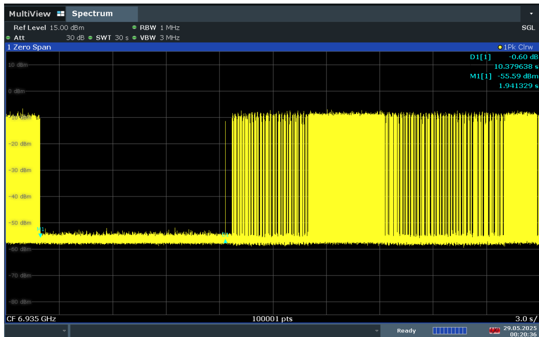
Plot 7-1334. Contention Based Protocol Timing Plot – UNII 8 – 20MHz Channel 197
