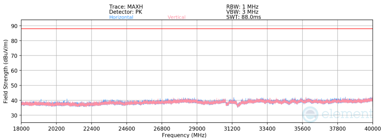
Plot 7-1363. Radiated Spurious Emissions 18-40GHz CDD Primary (802.11be – Ch. 105 – RU242)
