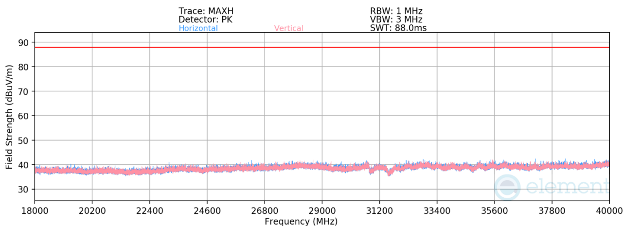
Plot 7-1367. Radiated Spurious Emissions 18-40GHz CDD Primary (802.11be – Ch. 149 – RU242)
