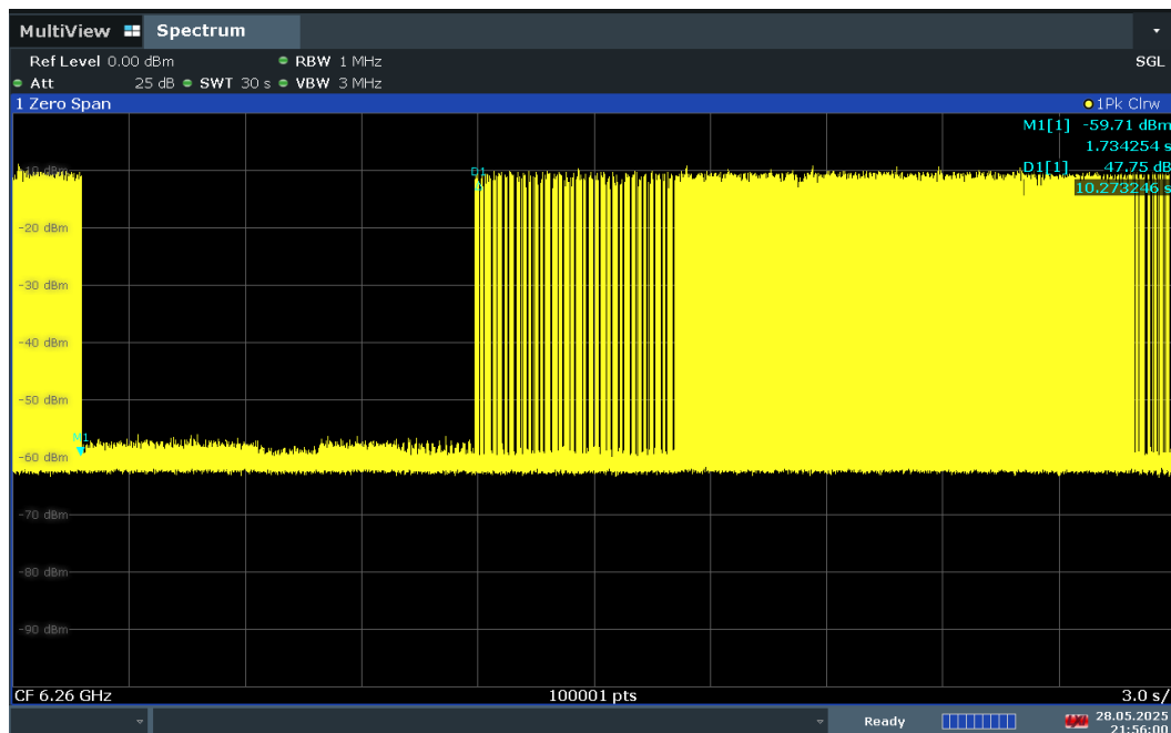
Plot 7-1323. Contention Based Protocol Timing Plot – UNII 5 – 160MHz Channel 47 – Low
