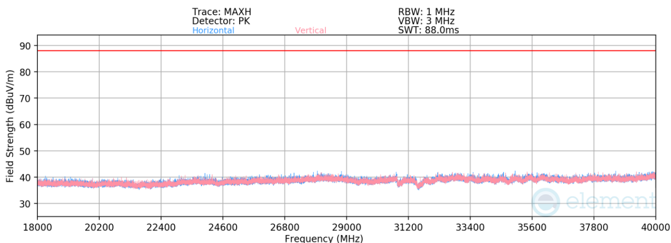
Plot 7-1375. Radiated Spurious Emissions 18-40GHz CDD Diversity (802.11be – Ch. 45 – RU26)
