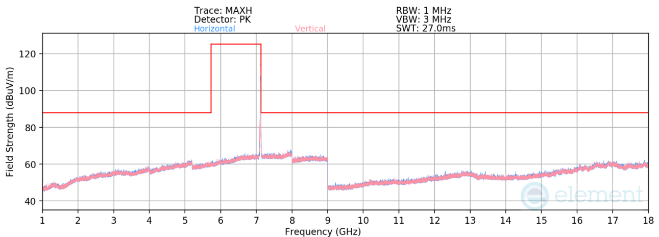
Plot 7-1372. Radiated Spurious Emissions above 1GHz SDM Primary (802.11be – Ch. 233 – RU242)
