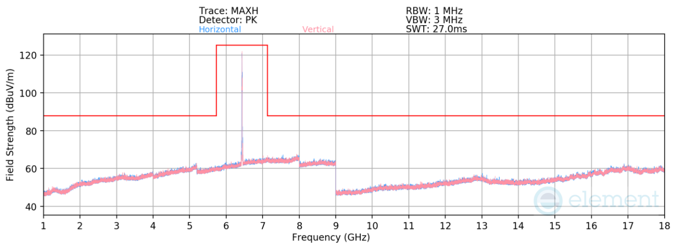
Plot 7-1377. Radiated Spurious Emissions above 1GHz CDD Diversity (802.11be – Ch. 97 – RU26)
