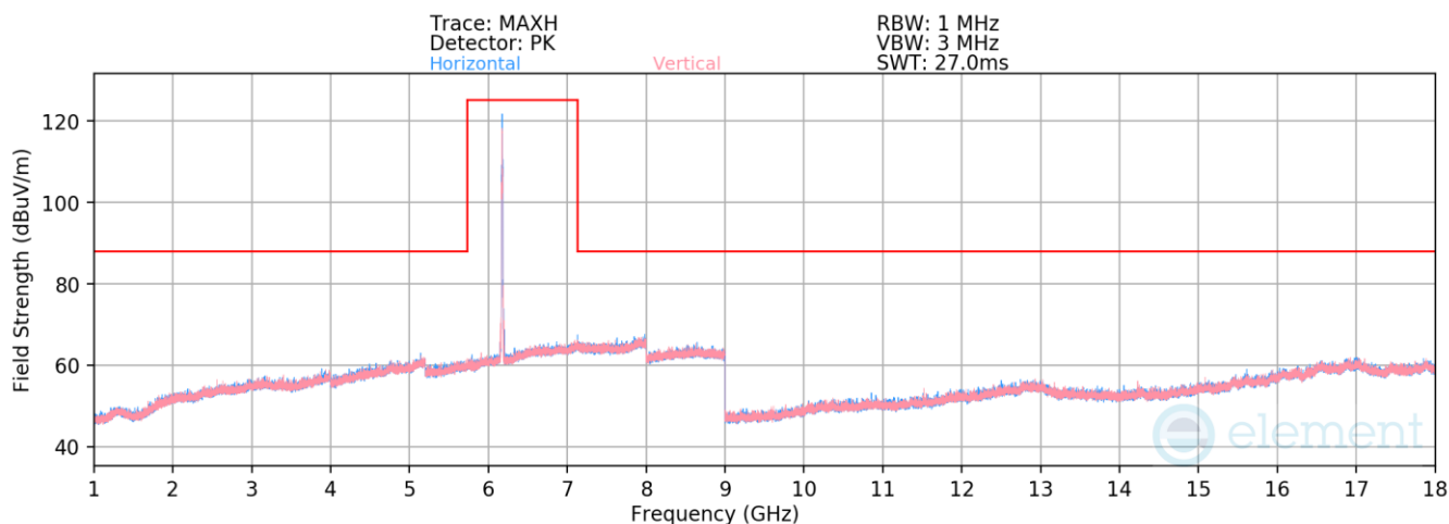
Plot 7-1342. Radiated Spurious Emissions above 1GHz CDD Primary (802.11be – Ch. 45 – RU26)
