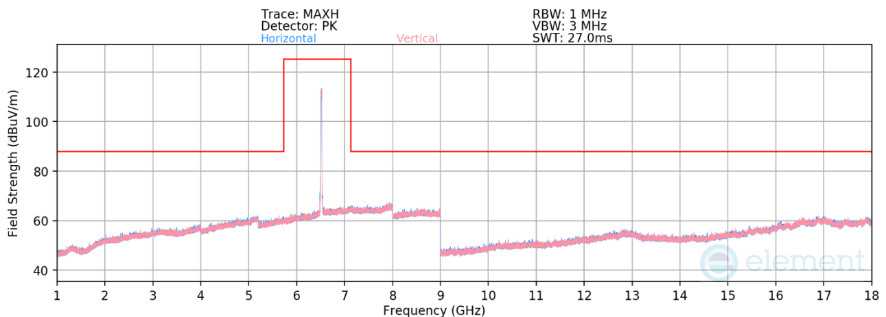
Plot 7-1364. Radiated Spurious Emissions above 1GHz CDD Primary (802.11be – Ch. 113 – RU242)
