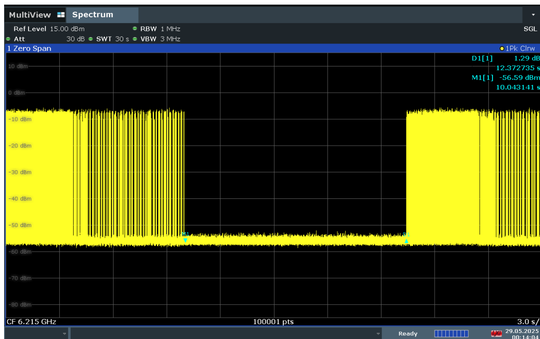
Plot 7-1322. Contention Based Protocol Timing Plot – UNII 5 – 20MHz Channel 53
