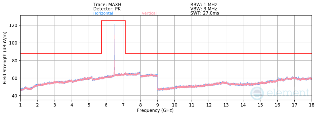
Plot 7-1346. Radiated Spurious Emissions above 1GHz CDD Primary (802.11be – Ch. 105 – RU26)
