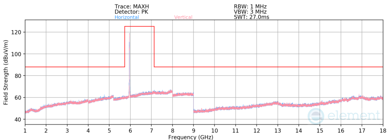
Plot 7-1341. Radiated Spurious Emissions above 1GHz CDD Primary (802.11be – Ch. 1 – RU26)
