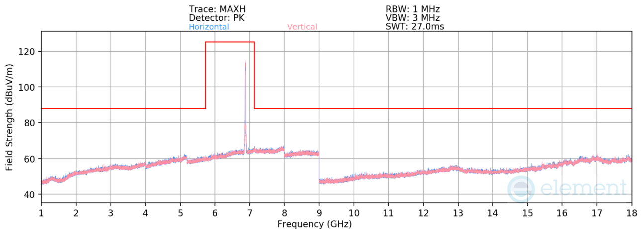
Plot 7-1368. Radiated Spurious Emissions above 1GHz SDM Primary (802.11be – Ch. 185 – RU242)
