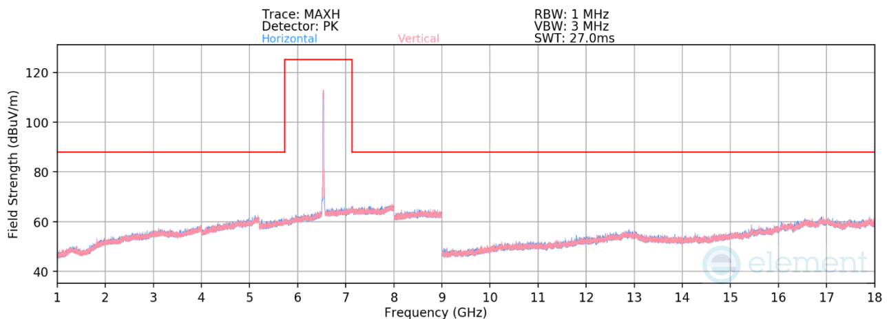
Plot 7-1365. Radiated Spurious Emissions above 1GHz CDD Primary (802.11be – Ch. 117 – RU242)
