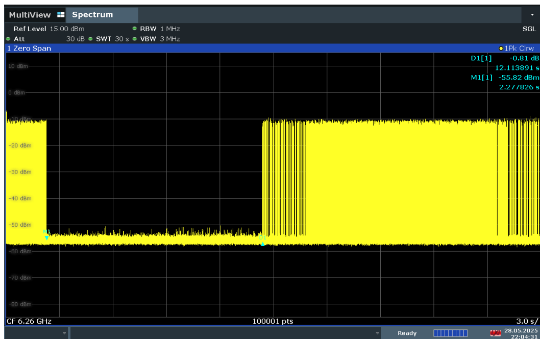
Plot 7-1325. Contention Based Protocol Timing Plot – UNII 5 – 160MHz Channel 47 – High
