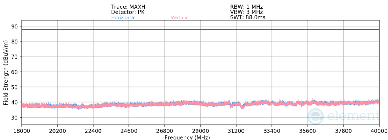
Plot 7-1343. Radiated Spurious Emissions 18-40GHz CDD Primary (802.11be – Ch. 45 – RU26)
