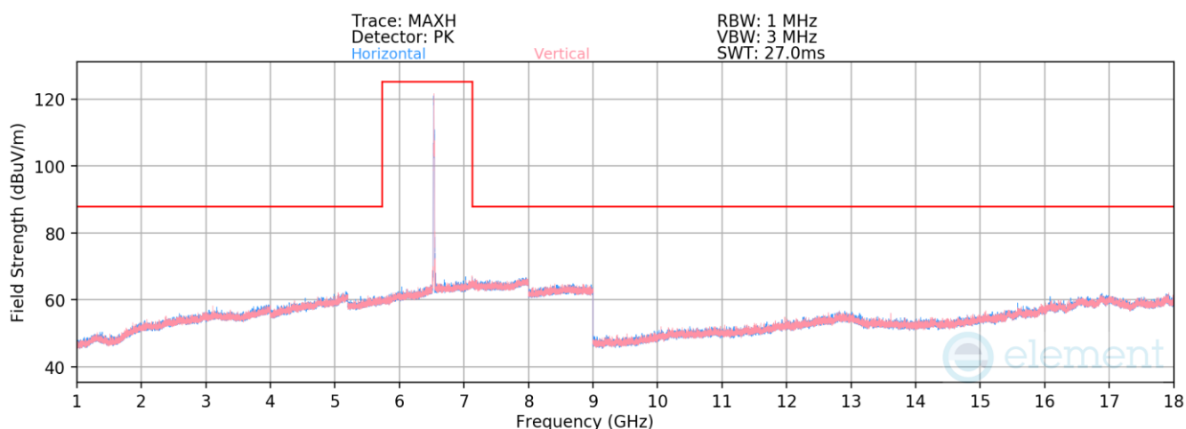
Plot 7-1349. Radiated Spurious Emissions above 1GHz CDD Primary (802.11be – Ch. 117 – RU26)
