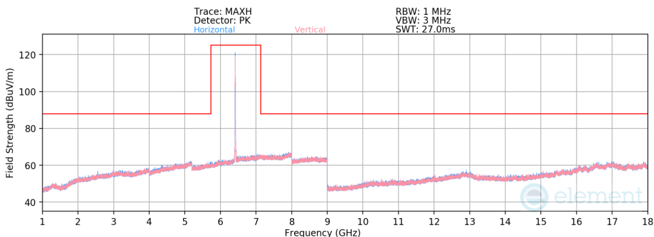
Plot 7-1344. Radiated Spurious Emissions above 1GHz CDD Primary (802.11be – Ch. 93 – RU26)
