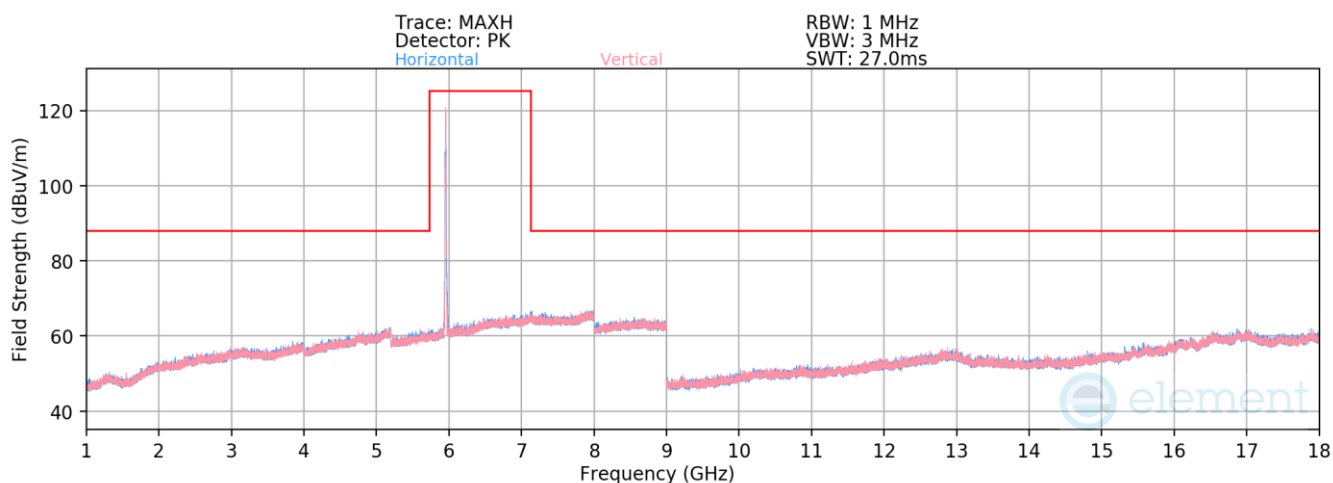
Plot 7-1373. Radiated Spurious Emissions above 1GHz CDD Diversity (802.11be – Ch. 1 – RU26)
