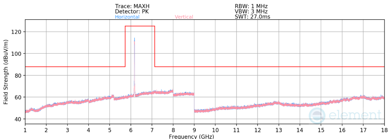
Plot 7-1358. Radiated Spurious Emissions above 1GHz CDD Primary (802.11be – Ch. 45 – RU242)
