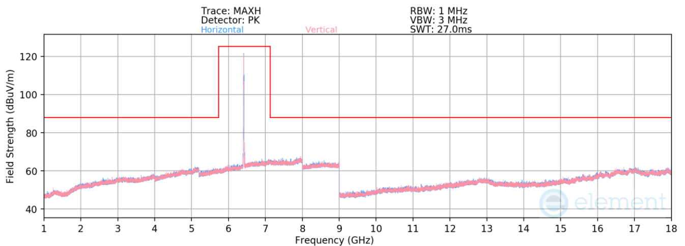
Plot 7-1376. Radiated Spurious Emissions above 1GHz CDD Diversity (802.11be – Ch. 93 – RU26)
