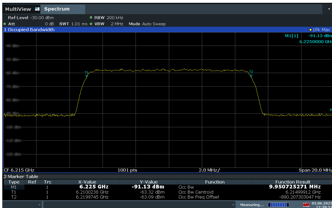
Plot 7-1306. AWGN Signal – UNII 5 – 20MHz
