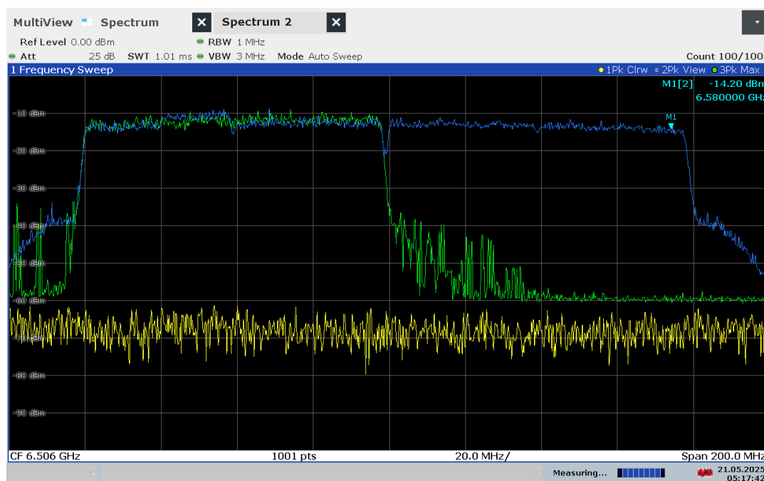
Plot 7-1340. 160MHz Bandwidth, AWGN Signal Injected – 6580MHz
