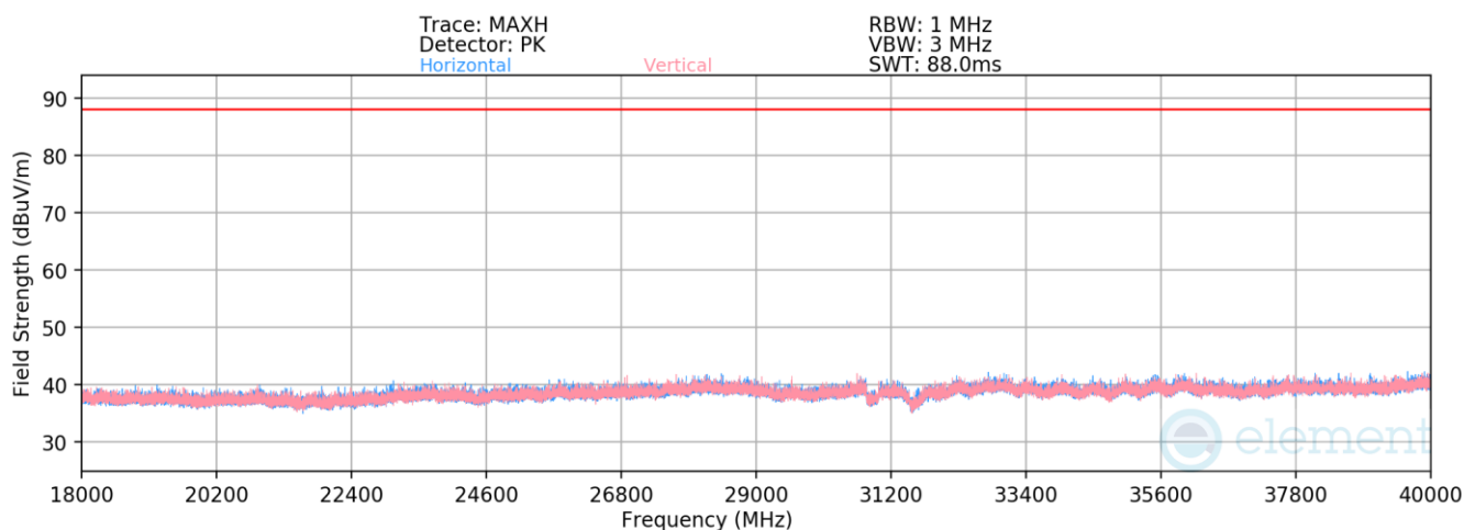
Plot 7-1355. Radiated Spurious Emissions 18-40GHz CDD Primary (802.11be – Ch. 209 – RU26)
