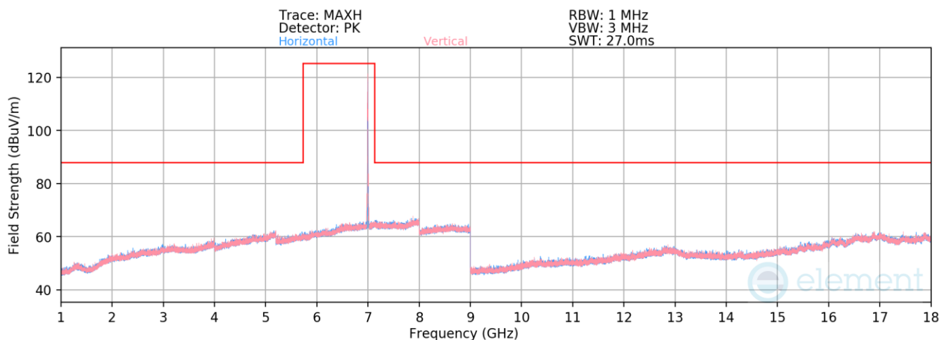
Plot 7-1354. Radiated Spurious Emissions above 1GHz CDD Primary (802.11be – Ch. 209 – RU26)
