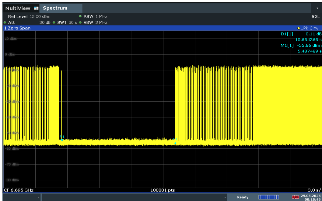
Plot 7-1330. Contention Based Protocol Timing Plot – UNII 7 – 20MHz Channel 149
