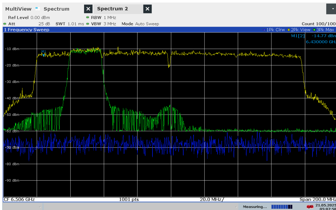
Plot 7-1338. 160MHz Bandwidth, AWGN Signal Injected – 6430Mhz
