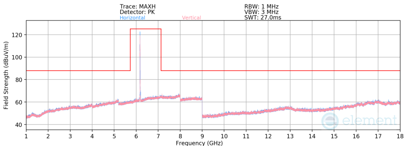
Plot 7-1374. Radiated Spurious Emissions above 1GHz CDD Diversity (802.11be – Ch. 45 – RU26)
