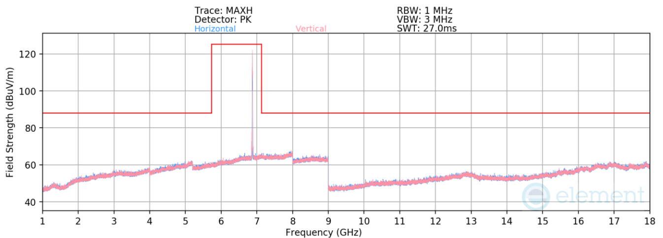
Plot 7-1352. Radiated Spurious Emissions above 1GHz CDD Primary (802.11be – Ch. 185 – RU26)
