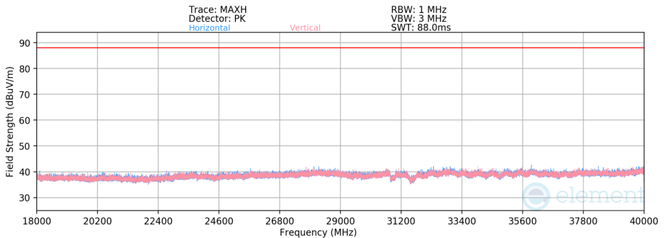
Plot 7-1347. Radiated Spurious Emissions 18-40GHz CDD Primary (802.11be – Ch. 105 – RU26)
