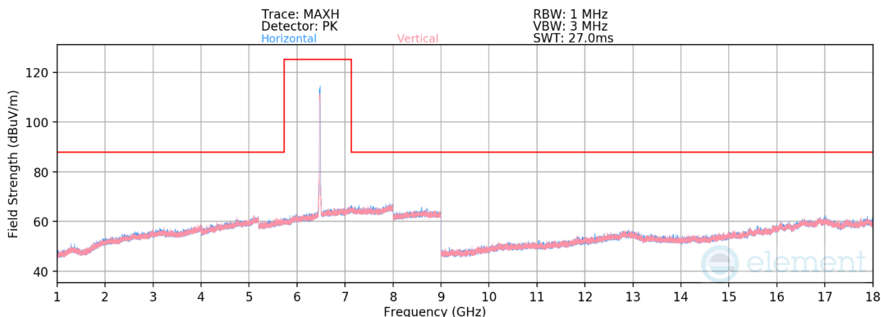
Plot 7-1362. Radiated Spurious Emissions above 1GHz CDD Primary (802.11be – Ch. 105 – RU242)
