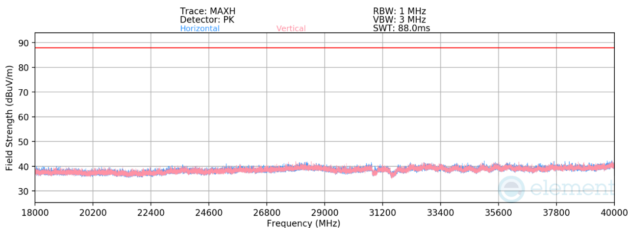
Plot 7-1359. Radiated Spurious Emissions 18-40GHz CDD Primary (802.11be – Ch. 45 – RU242)
