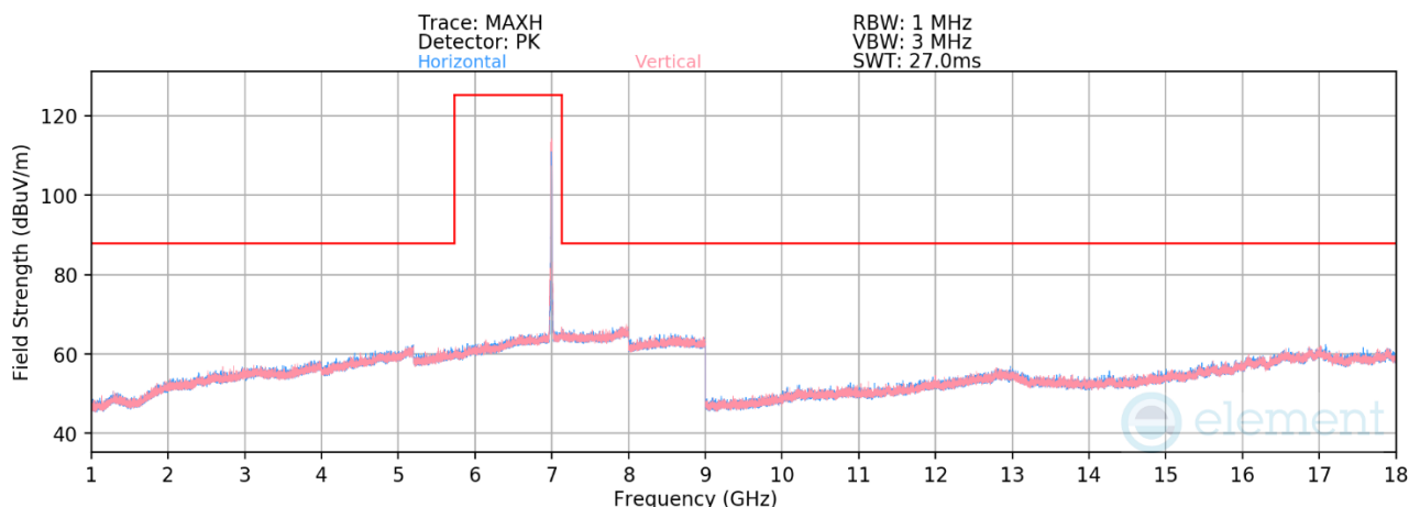
Plot 7-1370. Radiated Spurious Emissions above 1GHz SDM Primary (802.11be – Ch. 209 – RU242)
