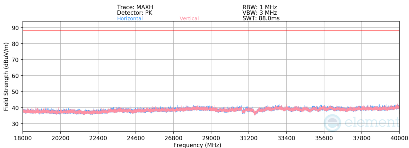
Plot 7-1351. Radiated Spurious Emissions 18-40GHz CDD Primary (802.11be – Ch. 149 – RU26)
