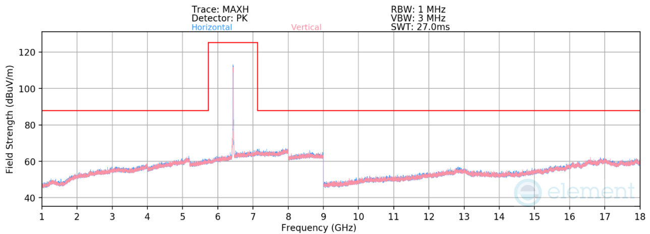
Plot 7-1361. Radiated Spurious Emissions above 1GHz CDD Primary (802.11be – Ch. 97 – RU242)
