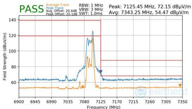
Plot 7-1708 SDM Primary Radiated Upper Band Edge (Peak & Average – UNII Band 8) - RU26
