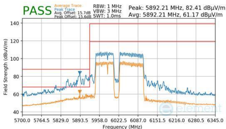
Plot 7-1765 CDD Primary Radiated Lower Band Edge (Peak & Average – UNII Band 5) - RU996+484+242 (L)
