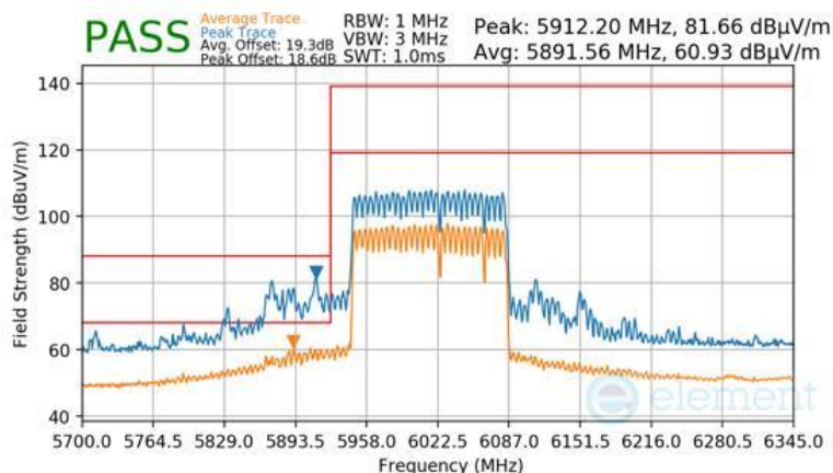
Plot 7-1763 CDD Primary Radiated Lower Band Edge (Peak & Average – UNII Band 5) - RU996+484+242
