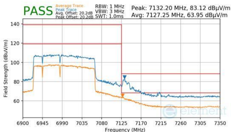
Plot 7-1673 Antenna WF7 Radiated Upper Band Edge (Peak & Average – UNII Band 8) - RU996+484+242 (L)
