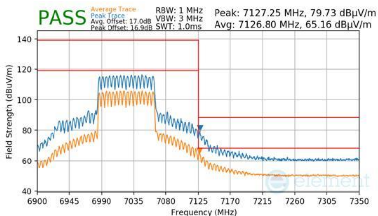
Plot 7-1733 SDM Primary Radiated Upper Band Edge (Peak & Average – UNII Band 8) - RU996
