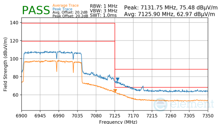
Plot 7-1683 Antenna WF7 Radiated Upper Band Edge (Peak & Average – UNII Band 8) - RU996+484+242
