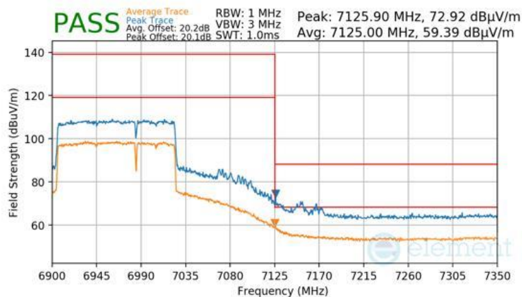
Plot 7-1657 Antenna WF7 Radiated Upper Band Edge (Peak & Average – UNII Band 8) - RU996+484 (H)
