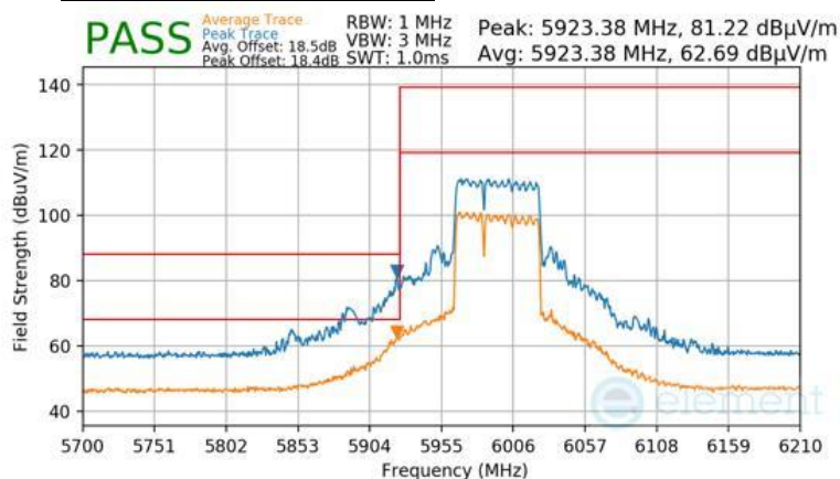
Plot 7-1719 CDD Primary Radiated Lower Band Edge (Peak & Average – UNII Band 5) - RU484+242
