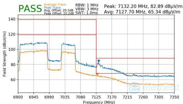
Plot 7-1655 Antenna WF7 Radiated Upper Band Edge (Peak & Average – UNII Band 8) - RU996+484 (H)
