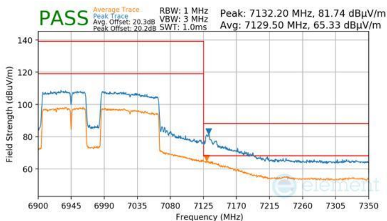
Plot 7-1682 Antenna WF7 Radiated Upper Band Edge (Peak & Average – UNII Band 8) - RU996+484+242 (L)
