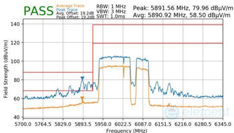
Plot 7-1665 Antenna WF7 Radiated Lower Band Edge (Peak & Average – UNII Band 5) - RU996+484+242
