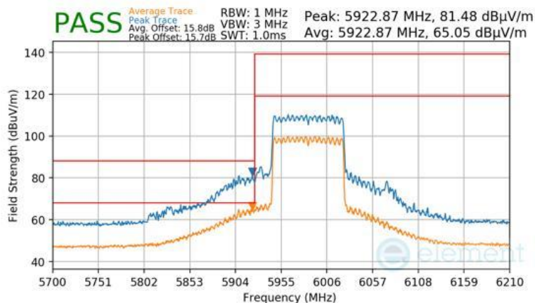
Plot 7-1731 CDD Primary Radiated Lower Band Edge (Peak & Average – UNII Band 5) - RU996
