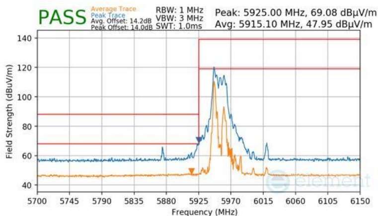
Plot 7-1797 CDD Diversity Radiated Lower Band Edge (Peak & Average – UNII Band 5) - RU26
