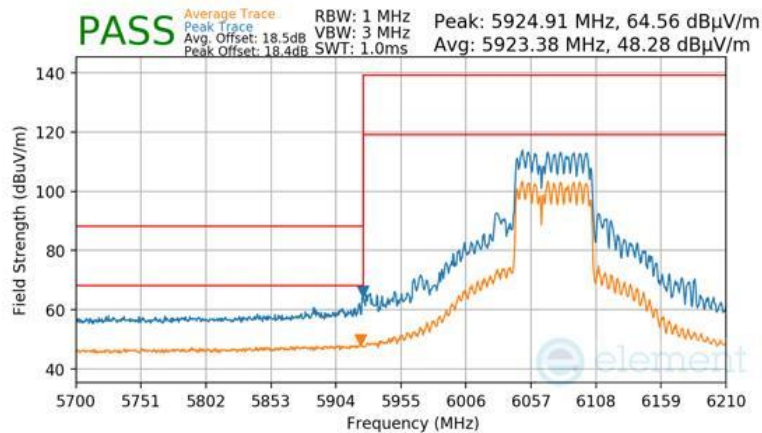
Plot 7-1723 CDD Primary Radiated Lower Band Edge (Peak & Average – UNII Band 5) - RU484+242
