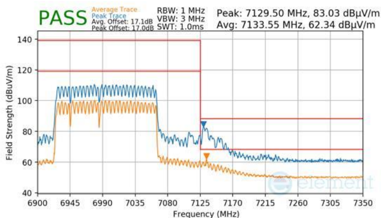
Plot 7-1768 SDM Primary Radiated Upper Band Edge (Peak & Average – UNII Band 8) - RU996+484+242 (L)
