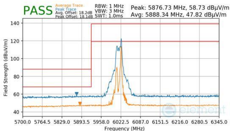
Plot 7-1735 CDD Primary Radiated Lower Band Edge (Peak & Average – UNII Band 5) - RU26
