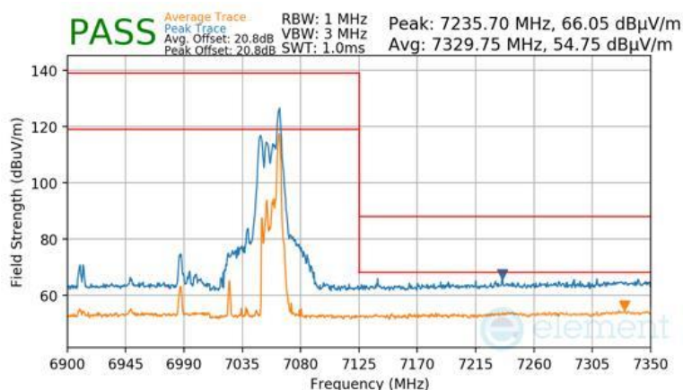
Plot 7-1718 SDM Primary Radiated Upper Band Edge (Peak & Average – UNII Band 8) - RU26
