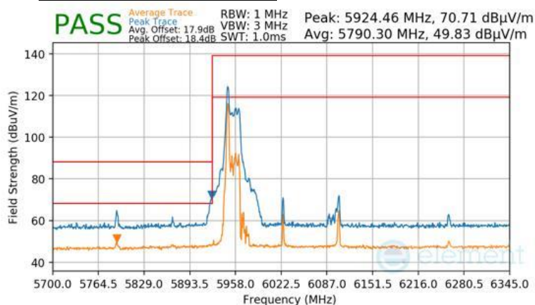
Plot 7-1734 CDD Primary Radiated Lower Band Edge (Peak & Average – UNII Band 5) - RU26
