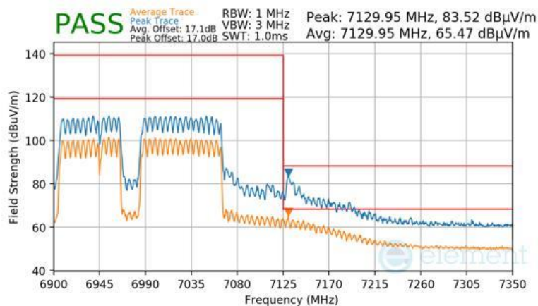
Plot 7-1777 SDM Primary Radiated Upper Band Edge (Peak & Average – UNII Band 8) - RU996+484+242 (L)
