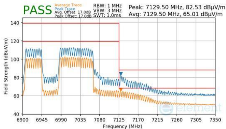
Plot 7-1753 SDM Primary Radiated Upper Band Edge (Peak & Average – UNII Band 8) - RU996+484 (L)
