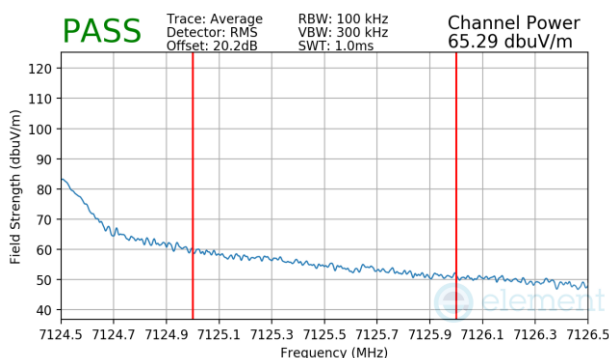
Plot 7-1796 SDM Diversity WF5B Radiated Upper Band Edge (Average – UNII Band 8)
