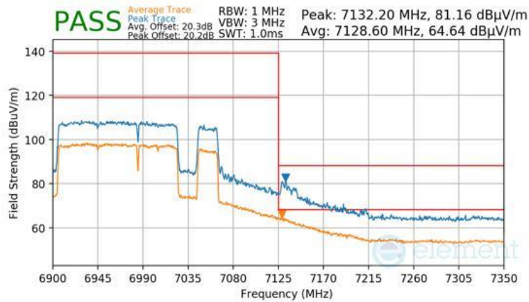
Plot 7-1678 Antenna WF7 Radiated Upper Band Edge (Peak & Average – UNII Band 8) - RU996+484+242 (H)
