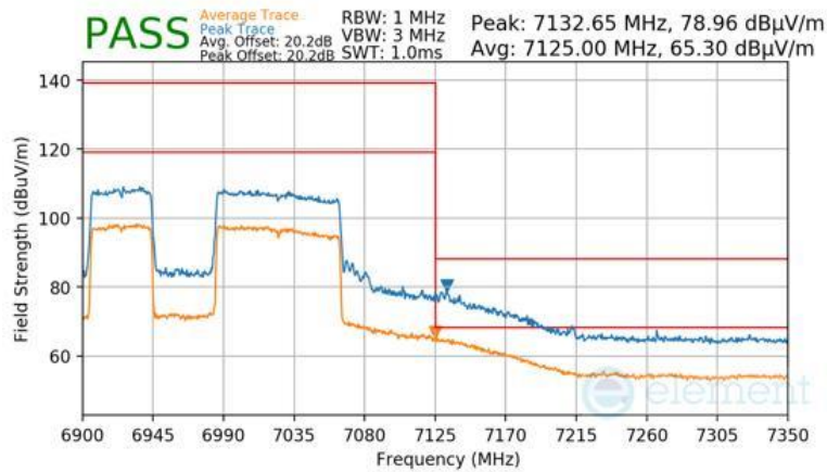
Plot 7-1658 Antenna WF7 Radiated Upper Band Edge (Peak & Average – UNII Band 8) - RU996+484 (L)
