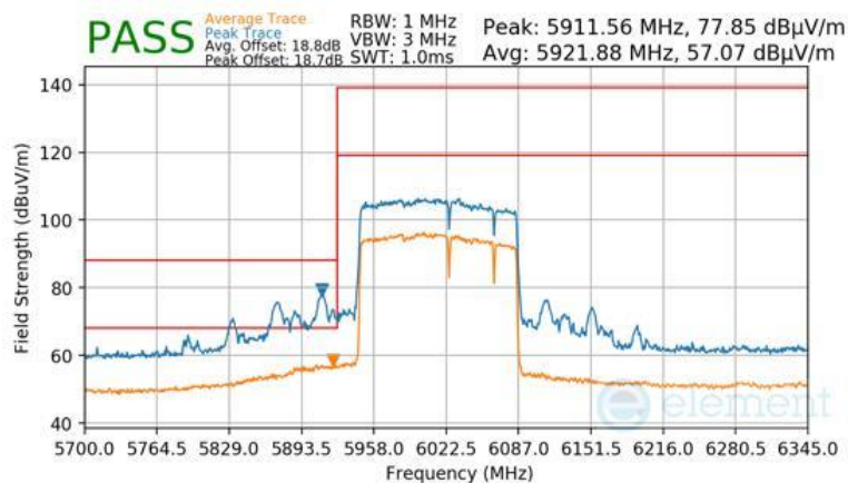
Plot 7-1671 Antenna WF7 Radiated Lower Band Edge (Peak & Average – UNII Band 5) - RU996+484+242
