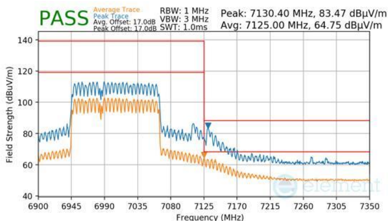
Plot 7-1749 SDM Primary Radiated Upper Band Edge (Peak & Average – UNII Band 8) - RU996+484 (L)
