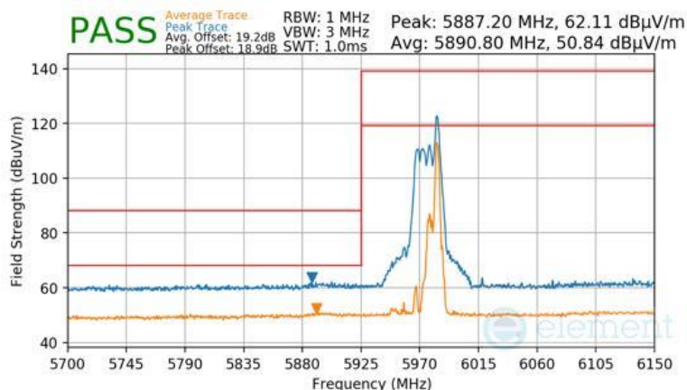
Plot 7-1689 CDD Primary Radiated Lower Band Edge (Peak & Average – UNII Band 5) - RU26
