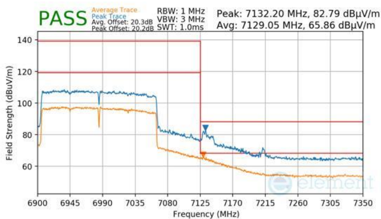
Plot 7-1685 Antenna WF7 Radiated Upper Band Edge (Peak & Average – UNII Band 8) - RU996X2
