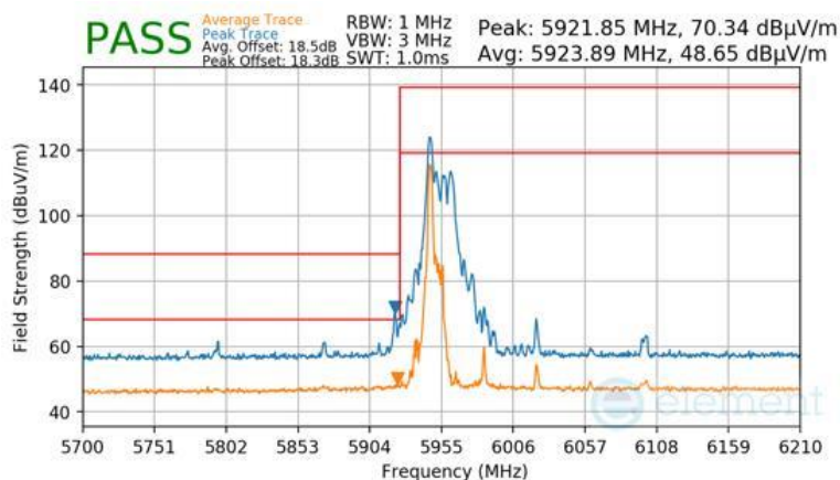
Plot 7-1713 CDD Primary Radiated Lower Band Edge (Peak & Average – UNII Band 5) - RU26
