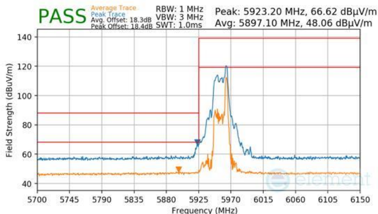
Plot 7-1687 CDD Primary Radiated Lower Band Edge (Peak & Average – UNII Band 5) - RU26
