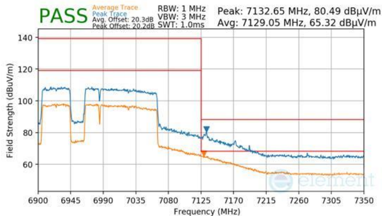
Plot 7-1679 Antenna WF7 Radiated Upper Band Edge (Peak & Average – UNII Band 8) - RU996+484+242 (L)
