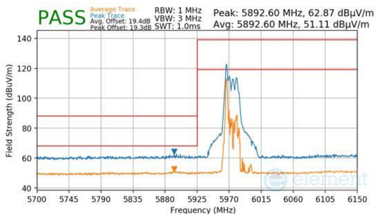
Plot 7-1782 CDD Diversity Radiated Lower Band Edge (Peak & Average – UNII Band 5) - RU26
