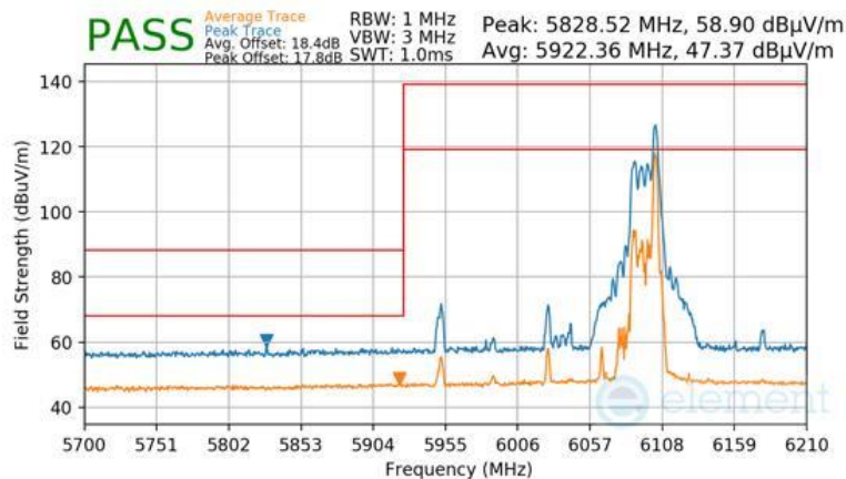
Plot 7-1716 CDD Primary Radiated Lower Band Edge (Peak & Average – UNII Band 5) - RU26
