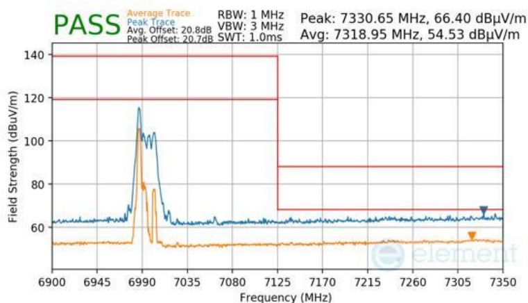
Plot 7-1717 SDM Primary Radiated Upper Band Edge (Peak & Average – UNII Band 8) - RU26
