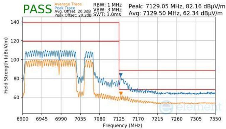
Plot 7-1772 SDM Primary Radiated Upper Band Edge (Peak & Average – UNII Band 8) - RU996+484+242
