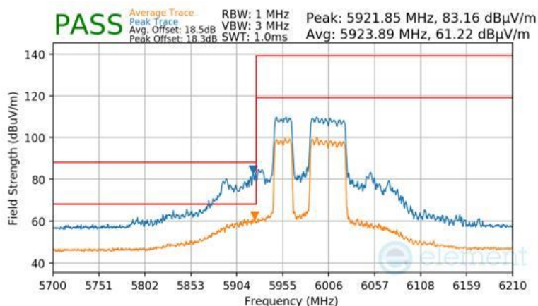
Plot 7-1720 CDD Primary Radiated Lower Band Edge (Peak & Average – UNII Band 5) - RU484+242
