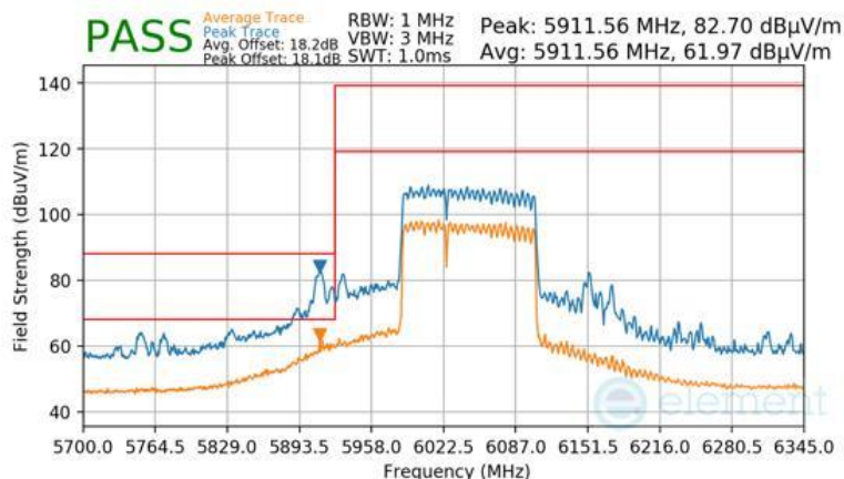
Plot 7-1742 CDD Primary Radiated Lower Band Edge (Peak & Average – UNII Band 5) - RU996+484 (L)
