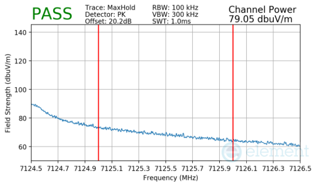
Plot 7-1701 SDM Primary Radiated Upper Band Edge (Peak – UNII Band 8)
