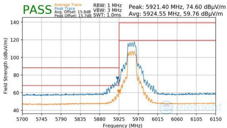
Plot 7-1698 CDD Primary Radiated Lower Band Edge (Peak & Average – UNII Band 5) - RU242
