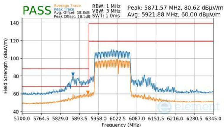
Plot 7-1747 CDD Primary Radiated Lower Band Edge (Peak & Average – UNII Band 5) - RU996+484
