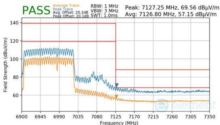
Plot 7-1751 SDM Primary Radiated Upper Band Edge (Peak & Average – UNII Band 8) - RU996+484
