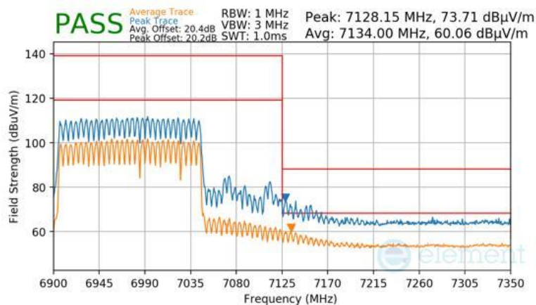
Plot 7-1775 SDM Primary Radiated Upper Band Edge (Peak & Average – UNII Band 8) - RU996+484+242
