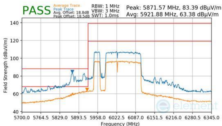
Plot 7-1663 Antenna WF7 Radiated Lower Band Edge (Peak & Average – UNII Band 5) - RU996+484+242 (L)
