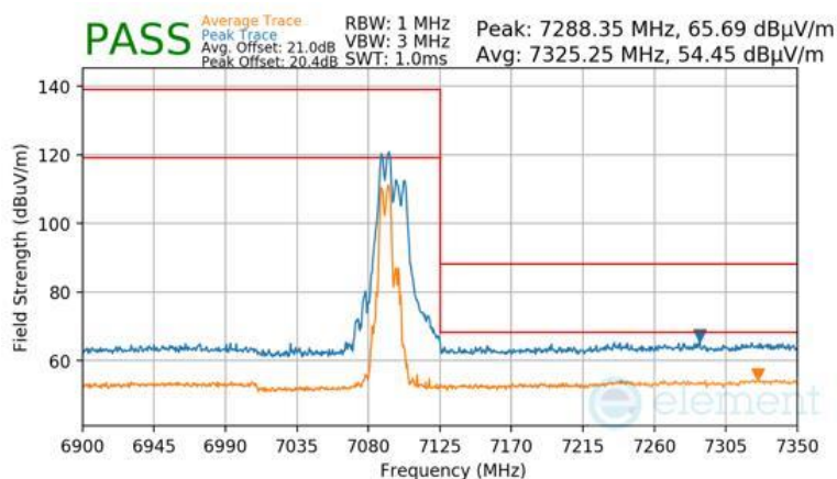
Plot 7-1790 SDM Diversity Radiated Upper Band Edge (Peak & Average – UNII Band 8) - RU52+26
