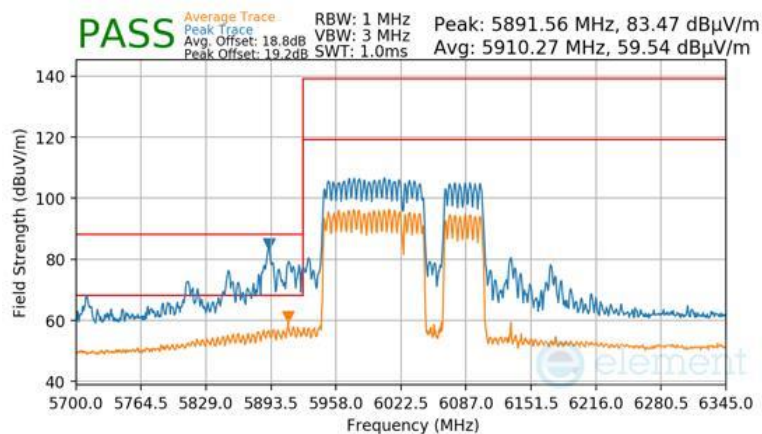
Plot 7-1757 CDD Primary Radiated Lower Band Edge (Peak & Average – UNII Band 5) - RU996+484+242
