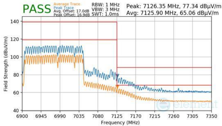
Plot 7-1776 SDM Primary Radiated Upper Band Edge (Peak & Average – UNII Band 8) - RU996+484+242 (H)
