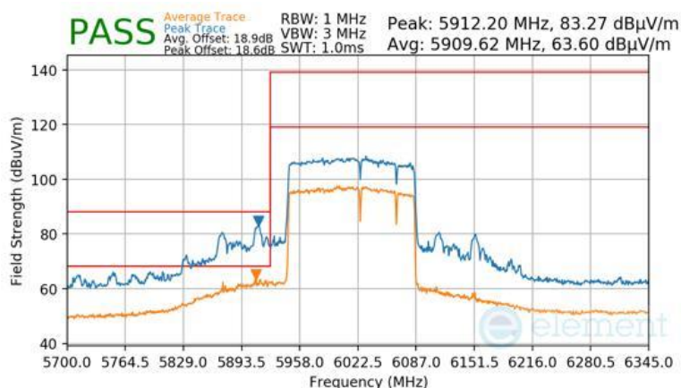
Plot 7-1669 Antenna WF7 Radiated Lower Band Edge (Peak & Average – UNII Band 5) - RU996+484+242 (H)
