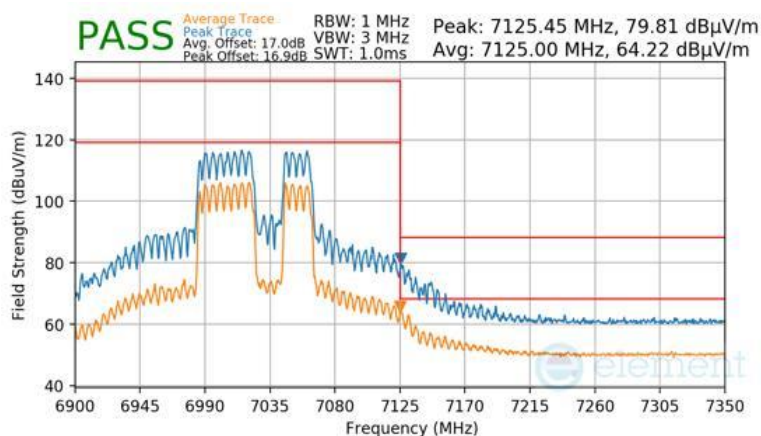
Plot 7-1729 SDM Primary Radiated Upper Band Edge (Peak & Average – UNII Band 8) - RU484+242
