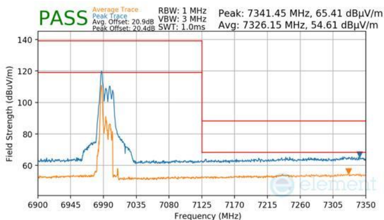
Plot 7-1740 SDM Primary Radiated Upper Band Edge (Peak & Average – UNII Band 8) - RU26
