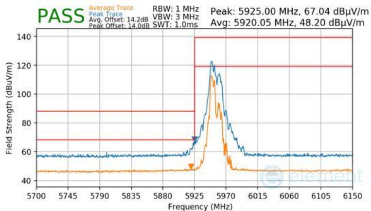
Plot 7-1786 CDD Diversity Radiated Lower Band Edge (Peak & Average – UNII Band 5) - RU52+26
