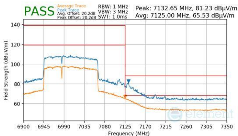
Plot 7-1654 Antenna WF7 Radiated Upper Band Edge (Peak & Average – UNII Band 8) - RU996+484 (L)
