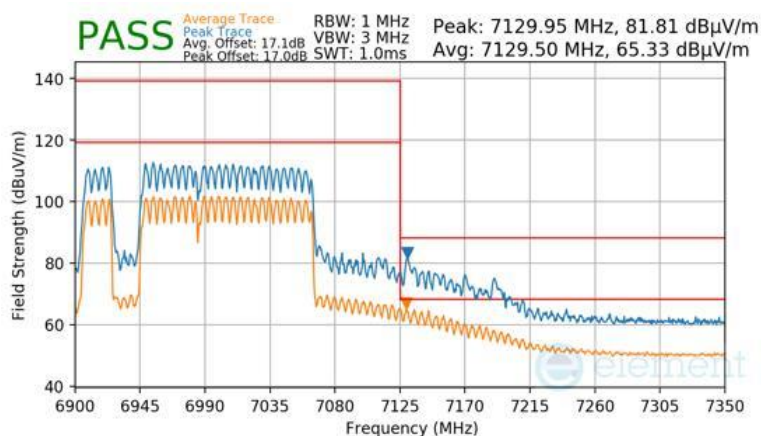
Plot 7-1770 SDM Primary Radiated Upper Band Edge (Peak & Average – UNII Band 8) - RU996+484+242 (L)
