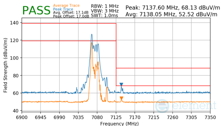
Plot 7-1707 SDM Primary Radiated Upper Band Edge (Peak & Average – UNII Band 8) - RU26
