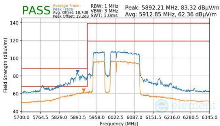
Plot 7-1666 Antenna WF7 Radiated Lower Band Edge (Peak & Average – UNII Band 5) - RU996+484+242 (L)
