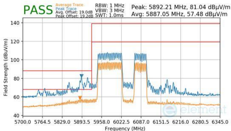
Plot 7-1744 CDD Primary Radiated Lower Band Edge (Peak & Average – UNII Band 5) - RU996+484
