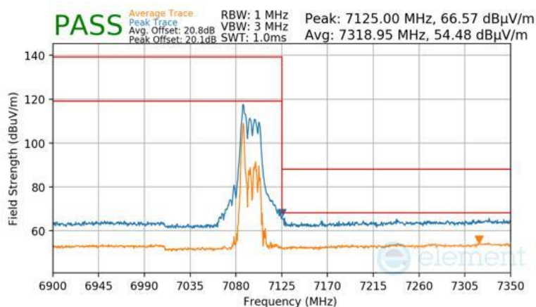
Plot 7-1784 SDM Diversity Radiated Upper Band Edge (Peak & Average – UNII Band 8) - RU26
