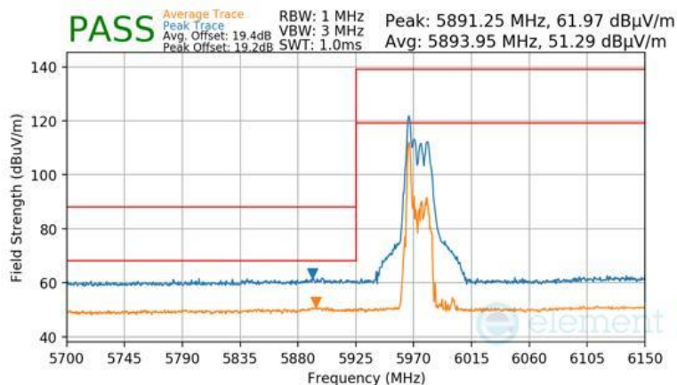
Plot 7-1688 CDD Primary Radiated Lower Band Edge (Peak & Average – UNII Band 5) - RU26
