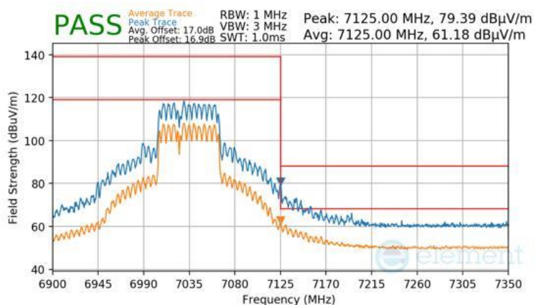
Plot 7-1727 SDM Primary Radiated Upper Band Edge (Peak & Average – UNII Band 8) - RU484+242
