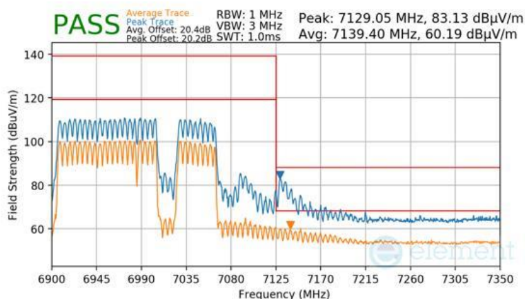
Plot 7-1769 SDM Primary Radiated Upper Band Edge (Peak & Average – UNII Band 8) - RU996+484+242
