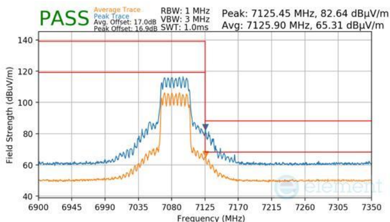
Plot 7-1712 SDM Primary Radiated Upper Band Edge (Peak & Average – UNII Band 8) - RU484
