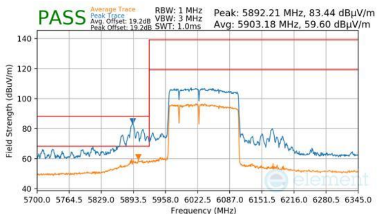
Plot 7-1661 Antenna WF7 Radiated Lower Band Edge (Peak & Average – UNII Band 5) - RU996+484+242 (L)
