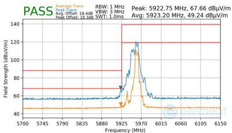
Plot 7-1693 CDD Primary Radiated Lower Band Edge (Peak & Average – UNII Band 5) - RU52+26
