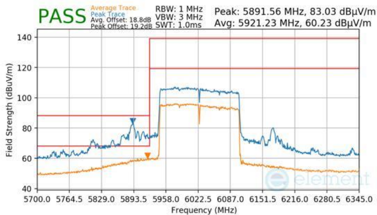
Plot 7-1684 Antenna WF7 Radiated Lower Band Edge (Peak & Average – UNII Band 5) - RU996X2
