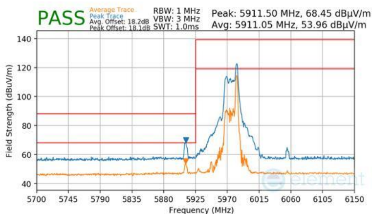
Plot 7-1704 CDD Primary Radiated Lower Band Edge (Peak & Average – UNII Band 5) - RU26
