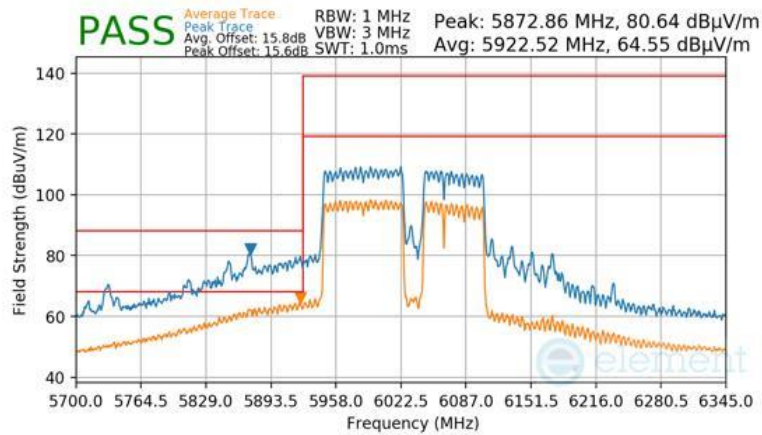
Plot 7-1756 CDD Primary Radiated Lower Band Edge (Peak & Average – UNII Band 5) - RU996+484+242 (H)
