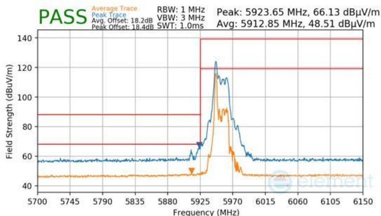
Plot 7-1686 CDD Primary Radiated Lower Band Edge (Peak & Average – UNII Band 5) - RU26
