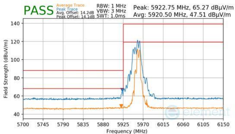
Plot 7-1787 CDD Diversity Radiated Lower Band Edge (Peak & Average – UNII Band 5) - RU52+26
