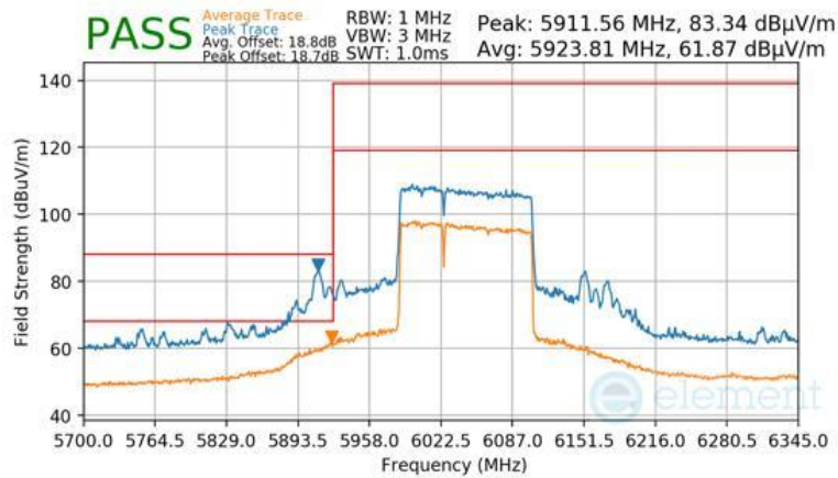
Plot 7-1648 Antenna WF7 Radiated Lower Band Edge (Peak & Average – UNII Band 5) - RU996+484 (L)
