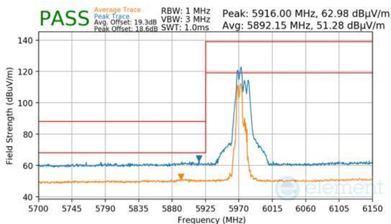
Plot 7-1788 CDD Diversity Radiated Lower Band Edge (Peak & Average – UNII Band 5) - RU52+26
