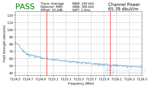
Plot 7-1702 SDM Primary Radiated Upper Band Edge (Average – UNII Band 8)
