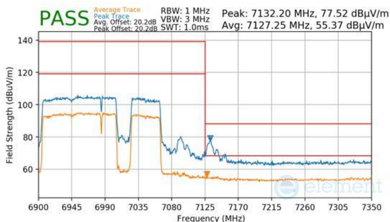
Plot 7-1677 Antenna WF7 Radiated Upper Band Edge (Peak & Average – UNII Band 8) - RU996+484+242
