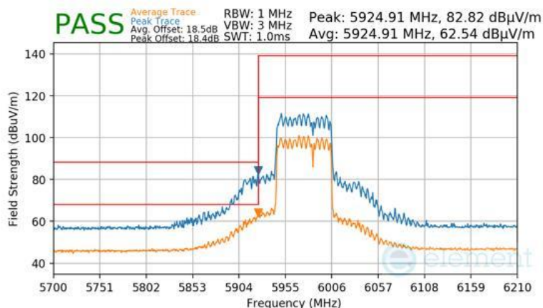
Plot 7-1722 CDD Primary Radiated Lower Band Edge (Peak & Average – UNII Band 5) - RU484+242
