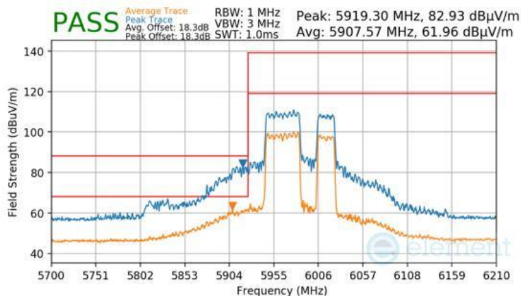
Plot 7-1721 CDD Primary Radiated Lower Band Edge (Peak & Average – UNII Band 5) - RU484+242
