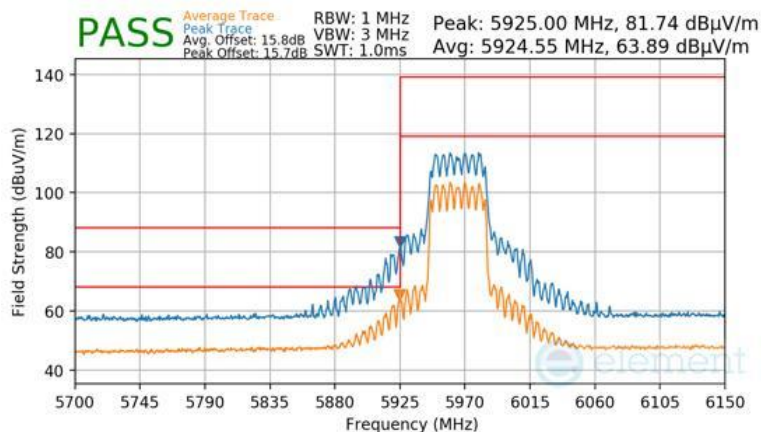
Plot 7-1709 CDD Primary Radiated Lower Band Edge (Peak & Average – UNII Band 5) - RU484
