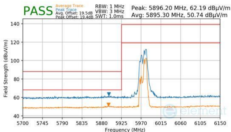
Plot 7-1789 CDD Diversity Radiated Lower Band Edge (Peak & Average – UNII Band 5) - RU52+26
