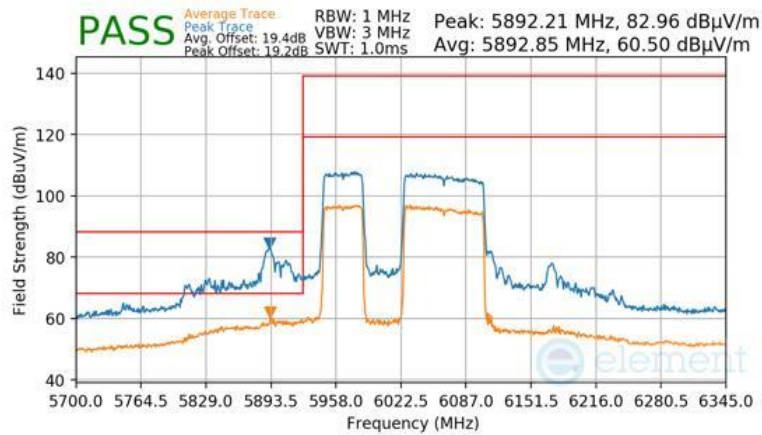
Plot 7-1652 Antenna WF7 Radiated Lower Band Edge (Peak & Average – UNII Band 5) - RU996+484 (L)
