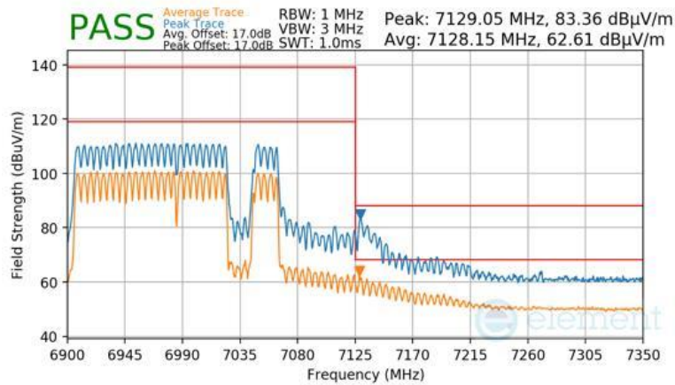
Plot 7-1774 SDM Primary Radiated Upper Band Edge (Peak & Average – UNII Band 8) - RU996+484+242 (H)
