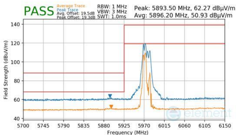
Plot 7-1694 CDD Primary Radiated Lower Band Edge (Peak & Average – UNII Band 5) - RU52+26
