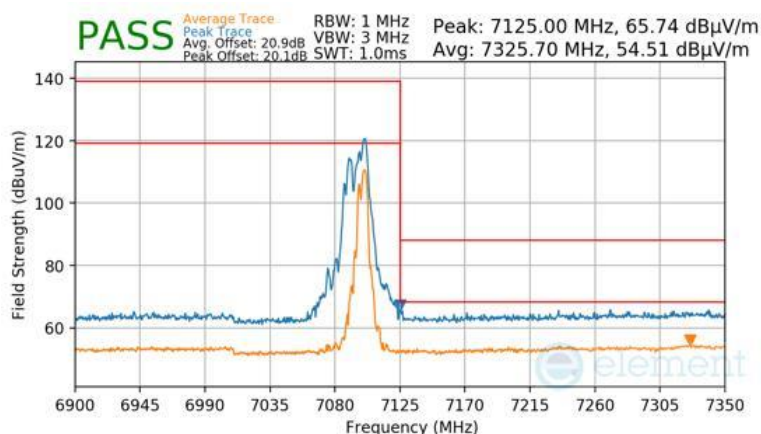
Plot 7-1791 SDM Diversity Radiated Upper Band Edge (Peak & Average – UNII Band 8) - RU52+26
