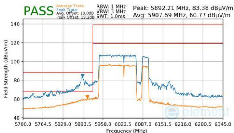
Plot 7-1667 Antenna WF7 Radiated Lower Band Edge (Peak & Average – UNII Band 5) - RU996+484+242 (H)
