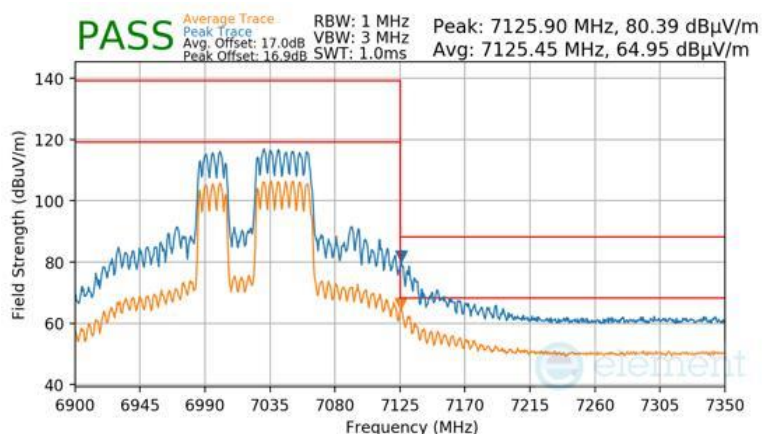
Plot 7-1728 SDM Primary Radiated Upper Band Edge (Peak & Average – UNII Band 8) - RU484+242
