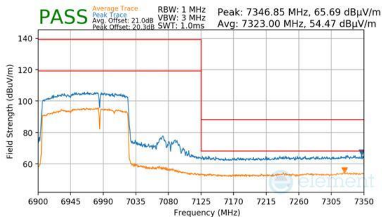
Plot 7-1659 Antenna WF7 Radiated Upper Band Edge (Peak & Average – UNII Band 8) - RU996+484
