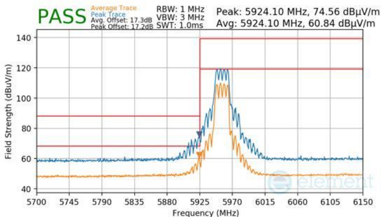
Plot 7-1792 CDD Diversity Radiated Lower Band Edge (Peak & Average – UNII Band 5) - RU242
