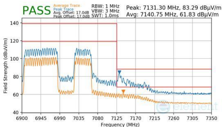
Plot 7-1750 SDM Primary Radiated Upper Band Edge (Peak & Average – UNII Band 8) - RU996+484 (H)
