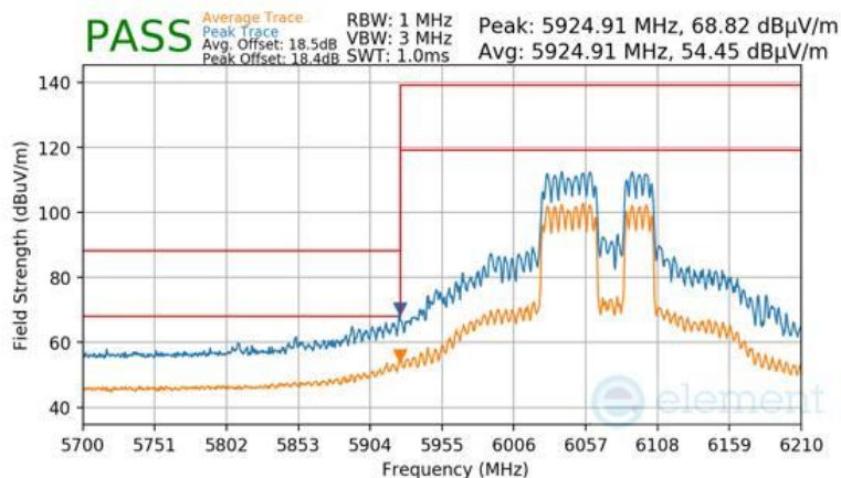
Plot 7-1725 CDD Primary Radiated Lower Band Edge (Peak & Average – UNII Band 5) - RU484+242
