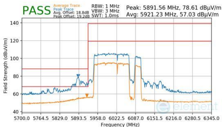
Plot 7-1668 Antenna WF7 Radiated Lower Band Edge (Peak & Average – UNII Band 5) - RU996+484+242
