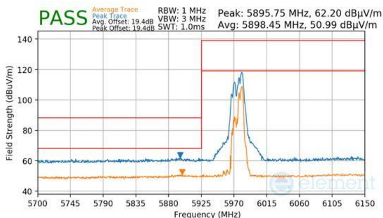
Plot 7-1695 CDD Primary Radiated Lower Band Edge (Peak & Average – UNII Band 5) - RU52+26
