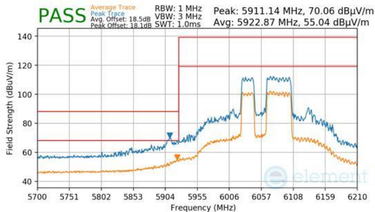
Plot 7-1724 CDD Primary Radiated Lower Band Edge (Peak & Average – UNII Band 5) - RU484+242
