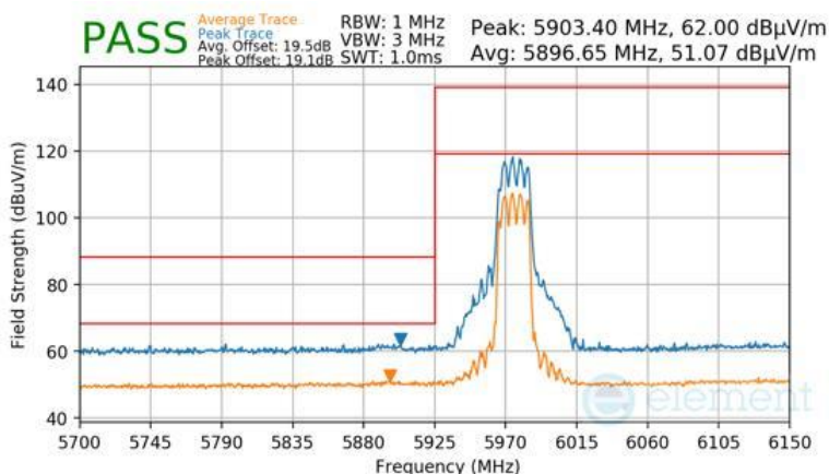
Plot 7-1793 CDD Diversity Radiated Lower Band Edge (Peak & Average – UNII Band 5) - RU242
