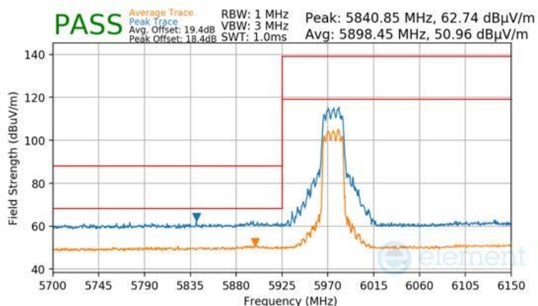
Plot 7-1699 CDD Primary Radiated Lower Band Edge (Peak & Average – UNII Band 5) - RU242
