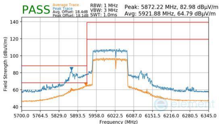
Plot 7-1745 CDD Primary Radiated Lower Band Edge (Peak & Average – UNII Band 5) - RU996+484 (H)
