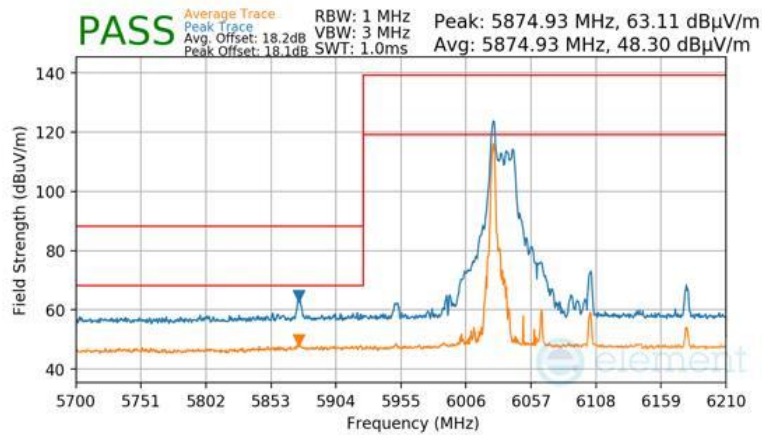
Plot 7-1715 CDD Primary Radiated Lower Band Edge (Peak & Average – UNII Band 5) - RU26
