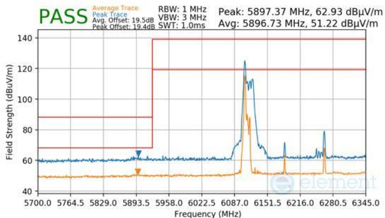
Plot 7-1736 CDD Primary Radiated Lower Band Edge (Peak & Average – UNII Band 5) - RU26
