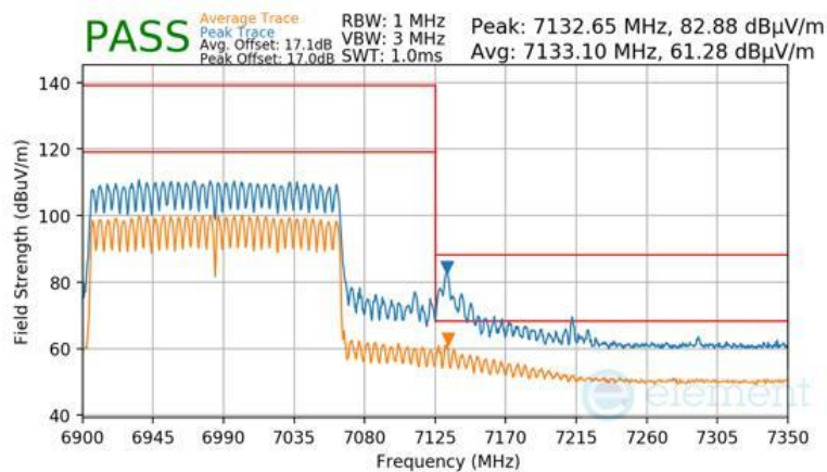
Plot 7-1779 SDM Primary Radiated Upper Band Edge (Peak & Average – UNII Band 8) - RU996X2
