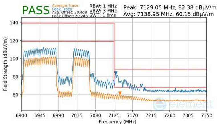
Plot 7-1748 SDM Primary Radiated Upper Band Edge (Peak & Average – UNII Band 8) - RU996+484
