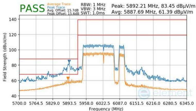
Plot 7-1762 CDD Primary Radiated Lower Band Edge (Peak & Average – UNII Band 5) - RU996+484+242 (H)
