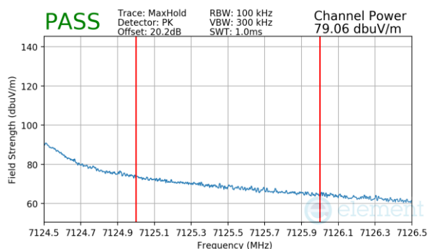
Plot 7-1795 SDM Diversity Radiated Upper Band Edge (Peak – UNII Band 8)
