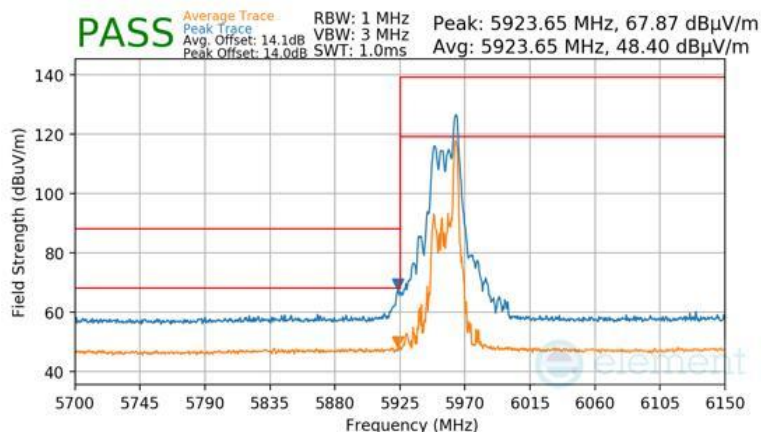
Plot 7-1781 CDD Diversity Radiated Lower Band Edge (Peak & Average – UNII Band 5) - RU26
