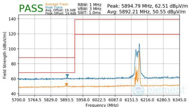
Plot 7-1737 CDD Primary Radiated Lower Band Edge (Peak & Average – UNII Band 5) - RU26
