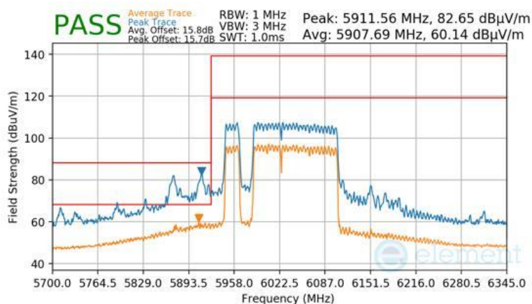
Plot 7-1758 CDD Primary Radiated Lower Band Edge (Peak & Average – UNII Band 5) - RU996+484+242 (L)
