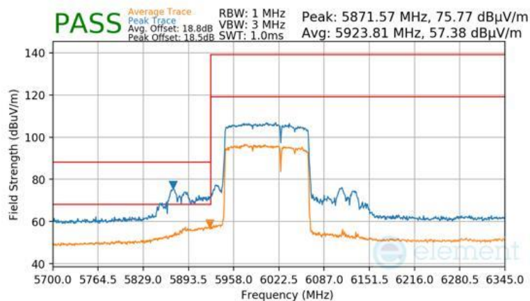
Plot 7-1653 Antenna WF7 Radiated Lower Band Edge (Peak & Average – UNII Band 5) - RU996+484
