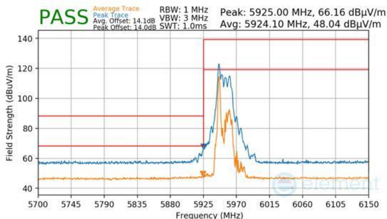
Plot 7-1780 CDD Diversity Radiated Lower Band Edge (Peak & Average – UNII Band 5) - RU26
