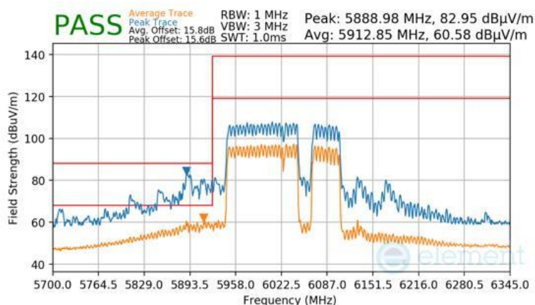
Plot 7-1759 CDD Primary Radiated Lower Band Edge (Peak & Average – UNII Band 5) - RU996+484+242 (H)
