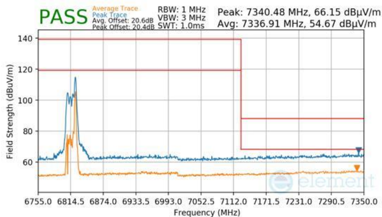
Plot 7-1739 SDM Primary Radiated Upper Band Edge (Peak & Average – UNII Band 7) - RU26
