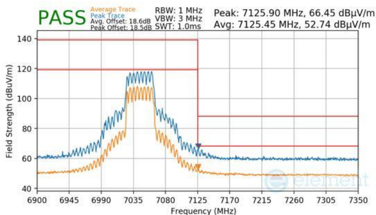
Plot 7-1711 SDM Primary Radiated Upper Band Edge (Peak & Average – UNII Band 8) - RU484
