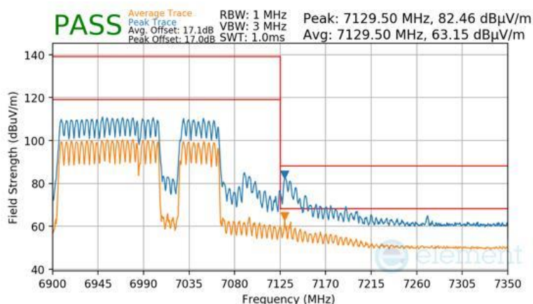
Plot 7-1771 SDM Primary Radiated Upper Band Edge (Peak & Average – UNII Band 8) - RU996+484+242 (H)
