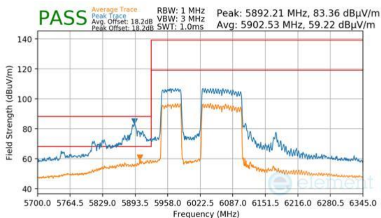
Plot 7-1746 CDD Primary Radiated Lower Band Edge (Peak & Average – UNII Band 5) - RU996+484 (L)
