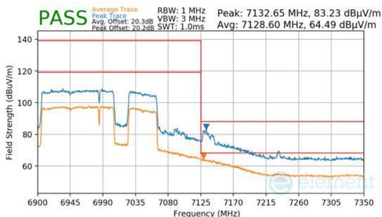
Plot 7-1675 Antenna WF7 Radiated Upper Band Edge (Peak & Average – UNII Band 8) - RU996+484+242 (H)
