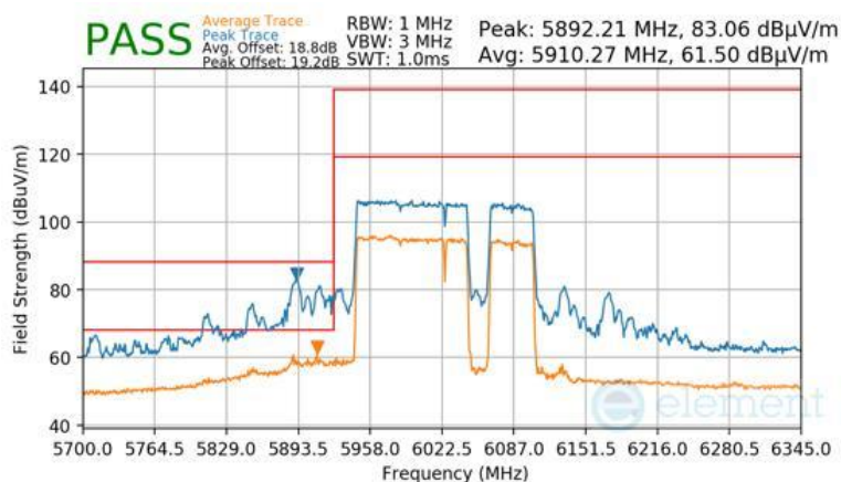
Plot 7-1664 Antenna WF7 Radiated Lower Band Edge (Peak & Average – UNII Band 5) - RU996+484+242 (H)
