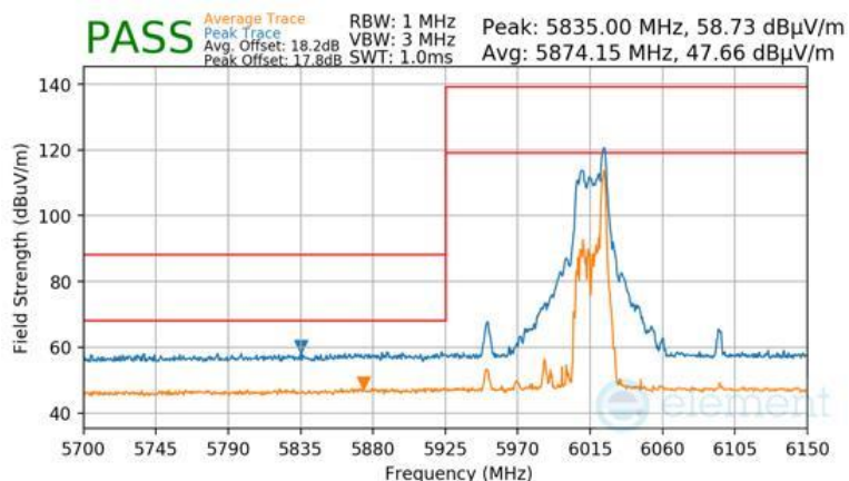
Plot 7-1706 CDD Primary Radiated Lower Band Edge (Peak & Average – UNII Band 5) - RU26
