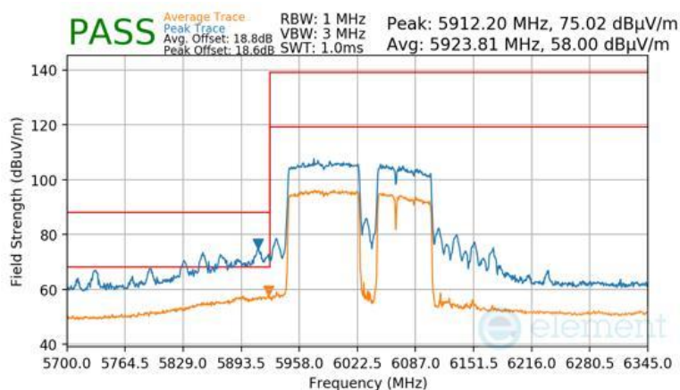
Plot 7-1662 Antenna WF7 Radiated Lower Band Edge (Peak & Average – UNII Band 5) - RU996+484+242
