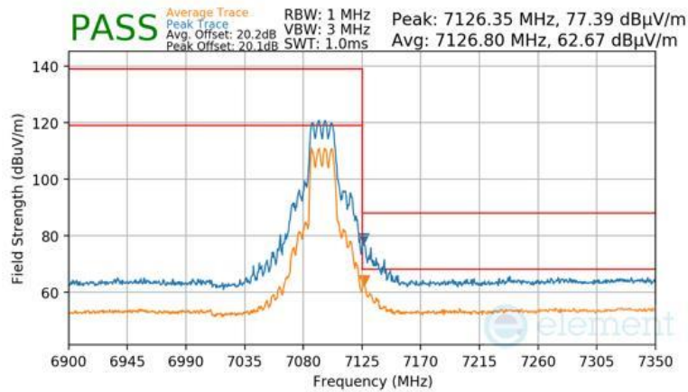
Plot 7-1700 SDM Primary Radiated Upper Band Edge (Peak & Average – UNII Band 8) - RU242
