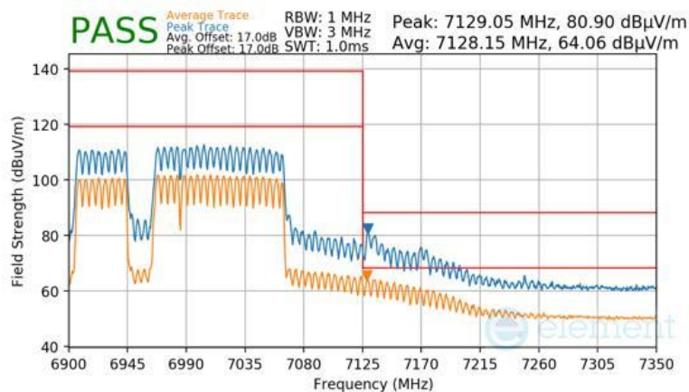
Plot 7-1773 SDM Primary Radiated Upper Band Edge (Peak & Average – UNII Band 8) - RU996+484+242 (L)
