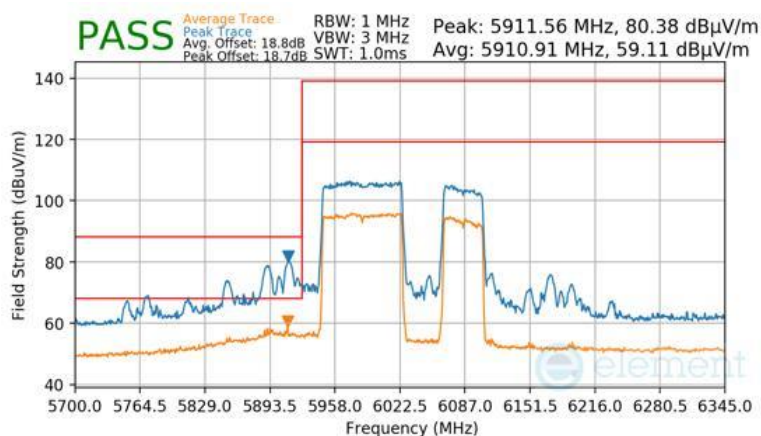
Plot 7-1650 Antenna WF7 Radiated Lower Band Edge (Peak & Average – UNII Band 5) - RU996+484
