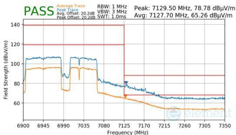
Plot 7-1672 Antenna WF7 Radiated Upper Band Edge (Peak & Average – UNII Band 8) - RU996+484+242 (H)
