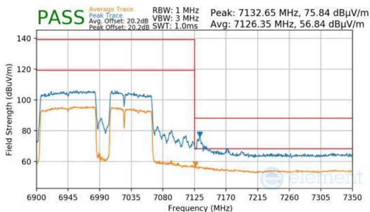
Plot 7-1674 Antenna WF7 Radiated Upper Band Edge (Peak & Average – UNII Band 8) - RU996+484+242
