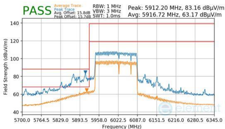
Plot 7-1764 CDD Primary Radiated Lower Band Edge (Peak & Average – UNII Band 5) - RU996+484+242 (H)
