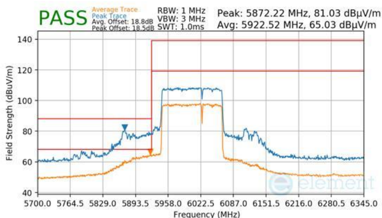
Plot 7-1651 Antenna WF7 Radiated Lower Band Edge (Peak & Average – UNII Band 5) - RU996+484 (H)
