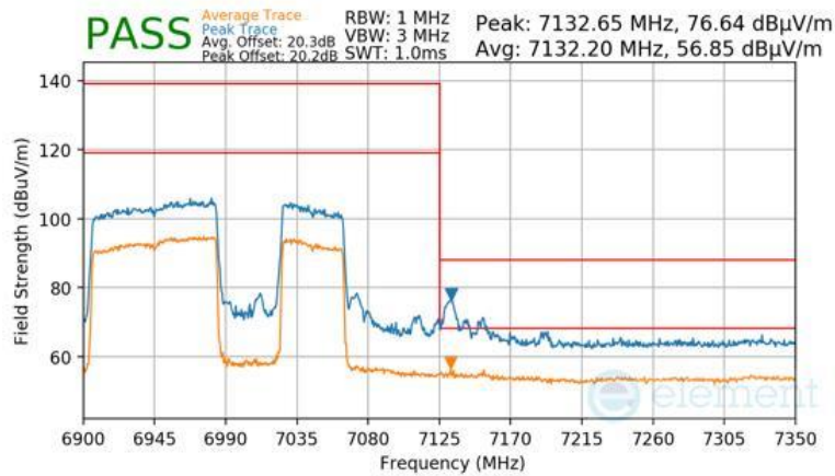
Plot 7-1656 Antenna WF7 Radiated Upper Band Edge (Peak & Average – UNII Band 8) - RU996+484
