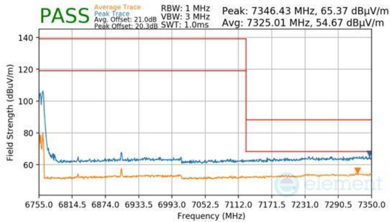
Plot 7-1738 SDM Primary Radiated Upper Band Edge (Peak & Average – UNII Band 7) - RU26
