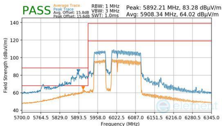
Plot 7-1761 CDD Primary Radiated Lower Band Edge (Peak & Average – UNII Band 5) - RU996+484+242 (L)
