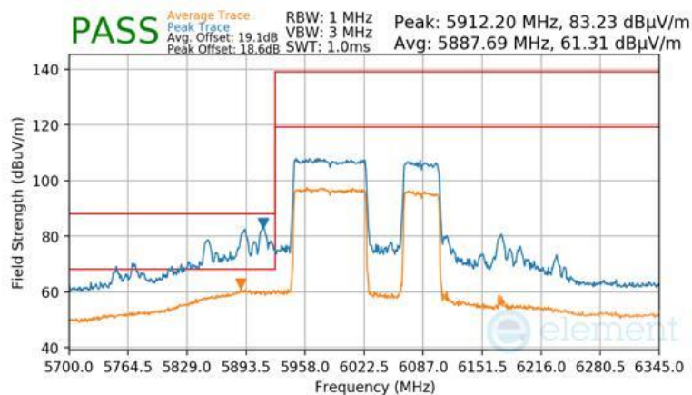
Plot 7-1649 Antenna WF7 Radiated Lower Band Edge (Peak & Average – UNII Band 5) - RU996+484 (H)
