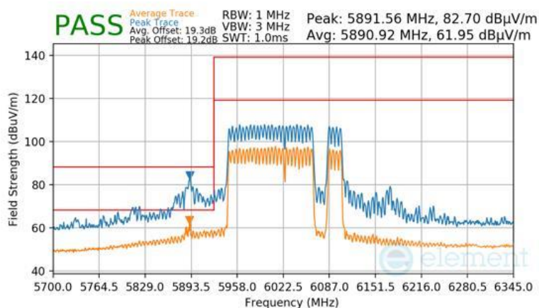
Plot 7-1760 CDD Primary Radiated Lower Band Edge (Peak & Average – UNII Band 5) - RU996+484+242
