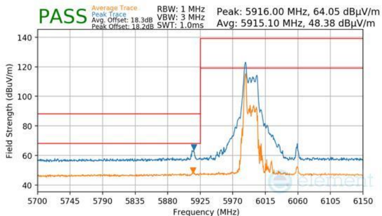
Plot 7-1705 CDD Primary Radiated Lower Band Edge (Peak & Average – UNII Band 5) - RU26
