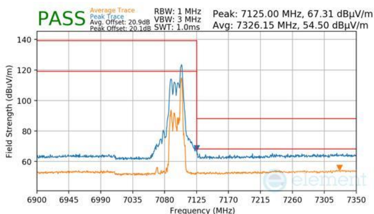
Plot 7-1785 SDM Diversity Radiated Upper Band Edge (Peak & Average – UNII Band 8) - RU26
