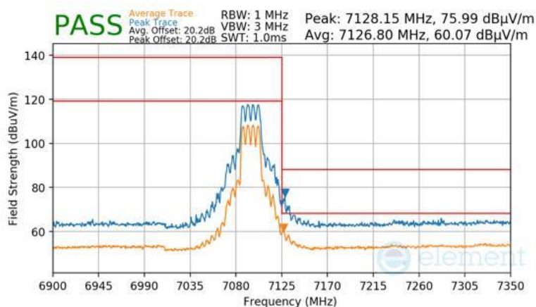
Plot 7-1794 SDM Diversity Radiated Upper Band Edge (Peak & Average – UNII Band 8) - RU242
