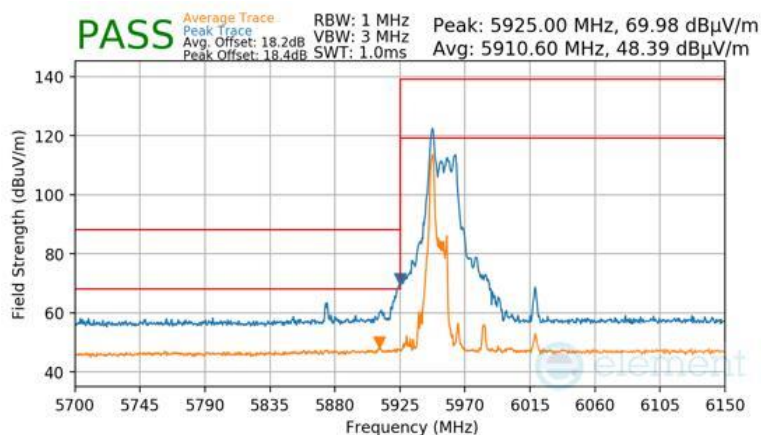
Plot 7-1703 CDD Primary Radiated Lower Band Edge (Peak & Average – UNII Band 5) - RU26
