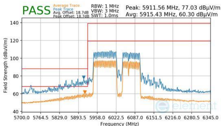
Plot 7-1755 CDD Primary Radiated Lower Band Edge (Peak & Average – UNII Band 5) - RU996+484+242
