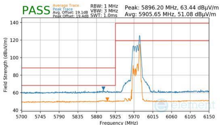
Plot 7-1783 CDD Diversity Radiated Lower Band Edge (Peak & Average – UNII Band 5) - RU26
