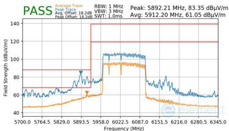
Plot 7-1754 CDD Primary Radiated Lower Band Edge (Peak & Average – UNII Band 5) - RU996+484+242 (L)
