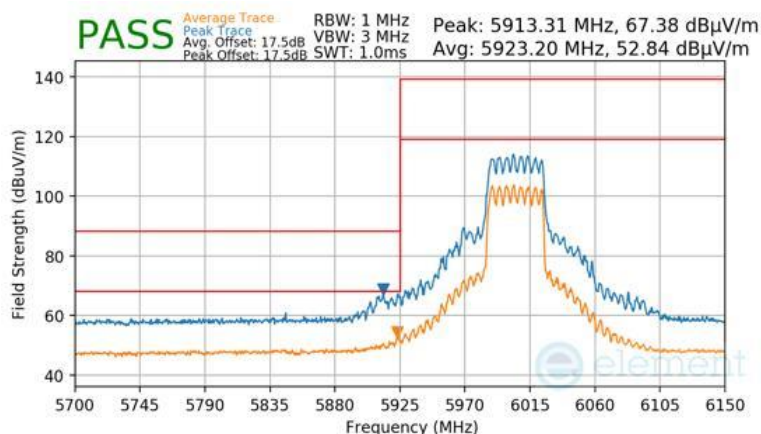
Plot 7-1710 CDD Primary Radiated Lower Band Edge (Peak & Average – UNII Band 5) - RU484
