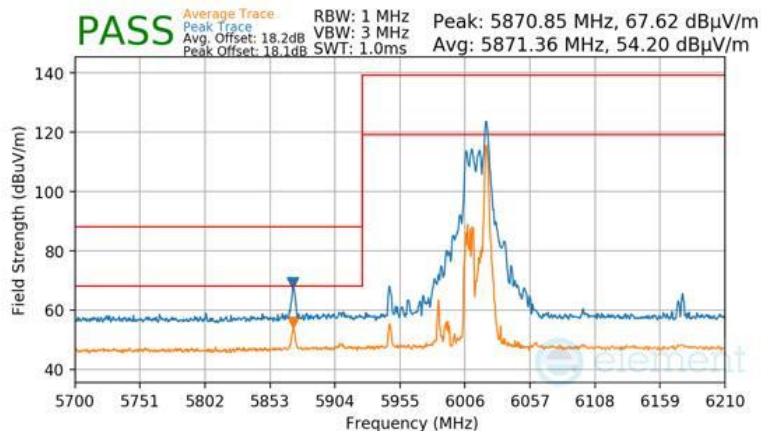
Plot 7-1714 CDD Primary Radiated Lower Band Edge (Peak & Average – UNII Band 5) - RU26
