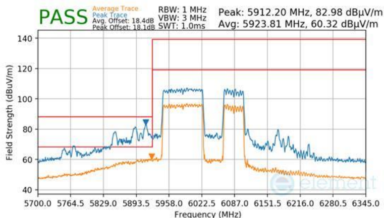
Plot 7-1743 CDD Primary Radiated Lower Band Edge (Peak & Average – UNII Band 5) - RU996+484 (H)
