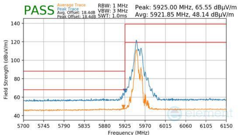
Plot 7-1692 CDD Primary Radiated Lower Band Edge (Peak & Average – UNII Band 5) - RU52+26
