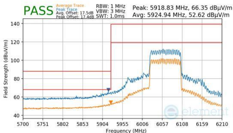
Plot 7-1732 CDD Primary Radiated Lower Band Edge (Peak & Average – UNII Band 5) - RU996
