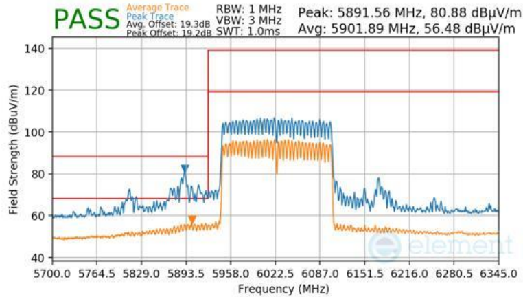
Plot 7-1778 CDD Primary Radiated Lower Band Edge (Peak & Average – UNII Band 5) - RU996X2
