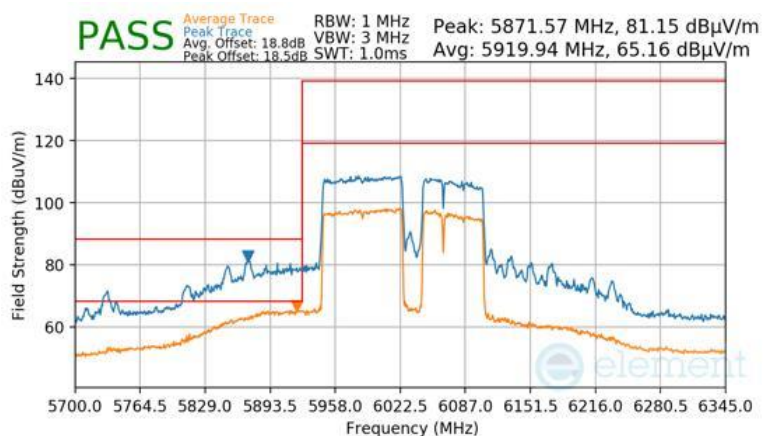
Plot 7-1660 Antenna WF7 Radiated Lower Band Edge (Peak & Average – UNII Band 5) - RU996+484+242 (H)
