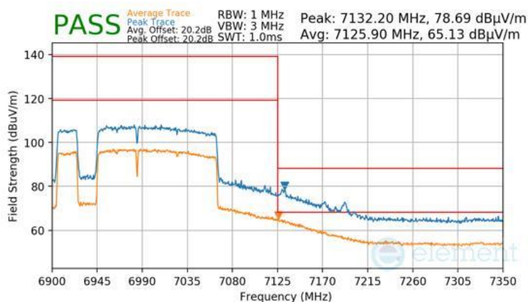
Plot 7-1676 Antenna WF7 Radiated Upper Band Edge (Peak & Average – UNII Band 8) - RU996+484+242 (L)
