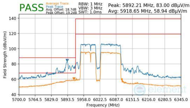
Plot 7-1670 Antenna WF7 Radiated Lower Band Edge (Peak & Average – UNII Band 5) - RU996+484+242 (L)
