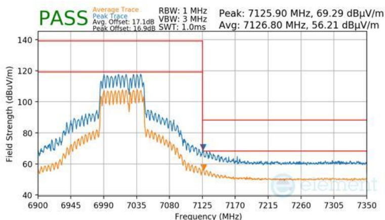
Plot 7-1730 SDM Primary Radiated Upper Band Edge (Peak & Average – UNII Band 8) - RU484+242
