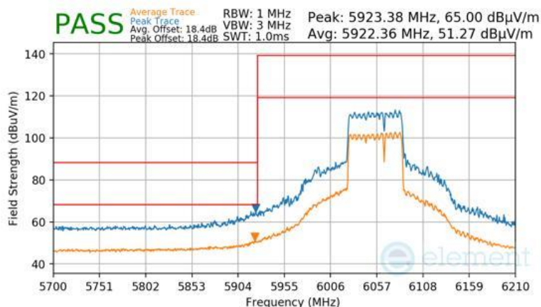
Plot 7-1726 CDD Primary Radiated Lower Band Edge (Peak & Average – UNII Band 5) - RU484+242
