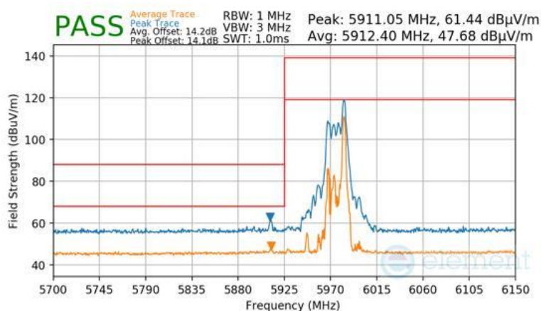
Plot 7-1798 CDD Diversity Radiated Lower Band Edge (Peak & Average – UNII Band 5) - RU26
