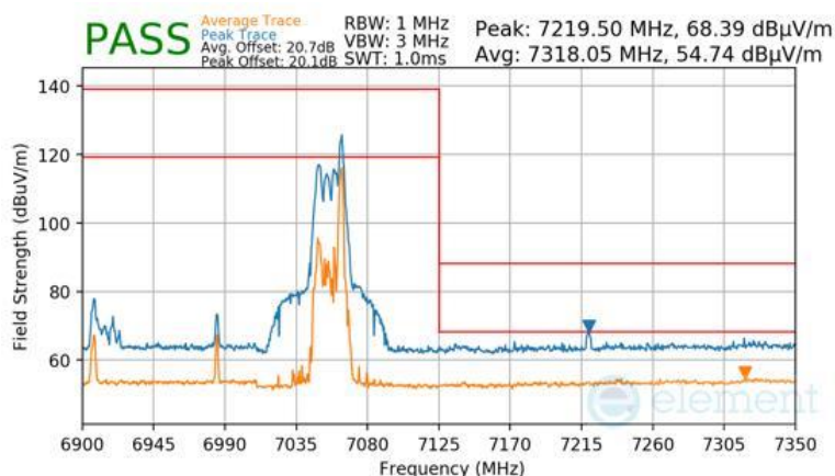
Plot 7-1741 SDM Primary Radiated Upper Band Edge (Peak & Average – UNII Band 8) - RU26
