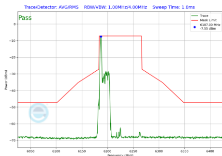
Plot 7-487 In-Band Emission Plot Antenna WF8 (80MHz BW 802.11be(RU) RU26 Index0 (UNII Band 5) - Ch.55)
