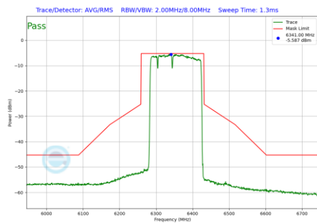
Plot 7-459 In-Band Emission Plot Antenna WF5B (160MHz BW 802.11be(RU) RU996+484+242 Index96 (UNII Band 5) - Ch.79)
