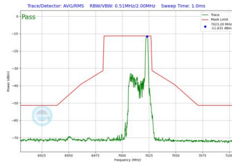
Plot 7-542 In-Band Emission Plot Antenna WF7 (40MHz BW 802.11be(RU) RU26 Index17 (UNII Band 8) - Ch.211)
