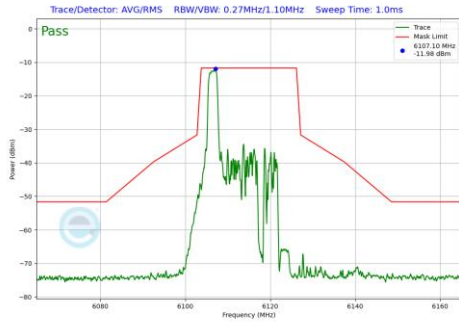
Plot 7-529 In-Band Emission Plot Antenna WF7 (20MHz BW 802.11be(RU) RU26 Index0 (UNII Band 5) - Ch.33)
