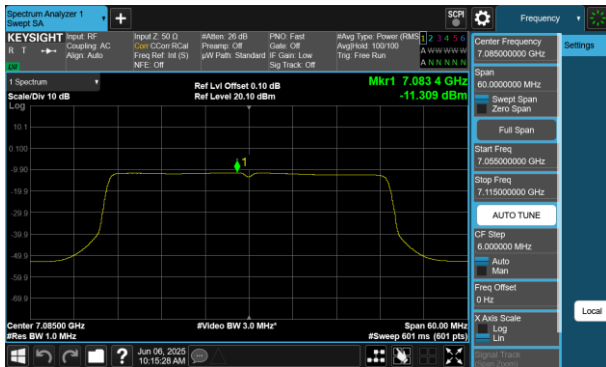
Plot 7-434 PSD SDM Diversity Antenna WF8 (40MHz BW 802.11be(RU) RU484 Index65 - Ch.227)
