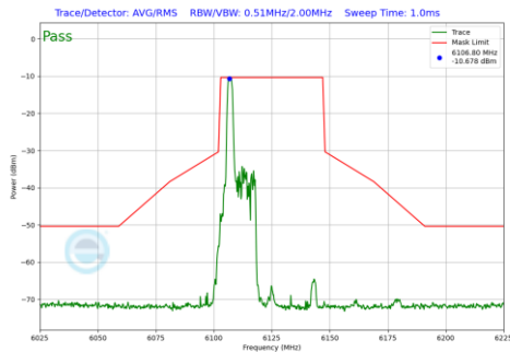
Plot 7-442 In-Band Emission Plot Antenna WF5B (40MHz BW 802.11be(RU) RU26 Index0 (UNII Band 5) - Ch.35)
