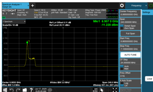
Plot 7-422 PSD SDM Diversity Antenna WF8 (160MHz BW 802.11be(RU) RU26 Index0 - Ch.207)
