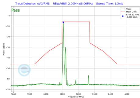
Plot 7-532 In-Band Emission Plot Antenna WF7 (160MHz BW 802.11be(RU) RU26 Index0 (UNII Band 5) - Ch.47)
