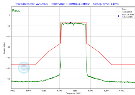
Plot 7-515 In-Band Emission Plot Antenna WF8 (80MHz BW 802.11be(RU) RU996 Index67 (UNII Band 5) - Ch.39)
