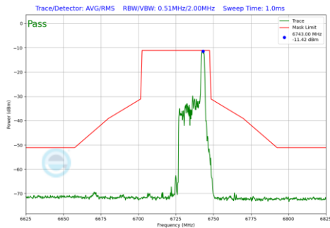
Plot 7-450 In-Band Emission Plot Antenna WF5B (40MHz BW 802.11be(RU) RU26 Index17 (UNII Band 7) - Ch.155)
