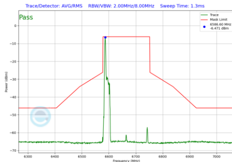
Plot 7-496 In-Band Emission Plot Antenna WF8 (160MHz BW 802.11be(RU) RU26 Index0 (UNII Band 7) - Ch.143)
