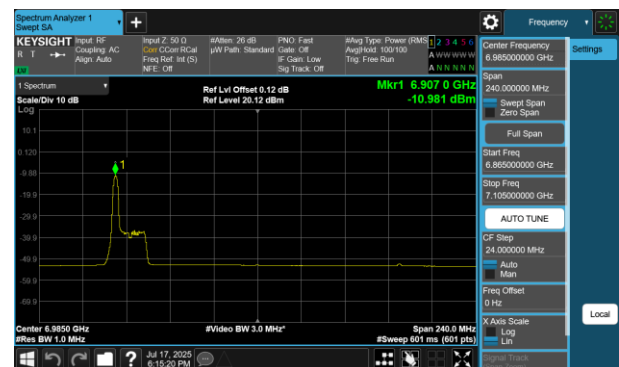
Plot 7-426 PSD SDM Diversity Antenna WF7 (160MHz BW 802.11be(RU) RU26 Index0 - Ch.207)
