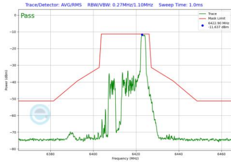
Plot 7-485 In-Band Emission Plot Antenna WF8 (20MHz BW 802.11be(RU) RU26 Index8 (UNII Band 5) - Ch.93)
