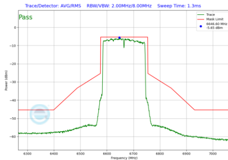
Plot 7-480 In-Band Emission Plot Antenna WF5B (160MHz BW 802.11be(RU) RU996X2 Index68 (UNII Band 7) - Ch.143)
