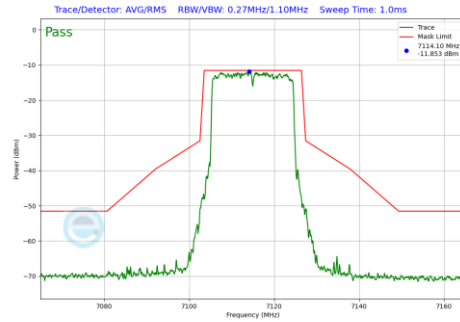
Plot 7-525 In-Band Emission Plot Antenna WF8 (20MHz BW 802.11be(RU) RU242 Index61 (UNII Band 8) - Ch.233)
