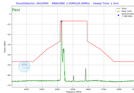
Plot 7-536 In-Band Emission Plot Antenna WF7 (160MHz BW 802.11be(RU) RU26 Index0 (UNII Band 6) - Ch.111)
