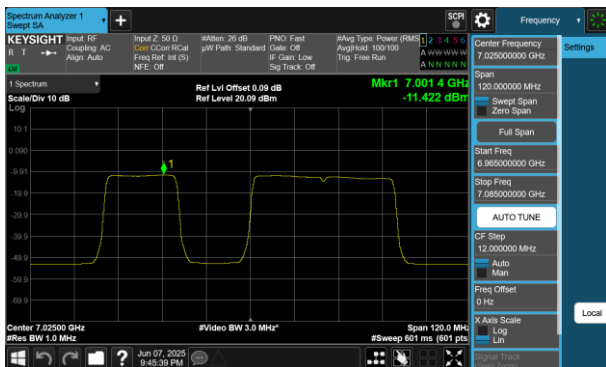
Plot 7-428 PSD SDM Diversity Antenna WF8 (80MHz BW 802.11be(RU) RU484+242 Index91 - Ch.215)
