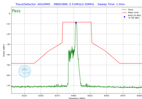
Plot 7-486 In-Band Emission Plot Antenna WF8 (40MHz BW 802.11be(RU) RU26 Index8 (UNII Band 5) - Ch.91)
