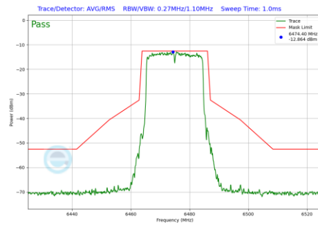
Plot 7-473 In-Band Emission Plot Antenna WF5B (20MHz BW 802.11be(RU) RU242 Index61 (UNII Band 6) - Ch.105)
