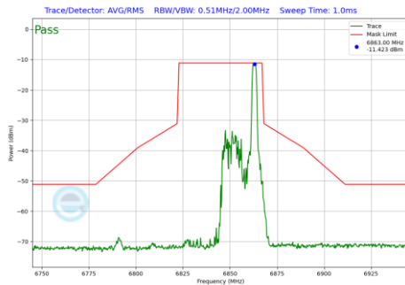
Plot 7-538 In-Band Emission Plot Antenna WF7 (40MHz BW 802.11be(RU) RU26 Index17 (UNII Band 7) - Ch.179)
