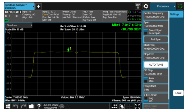
Plot 7-439 PSD SDM Diversity Antenna WF7 (80MHz BW 802.11be(RU) RU996 Index67 - Ch.215)
