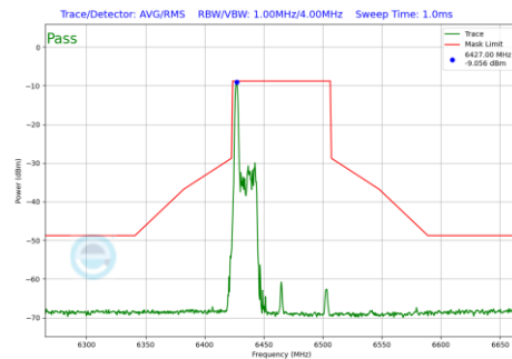
Plot 7-535 In-Band Emission Plot Antenna WF7 (80MHz BW 802.11be(RU) RU26 Index0 (UNII Band 6) - Ch.103)
