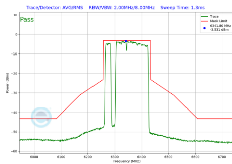
Plot 7-503 In-Band Emission Plot Antenna WF8 (160MHz BW 802.11be(RU) RU996+484+242 Index97 (UNII Band 5) - Ch.79)
