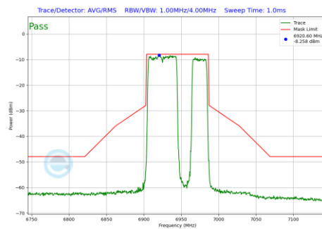
Plot 7-467 In-Band Emission Plot Antenna WF5B (80MHz BW 802.11be(RU) RU484+242 Index92 (UNII Band 8) - Ch.199)
