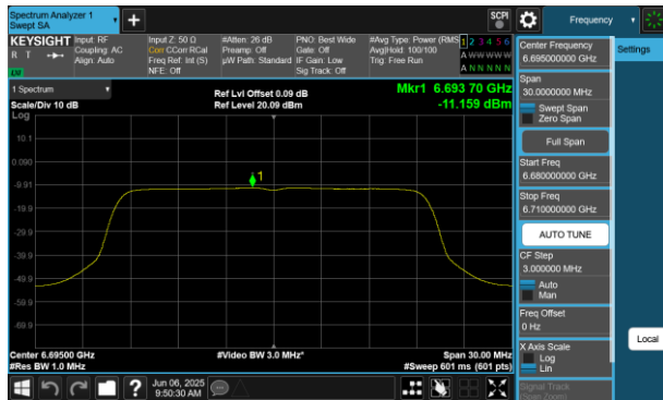
Plot 7-411 PSD SDM Diversity Antenna WF8 (20MHz BW 802.11be(RU) RU242 Index61 - Ch.149)
