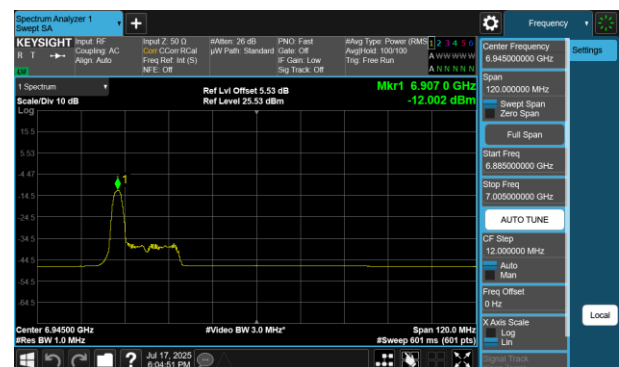
Plot 7-425 PSD SDM Diversity Antenna WF7 (80MHz BW 802.11be(RU) RU26 Index0 - Ch.199)
