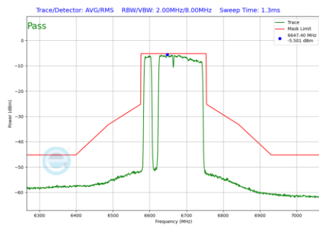
Plot 7-465 In-Band Emission Plot Antenna WF5B (160MHz BW 802.11be(RU) RU996+484+242 Index97 (UNII Band 7) - Ch.143)
