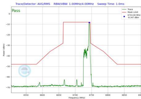
Plot 7-539 In-Band Emission Plot Antenna WF7 (80MHz BW 802.11be(RU) RU26 Index36 (UNII Band 7) - Ch.151)
