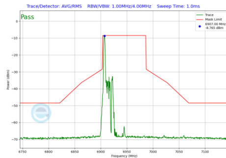
Plot 7-543 In-Band Emission Plot Antenna WF7 (80MHz BW 802.11be(RU) RU26 Index0 (UNII Band 8) - Ch.199)
