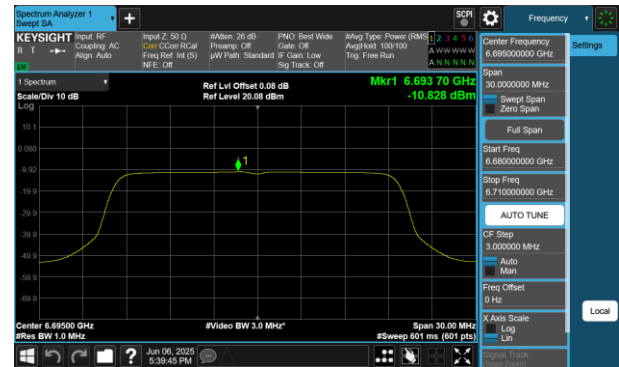
Plot 7-415 PSD SDM Diversity Antenna WF7 (20MHz BW 802.11be(RU) RU242 Index61 - Ch.149)
