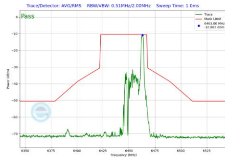
Plot 7-534 In-Band Emission Plot Antenna WF7 (40MHz BW 802.11be(RU) RU26 Index17 (UNII Band 6) - Ch.99)
