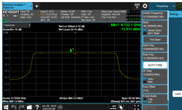
Plot 7-412 PSD SDM Diversity Antenna WF8 (40MHz BW 802.11be(RU) RU484 Index65 - Ch.155)
