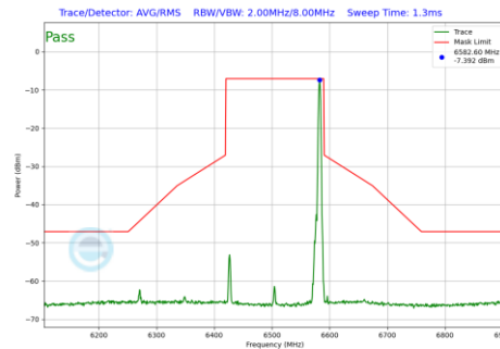
Plot 7-448 In-Band Emission Plot Antenna WF5B (160MHz BW 802.11be(RU) RU26 Index36 (UNII Band 6) - Ch.111)
