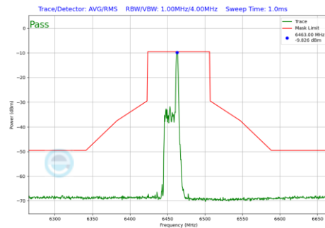
Plot 7-447 In-Band Emission Plot Antenna WF5B (80MHz BW 802.11be(RU) RU26 Index17 (UNII Band 6) - Ch.103)
