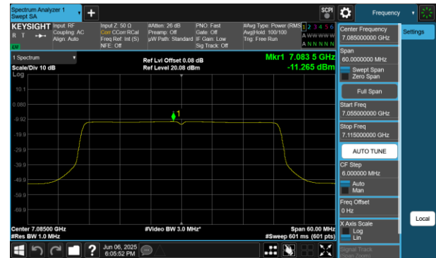
Plot 7-438 PSD SDM Diversity Antenna WF7 (40MHz BW 802.11be(RU) RU484 Index65 - Ch.227)
