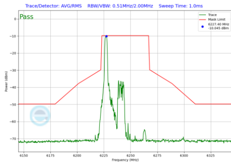
Plot 7-530 In-Band Emission Plot Antenna WF7 (40MHz BW 802.11be(RU) RU26 Index0 (UNII Band 5) - Ch.59)
