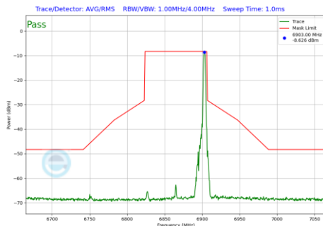
Plot 7-495 In-Band Emission Plot Antenna WF8 (80MHz BW 802.11be(RU) RU26 Index36 (UNII Band 7) - Ch.183)
