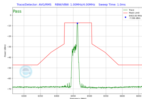
Plot 7-491 In-Band Emission Plot Antenna WF8 (80MHz BW 802.11be(RU) RU26 Index17 (UNII Band 6) - Ch.103)
