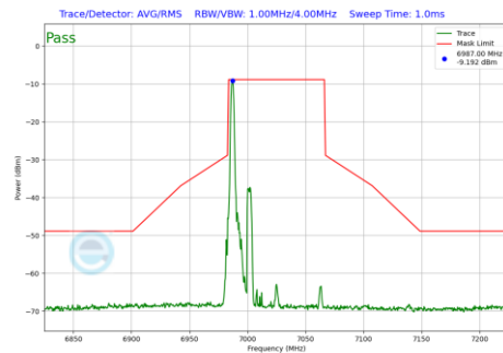
Plot 7-455 In-Band Emission Plot Antenna WF5B (80MHz BW 802.11be(RU) RU26 Index0 (UNII Band 8) - Ch.215)
