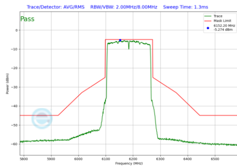
Plot 7-516 In-Band Emission Plot Antenna WF8 (160MHz BW 802.11be(RU) RU996X2 Index68 (UNII Band 5) - Ch.47)
