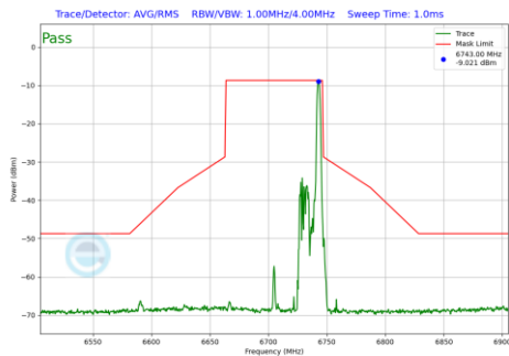
Plot 7-451 In-Band Emission Plot Antenna WF5B (80MHz BW 802.11be(RU) RU26 Index36 (UNII Band 7) - Ch.151)
