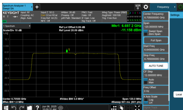
Plot 7-413 PSD SDM Diversity Antenna WF8 (80MHz BW 802.11be(RU) RU996 Index67 - Ch.151)
