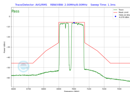
Plot 7-468 In-Band Emission Plot Antenna WF5B (160MHz BW 802.11be(RU) RU996+484+242 Index99 (UNII Band 8) - Ch.207)
