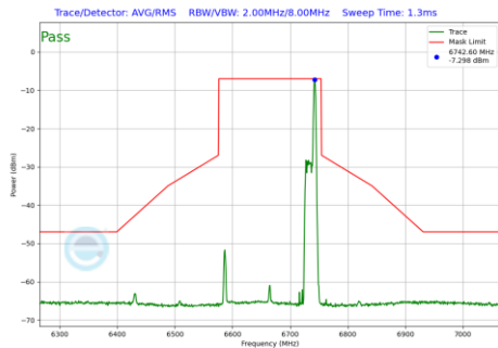
Plot 7-452 In-Band Emission Plot Antenna WF5B (160MHz BW 802.11be(RU) RU26 Index36 (UNII Band 7) - Ch.143)
