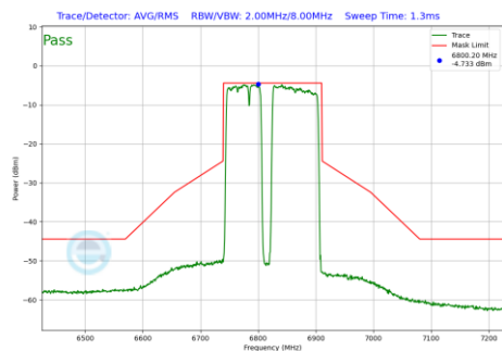
Plot 7-509 In-Band Emission Plot Antenna WF8 (160MHz BW 802.11be(RU) RU996+484+242 Index99 (UNII Band 7) - Ch.175)
