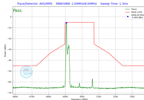
Plot 7-500 In-Band Emission Plot Antenna WF8 (160MHz BW 802.11be(RU) RU26 Index0 (UNII Band 8) - Ch.207)
