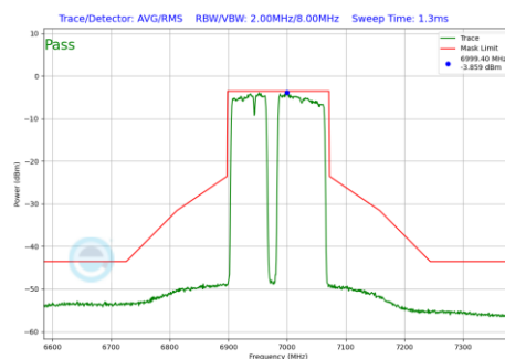
Plot 7-512 In-Band Emission Plot Antenna WF8 (160MHz BW 802.11be(RU) RU996+484+242 Index99 (UNII Band 8) - Ch.207)
