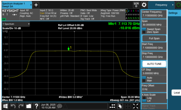
Plot 7-433 PSD SDM Diversity Antenna WF8 (20MHz BW 802.11be(RU) RU242 Index61 - Ch.233)
