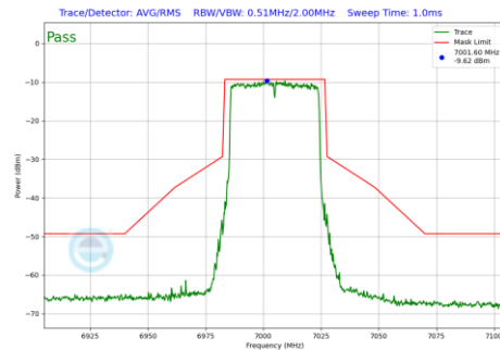
Plot 7-526 In-Band Emission Plot Antenna WF8 (40MHz BW 802.11be(RU) RU484 Index65 (UNII Band 8) - Ch.211)
