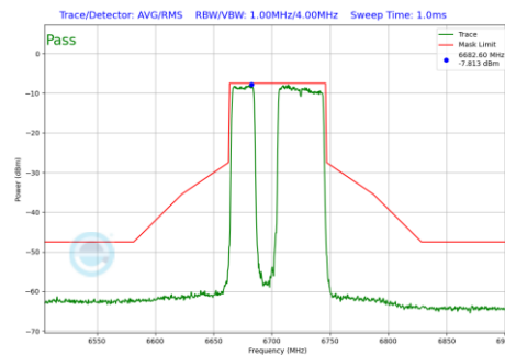
Plot 7-464 In-Band Emission Plot Antenna WF5B (80MHz BW 802.11be(RU) RU484+242 Index91 (UNII Band 7) - Ch.151)
