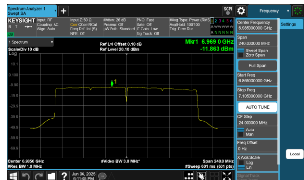
Plot 7-440 PSD SDM Diversity Antenna WF7 (160MHz BW 802.11be(RU) RU996X2 Index68 - Ch.207)
