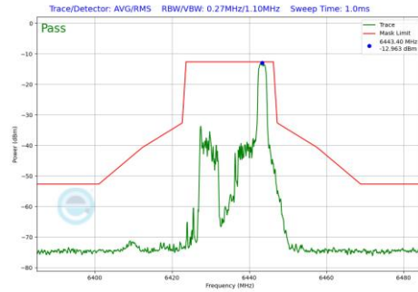
Plot 7-445 In-Band Emission Plot Antenna WF5B (20MHz BW 802.11be(RU) RU26 Index8 (UNII Band 6) - Ch.97)
