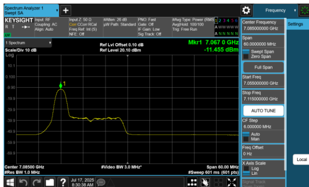
Plot 7-420 PSD SDM Diversity Antenna WF8 (40MHz BW 802.11be(RU) RU26 Index0 - Ch.227)
