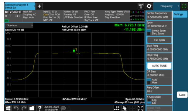
Plot 7-416 PSD SDM Diversity Antenna WF7 (40MHz BW 802.11be(RU) RU484 Index65 - Ch.155)
