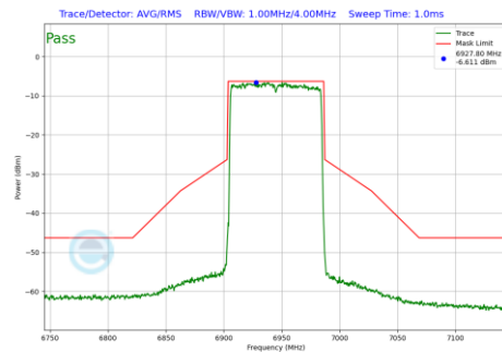
Plot 7-527 In-Band Emission Plot Antenna WF8 (80MHz BW 802.11be(RU) RU996 Index67 (UNII Band 8) - Ch.199)
