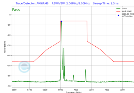
Plot 7-544 In-Band Emission Plot Antenna WF7 (160MHz BW 802.11be(RU) RU26 Index0 (UNII Band 8) - Ch.207)
