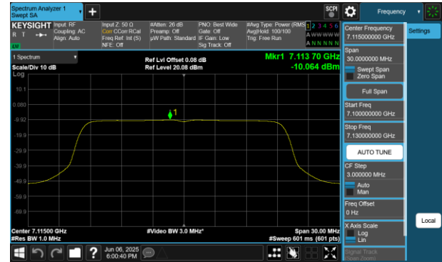
Plot 7-437 PSD SDM Diversity Antenna WF7 (20MHz BW 802.11be(RU) RU242 Index61 - Ch.233)
