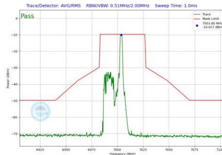
Plot 7-498 In-Band Emission Plot Antenna WF8 (40MHz BW 802.11be(RU) RU26 Index8 (UNII Band 8) - Ch.211)
