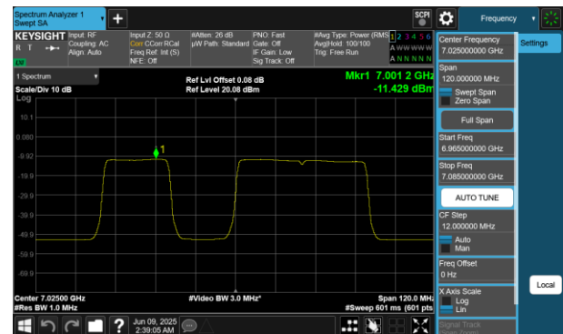
Plot 7-431 PSD SDM Diversity Antenna WF7 (80MHz BW 802.11be(RU) RU484+242 Index91 - Ch.215)
