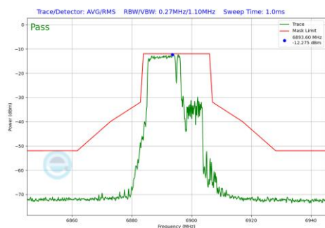
Plot 7-510 In-Band Emission Plot Antenna WF8 (20MHz BW 802.11be(RU) RU106+26 Index82 (UNII Band 8) - Ch.189)
