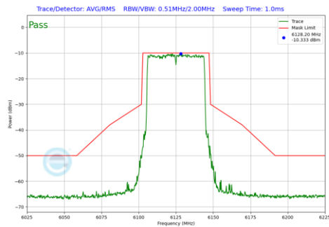
Plot 7-514 In-Band Emission Plot Antenna WF8 (40MHz BW 802.11be(RU) RU484 Index65 (UNII Band 5) - Ch.35)
