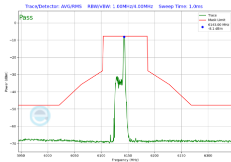
Plot 7-443 In-Band Emission Plot Antenna WF5B (80MHz BW 802.11be(RU) RU26 Index17 (UNII Band 5) - Ch.39)
