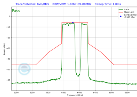
Plot 7-502 In-Band Emission Plot Antenna WF8 (80MHz BW 802.11be(RU) RU484+242 Index92 (UNII Band 5) - Ch.87)
