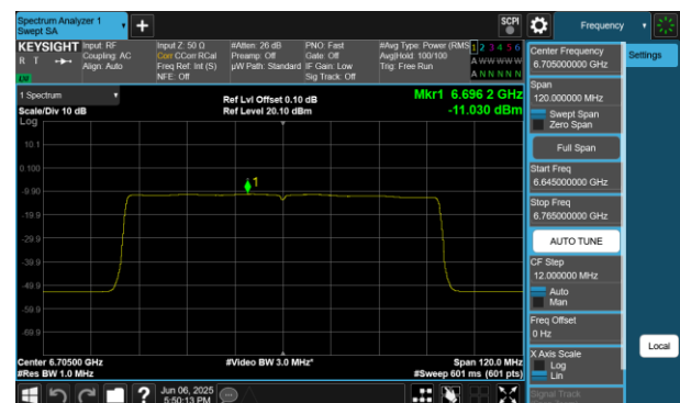
Plot 7-417 PSD SDM Diversity Antenna WF7 (80MHz BW 802.11be(RU) RU996 Index67 - Ch.151)
