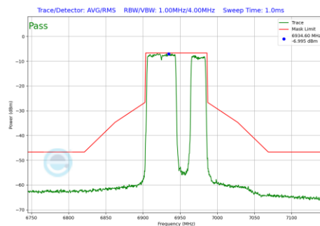
Plot 7-511 In-Band Emission Plot Antenna WF8 (80MHz BW 802.11be(RU) RU484+242 Index92 (UNII Band 8) - Ch.199)
