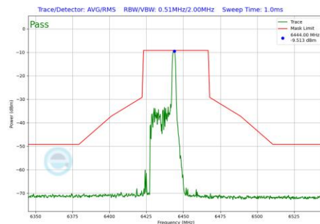
Plot 7-490 In-Band Emission Plot Antenna WF8 (40MHz BW 802.11be(RU) RU26 Index8 (UNII Band 6) - Ch.99)
