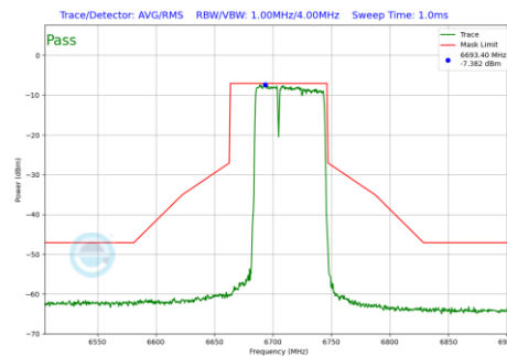
Plot 7-508 In-Band Emission Plot Antenna WF8 (80MHz BW 802.11be(RU) RU484+242 Index90 (UNII Band 7) - Ch.151)
