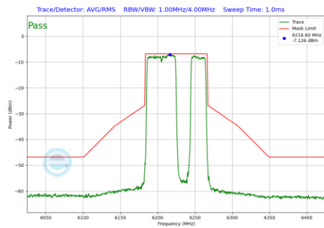
Plot 7-458 In-Band Emission Plot Antenna WF5B (80MHz BW 802.11be(RU) RU484+242 Index92 (UNII Band 5) - Ch.55)
