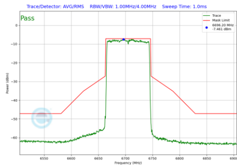
Plot 7-523 In-Band Emission Plot Antenna WF8 (80MHz BW 802.11be(RU) RU996 Index67 (UNII Band 7) - Ch.151)
