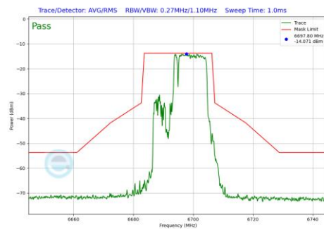
Plot 7-463 In-Band Emission Plot Antenna WF5B (20MHz BW 802.11be(RU) RU106+26 Index83 (UNII Band 7) - Ch.149)
