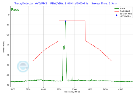
Plot 7-444 In-Band Emission Plot Antenna WF5B (160MHz BW 802.11be(RU) RU26 Index17 (UNII Band 5) - Ch.47)
