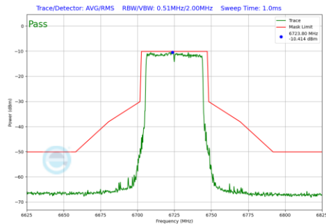
Plot 7-522 In-Band Emission Plot Antenna WF8 (40MHz BW 802.11be(RU) RU484 Index65 (UNII Band 7) - Ch.155)
