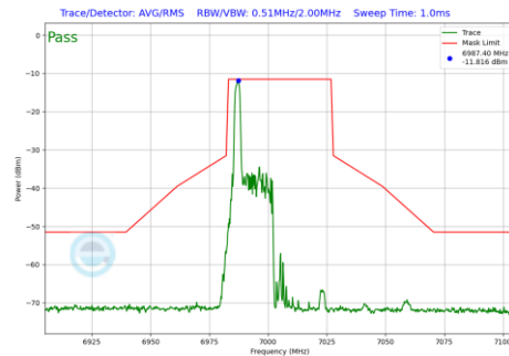
Plot 7-454 In-Band Emission Plot Antenna WF5B (40MHz BW 802.11be(RU) RU26 Index0 (UNII Band 8) - Ch.211)
