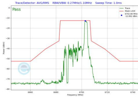
Plot 7-537 In-Band Emission Plot Antenna WF7 (20MHz BW 802.11be(RU) RU26 Index8 (UNII Band 7) - Ch.149)
