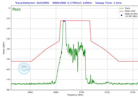
Plot 7-493 In-Band Emission Plot Antenna WF8 (20MHz BW 802.11be(RU) RU26 Index0 (UNII Band 7) - Ch.149)
