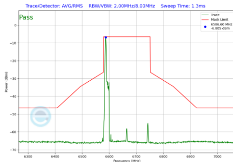
Plot 7-540 In-Band Emission Plot Antenna WF7 (160MHz BW 802.11be(RU) RU26 Index0 (UNII Band 7) - Ch.143)
