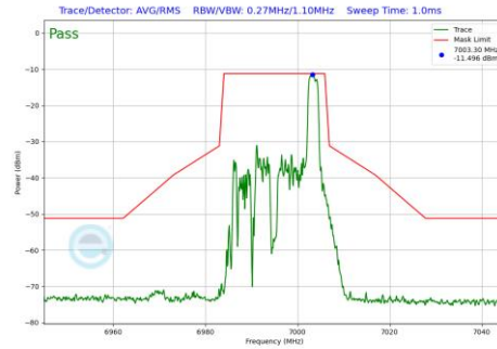
Plot 7-497 In-Band Emission Plot Antenna WF8 (20MHz BW 802.11be(RU) RU26 Index8 (UNII Band 8) - Ch.209)
