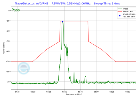
Plot 7-494 In-Band Emission Plot Antenna WF8 (40MHz BW 802.11be(RU) RU26 Index0 (UNII Band 7) - Ch.123)
