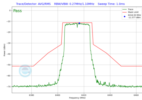
Plot 7-513 In-Band Emission Plot Antenna WF8 (20MHz BW 802.11be(RU) RU242 Index61 (UNII Band 5) - Ch.93)
