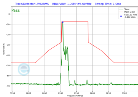
Plot 7-531 In-Band Emission Plot Antenna WF7 (80MHz BW 802.11be(RU) RU26 Index0 (UNII Band 5) - Ch.39)
