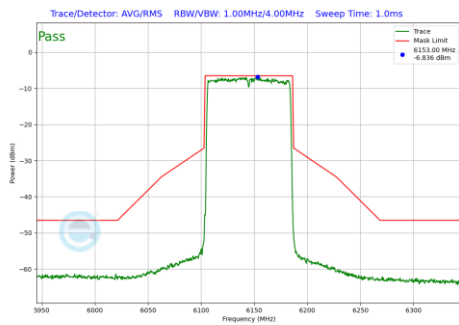
Plot 7-471 In-Band Emission Plot Antenna WF5B (80MHz BW 802.11be(RU) RU996 Index67 (UNII Band 5) - Ch.39)
