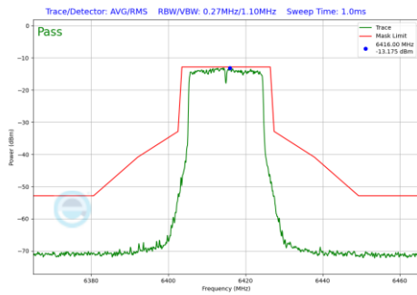
Plot 7-469 In-Band Emission Plot Antenna WF5B (20MHz BW 802.11be(RU) RU242 Index61 (UNII Band 5) - Ch.93)
