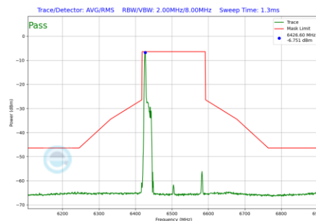
Plot 7-492 In-Band Emission Plot Antenna WF8 (160MHz BW 802.11be(RU) RU26 Index0 (UNII Band 6) - Ch.111)
