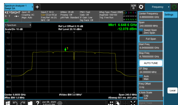
Plot 7-418 PSD SDM Diversity Antenna WF7 (160MHz BW 802.11be(RU) RU996X2 Index68 - Ch.143)
