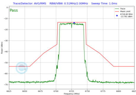
Plot 7-742 In-Band Emission Plot CDD Diversity Antenna WF8 (40MHz BW 802.11be(RU) RU484 Index65 (UNII Band 7) - Ch.155)
