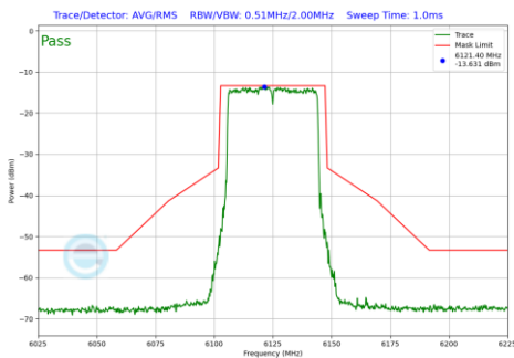
Plot 7-734 In-Band Emission Plot CDD Diversity Antenna WF8 (40MHz BW 802.11be(RU) RU484 Index65 (UNII Band 5) - Ch.35)
