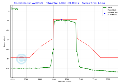
Plot 7-748 In-Band Emission Plot CDD Diversity Antenna WF8 (160MHz BW 802.11be(RU) RU996X2 Index68 (UNII Band 8) - Ch.207)
