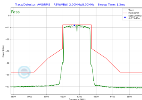
Plot 7-736 In-Band Emission Plot CDD Diversity Antenna WF8 (160MHz BW 802.11be(RU) RU996X2 Index68 (UNII Band 5) - Ch.47)
