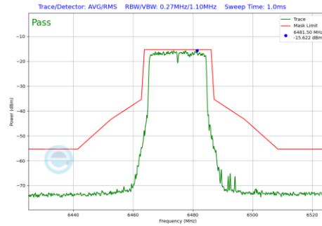
Plot 7-737 In-Band Emission Plot CDD Diversity Antenna WF8 (20MHz BW 802.11be(RU) RU242 Index61 (UNII Band 6) - Ch.105)
