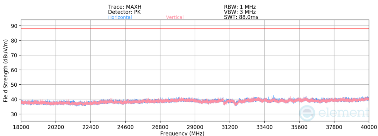
Plot 7-794. Radiated Spurious Emissions 18-40GHz SDM Primary (802.11be – Ch. 149 – RU26)
