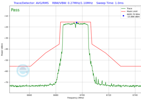
Plot 7-741 In-Band Emission Plot CDD Diversity Antenna WF8 (20MHz BW 802.11be(RU) RU242 Index61 (UNII Band 7) - Ch.149)
