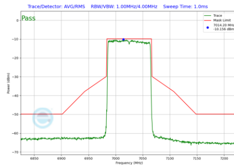
Plot 7-747 In-Band Emission Plot CDD Diversity Antenna WF8 (80MHz BW 802.11be(RU) RU996 Index67 (UNII Band 8) - Ch.215)
