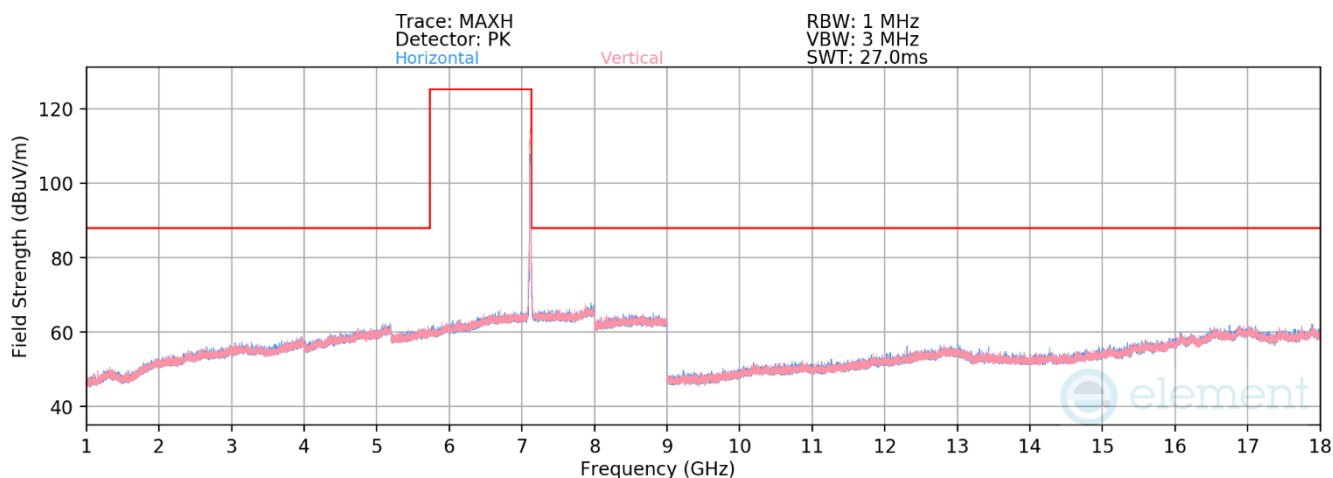
Plot 7-815. Radiated Spurious Emissions above 1GHz SDM Primary (802.11be – Ch. 229 – RU242)
