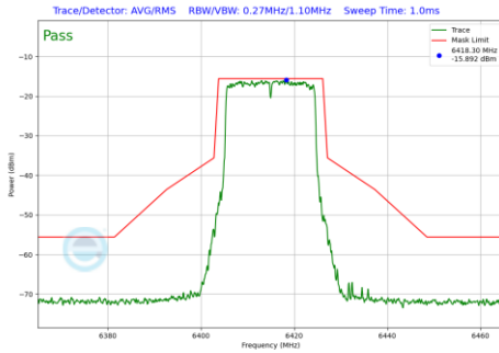
Plot 7-733 In-Band Emission Plot CDD Diversity Antenna WF8 (20MHz BW 802.11be(RU) RU242 Index61 (UNII Band 5) - Ch.93)
