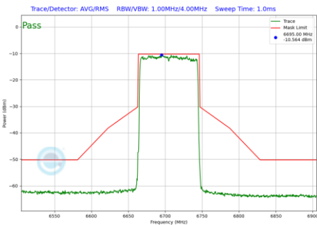
Plot 7-743 In-Band Emission Plot CDD Diversity Antenna WF8 (80MHz BW 802.11be(RU) RU996 Index67 (UNII Band 7) - Ch.151)
