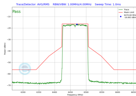
Plot 7-739 In-Band Emission Plot CDD Diversity Antenna WF8 (80MHz BW 802.11be(RU) RU996 Index67 (UNII Band 6) - Ch.103)
