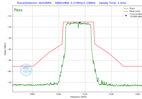
Plot 7-745 In-Band Emission Plot CDD Diversity Antenna WF8 (20MHz BW 802.11be(RU) RU242 Index61 (UNII Band 8) - Ch.233)
