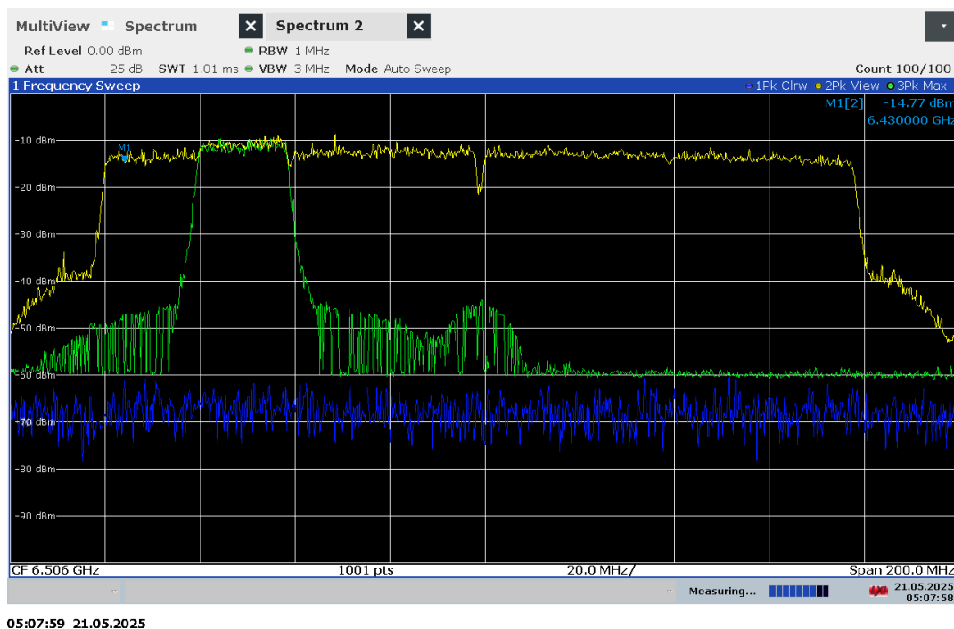
Plot 7-781. 160MHz Bandwidth, AWGN Signal Injected – 6430MHz
