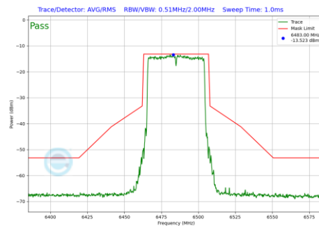
Plot 7-738 In-Band Emission Plot CDD Diversity Antenna WF8 (40MHz BW 802.11be(RU) RU484 Index65 (UNII Band 6) - Ch.107)
