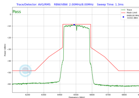
Plot 7-740 In-Band Emission Plot CDD Diversity Antenna WF8 (160MHz BW 802.11be(RU) RU996X2 Index68 (UNII Band 6) - Ch.111)
