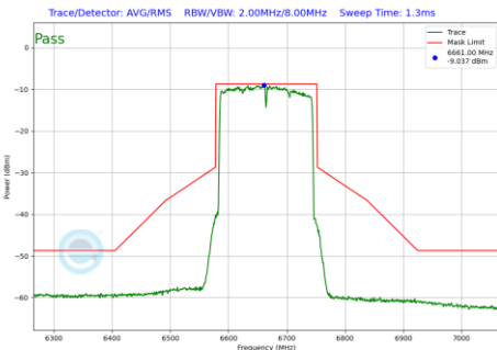
Plot 7-744 In-Band Emission Plot CDD Diversity Antenna WF8 (160MHz BW 802.11be(RU) RU996X2 Index68 (UNII Band 7) - Ch.143)
