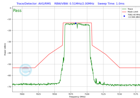
Plot 7-746 In-Band Emission Plot CDD Diversity Antenna WF8 (40MHz BW 802.11be(RU) RU484 Index65 (UNII Band 8) - Ch.227)
