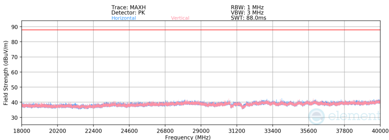
Plot 7-798. Radiated Spurious Emissions 18-40GHz SDM Primary (802.11be – Ch. 209 – RU26)
