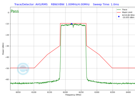
Plot 7-735 In-Band Emission Plot CDD Diversity Antenna WF8 (80MHz BW 802.11be(RU) RU996 Index67 (UNII Band 5) - Ch.55)
