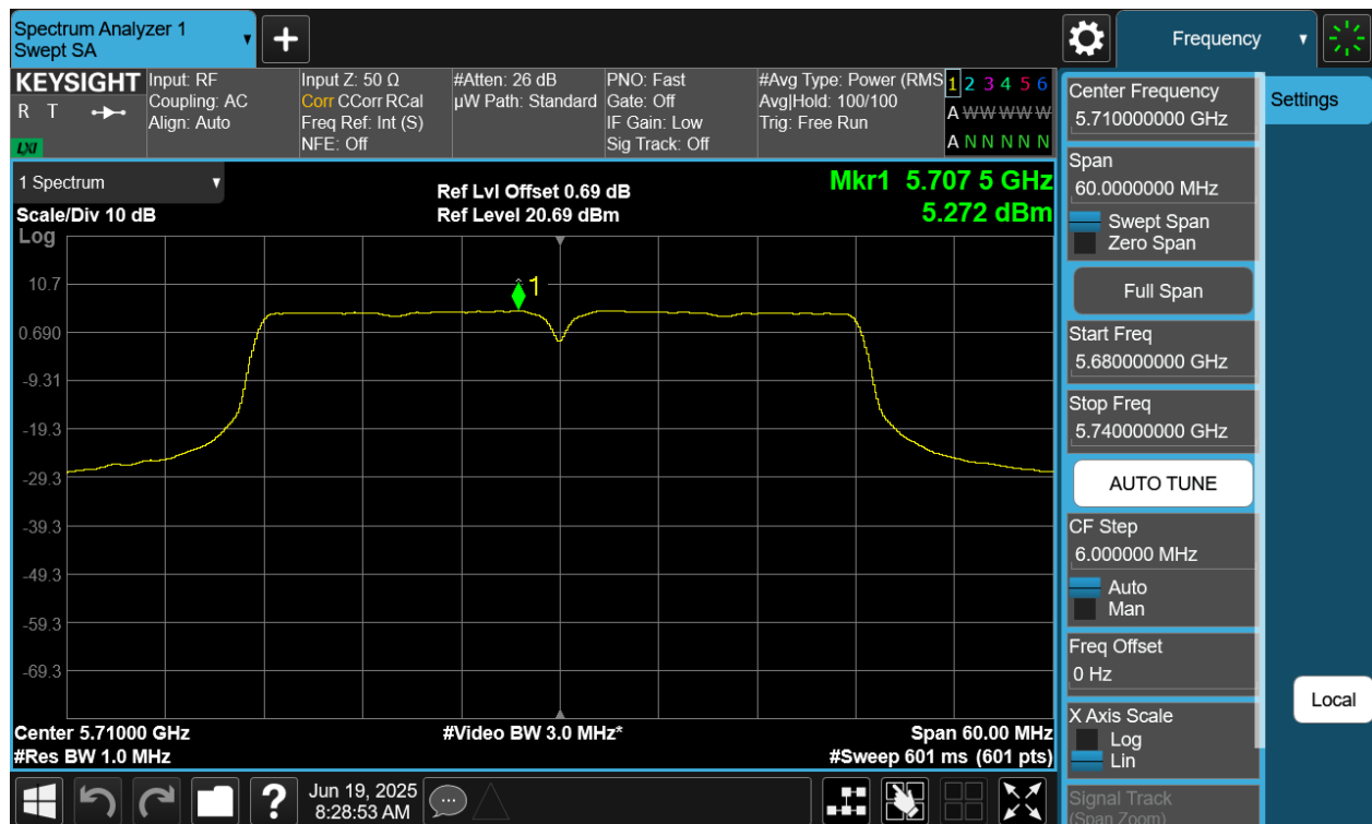
Plot 7-56 PSD CDD Primary Antenna WF5B (40MHz BW 802.11n - Ch.142)
