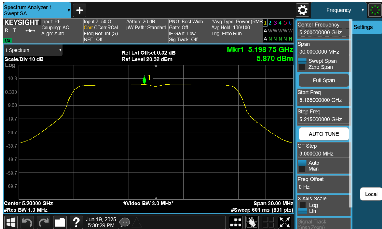
Plot 7-59 PSD CDD Primary Antenna WF8 (20MHz BW 802.11a - Ch.40)
