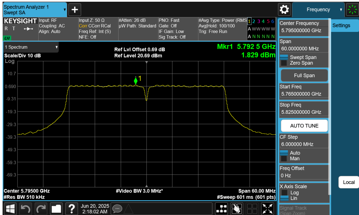
Plot 7-67 PSD CDD Primary Antenna WF8 (40MHz BW 802.11n - Ch.159)
