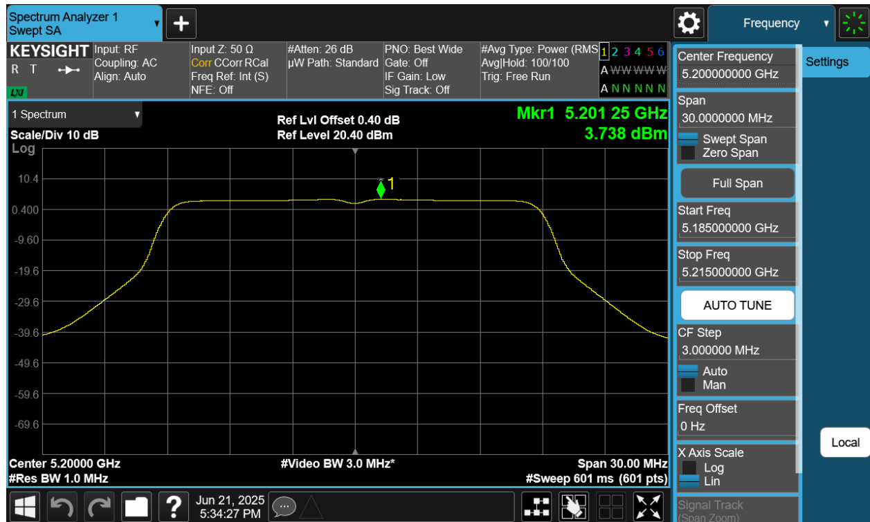
Plot 7-73 PSD CDD Primary Antenna WF8 (20MHz BW 802.11n - Ch.40)
