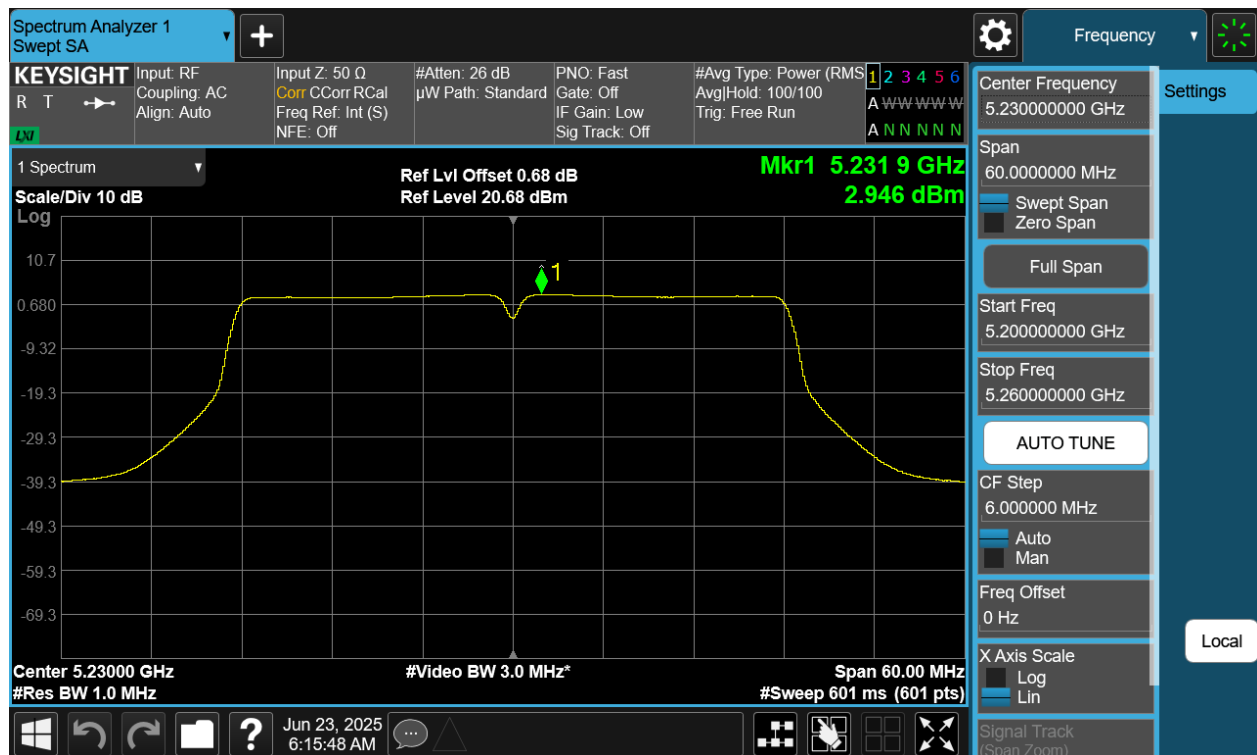
Plot 7-96 PSD CDD Diversity Antenna WF7 (40MHz BW 802.11n - Ch.46)
