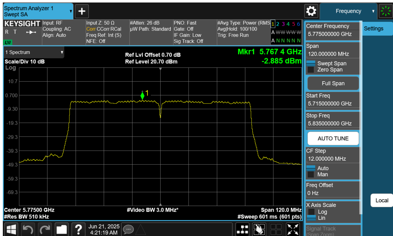
Plot 7-90 PSD CDD Diversity Antenna WF7 (80MHz BW 802.11ac - Ch.155)
