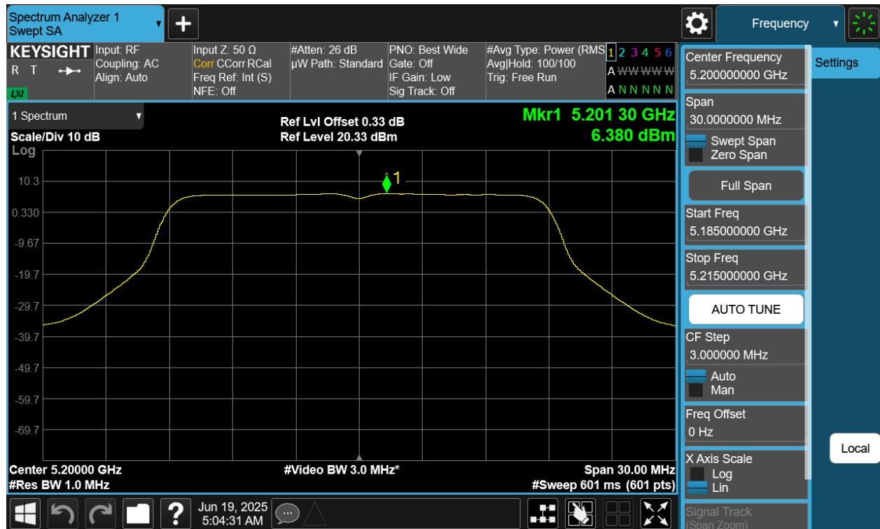
Plot 7-55 PSD CDD Primary Antenna WF5B (20MHz BW 802.11a - Ch.40)
