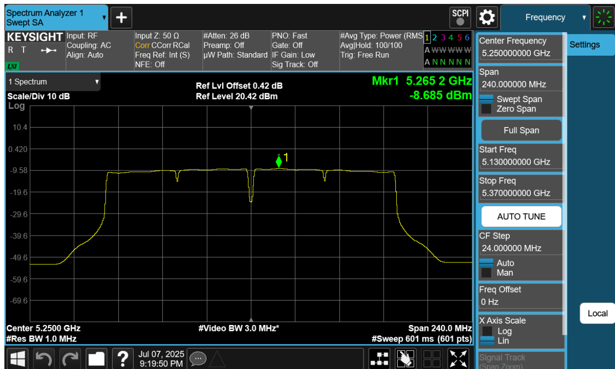
Plot 7-72 PSD CDD Primary Antenna WF5B (160MHz BW 802.11ac - Ch.50)
