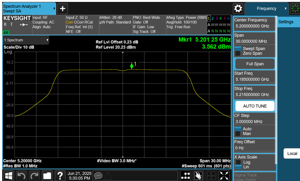
Plot 7-91 PSD CDD Diversity Antenna WF8 (20MHz BW 802.11n - Ch.40)
