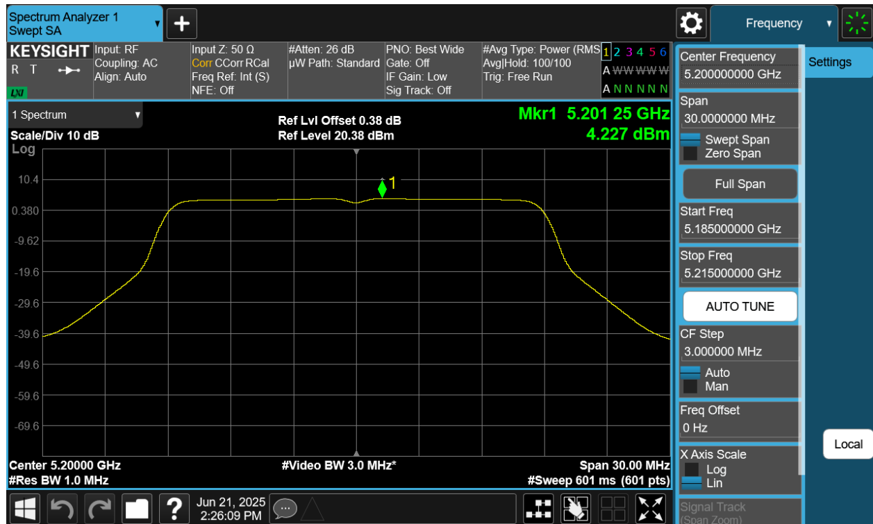
Plot 7-69 PSD CDD Primary Antenna WF5B (20MHz BW 802.11n - Ch.40)
