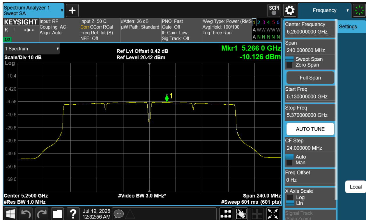
Plot 7-76 PSD CDD Primary Antenna WF8 (160MHz BW 802.11ac - Ch.50)
