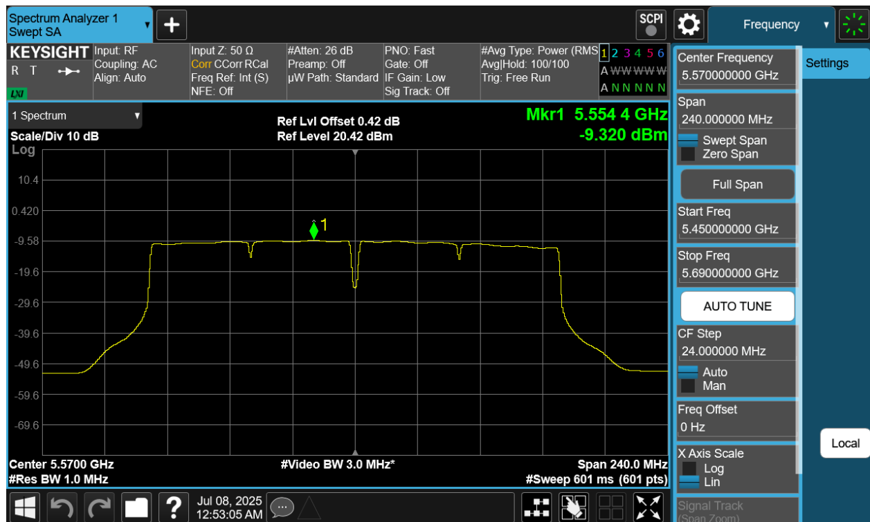
Plot 7-62 PSD CDD Primary Antenna WF8 (160MHz BW 802.11ac - Ch.114)
