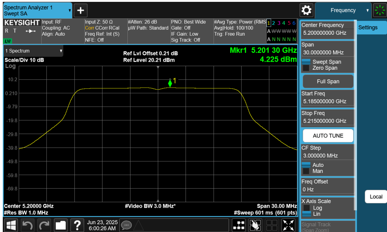
Plot 7-95 PSD CDD Diversity Antenna WF7 (20MHz BW 802.11n - Ch.40)
