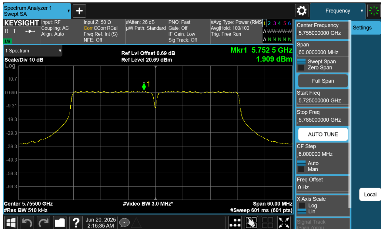
Plot 7-86 PSD CDD Diversity Antenna WF8 (40MHz BW 802.11n - Ch.151)
