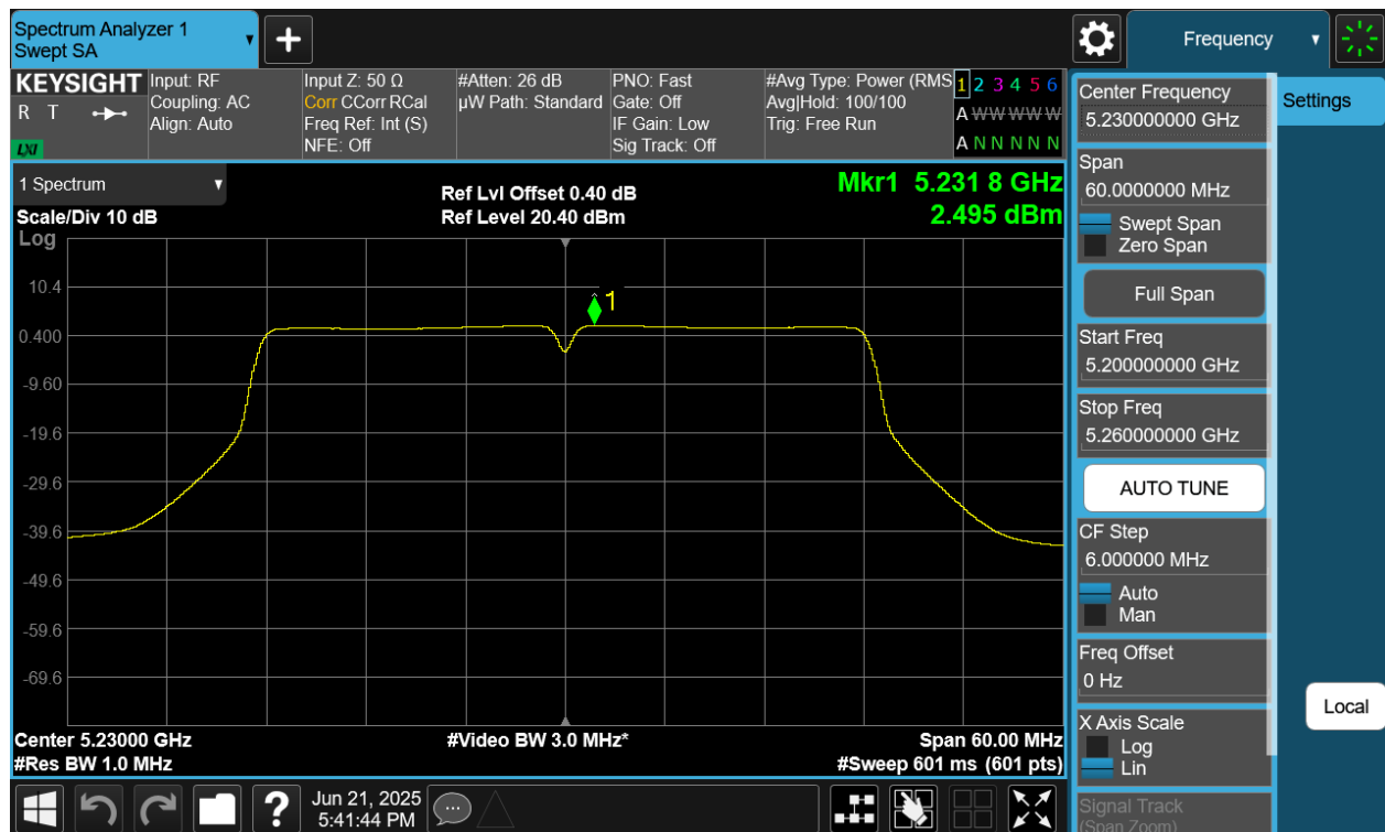
Plot 7-74 PSD CDD Primary Antenna WF8 (40MHz BW 802.11n - Ch.46)
