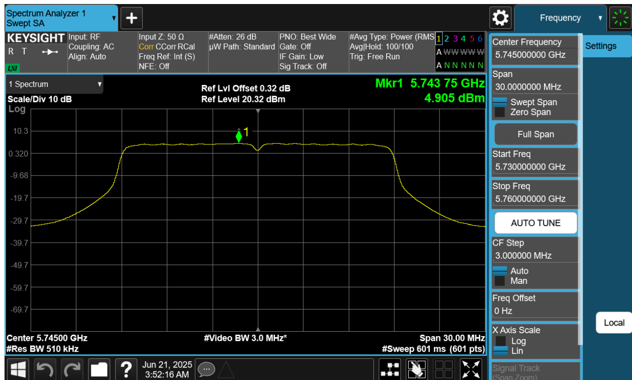
Plot 7-88 PSD CDD Diversity Antenna WF7 (20MHz BW 802.11a - Ch.149)
