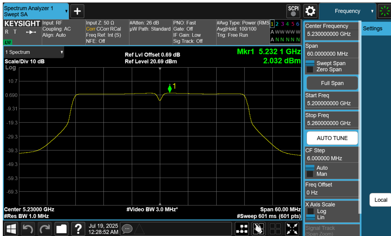
Plot 7-92 PSD CDD Diversity Antenna WF8 (40MHz BW 802.11n - Ch.46)
