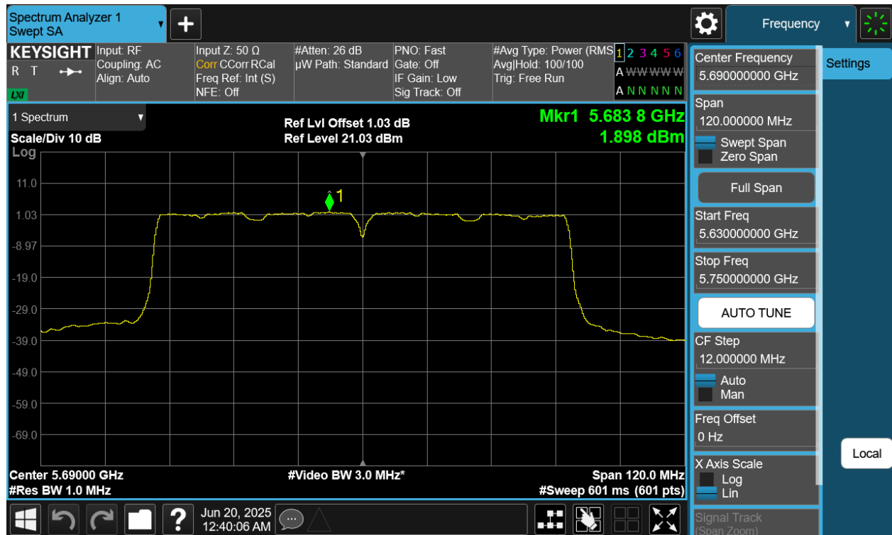
Plot 7-61 PSD CDD Primary Antenna WF8 (80MHz BW 802.11ac - Ch.138)
