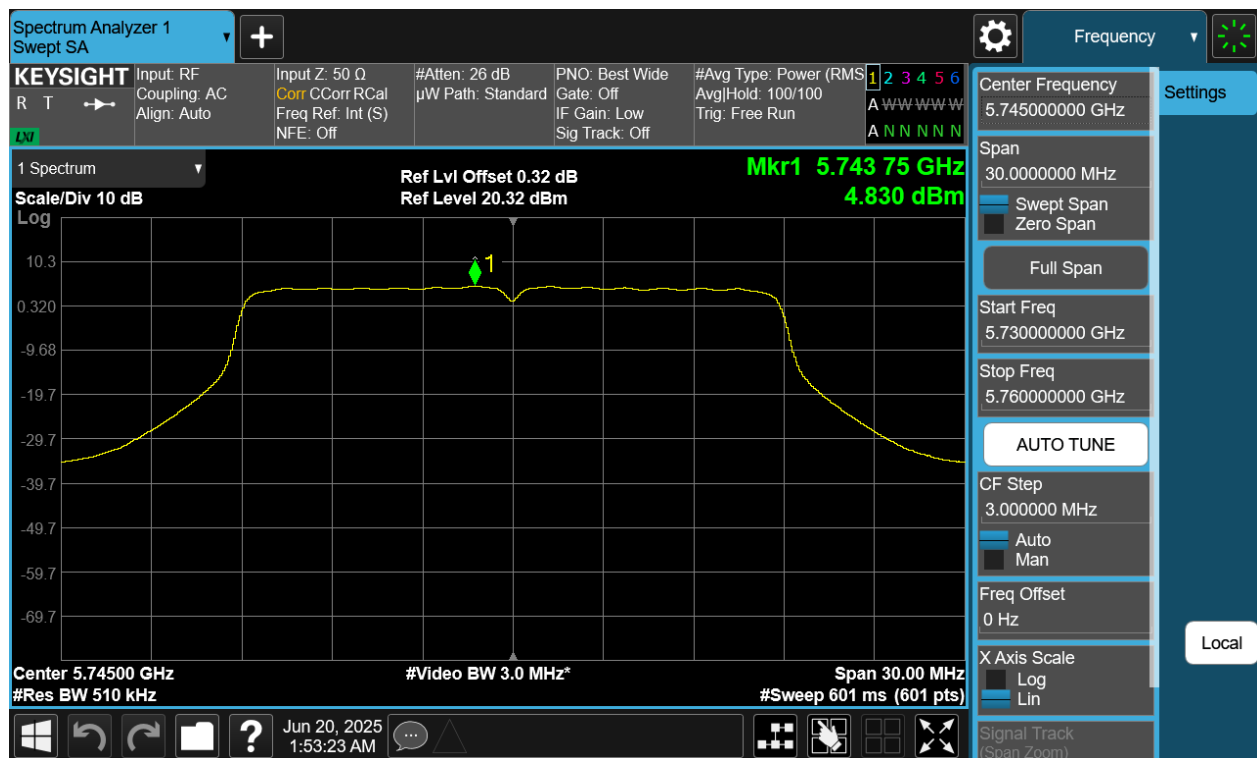
Plot 7-66 PSD CDD Primary Antenna WF8 (20MHz BW 802.11a - Ch.149)
