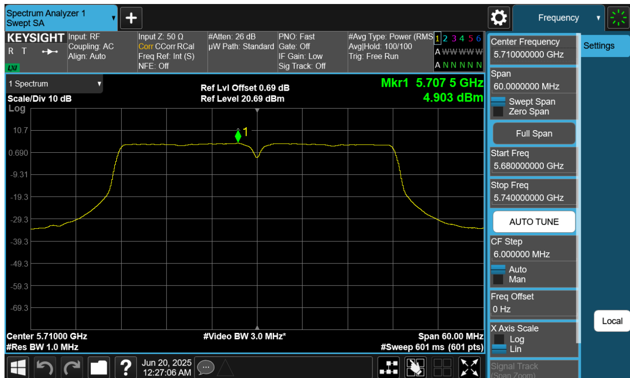
Plot 7-60 PSD CDD Primary Antenna WF8 (40MHz BW 802.11n - Ch.142)
