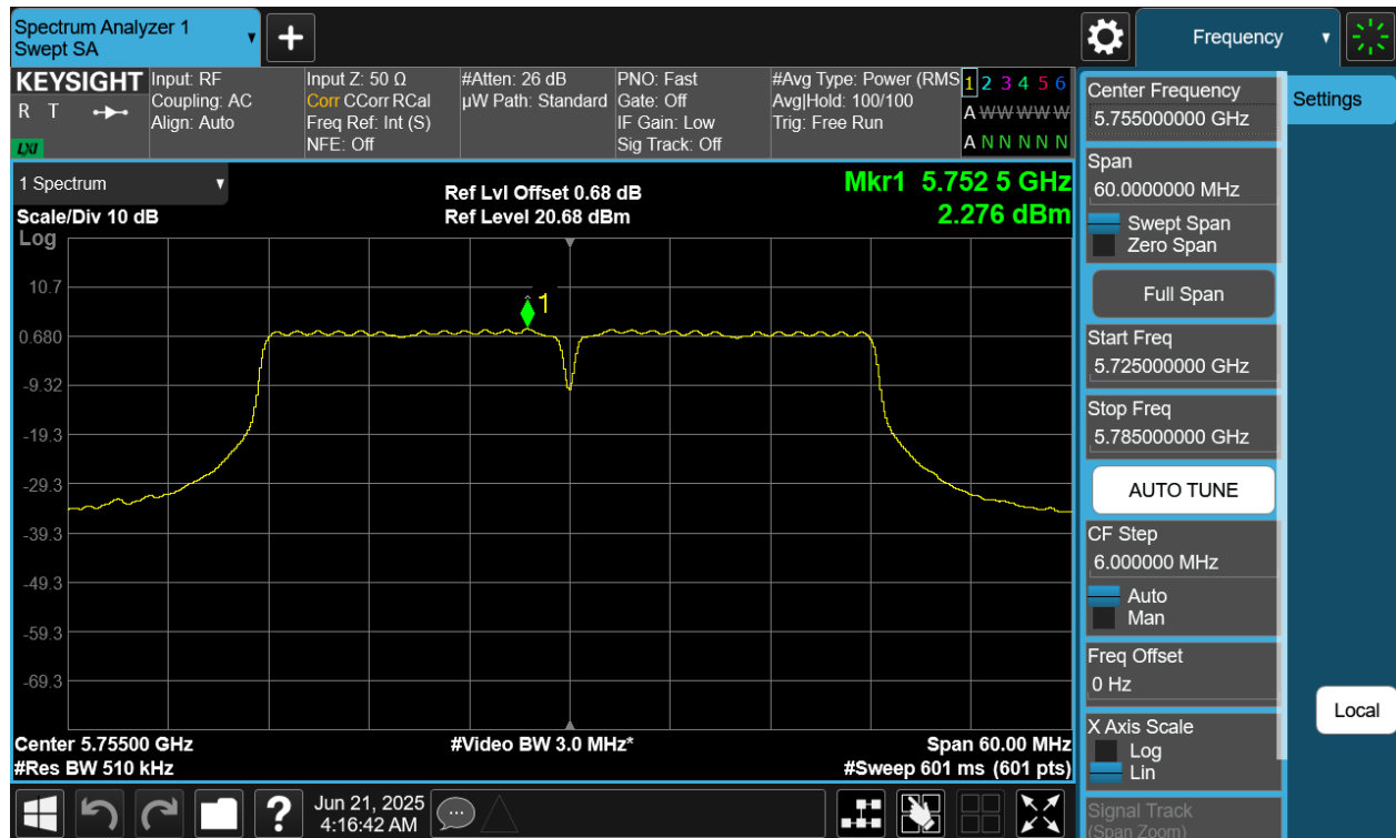
Plot 7-89 PSD CDD Diversity Antenna WF7 (40MHz BW 802.11n - Ch.151)
