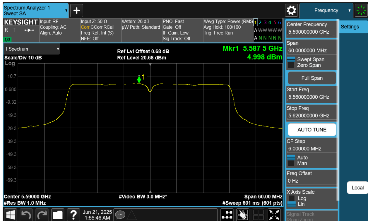
Plot 7-82 PSD CDD Diversity Antenna WF7 (40MHz BW 802.11n - Ch.118)
