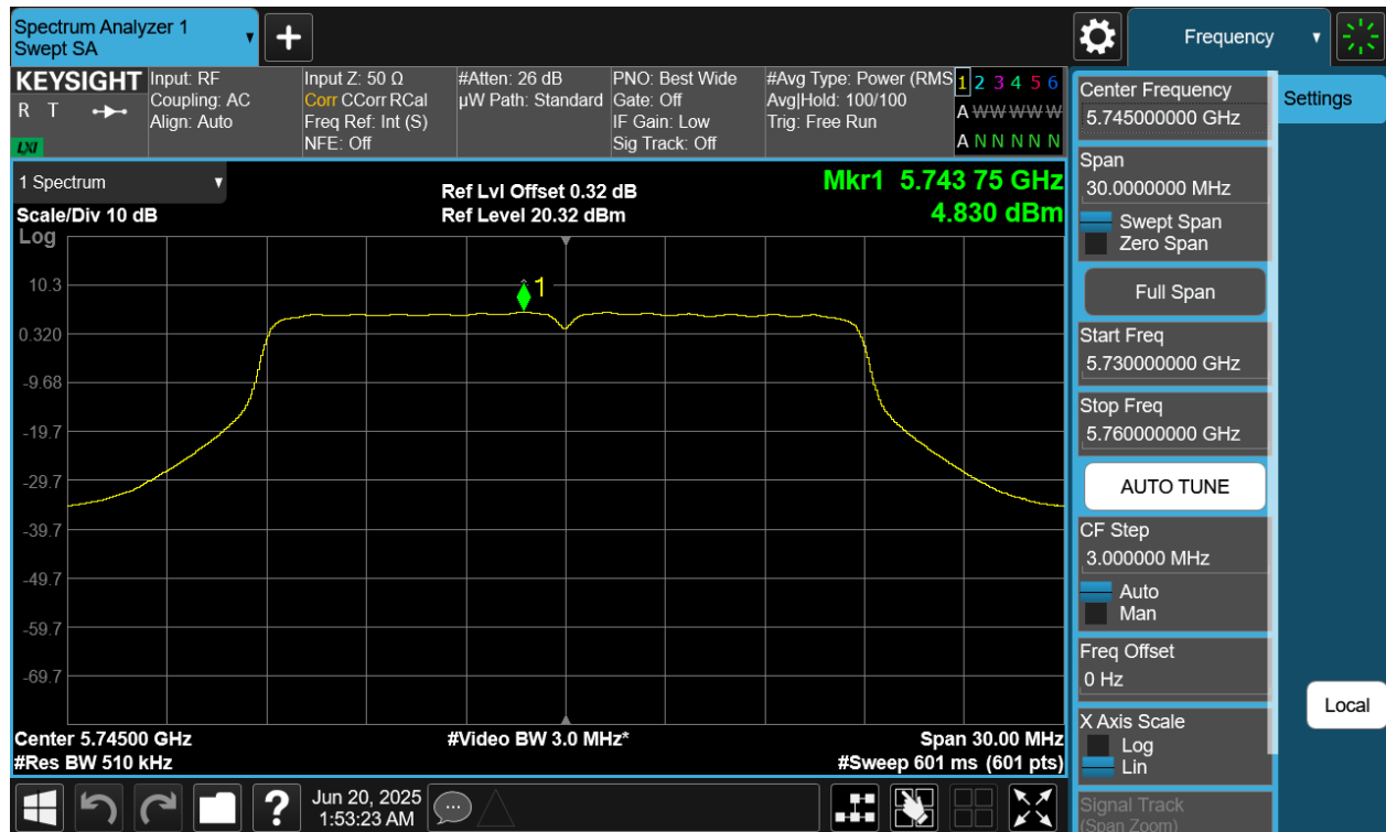
Plot 7-85 PSD CDD Diversity Antenna WF8 (20MHz BW 802.11a - Ch.149)
