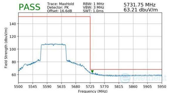
Plot 7-347. Antenna WF7 (Peak, Ch.122 (FCC ONLY), 802.11ac, MCS9)
