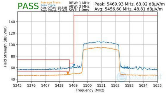
Plot 7-216. Antenna WF5B (Peak & Average, Ch.106, 802.11be(SU), MCS11)
