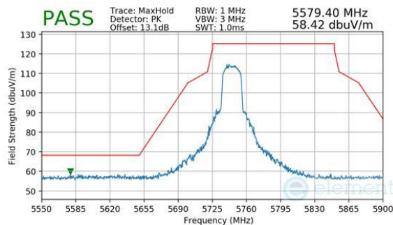
Plot 7-249. Antenna WF8 (Peak, Ch.149, 802.11be(SU), MCS11)
