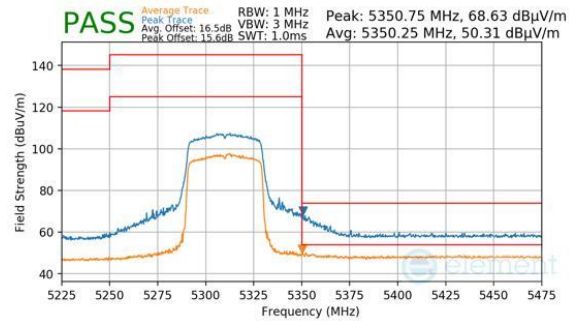
Plot 7-334. Antenna WF7 (Peak & Average, Ch.62, 802.11be(SU), MCS11)
