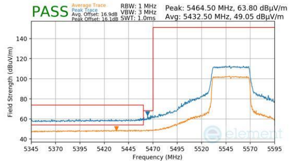
Plot 7-336. Antenna WF7 (Peak & Average, Ch.110, 802.11be(SU), MCS11)
