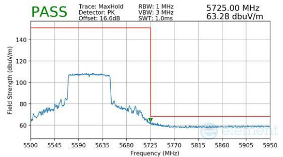
Plot 7-354. Antenna WF7 (Peak, Ch.122 (FCC ONLY), 802.11be(SU), MCS11)
