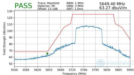
Plot 7-355. Antenna WF7 (Peak, Ch.155, 802.11be(SU), MCS11)
