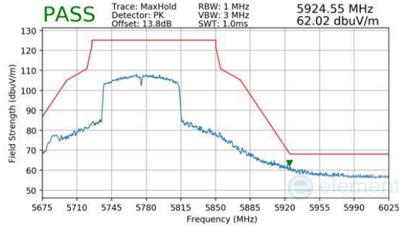
Plot 7-213. Antenna WF5B (Peak, Ch.155, 802.11ac, MCS9)
