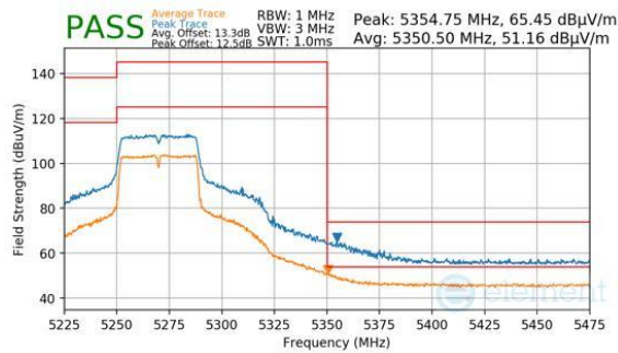
Plot 7-187. Antenna WF5B (Peak & Average, Ch.54, 802.11n, MCS7)
