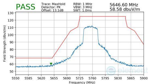
Plot 7-205. Antenna WF5B (Peak, Ch.151, 802.11be(SU), MCS11)
