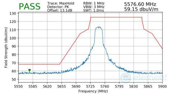
Plot 7-238. Antenna WF8 (Peak, Ch.149, 802.11n, MCS7)
