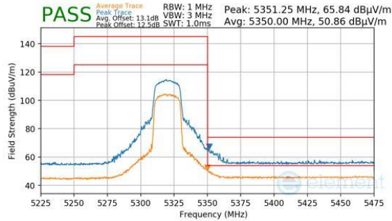
Plot 7-243. Antenna WF8 (Peak & Average, Ch.64, 802.11be(SU), MCS11)
