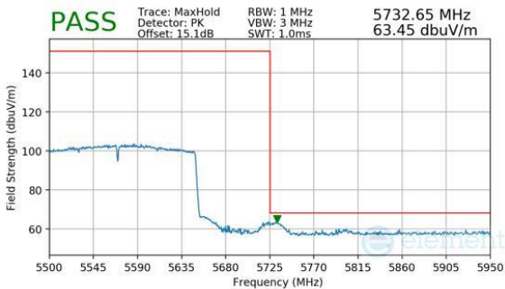
Plot 7-228. Antenna WF5B (Peak, Ch.114 (FCC ONLY), 802.11be(SU), MCS11)
