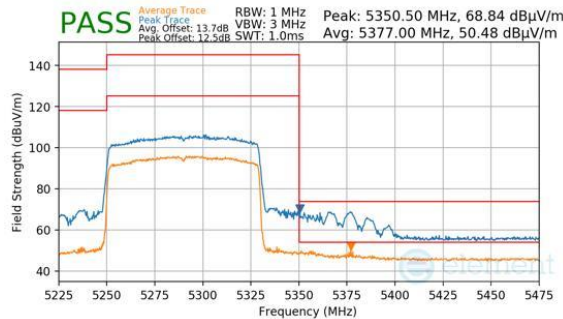
Plot 7-215. Antenna WF5B (Peak & Average, Ch.58, 802.11be(SU), MCS11)
