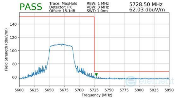
Plot 7-272. Antenna WF8 (Peak, Ch.134, 802.11be(SU), MCS11)
