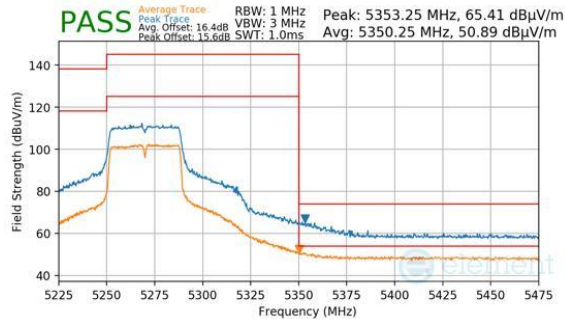
Plot 7-321. Antenna WF7 (Peak & Average, Ch.54, 802.11n, MCS7)
