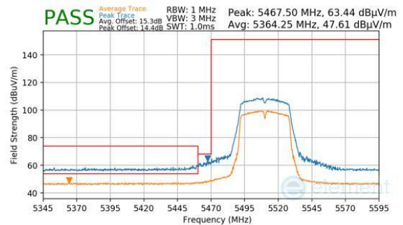
Plot 7-189. Antenna WF5B (Peak & Average, Ch.102, 802.11n, MCS7)
