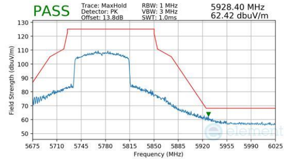
Plot 7-220. Antenna WF5B (Peak, Ch.155, 802.11be(SU), MCS11)
