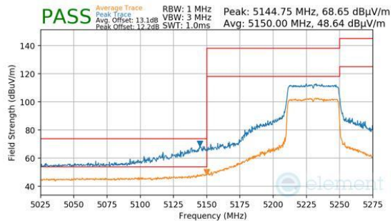
Plot 7-264. Antenna WF8 (Peak & Average, Ch.46, 802.11be(SU), MCS11)
