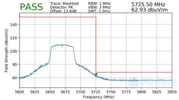
Plot 7-328. Antenna WF7 (Peak, Ch.134, 802.11n, MCS7)
