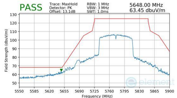
Plot 7-348. Antenna WF7 (Peak, Ch.155, 802.11ac, MCS9)
