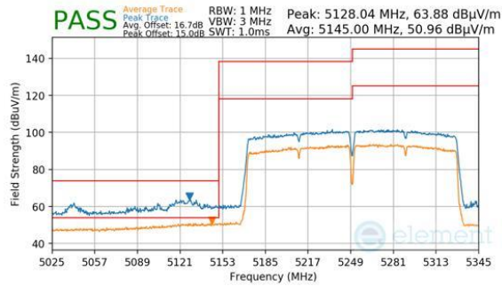
Plot 7-221. Antenna WF5B (Peak & Average, Ch.50, 802.11ac, MCS9)
