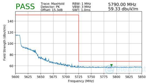
Plot 7-270. Antenna WF8 (Peak, Ch.118 (FCC ONLY), 802.11be(SU), MCS11)
