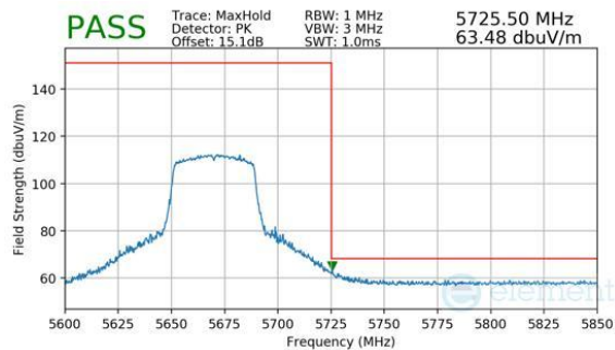
Plot 7-204. Antenna WF5B (Peak, Ch.134, 802.11be(SU), MCS11)
