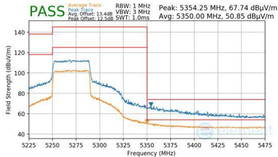
Plot 7-265. Antenna WF8 (Peak & Average, Ch.54, 802.11be(SU), MCS11)
