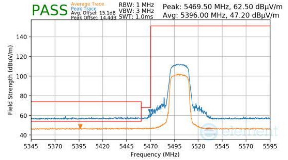
Plot 7-244. Antenna WF8 (Peak & Average, Ch.100, 802.11be(SU), MCS11)
