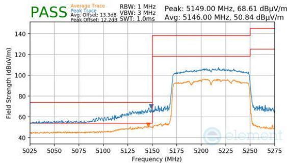
Plot 7-214. Antenna WF5B (Peak & Average, Ch.42, 802.11be(SU), MCS11)
