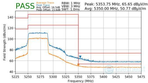
Plot 7-333. Antenna WF7 (Peak & Average, Ch.54, 802.11be(SU), MCS11)
