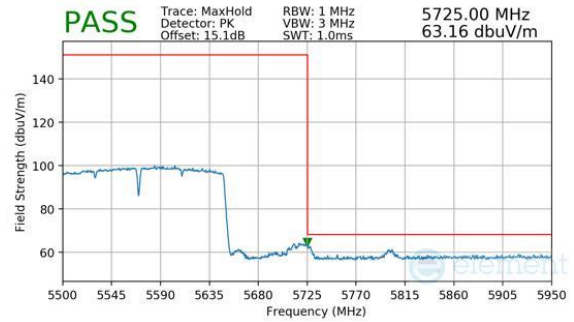
Plot 7-224. Antenna WF5B (Peak, Ch.114 (FCC ONLY), 802.11ac, MCS9)
