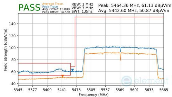
Plot 7-227. Antenna WF5B (Peak & Average, Ch.114 (FCC ONLY), 802.11be(SU), MCS11)
