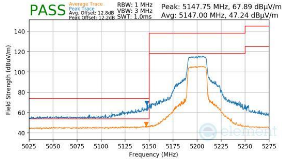
Plot 7-241. Antenna WF8 (Peak & Average, Ch.40, 802.11be(SU), MCS11)
