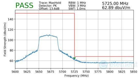
Plot 7-340. Antenna WF7 (Peak, Ch.134, 802.11be(SU), MCS11)
