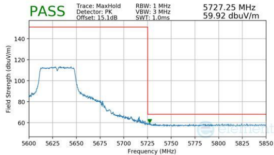
Plot 7-192. Antenna WF5B (Peak, Ch.126 (FCC ONLY), 802.11n, MCS7)
