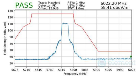
Plot 7-318. Antenna WF7 (Peak, Ch.165, 802.11be(SU), MCS11)
