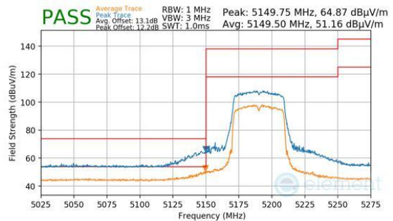
Plot 7-196. Antenna WF5B (Peak & Average, Ch.38, 802.11be(SU), MCS11)
