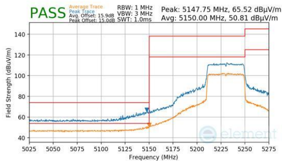
Plot 7-332. Antenna WF7 (Peak & Average, Ch.46, 802.11be(SU), MCS11)
