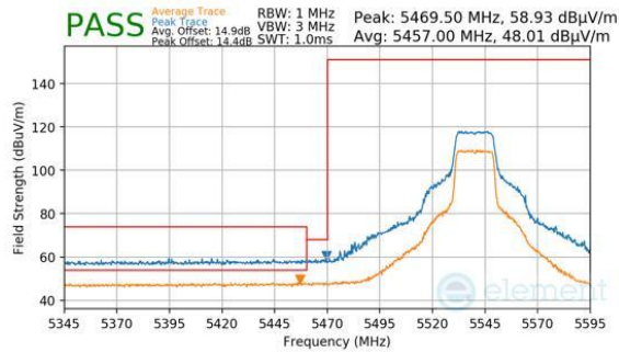
Plot 7-235. Antenna WF8 (Peak & Average, Ch.108, 802.11n, MCS7)
