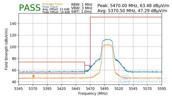
Plot 7-233. Antenna WF8 (Peak & Average, Ch.100, 802.11n, MCS7)
