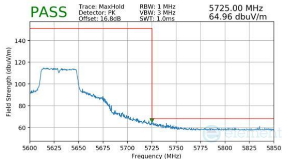
Plot 7-259. Antenna WF8 (Peak, Ch.126 (FCC ONLY), 802.11n, MCS7)
