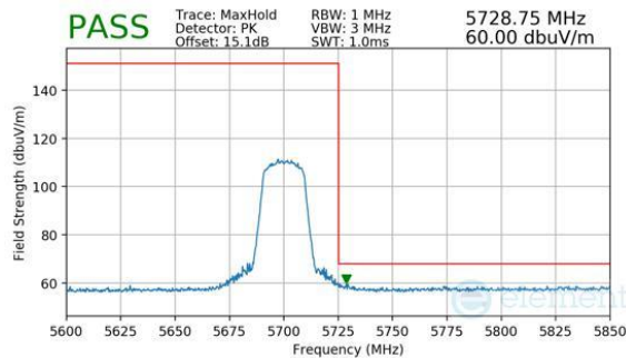
Plot 7-248. Antenna WF8 (Peak, Ch.140, 802.11be(SU), MCS11)
