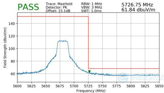
Plot 7-236. Antenna WF8 (Peak, Ch.136, 802.11n, MCS7)
