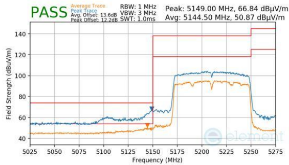
Plot 7-207. Antenna WF5B (Peak & Average, Ch.42, 802.11ac, MCS9)
