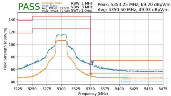
Plot 7-231. Antenna WF8 (Peak & Average, Ch.60, 802.11n, MCS7)
