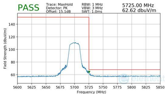
Plot 7-237. Antenna WF8 (Peak, Ch.140, 802.11n, MCS7)
