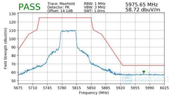
Plot 7-195. Antenna WF5B (Peak, Ch.159, 802.11n, MCS7)
