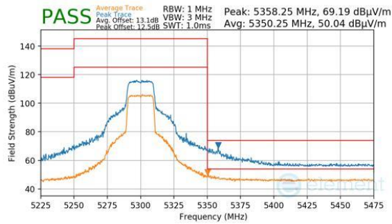
Plot 7-242. Antenna WF8 (Peak & Average, Ch.60, 802.11be(SU), MCS11)
