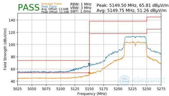
Plot 7-186. Antenna WF5B (Peak & Average, Ch.46, 802.11n, MCS7)
