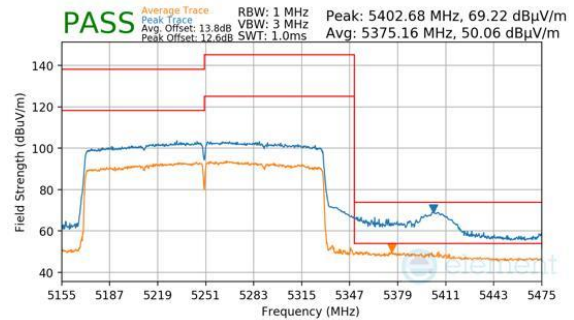
Plot 7-226. Antenna WF5B (Peak & Average, Ch.50, 802.11be(SU), MCS11)
