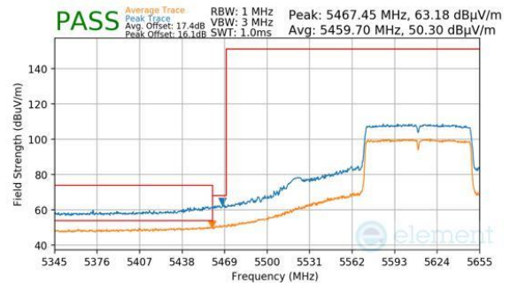
Plot 7-346. Antenna WF7 (Peak & Average, Ch.122 (FCC ONLY), 802.11ac, MCS9)
