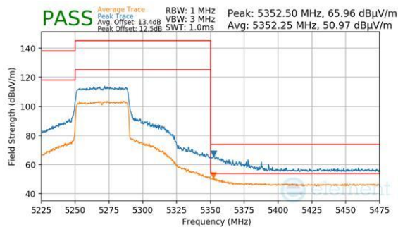
Plot 7-198. Antenna WF5B (Peak & Average, Ch.54, 802.11be(SU), MCS11)
