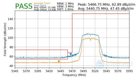
Plot 7-255. Antenna WF8 (Peak & Average, Ch.102, 802.11n, MCS7)
