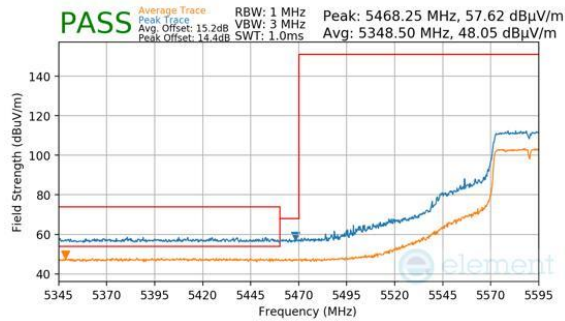
Plot 7-191. Antenna WF5B (Peak & Average, Ch.118 (FCC ONLY), 802.11n, MCS7)
