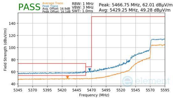
Plot 7-337. Antenna WF7 (Peak & Average, Ch.118 (FCC ONLY), 802.11be(SU), MCS11)
