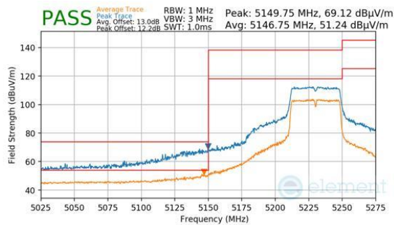
Plot 7-252. Antenna WF8 (Peak & Average, Ch.46, 802.11n, MCS7)
