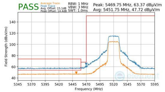
Plot 7-245. Antenna WF8 (Peak & Average, Ch.104, 802.11be(SU), MCS11)
