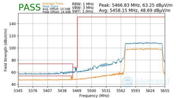
Plot 7-217. Antenna WF5B (Peak & Average, Ch.122 (FCC ONLY), 802.11be(SU), MCS11)
