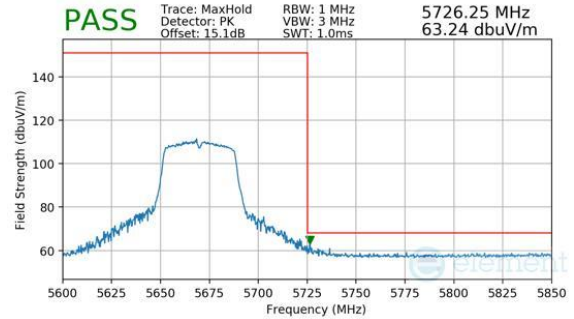
Plot 7-260. Antenna WF8 (Peak, Ch.134, 802.11n, MCS7)
