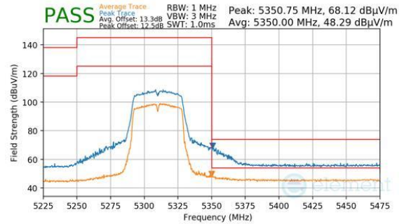
Plot 7-188. Antenna WF5B (Peak & Average, Ch.62, 802.11n, MCS7)
