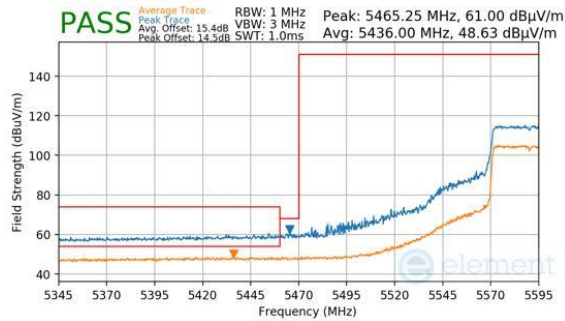
Plot 7-269. Antenna WF8 (Peak & Average, Ch.118 (FCC ONLY), 802.11be(SU), MCS11)
