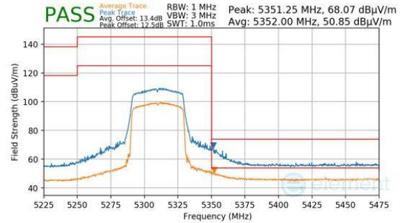
Plot 7-266. Antenna WF8 (Peak & Average, Ch.62, 802.11be(SU), MCS11)
