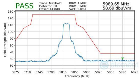
Plot 7-239. Antenna WF8 (Peak, Ch.165, 802.11n, MCS7)
