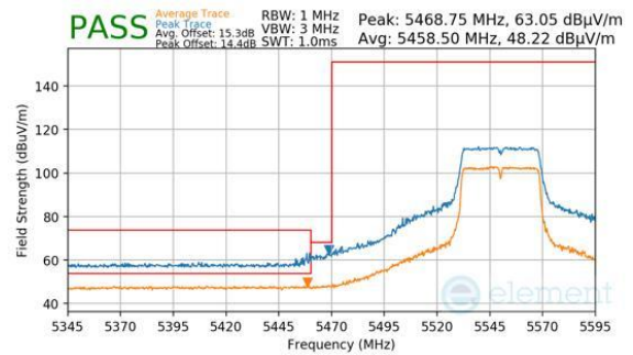
Plot 7-190. Antenna WF5B (Peak & Average, Ch.110, 802.11n, MCS7)
