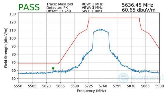
Plot 7-273. Antenna WF8 (Peak, Ch.151, 802.11be(SU), MCS11)
