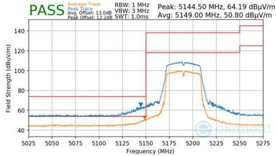
Plot 7-251. Antenna WF8 (Peak & Average, Ch.38, 802.11n, MCS7)
