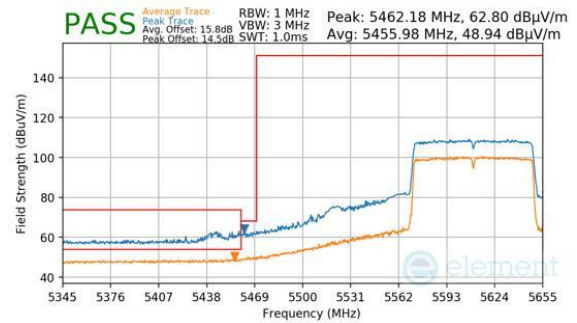
Plot 7-210. Antenna WF5B (Peak & Average, Ch.122 (FCC ONLY), 802.11ac, MCS9)
