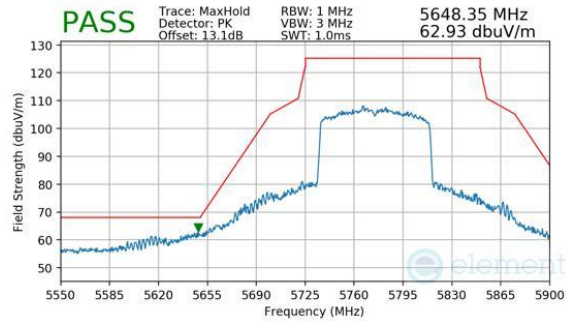
Plot 7-219. Antenna WF5B (Peak, Ch.155, 802.11be(SU), MCS11)
