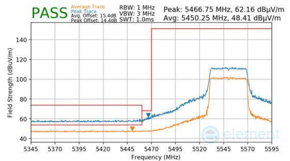
Plot 7-201. Antenna WF5B (Peak & Average, Ch.110, 802.11be(SU), MCS11)
