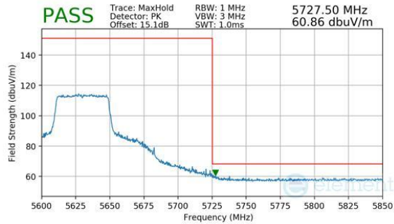
Plot 7-203. Antenna WF5B (Peak, Ch.126 (FCC ONLY), 802.11be(SU), MCS11)
