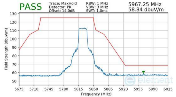
Plot 7-250. Antenna WF8 (Peak, Ch.165, 802.11be(SU), MCS11)
