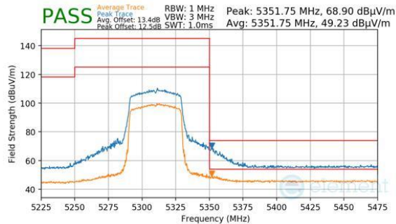
Plot 7-199. Antenna WF5B (Peak & Average, Ch.62, 802.11be(SU), MCS11)
