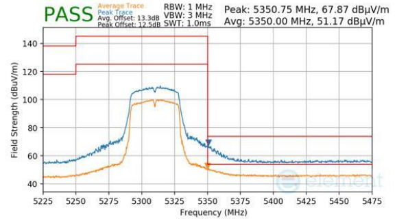
Plot 7-254. Antenna WF8 (Peak & Average, Ch.62, 802.11n, MCS7)
