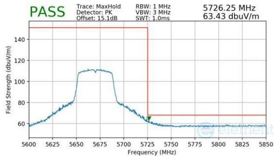
Plot 7-193. Antenna WF5B (Peak, Ch.134, 802.11n, MCS7)
