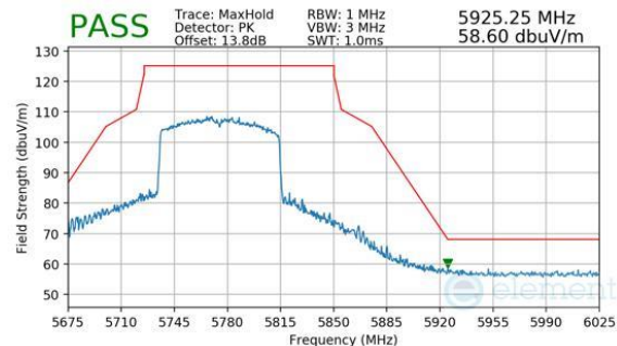
Plot 7-356. Antenna WF7 (Peak, Ch.155, 802.11be(SU), MCS11)
