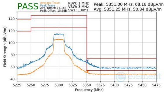
Plot 7-299. Antenna WF7 (Peak & Average, Ch.60, 802.11n, MCS7)
