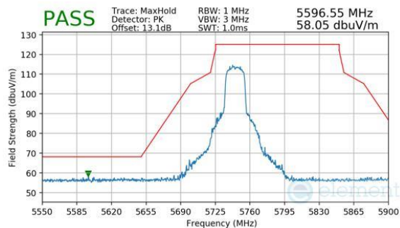
Plot 7-317. Antenna WF7 (Peak, Ch.149, 802.11be(SU), MCS11)
