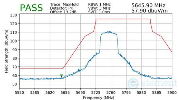
Plot 7-341. Antenna WF7 (Peak, Ch.151, 802.11be(SU), MCS11)
