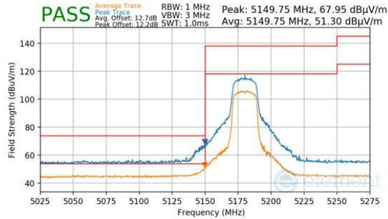
Plot 7-229. Antenna WF8 (Peak & Average, Ch.36, 802.11n, MCS7)
