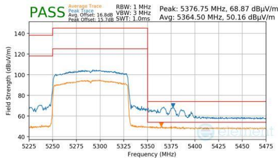
Plot 7-351. Antenna WF7 (Peak & Average, Ch.58, 802.11be(SU), MCS11)
