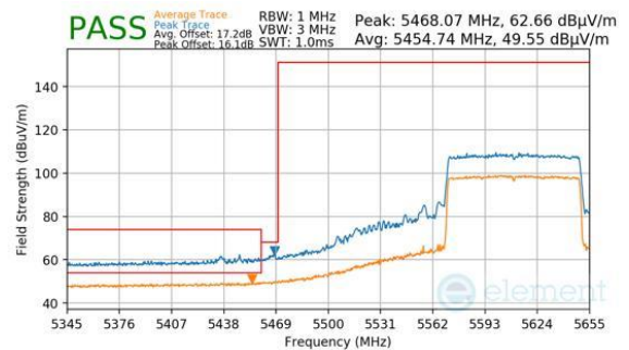
Plot 7-353. Antenna WF7 (Peak & Average, Ch.122 (FCC ONLY), 802.11be(SU), MCS11)
