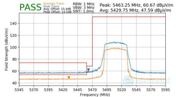
Plot 7-267. Antenna WF8 (Peak & Average, Ch.102, 802.11be(SU), MCS11)
