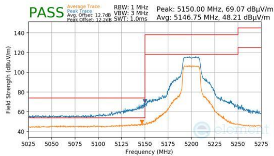
Plot 7-230. Antenna WF8 (Peak & Average, Ch.40, 802.11n, MCS7)
