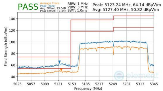
Plot 7-225. Antenna WF5B (Peak & Average, Ch.50, 802.11be(SU), MCS11)
