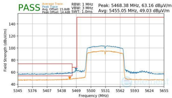
Plot 7-209. Antenna WF5B (Peak & Average, Ch.106, 802.11ac, MCS9)
