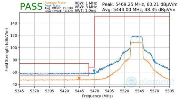
Plot 7-246. Antenna WF8 (Peak & Average, Ch.108, 802.11be(SU), MCS11)
