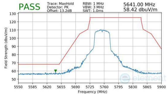
Plot 7-261. Antenna WF8 (Peak, Ch.151, 802.11n, MCS7)
