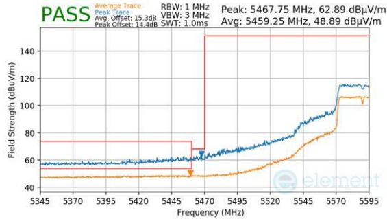
Plot 7-257. Antenna WF8 (Peak & Average, Ch.118 (FCC ONLY), 802.11n, MCS7)
