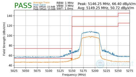
Plot 7-331. Antenna WF7 (Peak & Average, Ch.38, 802.11be(SU), MCS11)
