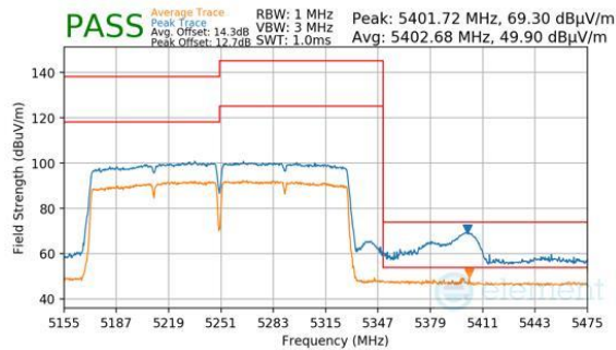
Plot 7-222. Antenna WF5B (Peak & Average, Ch.50, 802.11ac, MCS9)
