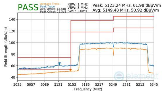
Plot 7-293. Antenna WF8 (Peak & Average, Ch.50, 802.11be(SU), MCS11)
