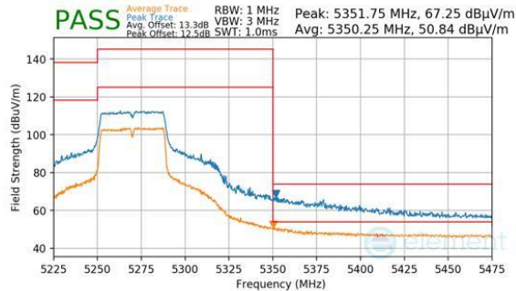
Plot 7-253. Antenna WF8 (Peak & Average, Ch.54, 802.11n, MCS7)
