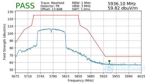
Plot 7-349. Antenna WF7 (Peak, Ch.155, 802.11ac, MCS9)
