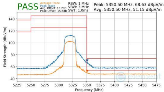
Plot 7-311. Antenna WF7 (Peak & Average, Ch.64, 802.11be(SU), MCS11)
