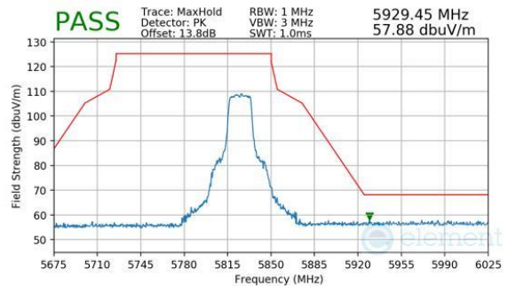
Plot 7-307. Antenna WF7 (Peak, Ch.165, 802.11n, MCS7)
