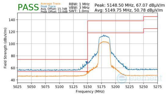
Plot 7-308. Antenna WF7 (Peak & Average, Ch.36, 802.11be(SU), MCS11)
