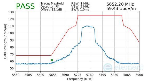
Plot 7-329. Antenna WF7 (Peak, Ch.151, 802.11n, MCS7)
