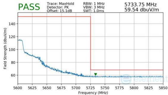
Plot 7-258. Antenna WF8 (Peak, Ch.118 (FCC ONLY), 802.11n, MCS7)
