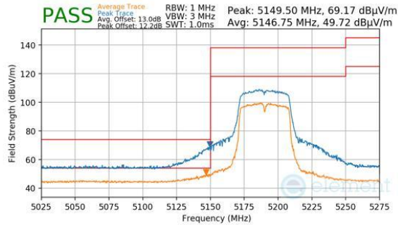
Plot 7-185. Antenna WF5B (Peak & Average, Ch.38, 802.11n, MCS7)
