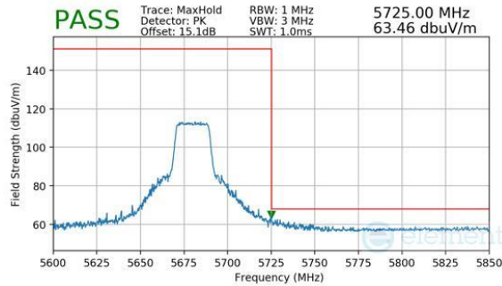
Plot 7-247. Antenna WF8 (Peak, Ch.136, 802.11be(SU), MCS11)
