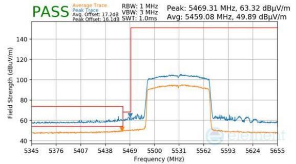
Plot 7-352. Antenna WF7 (Peak & Average, Ch.106, 802.11be(SU), MCS11)
