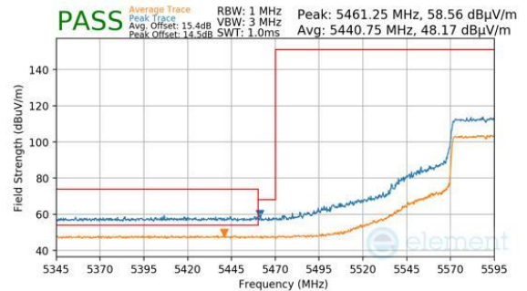
Plot 7-202. Antenna WF5B (Peak & Average, Ch.118 (FCC ONLY), 802.11be(SU), MCS11)
