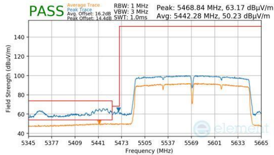
Plot 7-223. Antenna WF5B (Peak & Average, Ch.114 (FCC ONLY), 802.11ac, MCS9)
