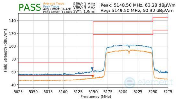
Plot 7-343. Antenna WF7 (Peak & Average, Ch.42, 802.11ac, MCS9)
