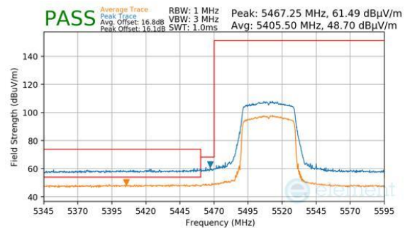
Plot 7-335. Antenna WF7 (Peak & Average, Ch.102, 802.11be(SU), MCS11)
