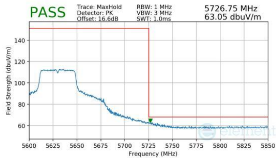
Plot 7-327. Antenna WF7 (Peak, Ch.126 (FCC ONLY), 802.11n, MCS7)
