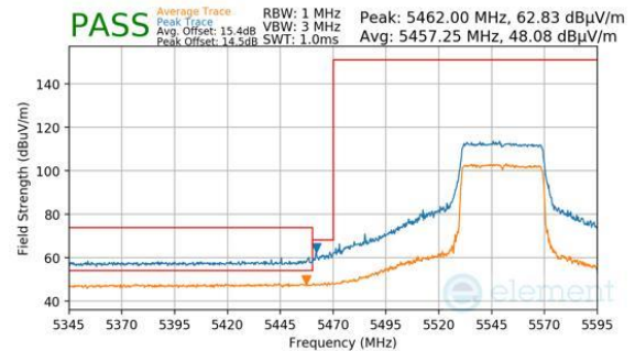
Plot 7-268. Antenna WF8 (Peak & Average, Ch.110, 802.11be(SU), MCS11)
