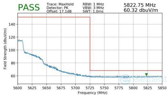
Plot 7-338. Antenna WF7 (Peak, Ch.118 (FCC ONLY), 802.11be(SU), MCS11)
