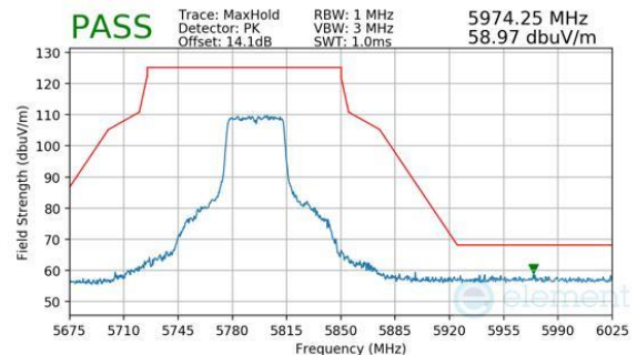
Plot 7-262. Antenna WF8 (Peak, Ch.159, 802.11n, MCS7)
