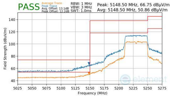
Plot 7-197. Antenna WF5B (Peak & Average, Ch.46, 802.11be(SU), MCS11)
