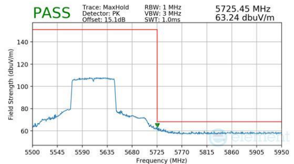
Plot 7-211. Antenna WF5B (Peak, Ch.122 (FCC ONLY), 802.11ac, MCS9)
