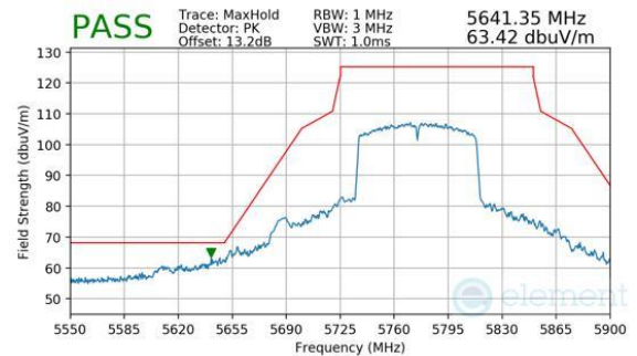
Plot 7-212. Antenna WF5B (Peak, Ch.155, 802.11ac, MCS9)
