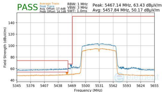
Plot 7-345. Antenna WF7 (Peak & Average, Ch.106, 802.11ac, MCS9)
