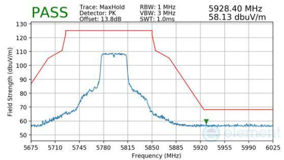
Plot 7-330. Antenna WF7 (Peak, Ch.159, 802.11n, MCS7)
