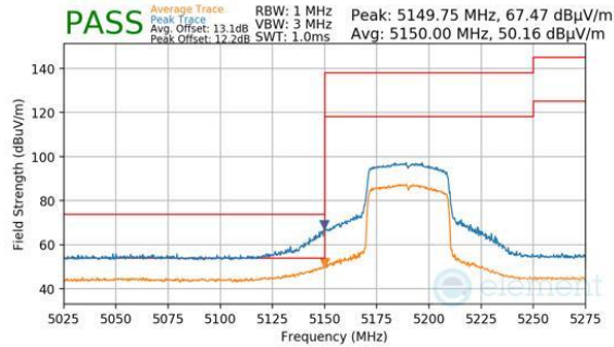
Plot 7-263. Antenna WF8 (Peak & Average, Ch.38, 802.11be(SU), MCS11)
