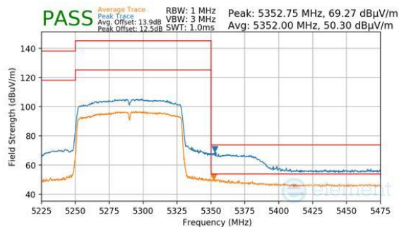
Plot 7-208. Antenna WF5B (Peak & Average, Ch.58, 802.11ac, MCS9)
