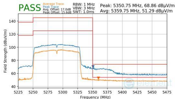
Plot 7-344. Antenna WF7 (Peak & Average, Ch.58, 802.11ac, MCS9)
