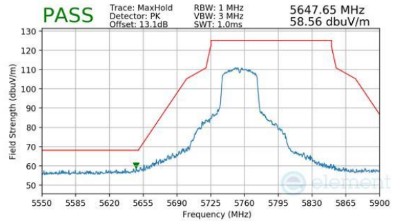
Plot 7-194. Antenna WF5B (Peak, Ch.151, 802.11n, MCS7)
