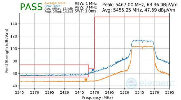
Plot 7-256. Antenna WF8 (Peak & Average, Ch.110, 802.11n, MCS7)
