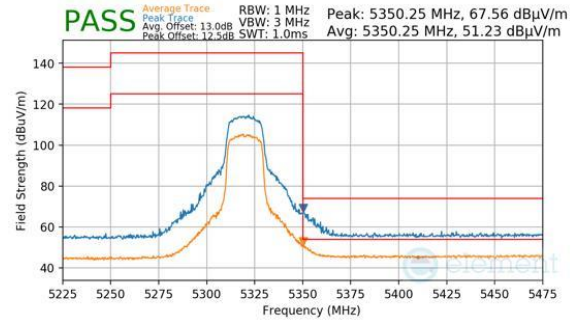
Plot 7-232. Antenna WF8 (Peak & Average, Ch.64, 802.11n, MCS7)
