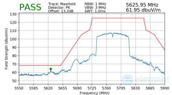
Plot 7-280. Antenna WF8 (Peak, Ch.155, 802.11ac, MCS9)
