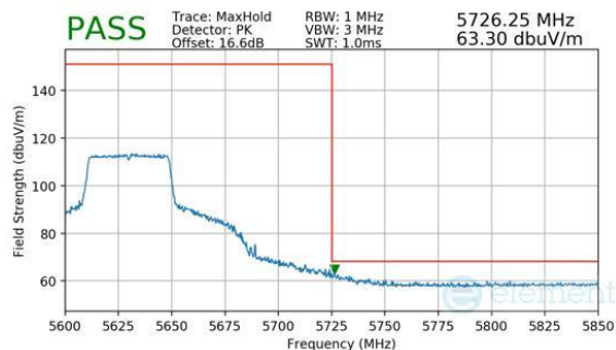
Plot 7-339. Antenna WF7 (Peak, Ch.126 (FCC ONLY), 802.11be(SU), MCS11)
