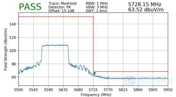
Plot 7-218. Antenna WF5B (Peak, Ch.122 (FCC ONLY), 802.11be(SU), MCS11)
