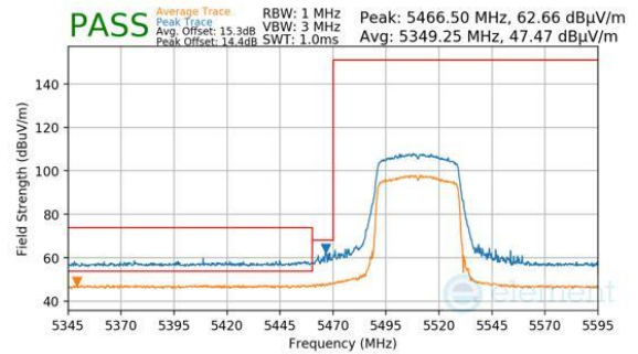
Plot 7-200. Antenna WF5B (Peak & Average, Ch.102, 802.11be(SU), MCS11)
