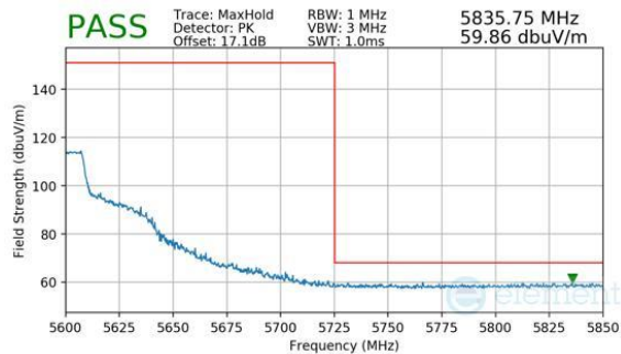
Plot 7-326. Antenna WF7 (Peak, Ch.118 (FCC ONLY), 802.11n, MCS7)
