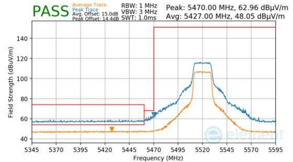
Plot 7-234. Antenna WF8 (Peak & Average, Ch.104, 802.11n, MCS7)
