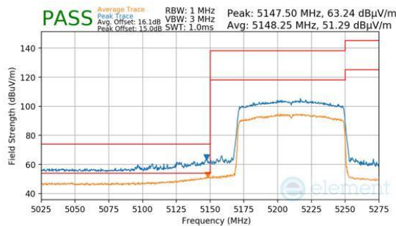
Plot 7-350. Antenna WF7 (Peak & Average, Ch.42, 802.11be(SU), MCS11)
