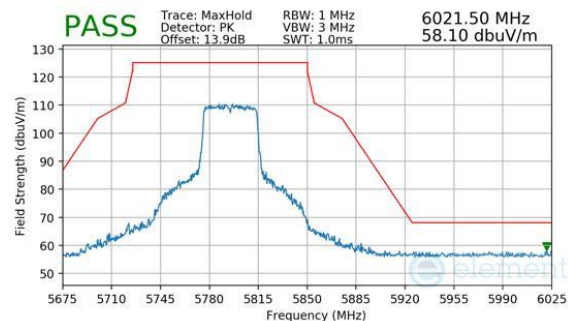
Plot 7-342. Antenna WF7 (Peak, Ch.159, 802.11be(SU), MCS11)
