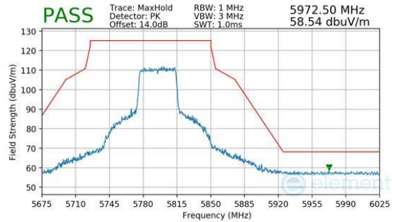
Plot 7-206. Antenna WF5B (Peak, Ch.159, 802.11be(SU), MCS11)
